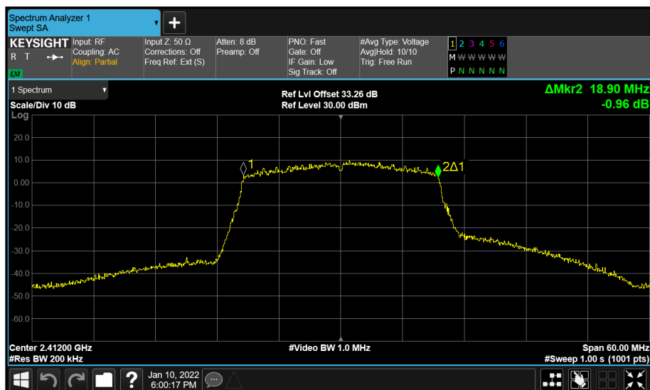
Figure 71 - Core 1 (B) 2412 MHz (CH1) 99% Bandwidth
