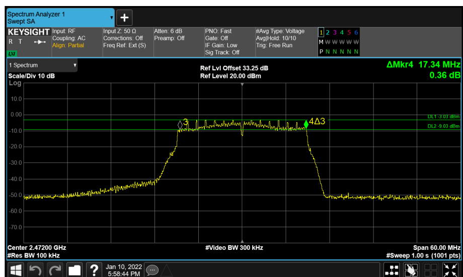
Figure 62 - Core 1 (B) 2472 MHz (CH13) 6 dB Bandwidth
