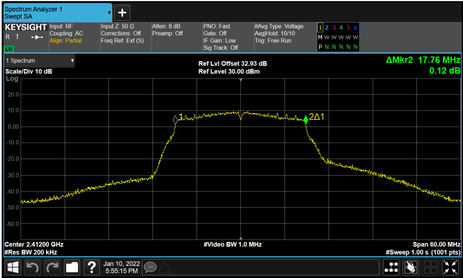
Figure 51 - Core 0 (A) 2412 MHz (CH1) 99% Bandwidth
