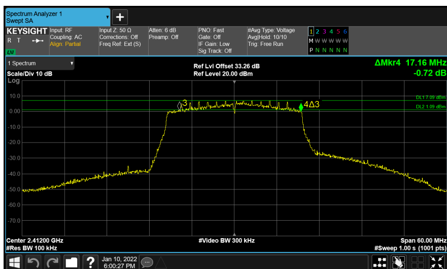
Figure 72 - Core 1 (B) 2412 MHz (CH1) 6 dB Bandwidth
