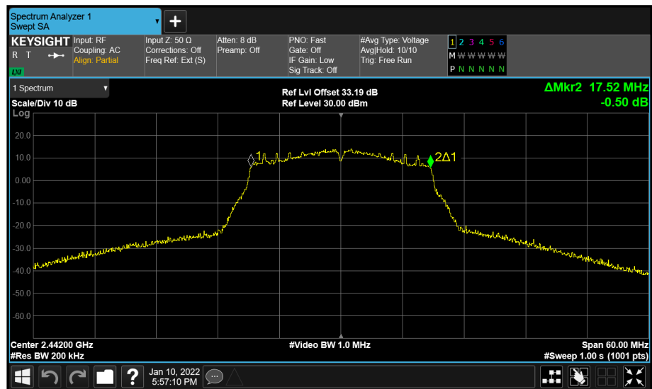
Figure 57 - Core 1 (B) 2442 MHz (CH7) 99% Bandwidth
