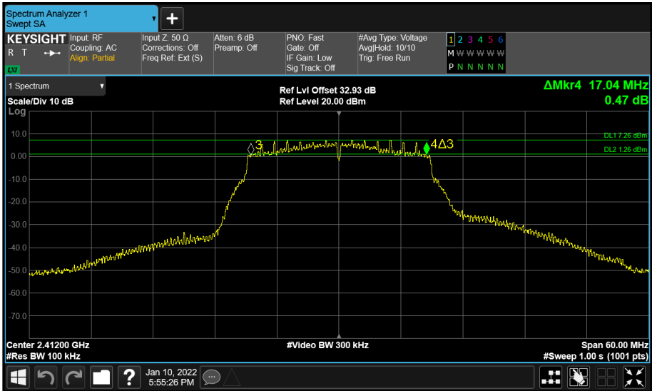
Figure 52 - Core 0 (A) 2412 MHz (CH1) 6 dB Bandwidth
