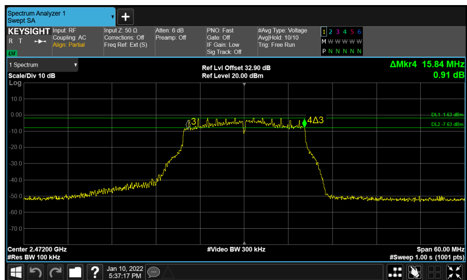
Figure 44 - Core 0 (A) 2472 MHz (CH13) 6 dB Bandwidth
