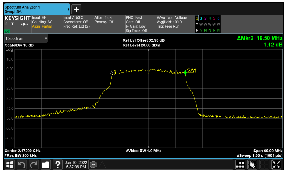
Figure 43 - Core 0 (A) 2472 MHz (CH13) 99% Bandwidth
