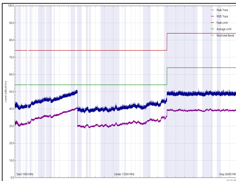
Figure 159 - 2476 MHz (CH74), HDR4, iPA, Core 2, 1 GHz to 26 GHz, Horizontal
