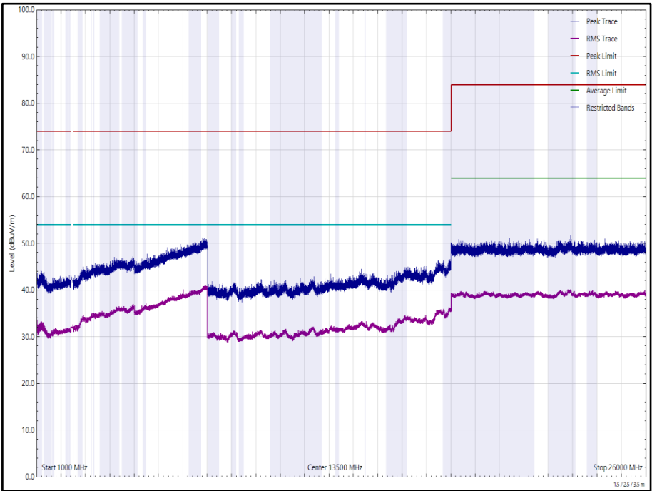
Figure 261 - 2440 MHz (CH17), LE1M, ePA, Core 0 + Core 1, 1 GHz to 26 GHz, Horizontal
