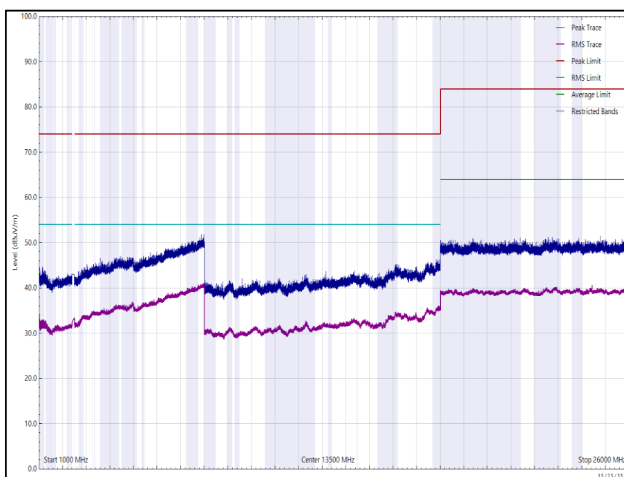
Figure 265 - 2480 MHz (CH39), LE1M, ePA, Core 0 + Core 1, 1 GHz to 26 GHz, Vertical
