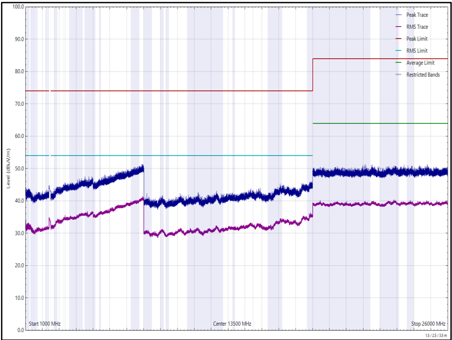
Figure 263 - 2440 MHz (CH17), LE1M, ePA, Core 0 + Core 1, 1 GHz to 26 GHz, Vertical
