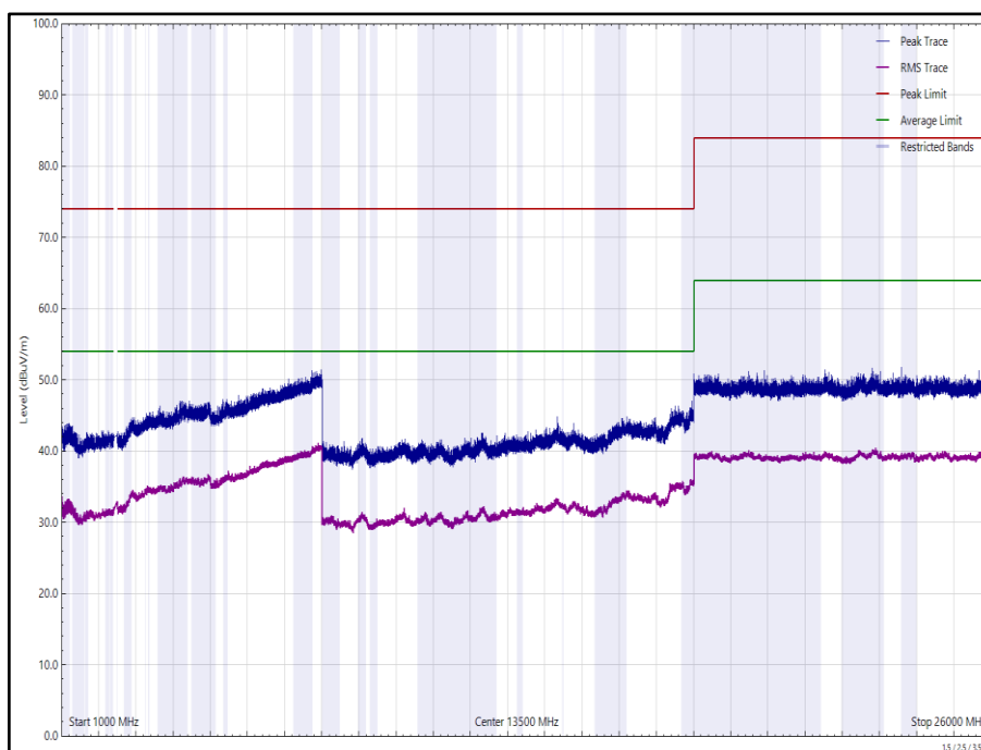
Figure 151 - 2476 MHz (CH74), HDR4, iPA, Core 0 + Core 1, 1 GHz to 26 GHz, Horizontal
