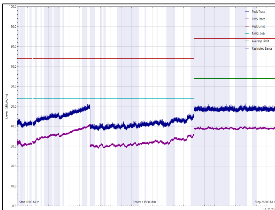
Figure 264 - 2480 MHz (CH39), LE1M, ePA, Core 0 + Core 1, 1 GHz to 26 GHz, Horizontal
