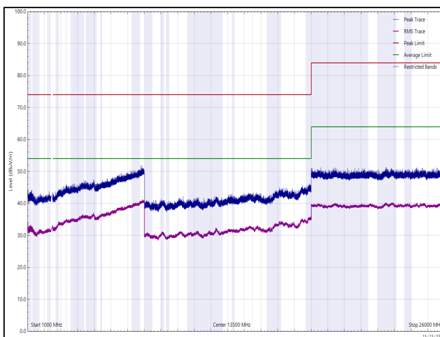
Figure 160 - 2476 MHz (CH74), HDR4, iPA, Core 2, 1 GHz to 26 GHz, Vertical
