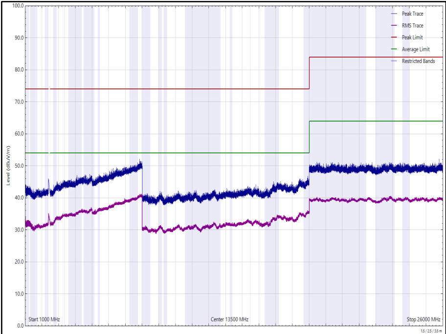
Figure 146 - 2404 MHz (CH2), HDR4, iPA, Core 0 + Core 1, 1 GHz to 26 GHz, Vertical
