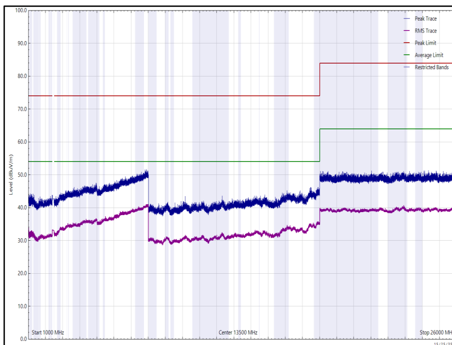
Figure 152 - 2476 MHz (CH74), HDR4, iPA, Core 0 + Core 1, 1 GHz to 26 GHz, Vertical
