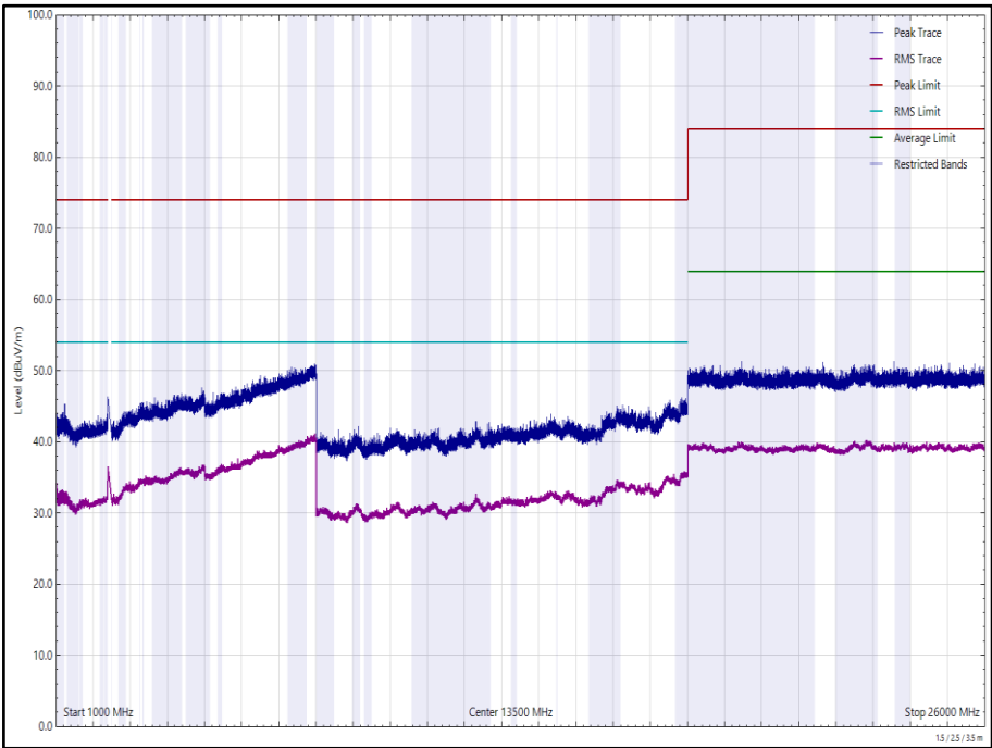
Figure 259 - 2402 MHz (CH37), LE1M, ePA, Core 0 + Core 1, 1 GHz to 26 GHz, Vertical
