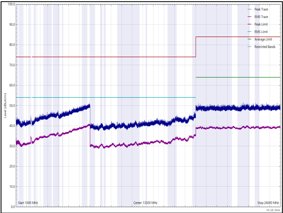
Figure 271 - 2440 MHz (CH17), LE1M, iPA, Core 0 + Core 1, 1 GHz to 26 GHz, Vertical
