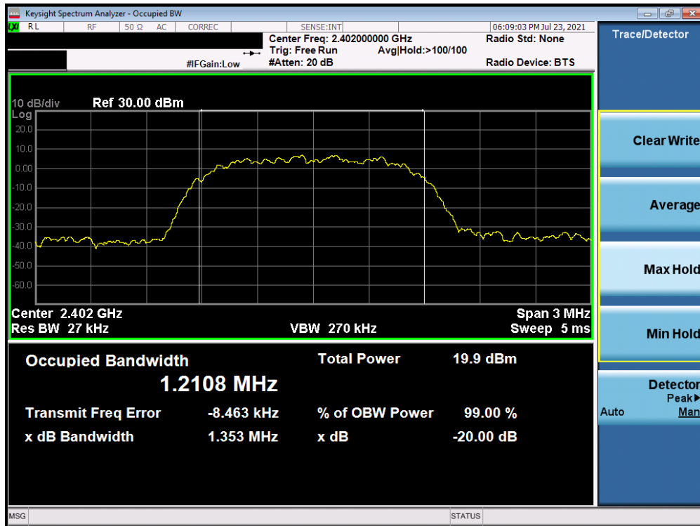
Plot 7-4. 20dB BW 99% OBW Plot Ant-A (Bluetooth, 8DPSK, ePA – Ch. 0)
