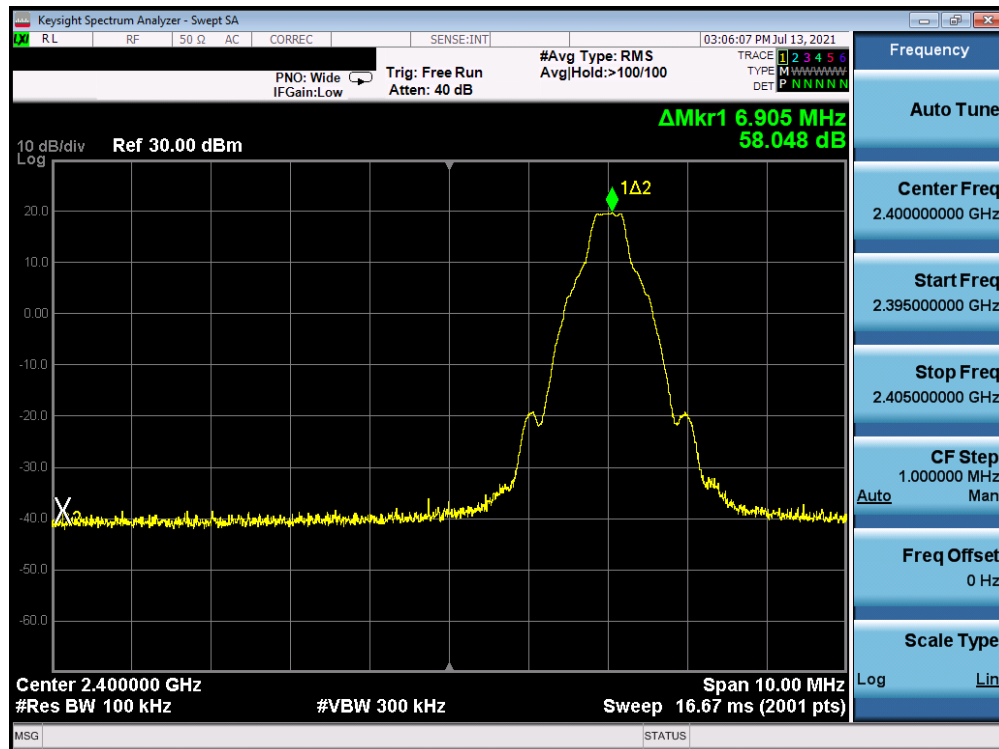
Plot 7-7. Band Edge Plot Ant-A (Bluetooth with Hopping Disabled, GFSK, ePA – Ch. 0)
