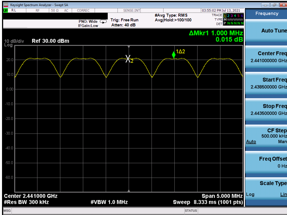
Plot 7-15. Channel Spacing Plot Ant-A (Bluetooth, GFSK, ePA)
