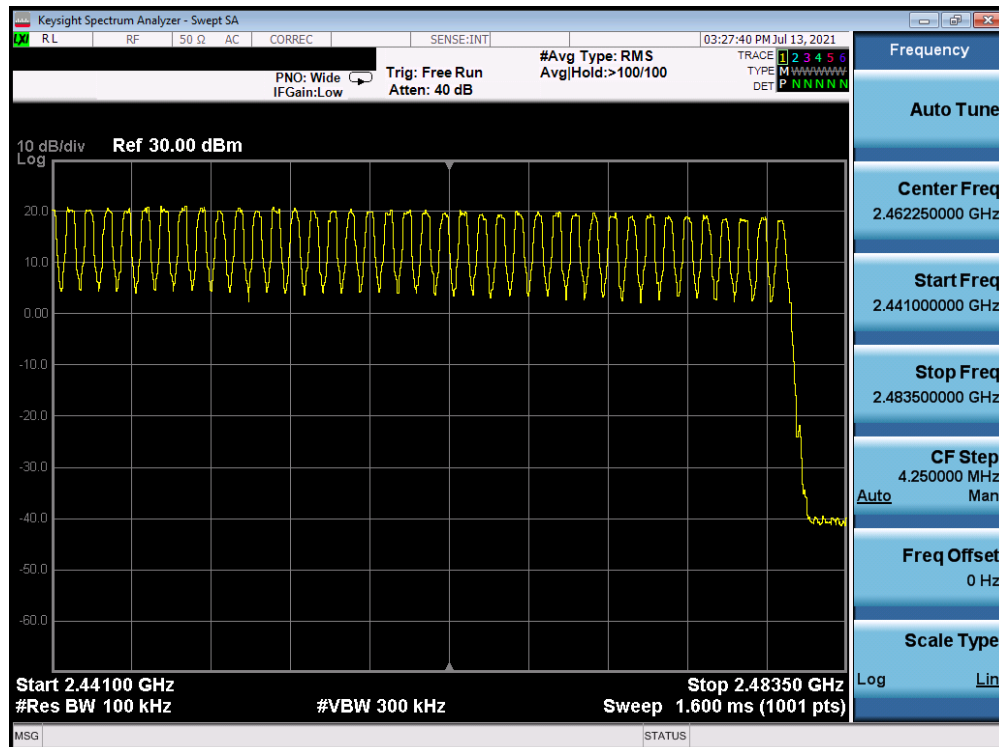
Plot 7-20. High End Spectrum Channel Hopping Plot Ant-A (Bluetooth, GFSK, ePA)
