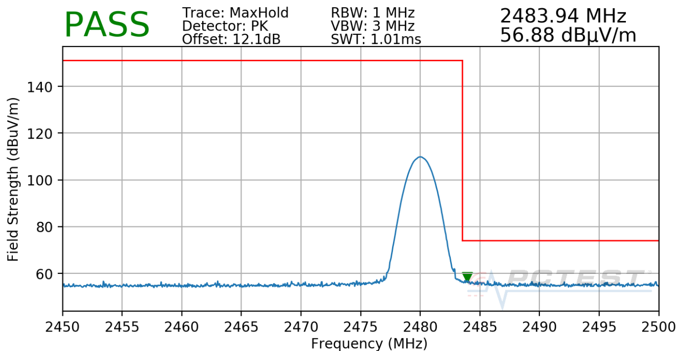
Plot 7-40. Radiated Restricted Upper Band Edge Measurement Ant-A (Peak)
