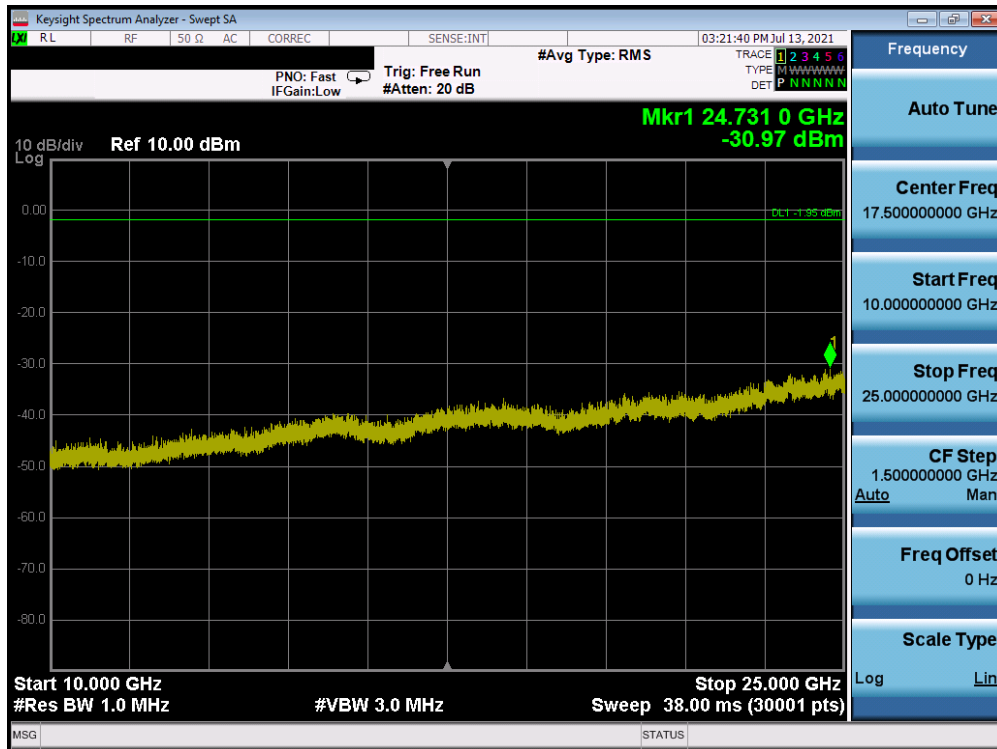
Plot 7-28. Conducted Spurious Plot Ant-A (Bluetooth, GFSK, ePA – Ch. 78)
