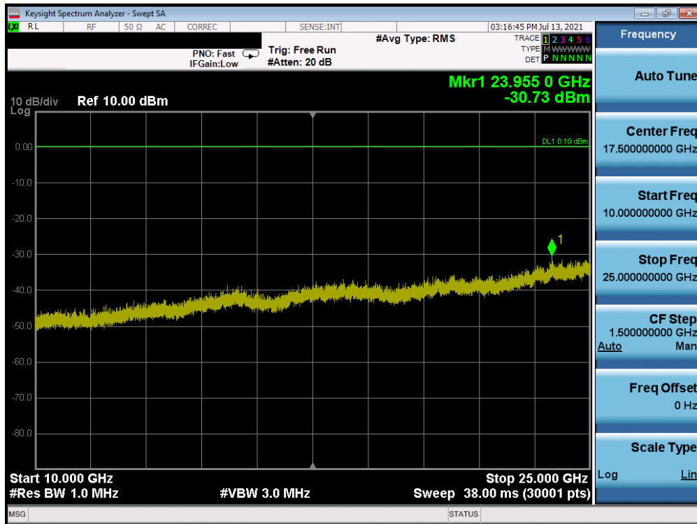
Plot 7-26. Conducted Spurious Plot Ant-A (Bluetooth, GFSK, ePA Ch. 39)
