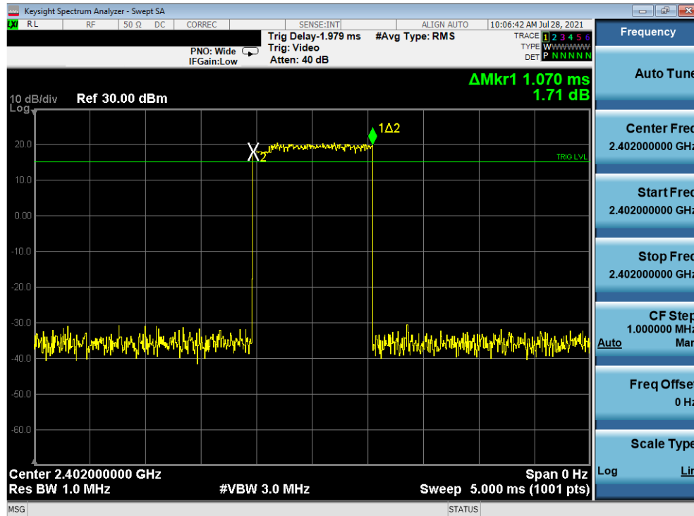
Plot 7-18. Time of Occupancy Plot Ant-A (Bluetooth, 8DPSK, ePA)
