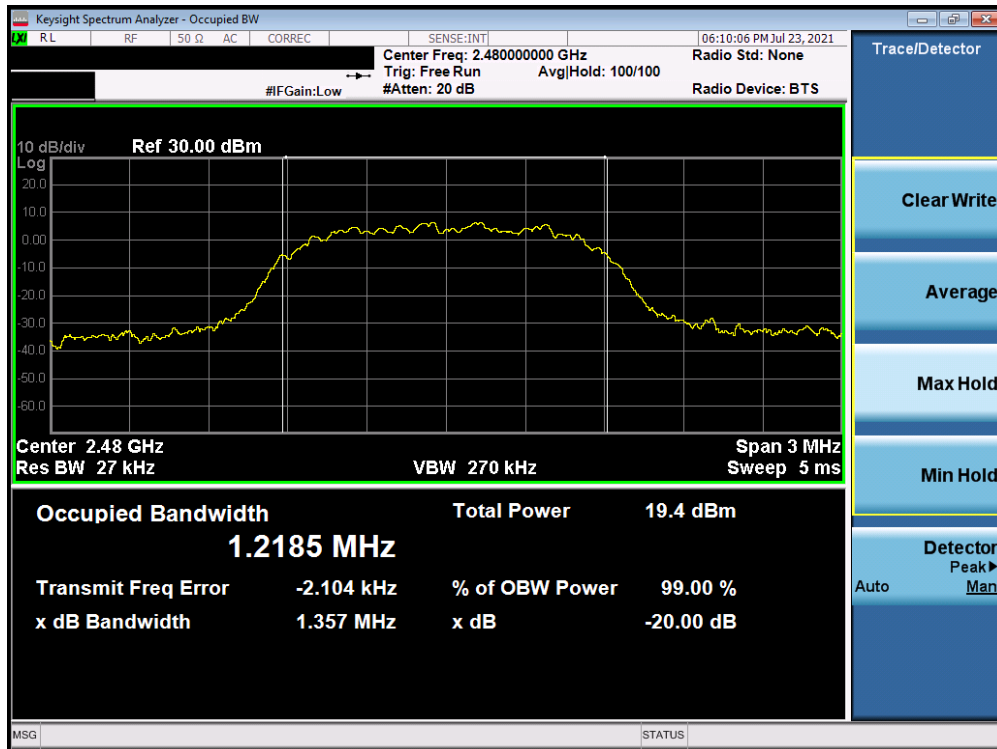
Plot 7-6. 20dB BW 99% OBW Plot Ant-A (Bluetooth, 8DPSK, ePA – Ch. 78)
