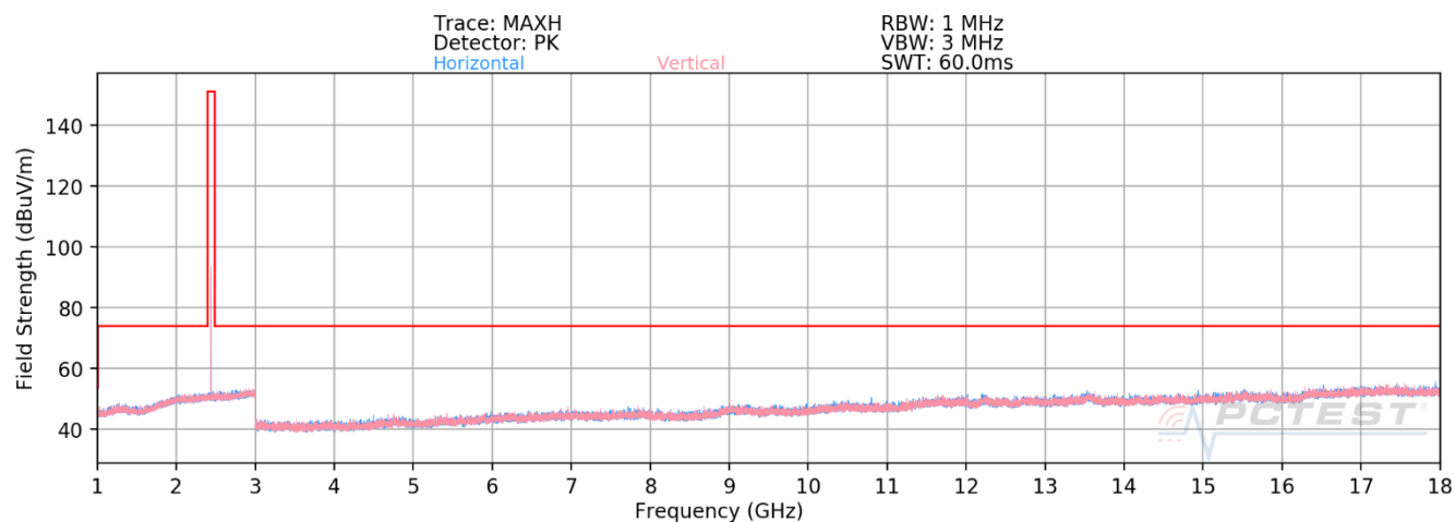
Plot 7-1: Radiated Spurious Emissions above 1GHz (BT GFSK ePA – Ch. 39)
