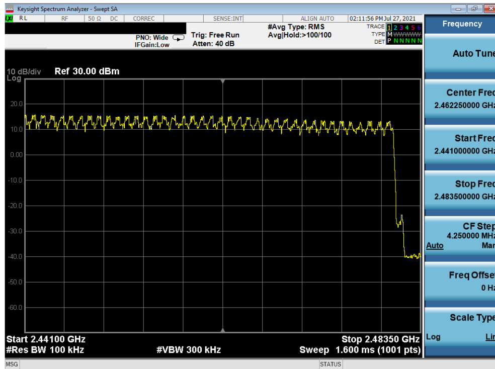
Plot 7-22. High End Spectrum Channel Hopping Plot Ant-A (Bluetooth, 8DPSK, ePA)
