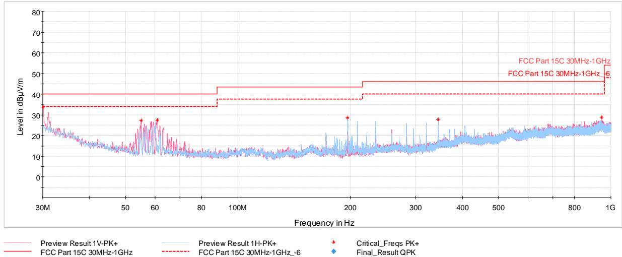
Plot 7-41. Radiated Spurious Emissions Below 1GHz Antenna A (GFSK ePA – Ch.39, with AC/DC Adapter)
