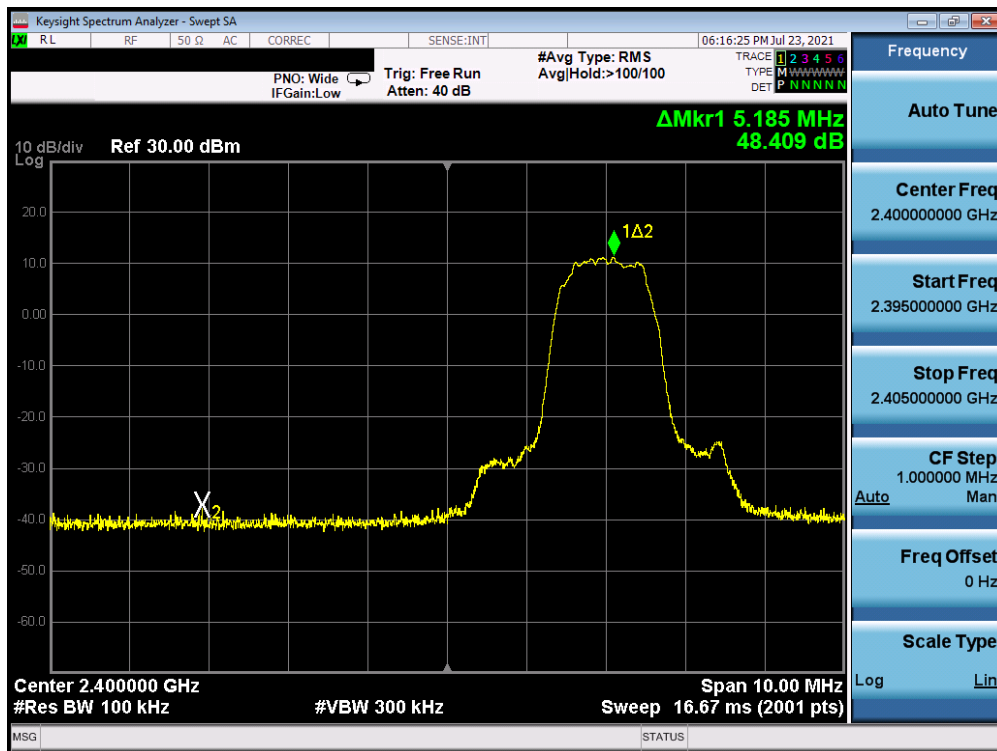
Plot 7-11. Band Edge Plot Ant-A (Bluetooth with Hopping Disabled, 8DPSK, ePA – Ch. 0)
