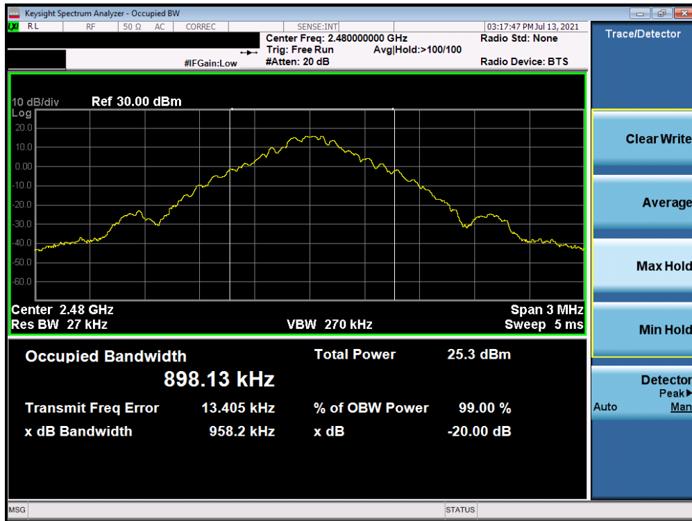
Plot 7-3. 20dB BW 99% OBW Plot Ant-A (Bluetooth, GFSK, ePA – Ch. 78)
