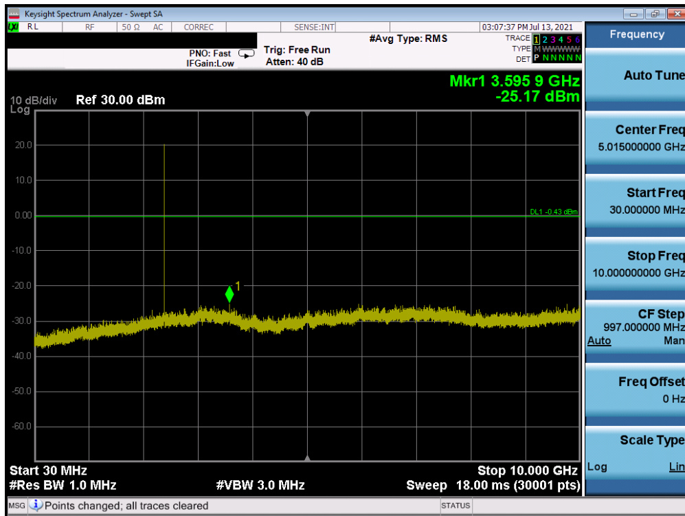
Plot 7-23. Conducted Spurious Plot Ant-A (Bluetooth, GFSK, ePA – Ch. 0)
