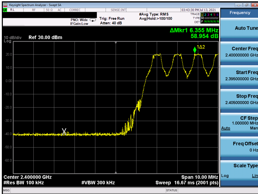
Plot 7-10. Band Edge Plot Ant-A (Bluetooth with Hopping Enabled, GFSK, ePA)
