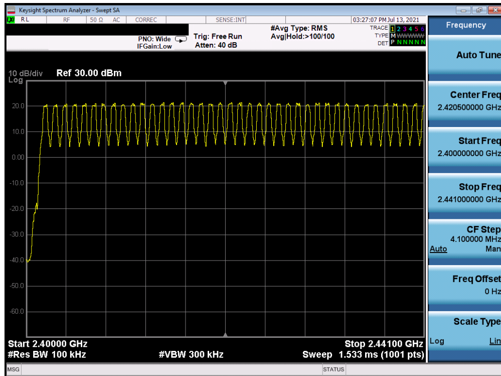
Plot 7-19. Low End Spectrum Channel Hopping Plot Ant-A (Bluetooth, GFSK, ePA)
