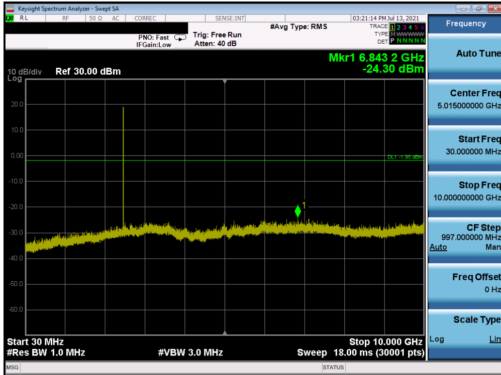
Plot 7-27. Conducted Spurious Plot Ant-A (Bluetooth, GFSK, ePA – Ch. 78)
