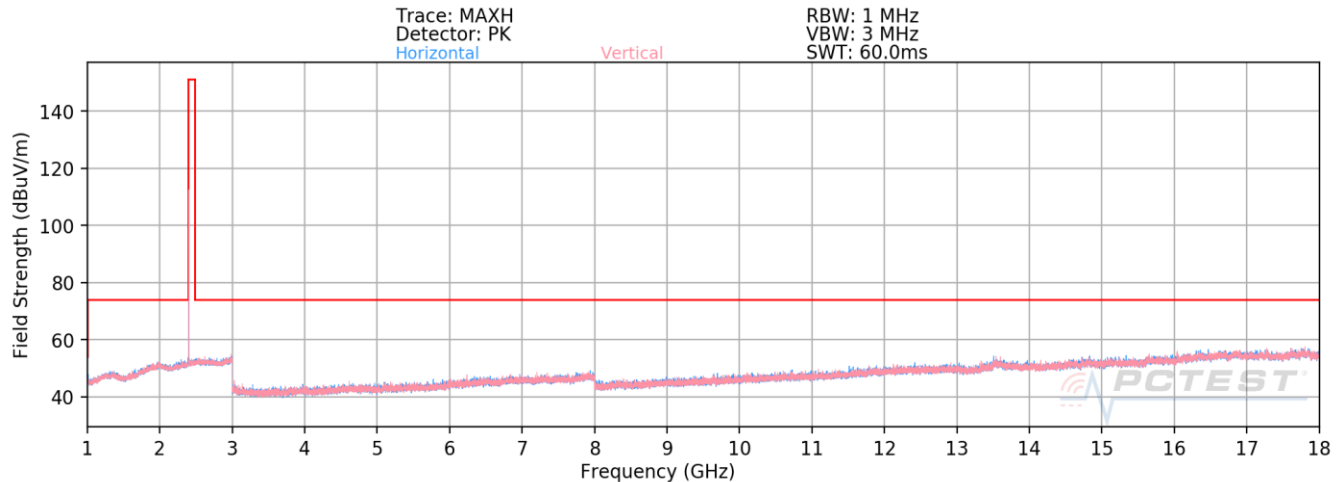
Plot 7-29. Radiated Spurious Emissions Plot above 1GHz Ant-A (BT GFSK ePA – Ch. 0)
