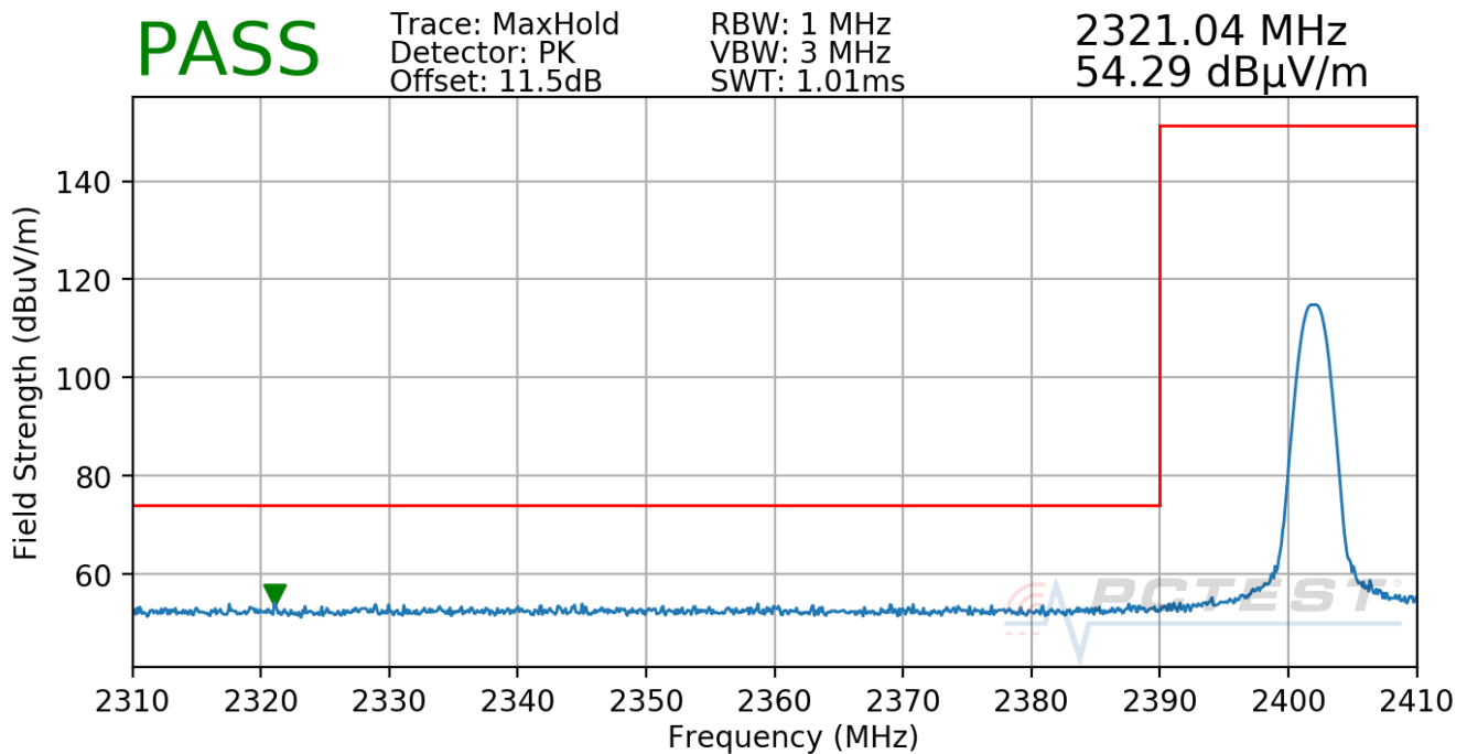
Plot 7-37. Radiated Restricted Lower Band Edge Measurement Ant-A (Peak)
