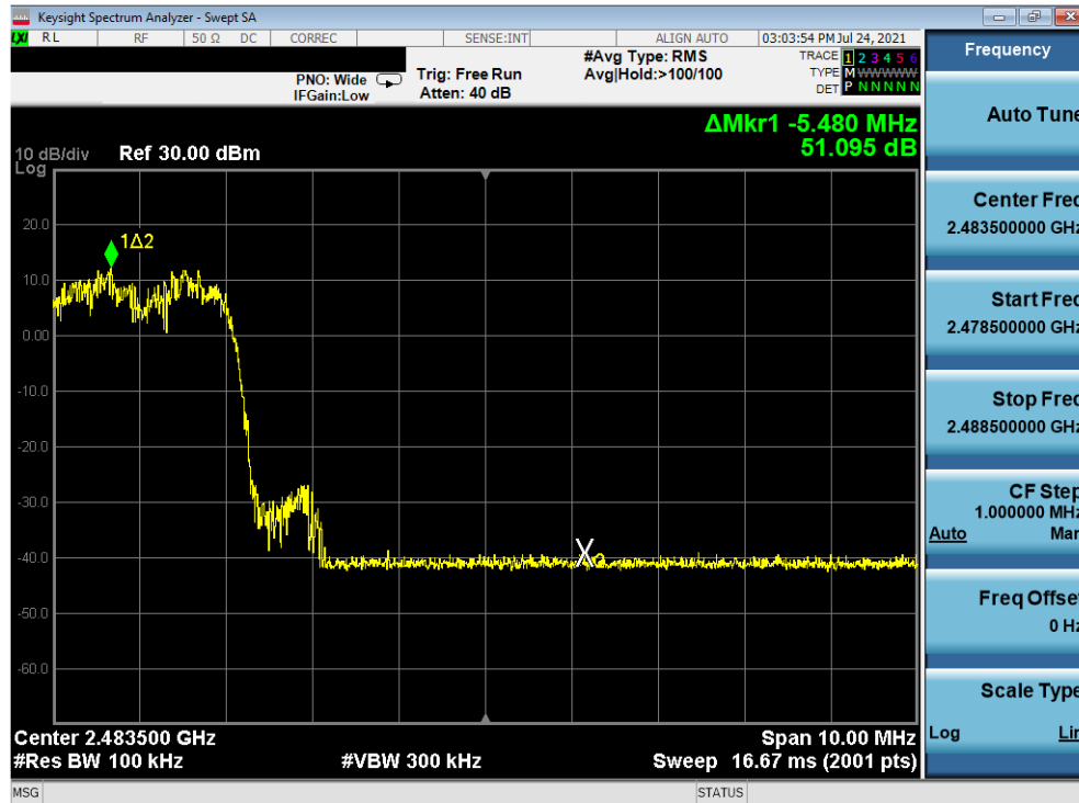
Plot 7-13. Band Edge Plot Ant-A (Bluetooth with Hopping Enabled, 8DPSK, ePA)
