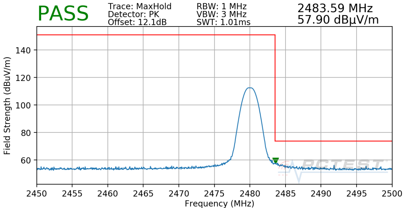
Plot 7-39. Radiated Restricted Upper Band Edge Measurement Ant-A (Peak)
