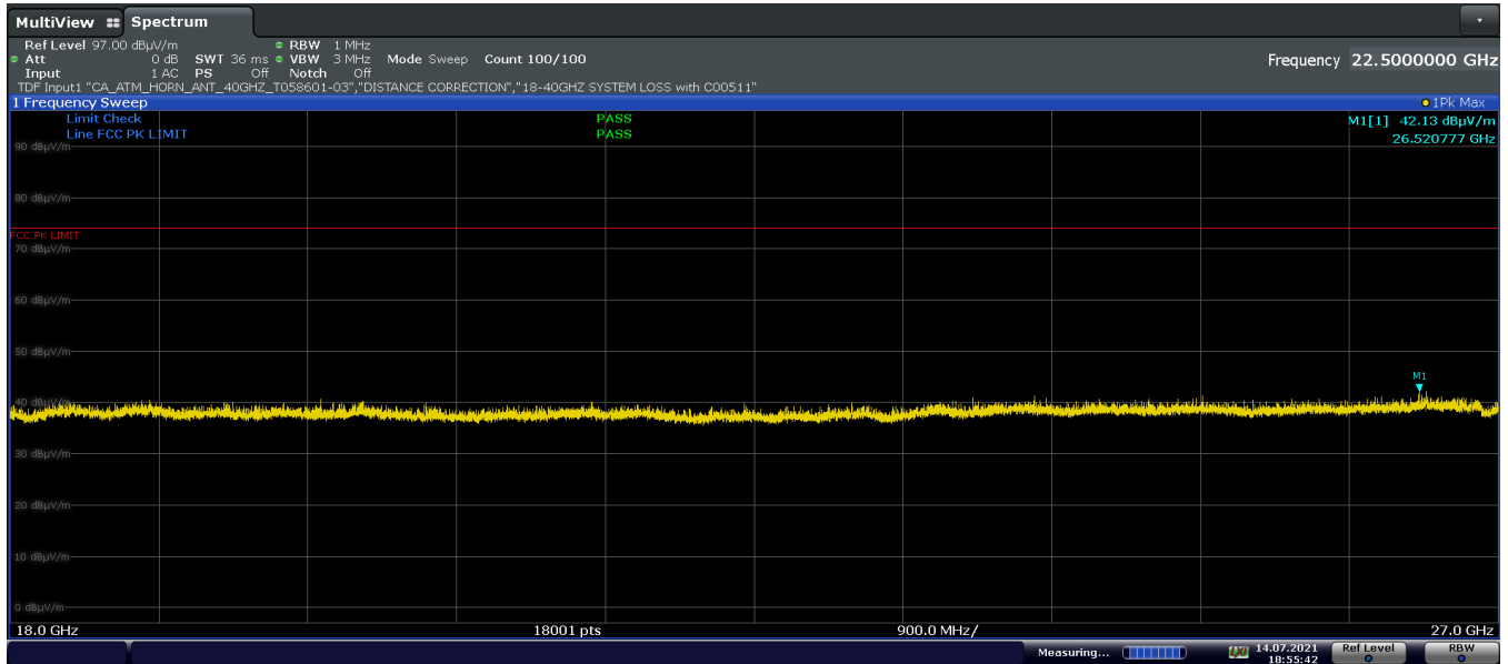
Plot 7-32. Radiated Spurious Emissions Above 18GHz Antenna A (GFSK ePA – Ch.39, Pol. H)
