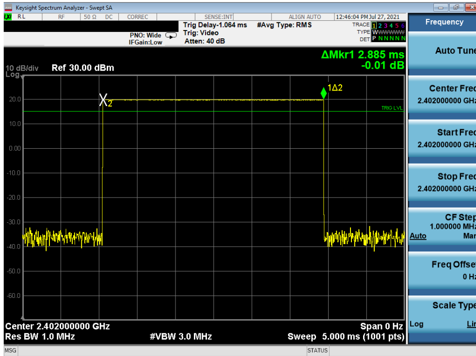
Plot 7-17. Time of Occupancy Plot Ant-A (Bluetooth, GFSK, ePA)
