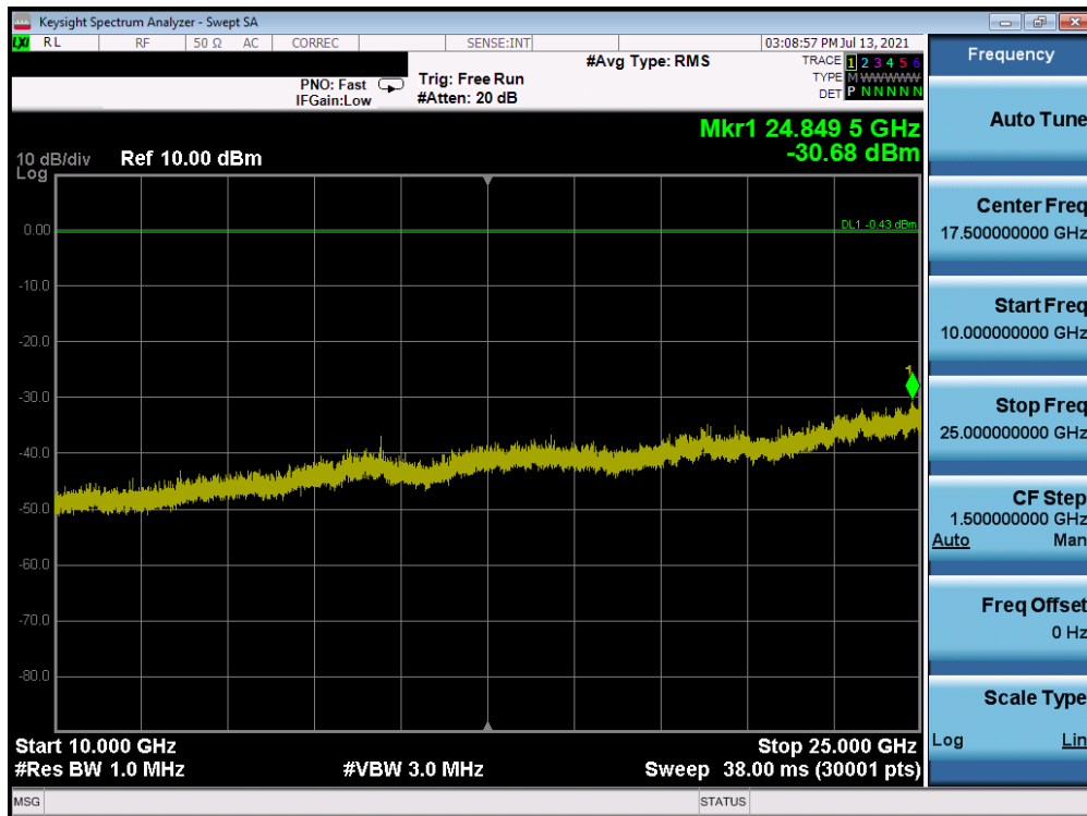
Plot 7-24. Conducted Spurious Plot Ant-A (Bluetooth, GFSK, ePA – Ch. 0)
