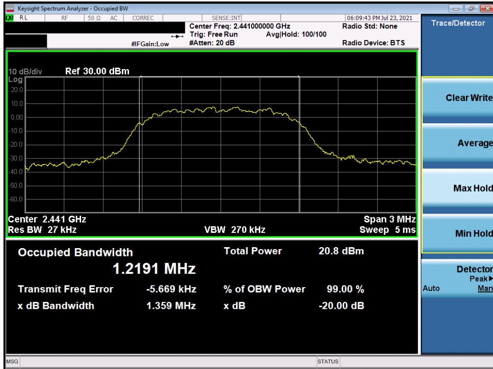
Plot 7-5. 20dB BW 99% OBW Plot Ant-A (Bluetooth, 8DPSK, ePA – Ch. 39)
