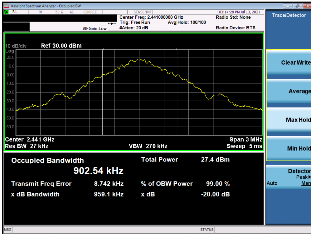
Plot 7-2. 20dB BW 99% OBW Plot Ant-A (Bluetooth, GFSK, ePA – Ch. 39)
