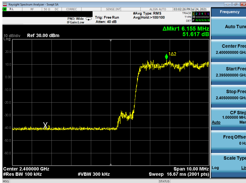
Plot 7-14. Band Edge Plot Ant-A (Bluetooth with Hopping Enabled, 8DPSK, ePA)
