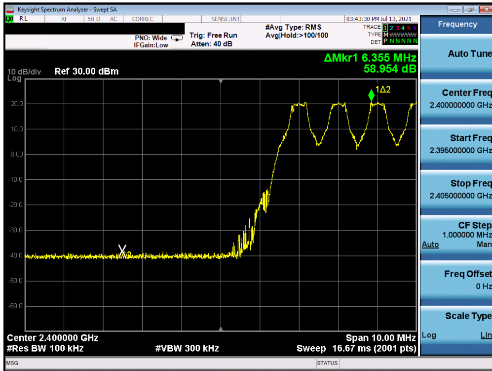
Plot 7-9. Band Edge Plot Ant-A (Bluetooth with Hopping Enabled, GFSK, ePA)
