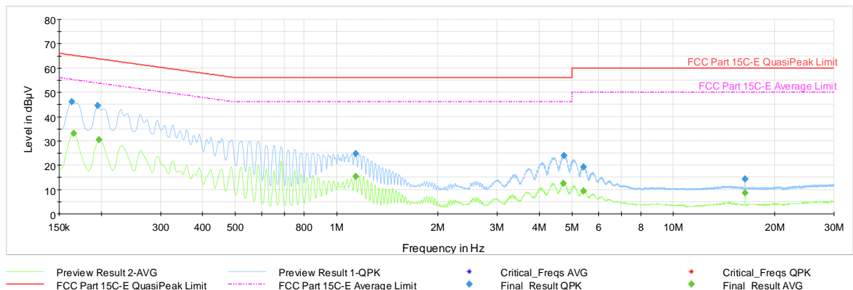
Plot 7-42. AC Line-Conducted Test Plot Antenna A (L1, GFSK ePA – Ch.39, with AC/DC Adapter)
