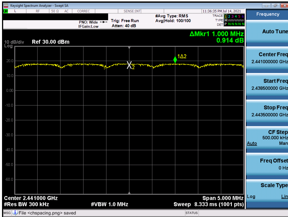
Plot 7-16. Channel Spacing Plot Ant-A (Bluetooth, 8DPSK, ePA)
