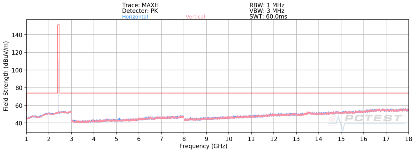
Plot 7-30. Radiated Spurious Emissions Plot above 1GHz Ant-A (BT GFSK ePA – Ch. 39)
