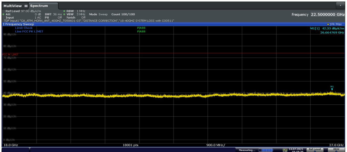
Plot 7-33. Radiated Spurious Emissions Above 18GHz Antenna A (GFSK ePA – Ch.39, Pol. V)
