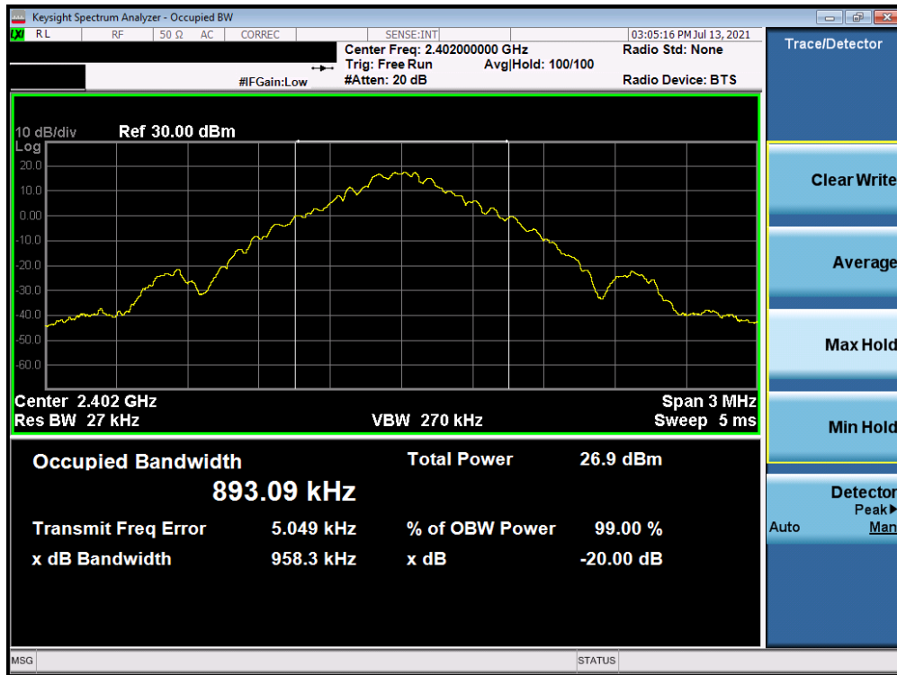
Plot 7-1. 20dB BW and 99% OBW Plot Ant-A (Bluetooth, GFSK, ePA – Ch. 0)
