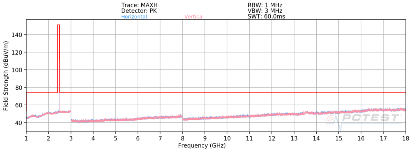
Plot 7-31. Radiated Spurious Emissions Plot above 1GHz Ant-A (BT GFSK ePA – Ch. 78)
