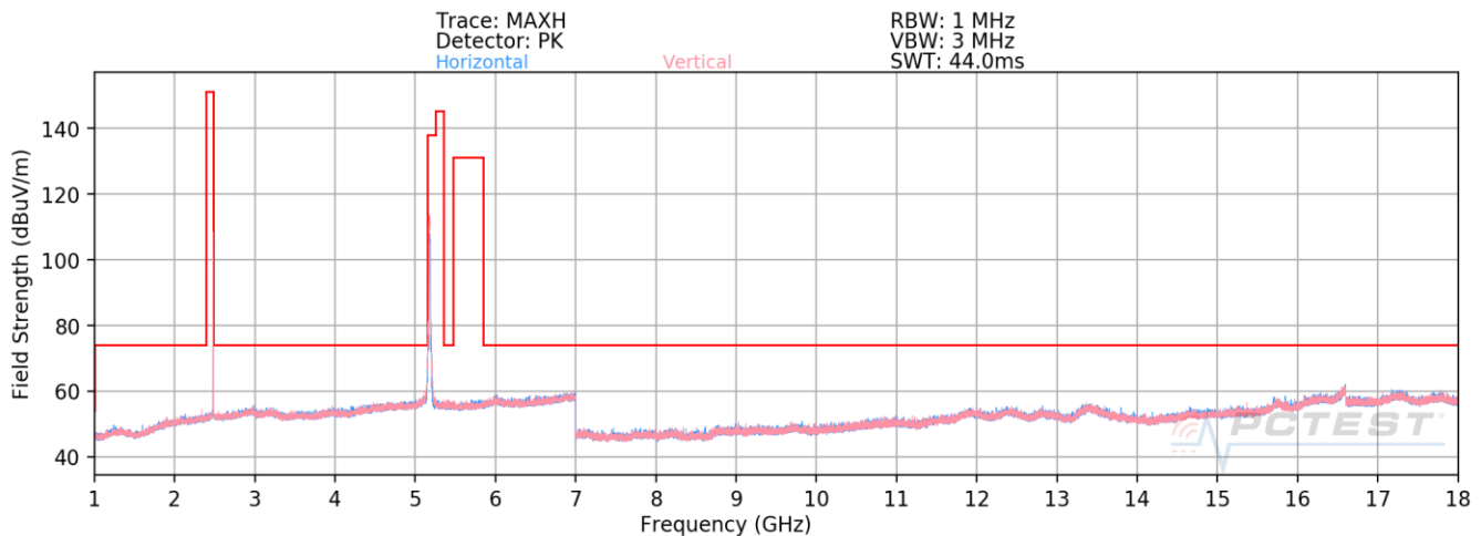
Plot 7-34. Radiated Spurious Emissions Plot above 1GHz Simultaneous Tx
