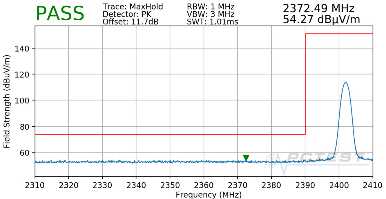
Plot 7-38. Radiated Restricted Lower Band Edge Measurement Ant-A (Peak)
