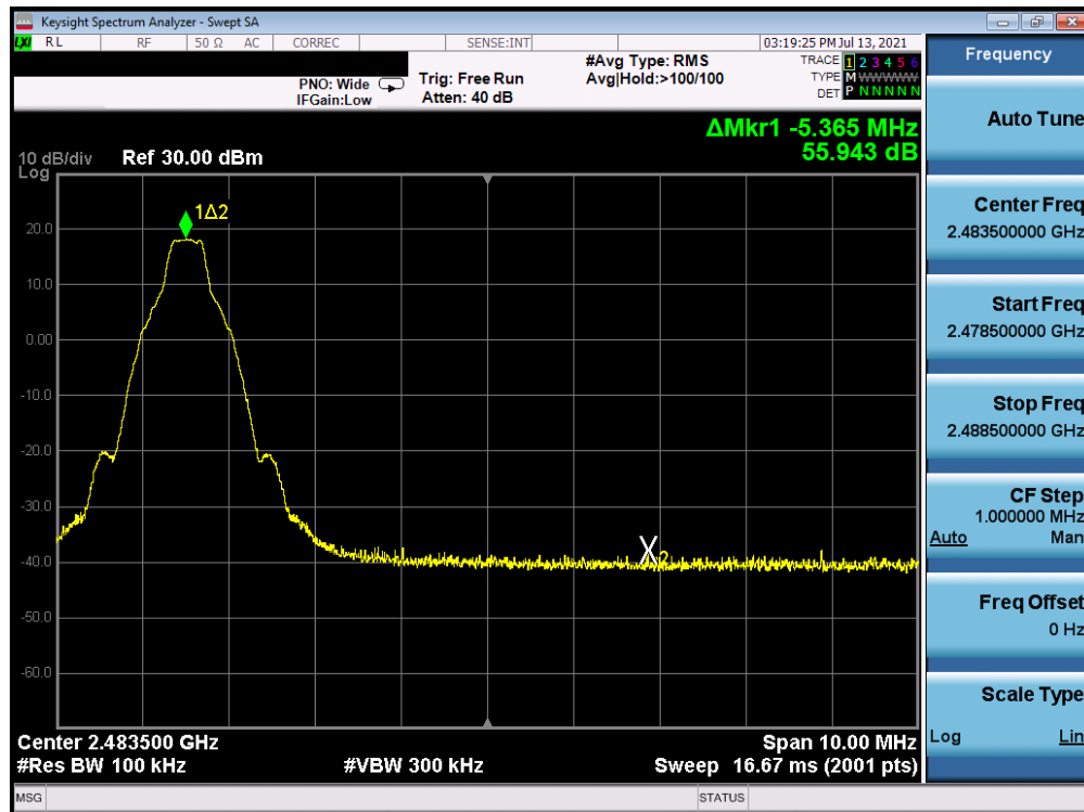
Plot 7-8. Band Edge Plot Ant-A (Bluetooth with Hopping Disabled, GFSK, ePA – Ch. 78)
