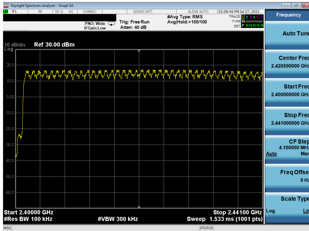
Plot 7-21. Low End Spectrum Channel Hopping Plot Ant-A (Bluetooth, 8DPSK, ePA)
