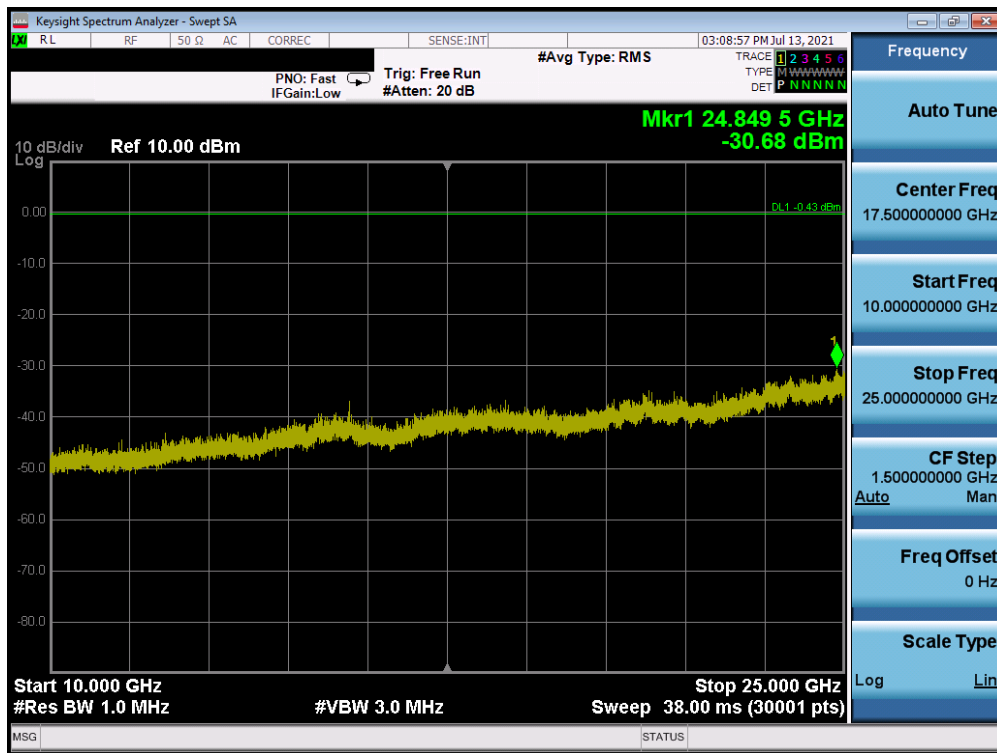
Plot 7-25. Conducted Spurious Plot Ant-A (Bluetooth, GFSK, ePA – Ch. 39)
