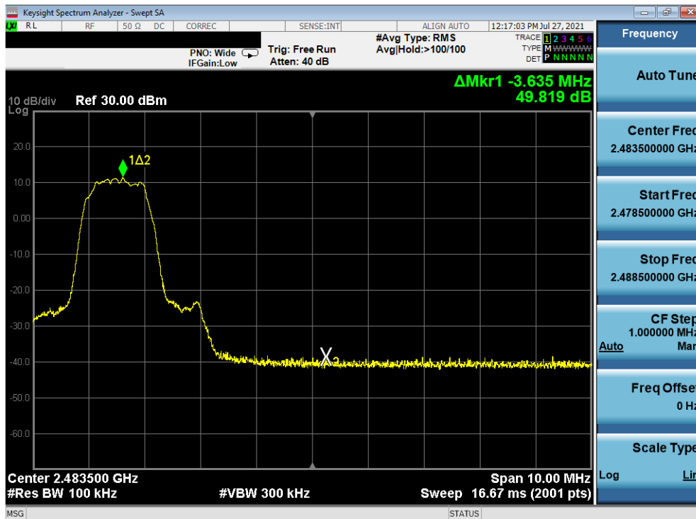
Plot 7-12. Band Edge Plot Ant-A (Bluetooth with Hopping Disabled, 8DPSK, ePA – Ch. 78)
