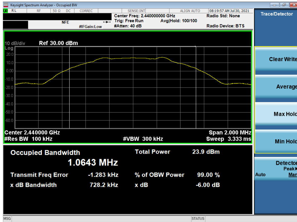
Plot 7-2. 6dB BW & 99% OBW Plot Antenna A (Bluetooth (LE), 1Mbps, ePA – Ch. 19)
