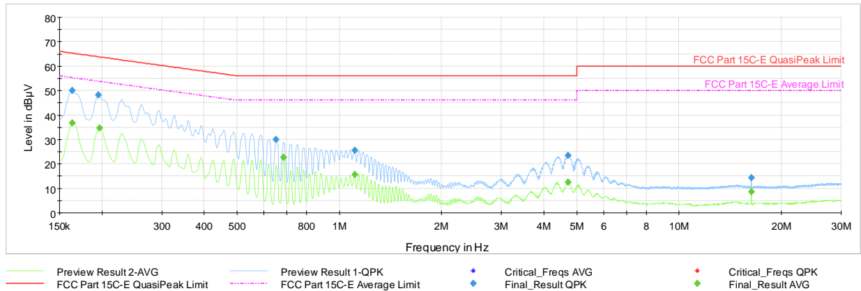
Plot 7-26. AC Line Conducted Plot with Bluetooth LE (1Mbps, ePA – Ch.19 L1, with AC/DC Adapter)
