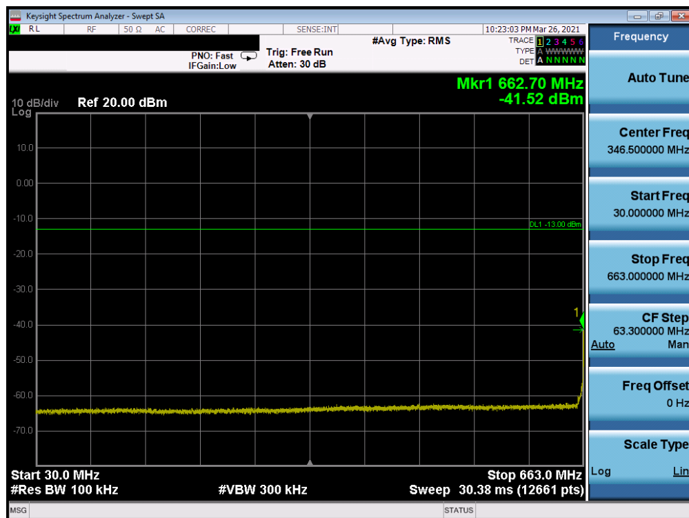
Plot 7-62. CSE (LTE Band 71 - 20MHz QPSK - RB Size 1, RB Offset 0 - Mid Channel)
