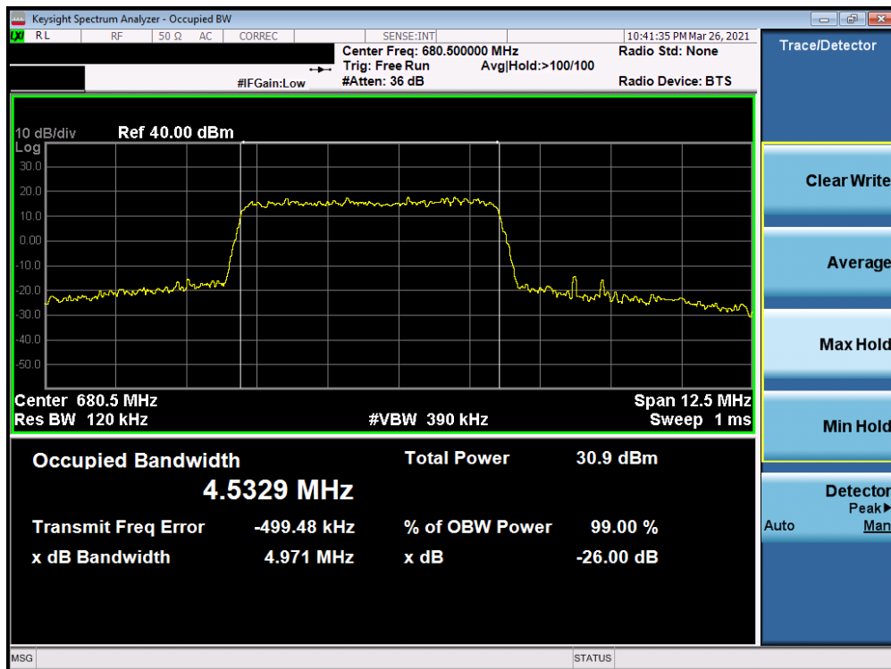
Plot 7-21. Occupied Bandwidth Plot (LTE Band 71 - 5MHz 64-QAM - Full RB Configuration)
