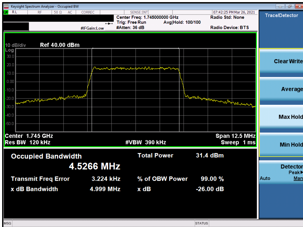
Plot 7-9. Occupied Bandwidth Plot (LTE Band 66/4 - 5MHz 64-QAM - Full RB Configuration)
