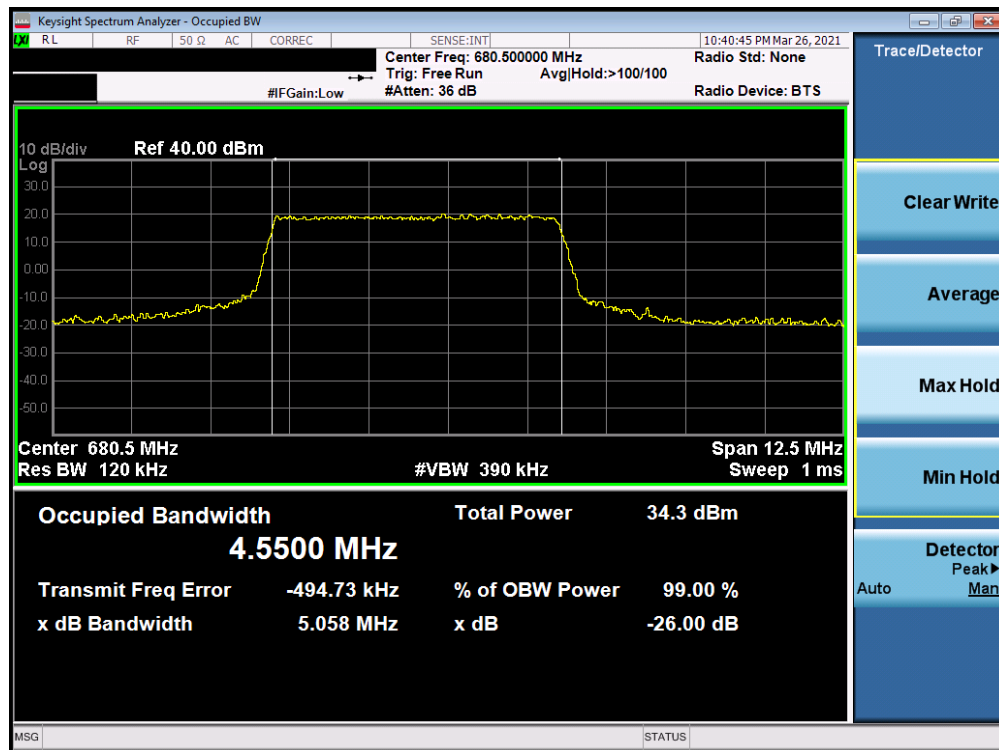
Plot 7-19. Occupied Bandwidth Plot (LTE Band 71 - 5MHz QPSK - Full RB Configuration)
