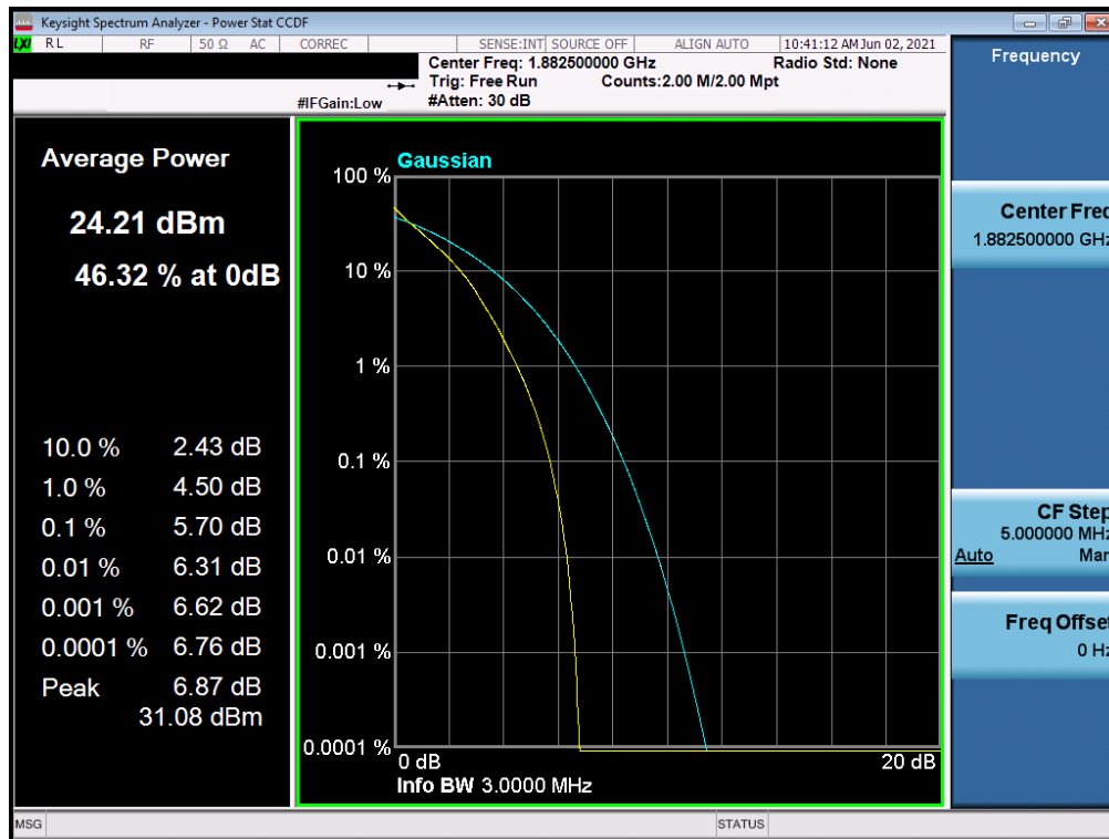
Plot 7-93. PAR Plot (LTE Band 25 - 3MHz QPSK - Full RB Configuration)
