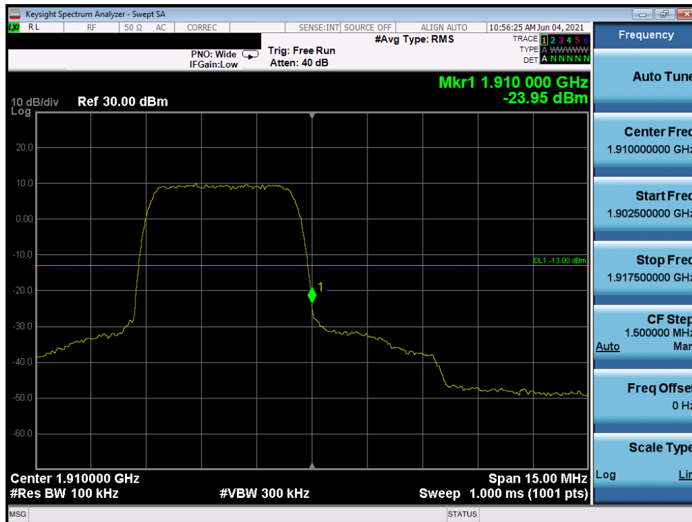
Plot 7-88. Upper Band Edge Plot (WCDMA PCS – Ch. 9538)
