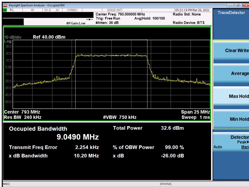
Plot 7-17. Occupied Bandwidth Plot (Band 14 - 10MHz 16-QAM - Full RB Configuration)
