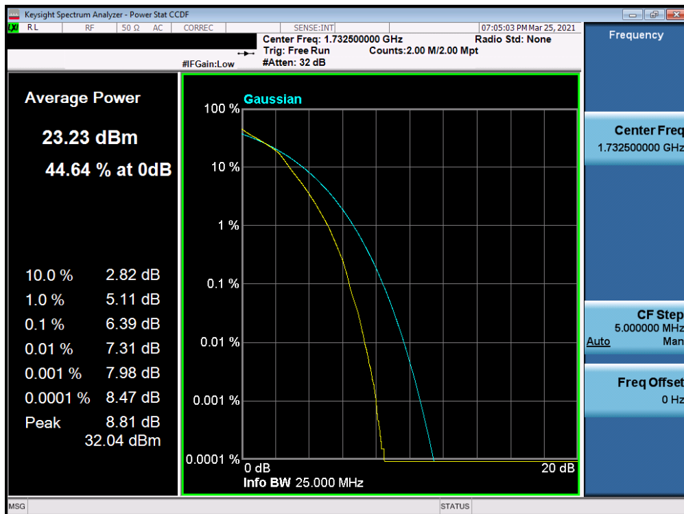
Plot 7-200. PAR Plot (LTE Band 4 - 15MHz 16-QAM - Full RB Configuration)
