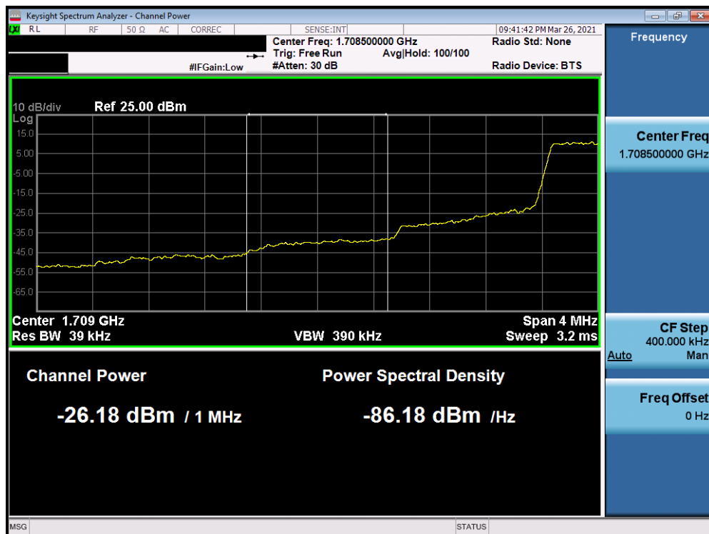
Plot 7-90. Lower Extended Band Edge Plot (Band 66 - 1.4MHz QPSK - Full RB Configuration)
