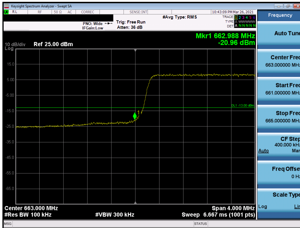
Plot 7-137. Lower Band Edge Plot (Band 71 - 5.0MHz QPSK - Full RB Configuration)
