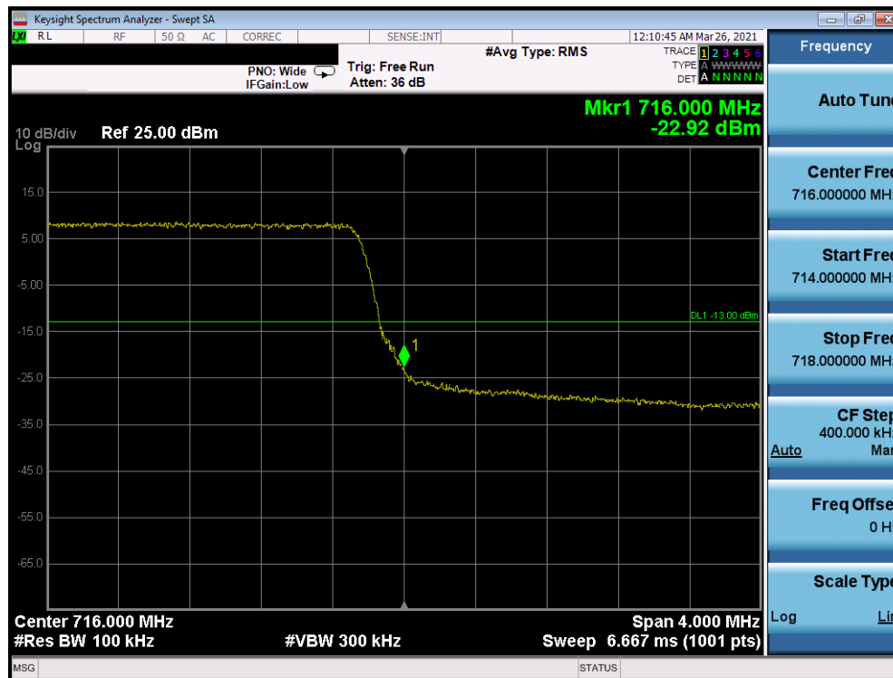
Plot 7-150. Upper Band Edge Plot (Band 12 - 5.0MHz QPSK - Full RB Configuration)
