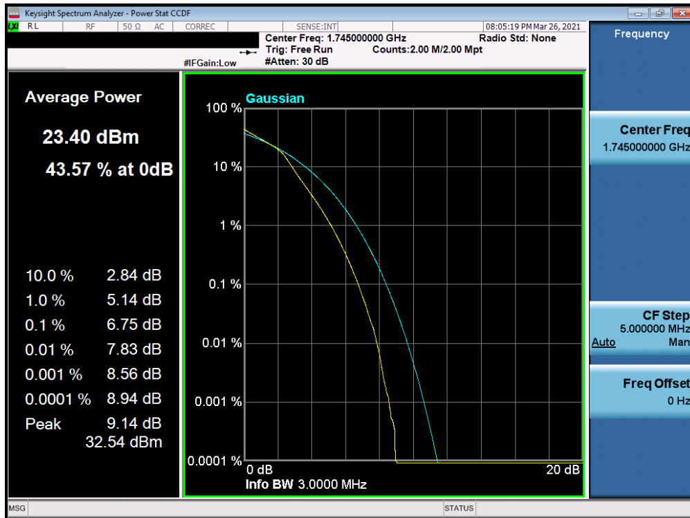
Plot 7-173. PAR Plot (LTE Band 66 - 3MHz 16-QAM - Full RB Configuration)
