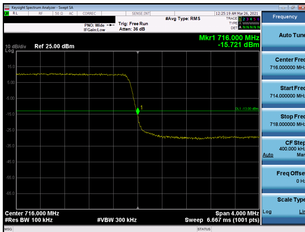
Plot 7-148. Upper Band Edge Plot (Band 12 - 3.0MHz QPSK - Full RB Configuration)
