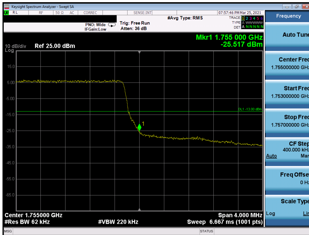
Plot 7-123. Upper Band Edge Plot (Band 4 - 5.0MHz QPSK - Full RB Configuration)
