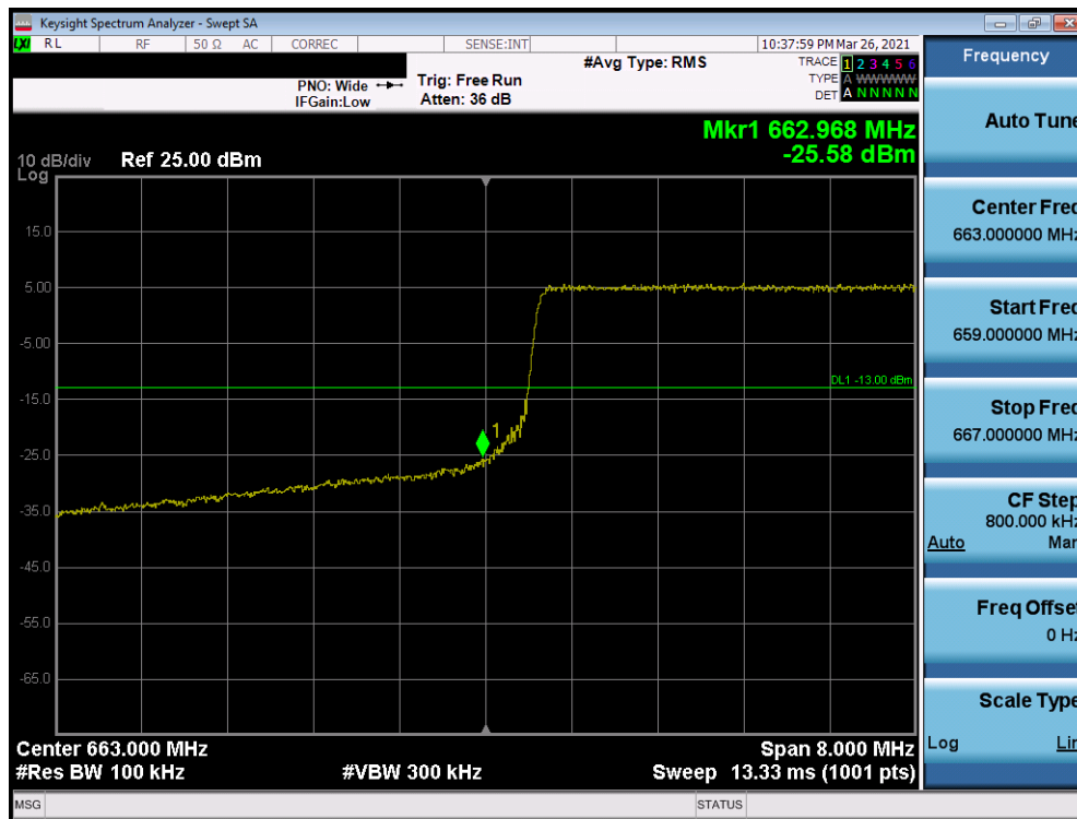
Plot 7-139. Lower Band Edge Plot (Band 71 - 10.0MHz QPSK - Full RB Configuration)
