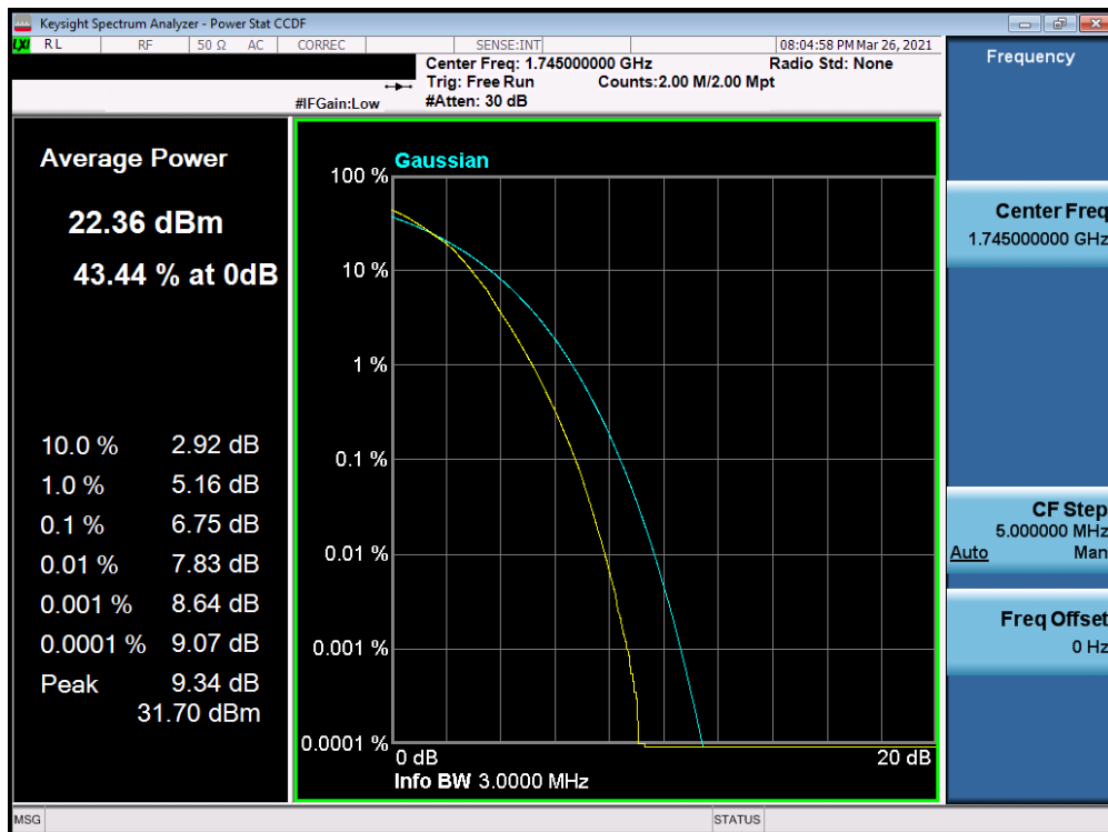
Plot 7-174. PAR Plot (LTE Band 66 - 3MHz 64-QAM - Full RB Configuration)
