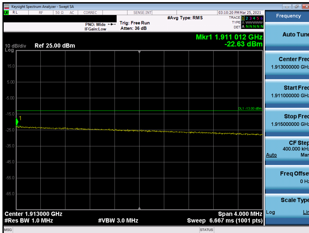
Plot 7-85. Extended Upper Band Edge Plot (LTE Band 2 - 20MHz QPSK – Full RB Configuration)
