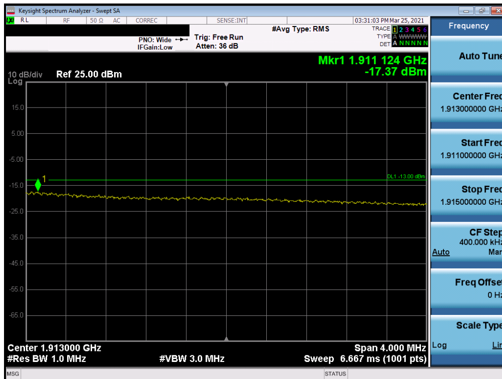
Plot 7-81. Extended Upper Band Edge Plot (LTE Band 2 - 15MHz QPSK – Full RB Configuration)
