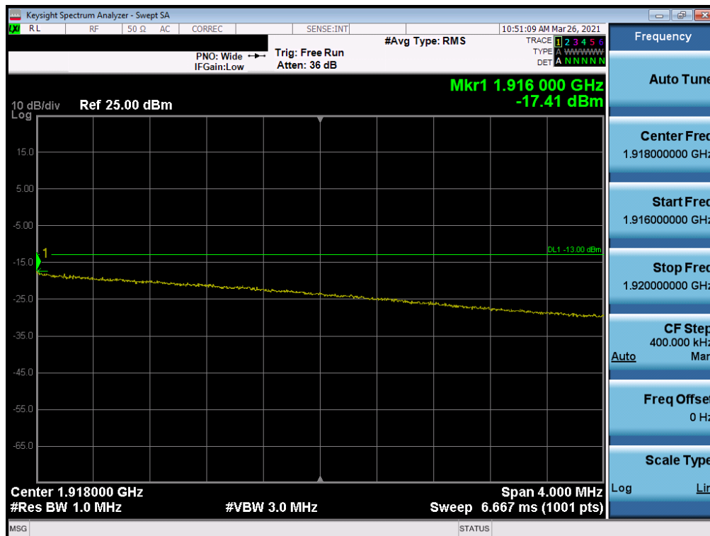
Plot 7-53. Extended Upper Band Edge Plot (LTE Band 25 - 10MHz QPSK – Full RB Configuration)
