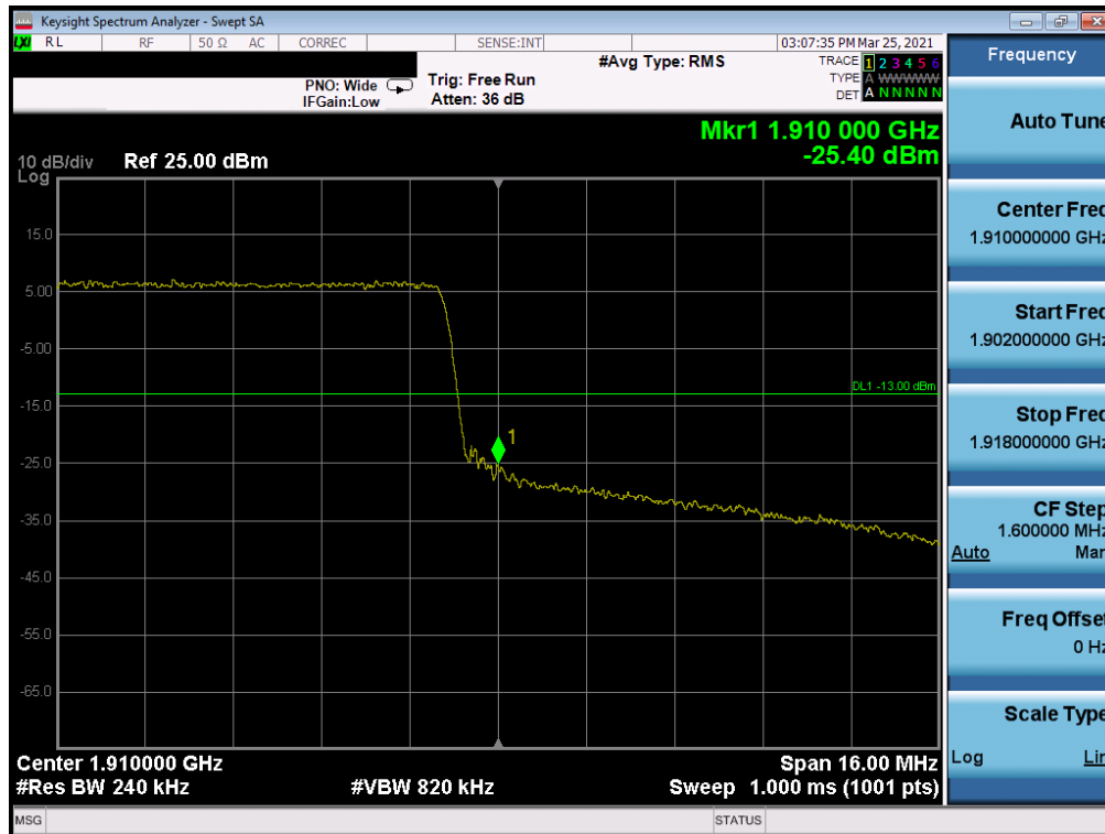
Plot 7-84. Upper Band Edge Plot (LTE Band 2 - 20MHz QPSK – Full RB Configuration)
