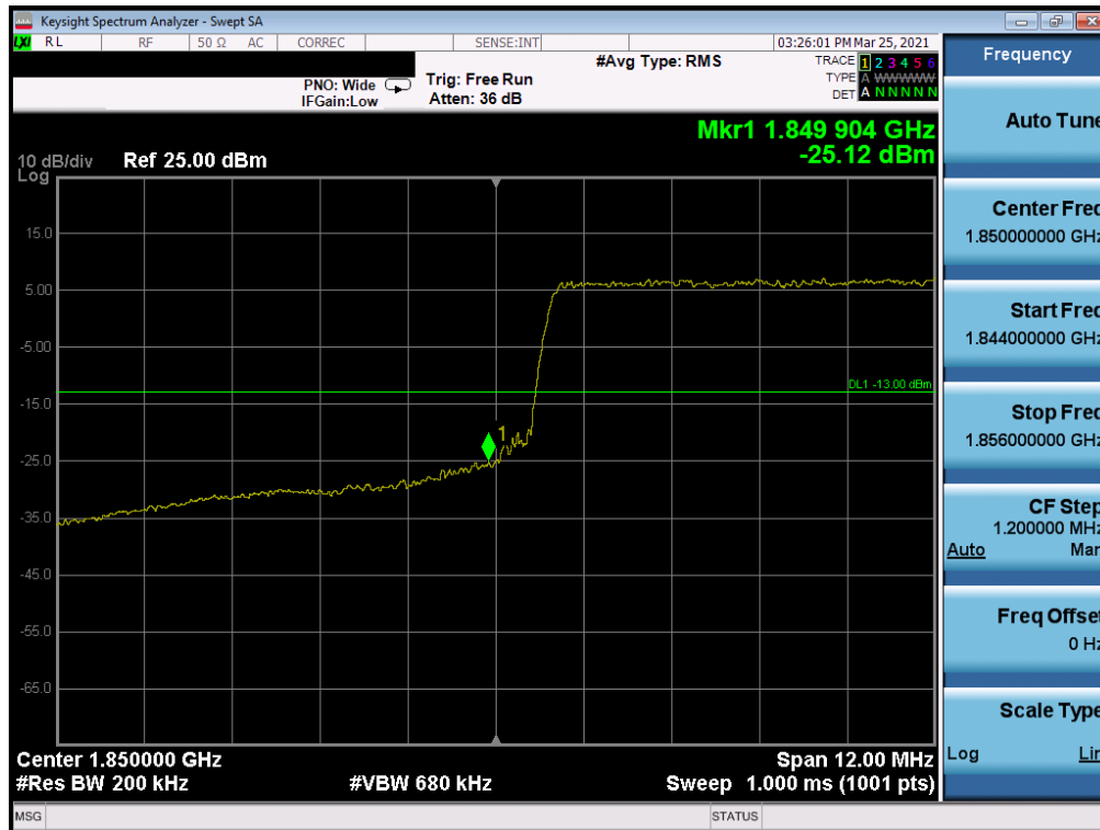
Plot 7-78. Lower Band Edge Plot (LTE Band 2 - 15MHz QPSK – Full RB Configuration)
