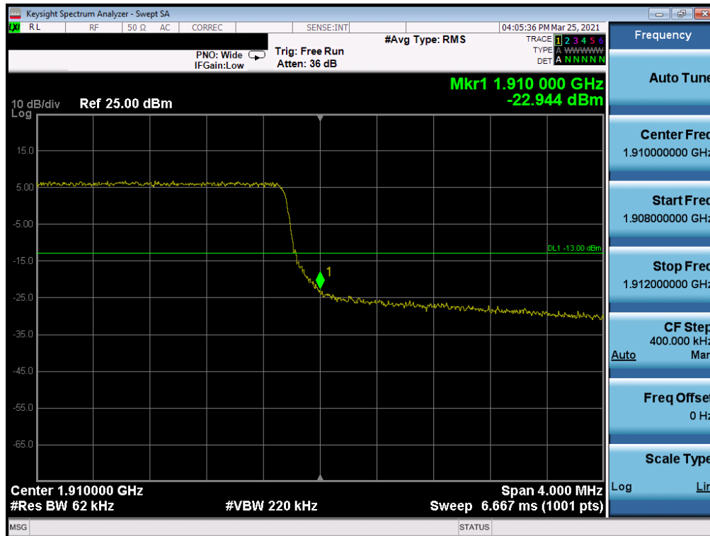
Plot 7-72. Upper Band Edge Plot (LTE Band 2 - 5MHz QPSK – Full RB Configuration)
