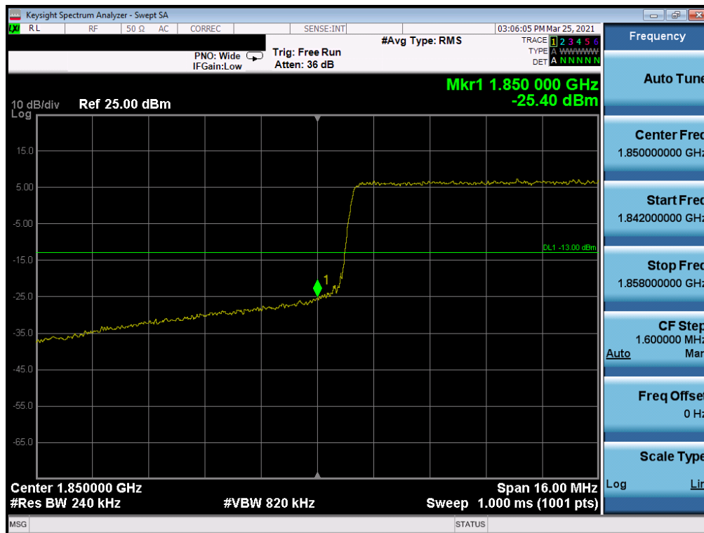
Plot 7-82. Lower Band Edge Plot (LTE Band 2 - 20MHz QPSK – Full RB Configuration)
