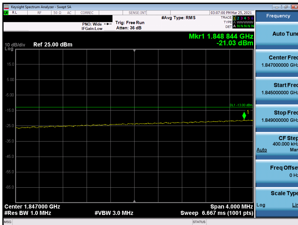
Plot 7-83. Extended Lower Band Edge Plot (LTE Band 2 - 20MHz QPSK – Full RB Configuration)
