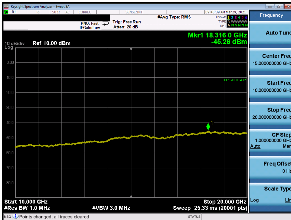
Plot 7-34. CSE (WCDMA Ch. 9400)
