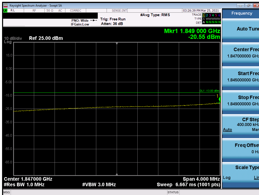
Plot 7-79. Extended Lower Band Edge Plot (LTE Band 2 - 15MHz QPSK – Full RB Configuration)
