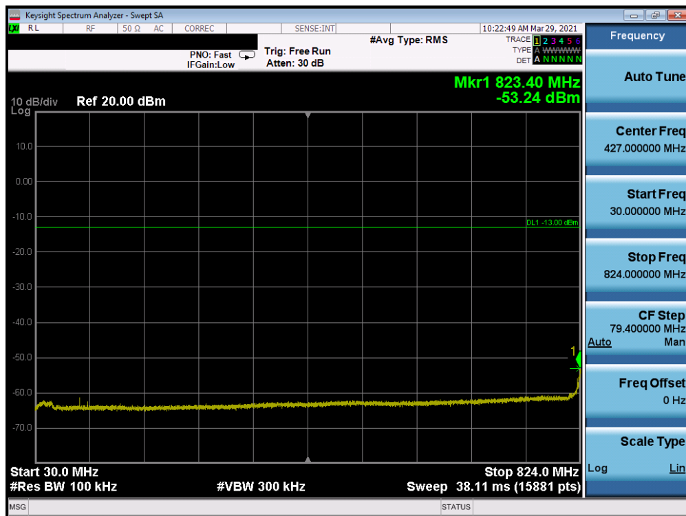
Plot 7-26. CSE (WCDMA Ch. 4183)
