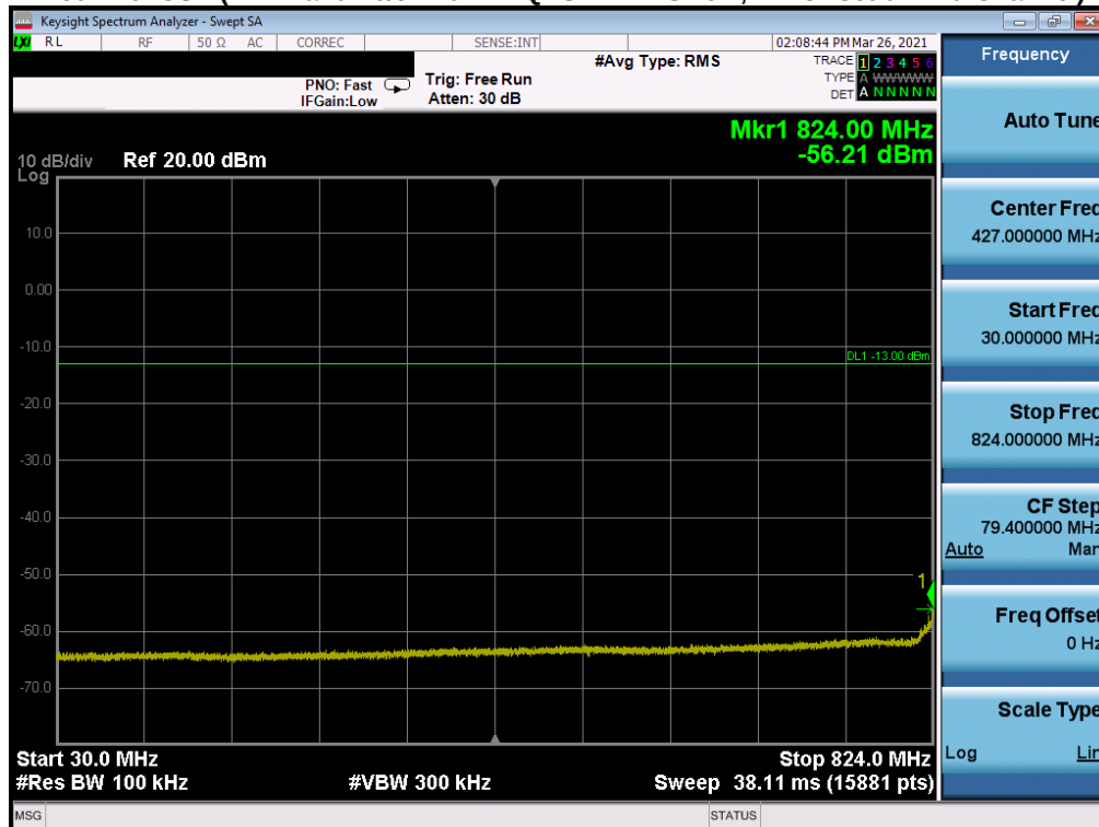
Plot 7-20. CSE (LTE Band 26/5 - 10MHz QPSK - RB Size 1, RB Offset 0 - High Channel)
