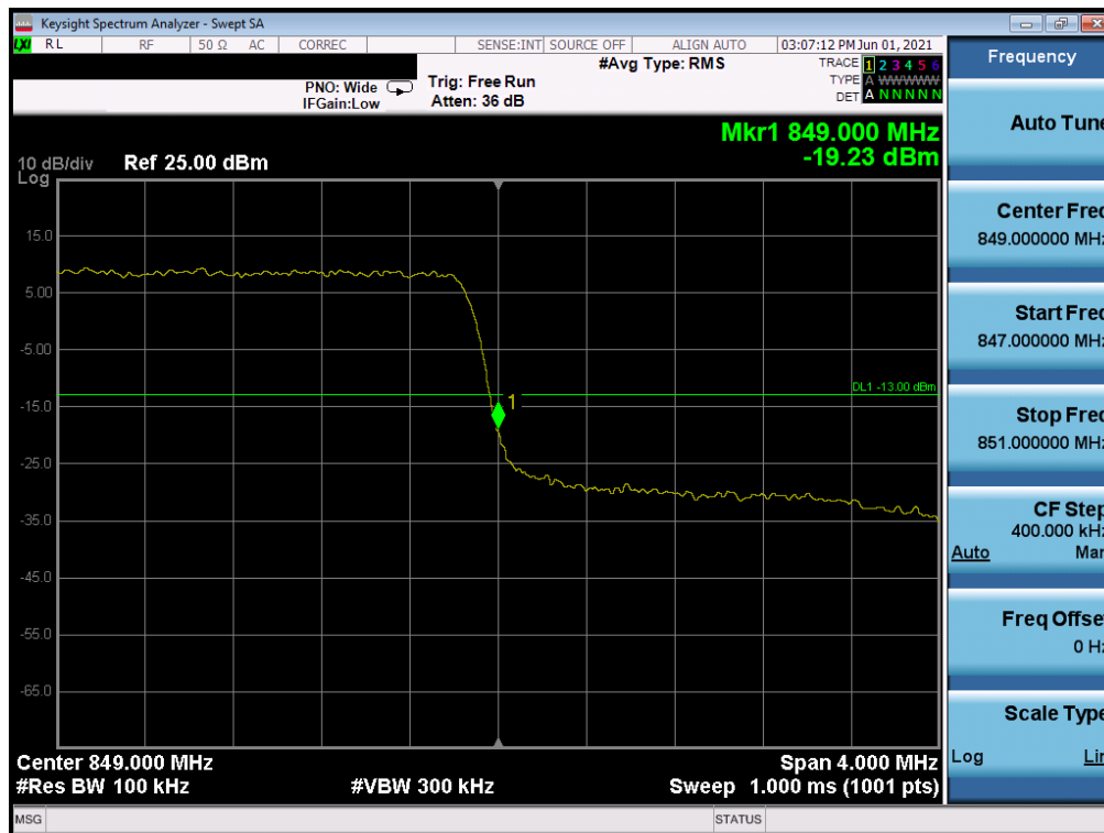
Plot 7-43. Upper Band Edge Plot (LTE Band 5 - 3MHz QPSK – Full RB Configuration)
