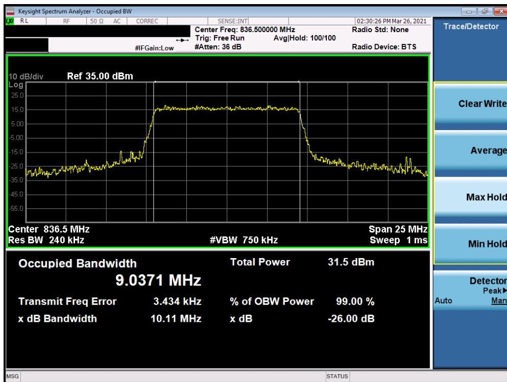
Plot 7-12. Occupied Bandwidth Plot (LTE Band 26/5 - 10MHz 64-QAM - Full RB Configuration)
