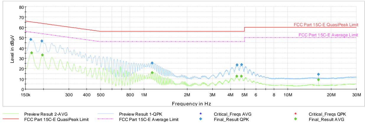
Plot 7-129. AC Line Conducted Plot with CDD 11n Ch.6 (L1, with AC/DC Adapter)
