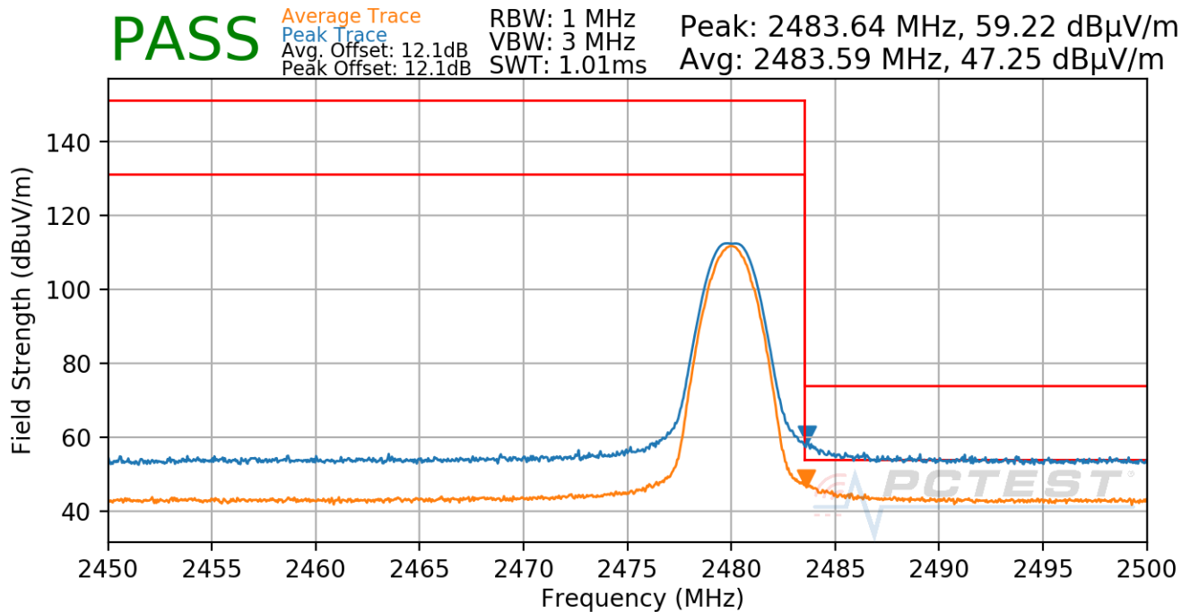
Plot 7-24. Radiated Restricted Upper Band Edge Measurement Antenna A (Average & Peak)
