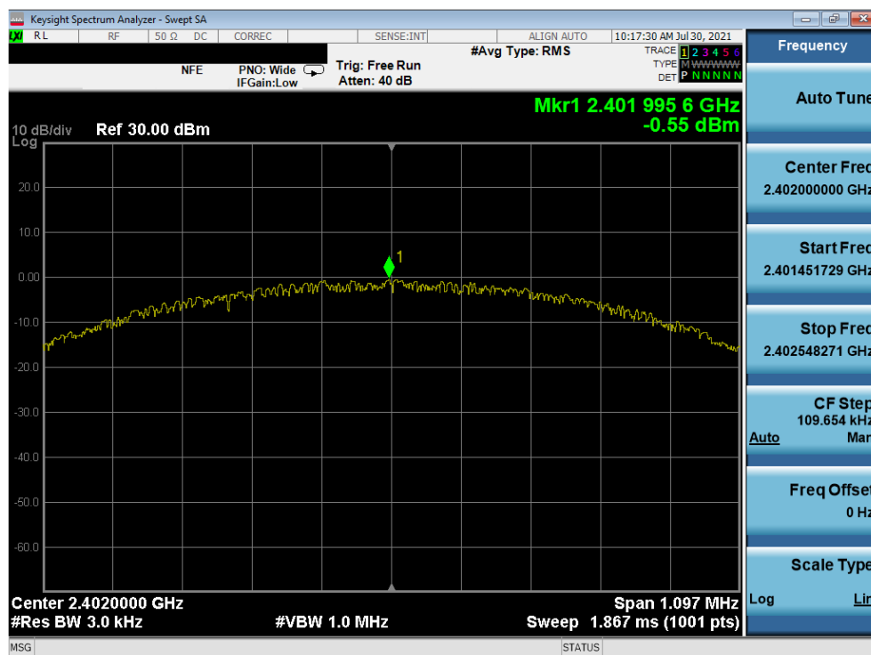
Plot 7-4. Power Spectral Density Plot Antenna A (Bluetooth (LE), 1Mbps, ePA – Ch. 0)
