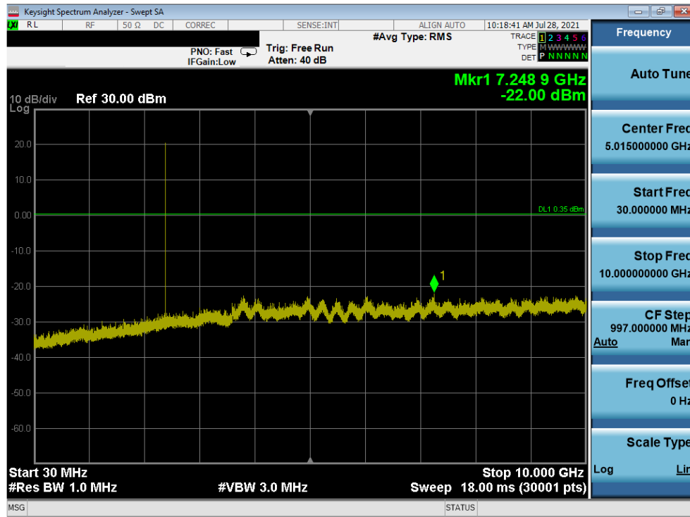
Plot 7-12. Conducted Spurious Plot Antenna A (Bluetooth (LE), 1Mbps, ePA – Ch. 0)
