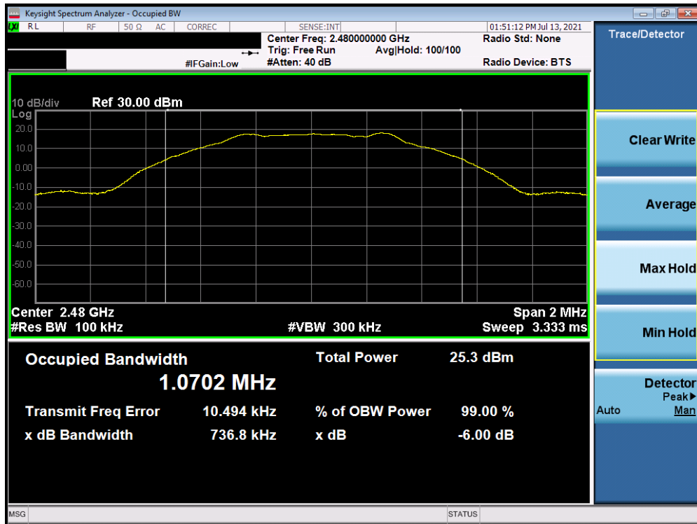
Plot 7-3. 6dB BW & 99% OBW Plot Antenna A (Bluetooth (LE), 1Mbps, ePA – Ch. 39)
