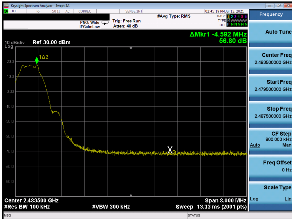
Plot 7-11. Band Edge Plot Antenna A (Bluetooth (LE), 1Mbps, ePA – Ch. 39)
