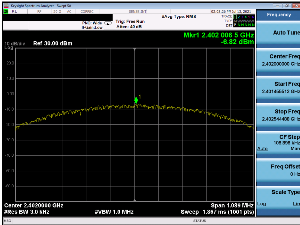
Plot 7-7. Power Spectral Density Plot Antenna A (Bluetooth (LE), 1Mbps, iPA – Ch. 0)
