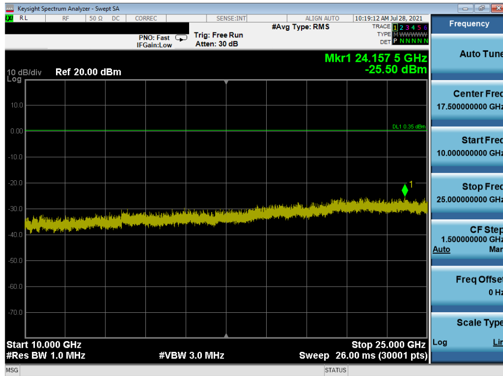
Plot 7-13. Conducted Spurious Plot Antenna A (Bluetooth (LE), 1Mbps, ePA – Ch. 0)
