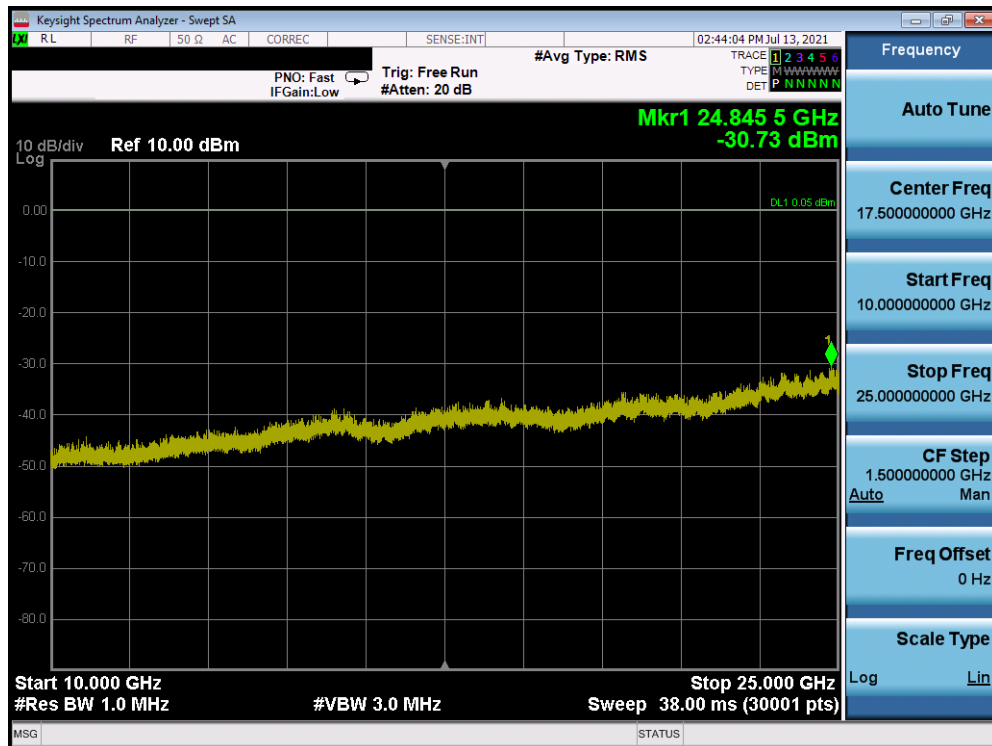
Plot 7-15. Conducted Spurious Plot Antenna A (Bluetooth (LE), 1Mbps, ePA – Ch. 19)
