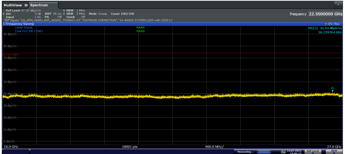
Plot 7-21. Radiated Spurious Plot Above 18GHz Antenna A (1Mbps, ePA – Ch.19, Pol. H)
