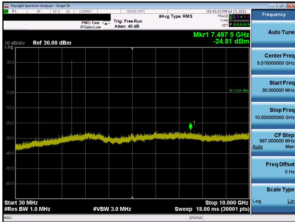
Plot 7-14. Conducted Spurious Plot Antenna A (Bluetooth (LE), 1Mbps, ePA – Ch. 19)
