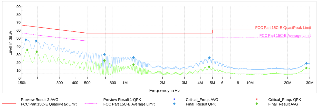
Plot 7-27. Line Conducted Plot with Bluetooth LE (1Mbps, ePA – Ch.19 N, with AC/DC Adapter)
