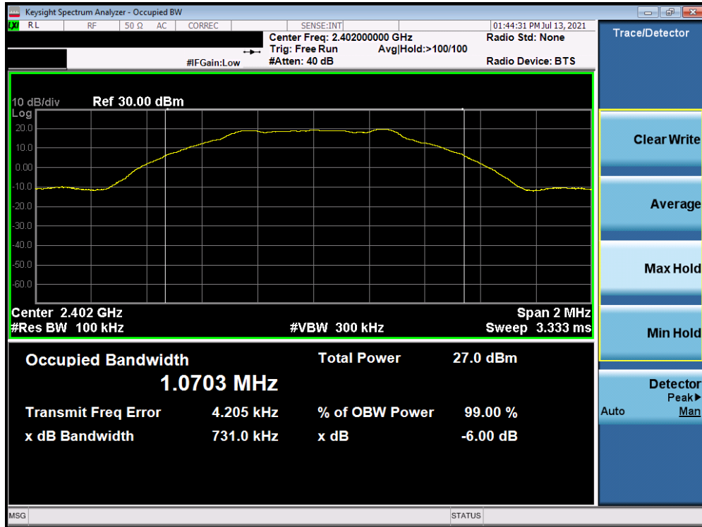
Plot 7-1. 6dB BW & 99% OBW Plot Antenna A (Bluetooth (LE), 1Mbps, ePA – Ch. 0)
