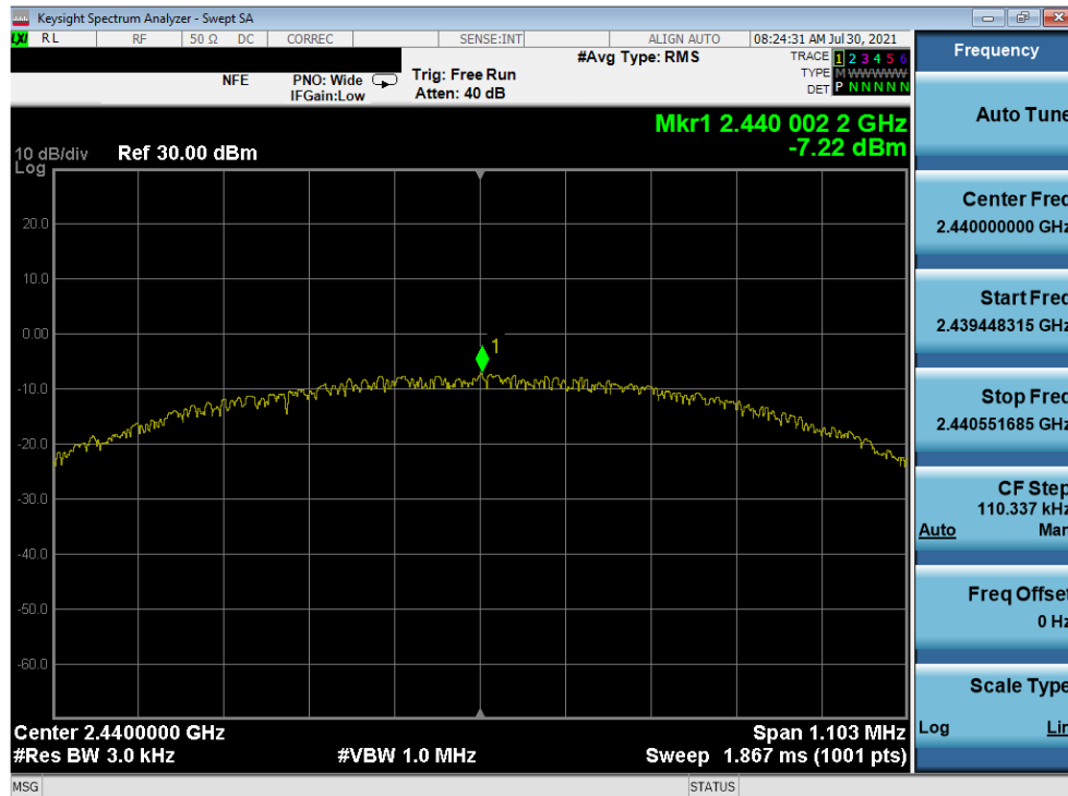
Plot 7-8. Power Spectral Density Plot Antenna A (Bluetooth (LE), 1Mbps, iPA – Ch. 19)
