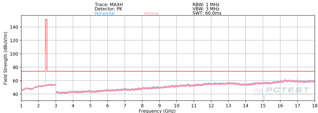
Plot 7-18. Radiated Spurious Plot Above 1GHz Antenna A (1Mbps, ePA – Ch. 0, Ant. Pol. H & V)
