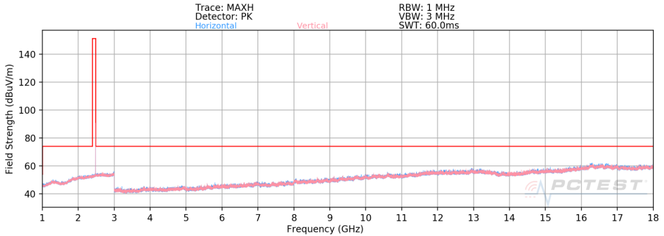
Plot 7-20. Radiated Spurious Plot Above 1GHz Antenna A (1Mbps ePA – Ch. 39, Ant. Pol. H & V)
