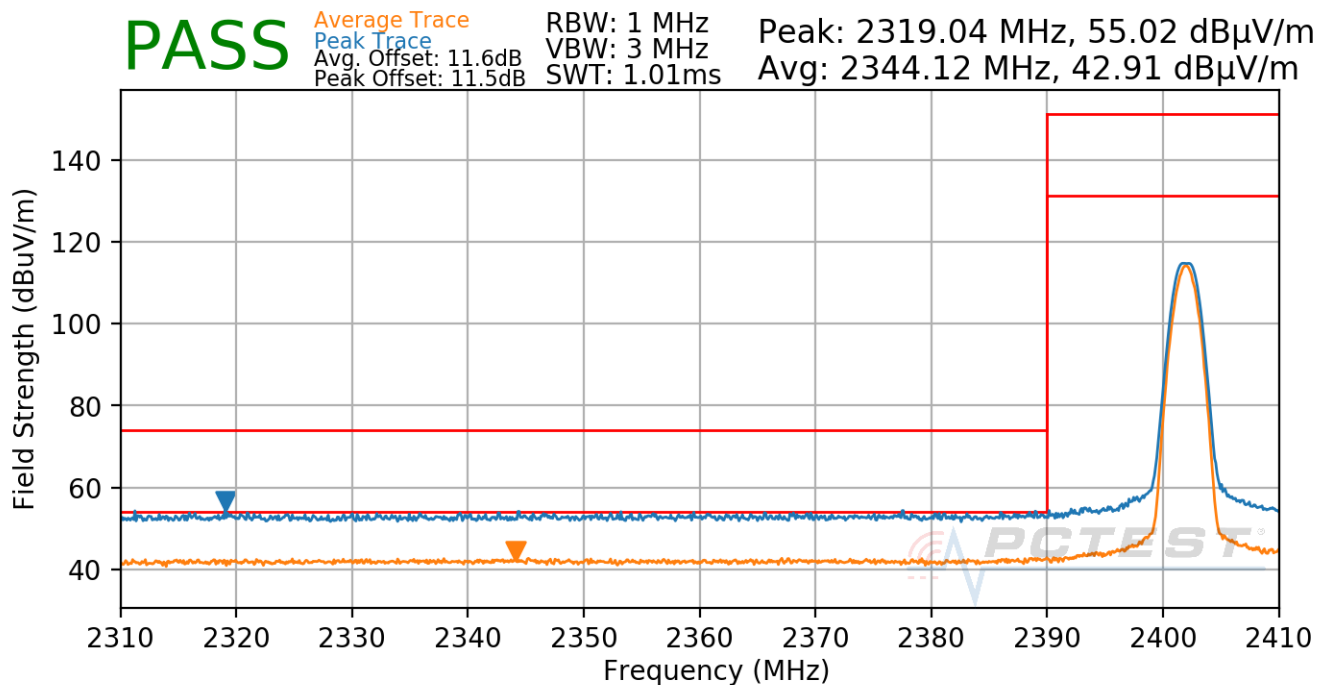
Plot 7-23. Radiated Restricted Lower Band Edge Measurement Antenna A (Average & Peak)
