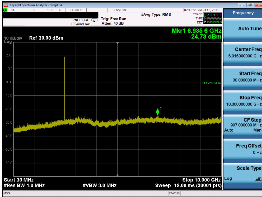
Plot 7-16. Conducted Spurious Plot Antenna A (Bluetooth (LE), 1Mbps, ePA – Ch. 39)
