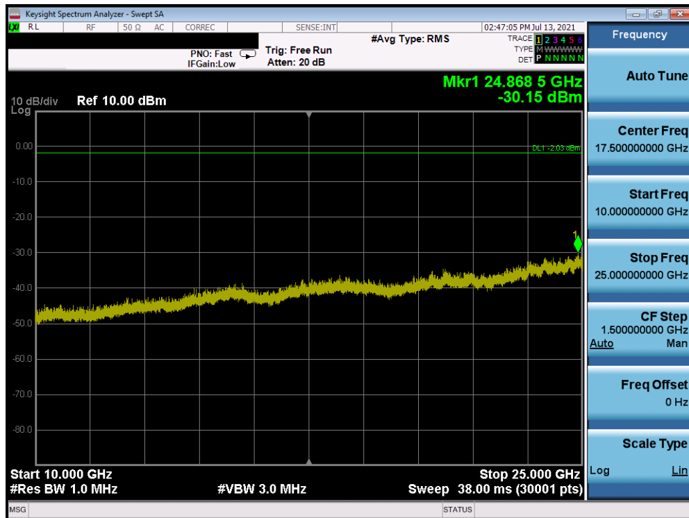
Plot 7-17. Conducted Spurious Plot Antenna A (Bluetooth (LE), 1Mbps, ePA – Ch. 39)
