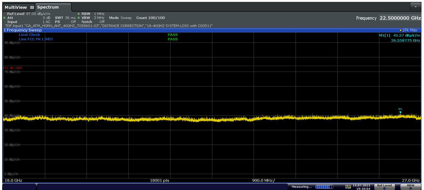
Plot 7-22. Radiated Spurious Plot Above 18GHz Antenna A (1Mbps, ePA – Ch19, Pol. V)
