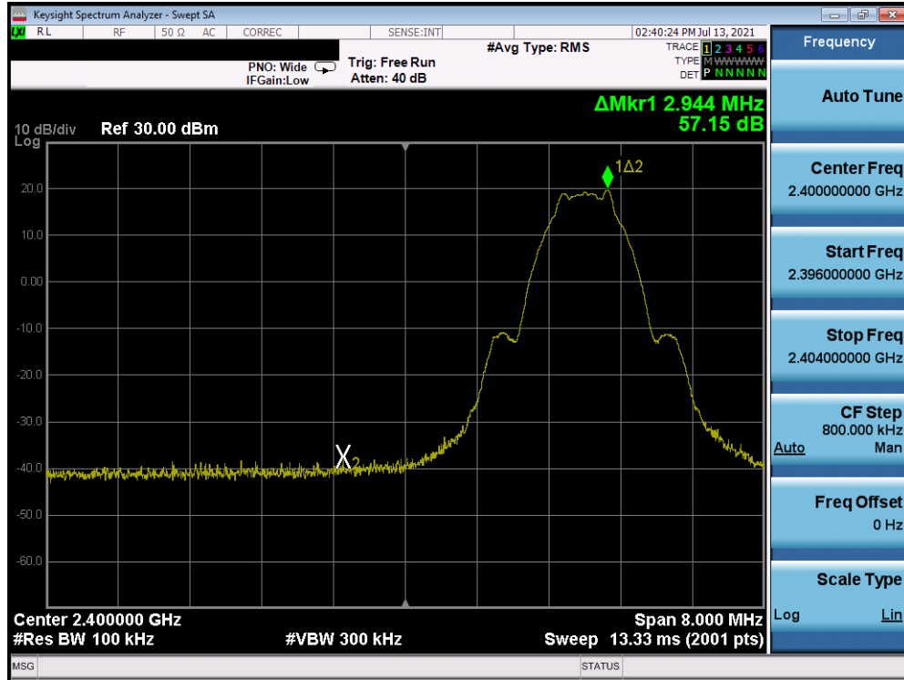
Plot 7-10. Band Edge Plot Antenna A (Bluetooth (LE), 1Mbps, ePA – Ch. 0)
