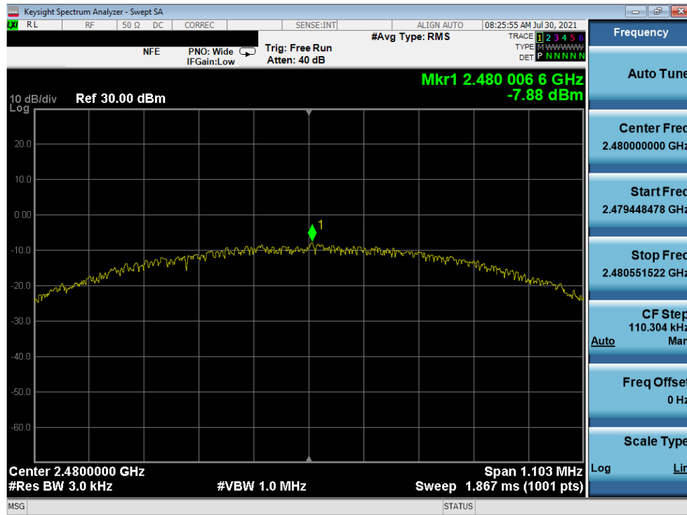
Plot 7-9. Power Spectral Density Plot Antenna A (Bluetooth (LE), 1Mbps, iPA – Ch. 39)
