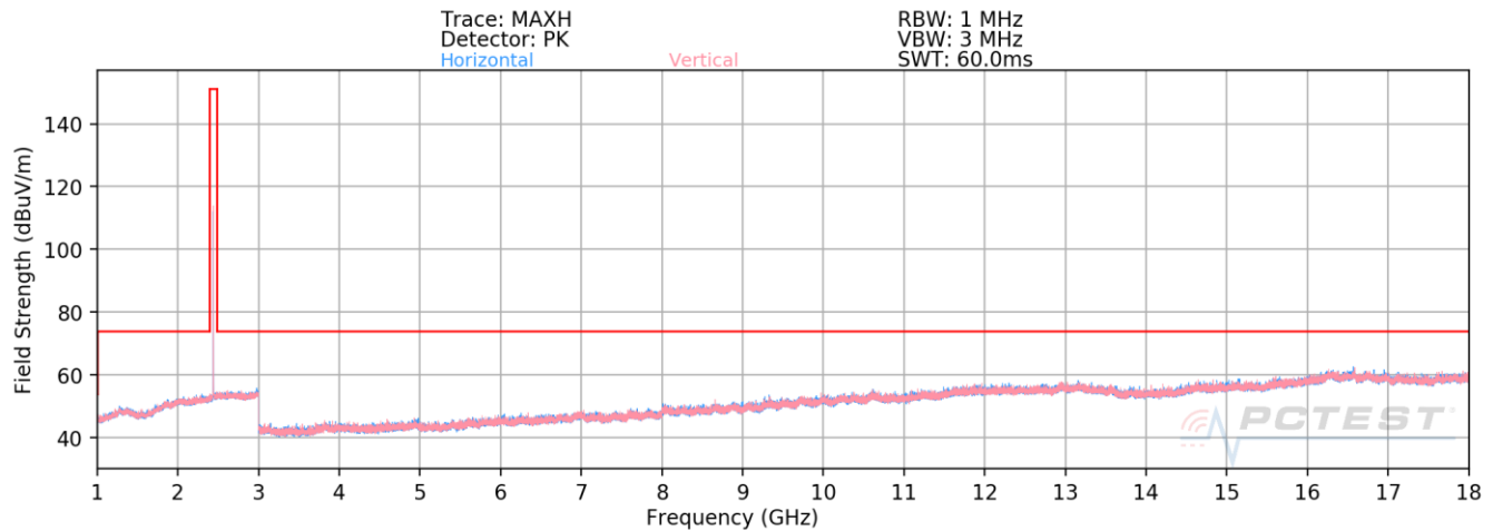
Plot 7-19. Radiated Spurious Plot Above 1GHz Antenna A (1Mbps, ePA – Ch. 19, Ant. Pol. H & V)
