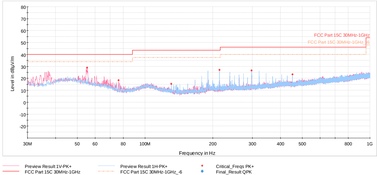
Plot 7-25. Radiated Spurious Plot Below 1GHz Antenna A (1Mbps, ePA – Ch. 19, Pol. H & V, with AC/DC Adapter)
