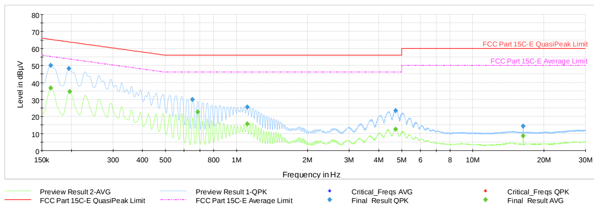
Plot 7-26. AC Line Conducted Plot with Bluetooth LE (1Mbps, ePA – Ch.19 L1, with AC/DC Adapter)
