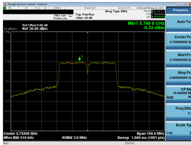
Plot 7-35. PSD Antenna A (40MHz BW 802.11n - Ch. 151, MCS7)
