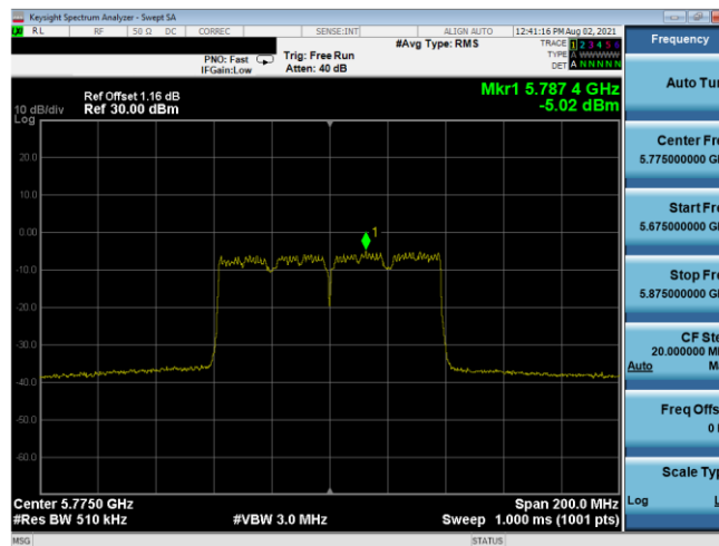
Plot 7-36. PSD Antenna A (80MHz BW 802.11ac - Ch. 155, MCS9)
