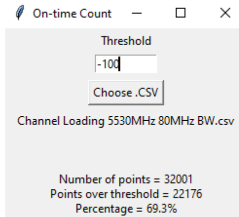
Figure 9-6. 5530MHz - Channel Loading Calculation - Mode 1 (80MHz)
