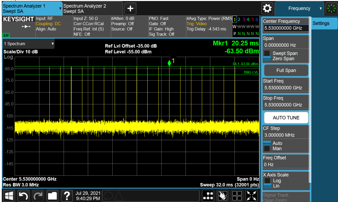
Figure 7-5. 5530MHz – Radar Pulse Type 0 (80MHz)
