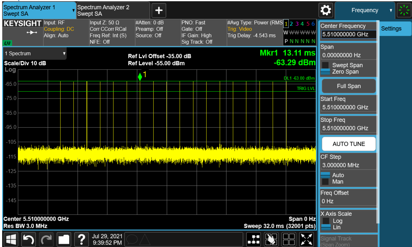
Figure 7-4. 5510MHz – Radar Pulse Type 0 (40MHz)
