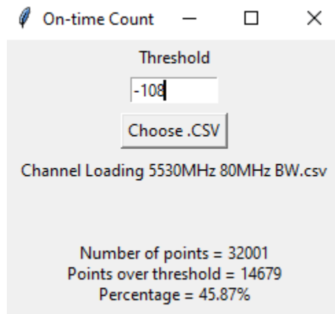
Figure 9-24. 5530MHz - Channel Loading Calculation - Mode 4 (80MHz)
