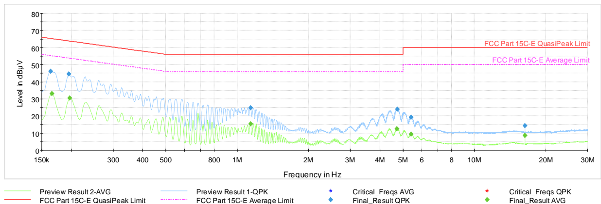
Plot 7-43. AC Line-Conducted Test Plot Antenna A (N, GFSK ePA – Ch.39, with AC/DC Adapter)
