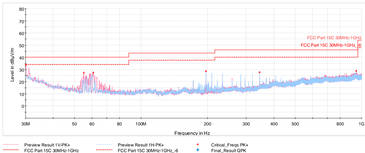
Plot 7-41. Radiated Spurious Emissions Below 1GHz Antenna A (GFSK ePA – Ch.39, with AC/DC Adapter)
