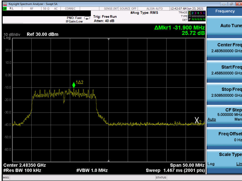
Plot 7-72. Band Edge Plot Antenna B (802.11g- Ch. 13) – 54Mbps
