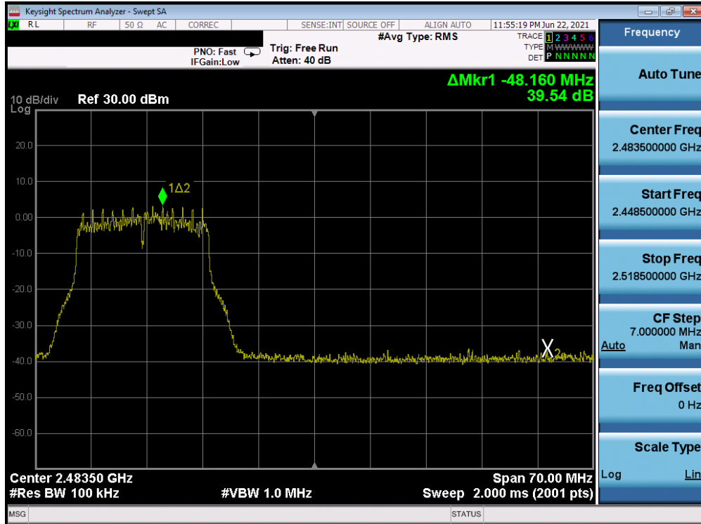
Plot 7-55. Band Edge Plot Antenna A (802.11g- Ch. 11) – 54Mbps
