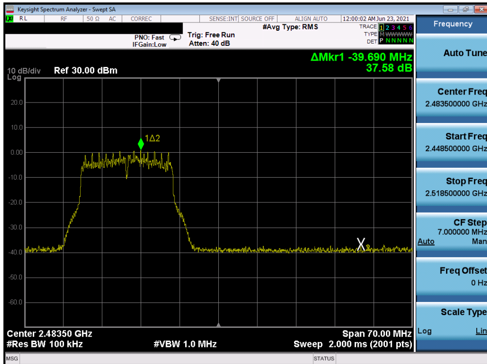
Plot 7-56. Band Edge Plot Antenna A (802.11g- Ch. 12) – 54Mbps
