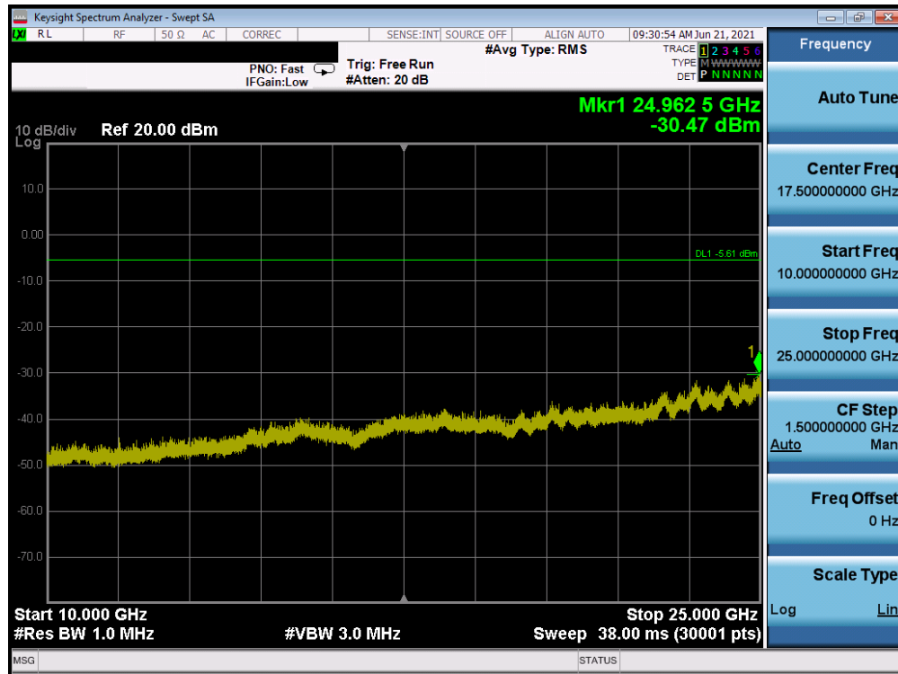
Plot 7-80. Conducted Spurious Plot Antenna A (802.11b – Ch. 1)
