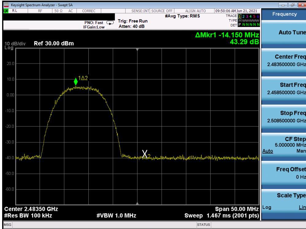
Plot 7-51. Band Edge Plot Antenna A (802.11b – Ch. 13) – 11Mbps
