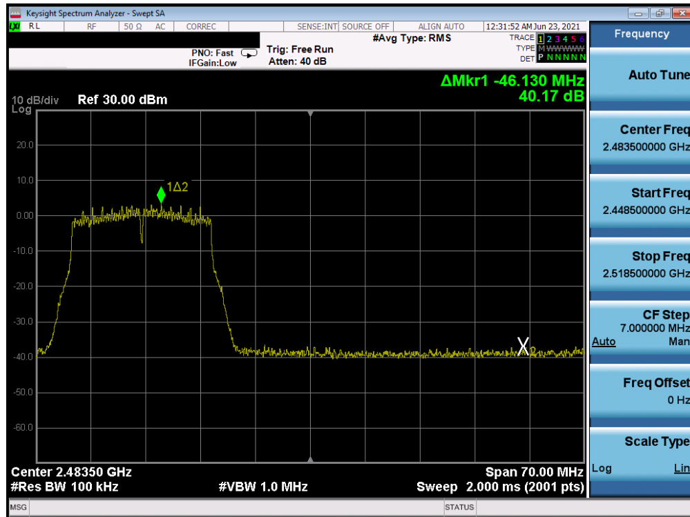
Plot 7-76. Band Edge Plot Antenna B (802.11n (2.4GHz) – Ch. 11) – MCS7
