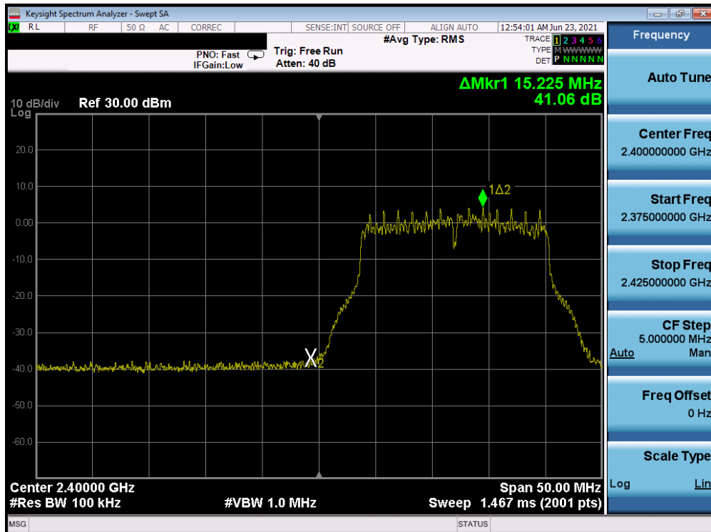
Plot 7-67. Band Edge Plot Antenna B (802.11g– Ch. 1) – 54Mbps
