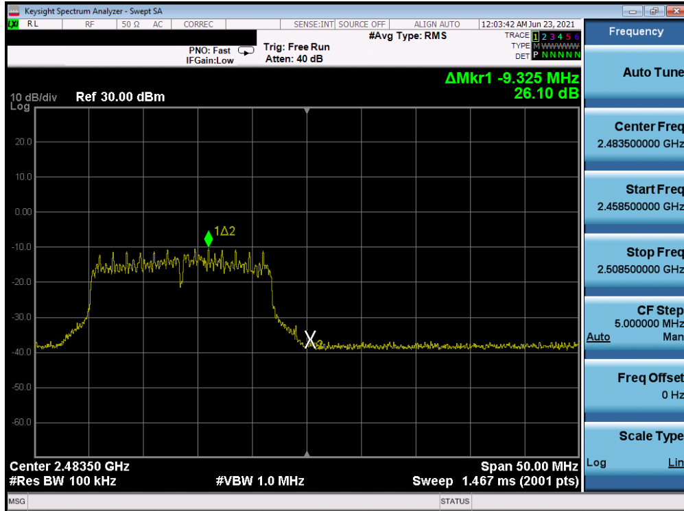
Plot 7-57. Band Edge Plot Antenna A (802.11g- Ch. 13) – 54Mbps
