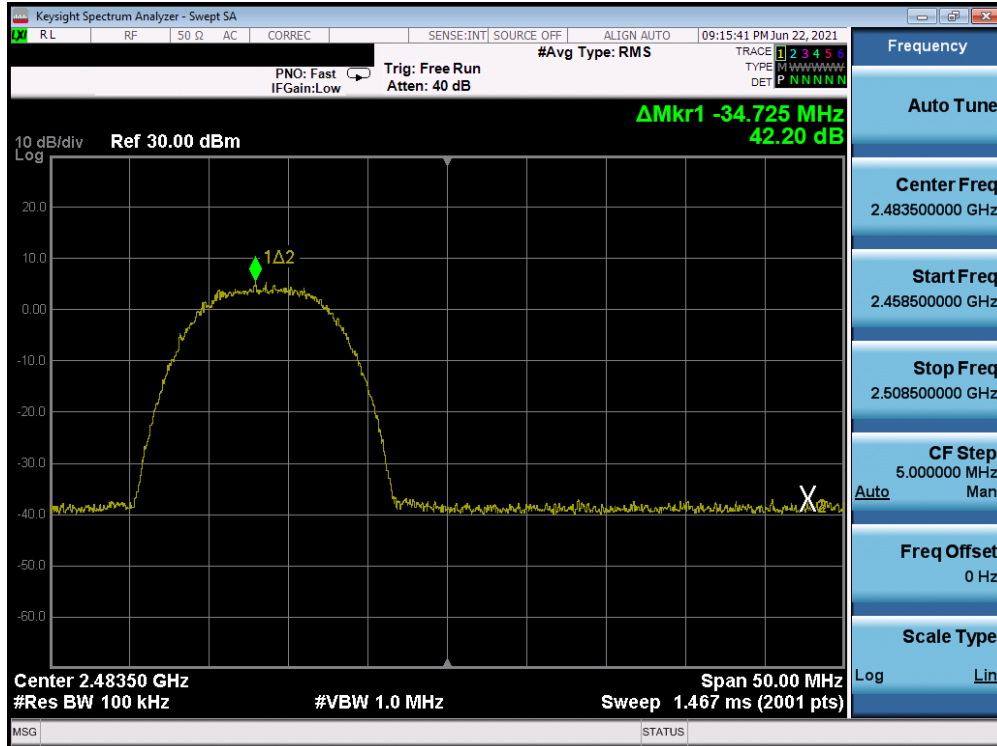
Plot 7-66. Band Edge Plot Antenna B (802.11b – Ch. 13) – 11Mbps
