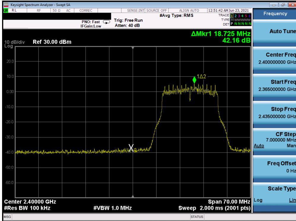
Plot 7-68. Band Edge Plot Antenna B (802.11g- Ch. 2) – 54Mbps
