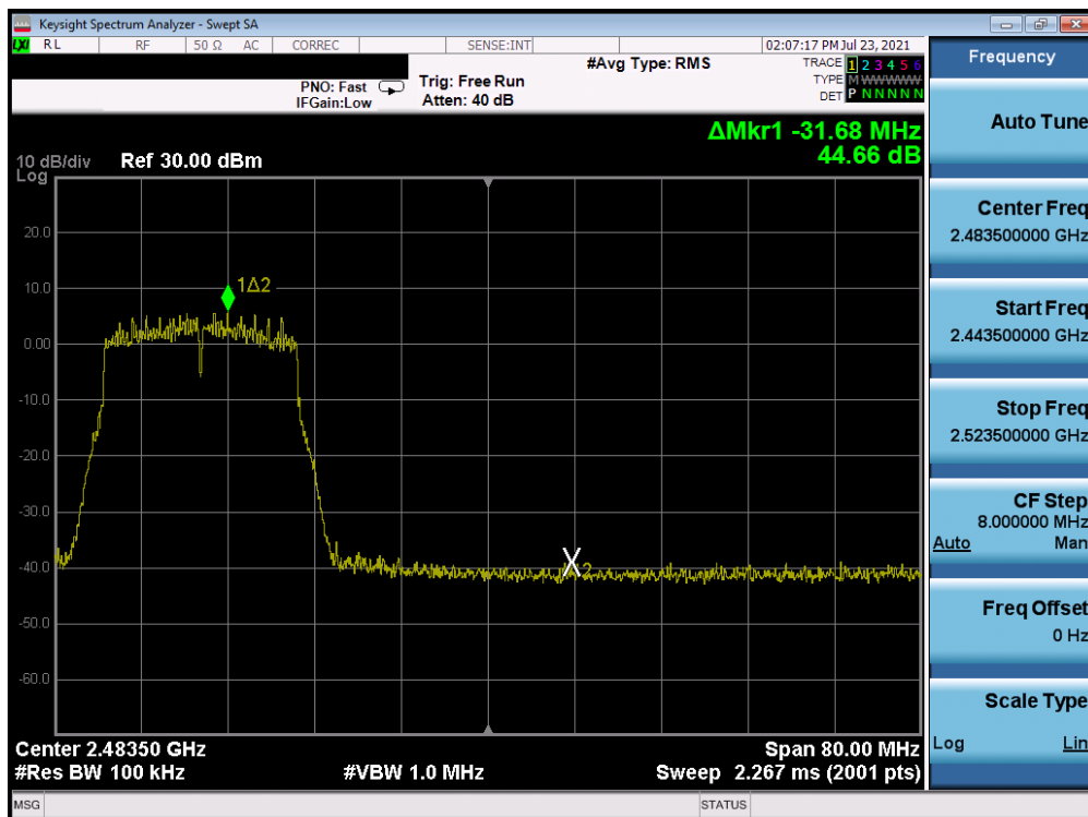
Plot 7-75. Band Edge Plot Antenna B (802.11n (2.4GHz) - Ch. 10) - MCS7
