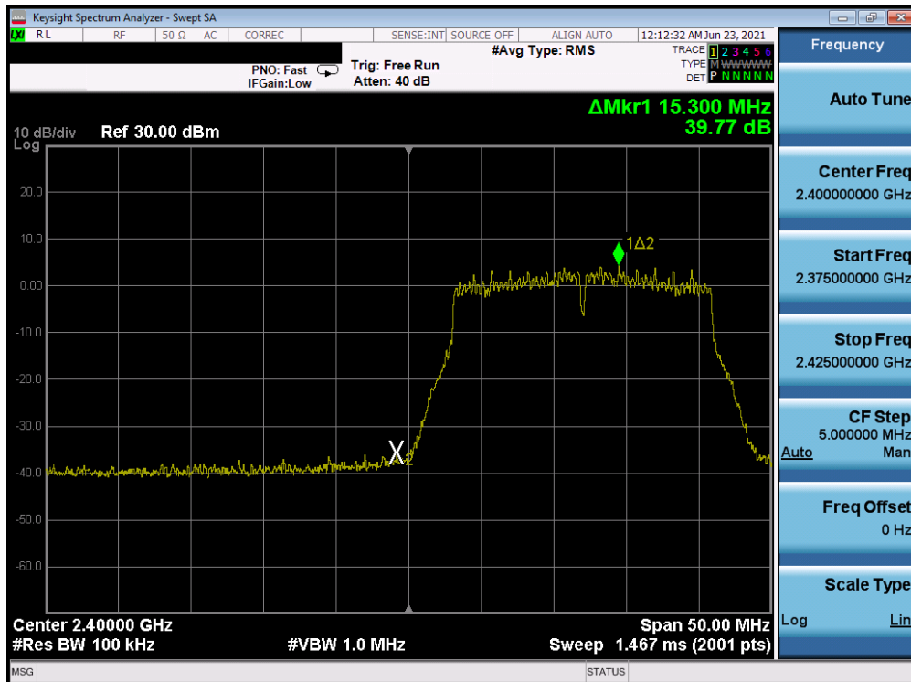
Plot 7-58. Band Edge Plot Antenna A (802.11n (2.4GHz) - Ch. 1) – MCS7
