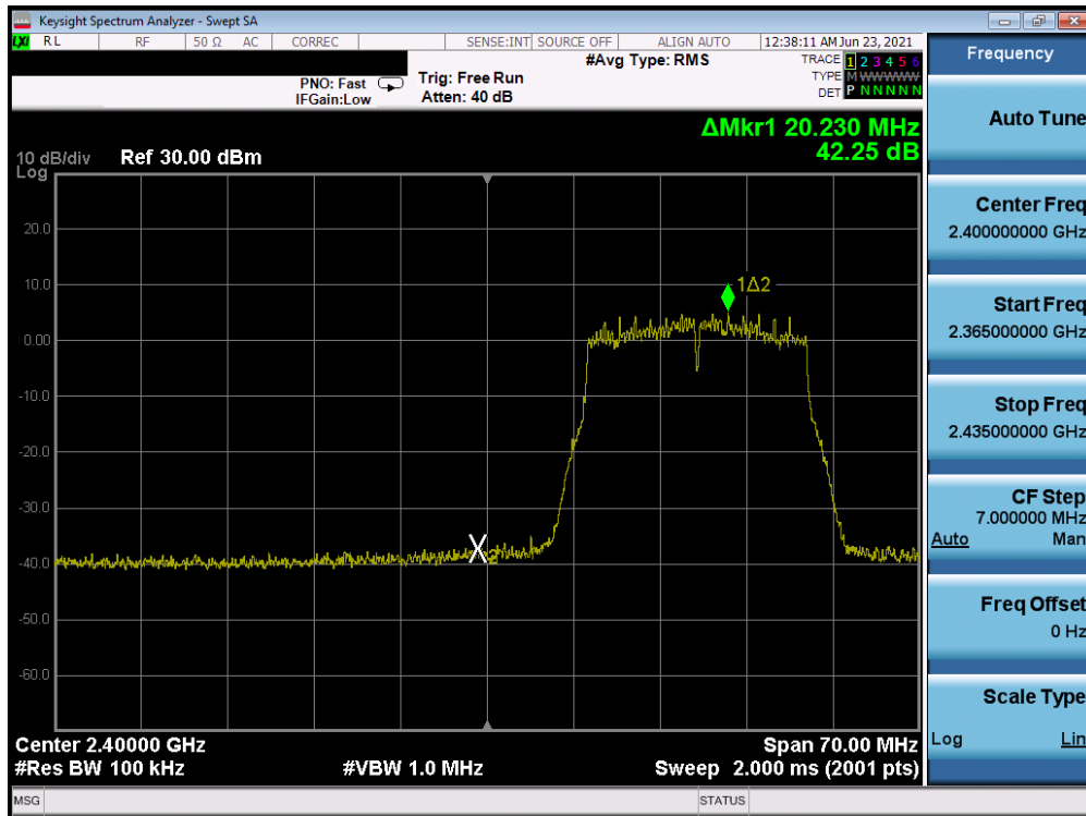
Plot 7-74. Band Edge Plot Antenna B (802.11n (2.4GHz) - Ch. 2) - MCS7
