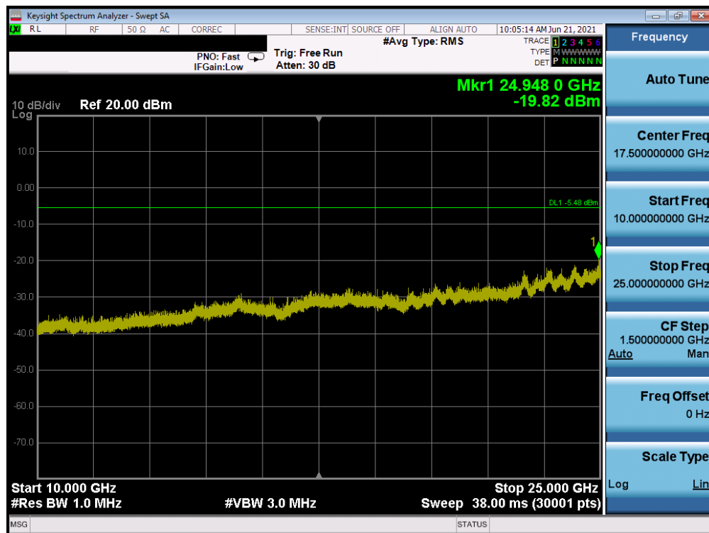
Plot 7-82. Conducted Spurious Plot Antenna A (802.11b – Ch. 6)
