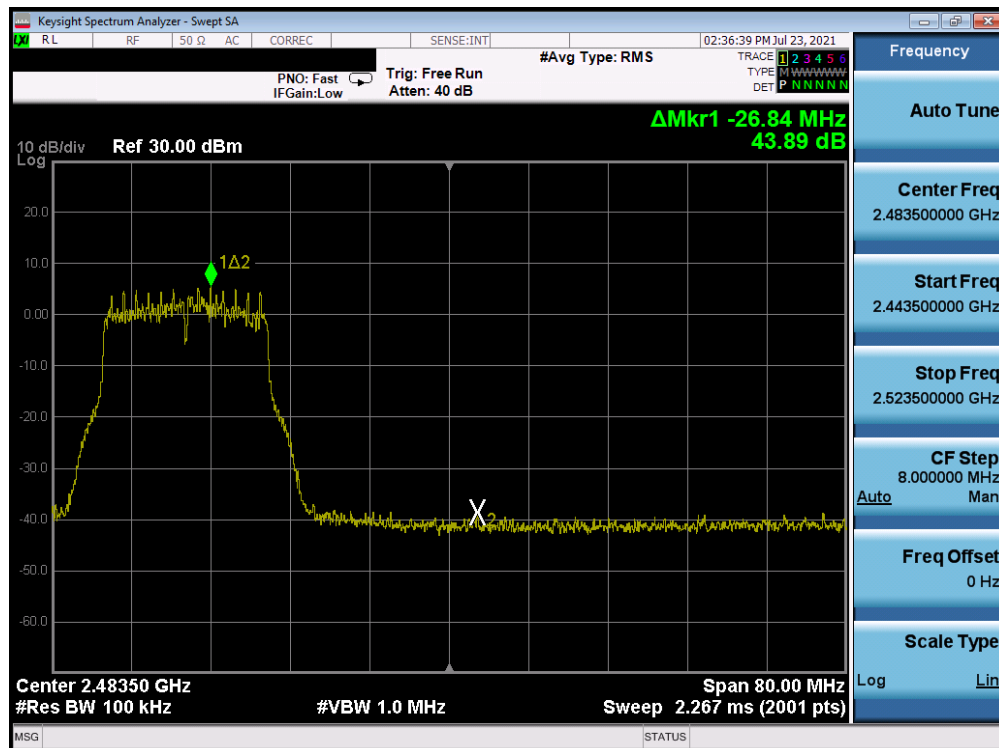
Plot 7-54. Band Edge Plot Antenna A (802.11g- Ch. 10) – 54Mbps
