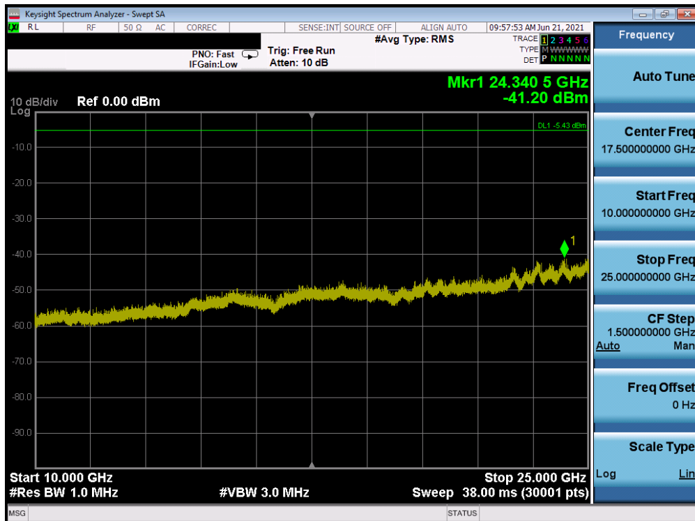
Plot 7-84. Conducted Spurious Plot Antenna A (802.11b – Ch. 11)
