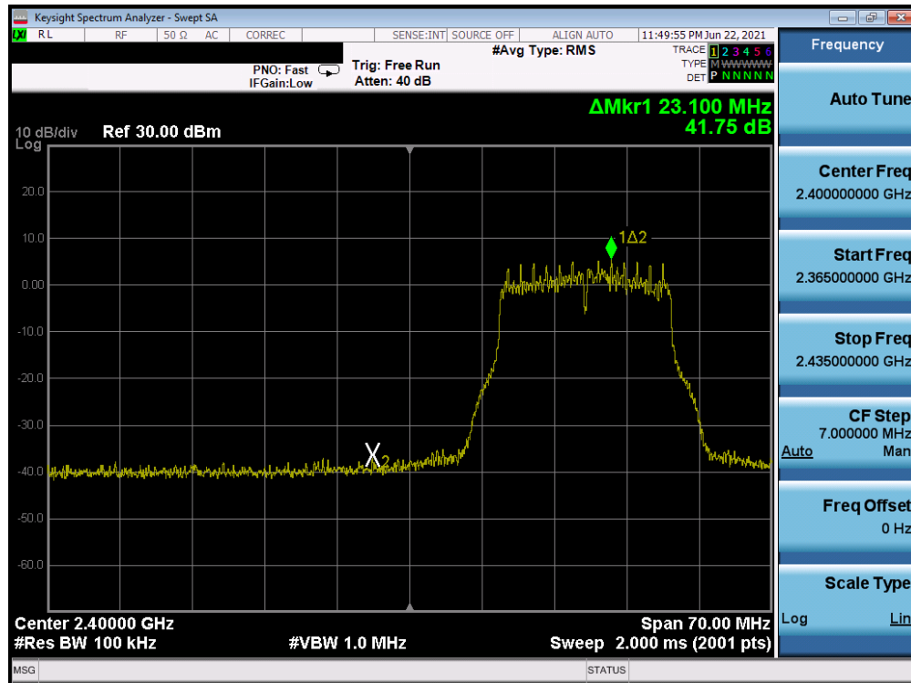
Plot 7-53. Band Edge Plot Antenna A (802.11g- Ch. 2) – 54Mbps
