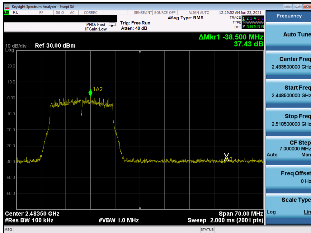
Plot 7-77. Band Edge Plot Antenna B (802.11n (2.4GHz) – Ch. 12) – MCS7
