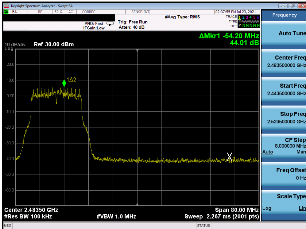
Plot 7-69. Band Edge Plot Antenna B (802.11g- Ch. 10) – 54Mbps
