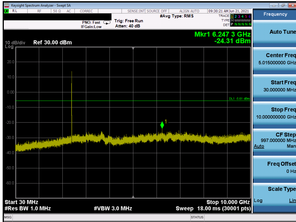
Plot 7-79. Conducted Spurious Plot Antenna A (802.11b – Ch. 1)
