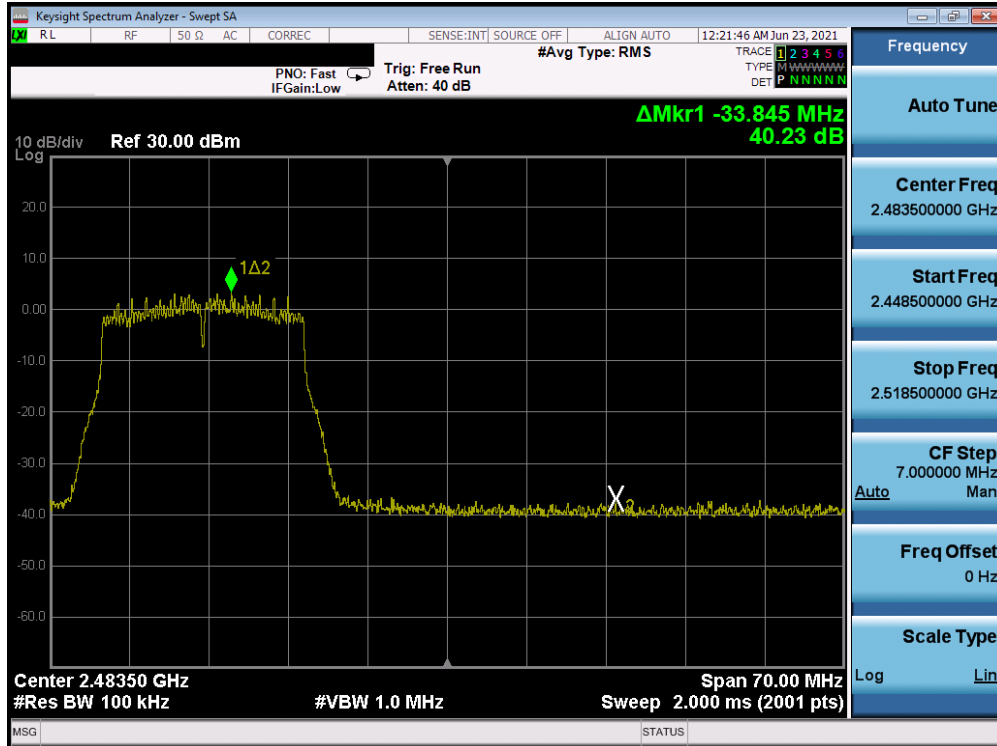
Plot 7-61. Band Edge Plot Antenna A (802.11n (2.4GHz) – Ch. 11) – MCS7
