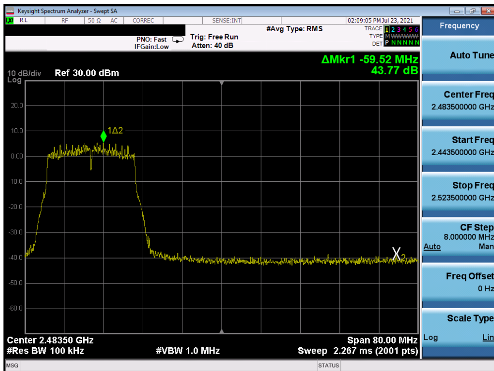
Plot 7-60. Band Edge Plot Antenna A (802.11n (2.4GHz) – Ch. 10) – MCS7
