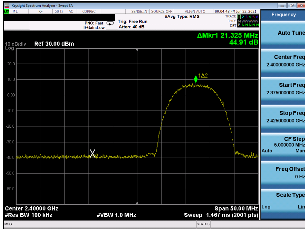
Plot 7-64. Band Edge Plot Antenna B (802.11b – Ch. 1) – 11Mbps
