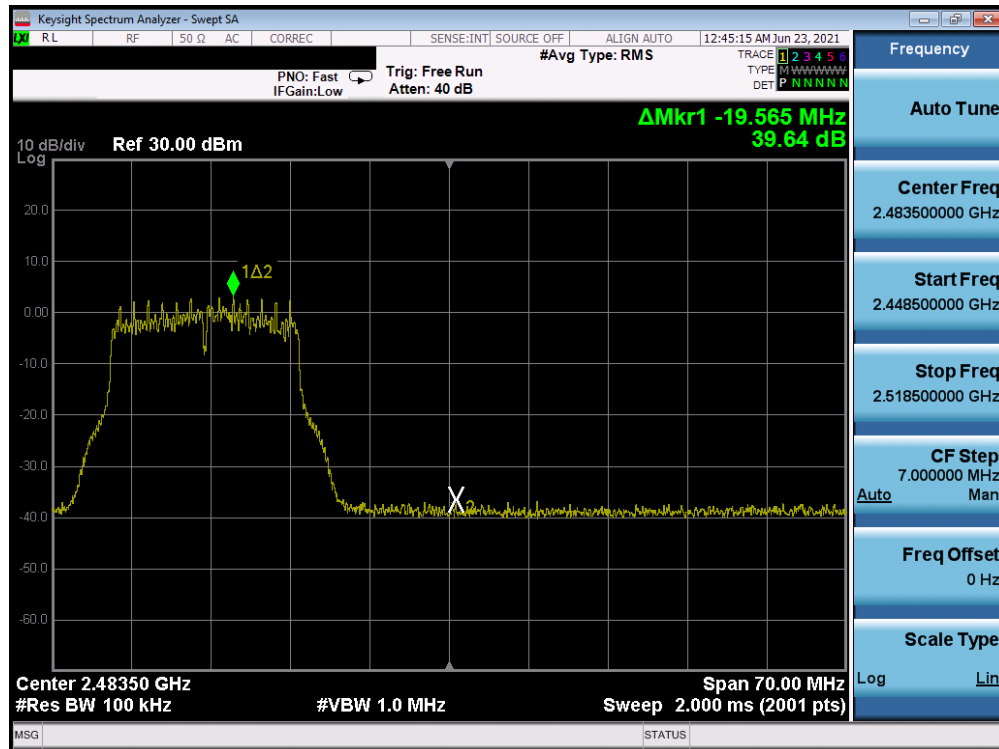
Plot 7-70. Band Edge Plot Antenna B (802.11g- Ch. 11) – 54Mbps
