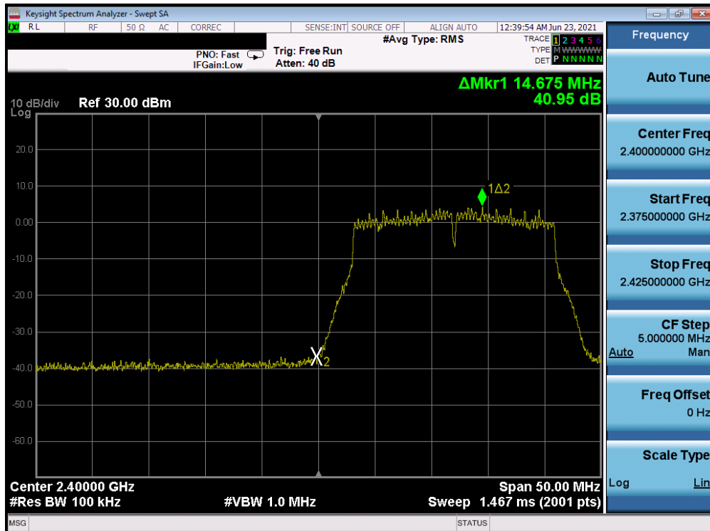
Plot 7-73. Band Edge Plot Antenna B (802.11n (2.4GHz) – Ch. 1) – MCS7
