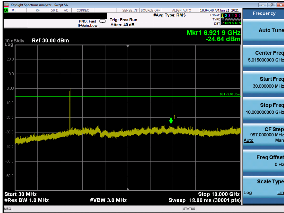
Plot 7-81. Conducted Spurious Plot Antenna A (802.11b – Ch. 6)
