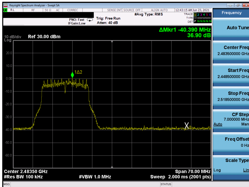
Plot 7-71. Band Edge Plot Antenna B (802.11g- Ch. 12) – 54Mbps
