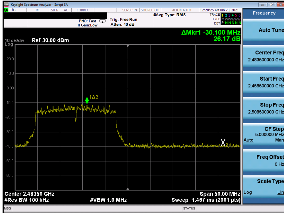
Plot 7-78. Band Edge Plot Antenna B (802.11n (2.4GHz) – Ch. 13) – MCS7
