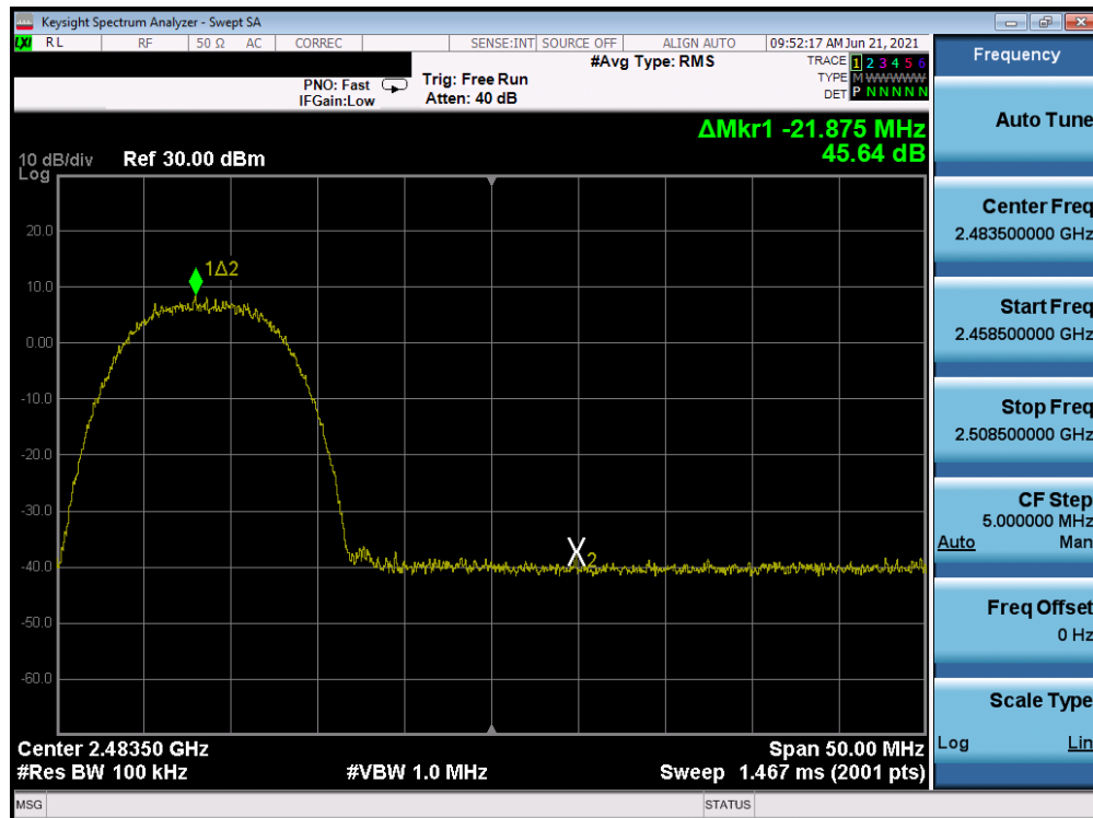
Plot 7-50. Band Edge Plot Antenna A (802.11b – Ch. 12) – 11Mbps
