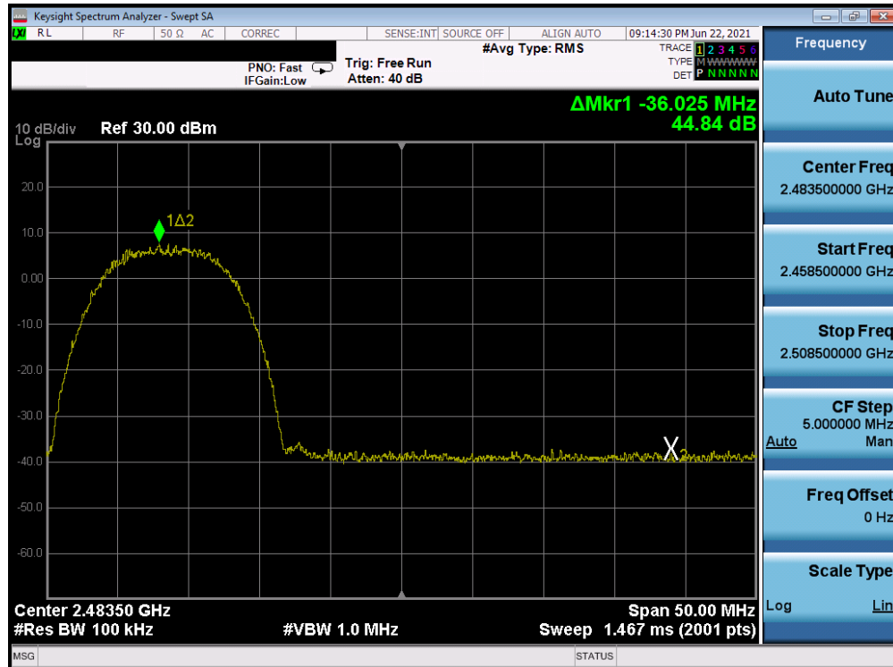
Plot 7-65. Band Edge Plot Antenna B (802.11b – Ch. 12) – 11Mbps
