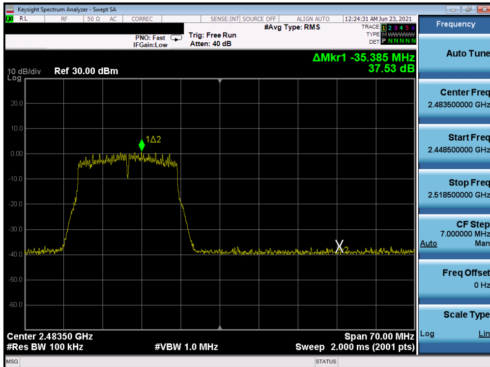
Plot 7-62. Band Edge Plot Antenna A (802.11n (2.4GHz) – Ch. 12) – MCS7
