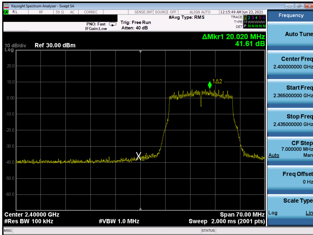
Plot 7-59. Band Edge Plot Antenna A (802.11n (2.4GHz) – Ch. 2) – MCS7
