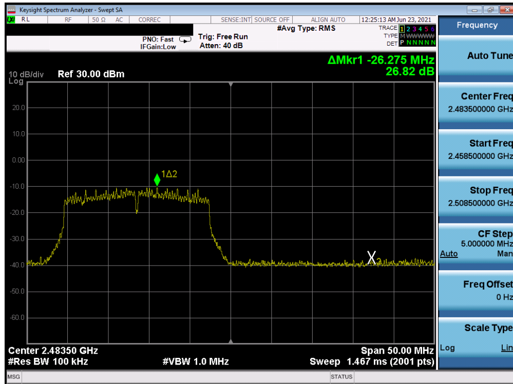
Plot 7-63. Band Edge Plot Antenna A (802.11n (2.4GHz) - Ch. 13) - MCS7
