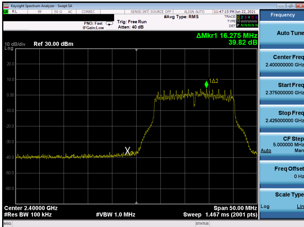
Plot 7-52. Band Edge Plot Antenna A (802.11g– Ch. 1) – 54Mbps
