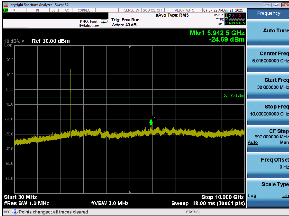
Plot 7-83. Conducted Spurious Plot Antenna A (802.11b – Ch. 11)
