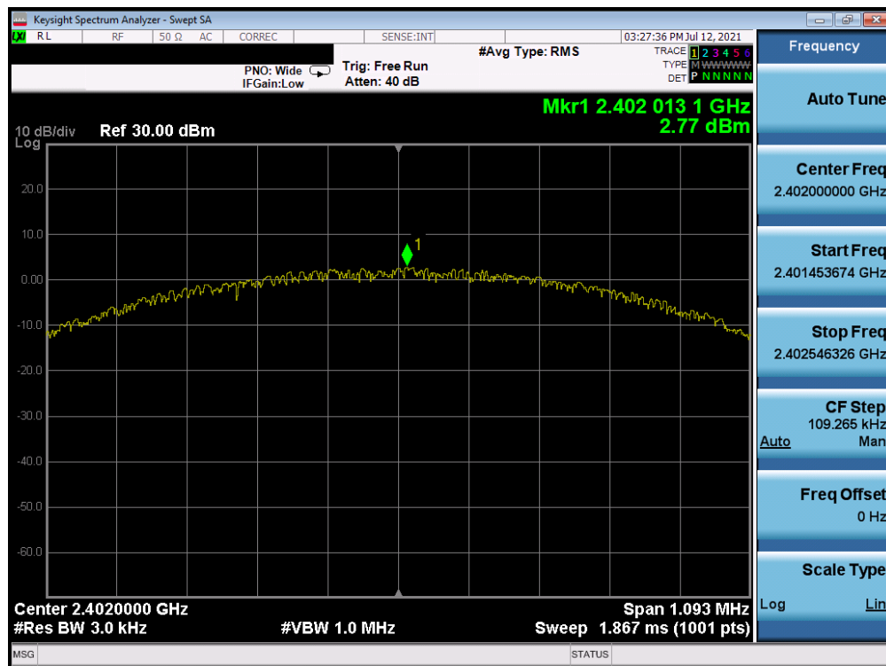
Plot 7-7. Power Spectral Density Plot (Bluetooth (LE), 1Mbps, ePA – Ch. 0, Antenna A)
