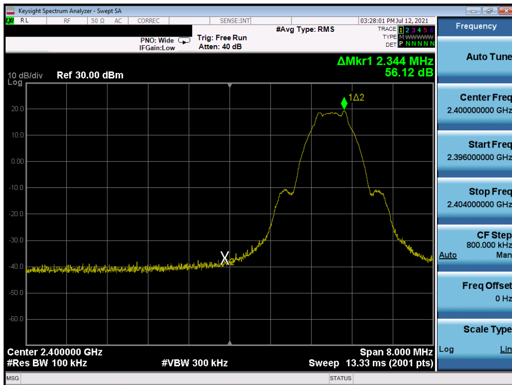
Plot 7-13. Band Edge Plot Antenna A (Bluetooth (LE), 1Mbps, ePA – Ch. 0)
