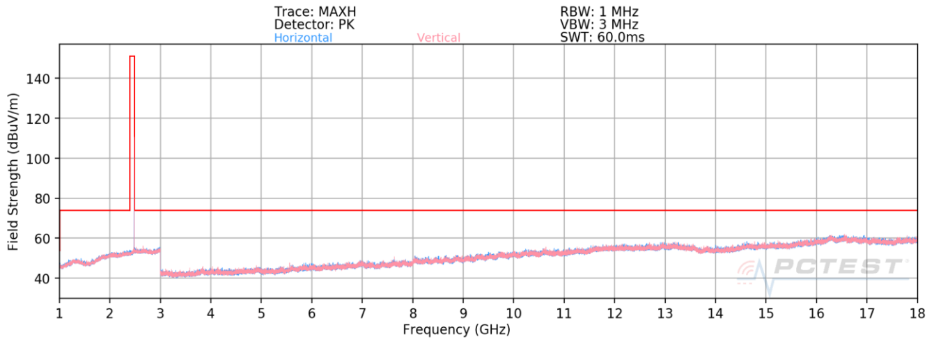
Plot 7-23. Radiated Spurious Emissions Plot Above 1GHz Antenna A (1Mbps ePA – Ch. 39, Ant. Pol. H & V)
