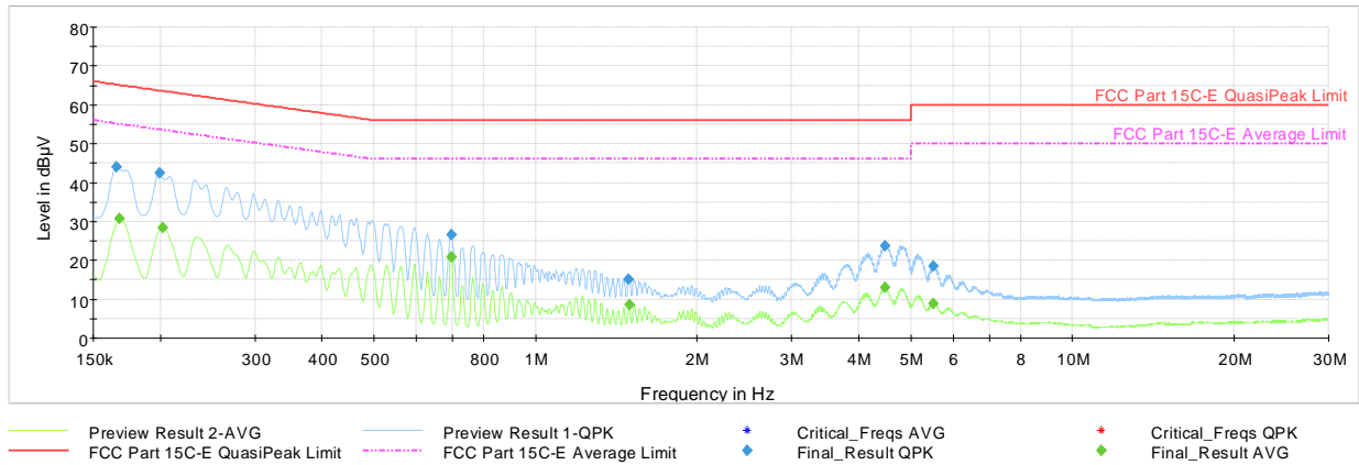
Plot 7-29. AC Line Conducted Plot with Bluetooth LE (1Mbps, ePA – Ch.19, L1, with AC/DC Adapter)
