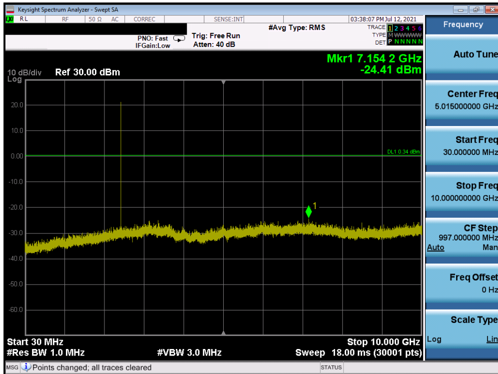
Plot 7-17. Conducted Spurious Plot Antenna A (Bluetooth (LE), 1Mbps, ePA – Ch. 19)
