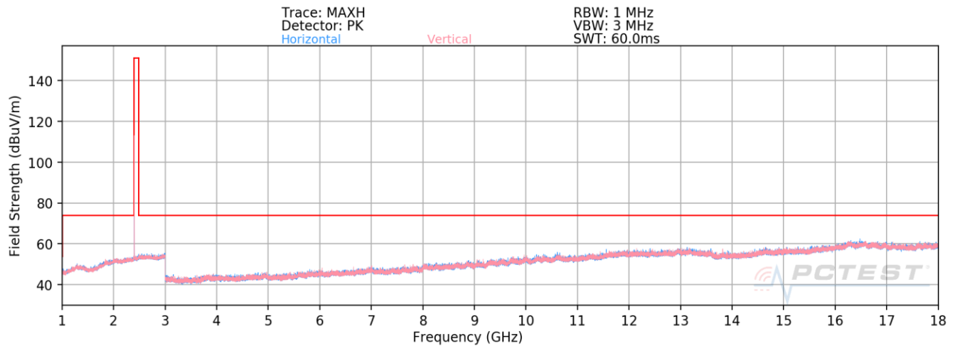
Plot 7-21. Radiated Spurious Emissions Plot Above 1GHz Antenna A (1Mbps, ePA – Ch. 0, Ant. Pol. H & V)
