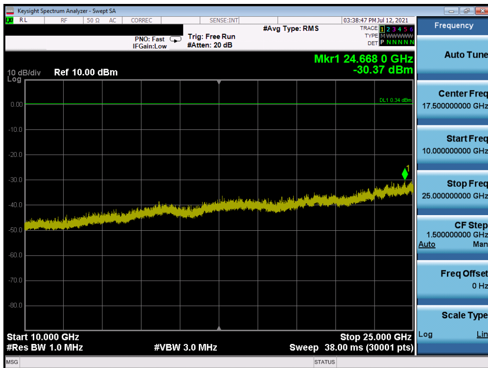
Plot 7-18. Conducted Spurious Plot Antenna A (Bluetooth (LE), 1Mbps, ePA – Ch. 19)
