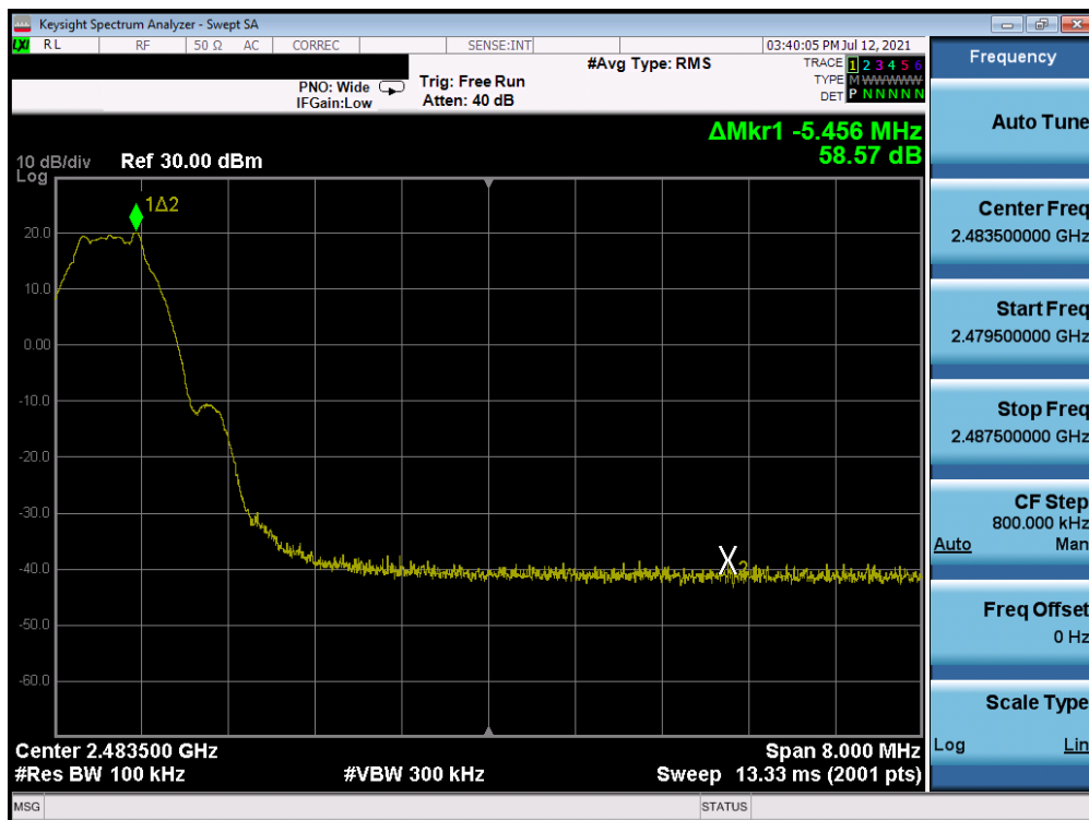
Plot 7-14. Band Edge Plot Antenna A (Bluetooth (LE), 1Mbps, ePA – Ch. 39)
