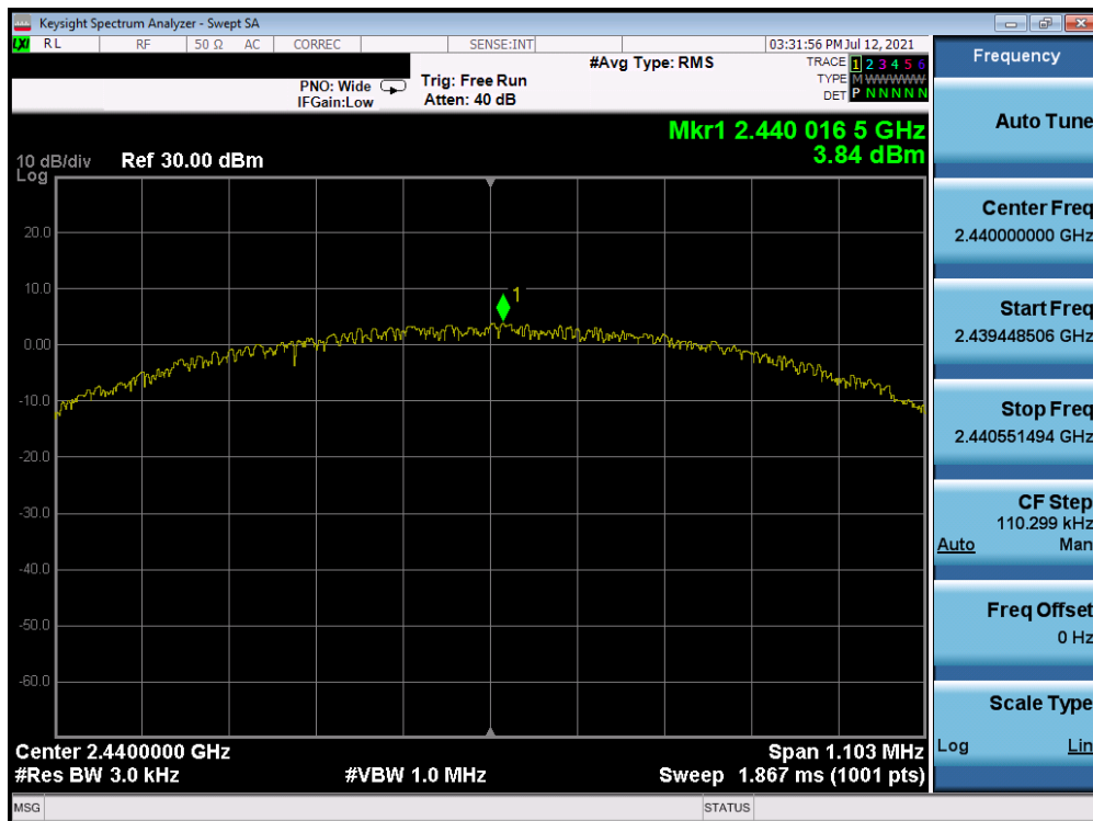
Plot 7-8. Power Spectral Density Plot Antenna A (Bluetooth (LE), 1Mbps, ePA – Ch. 19)
