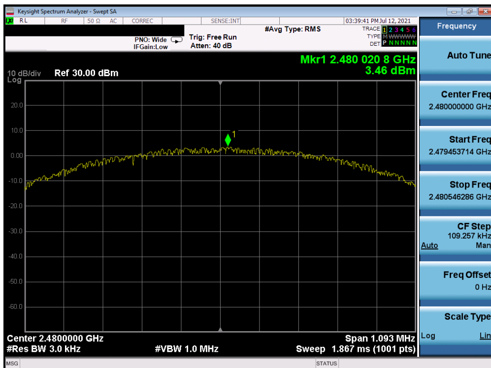
Plot 7-9. Power Spectral Density Plot Antenna A (Bluetooth (LE), 1Mbps, ePA – Ch. 39)
