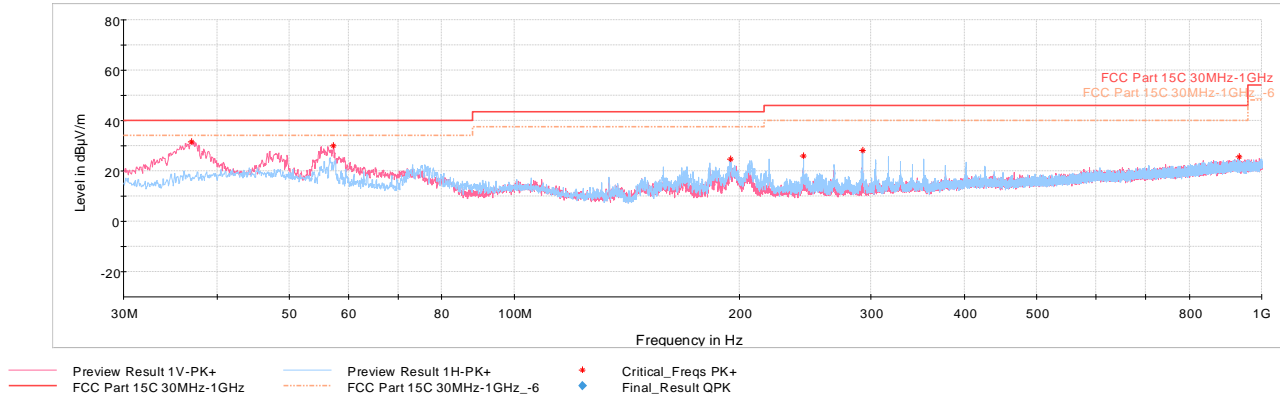
Plot 7-28. Radiated Spurious Emissions Below 1GHz Antenna A (1Mbps, ePA – Ch.19, Pol. H & V, with AC/DC Adapter)
