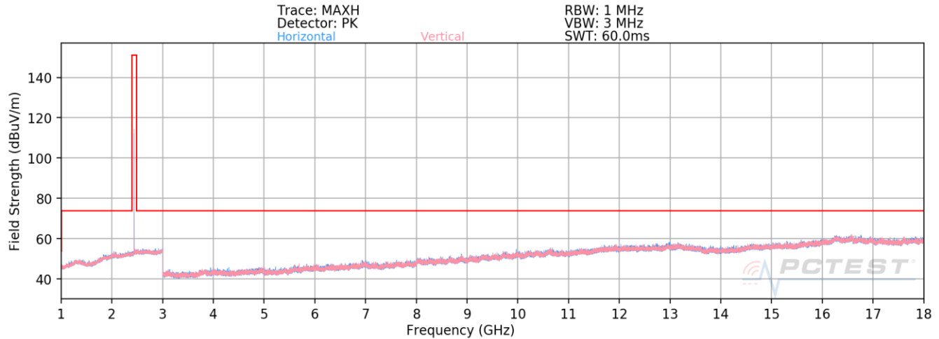
Plot 7-22. Radiated Spurious Emissions Plot Above 1GHz Antenna A (1Mbps, ePA – Ch. 19, Ant. Pol. H & V)
