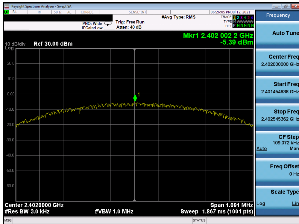
Plot 7-10. Power Spectral Density Plot Antenna A (Bluetooth (LE), 1Mbps, iPA – Ch. 0)
