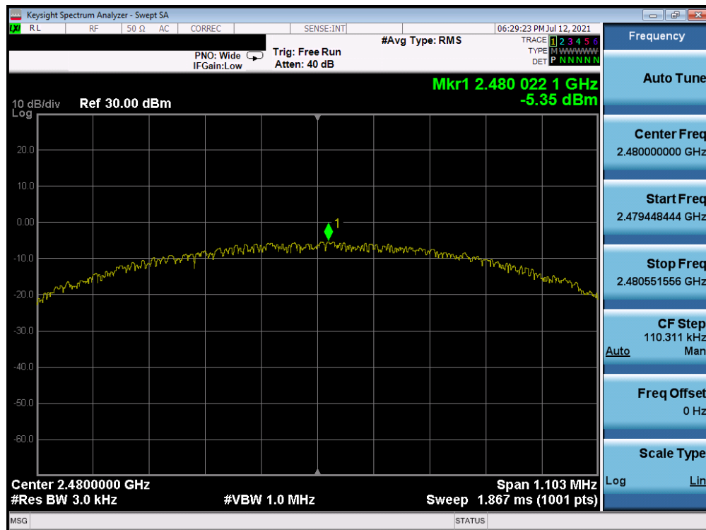
Plot 7-12. Power Spectral Density Plot Antenna A (Bluetooth (LE), 1Mbps, iPA – Ch. 39)
