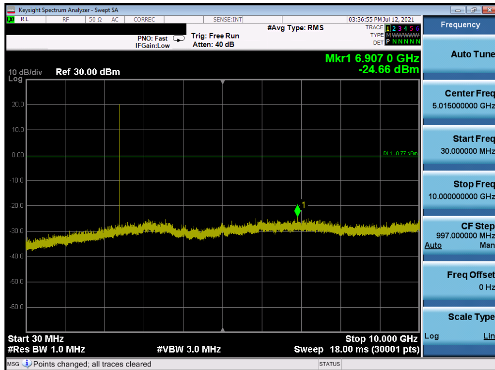
Plot 7-15. Conducted Spurious Plot Antenna A (Bluetooth (LE), 1Mbps, ePA – Ch. 0)
