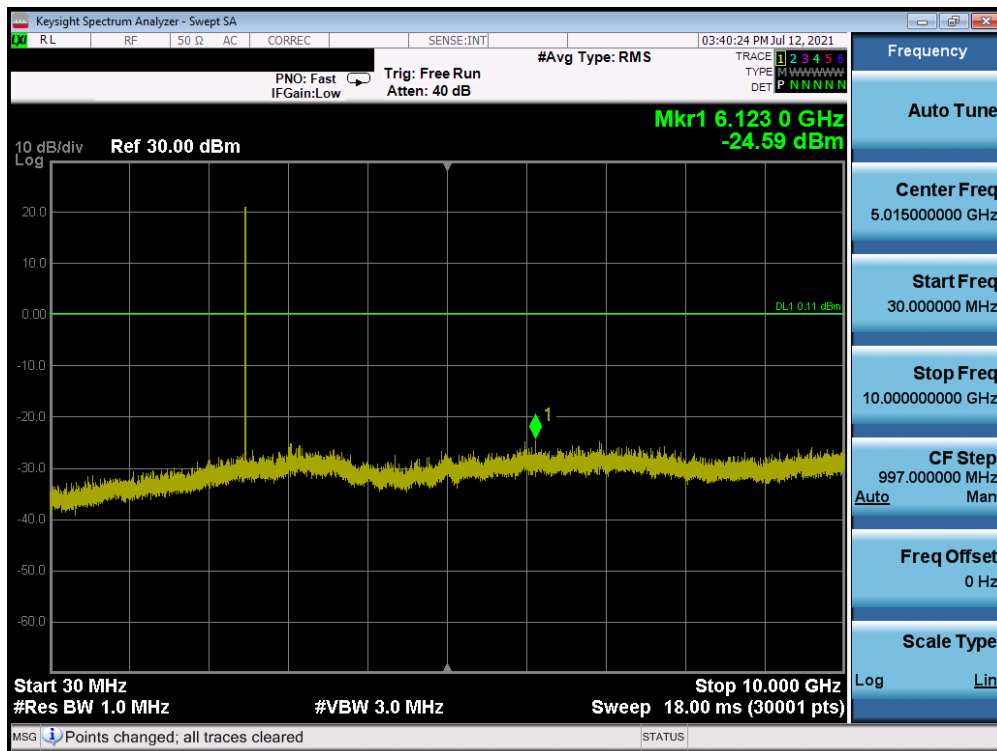
Plot 7-19. Conducted Spurious Plot Antenna A (Bluetooth (LE), 1Mbps, ePA – Ch. 39)
