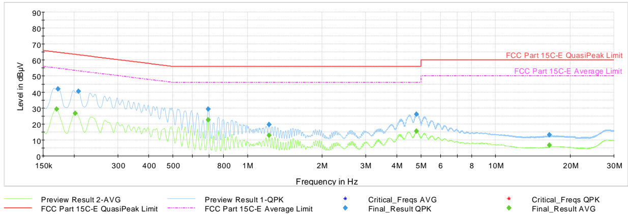
Plot 7-30. AC Line Conducted Plot with Bluetooth LE (1Mbps, ePA – Ch.19, N, with AC/DC Adapter)
