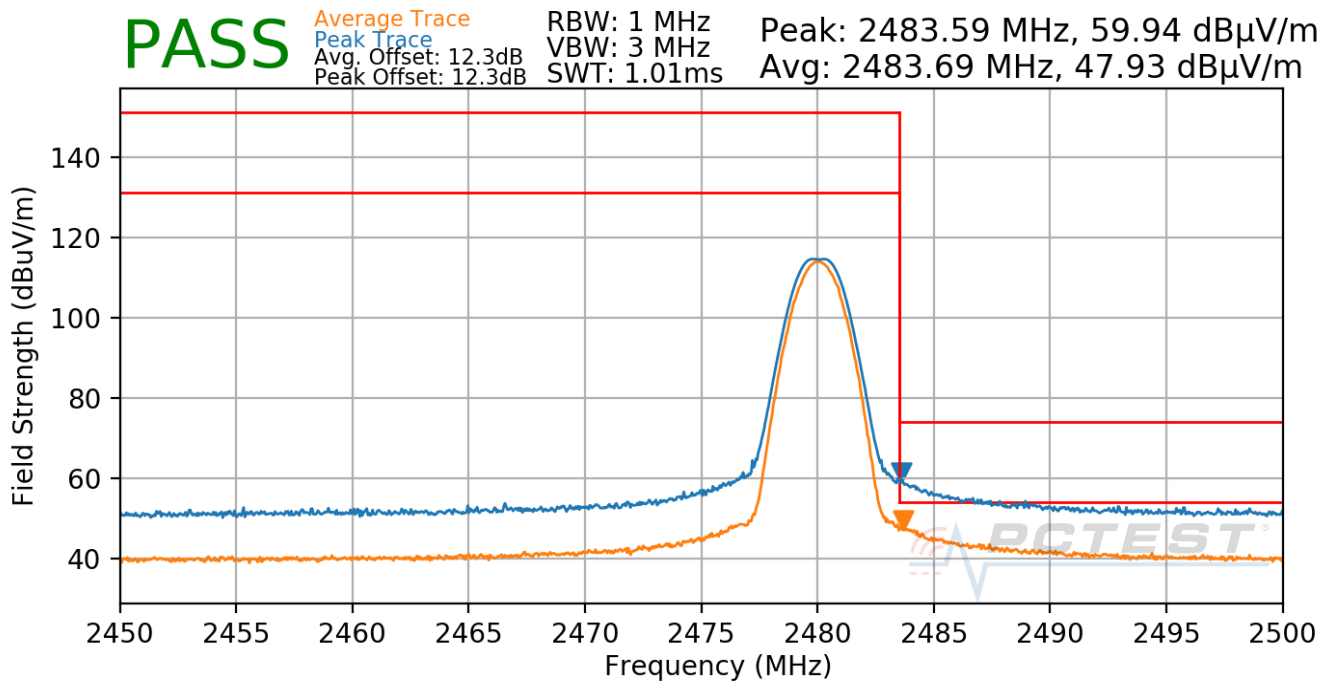
Plot 7-27. Radiated Restricted Upper Band Edge Measurement Antenna A (Average & Peak)
