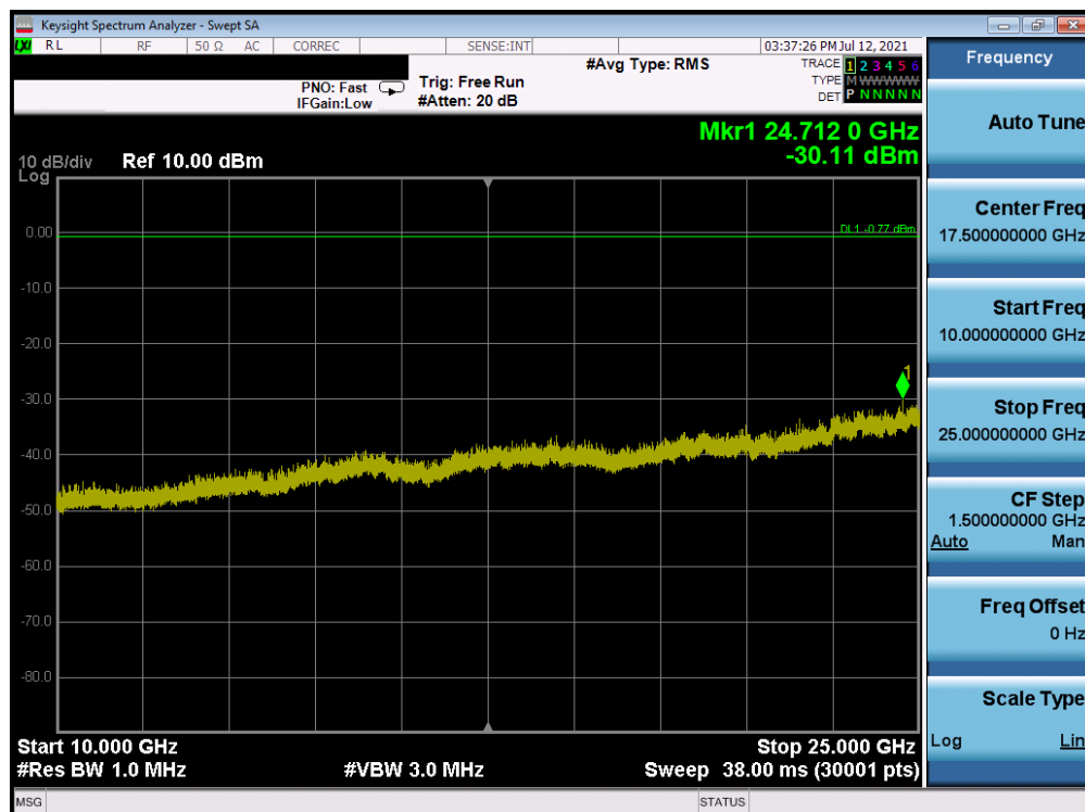
Plot 7-16. Conducted Spurious Plot Antenna A (Bluetooth (LE), 1Mbps, ePA – Ch. 0)
