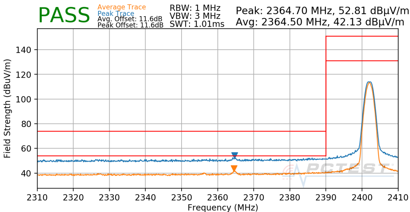
Plot 7-26. Radiated Restricted Lower Band Edge Measurement Antenna A (Average & Peak)
