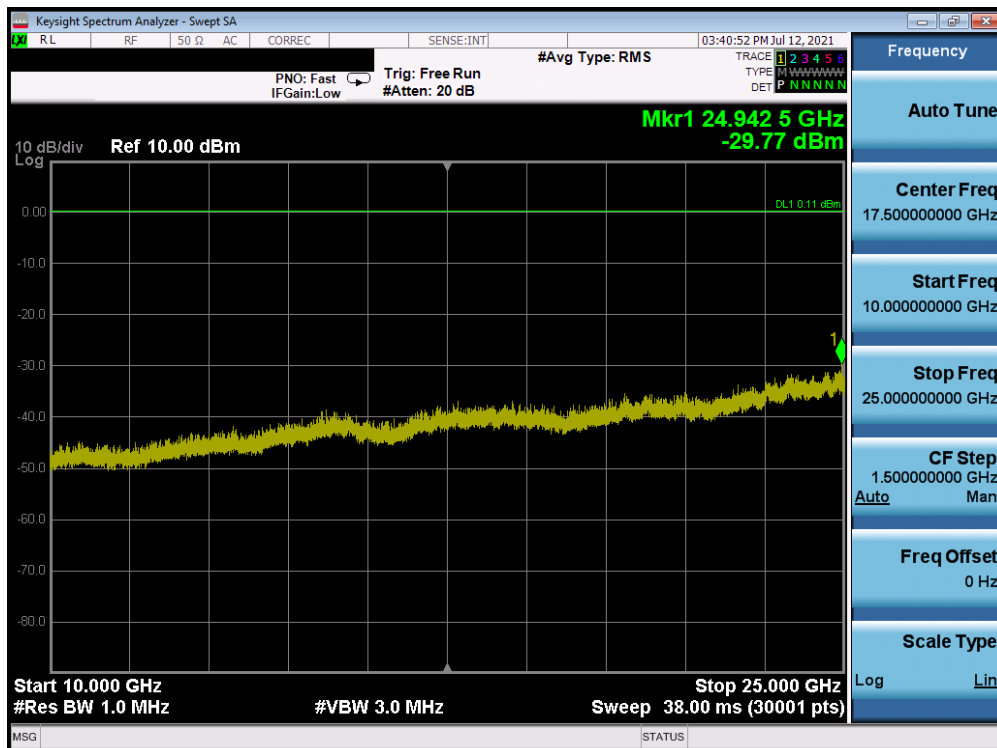
Plot 7-20. Conducted Spurious Plot Antenna A (Bluetooth (LE), 1Mbps, ePA – Ch. 39)
