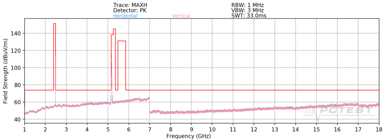
Plot 7-34. Radiated Spurious Emissions Above 1GHz Simultaneous Tx
