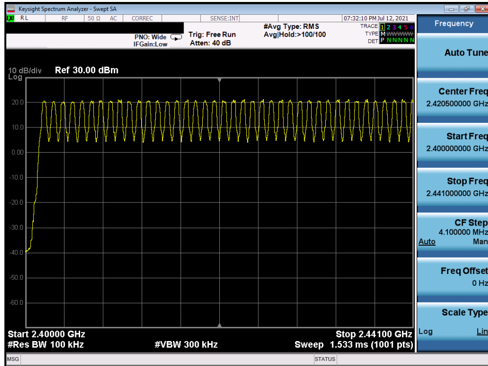
Plot 7-19. Low End Spectrum Channel Hopping Plot Antenna A (Bluetooth, GFSK, ePA)
