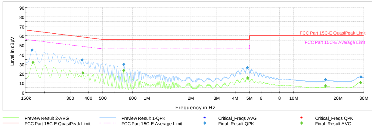
Plot 7-43. AC Line-Conducted Test Plot Antenna A (N, GFSK ePA – Ch.39, with AC/DC Adapter)
