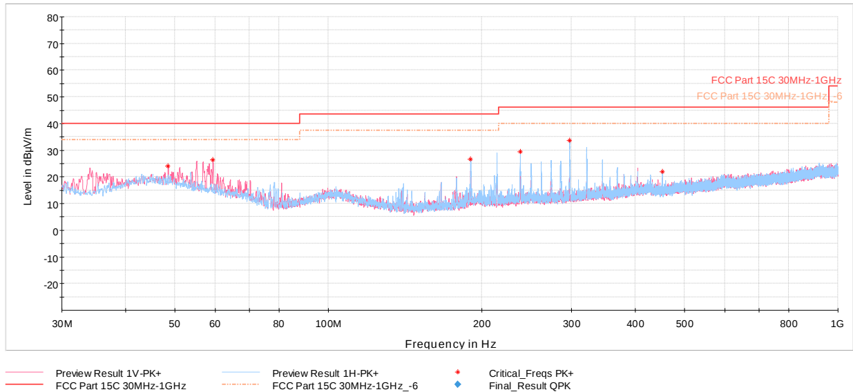
Plot 7-41. Radiated Spurious Emissions Below 1GHz Antenna A (GFSK ePA – Ch.39, with AC/DC Adapter)
