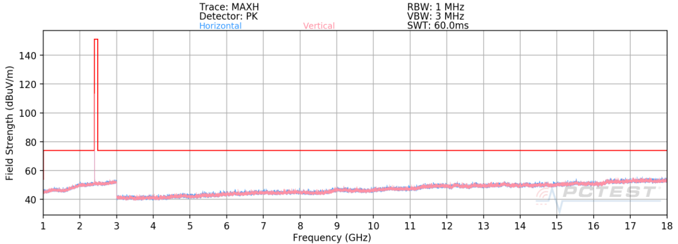
Plot 7-29. Radiated Spurious Emissions Above 1GHz Antenna A (BT GFSK ePA – Ch. 0)
