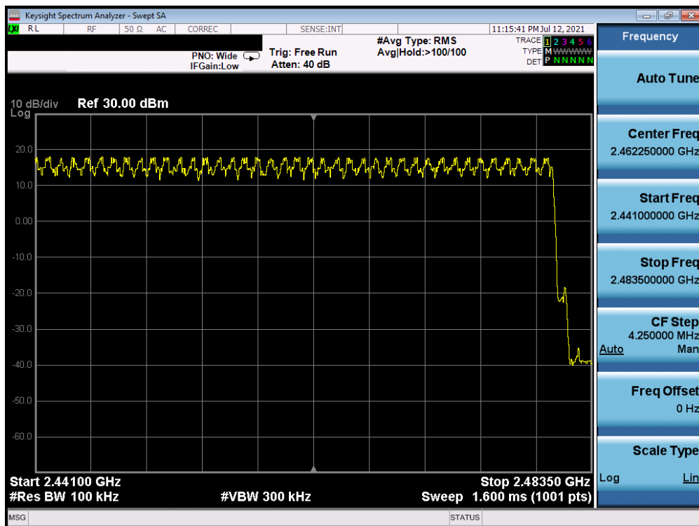
Plot 7-22. High End Spectrum Channel Hopping Plot Antenna A (Bluetooth, 8DPSK, ePA)
