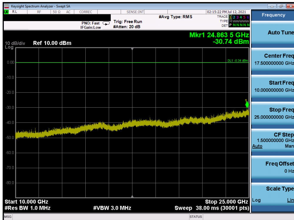
Plot 7-24. Conducted Spurious Plot Antenna A (Bluetooth, GFSK, ePA – Ch. 0)
