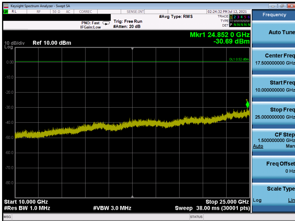
Plot 7-28. Conducted Spurious Plot Antenna A (Bluetooth, GFSK, ePA – Ch. 78)
