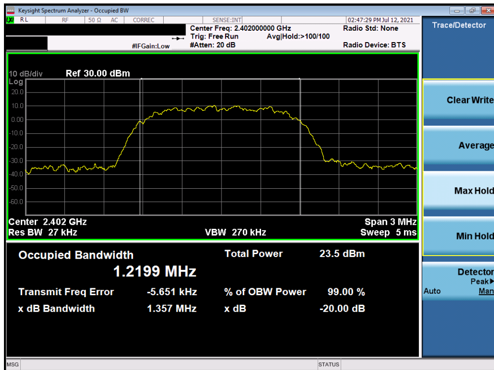
Plot 7-4. 20dB BW and 99% OBW Plot Antenna A (Bluetooth, 8DPSK, ePA – Ch. 0)
