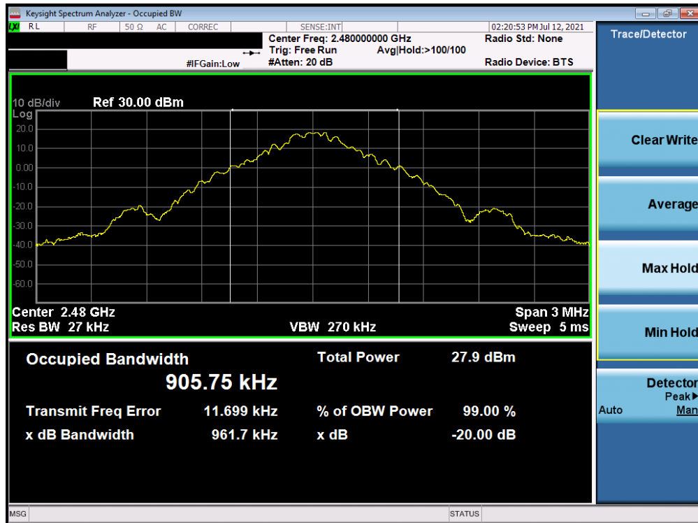
Plot 7-3. 20dB BW and 99% OBW Plot Antenna A (Bluetooth, GFSK, ePA – Ch. 78)
