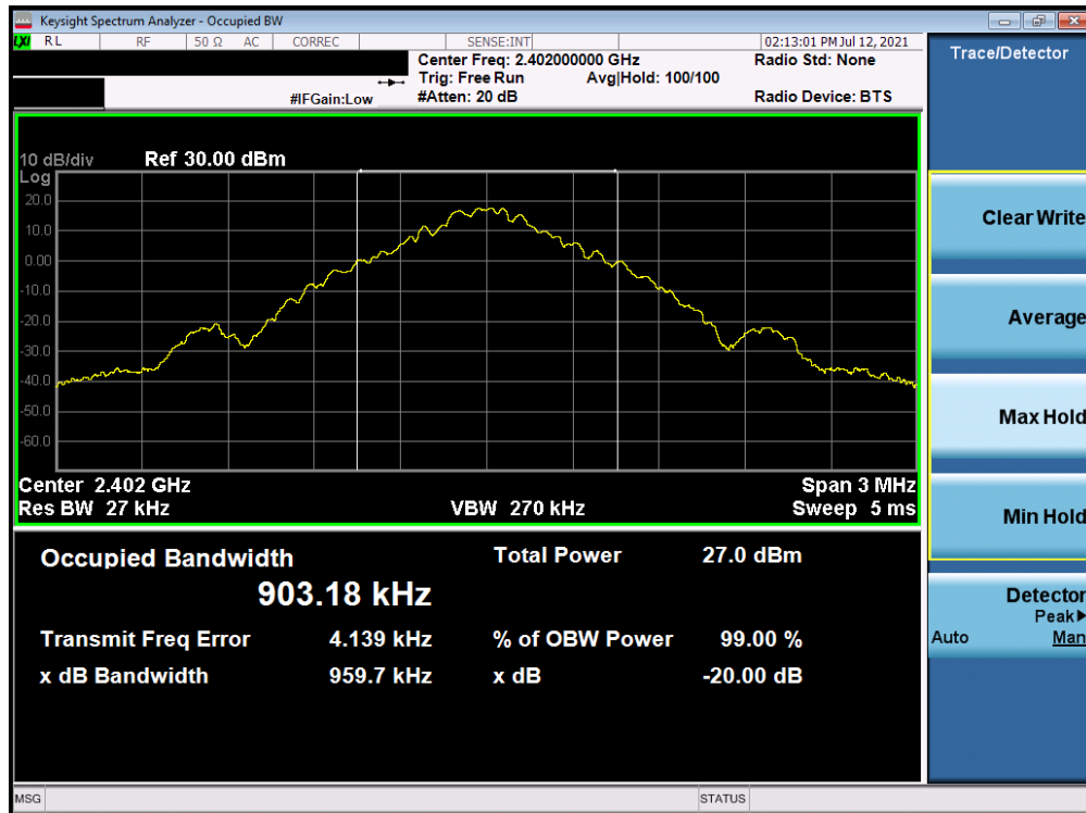
Plot 7-1. 20dB BW and 99% OBW Plot Antenna A (Bluetooth, GFSK, ePA – Ch. 0)
