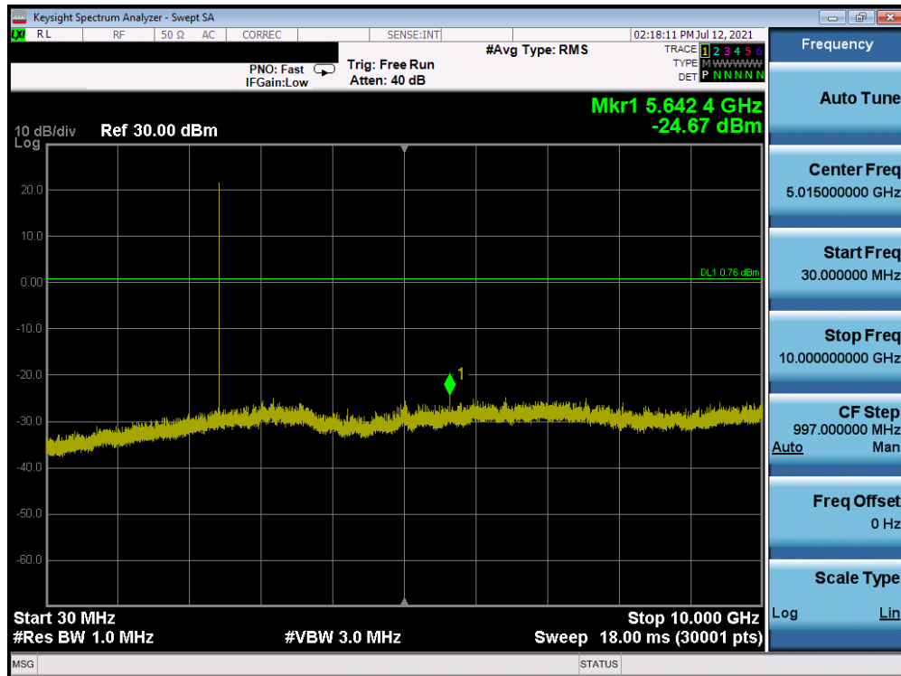
Plot 7-25. Conducted Spurious Plot Antenna A (Bluetooth, GFSK, ePA – Ch. 39)
