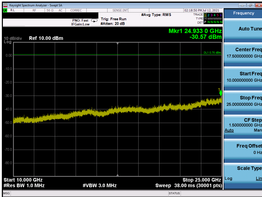
Plot 7-26. Conducted Spurious Plot Antenna A (Bluetooth, GFSK, ePA Ch. 39)
