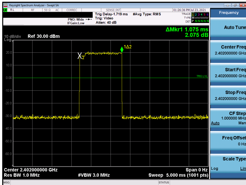
Plot 7-18. Time of Occupancy Plot Antenna A (Bluetooth, 8DPSK, ePA)
