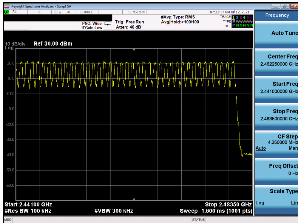
Plot 7-20. High End Spectrum Channel Hopping Plot Antenna A (Bluetooth, GFSK, ePA)
