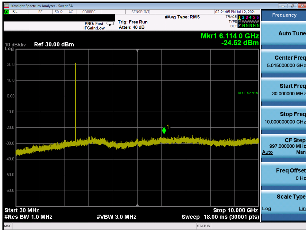
Plot 7-27. Conducted Spurious Plot Antenna A (Bluetooth, GFSK, ePA – Ch. 78)
