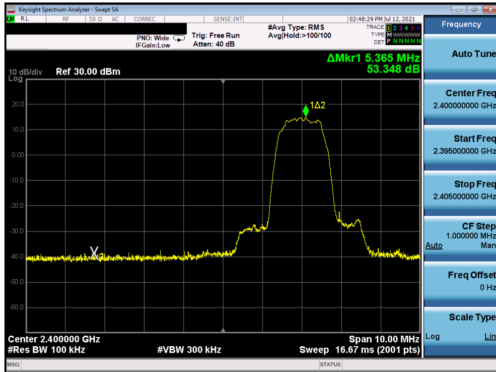
Plot 7-11. Band Edge Plot Antenna A (Bluetooth with Hopping Disabled, 8DPSK, ePA – Ch. 0)
