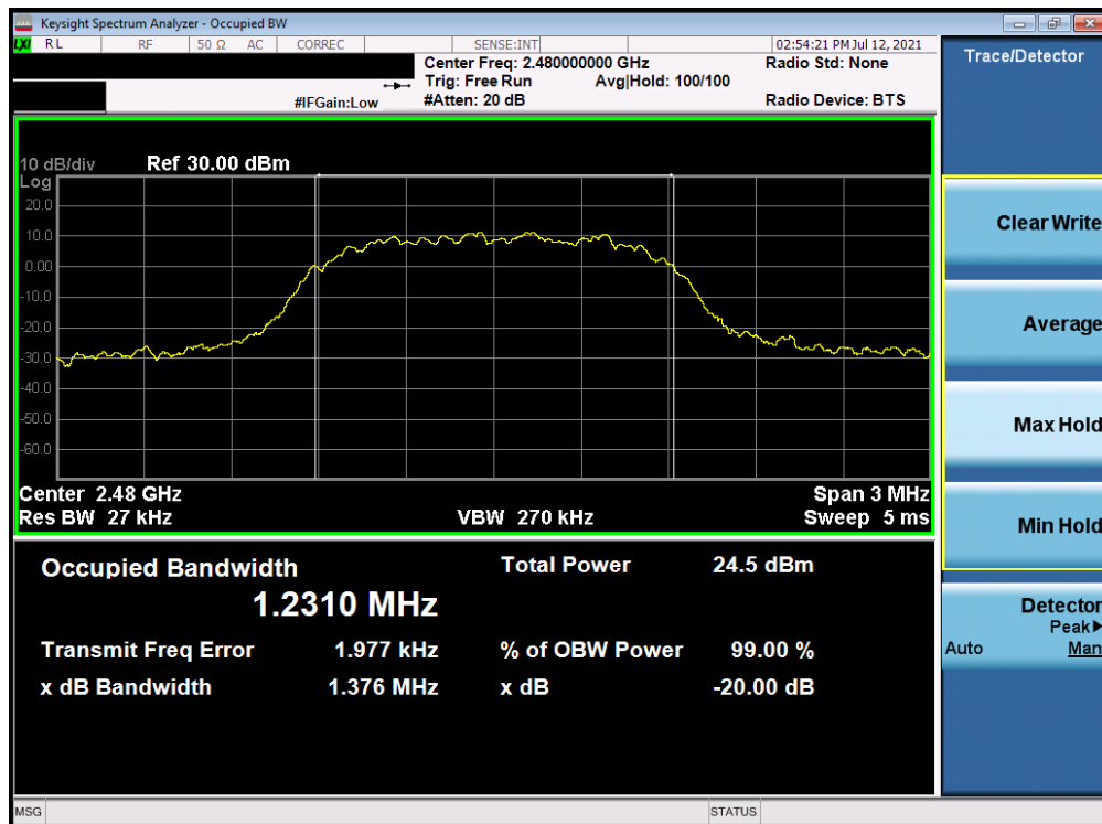
Plot 7-6. 20dB BW and 99% OBW Plot Antenna A (Bluetooth, 8DPSK, ePA – Ch. 78)
