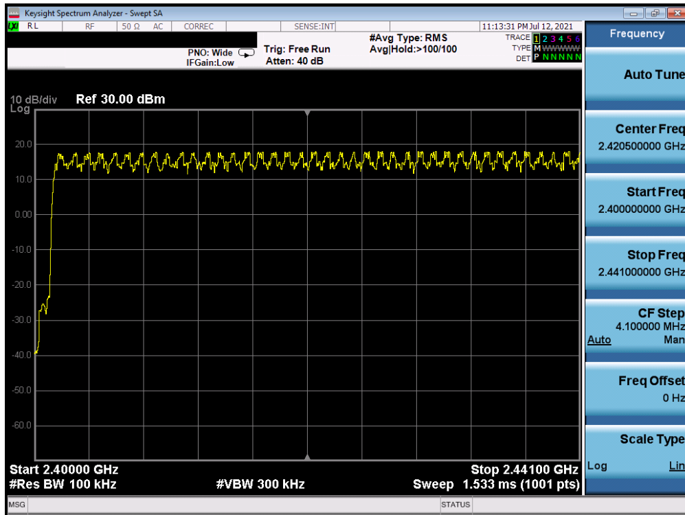
Plot 7-21. Low End Spectrum Channel Hopping Plot Antenna A (Bluetooth, 8DPSK, ePA)
