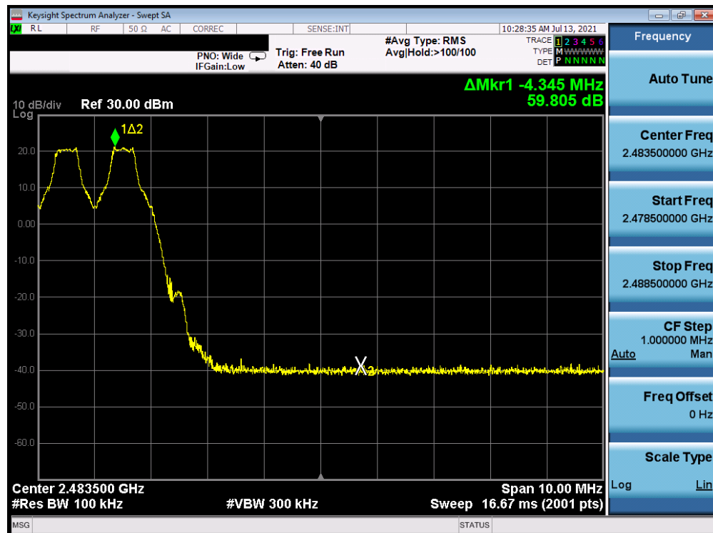
Plot 7-10. Band Edge Plot Antenna A (Bluetooth with Hopping Enabled, GFSK, ePA)
