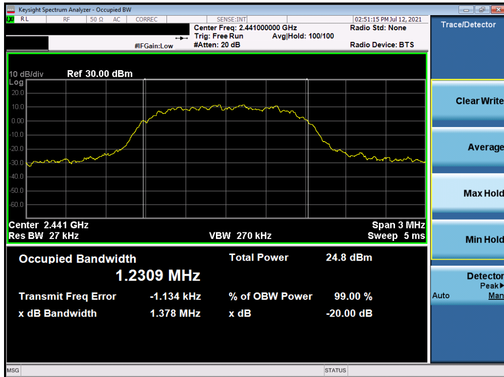
Plot 7-5. 20dB BW and 99% OBW Plot Antenna A (Bluetooth, 8DPSK, ePA – Ch. 39)
