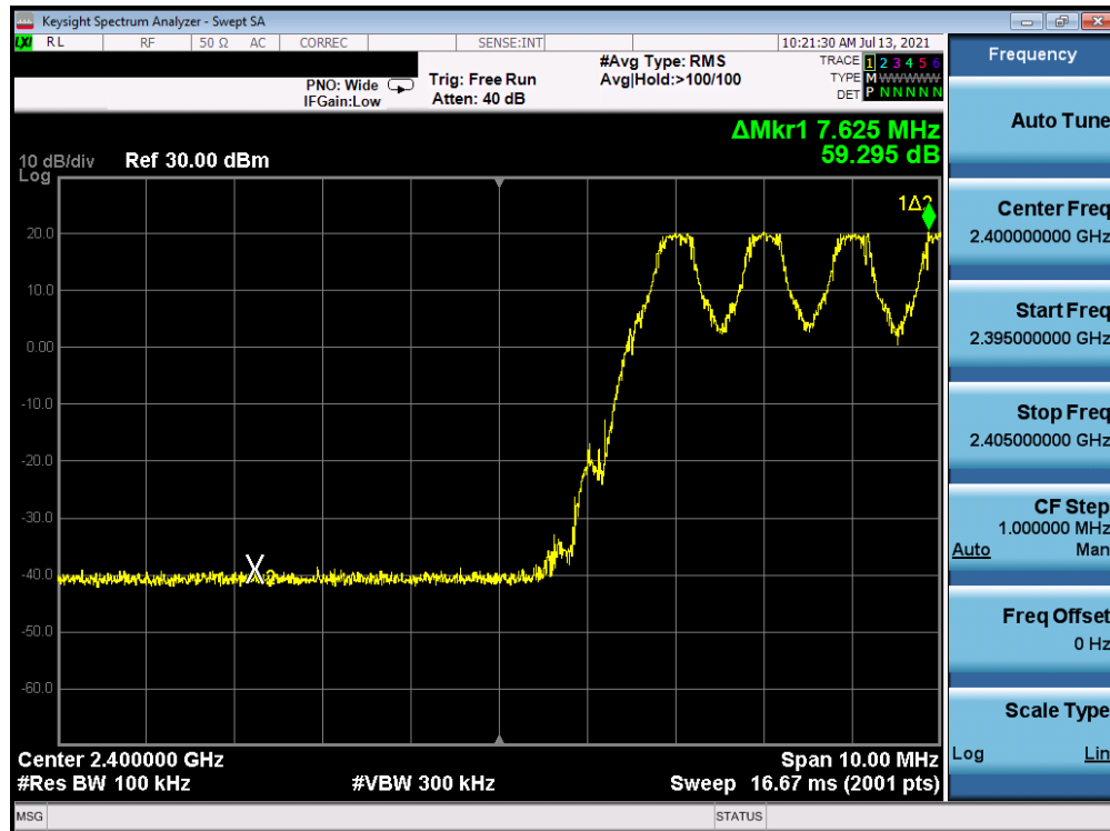
Plot 7-9. Band Edge Plot Antenna A (Bluetooth with Hopping Enabled, GFSK, ePA)
