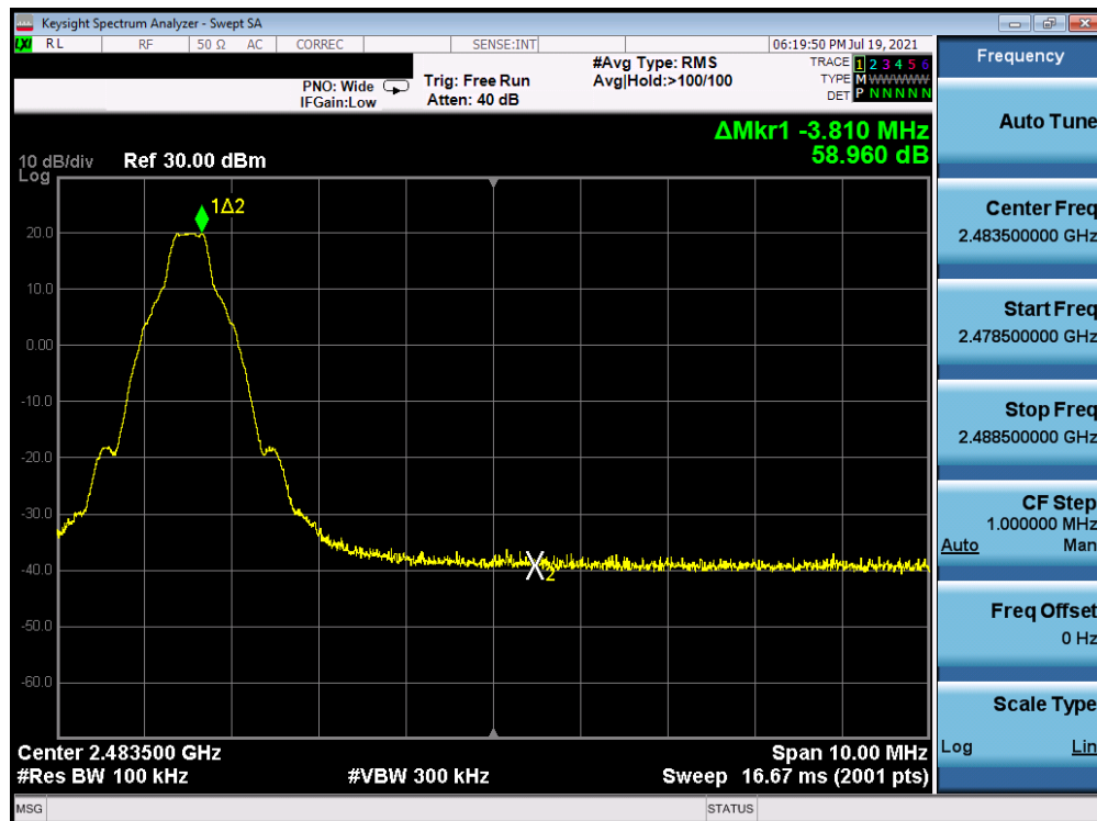
Plot 7-8. Band Edge Plot Antenna A (Bluetooth with Hopping Disabled, GFSK, ePA – Ch. 78)
