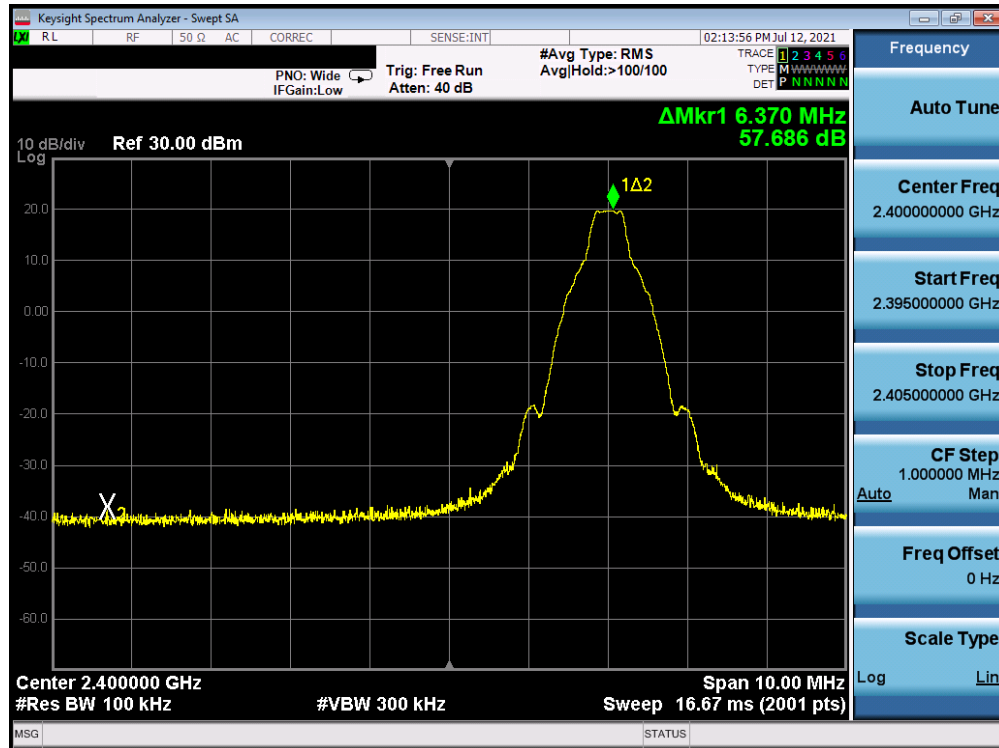
Plot 7-7. Band Edge Plot Antenna A (Bluetooth with Hopping Disabled, GFSK, ePA – Ch. 0)
