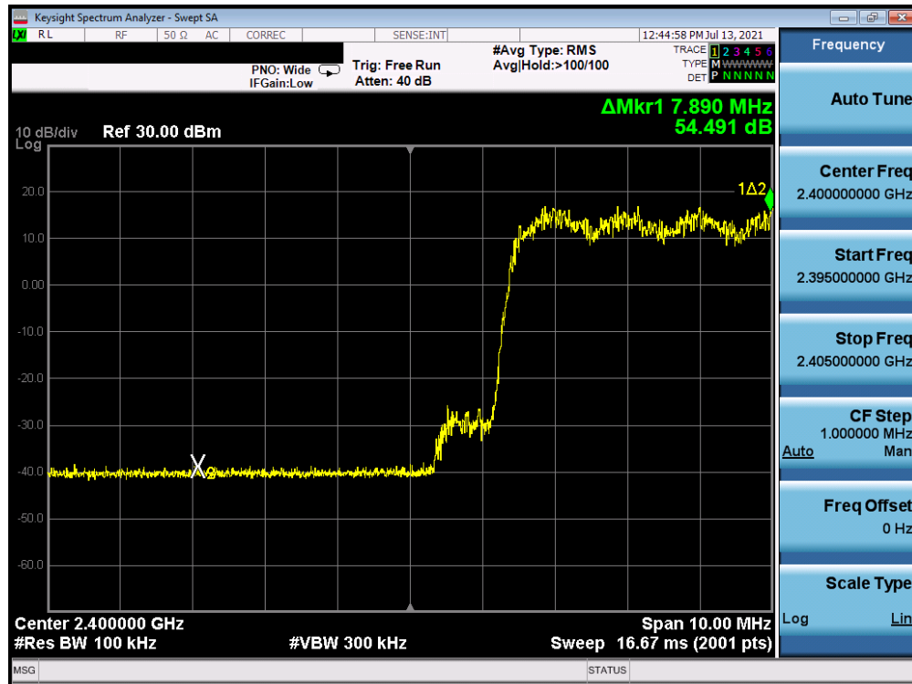
Plot 7-13. Band Edge Plot Antenna A (Bluetooth with Hopping Enabled, 8DPSK, ePA)
