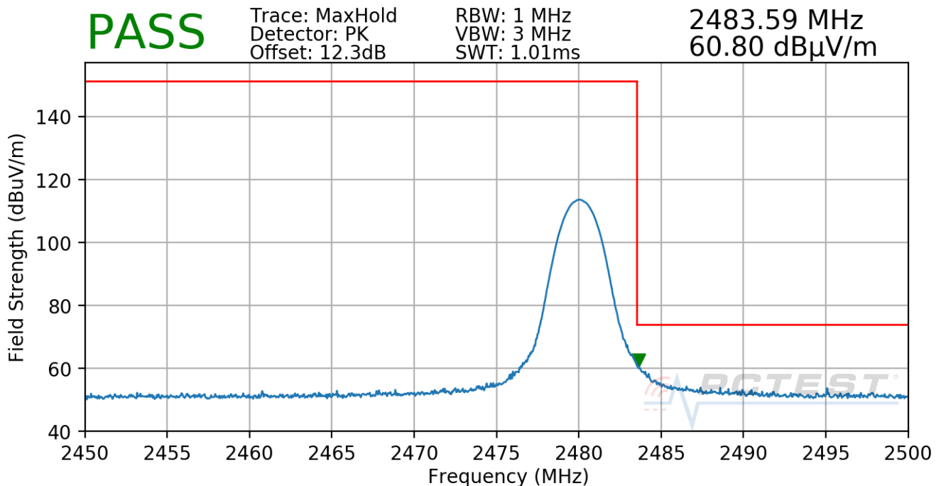
Plot 7-40. Radiated Restricted Upper Band Edge Measurement Antenna A (Average & Peak)
