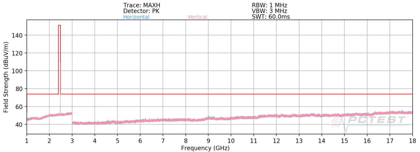
Plot 7-31. Radiated Spurious Emissions Above 1GHz Antenna A (BT GFSK ePA – Ch. 78)
