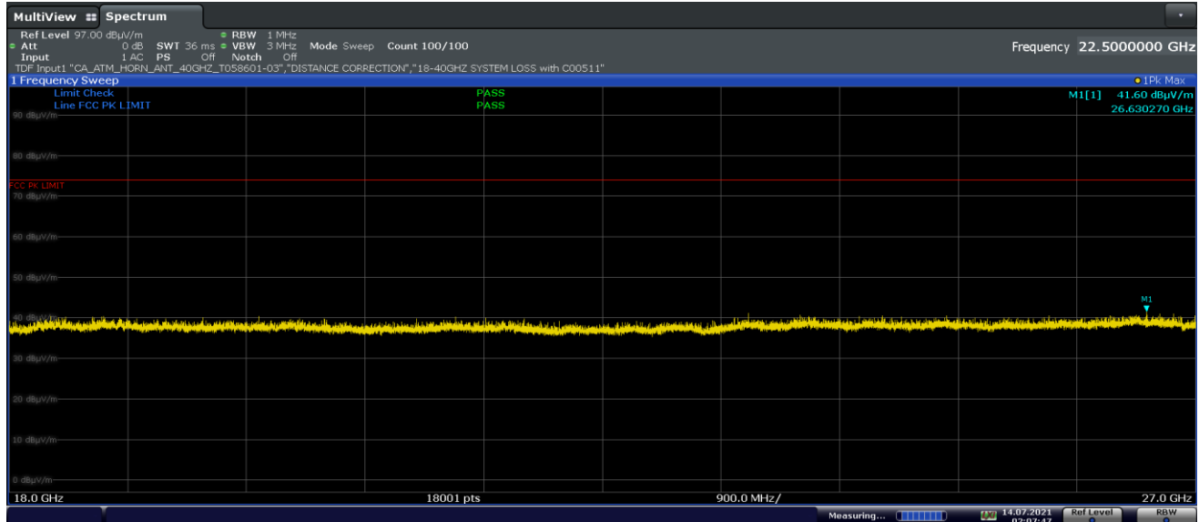
Plot 7-33. Radiated Spurious Emissions Above 18GHz Antenna A (GFSK ePA – Ch.39, Pol. V)
