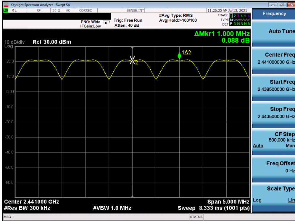
Plot 7-15. Channel Spacing Plot Antenna A (Bluetooth, GFSK, ePA)
