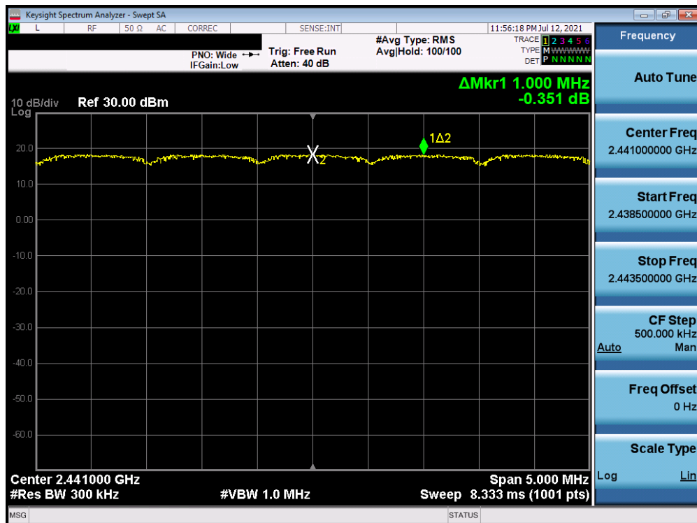
Plot 7-16. Channel Spacing Plot Antenna A (Bluetooth, 8DPSK, ePA)
