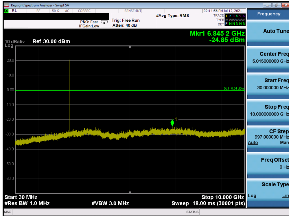
Plot 7-23. Conducted Spurious Plot Antenna A (Bluetooth, GFSK, ePA – Ch. 0)
