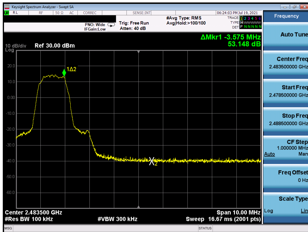
Plot 7-12. Band Edge Plot Antenna A (Bluetooth with Hopping Disabled, 8DPSK, ePA – Ch. 78)
