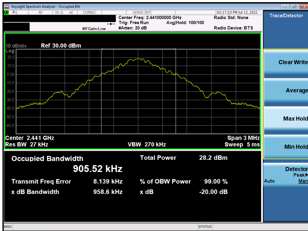
Plot 7-2. 20dB BW and 99% OBW Plot Antenna A (Bluetooth, GFSK, ePA – Ch. 39)
