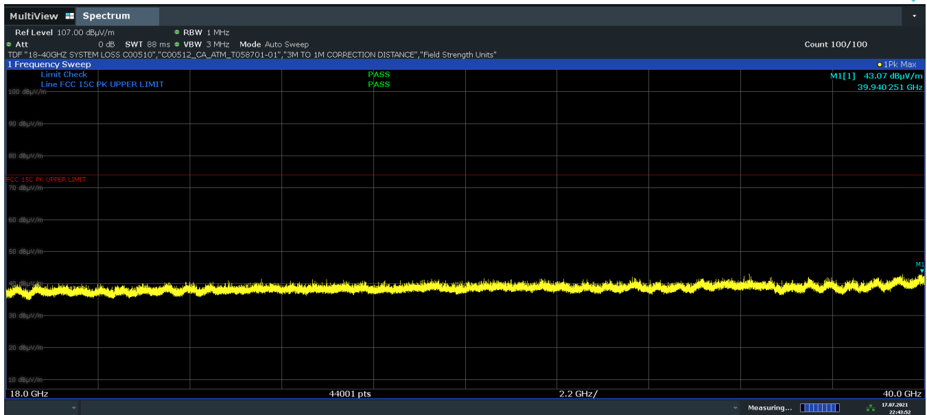
Plot 7-35. Radiated Spurious Emissions Simultaneous Tx 18-40GHz Pol. H
