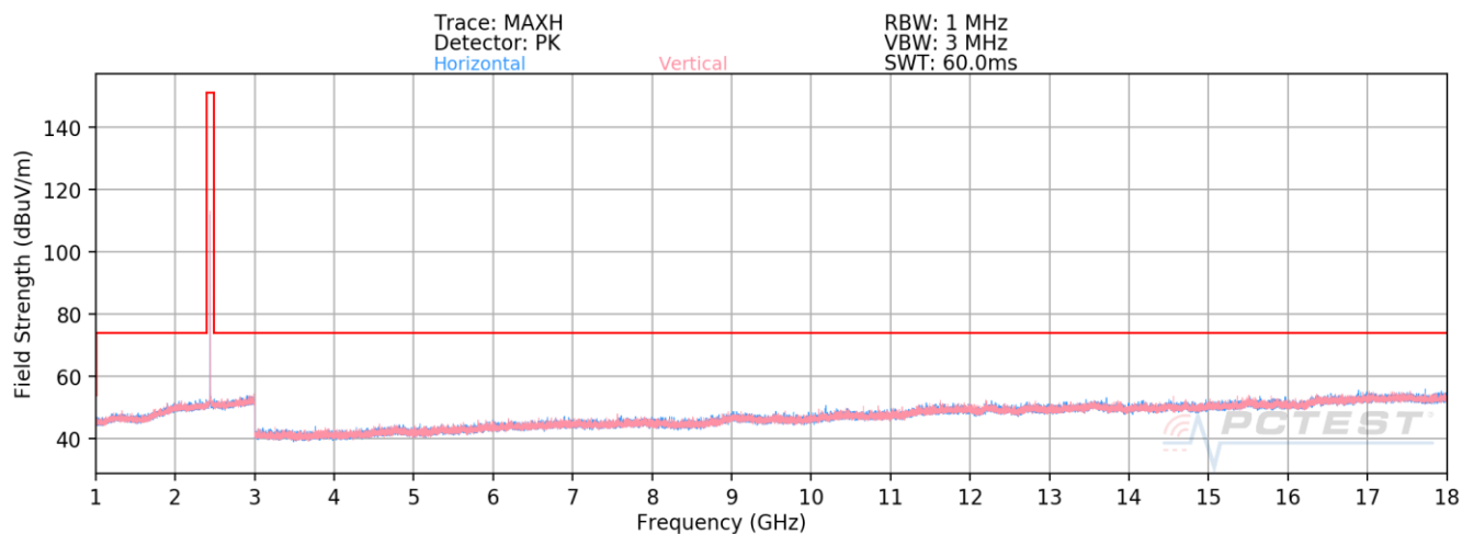
Plot 7-30. Radiated Spurious Emissions Above 1GHz Antenna A (BT GFSK ePA – Ch. 39)
