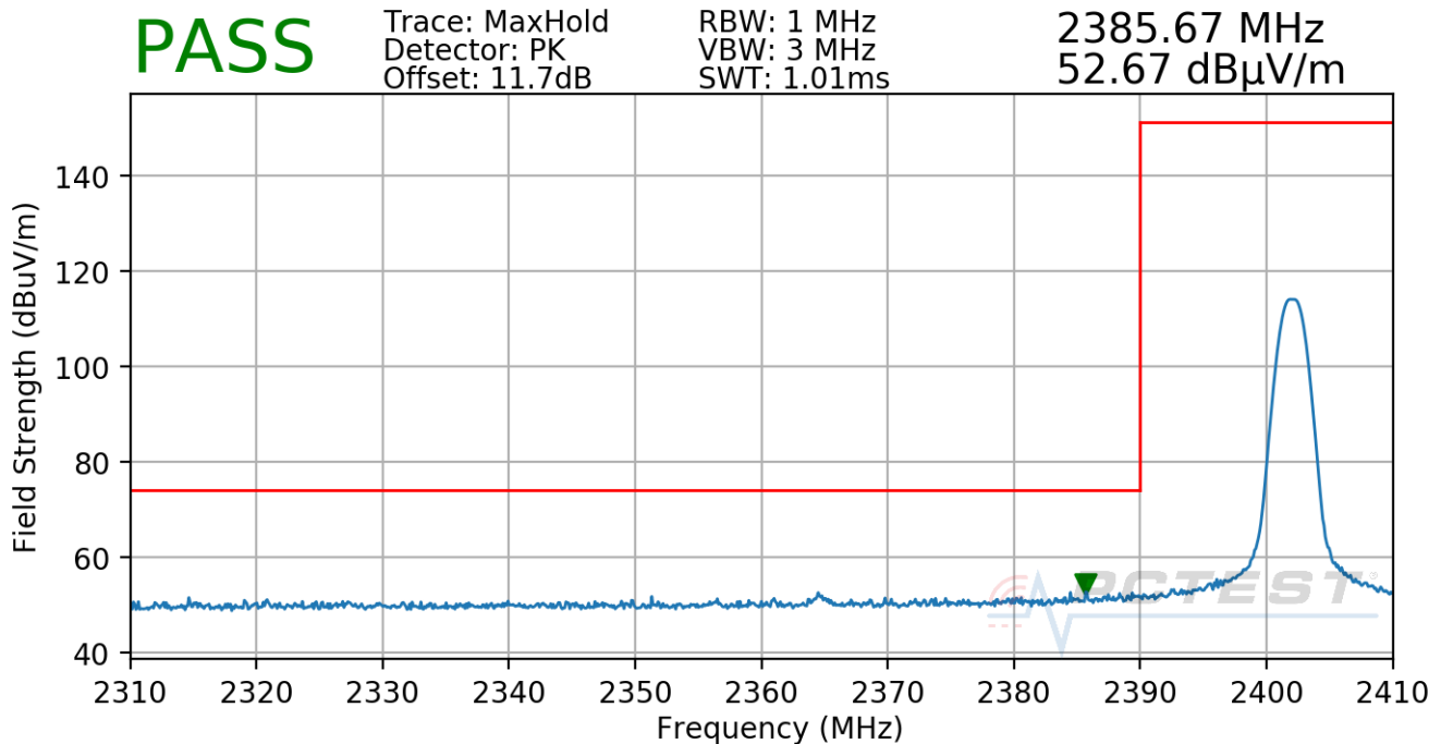
Plot 7-37. Radiated Restricted Lower Band Edge Measurement Antenna A (Average & Peak)
