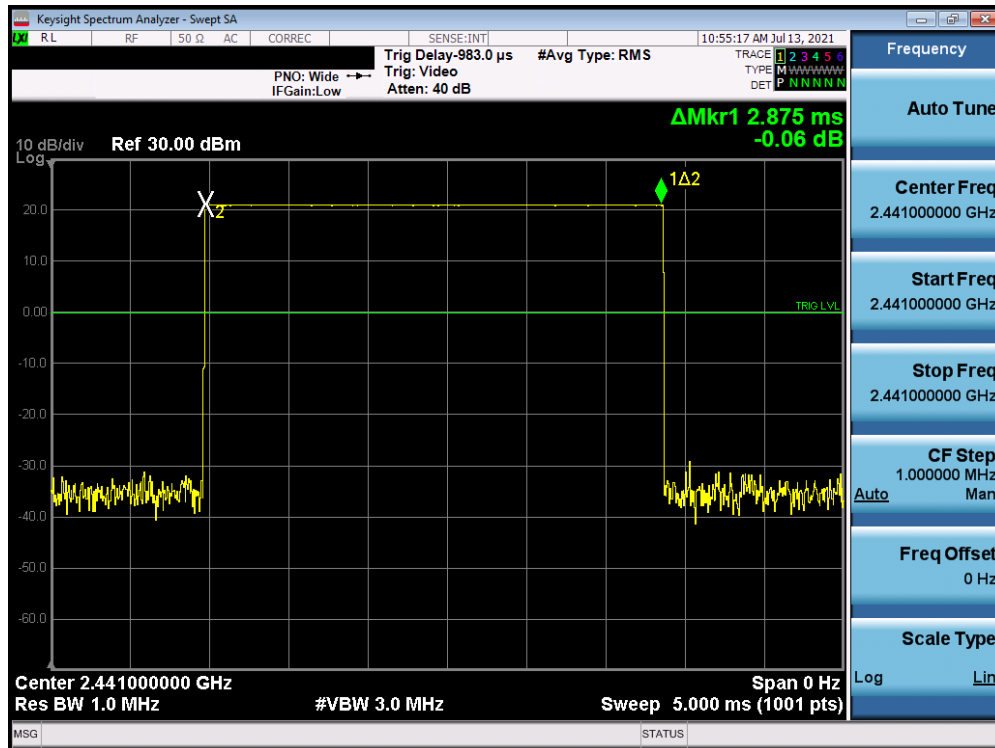
Plot 7-17. Time of Occupancy Plot Antenna A (Bluetooth, GFSK, ePA)
