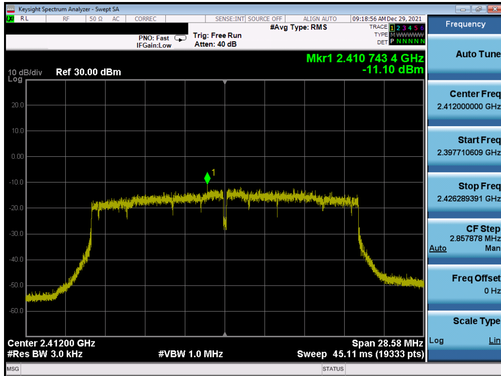
Plot 7-76. Power Spectral Density Plot Antenna 3a (802.11ax (SU - 2.4GHz) – Ch. 1) – MCS3
