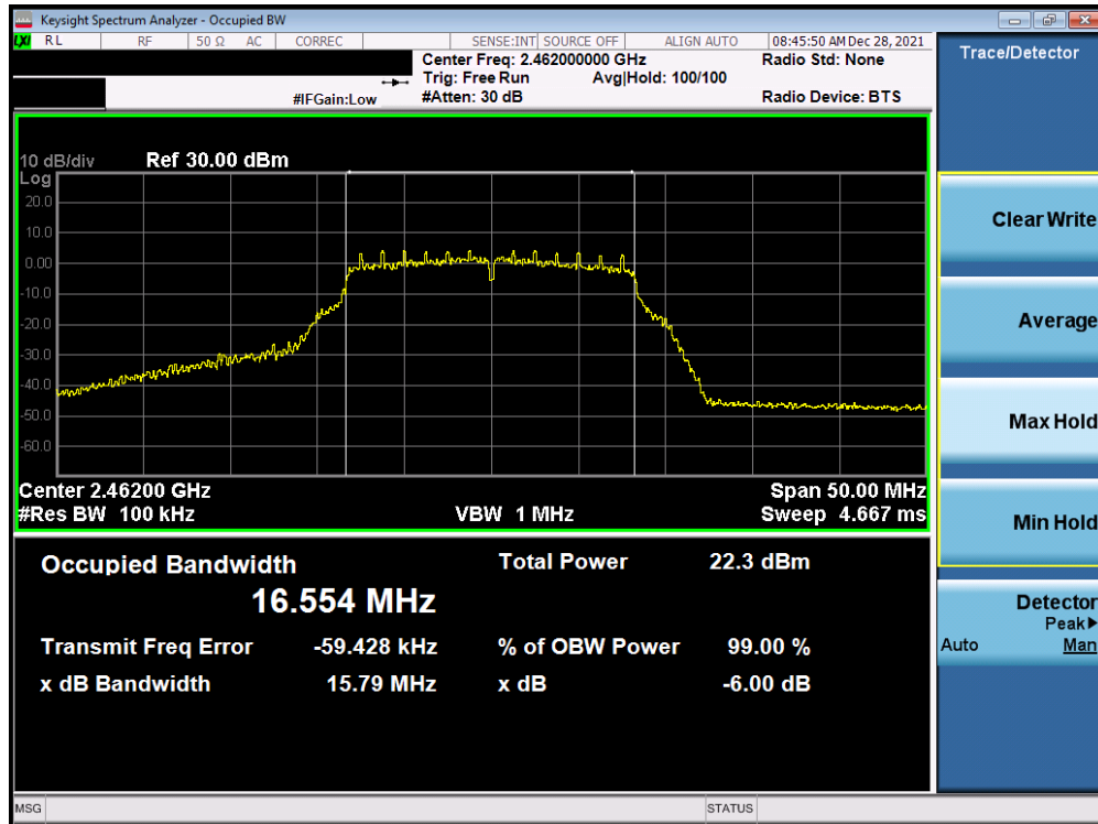
Plot 7-33. 6dB BW and 99% OBW Plot Antenna 1a (802.11g – Ch. 11) – 6Mbps
