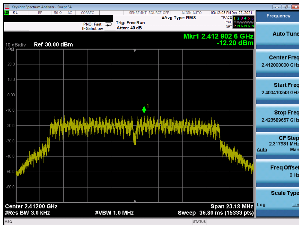
Plot 7-70. Power Spectral Density Plot Antenna 3a (802.11g – Ch. 1) – 18Mbps
