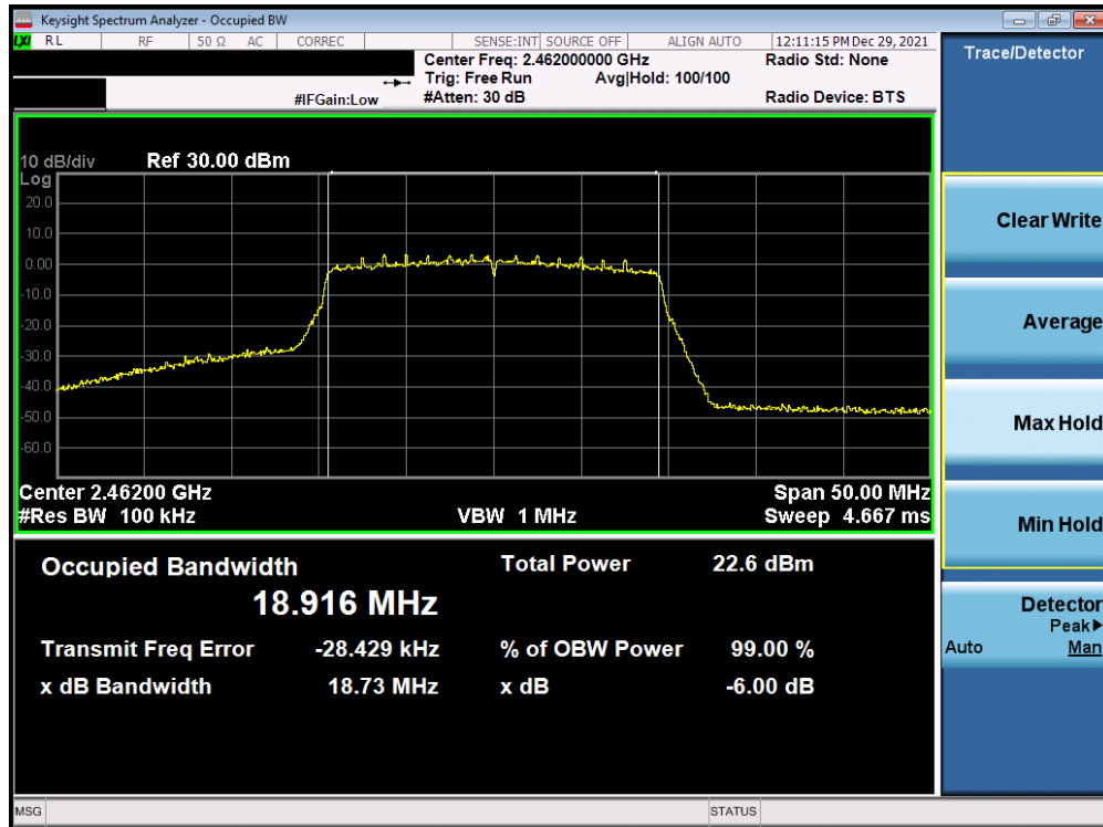
Plot 7-39. 6dB BW and 99% OBW Plot Antenna 1a (802. 11ax (SU - 2.4GHz) – Ch. 11) – MCS0
