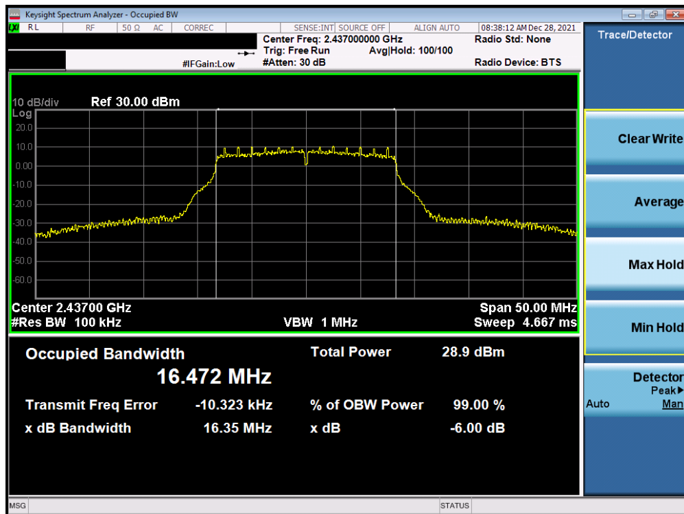
Plot 7-32. 6dB BW and 99% OBW Plot Antenna 1a (802.11g - Ch. 6) - 6Mbps
