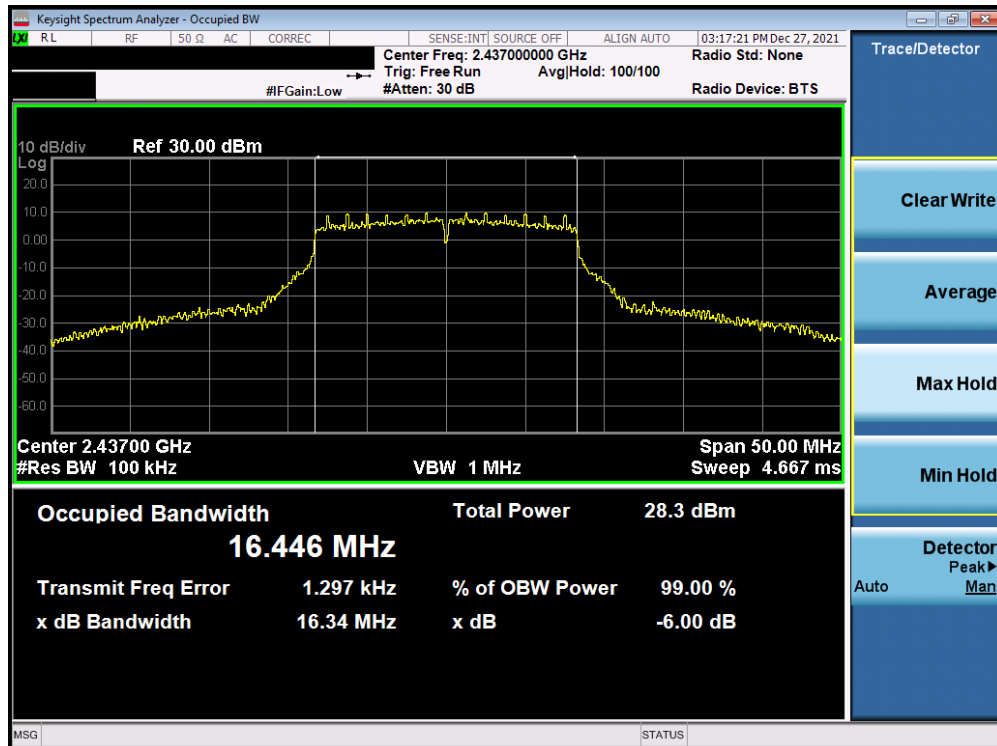
Plot 7-11. 6dB BW and 99% OBW Plot Antenna 3a (802.11g – Ch. 6) – 18Mbps
