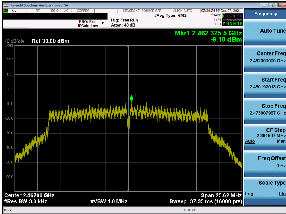
Plot 7-63. Power Spectral Density Plot Antenna 3a (802.11g - Ch. 11) - 6Mbps
