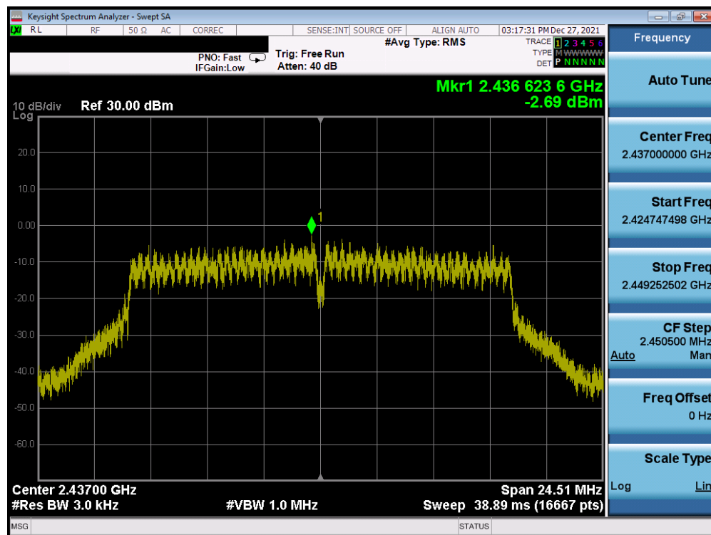
Plot 7-71. Power Spectral Density Plot Antenna 3a (802.11g – Ch. 6) – 18Mbps
