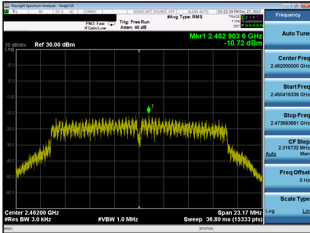
Plot 7-72. Power Spectral Density Plot Antenna 3a (802.11g – Ch. 11) – 18Mbps
