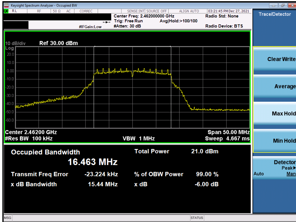
Plot 7-12. 6dB BW and 99% OBW Plot Antenna 3a (802.11g – Ch. 11) – 18Mbps
