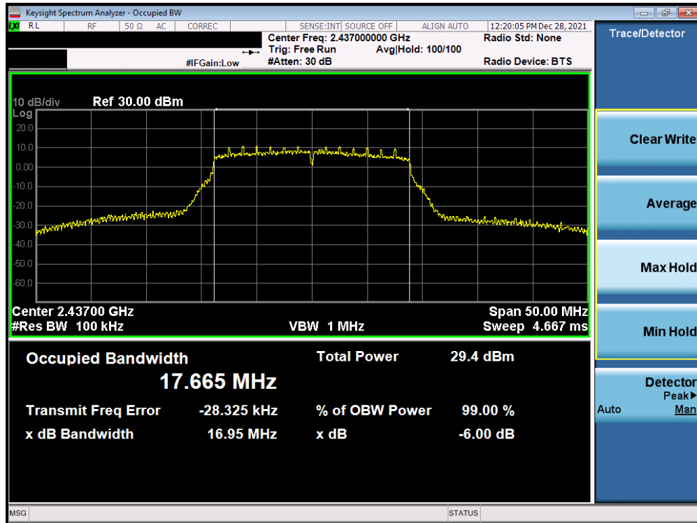
Plot 7-5. 6dB BW and 99% OBW Plot Antenna 3a (802.11n (2.4GHz) – Ch. 6) – MCS0
