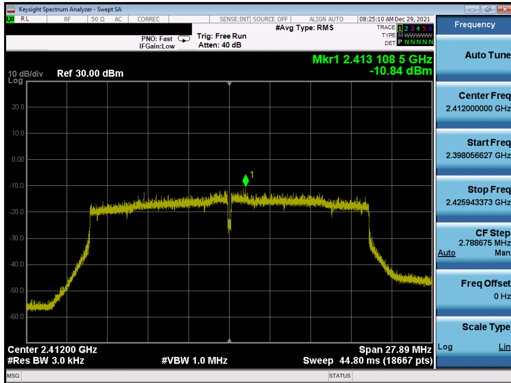
Plot 7-67. Power Spectral Density Plot Antenna 3a (802.11ax (SU - 2.4GHz) – Ch. 1) – MCS0
