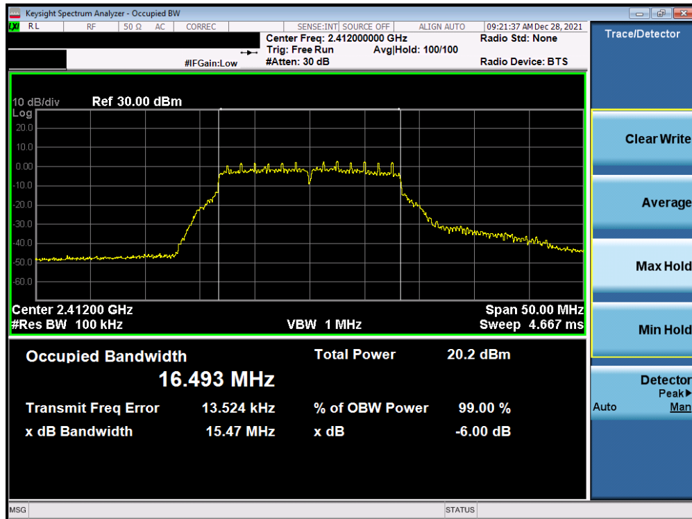
Plot 7-40. 6dB BW and 99% OBW Plot Antenna 1a (802.11g – Ch. 1) – 18Mbps
