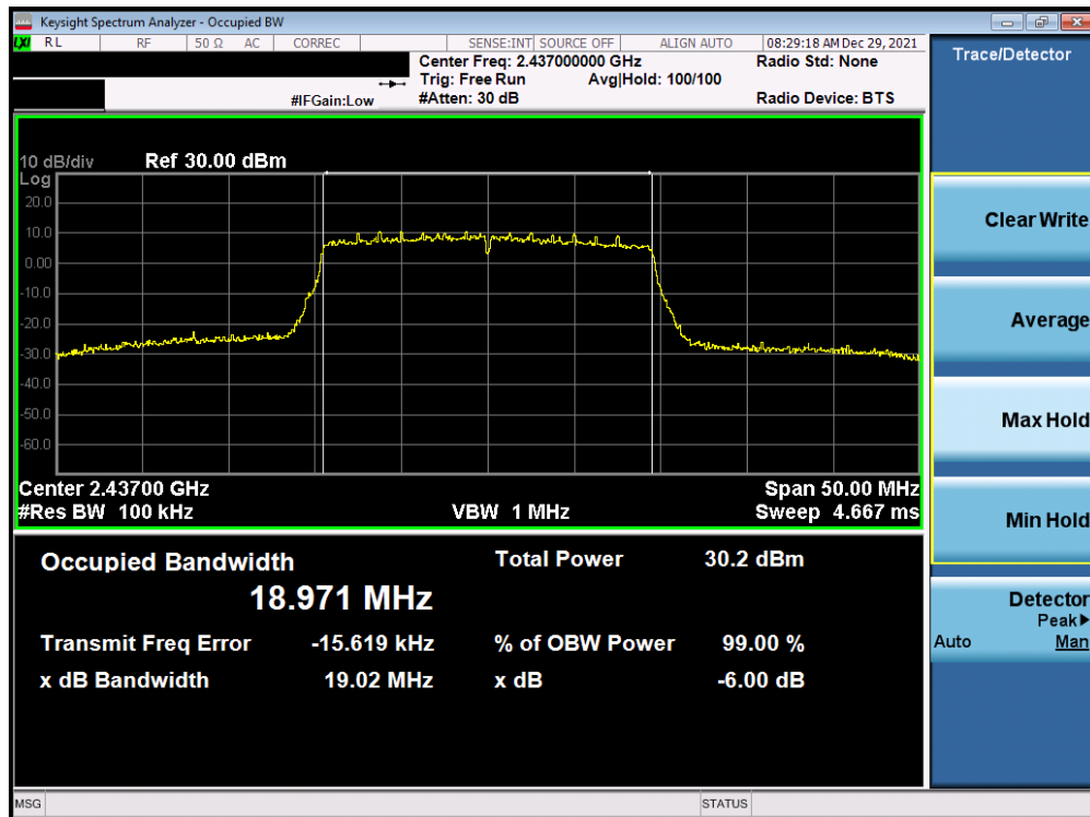
Plot 7-8. 6dB BW and 99% OBW Plot Antenna 3a (802.11ax (SU - 2.4GHz) – Ch. 6) – MCS0
