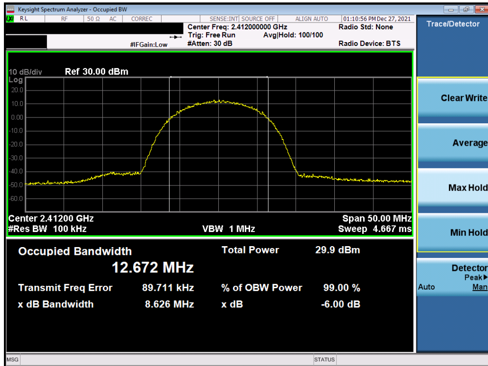
Plot 7-49. 6dB BW and 99% OBW Plot Antenna 1a (802.11b – Ch. 1) – 11Mbps
