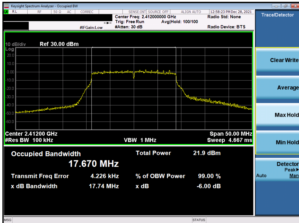
Plot 7-13. 6dB BW and 99% OBW Plot Antenna 3a (802.11n (2.4GHz) – Ch. 1) – MCS3
