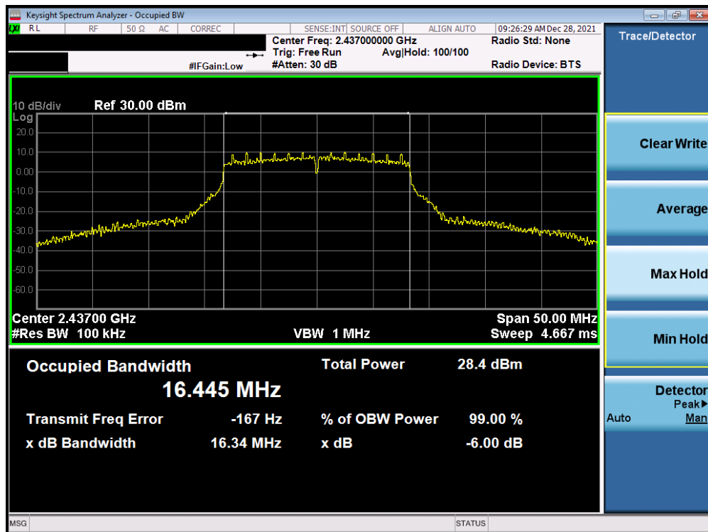
Plot 7-41. 6dB BW and 99% OBW Plot Antenna 1a (802.11g – Ch. 6) – 18Mbps
