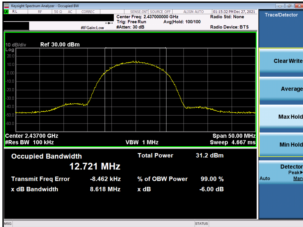
Plot 7-50. 6dB BW and 99% OBW Plot Antenna 1a (802.11b – Ch. 6) – 11Mbps
