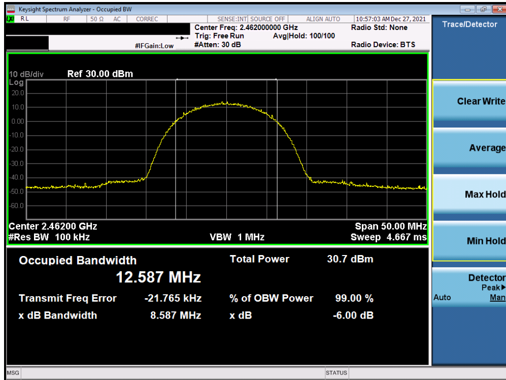
Plot 7-21. 6dB BW and 99% OBW Plot Antenna 3a (802.11b – Ch. 11) – 11Mbps
