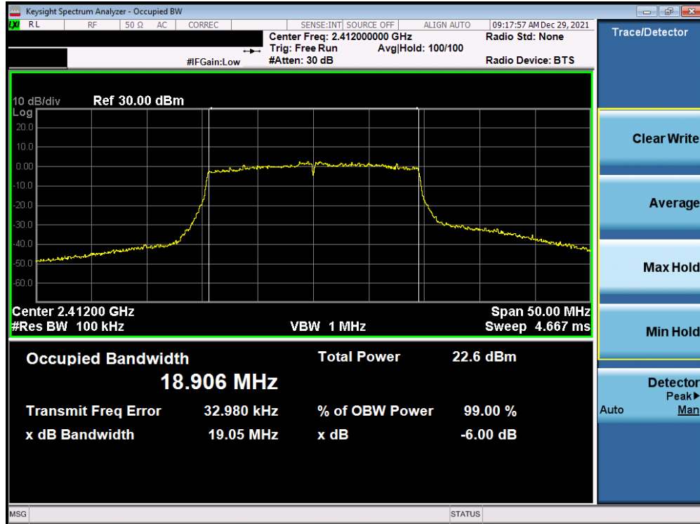
Plot 7-16. 6dB BW and 99% OBW Plot Antenna 3a (802. 11ax (SU - 2.4GHz) – Ch. 1) – MCS3
