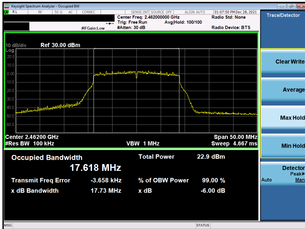
Plot 7-15. 6dB BW and 99% OBW Plot Antenna 3a (802.11n (2.4GHz) – Ch. 11) – MCS3
