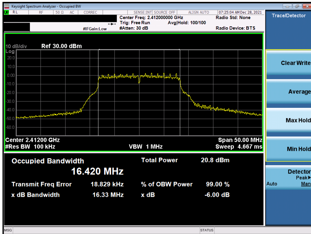
Plot 7-22. 6dB BW and 99% OBW Plot Antenna 3a (802.11g – Ch. 1) – 36Mbps
