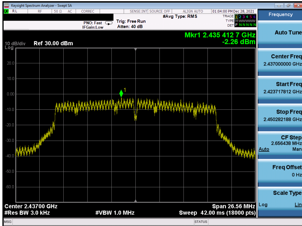
Plot 7-74. Power Spectral Density Plot Antenna 3a (802.11n (2.4GHz) – Ch. 6) – MCS3
