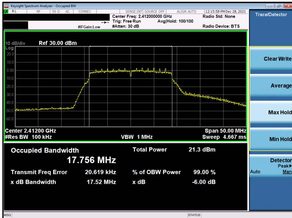
Plot 7-4. 6dB BW and 99% OBW Plot Antenna 3a (802.11n (2.4GHz) – Ch. 1) – MCS0
