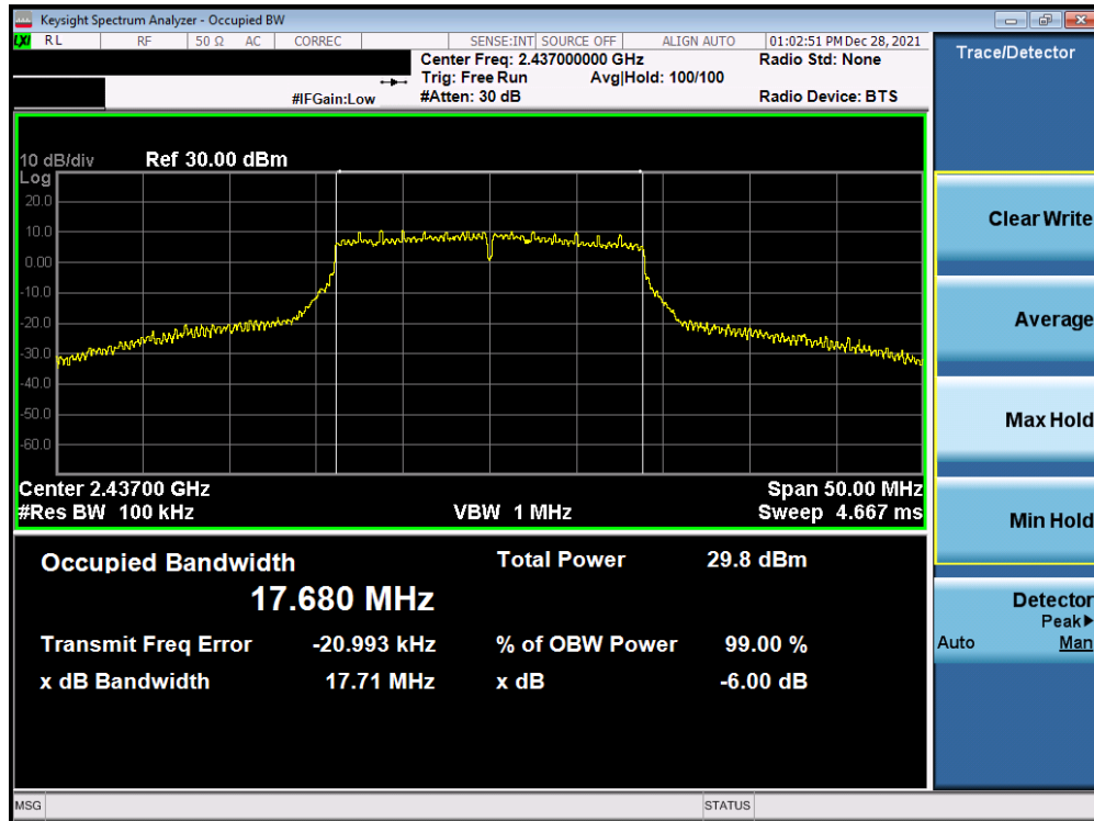
Plot 7-14. 6dB BW and 99% OBW Plot Antenna 3a (802.11n (2.4GHz) – Ch. 6) – MCS3
