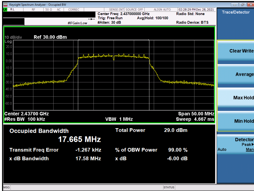
Plot 7-35. 6dB BW and 99% OBW Plot Antenna 1a (802.11n (2.4GHz) – Ch. 6) – MCS0
