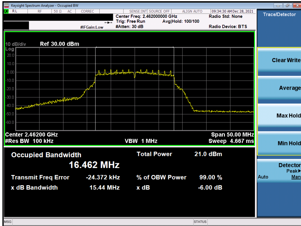
Plot 7-42. 6dB BW and 99% OBW Plot Antenna 1a (802.11g – Ch. 11) – 18Mbps
