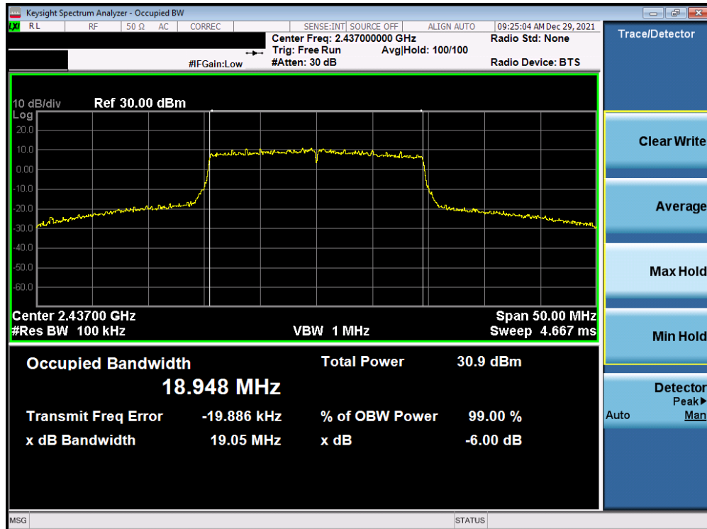
Plot 7-17. 6dB BW and 99% OBW Plot Antenna 3a (802. 11ax (SU - 2.4GHz) – Ch. 6) – MCS3
