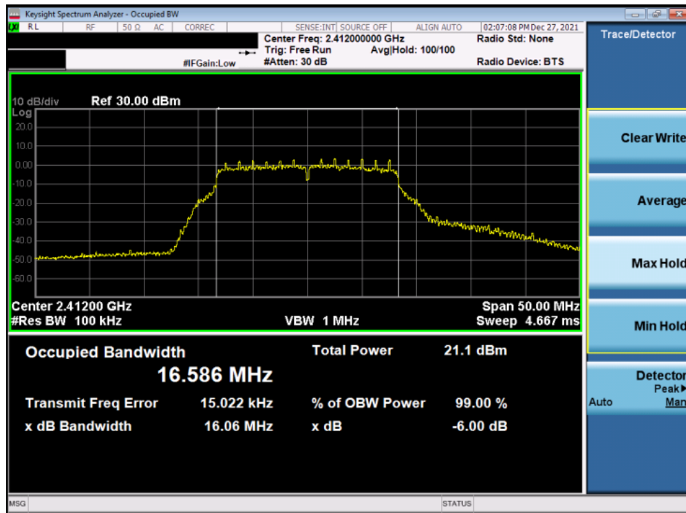
Plot 7-1. 6dB BW and 99% OBW Plot Antenna 3a (802.11g – Ch. 1) – 6Mbps
