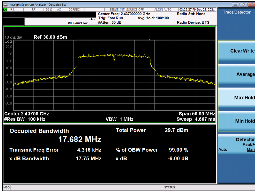
Plot 7-44. 6dB BW and 99% OBW Plot Antenna 1a (802.11n (2.4GHz) – Ch. 6) – MCS3
