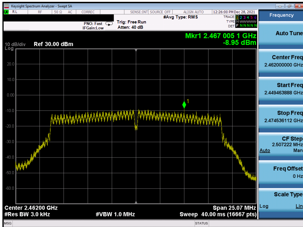
Plot 7-66. Power Spectral Density Plot Antenna 3a (802.11n (2.4GHz) – Ch. 11) – MCS0
