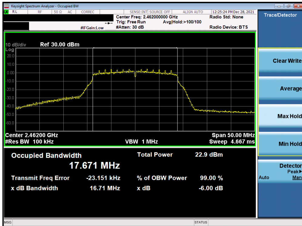
Plot 7-6. 6dB BW and 99% OBW Plot Antenna 3a (802.11n (2.4GHz) – Ch. 11) – MCS0
