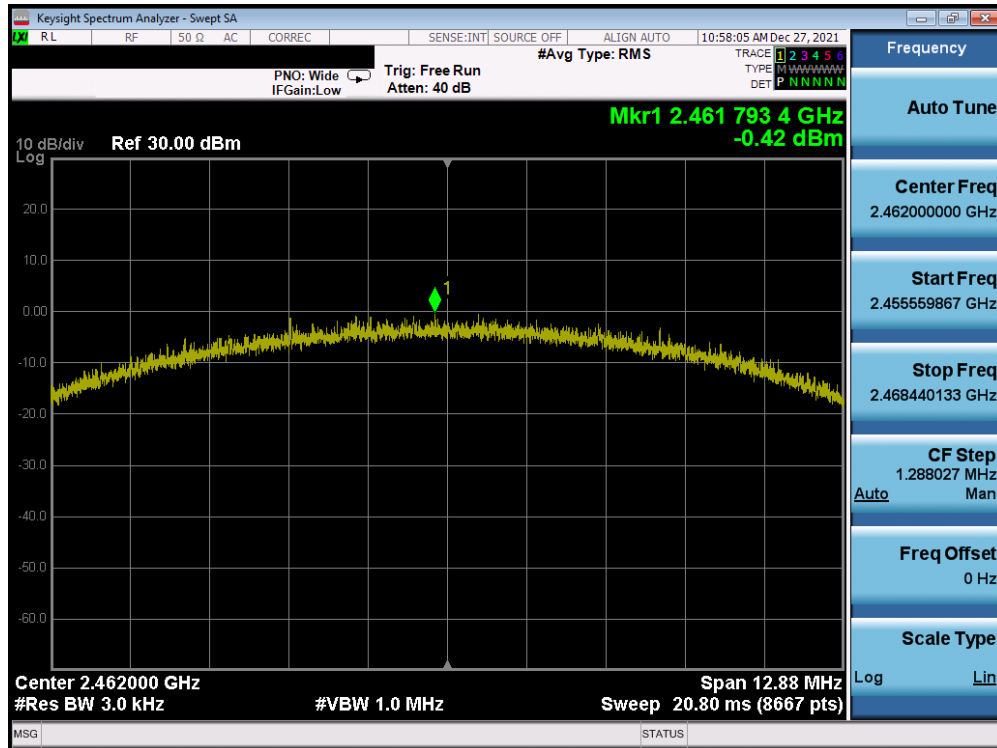
Plot 7-81. Power Spectral Density Plot Antenna 3a (802.11b – Ch. 11) – 11Mbps
