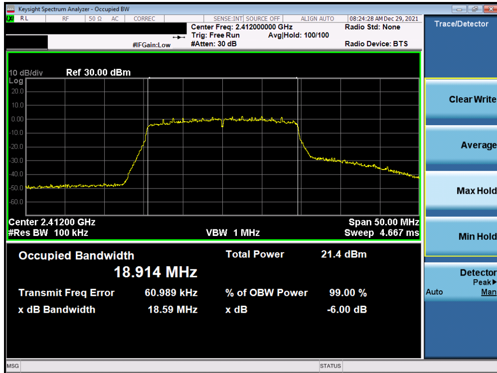
Plot 7-7. 6dB BW and 99% OBW Plot Antenna 3a (802.11ax (SU - 2.4GHz) – Ch. 1) – MCS0
