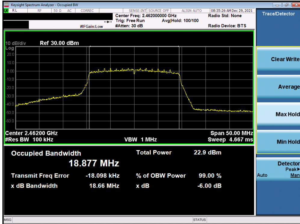
Plot 7-9. 6dB BW and 99% OBW Plot Antenna 3a (802. 11ax (SU - 2.4GHz) – Ch. 11) – MCS0
