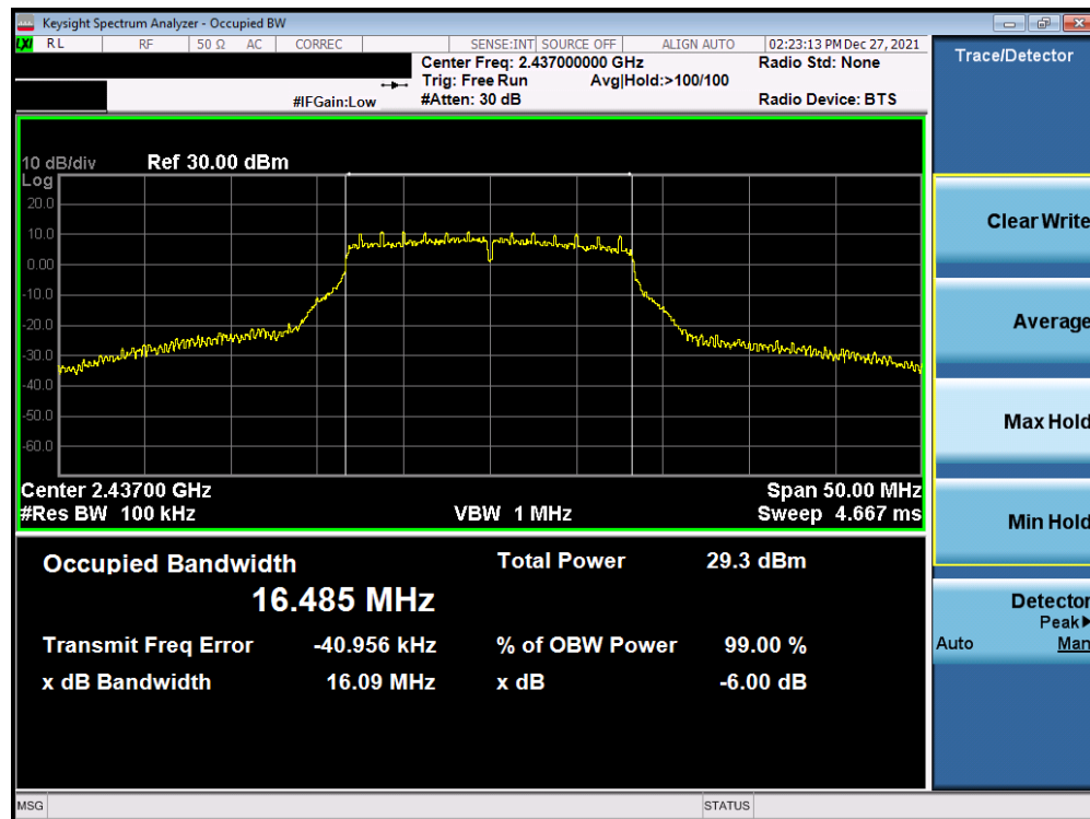
Plot 7-2. 6dB BW and 99% OBW Plot Antenna 3a (802.11g – Ch. 6) – 6Mbps
