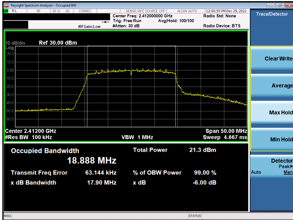
Plot 7-37. 6dB BW and 99% OBW Plot Antenna 1a (802.11ax (SU - 2.4GHz) – Ch. 1) – MCS0
