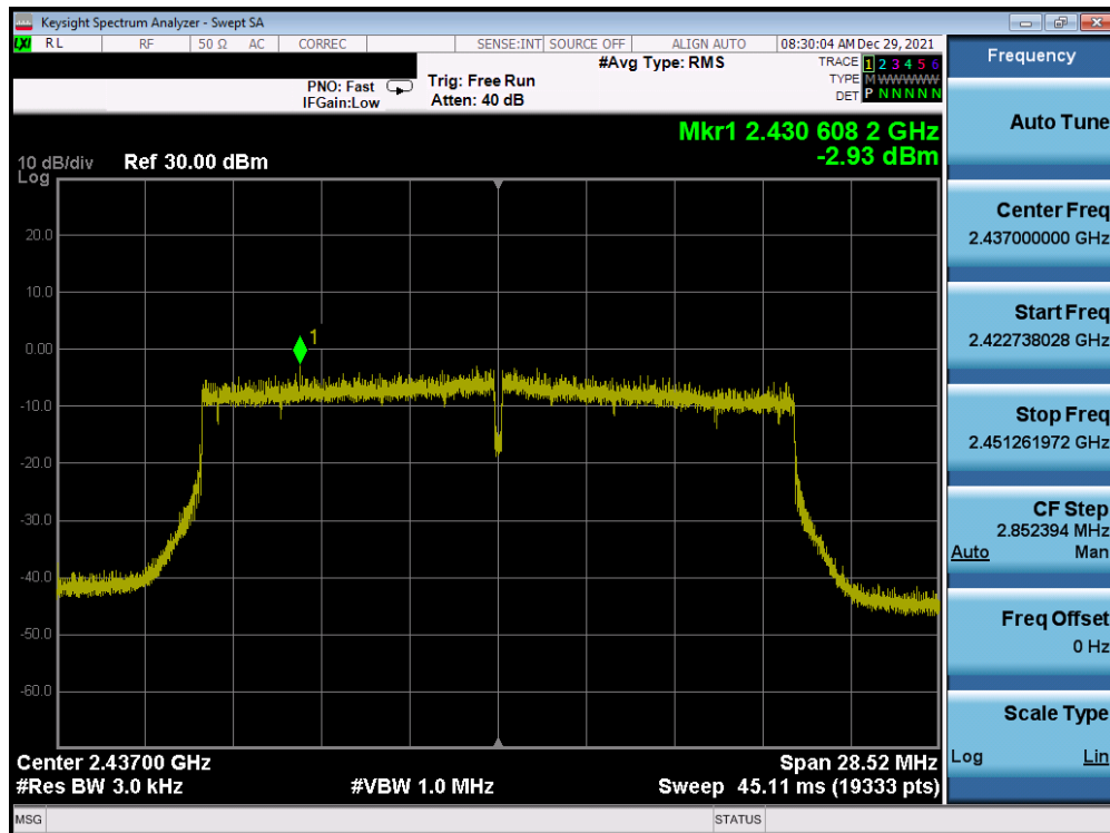
Plot 7-68. Power Spectral Density Plot Antenna 3a (802.11ax (SU - 2.4GHz) – Ch. 6) – MCS0
