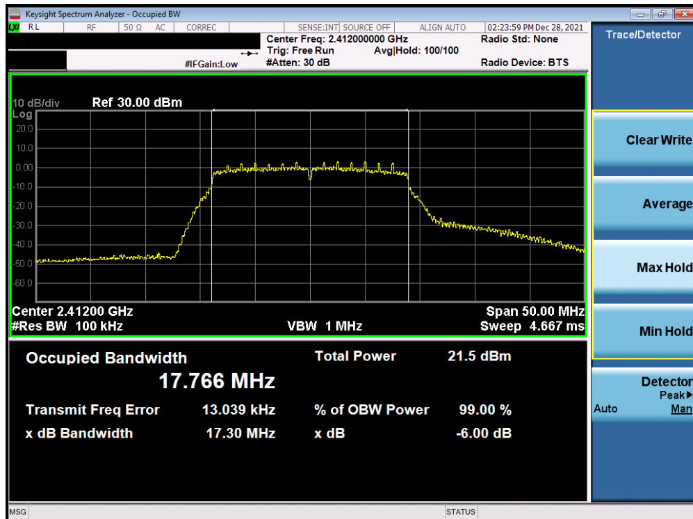
Plot 7-34. 6dB BW and 99% OBW Plot Antenna 1a (802.11n (2.4GHz) – Ch. 1) – MCS0
