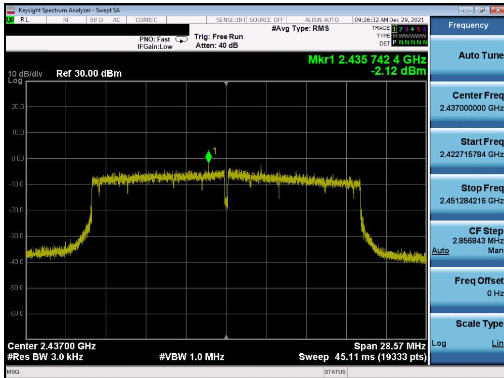
Plot 7-77. Power Spectral Density Plot Antenna 3a (802.11ax (SU - 2.4GHz) – Ch. 6) – MCS3
