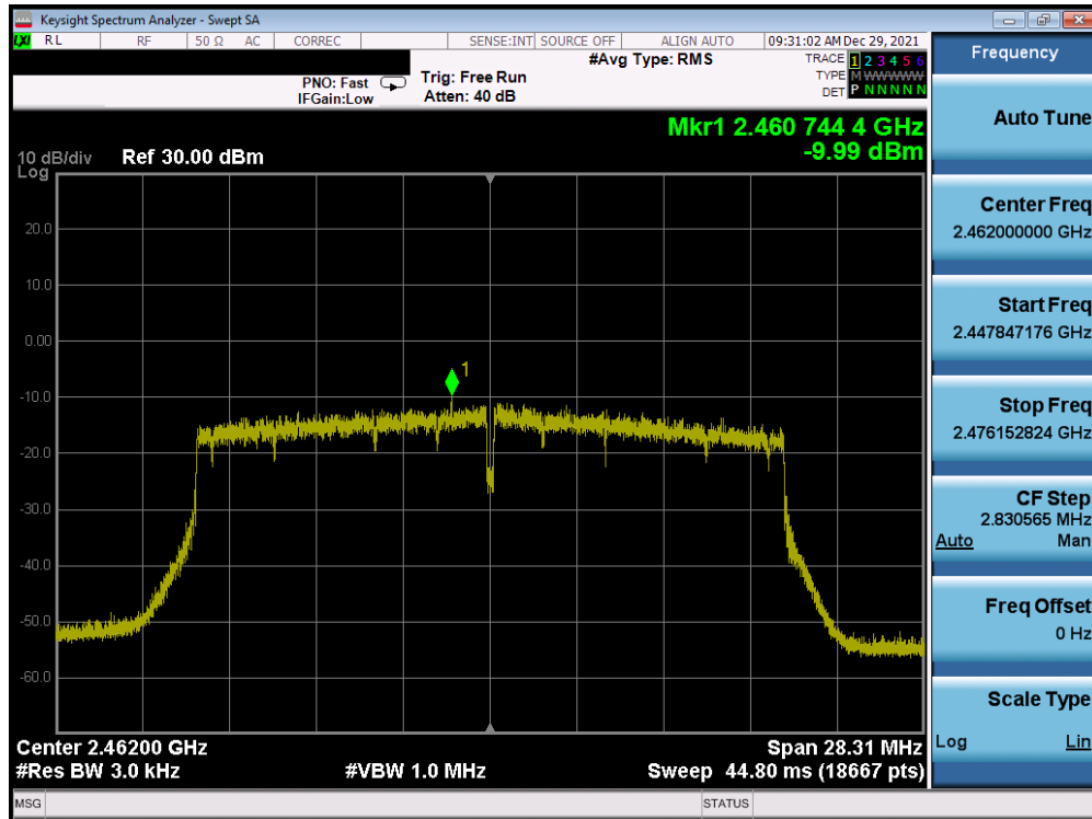
Plot 7-78. Power Spectral Density Plot Antenna 3a (802.11ax (SU - 2.4GHz) – Ch. 11) – MCS3
