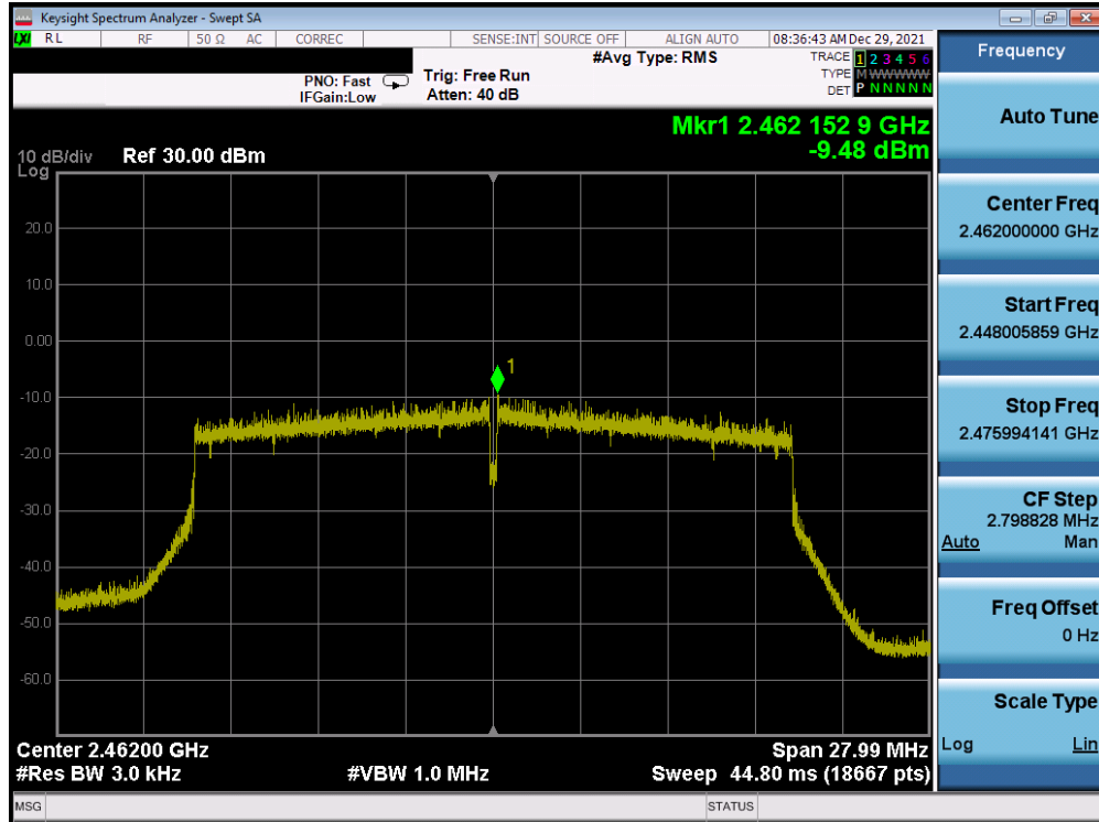
Plot 7-69. Power Spectral Density Plot Antenna 3a (802.11ax (SU - 2.4GHz) – Ch. 11) – MCS0
