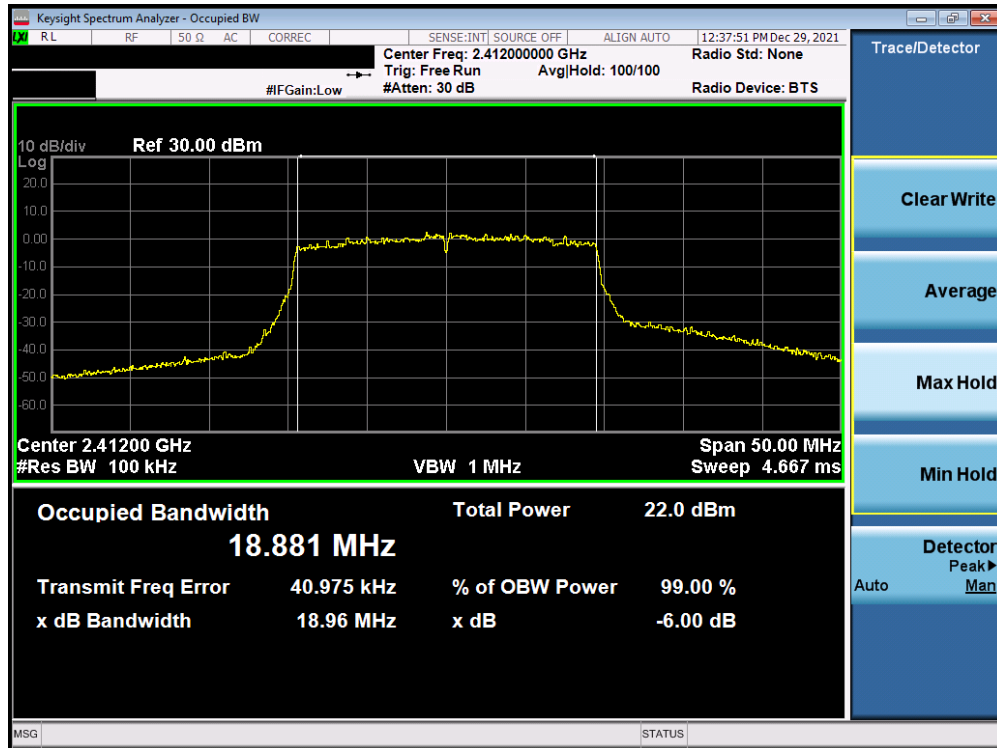
Plot 7-46. 6dB BW and 99% OBW Plot Antenna 1a (802. 11ax (SU - 2.4GHz) – Ch. 1) – MCS3
