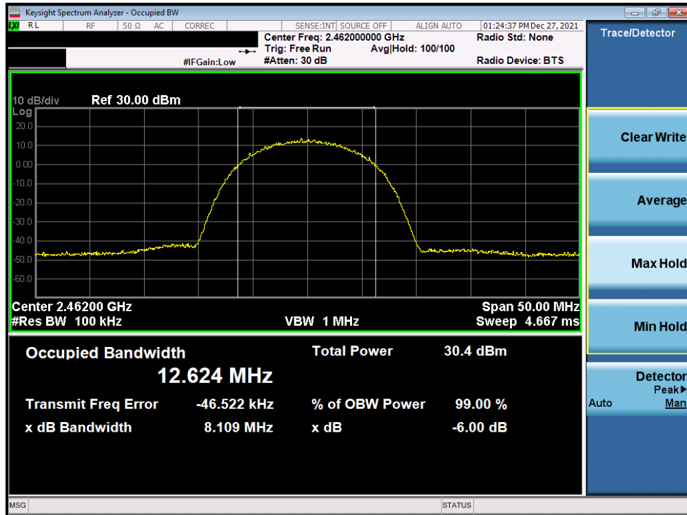
Plot 7-51. 6dB BW and 99% OBW Plot Antenna 1a (802.11b – Ch. 11) – 11Mbps
