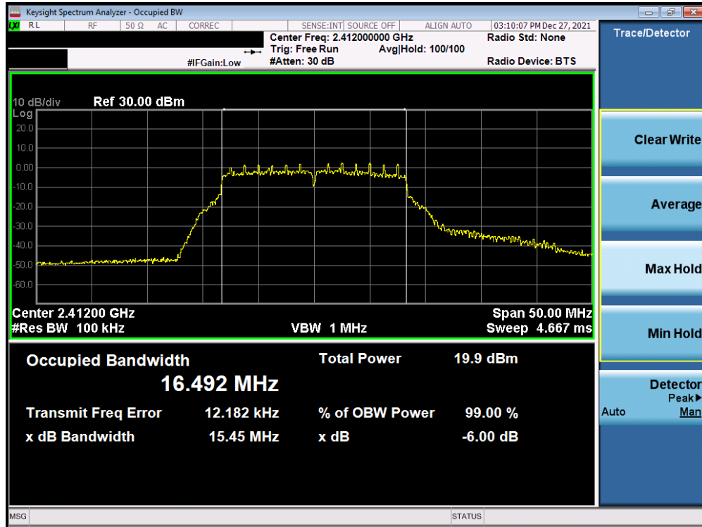
Plot 7-10. 6dB BW and 99% OBW Plot Antenna 3a (802.11g – Ch. 1) – 18Mbps
