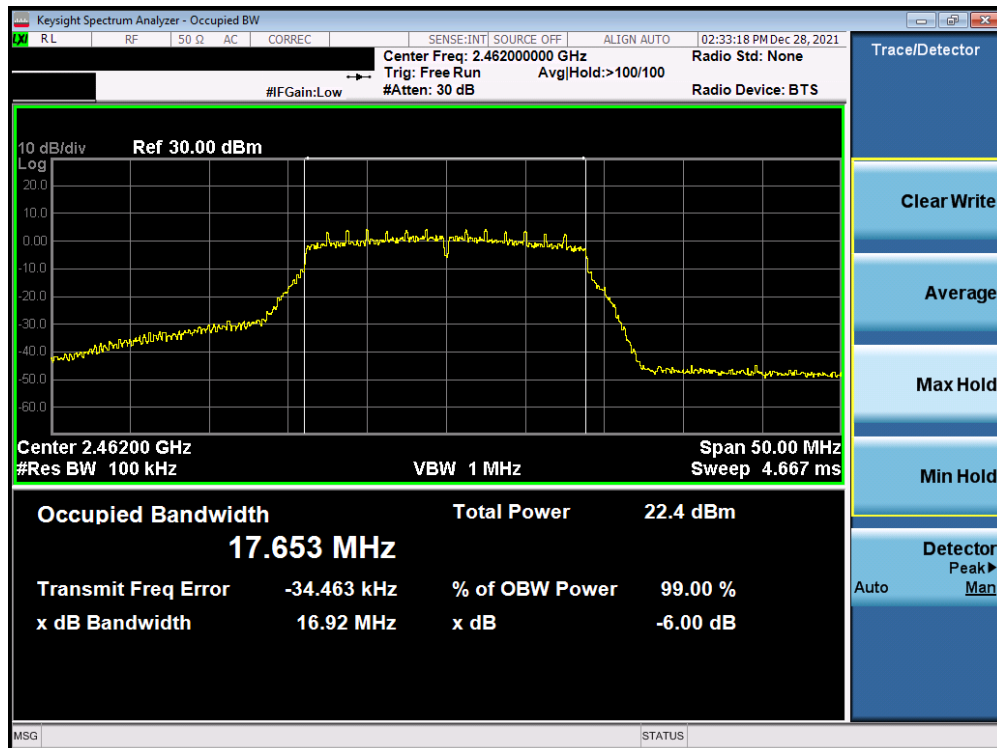
Plot 7-36. 6dB BW and 99% OBW Plot Antenna 1a (802.11n (2.4GHz) – Ch. 11) – MCS0
