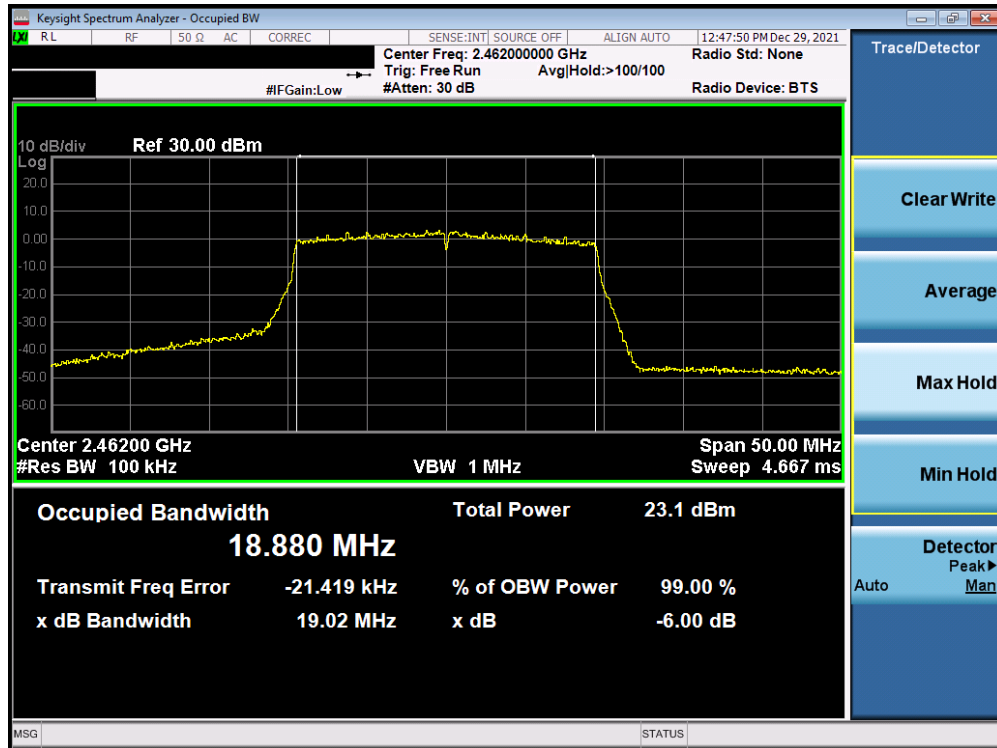
Plot 7-48. 6dB BW and 99% OBW Plot Antenna 1a (802. 11ax (SU - 2.4GHz) – Ch. 11) – MCS3
