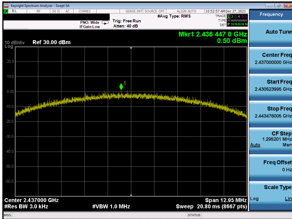
Plot 7-80. Power Spectral Density Plot Antenna 3a (802.11b – Ch. 6) – 11Mbps
