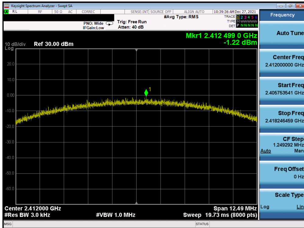
Plot 7-79. Power Spectral Density Plot Antenna 3a (802.11b – Ch. 1) – 11Mbps
