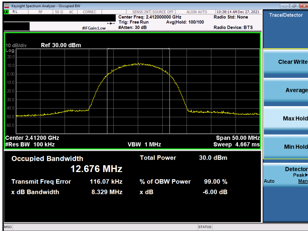
Plot 7-19. 6dB BW and 99% OBW Plot Antenna 3a (802.11b – Ch. 1) – 11Mbps
