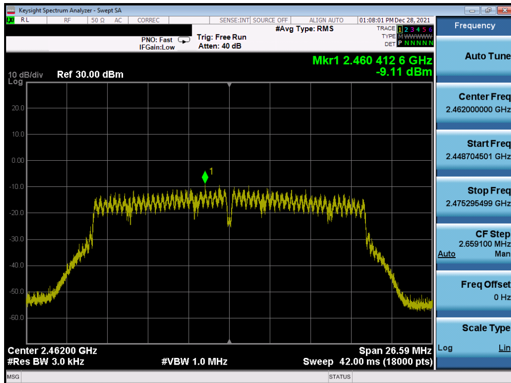
Plot 7-75. Power Spectral Density Plot Antenna 3a (802.11n (2.4GHz) – Ch. 11) – MCS3
