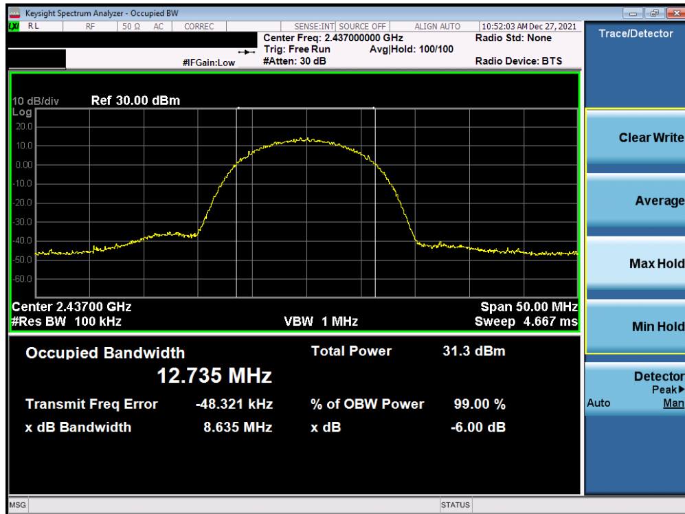
Plot 7-20. 6dB BW and 99% OBW Plot Antenna 3a (802.11b – Ch. 6) – 11Mbps
