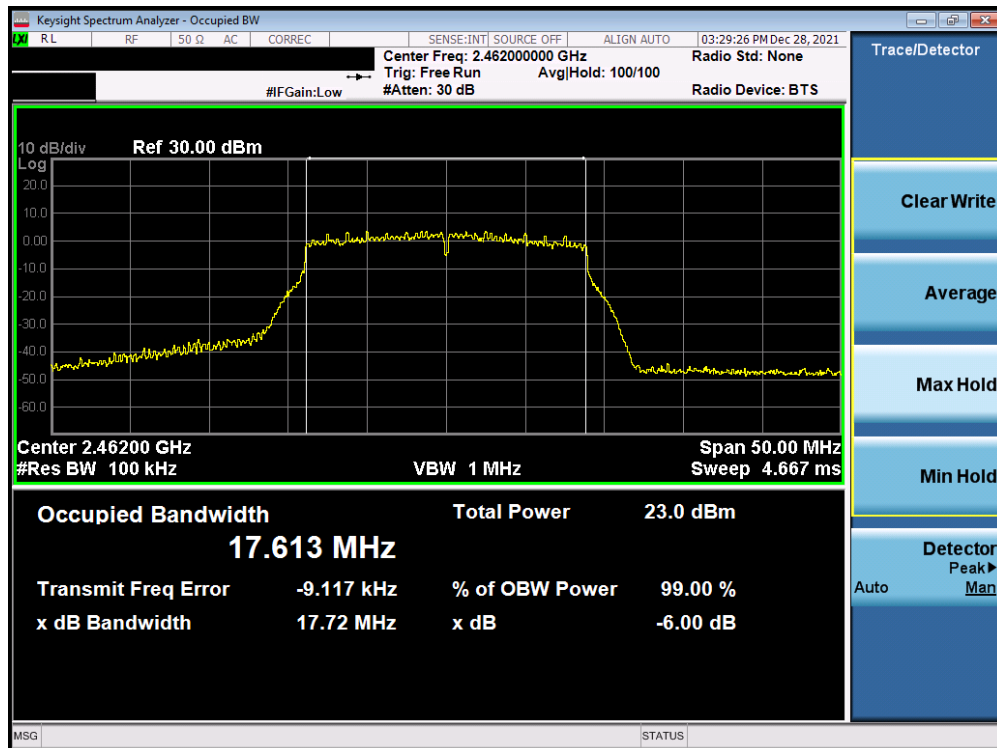
Plot 7-45. 6dB BW and 99% OBW Plot Antenna 1a (802.11n (2.4GHz) – Ch. 11) – MCS3
