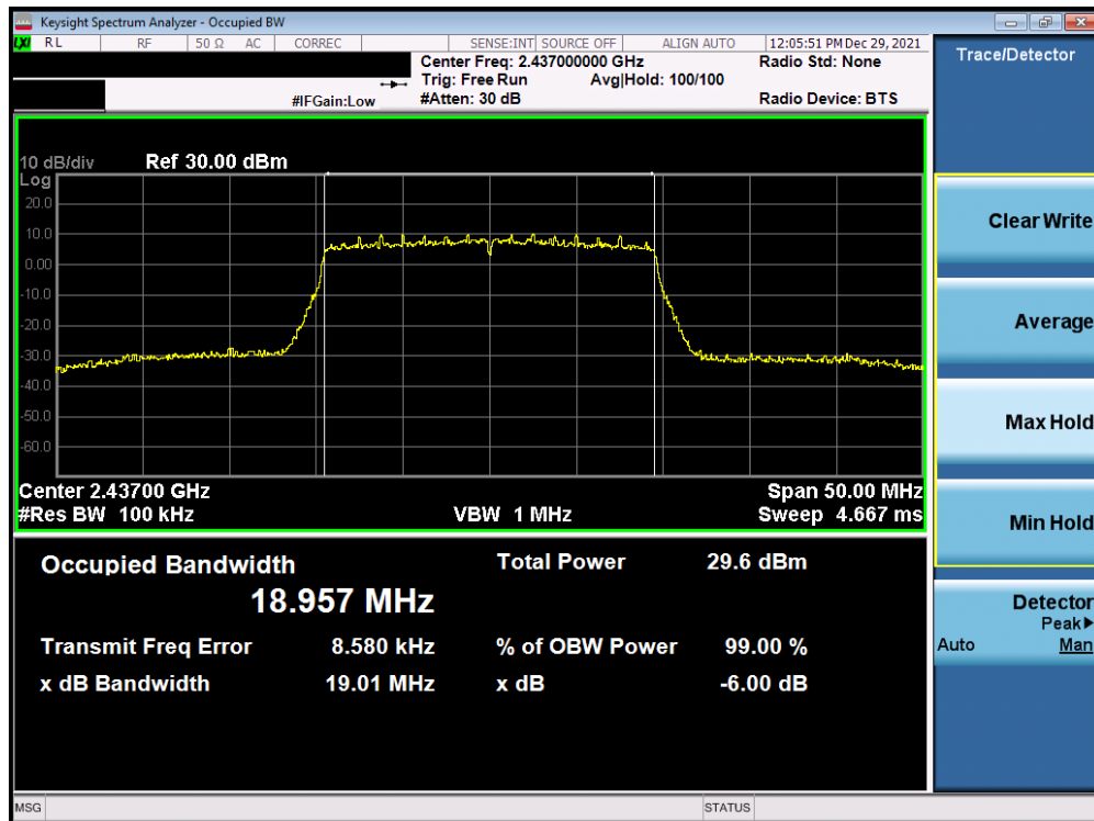
Plot 7-38. 6dB BW and 99% OBW Plot Antenna 1a (802.11ax (SU - 2.4GHz) – Ch. 6) – MCS0
