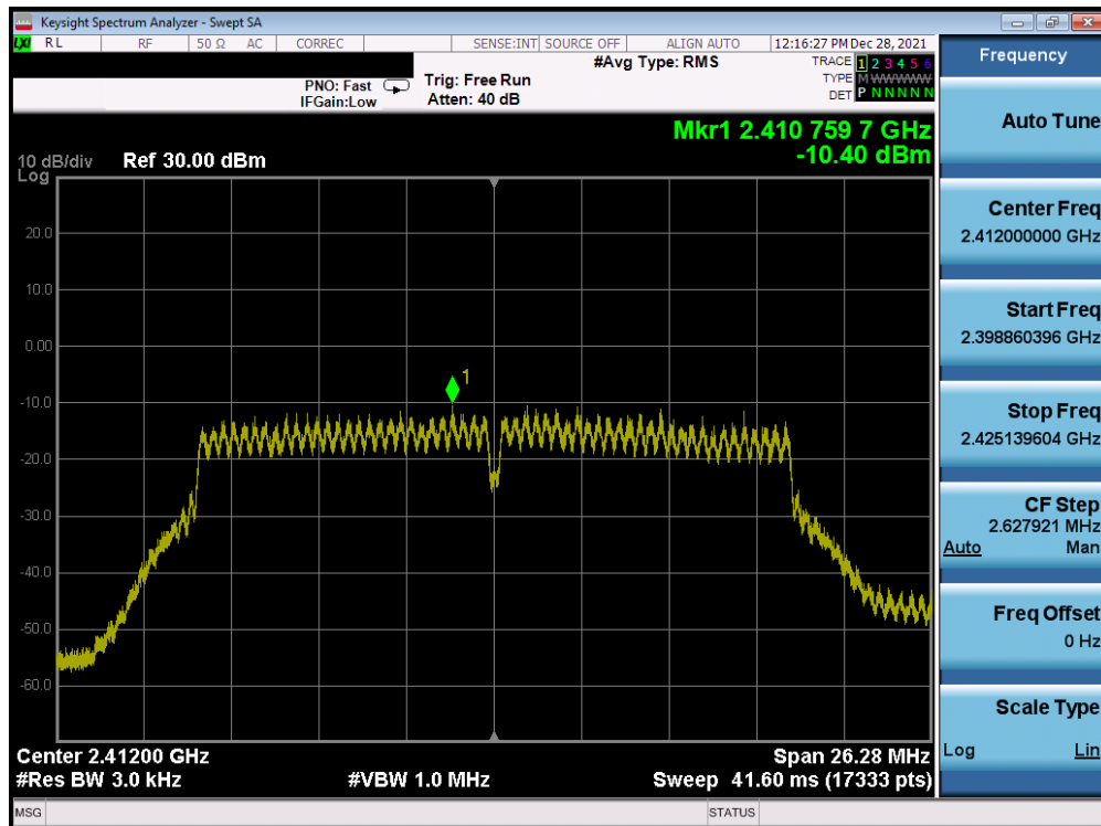
Plot 7-64. Power Spectral Density Plot Antenna 3a (802.11n (2.4GHz) - Ch. 1) - MCS0
