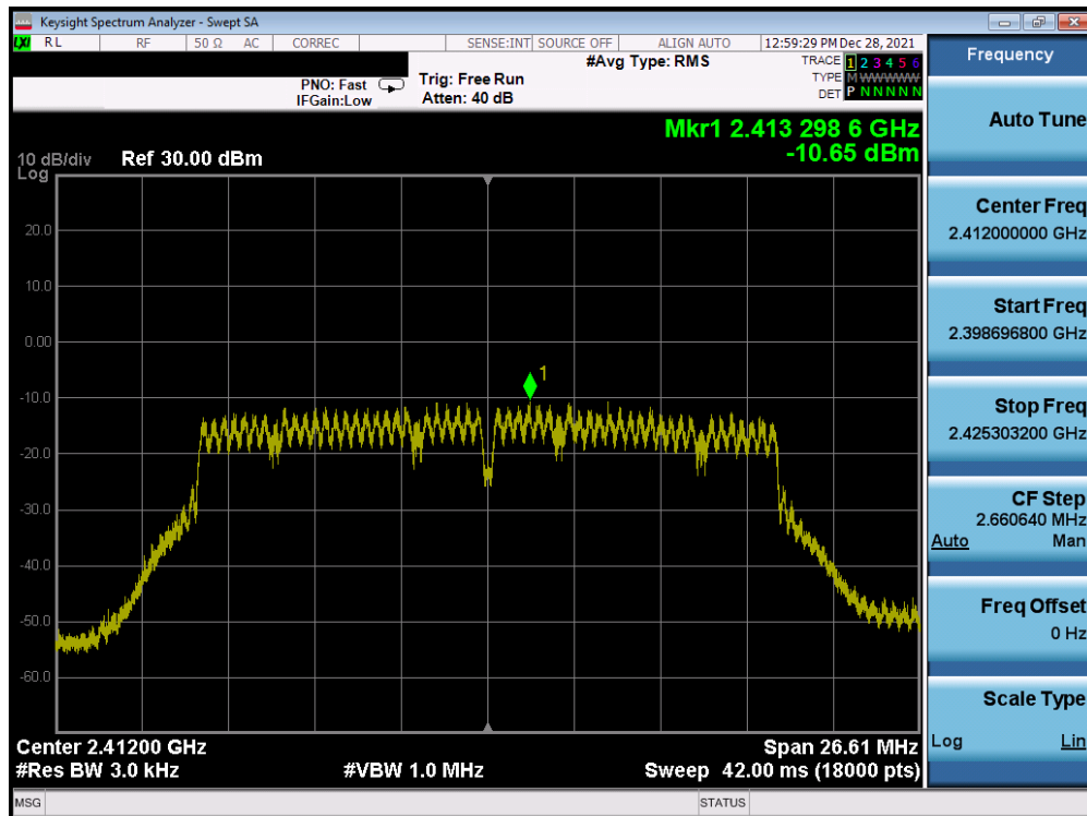
Plot 7-73. Power Spectral Density Plot Antenna 3a (802.11n (2.4GHz) – Ch. 1) – MCS3
