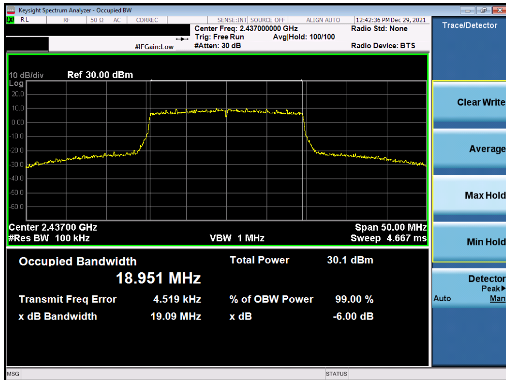
Plot 7-47. 6dB BW and 99% OBW Plot Antenna 1a (802. 11ax (SU - 2.4GHz) – Ch. 6) – MCS3
