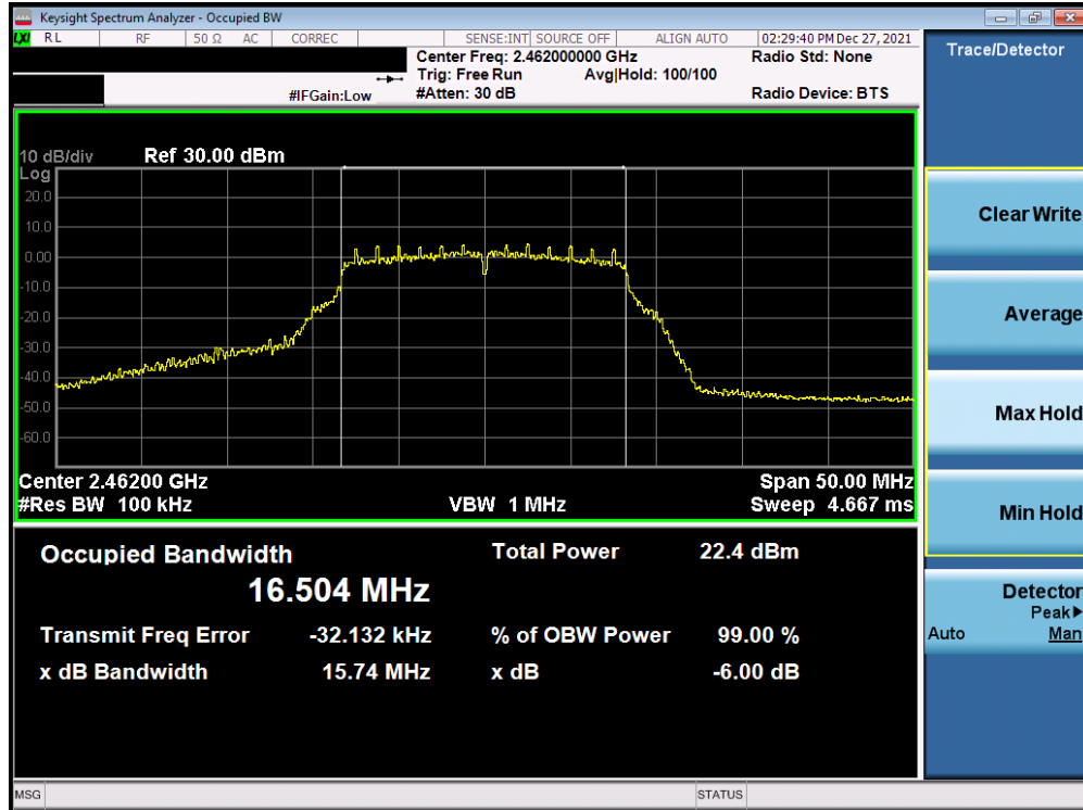
Plot 7-3. 6dB BW and 99% OBW Plot Antenna 3a (802.11g – Ch. 11) – 6Mbps
