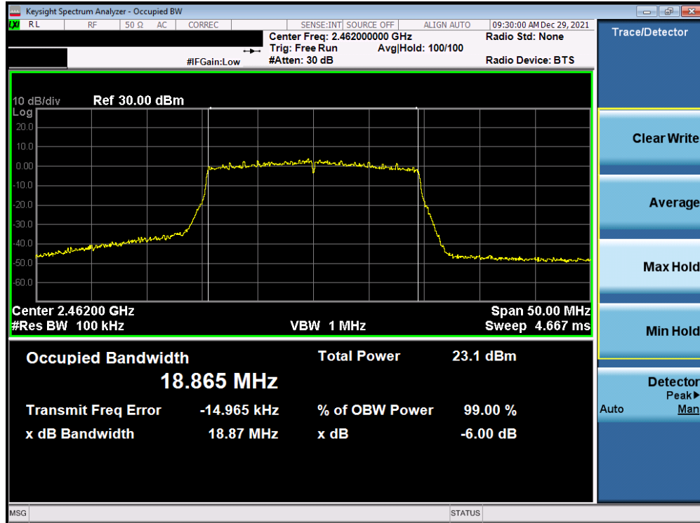
Plot 7-18. 6dB BW and 99% OBW Plot Antenna 3a (802. 11ax (SU - 2.4GHz) – Ch. 11) – MCS3
