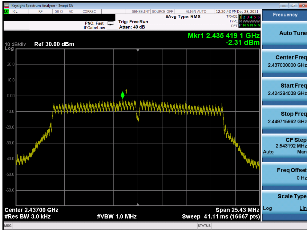
Plot 7-65. Power Spectral Density Plot Antenna 3a (802.11n (2.4GHz) – Ch. 6) – MCS0
