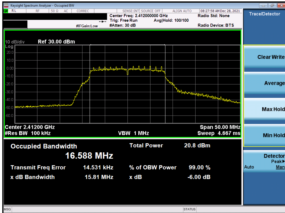
Plot 7-31. 6dB BW and 99% OBW Plot Antenna 1a (802.11g - Ch. 1) - 6Mbps
