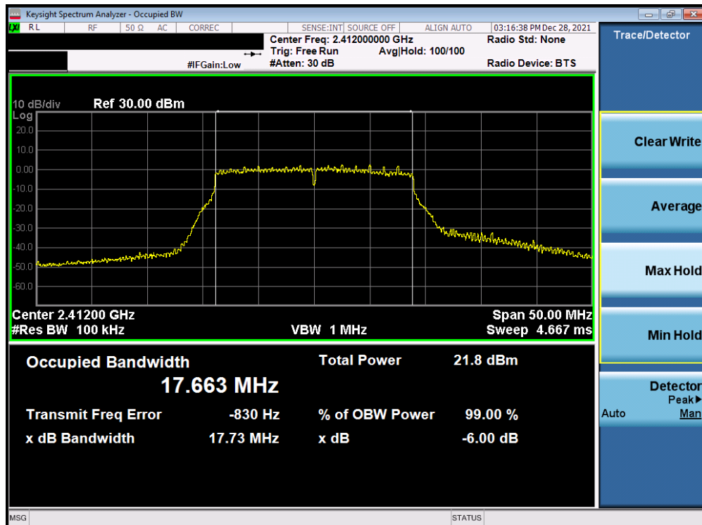
Plot 7-43. 6dB BW and 99% OBW Plot Antenna 1a (802.11n (2.4GHz) – Ch. 1) – MCS3
