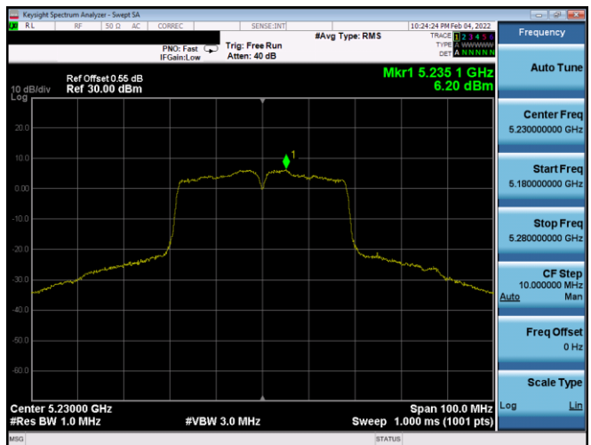
Plot 7-708. PSD CDD Diversity Antenna 3A (40MHz BW 802.11n - Ch. 46, MCS11)
