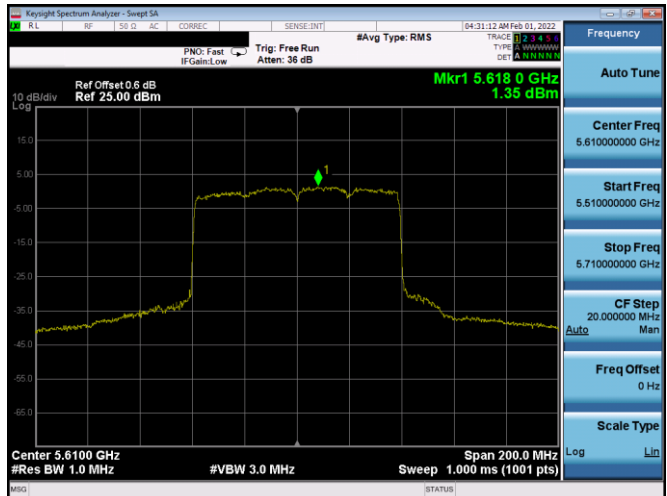
Plot 7-737. PSD CDD Diversity Antenna 2B (80MHz BW 802.11ax(SU) – Ch. 122, MCS3)
