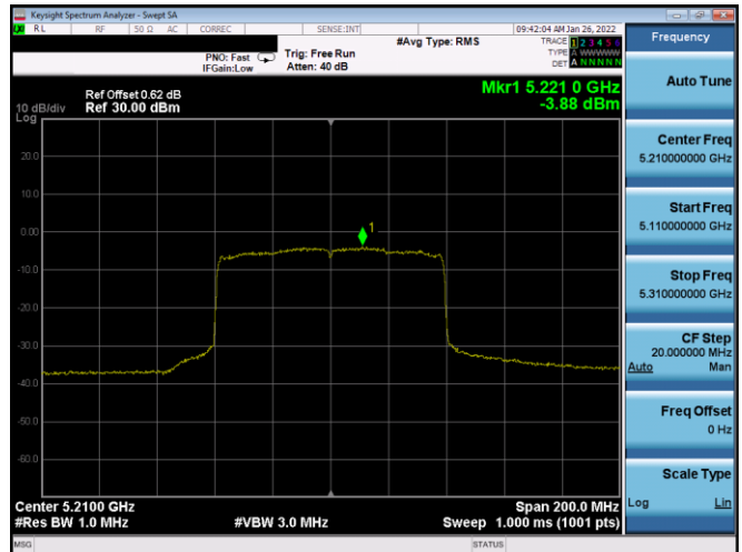
Plot 7-714. PSD CDD Diversity Antenna 3A (80MHz BW 802.11ax(SU) – Ch. 42, MCS3)
