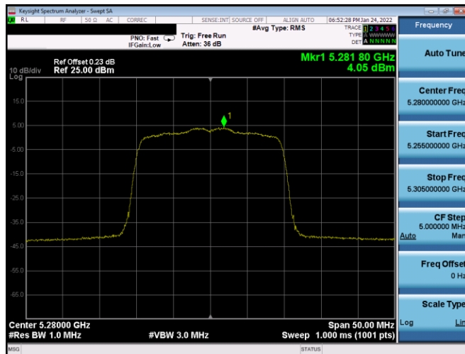
Plot 7-717. PSD CDD Diversity Antenna 2B (20MHz BW 802.11ax(SU) – Ch. 56, MCS3)
