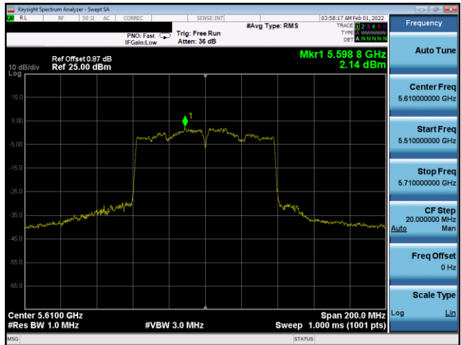
Plot 7-736. PSD CDD Diversity Antenna 3A (80MHz BW 802.11ac – Ch. 122, MCS3)
