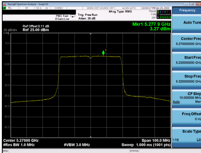
Plot 7-685. PSD CDD Diversity Antenna 2B (40MHz BW 802.11ax(SU) – Ch. 54, MCS0)
