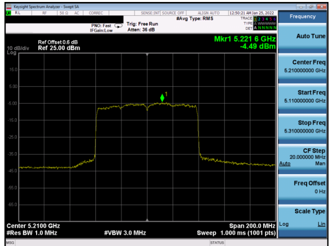
Plot 7-713. PSD CDD Diversity Antenna 2B (80MHz BW 802.11ax(SU) – Ch. 42, MCS3)
