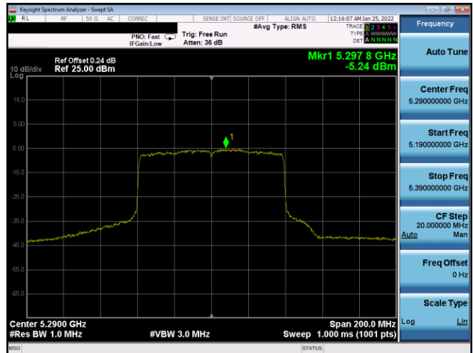
Plot 7-689. PSD CDD Diversity Antenna 2B (80MHz BW 802.11ax(SU) – Ch. 58, MCS0)
