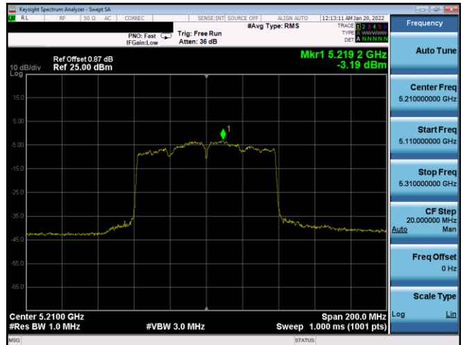
Plot 7-712. PSD CDD Diversity Antenna 3A (80MHz BW 802.11ac – Ch. 42, MCS3)
