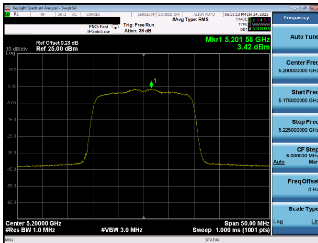
Plot 7-705. PSD CDD Diversity Antenna 2B (20MHz BW 802.11ax(SU) - Ch. 40, MCS3)
