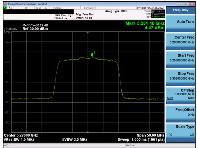
Plot 7-718. PSD CDD Diversity Antenna 3A (20MHz BW 802.11ax(SU) – Ch. 56, MCS3)
