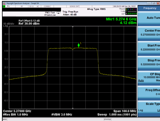
Plot 7-686. PSD CDD Diversity Antenna 3A (40MHz BW 802.11ax(SU) – Ch. 54, MCS0)
