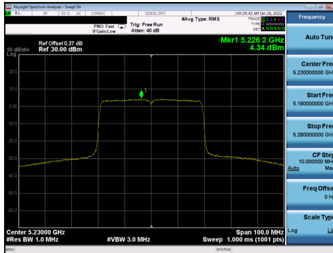
Plot 7-710. PSD CDD Diversity Antenna 3A (40MHz BW 802.11ax(SU) – Ch. 46, MCS3)
