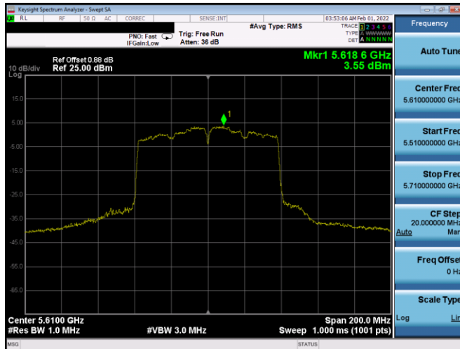
Plot 7-735. PSD CDD Diversity Antenna 2B (80MHz BW 802.11ac – Ch. 122, MCS3)
