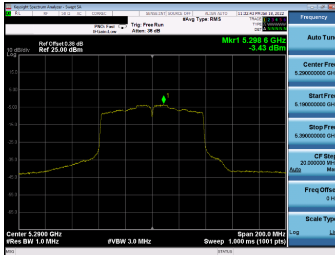
Plot 7-687. PSD CDD Diversity Antenna 2B (80MHz BW 802.11ac – Ch. 58, MCS0)
