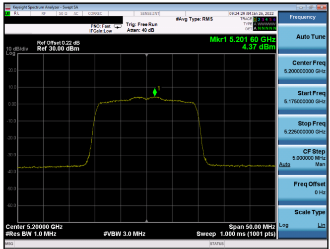
Plot 7-706. PSD CDD Diversity Antenna 3A (20MHz BW 802.11ax(SU) - Ch. 40, MCS3)
