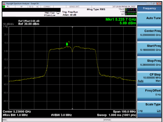
Plot 7-707. PSD CDD Diversity Antenna 2B (40MHz BW 802.11n - Ch. 46, MCS11)
