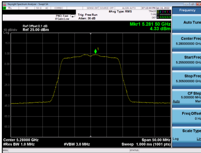
Plot 7-679. PSD CDD Diversity Antenna 2B (20MHz BW 802.11n – Ch. 56, MCS8)
