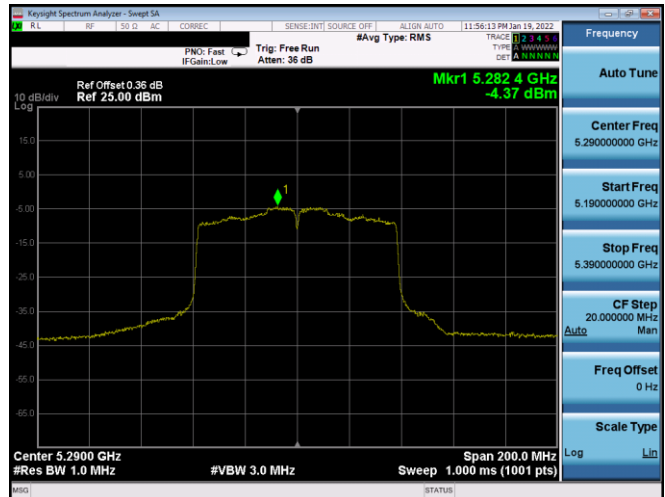
Plot 7-688. PSD CDD Diversity Antenna 3A (80MHz BW 802.11ac – Ch. 58, MCS0)
