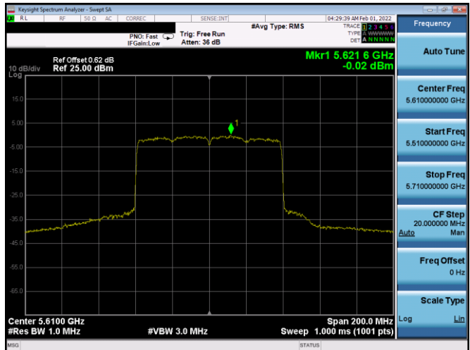
Plot 7-738. PSD CDD Diversity Antenna 3A (80MHz BW 802.11ax(SU) – Ch. 122, MCS3)
