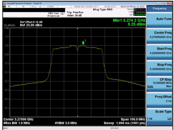
Plot 7-683. PSD CDD Diversity Antenna 2B (40MHz BW 802.11n – Ch. 54, MCS8)
