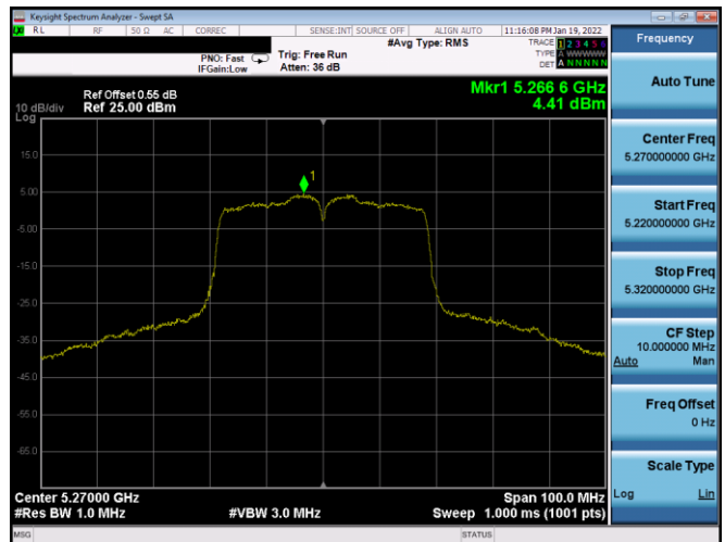
Plot 7-720. PSD CDD Diversity Antenna 3A (40MHz BW 802.11n – Ch. 54, MCS11)
