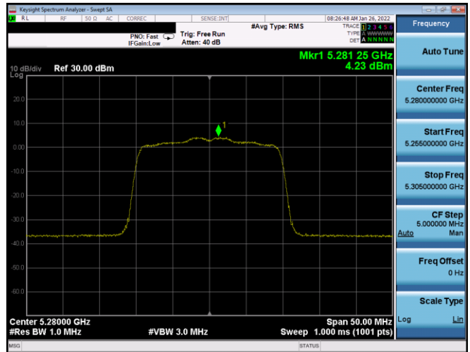
Plot 7-682. PSD CDD Diversity Antenna 3A (20MHz BW 802.11ax(SU) – Ch. 56, MCS0)
