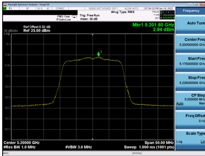
Plot 7-704. PSD CDD Diversity Antenna 3A (20MHz BW 802.11n - Ch. 40, MCS11)
