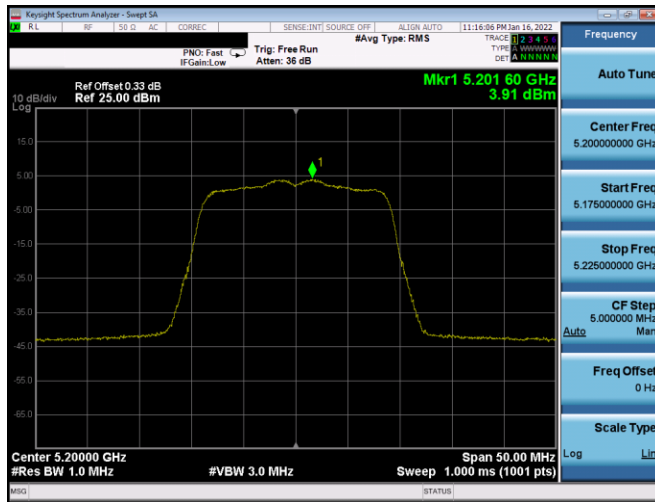
Plot 7-703. PSD CDD Diversity Antenna 2B (20MHz BW 802.11n - Ch. 40, MCS11)
