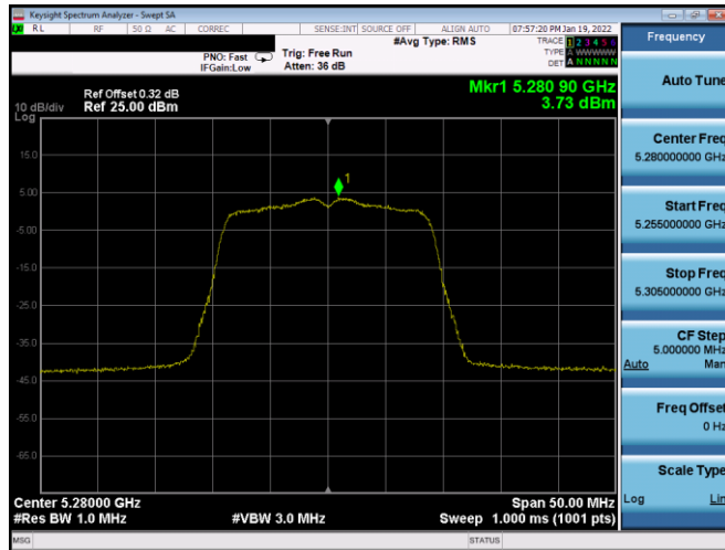
Plot 7-716. PSD CDD Diversity Antenna 3A (20MHz BW 802.11n – Ch. 56, MCS11)
