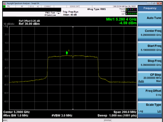
Plot 7-690. PSD CDD Diversity Antenna 3A (80MHz BW 802.11ax(SU) – Ch. 58, MCS0)
