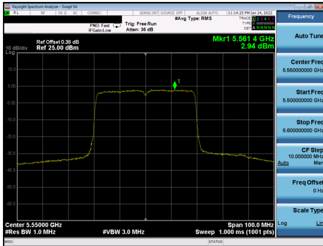
Plot 7-733. PSD CDD Diversity Antenna 2B (40MHz BW 802.11ax(SU) – Ch. 110, MCS3)
