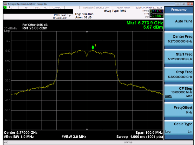
Plot 7-719. PSD CDD Diversity Antenna 2B (40MHz BW 802.11n – Ch. 54, MCS11)
