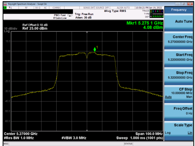
Plot 7-684. PSD CDD Diversity Antenna 3A (40MHz BW 802.11n – Ch. 54, MCS8)
