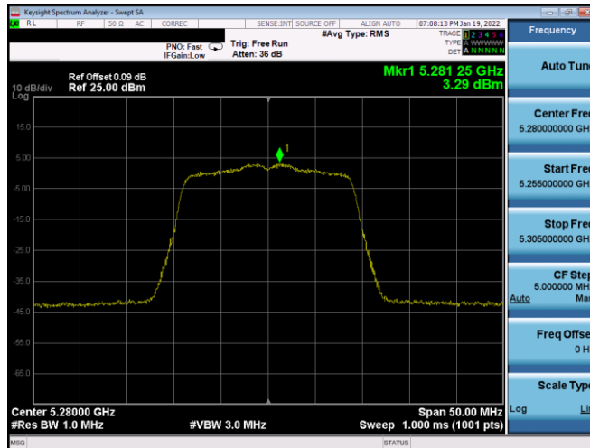
Plot 7-680. PSD CDD Diversity Antenna 3A (20MHz BW 802.11n – Ch. 56, MCS8)
