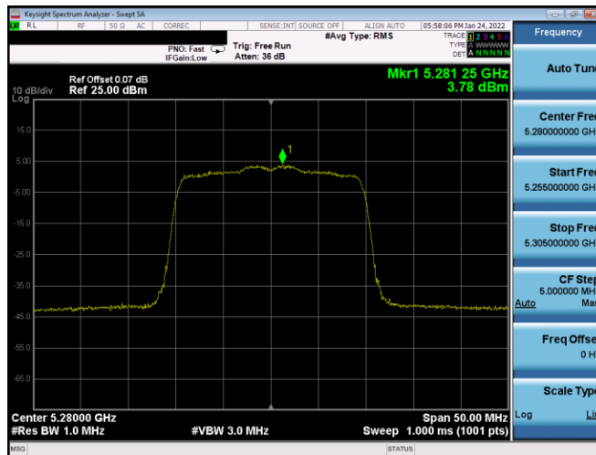
Plot 7-681. PSD CDD Diversity Antenna 2B (20MHz BW 802.11ax(SU) – Ch. 56, MCS0)
