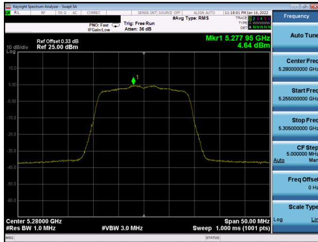
Plot 7-715. PSD CDD Diversity Antenna 2B (20MHz BW 802.11n – Ch. 56, MCS11)
