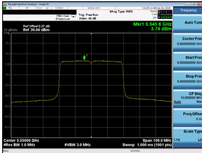
Plot 7-734. PSD CDD Diversity Antenna 3A (40MHz BW 802.11ax(SU) – Ch. 110, MCS3)
