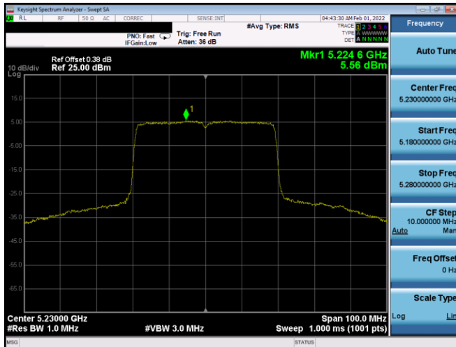
Plot 7-709. PSD CDD Diversity Antenna 2B (40MHz BW 802.11ax(SU) – Ch. 46, MCS3)
