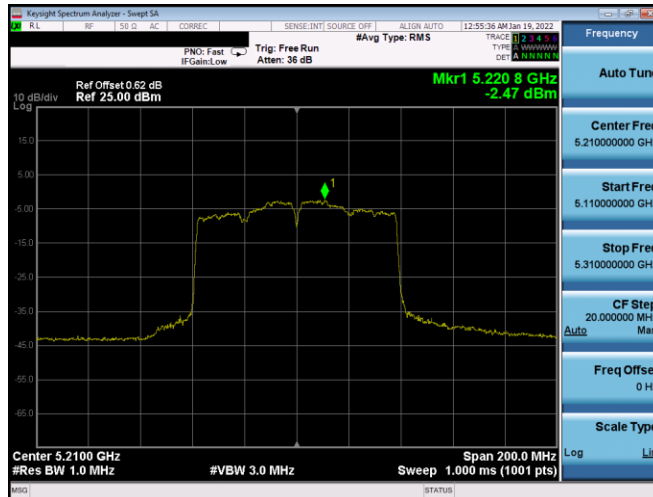
Plot 7-711. PSD CDD Diversity Antenna 2B (80MHz BW 802.11ac – Ch. 42, MCS3)
