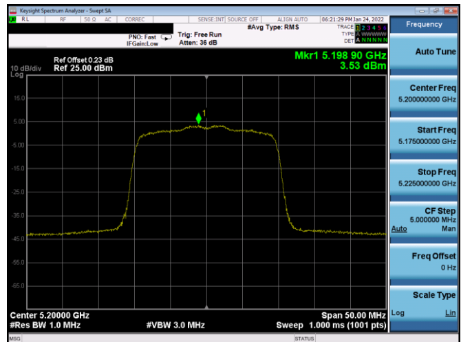
Plot 7-526. PSD CDD Primary Antenna 1B (20MHz BW 802.11ax(SU) - Ch. 40, MCS3)
