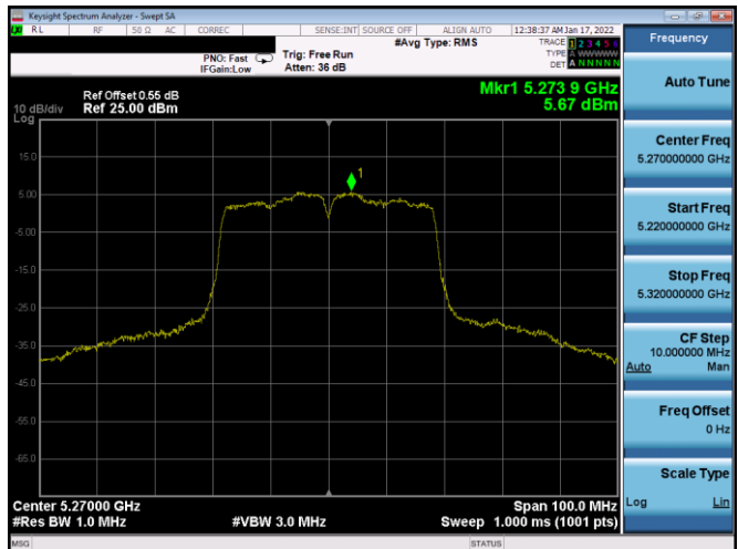
Plot 7-539. PSD CDD Primary Antenna 2B (40MHz BW 802.11n – Ch. 54, MCS11)
