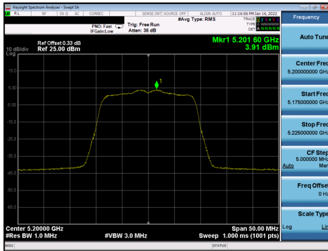
Plot 7-523. PSD CDD Primary Antenna 2B (20MHz BW 802.11n - Ch. 40, MCS11)
