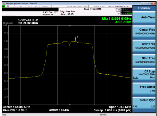
Plot 7-515. PSD CDD Primary Antenna 2B (40MHz BW 802.11n – Ch. 110, MCS8)
