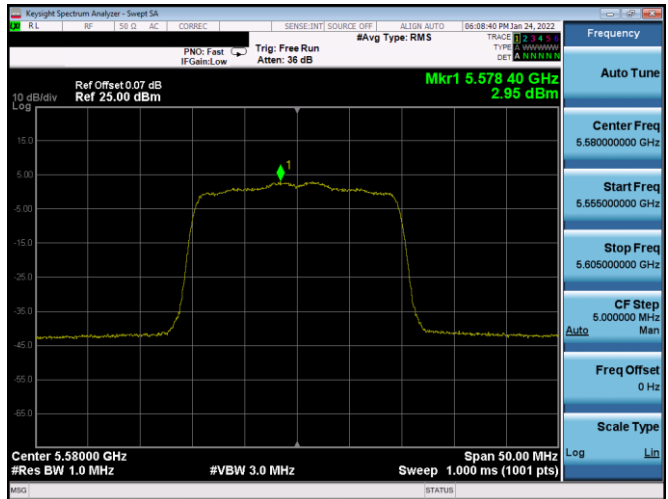
Plot 7-514. PSD CDD Primary Antenna 1B (20MHz BW 802.11ax(SU) – Ch. 116, MCS0)
