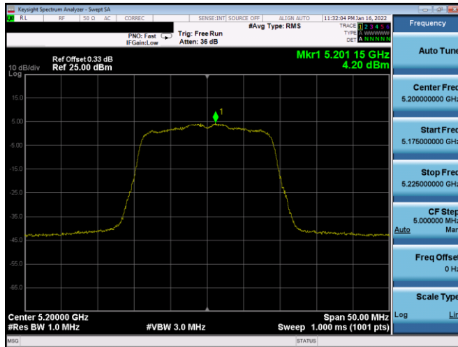
Plot 7-524. PSD CDD Primary Antenna 1B (20MHz BW 802.11n - Ch. 40, MCS11)
