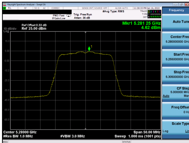
Plot 7-536. PSD CDD Primary Antenna 1B (20MHz BW 802.11n – Ch. 56, MCS11)
