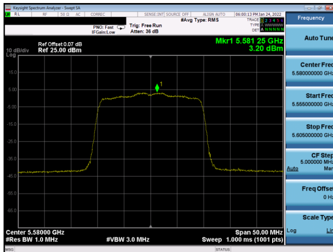
Plot 7-513. PSD CDD Primary Antenna 2B (20MHz BW 802.11ax(SU) – Ch. 116, MCS0)
