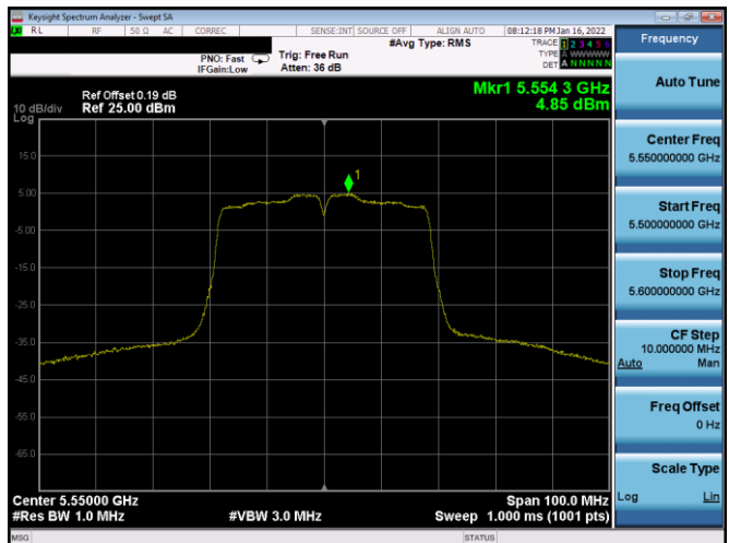
Plot 7-516. PSD CDD Primary Antenna 1B (40MHz BW 802.11n – Ch. 110, MCS8)
