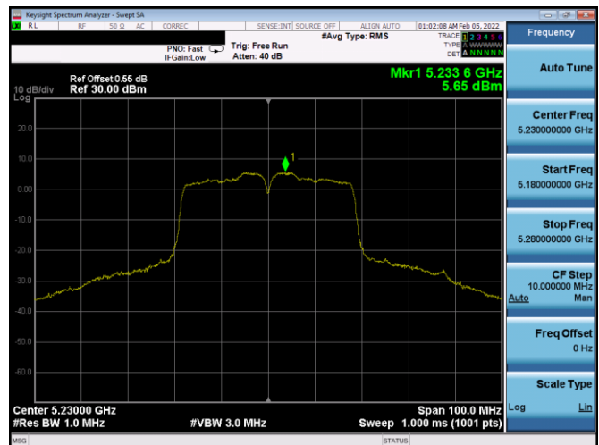
Plot 7-528. PSD CDD Antenna 1B (40MHz BW 802.11n - Ch. 46, MCS11)
