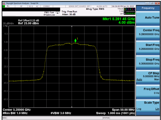
Plot 7-538. PSD CDD Primary Antenna 1B (20MHz BW 802.11ax(SU) – Ch. 56, MCS3)
