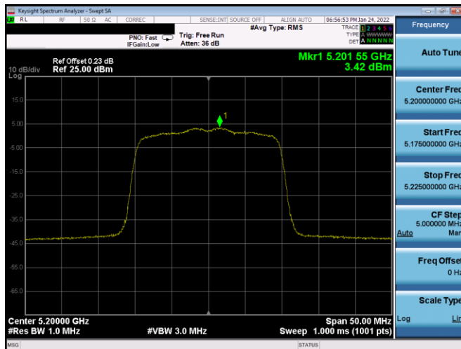
Plot 7-525. PSD CDD Primary Antenna 2B (20MHz BW 802.11ax(SU) - Ch. 40, MCS3)
