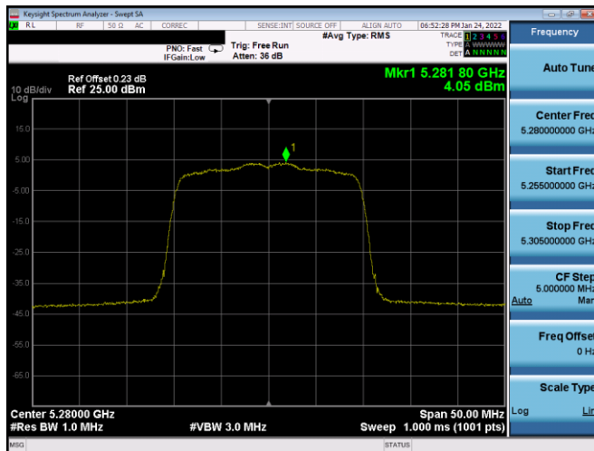
Plot 7-537. PSD CDD Primary Antenna 2B (20MHz BW 802.11ax(SU) – Ch. 56, MCS3)
