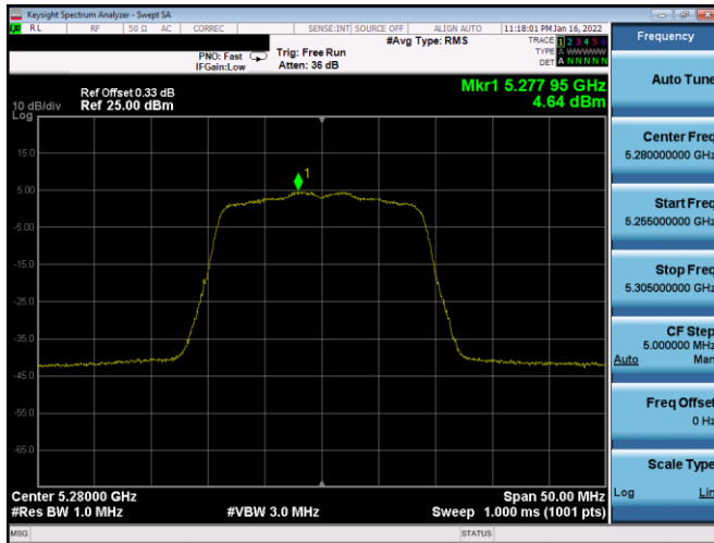
Plot 7-535. PSD CDD Primary Antenna 2B (20MHz BW 802.11n – Ch. 56, MCS11)
