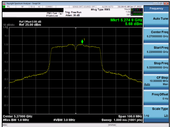
Plot 7-540. PSD CDD Primary Antenna 1B (40MHz BW 802.11n – Ch. 54, MCS11)
