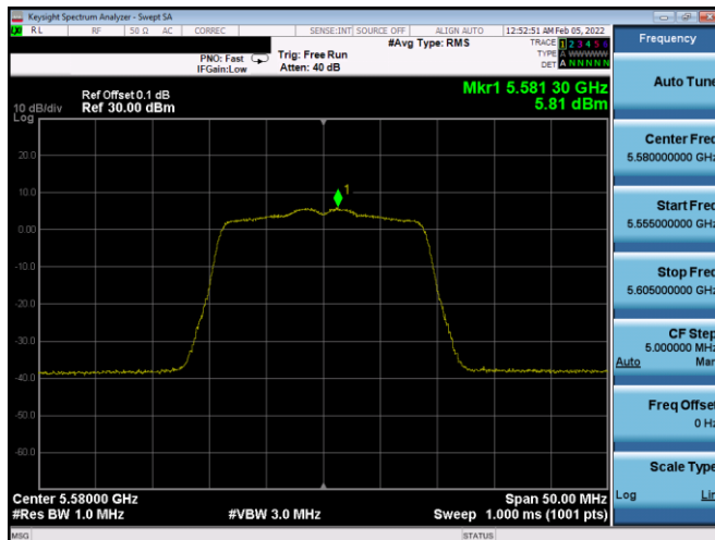
Plot 7-512. PSD CDD Primary Antenna 1B (20MHz BW 802.11n – Ch. 116, MCS8)
