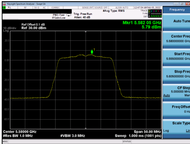
Plot 7-511. PSD CDD Primary Antenna 2B (20MHz BW 802.11n – Ch. 116, MCS8)
