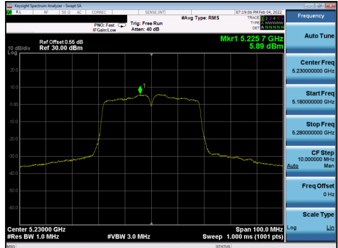
Plot 7-527. PSD CDD Primary Antenna 2B (40MHz BW 802.11n - Ch. 46, MCS11)
