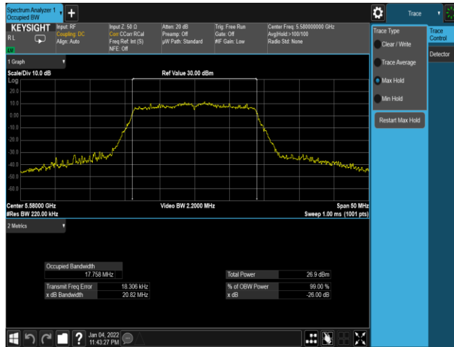
Plot 7-13. 26dB BW & 99% OBW Antenna 2B (20MHz BW 802.11n – Ch. 116, MCS0)
