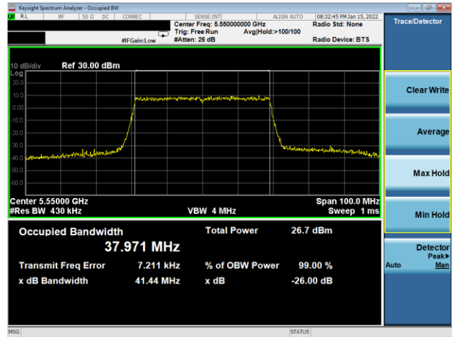
Plot 7-16. 26dB BW & 99% OBW Antenna 2B (40MHz BW 802.11ax(SU) – Ch. 110, MCS0)
