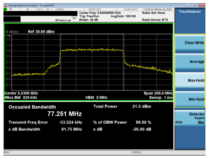
Plot 7-18. 26dB BW & 99% OBW Antenna 2B (80MHz BW 802.11ax(SU) – Ch. 106, MCS0)
