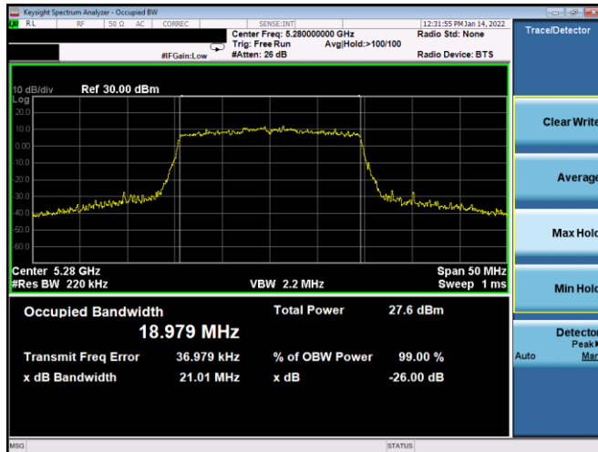
Plot 7-62. 26dB BW & 99% OBW Antenna 1B (20MHz BW 802.11ax(SU) – Ch. 56, MCS0)
