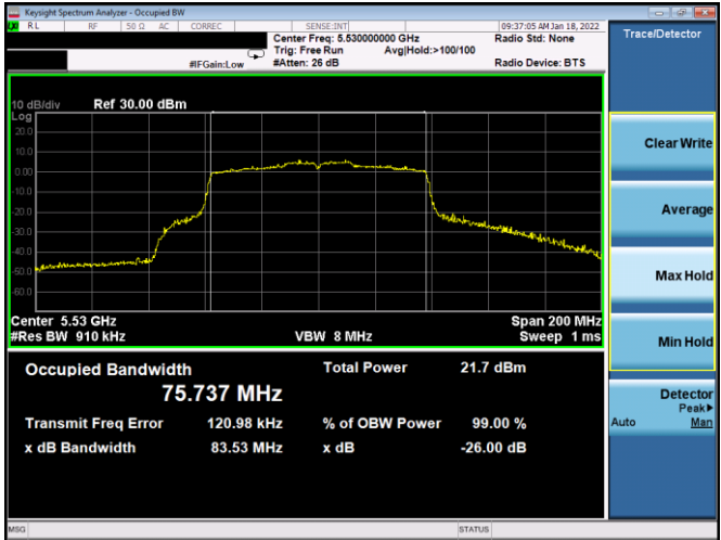
Plot 7-17. 26dB BW & 99% OBW Antenna 2B (80MHz BW 802.11ac – Ch. 106, MCS0)
