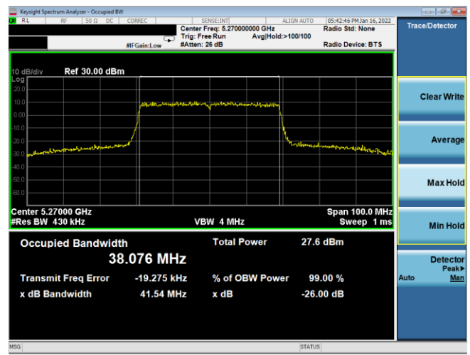
Plot 7-64. 26dB BW & 99% OBW Antenna 1B (40MHz BW 802.11ax(SU) – Ch. 54, MCS0)
