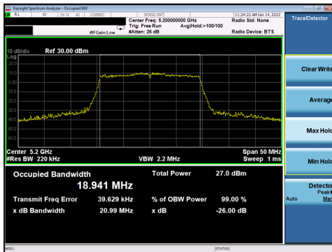
Plot 7-56. 26dB BW & 99% OBW Antenna 1B (20MHz BW 802.11ax(SU) – Ch. 40, MCS0)
