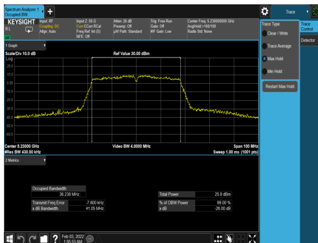
Plot 7-57. 26dB BW & 99% OBW Antenna 1B (40MHz BW 802.11n – Ch. 46, MCS0)
