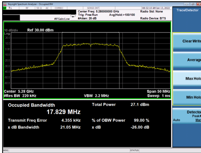
Plot 7-61. 26dB BW & 99% OBW Antenna 1B (20MHz BW 802.11n – Ch. 56, MCS0)
