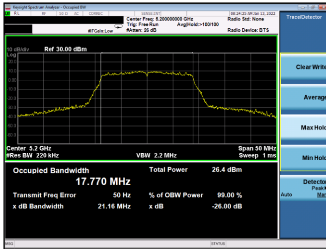
Plot 7-55. 26dB BW & 99% OBW Antenna 1B (20MHz BW 802.11n – Ch. 40, MCS0)
