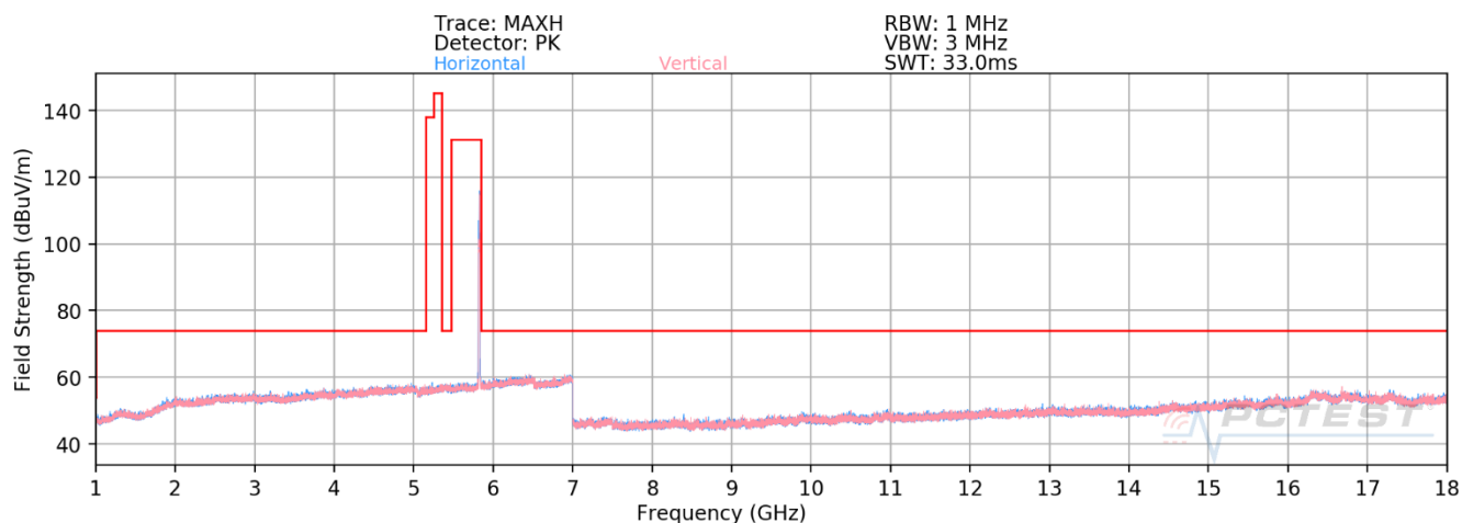
Plot 7-576. RSE above 1GHz Antenna 2b (11ax – Ch.165 – RU26)
