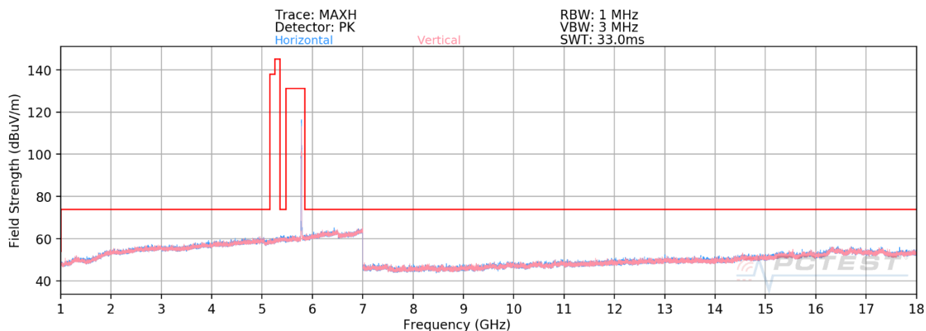
Plot 7-575. RSE above 1GHz Antenna 2b (11ax – Ch.157 – RU26)
