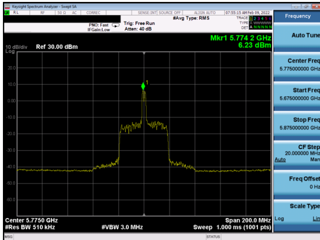
Plot 7-536. PSD CDD Diversity Antenna 3a (80MHz BW 11ax Index 18 - RU26 - Ch.155)
