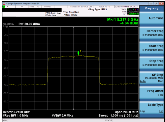
Plot 7-564. ISED PSD CDD Diversity Antenna 3a (80MHz BW 11ax - RU996 - Ch.42)
