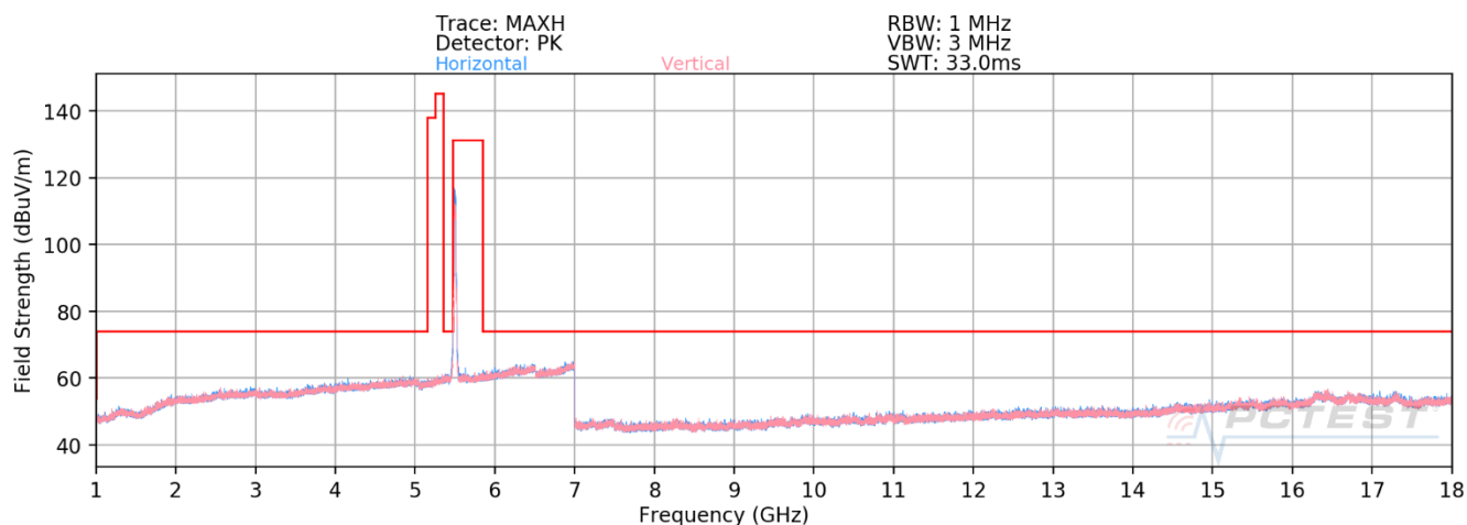
Plot 7-583. RSE above 1GHz Antenna 2b (11ax – Ch.100 – RU242)
