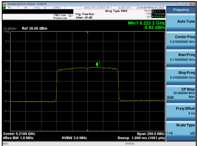
Plot 7-563. ISED PSD CDD Diversity Antenna 2b (80MHz BW 11ax - RU996 - Ch.42)
