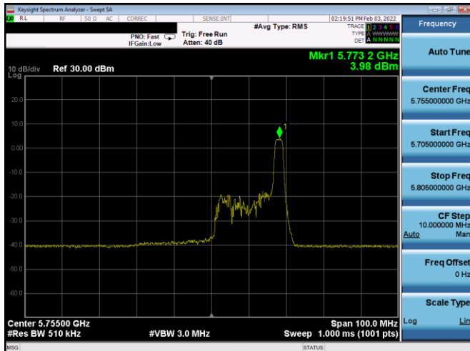
Plot 7-530. PSD CDD Diversity Antenna 3a (40MHz BW 11ax Index 17 – RU26 – Ch.151)
