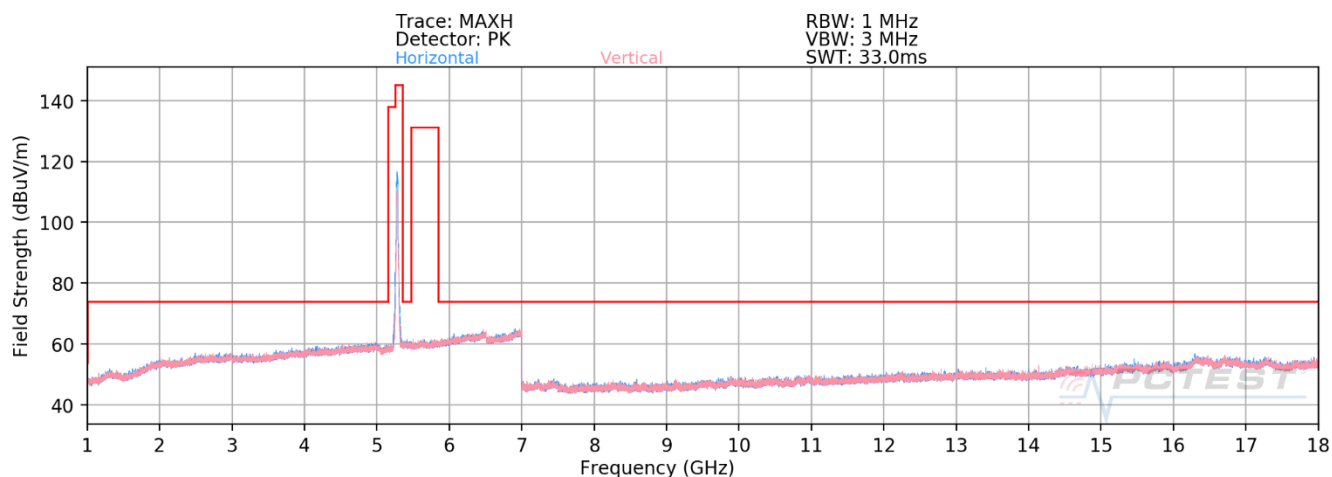
Plot 7-581. RSE above 1GHz Antenna 2b (11ax – Ch.56 – RU242)
