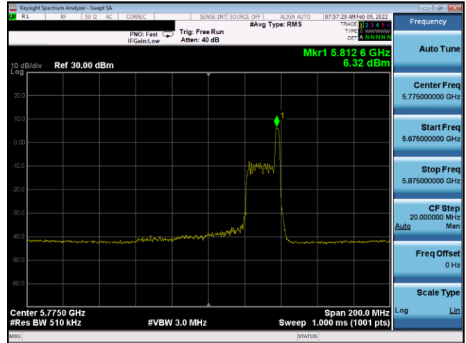
Plot 7-538. PSD CDD Diversity Antenna 3a (80MHz BW 11ax Index 36 - RU26 - Ch.155)
