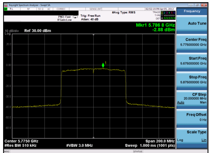
Plot 7-540. PSD CDD Diversity Antenna 3a (80MHz BW 11ax - RU996 - Ch.155)
