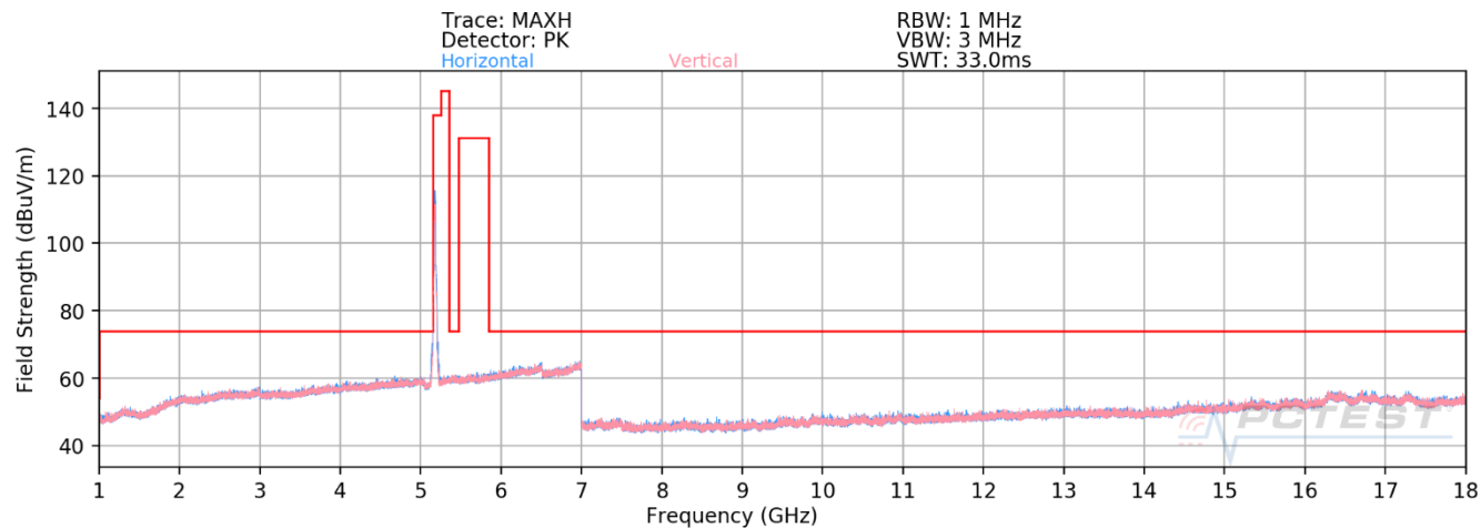
Plot 7-577. RSE above 1GHz Antenna 2b (11ax – Ch.36 – RU242)
