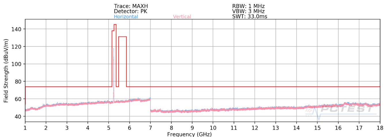
Plot 7-567. RSE above 1GHz Antenna 2b (11ax – Ch.48 – RU26)
