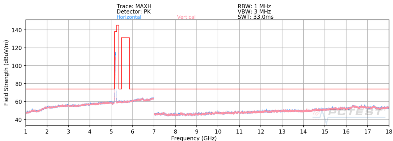
Plot 7-578. RSE above 1GHz Antenna 2b (11ax – Ch.40 – RU242)
