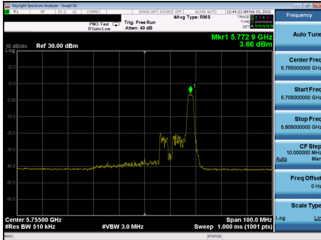
Plot 7-529. PSD CDD Diversity Antenna 2b (40MHz BW 11ax Index 17 – RU26 – Ch.151)
