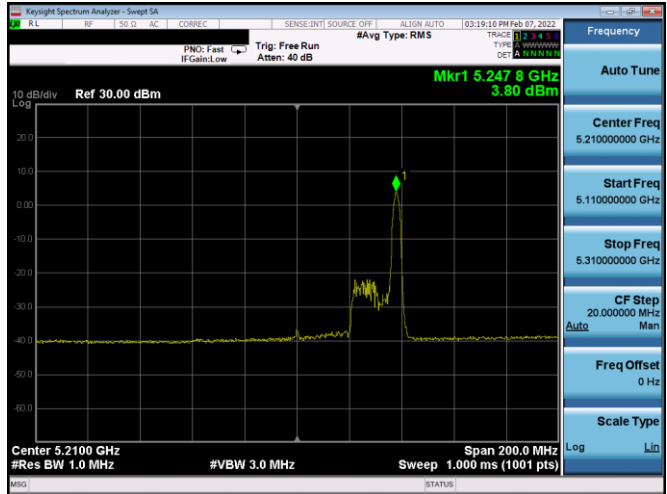
Plot 7-562. ISED PSD SDM Diversity Antenna 3a (80MHz BW 11ax Index 36 - RU26 - Ch.42)
