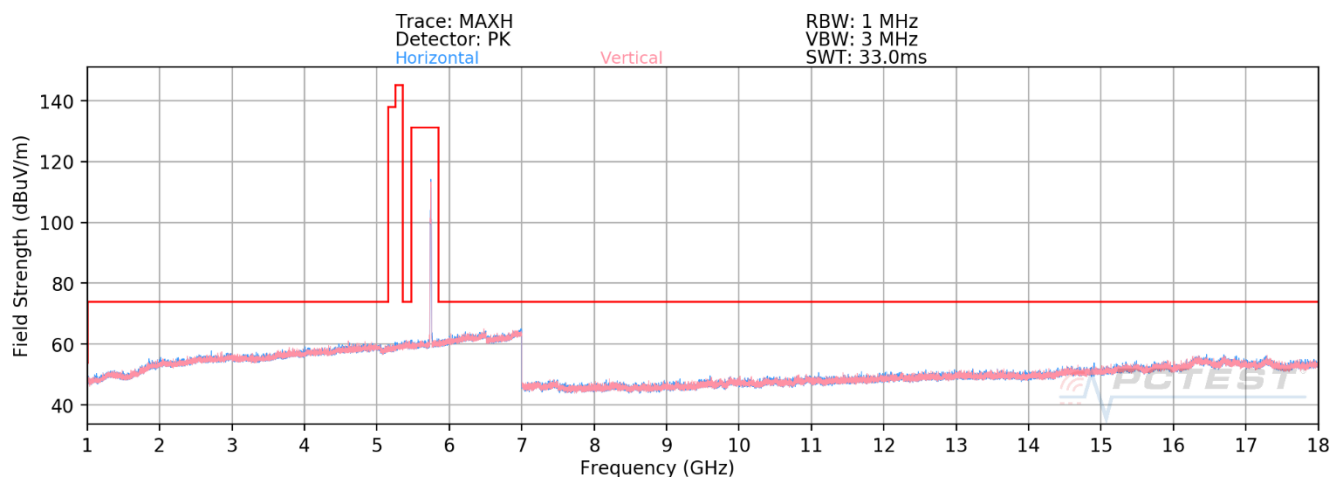
Plot 7-574. RSE above 1GHz Antenna 2b (11ax – Ch.149 – RU26)
