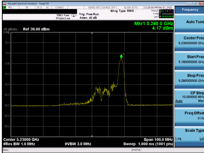
Plot 7-553. ISED PSD SDM Diversity Antenna 2b (40MHz BW 11ax Index 17 – RU26 – Ch.46)
