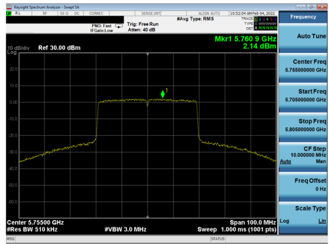
Plot 7-532. PSD CDD Diversity Antenna 3a (40MHz BW 11ax – RU484 – Ch.151)
