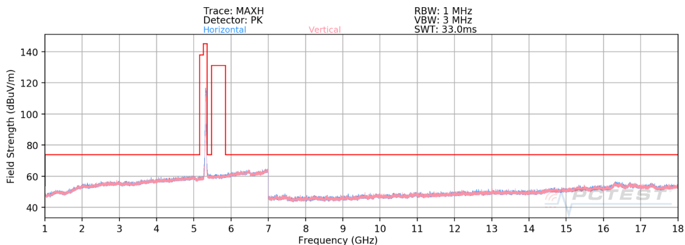
Plot 7-582. RSE above 1GHz Antenna 2b (11ax – Ch.64 – RU242)
