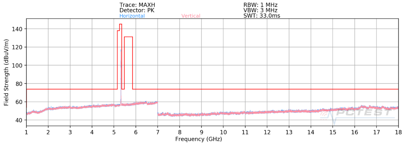
Plot 7-570. RSE above 1GHz Antenna 2b (11ax – Ch.64 – RU26)
