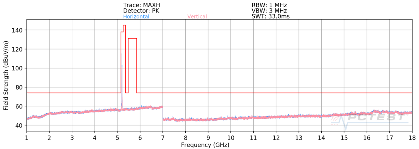
Plot 7-566. RSE above 1GHz Antenna 2b (11ax – Ch.40 – RU26)
