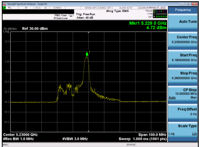
Plot 7-551. ISPD PSD SDM Diversity Antenna 2b (40MHz BW 11ax Index 8 - RU26 - Ch.46)
