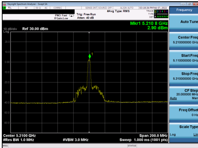
Plot 7-560. ISED PSD SDM Diversity Antenna 3a (80MHz BW 11ax Index 18 - RU26 - Ch.42)
