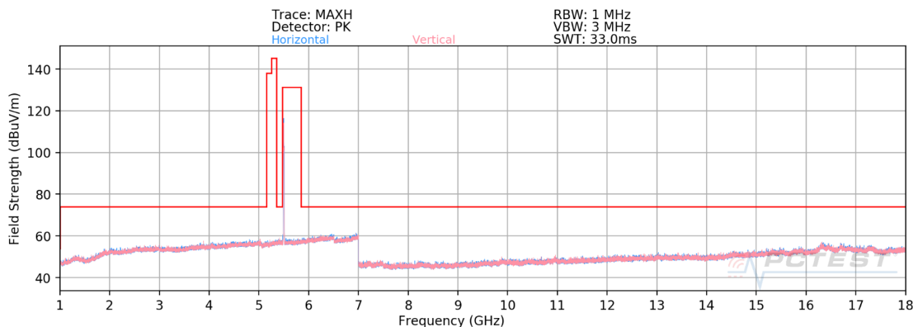
Plot 7-571. RSE above 1GHz Antenna 2b (11ax – Ch.100 – RU26)
