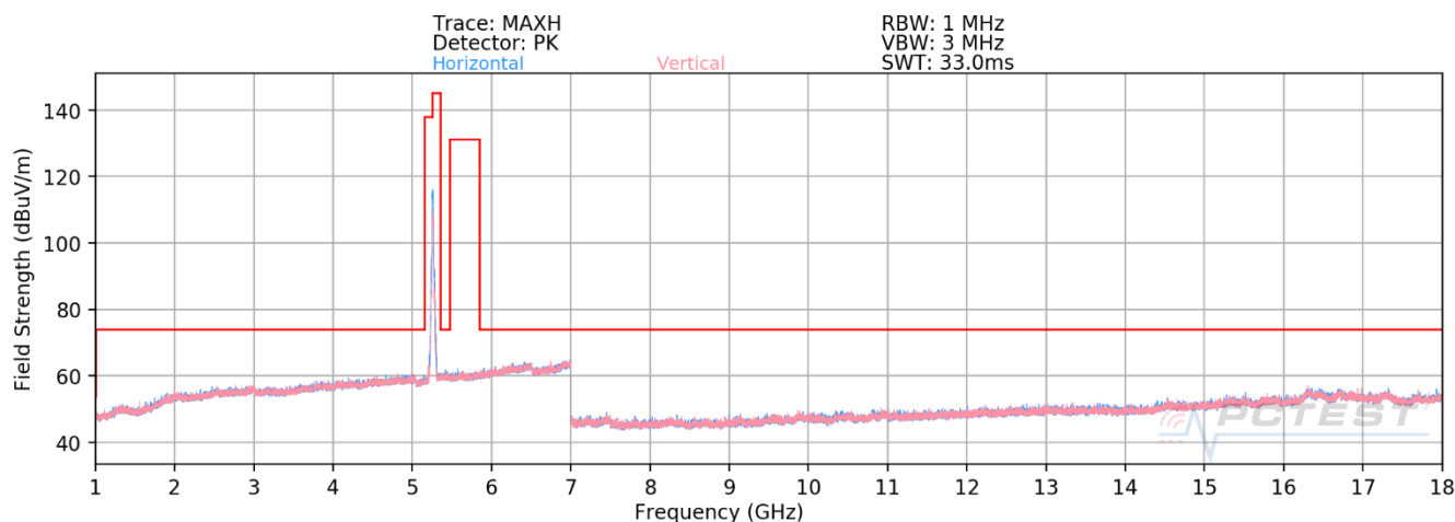
Plot 7-580. RSE above 1GHz Antenna 2b (11ax – Ch.52 – RU242)
