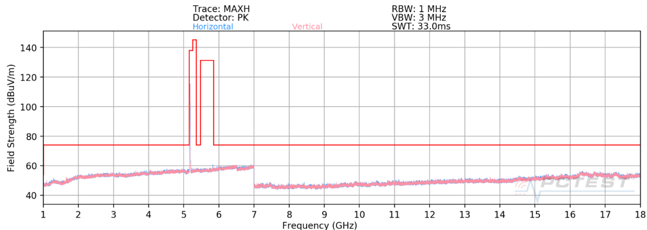
Plot 7-565. RSE above 1GHz Antenna 2b (11ax – Ch.36 – RU26)
