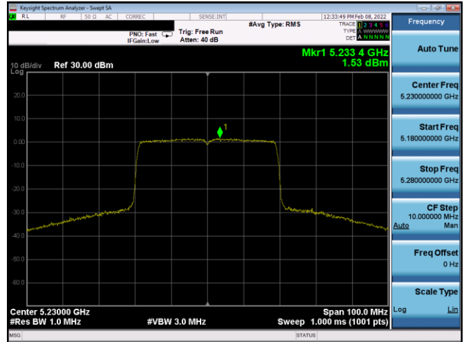
Plot 7-556. ISED PSD SDM Diversity Antenna 3a (40MHz BW 11ax – RU484 – Ch.46)
