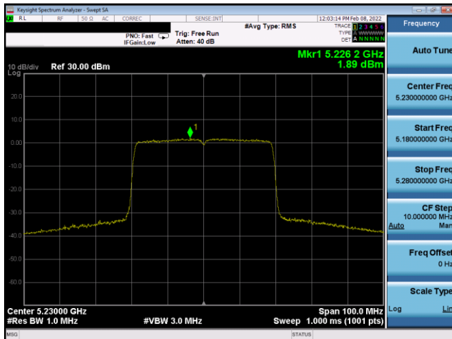
Plot 7-555. ISED PSD SDM Diversity Antenna 2b (40MHz BW 11ax – RU484 – Ch.46)
