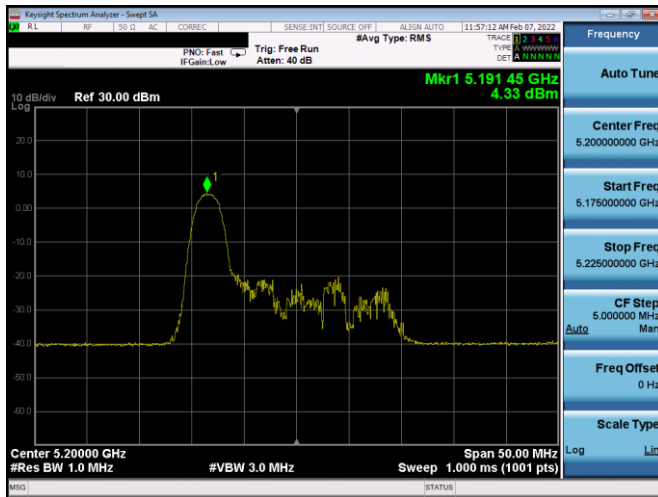
Plot 7-541. ISED PSD SDM Diversity Antenna 2b (20MHz BW 11ax Index 0 – RU26 – Ch.40)
