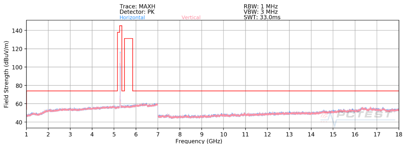
Plot 7-569. RSE above 1GHz Antenna 2b (11ax – Ch.56 – RU26)
