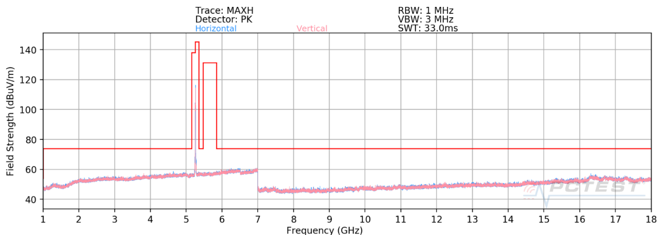
Plot 7-568. RSE above 1GHz Antenna 2b (11ax – Ch.52 – RU26)
