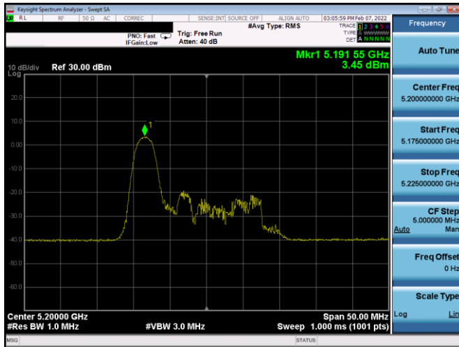
Plot 7-542. ISED PSD SDM Diversity Antenna 3a (20MHz BW 11ax Index 0 – RU26 – Ch.40)
