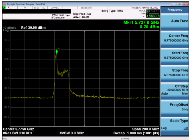
Plot 7-533. PSD CDD Diversity Antenna 2b (80MHz BW 11ax Index 0 – RU26 – Ch.155)
