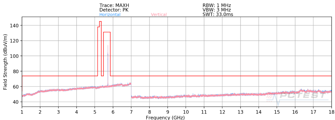
Plot 7-573. RSE above 1GHz Antenna 2b (11ax – Ch.144 – RU26)
