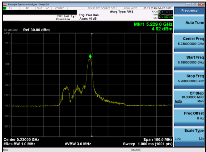
Plot 7-552. ISPD PSD SDM Diversity Antenna 3a (40MHz BW 11ax Index 8 - RU26 - Ch.46)
