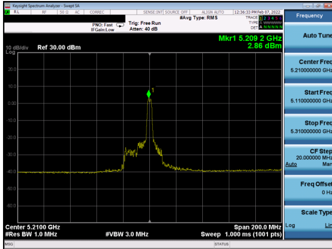
Plot 7-559. ISED PSD SDM Diversity Antenna 2b (80MHz BW 11ax Index 18 - RU26 - Ch.42)
