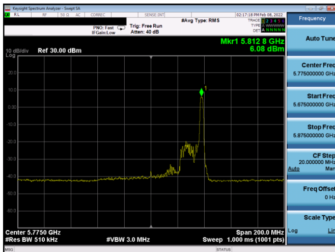
Plot 7-537. PSD CDD Diversity Antenna 2b (80MHz BW 11ax Index 36 - RU26 - Ch.155)
