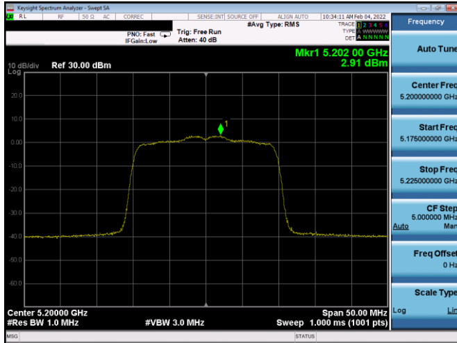
Plot 7-547. ISPD PSD SDM Diversity Antenna 2b (20MHz BW 11ax- RU242 - Ch.40)
