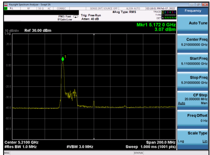
Plot 7-558. ISED PSD SDM Diversity Antenna 3a (80MHz BW 11ax Index 0 – RU26 – Ch.42)
