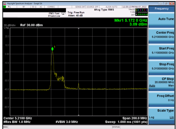
Plot 7-557. ISED PSD SDM Diversity Antenna 2b (80MHz BW 11ax Index 0 – RU26 – Ch.42)
