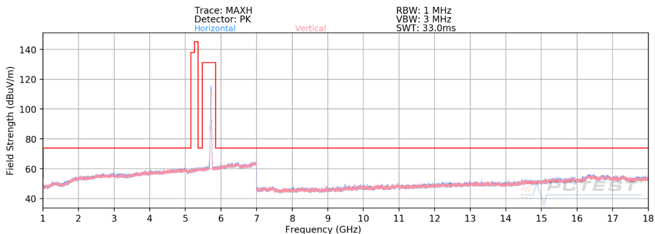
Plot 7-585. RSE above 1GHz Antenna 2b (11ax – Ch.144 – RU242)
