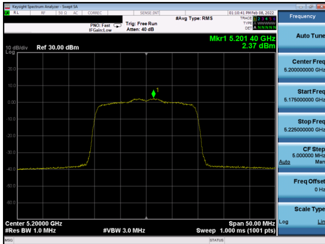
Plot 7-548. ISPD PSD SDM Diversity Antenna 3a (20MHz BW 11ax- RU242 - Ch.40)
