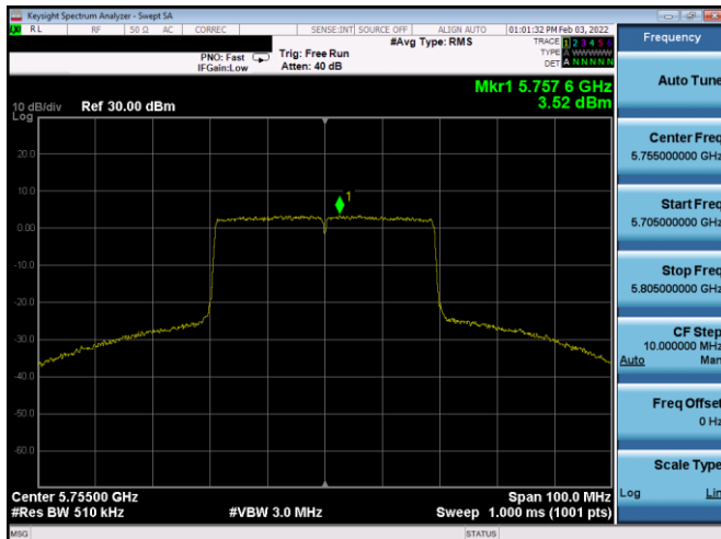
Plot 7-531. PSD CDD Diversity Antenna 2b (40MHz BW 11ax – RU484 – Ch.151)
