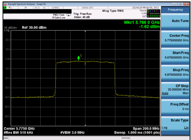
Plot 7-539. PSD CDD Diversity Antenna 2b (80MHz BW 11ax - RU996 - Ch.155)
