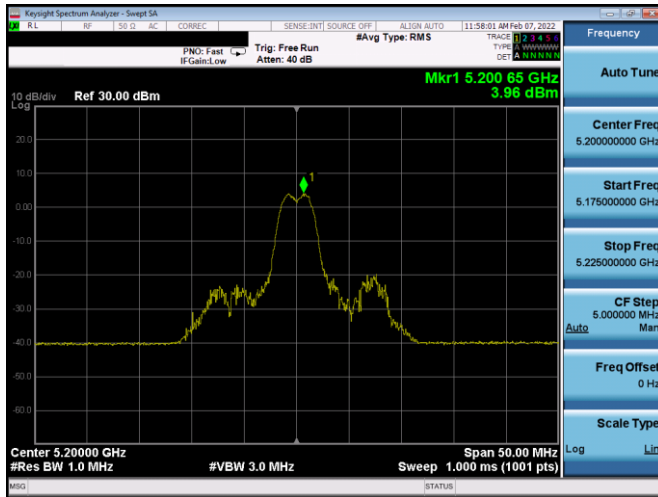
Plot 7-543. ISED PSD SDM Diversity Antenna 2b (20MHz BW 11ax Index 4 – RU26 – Ch.40)
