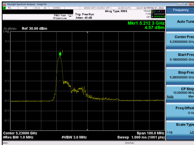
Plot 7-549. ISPD PSD SDM Diversity Antenna 2b (40MHz BW 11ax Index 0 - RU26 - Ch.46)
