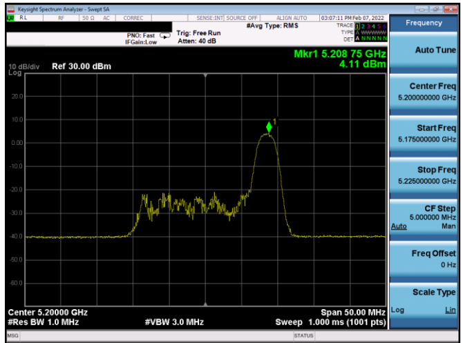
Plot 7-546. ISED PSD SDM Diversity Antenna 3a (20MHz BW 11ax Index 8 – RU26 – Ch.40)
