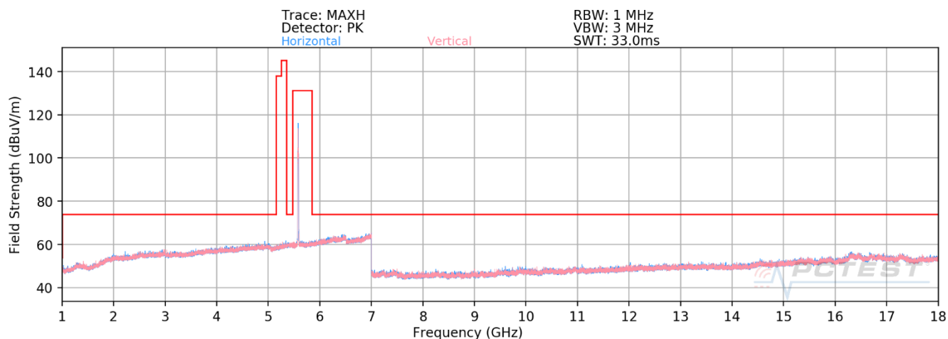
Plot 7-572. RSE above 1GHz Antenna 2b (11ax – Ch.116 – RU26)
