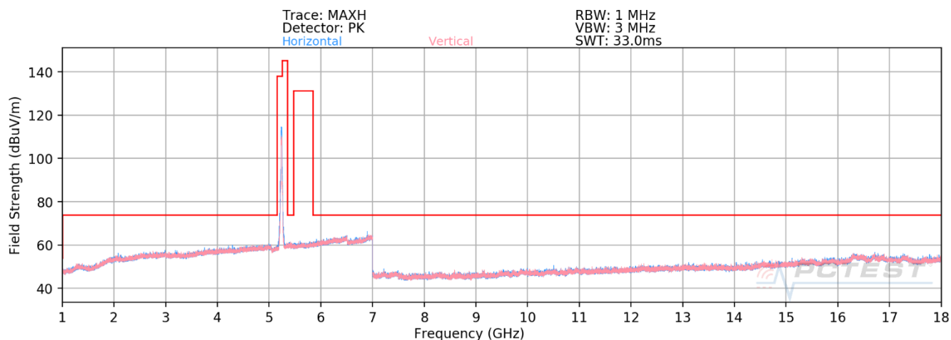
Plot 7-579. RSE above 1GHz Antenna 2b (11ax – Ch.48 – RU242)
