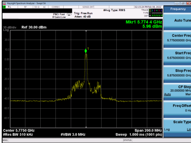
Plot 7-535. PSD CDD Diversity Antenna 2b (80MHz BW 11ax Index 18 - RU26 - Ch.155)
