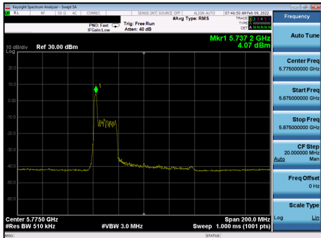
Plot 7-534. PSD CDD Diversity Antenna 3a (80MHz BW 11ax Index 0 – RU26 – Ch.155)
