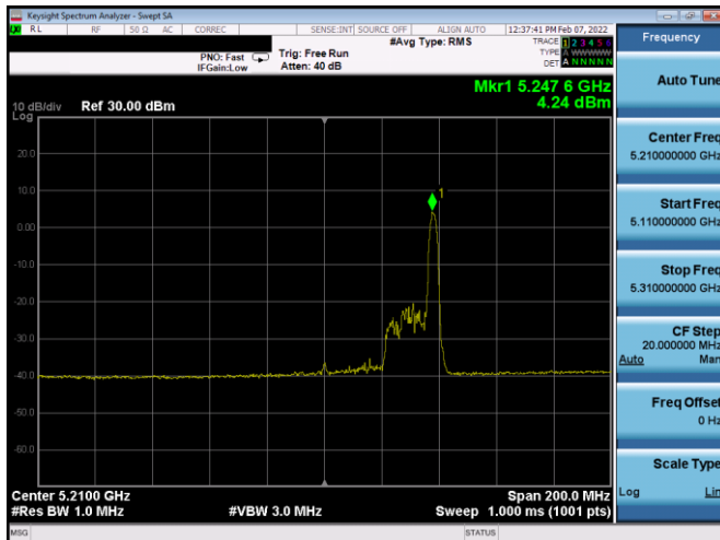
Plot 7-561. ISED PSD SDM Diversity Antenna 2b (80MHz BW 11ax Index 36 - RU26 - Ch.42)
