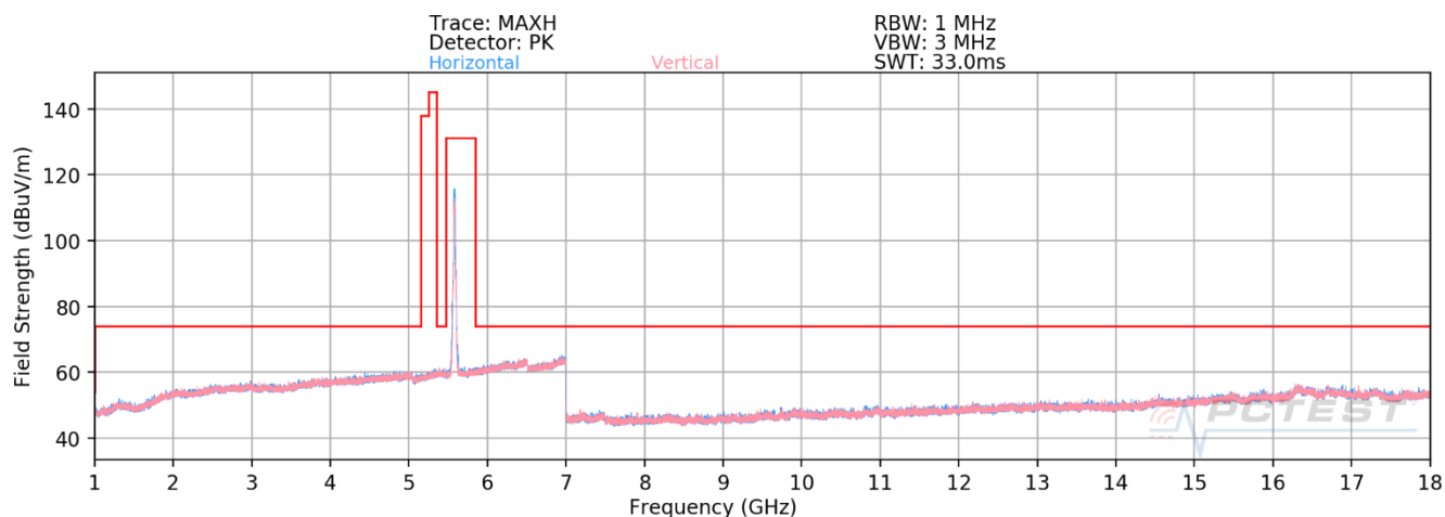
Plot 7-584. RSE above 1GHz Antenna 2b (11ax – Ch.116 – RU242)
