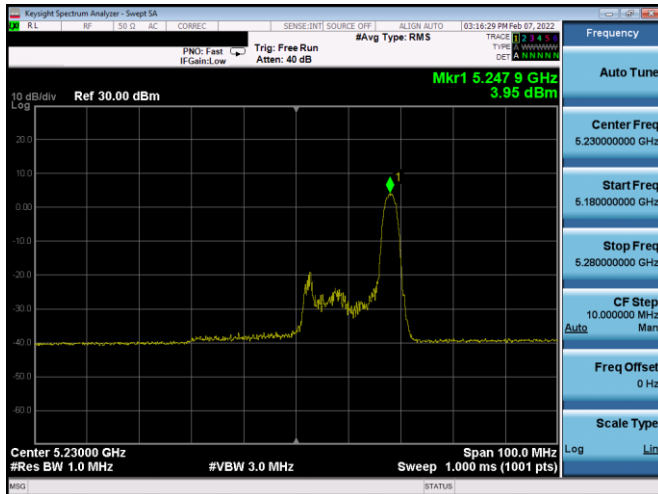
Plot 7-554. ISED PSD SDM Diversity Antenna 3a (40MHz BW 11ax Index 17 – RU26 – Ch.46)
