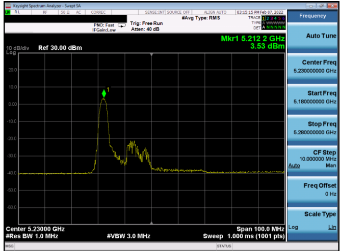
Plot 7-550. ISPD PSD SDM Diversity Antenna 3a (40MHz BW 11ax Index 0 - RU26 - Ch.46)
