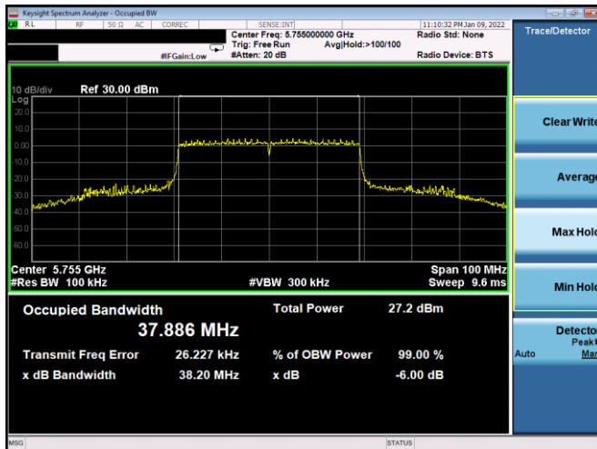
Plot 7-140. 6dB BW & 99% OBW Antenna 3a (40MHz BW 11ax – RU484 – Ch.151)
