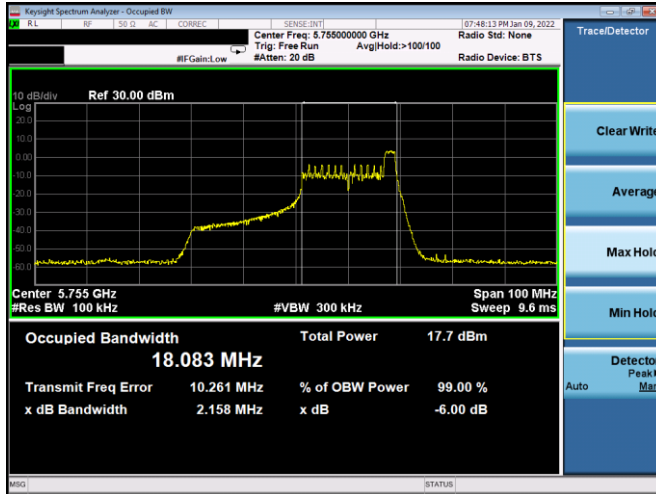
Plot 7-139. 6dB BW & 99% OBW Antenna 3a (40MHz BW 11ax Index 17 – RU26 – Ch.151)
