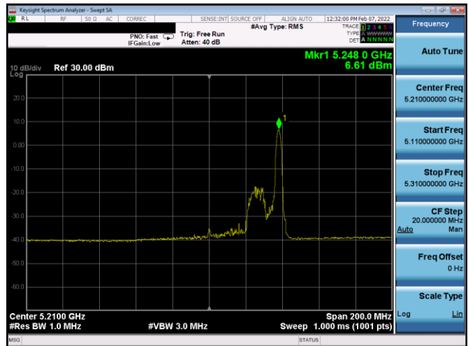
Plot 7-155. PSD Antenna 2b (80MHz BW 11ax Index 36 – RU26 – Ch.42)
