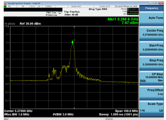
Plot 7-162. PSD Antenna 2b (40MHz BW 11ax Index 8 – RU26 – Ch.54)
