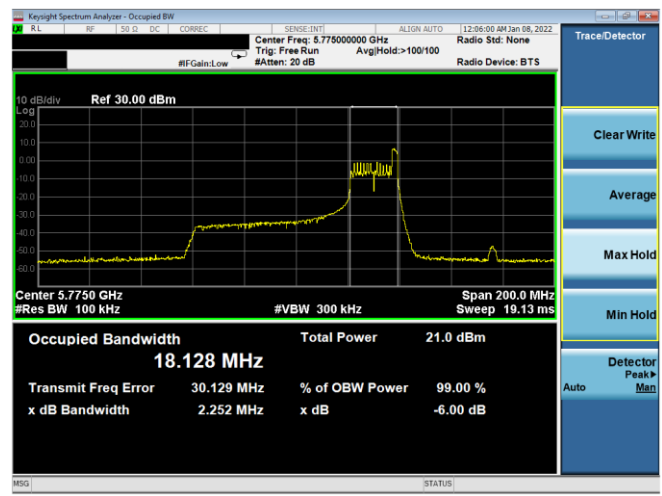
Plot 7-119. 6dB BW & 99% OBW Antenna 2b (80MHz BW 11ax Index 36 - RU26 - Ch.155)
