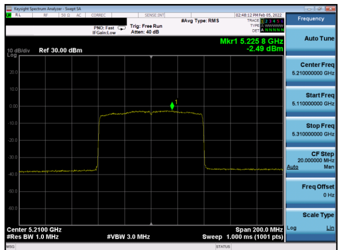
Plot 7-156. PSD Antenna 2b (80MHz BW 11ax – RU996 – Ch.42)
