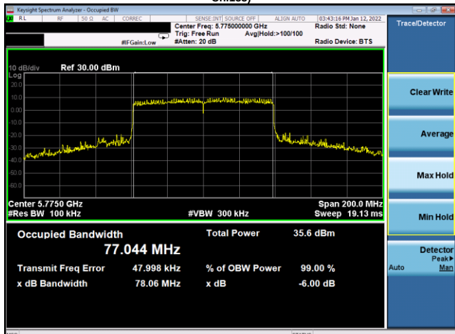
Plot 7-132. 6dB BW & 99% OBW Antenna 1b (80MHz BW 11ax – RU996 – Ch.155)
