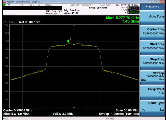
Plot 7-160. PSD Antenna 2b (20MHz BW 11ax– RU242 – Ch.56)
