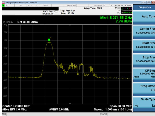
Plot 7-157. PSD Antenna 2b (20MHz BW 11ax Index 0 – RU26 – Ch.56)
