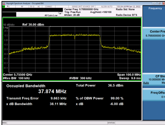
Plot 7-128. 6dB BW & 99% OBW Antenna 1b (40MHz BW 11ax – RU484 – Ch.151)
