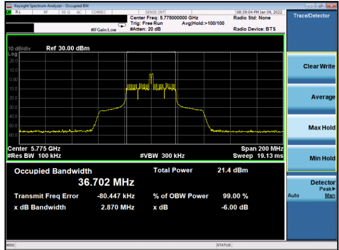
Plot 7-142. 6dB BW & 99% OBW Antenna 3a (80MHz BW 11ax Index 18 – RU26 – Ch.155)
