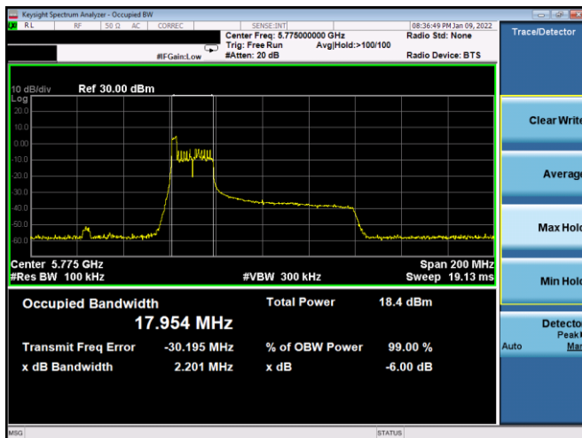
Plot 7-141. 6dB BW & 99% OBW Antenna 3a (80MHz BW 11ax Index 0 – RU26 – Ch.155)
