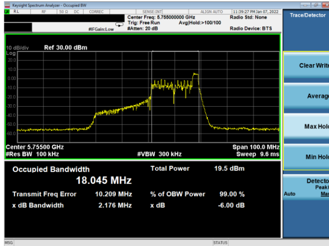
Plot 7-115. 6dB BW & 99% OBW Antenna 2b (40MHz BW 11ax Index 17 - RU26 - Ch.151)
