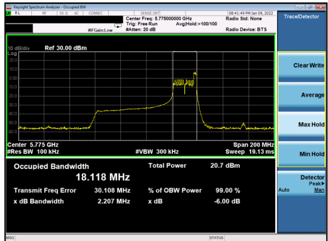
Plot 7-143. 6dB BW & 99% OBW Antenna 3a (80MHz BW 11ax Index 36 – RU26 – Ch.155)
