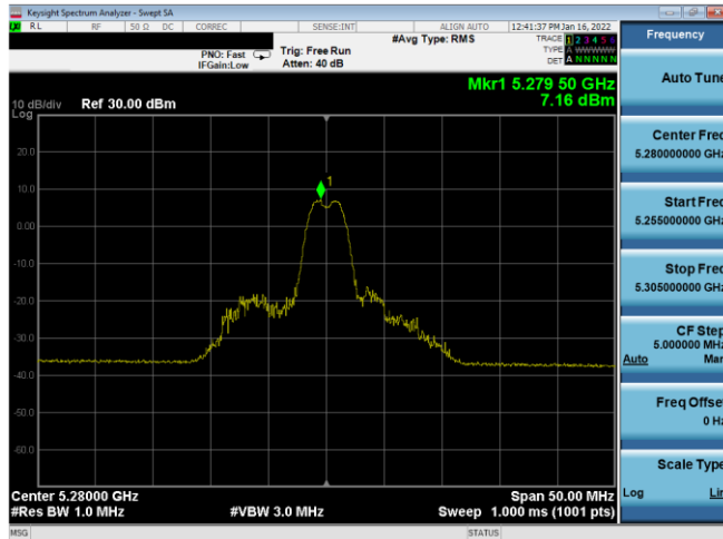
Plot 7-158. PSD Antenna 2b (20MHz BW 11ax Index 4 – RU26 – Ch.56)
