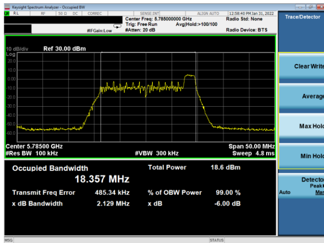
Plot 7-123. 6dB BW & 99% OBW Antenna 1b (20MHz BW 11ax Index 8– RU26 – Ch.157)
