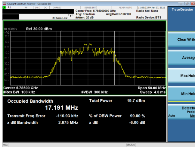
Plot 7-110. 6dB BW & 99% OBW Antenna 2b (20MHz BW 11ax Index 4 – RU26 – Ch.157)
