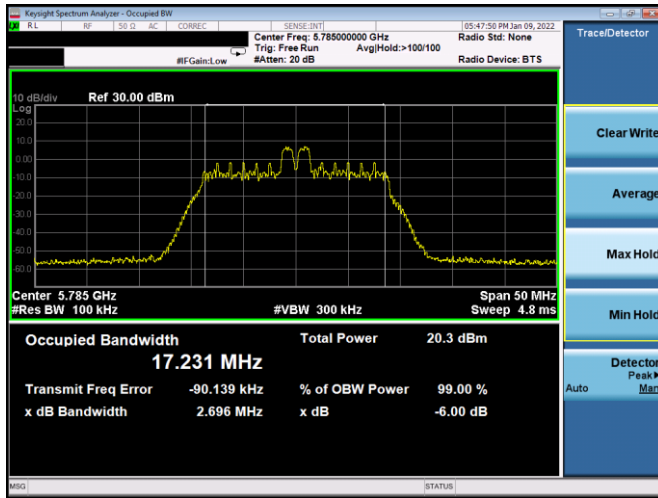
Plot 7-134. 6dB BW & 99% OBW Antenna 3a (20MHz BW 11ax Index 4 – RU26 – Ch.157)
