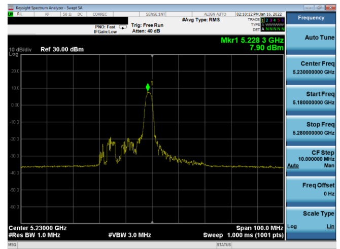
Plot 7-150. PSD Antenna 2b (40MHz BW 11ax Index 8 – RU26 – Ch.46)
