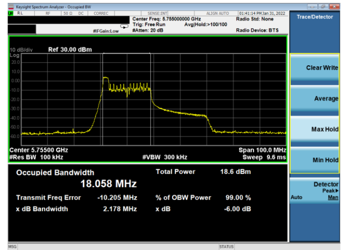
Plot 7-125. 6dB BW & 99% OBW Antenna 1b (40MHz BW 11ax Index 0 – RU26 – Ch.151)
