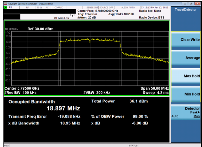
Plot 7-124. 6dB BW & 99% OBW Antenna 1b (20MHz BW 11ax– RU242 – Ch.157)
