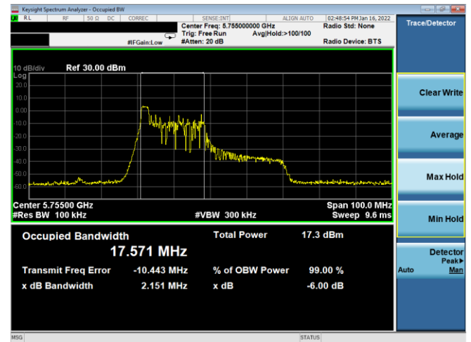
Plot 7-113. 6dB BW & 99% OBW Antenna 2b (40MHz BW 11ax Index 0 – RU26 – Ch.151)
