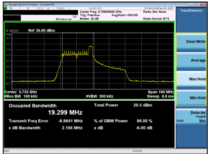
Plot 7-138. 6dB BW & 99% OBW Antenna 3a (40MHz BW 11ax Index 8 – RU26 – Ch.151)
