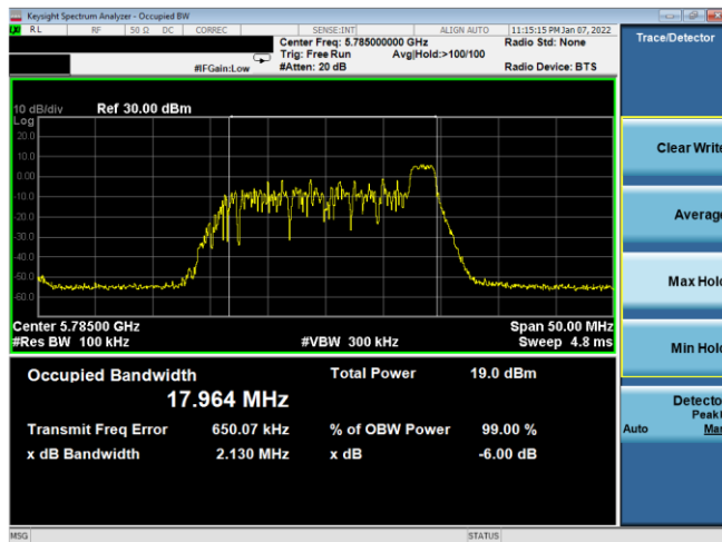
Plot 7-111. 6dB BW & 99% OBW Antenna 2b (20MHz BW 11ax Index 8– RU26 – Ch.157)
