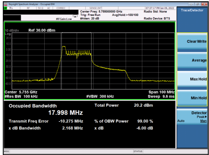
Plot 7-137. 6dB BW & 99% OBW Antenna 3a (40MHz BW 11ax Index 0 – RU26 – Ch.151)
