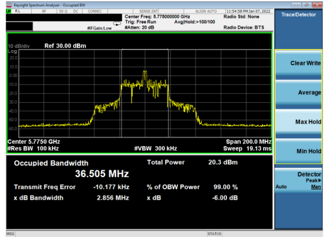
Plot 7-118. 6dB BW & 99% OBW Antenna 2b (80MHz BW 11ax Index 18 - RU26 - Ch.155)
