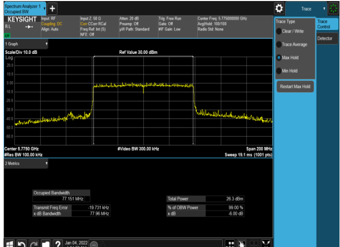
Plot 7-120. 6dB BW & 99% OBW Antenna 2b (80MHz BW 11ax - RU996 - Ch.155)
