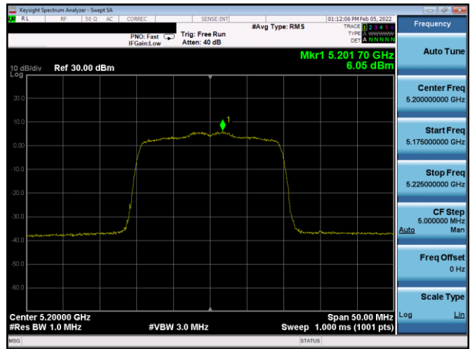
Plot 7-148. PSD Antenna 2b (20MHz BW 11ax– RU242 – Ch.40)
