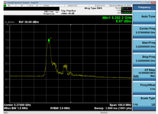
Plot 7-161. PSD Antenna 2b (40MHz BW 11ax Index 0 – RU26 – Ch.54)
