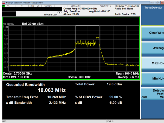
Plot 7-127. 6dB BW & 99% OBW Antenna 1b (40MHz BW 11ax Index 17 – RU26 – Ch.151)
