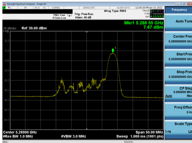
Plot 7-159. PSD Antenna 2b (20MHz BW 11ax Index 8– RU26 – Ch.56)
