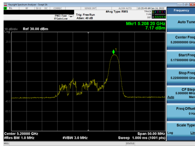
Plot 7-147. PSD Antenna 2b (20MHz BW 11ax Index 8– RU26 – Ch.40)
