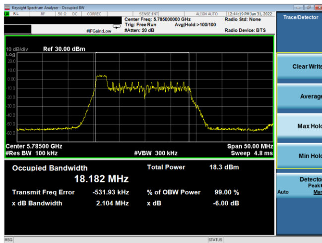
Plot 7-121. 6dB BW & 99% OBW Antenna 1b (20MHz BW 11ax Index 0 – RU26 – Ch.157)
