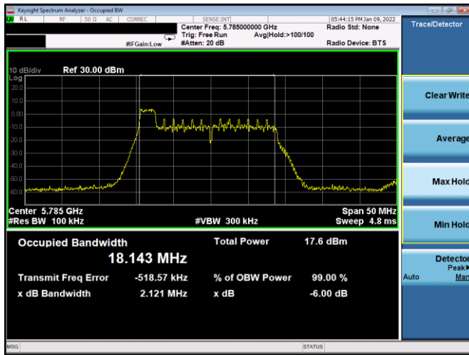
Plot 7-133. 6dB BW & 99% OBW Antenna 3a (20MHz BW 11ax Index 0 – RU26 – Ch.157)
