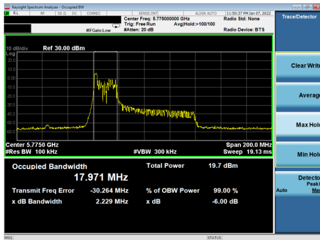
Plot 7-117. 6dB BW & 99% OBW Antenna 2b (80MHz BW 11ax Index 0 - RU26 - Ch.155)
