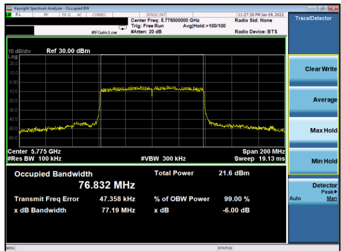
Plot 7-144. 6dB BW & 99% OBW Antenna 3a (80MHz BW 11ax – RU996 – Ch.155)
