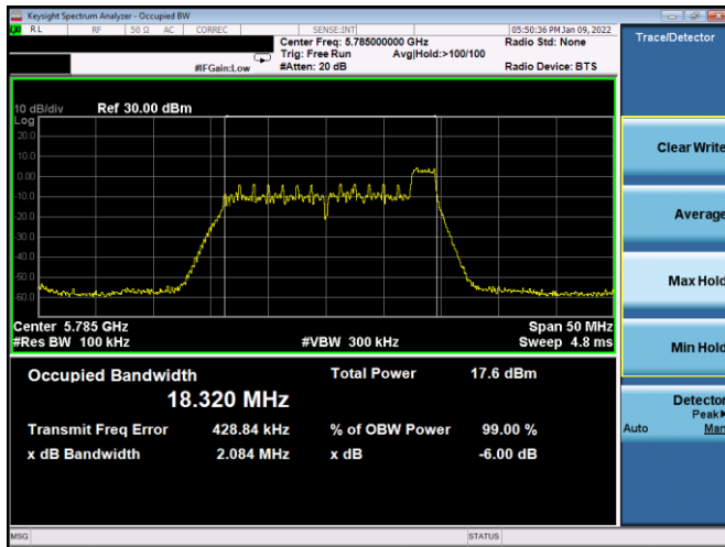
Plot 7-135. 6dB BW & 99% OBW Antenna 3a (20MHz BW 11ax Index 8– RU26 – Ch.157)
