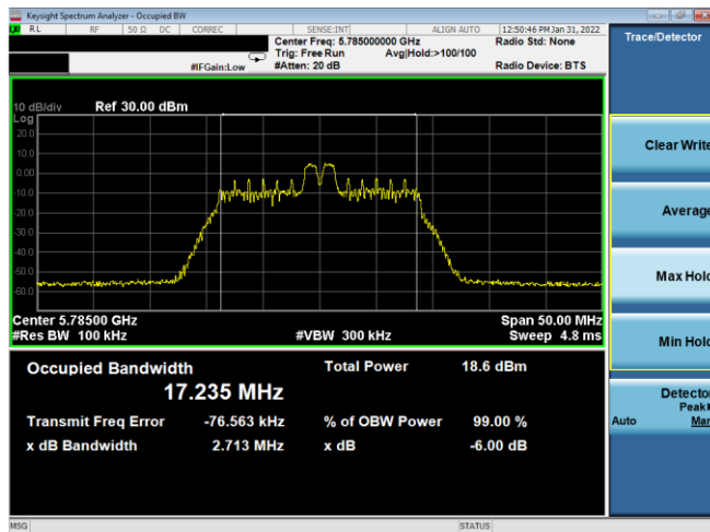
Plot 7-122. 6dB BW & 99% OBW Antenna 1b (20MHz BW 11ax Index 4 – RU26 – Ch.157)
