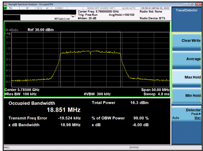
Plot 7-136. 6dB BW & 99% OBW Antenna 3a (20MHz BW 11ax– RU242 – Ch.157)
