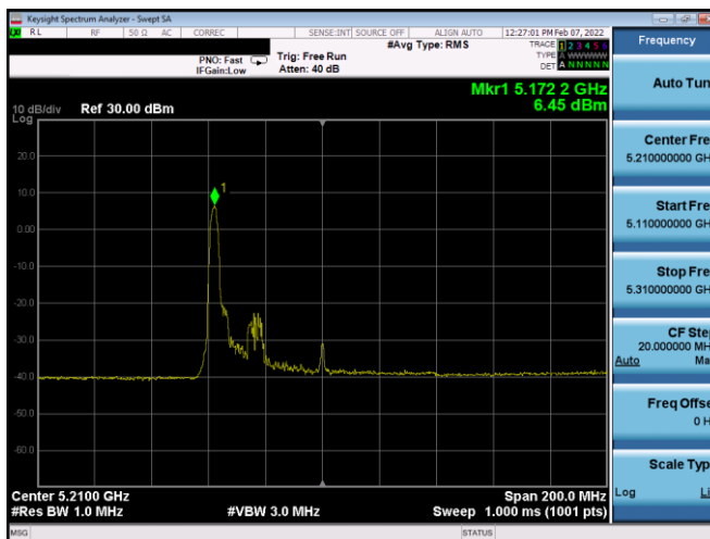
Plot 7-153. PSD Antenna 2b (80MHz BW 11ax Index 0 – RU26 – Ch.42)
