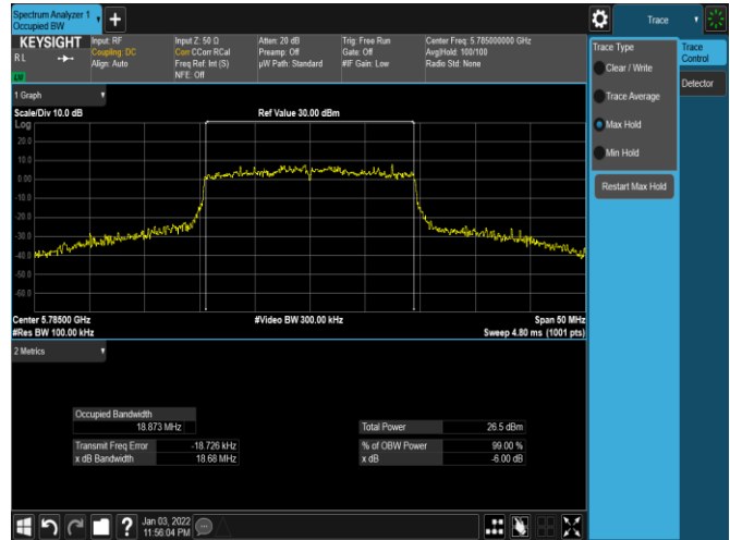
Plot 7-112. 6dB BW & 99% OBW Antenna 2b (20MHz BW 11ax– RU242 – Ch.157)
