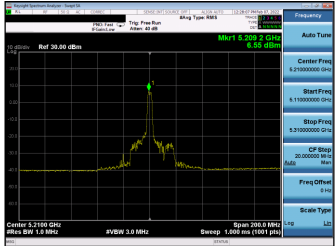
Plot 7-154. PSD Antenna 2b (80MHz BW 11ax Index 18 – RU26 – Ch.42)
