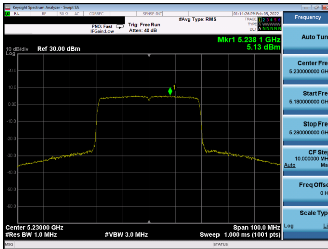
Plot 7-152. PSD Antenna 2b (40MHz BW 11ax – RU484 – Ch.46)
