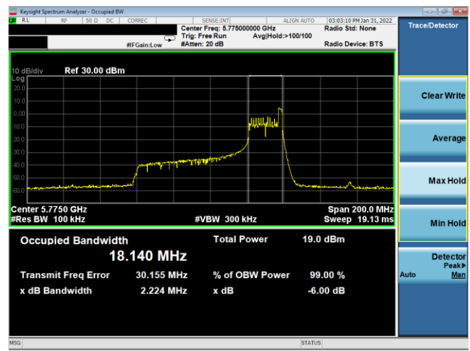
Plot 7-131. 6dB BW & 99% OBW Antenna 1b (80MHz BW 11ax Index 36 – RU26 – Ch.155)
