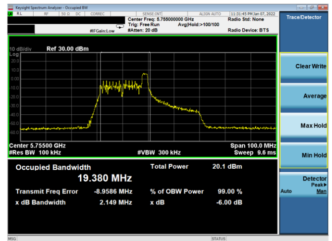
Plot 7-114. 6dB BW & 99% OBW Antenna 2b (40MHz BW 11ax Index 8 – RU26 – Ch.151)
