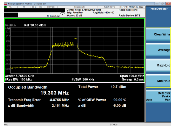
Plot 7-126. 6dB BW & 99% OBW Antenna 1b (40MHz BW 11ax Index 8 – RU26 – Ch.151)
