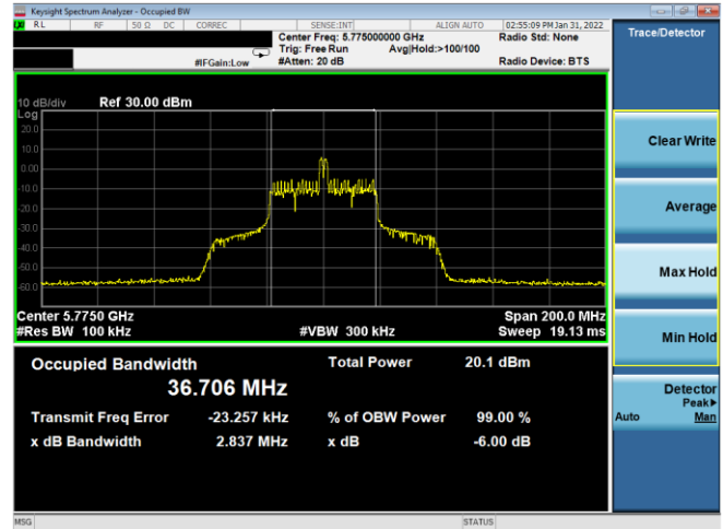
Plot 7-130. 6dB BW & 99% OBW Antenna 1b (80MHz BW 11ax Index 18 – RU26 – Ch.155)
