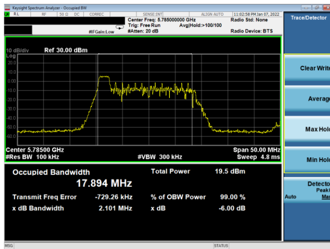
Plot 7-109. 6dB BW & 99% OBW Antenna 2b (20MHz BW 11ax Index 0 – RU26 – Ch.157)
