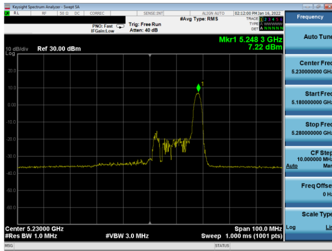
Plot 7-151. PSD Antenna 2b (40MHz BW 11ax Index 17 – RU26 – Ch.46)
