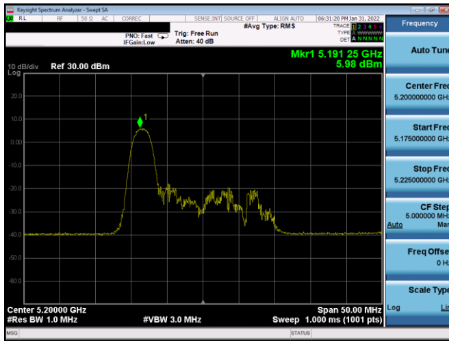
Plot 7-145. PSD Antenna 2b (20MHz BW 11ax Index 0 – RU26 – Ch.40)
