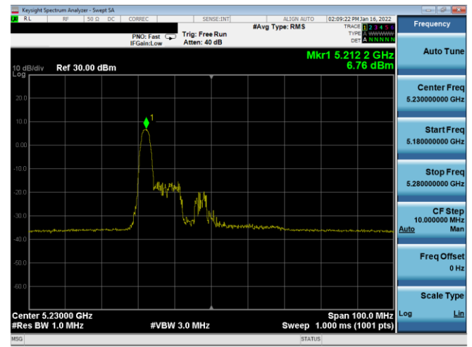
Plot 7-149. PSD Antenna 2b (40MHz BW 11ax Index 0 – RU26 – Ch.46)
