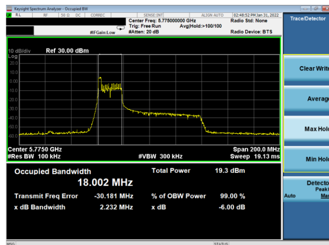
Plot 7-129. 6dB BW & 99% OBW Antenna 1b (80MHz BW 11ax Index 0 – RU26 – Ch.155)
