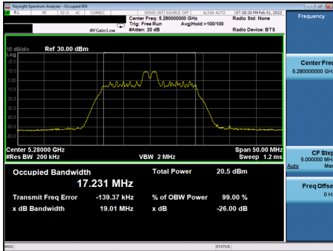
Plot 7-14. 26dB BW & 99% OBW Antenna 2b (20MHz BW 11ax Index 4 – RU26 – Ch.56)
