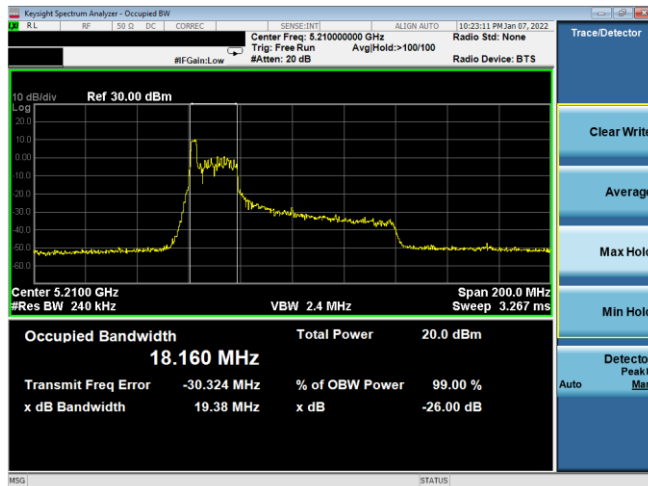
Plot 7-9. 26dB BW & 99% OBW Antenna 2b (80MHz BW 11ax Index 0 – RU26 – Ch.42)
