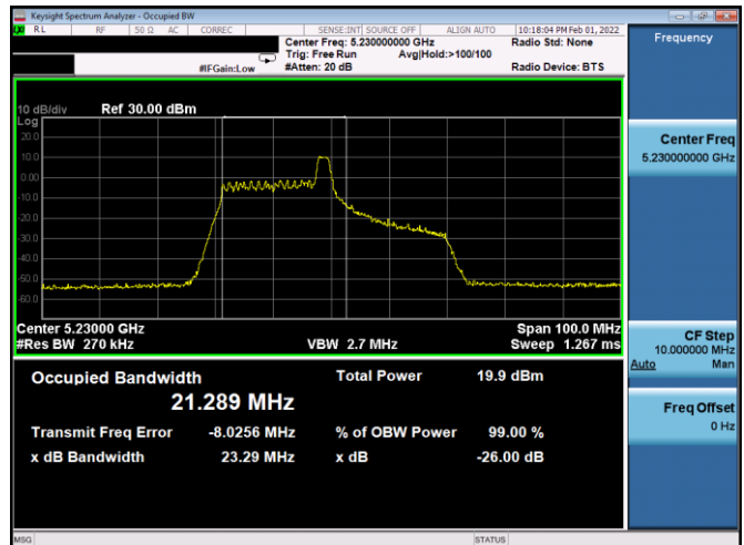
Plot 7-42. 26dB BW & 99% OBW Antenna 1b (40MHz BW 11ax Index 8 – RU26 – Ch.46)
