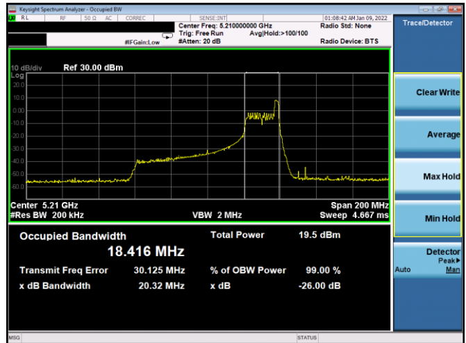
Plot 7-47. 26dB BW & 99% OBW Antenna 1b (80MHz BW 11ax Index 36 – RU26 – Ch.42)
