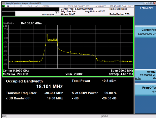
Plot 7-21. 26dB BW & 99% OBW Antenna 2b (80MHz BW 11ax Index 0 – RU26 – Ch.58)
