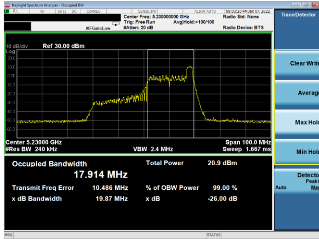
Plot 7-7. 26dB BW & 99% OBW Antenna 2b (40MHz BW 11ax Index 17 – RU26 – Ch.46)
