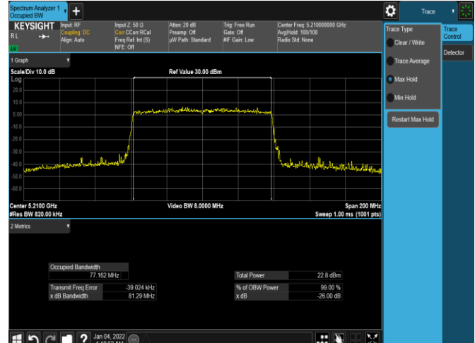
Plot 7-12. 26dB BW & 99% OBW Antenna 2b (80MHz BW 11ax – RU996 – Ch.42)
