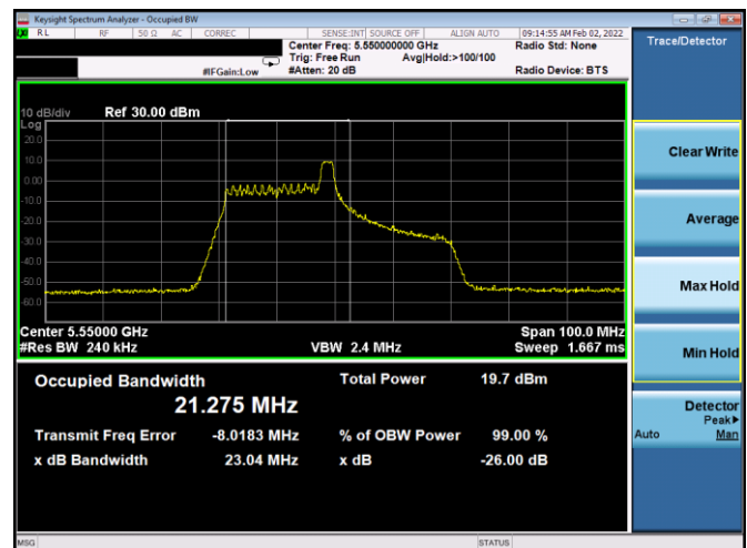
Plot 7-30. 26dB BW & 99% OBW Antenna 2b (40MHz BW 11ax Index 8 – RU26 – Ch.110)
