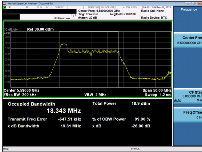
Plot 7-25. 26dB BW & 99% OBW Antenna 2b (20MHz BW 11ax Index 0 – RU26 – Ch.116)
