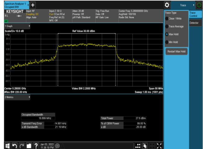
Plot 7-16. 26dB BW & 99% OBW Antenna 2b (20MHz BW 11ax– RU242 – Ch.56)
