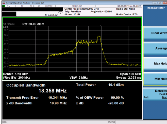
Plot 7-43. 26dB BW & 99% OBW Antenna 1b (40MHz BW 11ax Index 17 – RU26 – Ch.46)
