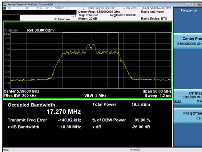
Plot 7-26. 26dB BW & 99% OBW Antenna 2b (20MHz BW 11ax Index 4 – RU26 – Ch.116)
