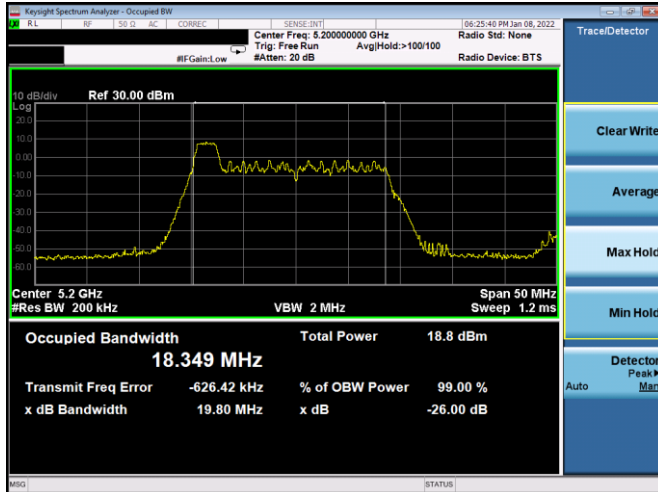
Plot 7-37. 26dB BW & 99% OBW Antenna 1b (20MHz BW 11ax Index 0 – RU26 – Ch.40)
