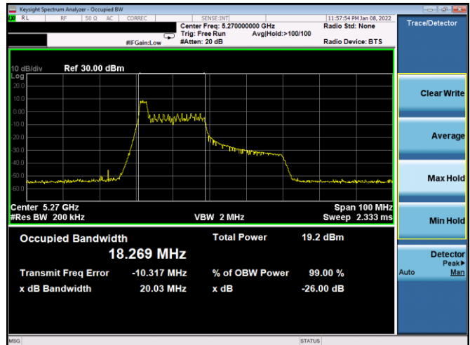
Plot 7-53. 26dB BW & 99% OBW Antenna 1b (40MHz BW 11ax Index 0 – RU26 – Ch.54)
