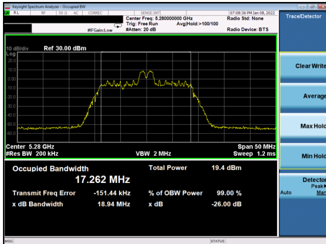
Plot 7-50. 26dB BW & 99% OBW Antenna 1b (20MHz BW 11ax Index 4 – RU26 – Ch.56)
