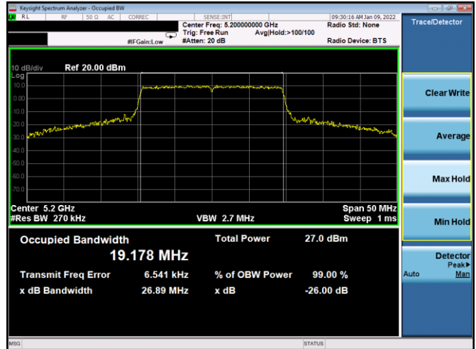
Plot 7-40. 26dB BW & 99% OBW Antenna 1b (20MHz BW 11ax– RU242 – Ch.40)
