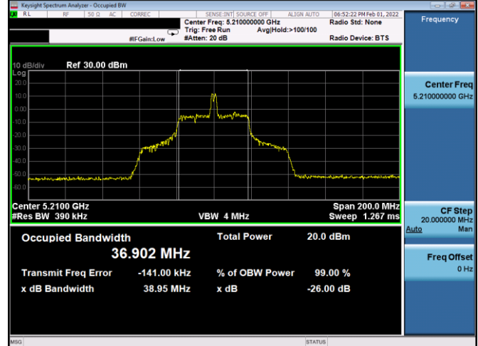
Plot 7-10. 26dB BW & 99% OBW Antenna 2b (80MHz BW 11ax Index 18 – RU26 – Ch.42)
