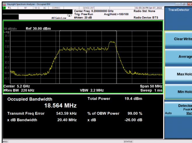
Plot 7-39. 26dB BW & 99% OBW Antenna 1b (20MHz BW 11ax Index 8– RU26 – Ch.40)
