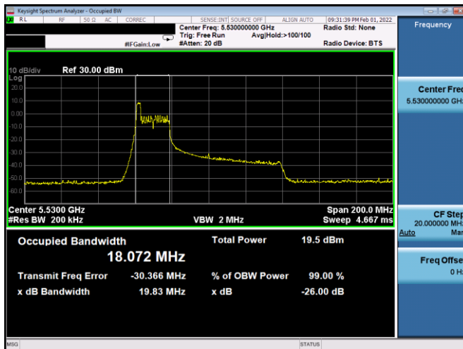
Plot 7-33. 26dB BW & 99% OBW Antenna 2b (80MHz BW 11ax Index 0 – RU26 – Ch.106)
