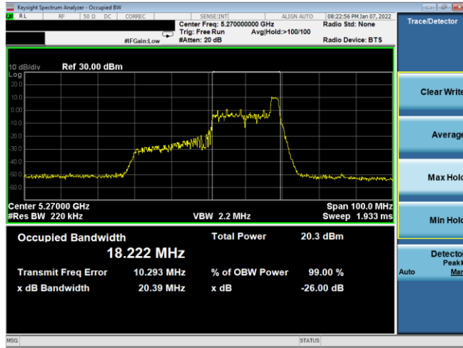
Plot 7-19. 26dB BW & 99% OBW Antenna 2b (40MHz BW 11ax Index 17 – RU26 – Ch.54)
