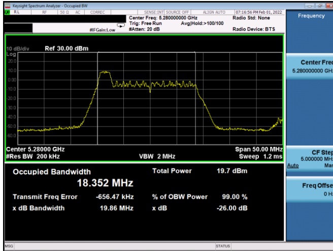
Plot 7-13. 26dB BW & 99% OBW Antenna 2b (20MHz BW 11ax Index 0 – RU26 – Ch.56)
