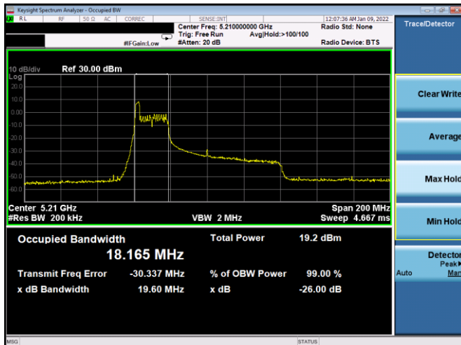
Plot 7-45. 26dB BW & 99% OBW Antenna 1b (80MHz BW 11ax Index 0 – RU26 – Ch.42)
