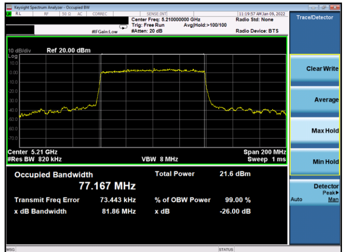
Plot 7-48. 26dB BW & 99% OBW Antenna 1b (80MHz BW 11ax – RU996 – Ch.42)
