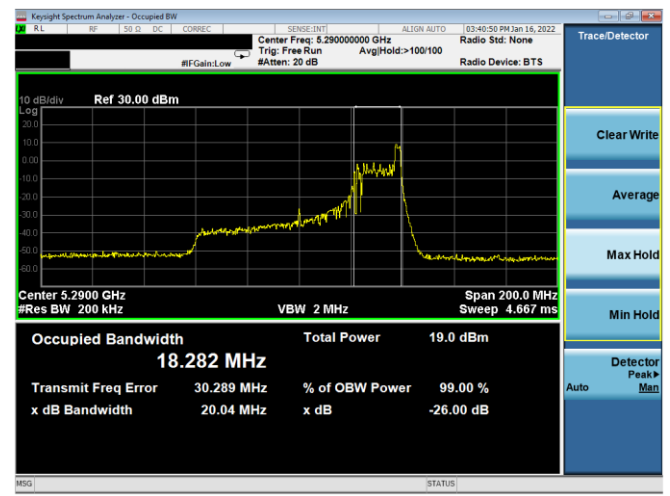
Plot 7-23. 26dB BW & 99% OBW Antenna 2b (80MHz BW 11ax Index 36 – RU26 – Ch.58)
