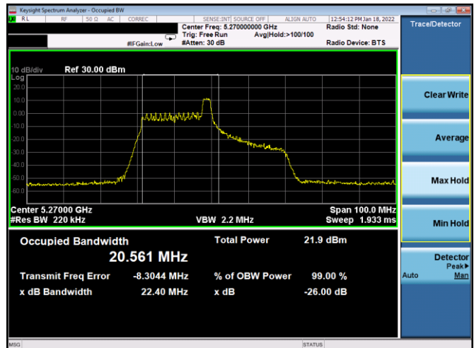
Plot 7-54. 26dB BW & 99% OBW Antenna 1b (40MHz BW 11ax Index 8 – RU26 – Ch.54)
