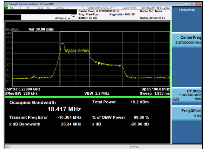
Plot 7-17. 26dB BW & 99% OBW Antenna 2b (40MHz BW 11ax Index 0 – RU26 – Ch.54)
