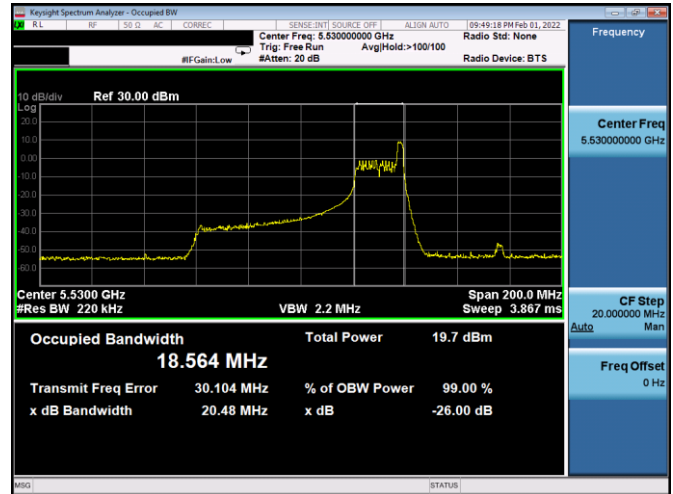
Plot 7-35. 26dB BW & 99% OBW Antenna 2b (80MHz BW 11ax Index 36 – RU26 – Ch.106)
