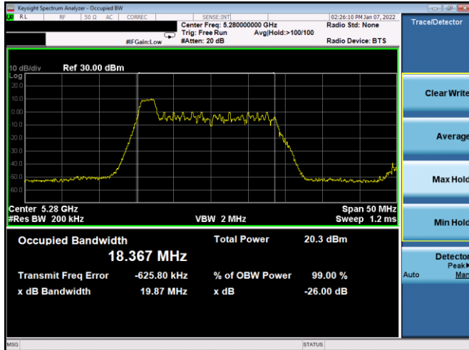
Plot 7-49. 26dB BW & 99% OBW Antenna 1b (20MHz BW 11ax Index 0 – RU26 – Ch.56)
