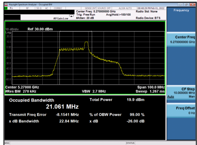
Plot 7-18. 26dB BW & 99% OBW Antenna 2b (40MHz BW 11ax Index 8 – RU26 – Ch.54)
