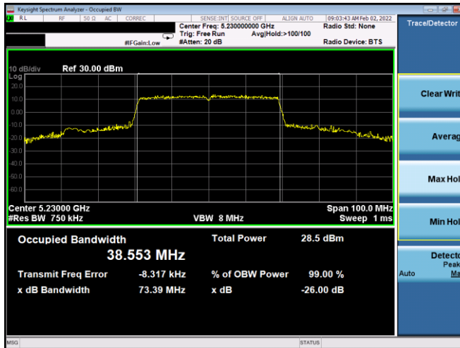
Plot 7-8. 26dB BW & 99% OBW Antenna 2b (40MHz BW 11ax – RU484 – Ch.46)
