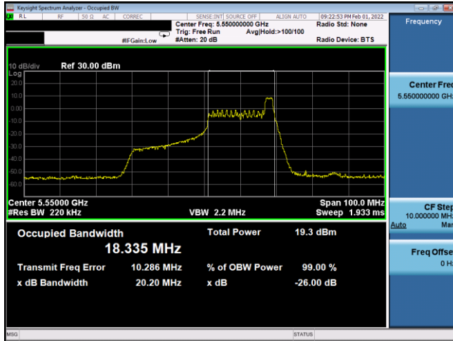
Plot 7-31. 26dB BW & 99% OBW Antenna 2b (40MHz BW 11ax Index 17 – RU26 – Ch.110)
