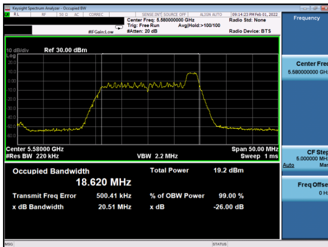
Plot 7-27. 26dB BW & 99% OBW Antenna 2b (20MHz BW 11ax Index 8 – RU26 – Ch.116)
