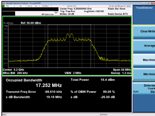
Plot 7-38. 26dB BW & 99% OBW Antenna 1b (20MHz BW 11ax Index 4 – RU26 – Ch.40)
