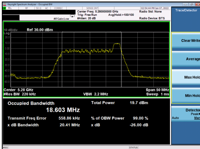
Plot 7-51. 26dB BW & 99% OBW Antenna 1b (20MHz BW 11ax Index 8– RU26 – Ch.56)
