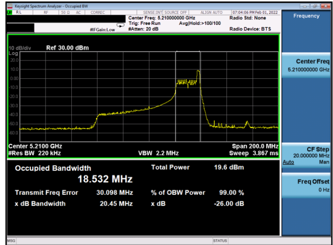
Plot 7-11. 26dB BW & 99% OBW Antenna 2b (80MHz BW 11ax Index 36 – RU26 – Ch.42)
