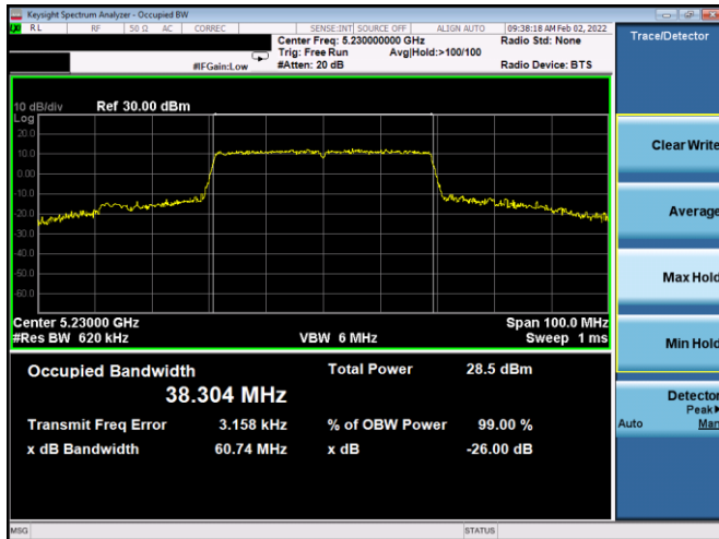
Plot 7-44. 26dB BW & 99% OBW Antenna 1b (40MHz BW 11ax – RU484 – Ch.46)
