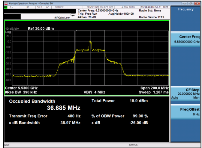
Plot 7-34. 26dB BW & 99% OBW Antenna 2b (80MHz BW 11ax Index 18 – RU26 – Ch.106)
