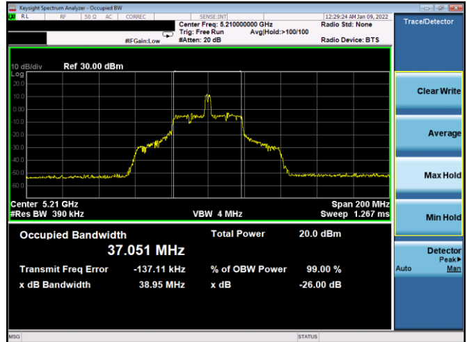
Plot 7-46. 26dB BW & 99% OBW Antenna 1b (80MHz BW 11ax Index 18 – RU26 – Ch.42)
