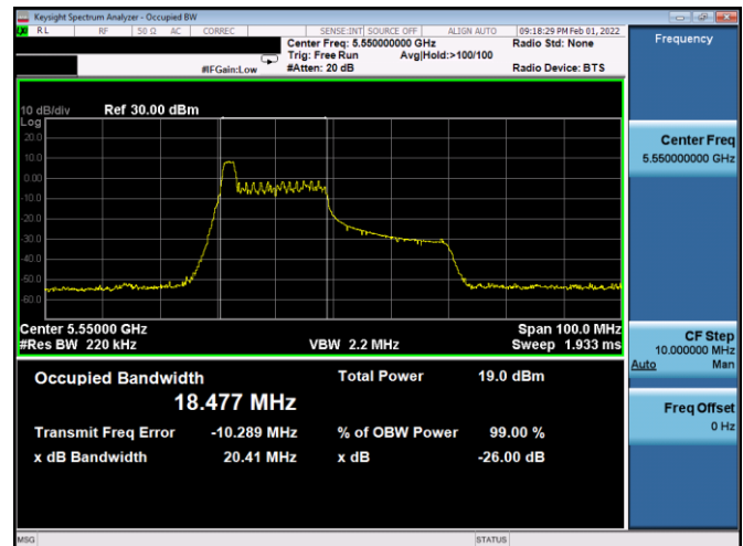
Plot 7-29. 26dB BW & 99% OBW Antenna 2b (40MHz BW 11ax Index 0 – RU26 – Ch.110)
