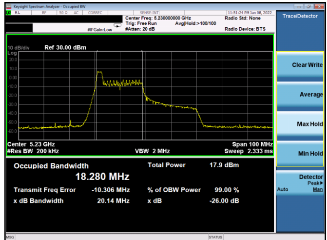
Plot 7-41. 26dB BW & 99% OBW Antenna 1b (40MHz BW 11ax Index 0 – RU26 – Ch.46)
