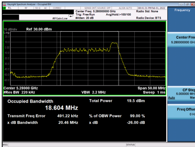
Plot 7-15. 26dB BW & 99% OBW Antenna 2b (20MHz BW 11ax Index 8– RU26 – Ch.56)
