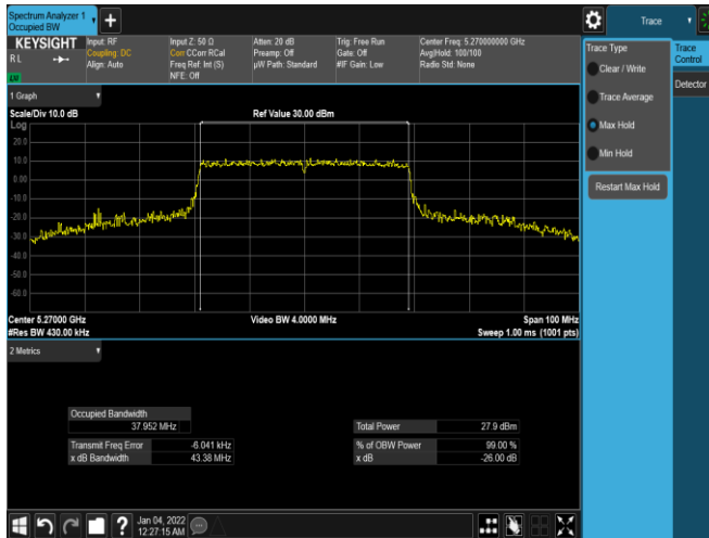
Plot 7-20. 26dB BW & 99% OBW Antenna 2b (40MHz BW 11ax – RU484 – Ch.54)
