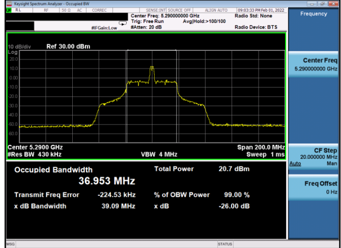
Plot 7-22. 26dB BW & 99% OBW Antenna 2b (80MHz BW 11ax Index 18 – RU26 – Ch.58)
