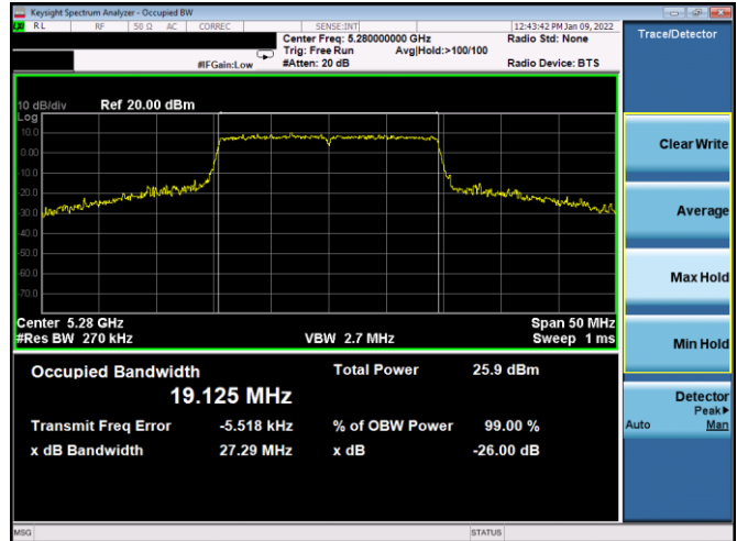
Plot 7-52. 26dB BW & 99% OBW Antenna 1b (20MHz BW 11ax– RU242 – Ch.56)
