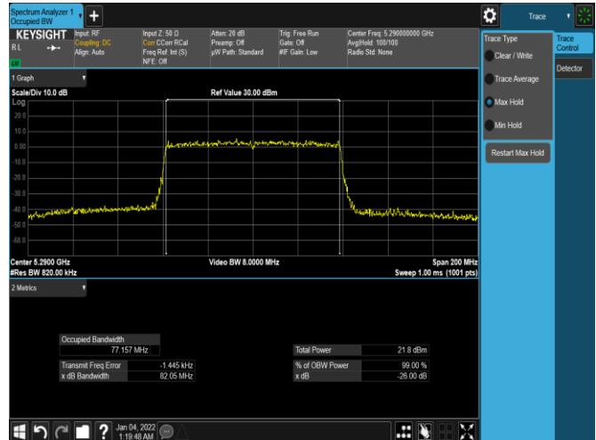
Plot 7-24. 26dB BW & 99% OBW Antenna 2b (80MHz BW 11ax – RU996 – Ch.58)
