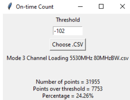
Figure 9-18. 5530MHz - Channel Loading Calculation - Mode 3 (80MHz)
