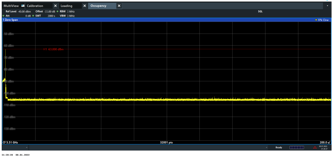
Figure 9-38. 5510MHz - Non-Occupancy Period (30 Minutes) - Mode 1 (40MHz)
