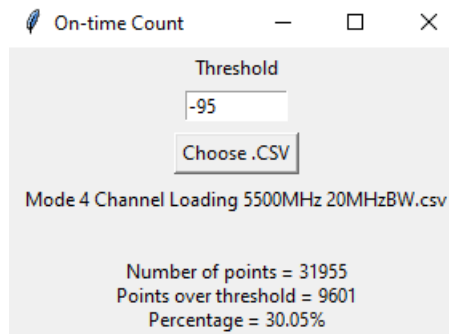
Figure 9-20. 5500MHz - Channel Loading Calculation - Mode 4 (20MHz)
