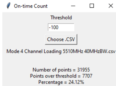
Figure 9-22. 5510MHz - Channel Loading Calculation - Mode 4 (40MHz)
