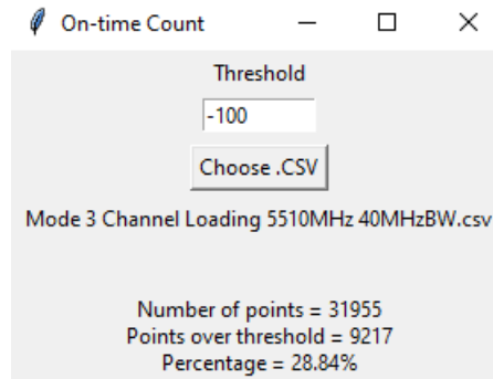
Figure 9-16. 5510MHz - Channel Loading Calculation - Mode 3 (40MHz)
