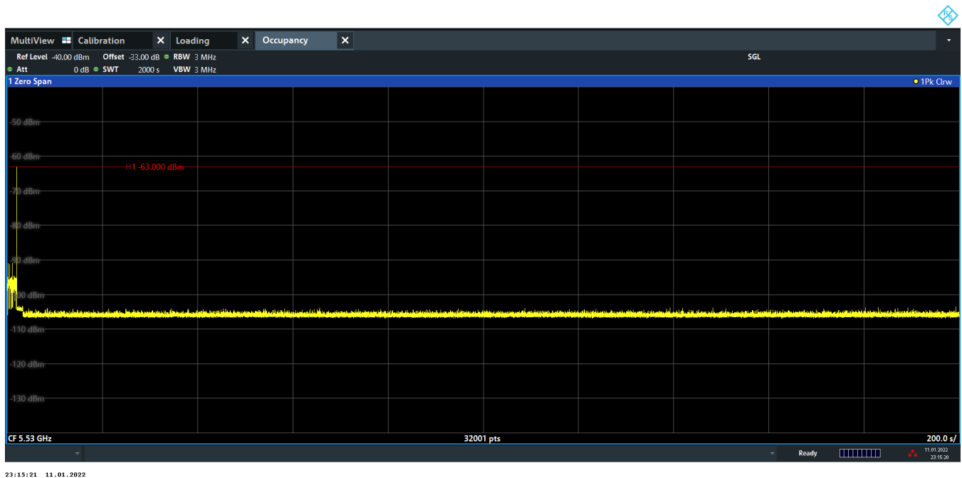
Figure 9-45. 5530MHz - Non-Occupancy Period (30 Minutes) - Mode 3 (80MHz)
