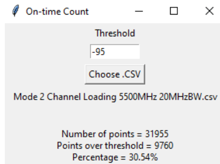
Figure 9-8. 5500MHz - Channel Loading Calculation - Mode 2 (20MHz)
