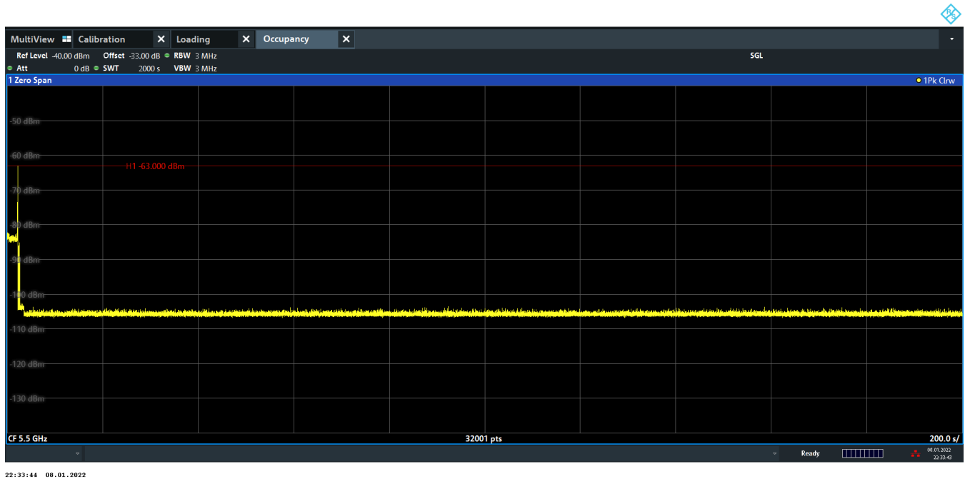
Figure 9-37. 5500MHz - Non-Occupancy Period (30 Minutes) - Mode 1 (20MHz)
