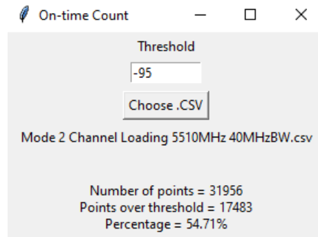
Figure 9-10. 5510MHz - Channel Loading Calculation - Mode 2 (40MHz)
