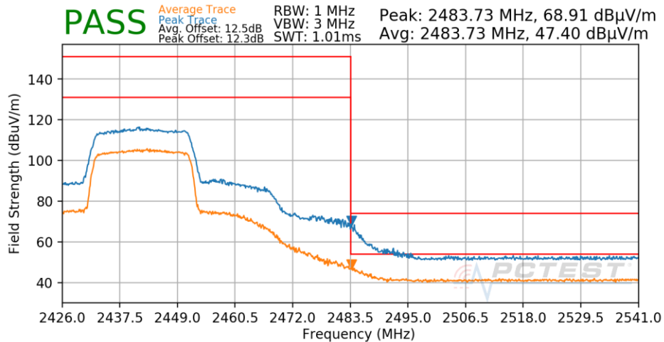
Plot 7-504. Radiated Restricted Upper Band Edge Measurement Antenna 3a
