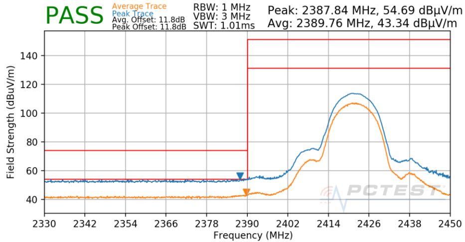
Plot 7-523. Radiated Restricted Lower Band Edge Measurement Antenna 1a
