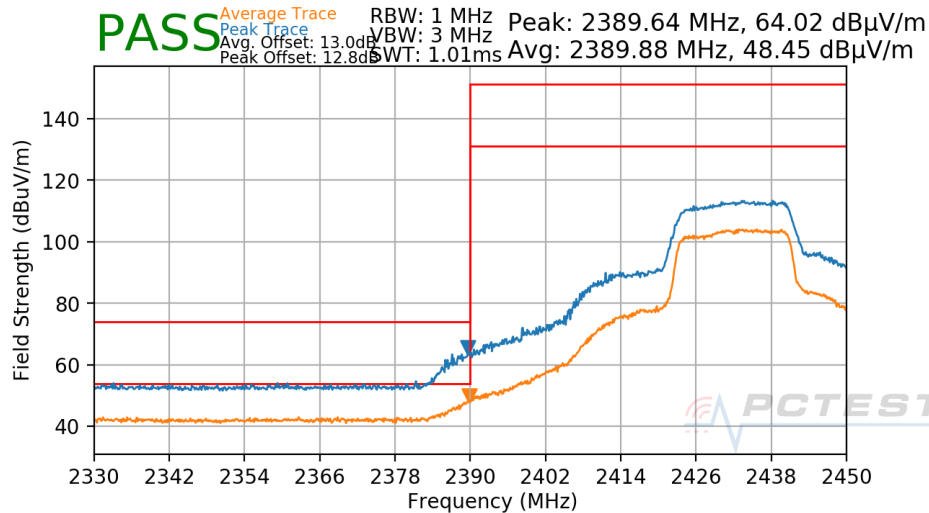
Plot 7-541. Radiated Restricted Lower Band Edge Measurement Antenna 1a
