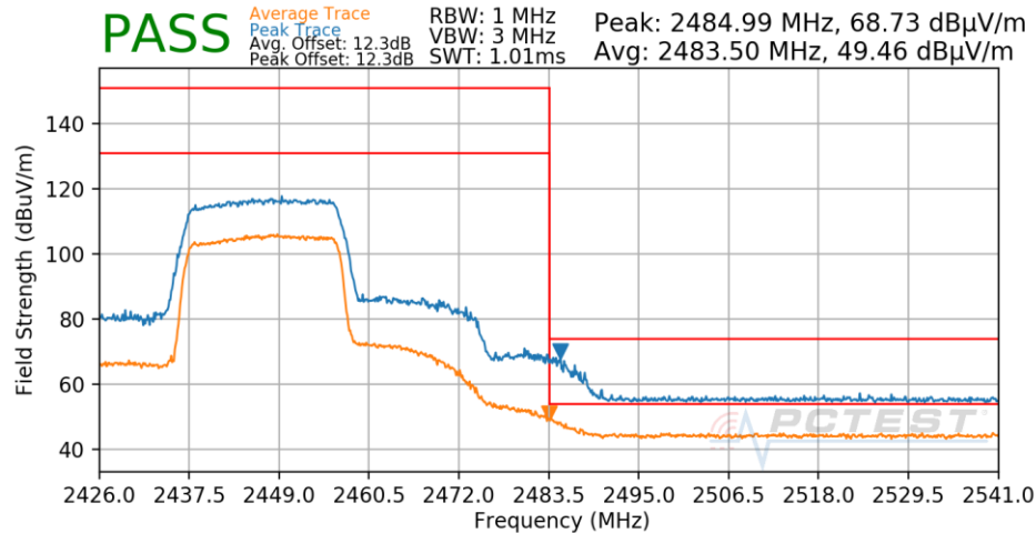
Plot 7-506. Radiated Restricted Upper Band Edge Measurement Antenna 3a
