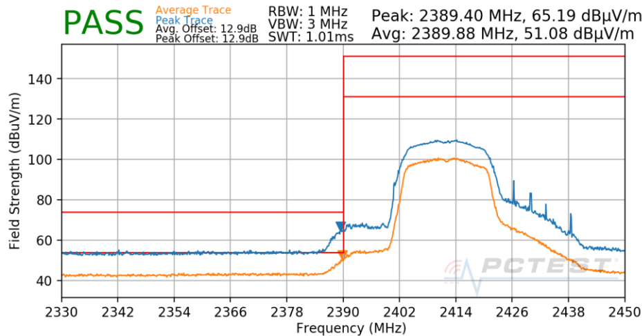
Plot 7-529. Radiated Restricted Lower Band Edge Measurement Antenna 1a
