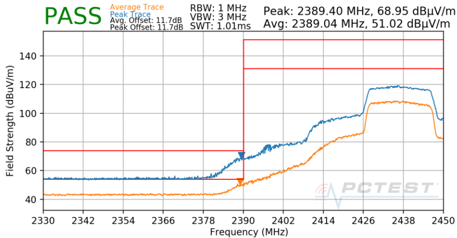
Plot 7-499. Radiated Restricted Lower Band Edge Measurement Antenna 3a
