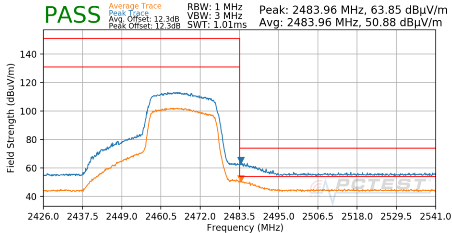
Plot 7-518. Radiated Restricted Upper Band Edge Measurement Antenna 3a
