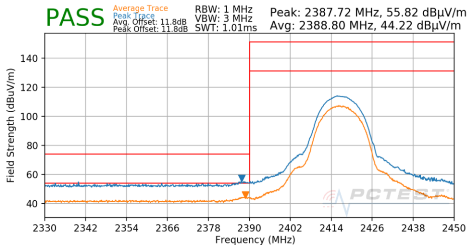
Plot 7-522. Radiated Restricted Lower Band Edge Measurement Antenna 1a
