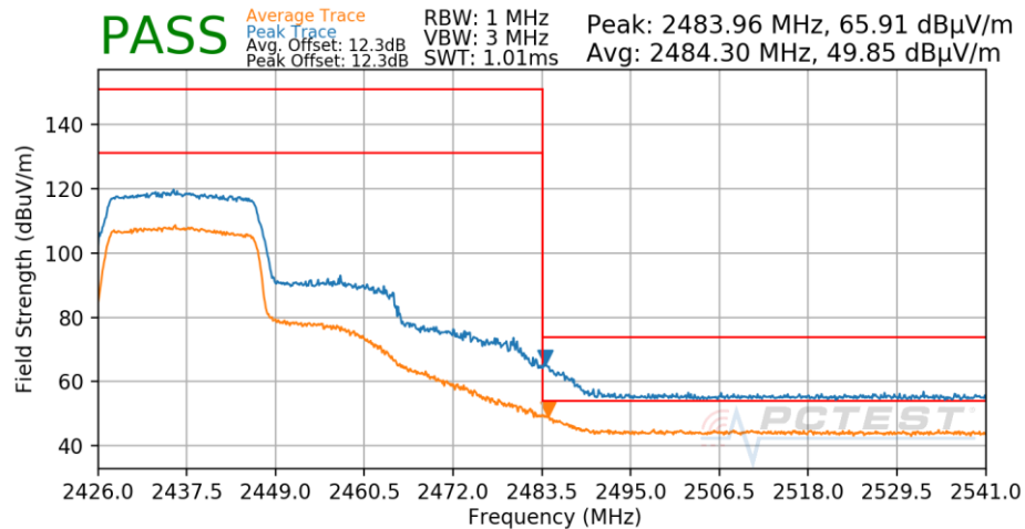
Plot 7-500. Radiated Restricted Upper Band Edge Measurement Antenna 3a
