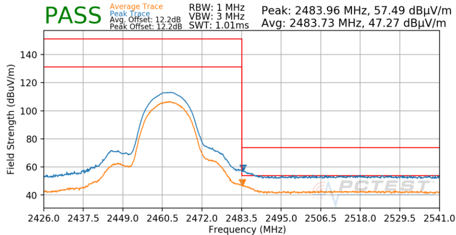
Plot 7-526. Radiated Restricted Upper Band Edge Measurement Antenna 1a
