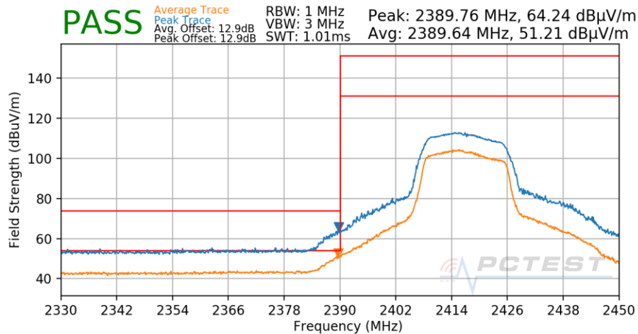
Plot 7-532. Radiated Restricted Lower Band Edge Measurement Antenna 1a
