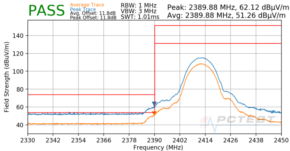
Plot 7-521. Radiated Restricted Lower Band Edge Measurement Antenna 1a
