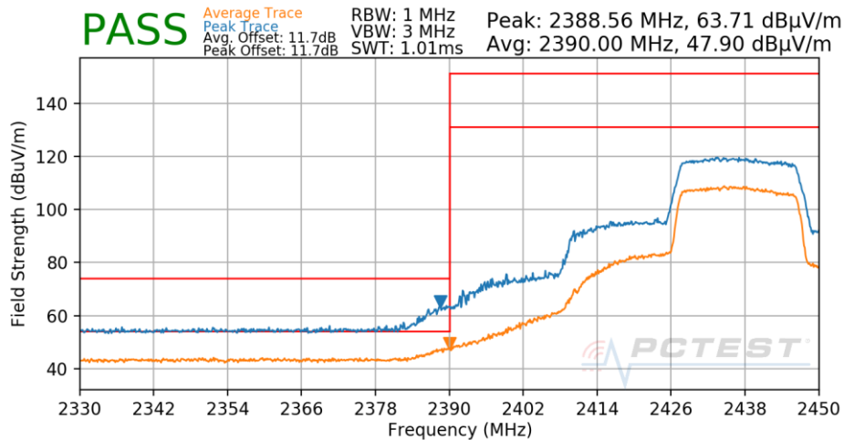
Plot 7-498. Radiated Restricted Lower Band Edge Measurement Antenna 3a
