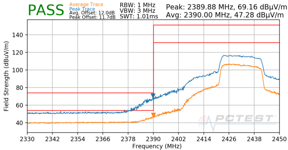
Plot 7-497. Radiated Restricted Lower Band Edge Measurement Antenna 3a
