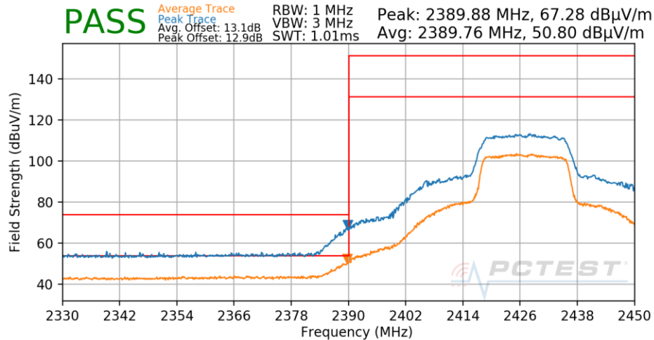
Plot 7-539. Radiated Restricted Lower Band Edge Measurement Antenna 1a
