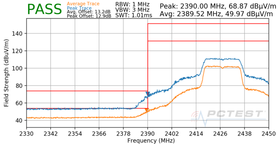
Plot 7-540. Radiated Restricted Lower Band Edge Measurement Antenna 1a
