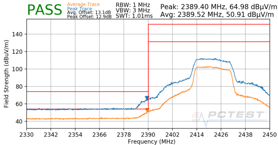
Plot 7-536. Radiated Restricted Lower Band Edge Measurement Antenna 1a
