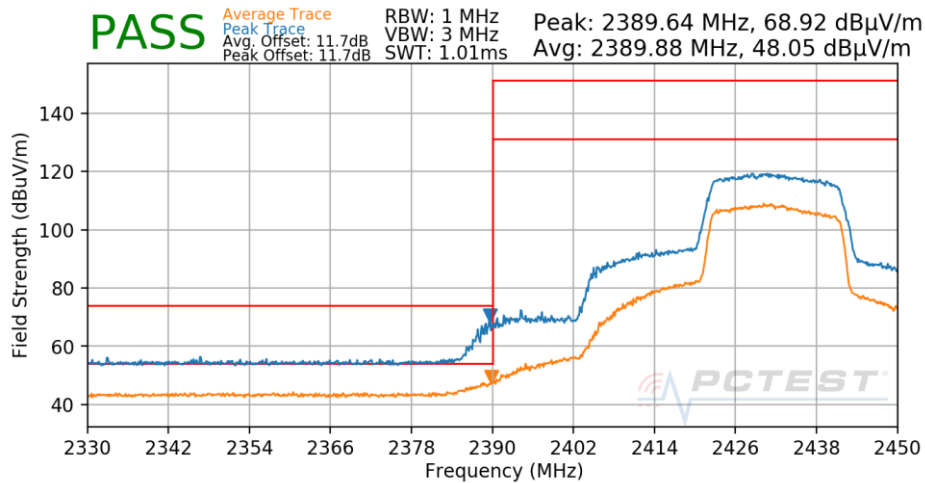
Plot 7-495. Radiated Restricted Lower Band Edge Measurement Antenna 3a
