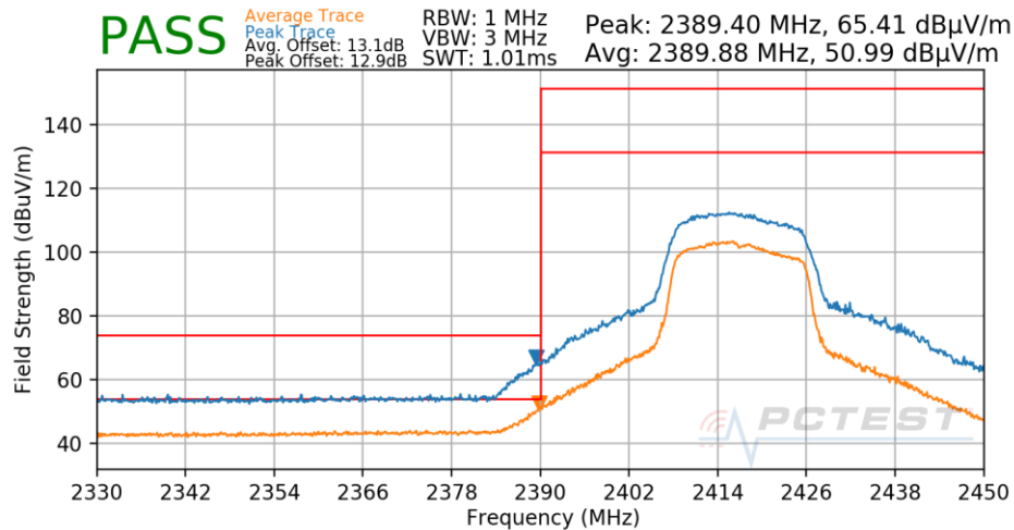
Plot 7-533. Radiated Restricted Lower Band Edge Measurement Antenna 1a
