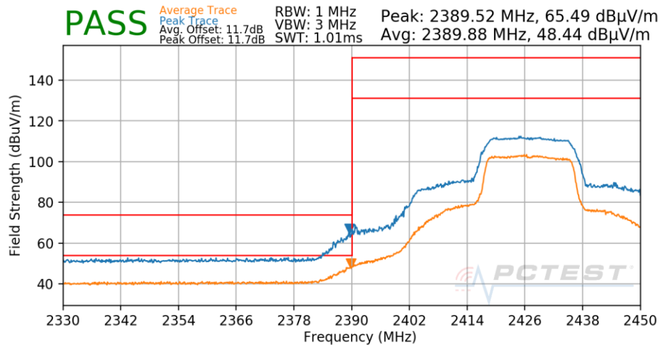
Plot 7-538. Radiated Restricted Lower Band Edge Measurement Antenna 1a
