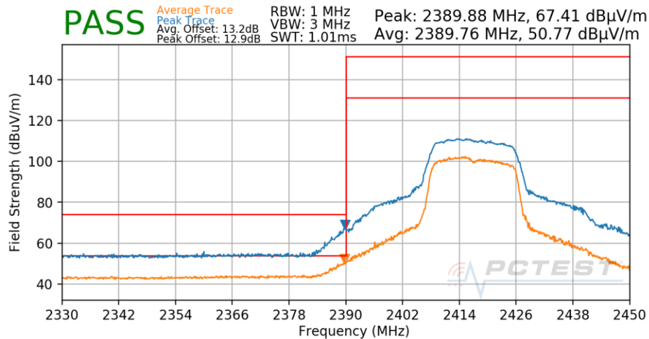
Plot 7-534. Radiated Restricted Lower Band Edge Measurement Antenna 1a
