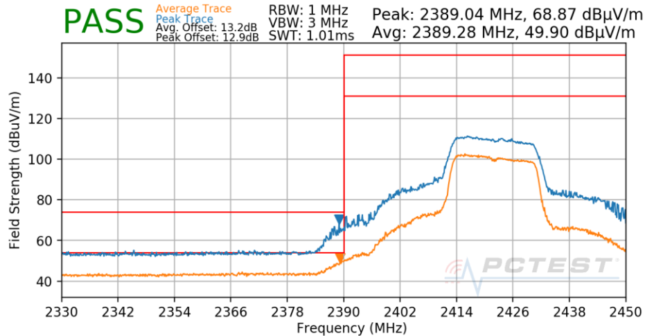
Plot 7-537. Radiated Restricted Lower Band Edge Measurement Antenna 1a
