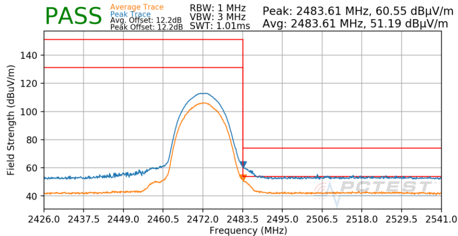
Plot 7-528. Radiated Restricted Upper Band Edge Measurement Antenna 1a
