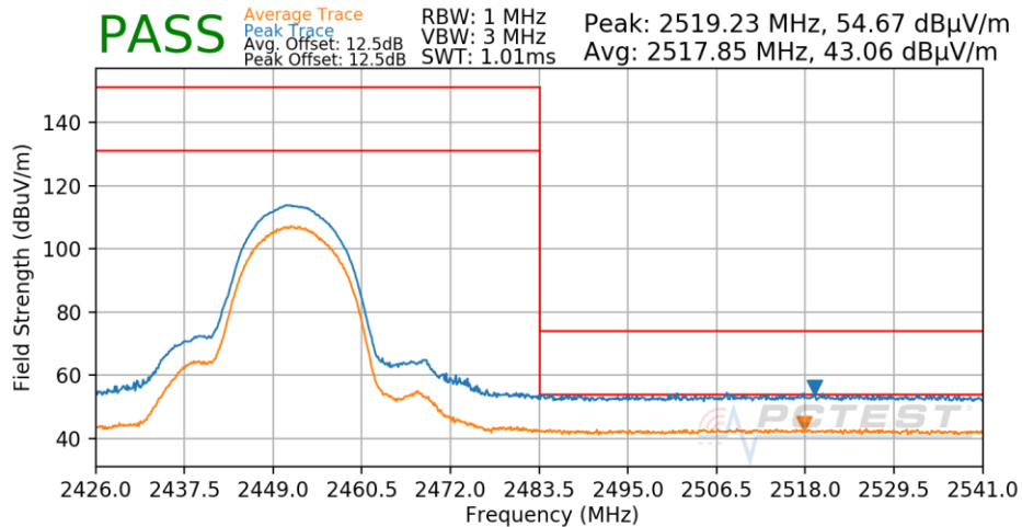
Plot 7-524. Radiated Restricted Upper Band Edge Measurement Antenna 1a
