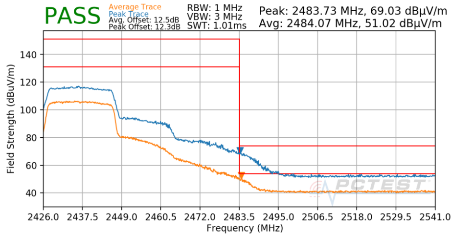
Plot 7-501. Radiated Restricted Upper Band Edge Measurement Antenna 3a
