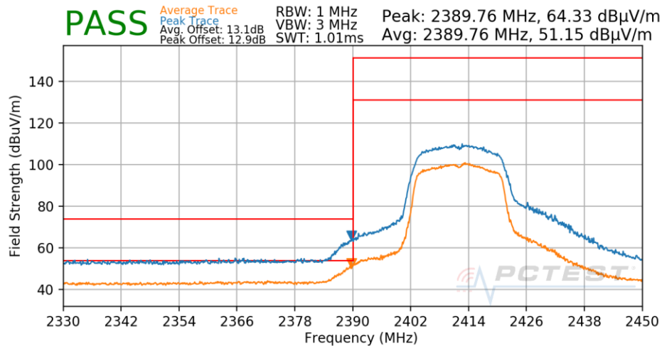
Plot 7-530. Radiated Restricted Lower Band Edge Measurement Antenna 1a
