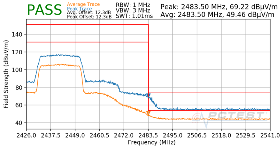
Plot 7-503. Radiated Restricted Upper Band Edge Measurement Antenna 3a
