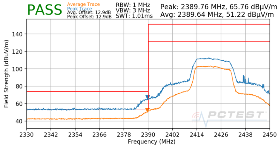
Plot 7-535. Radiated Restricted Lower Band Edge Measurement Antenna 1a
