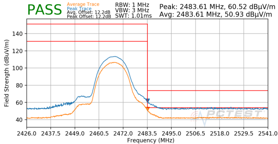
Plot 7-527. Radiated Restricted Upper Band Edge Measurement Antenna 1a
