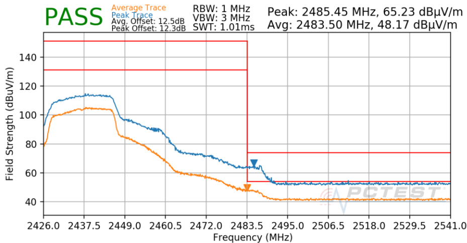
Plot 7-542. Radiated Restricted Upper Band Edge Measurement Antenna 1a
