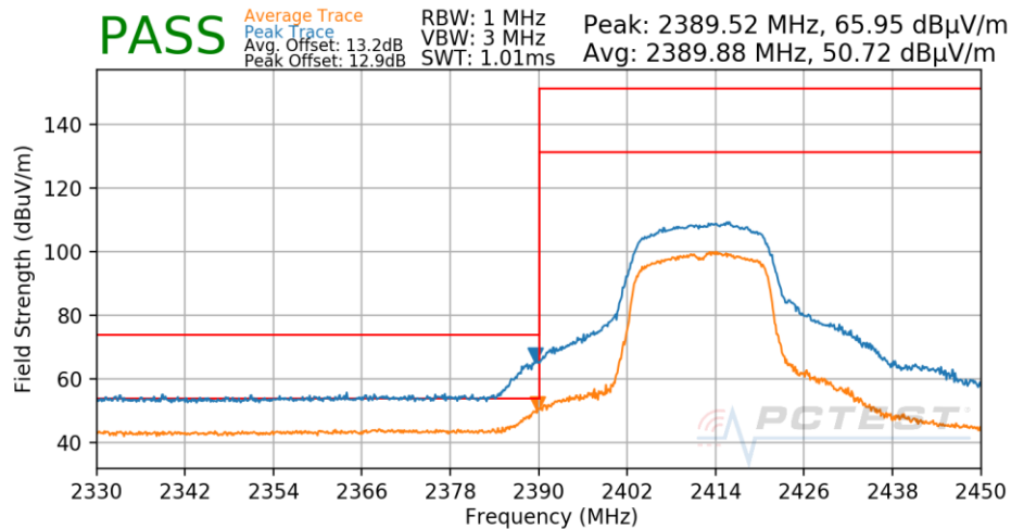
Plot 7-531. Radiated Restricted Lower Band Edge Measurement Antenna 1a
