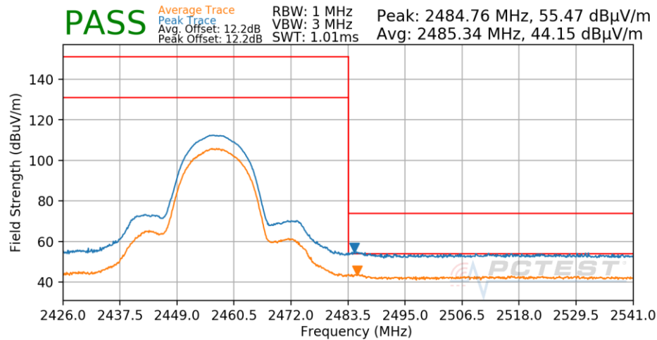
Plot 7-525. Radiated Restricted Upper Band Edge Measurement Antenna 1a
