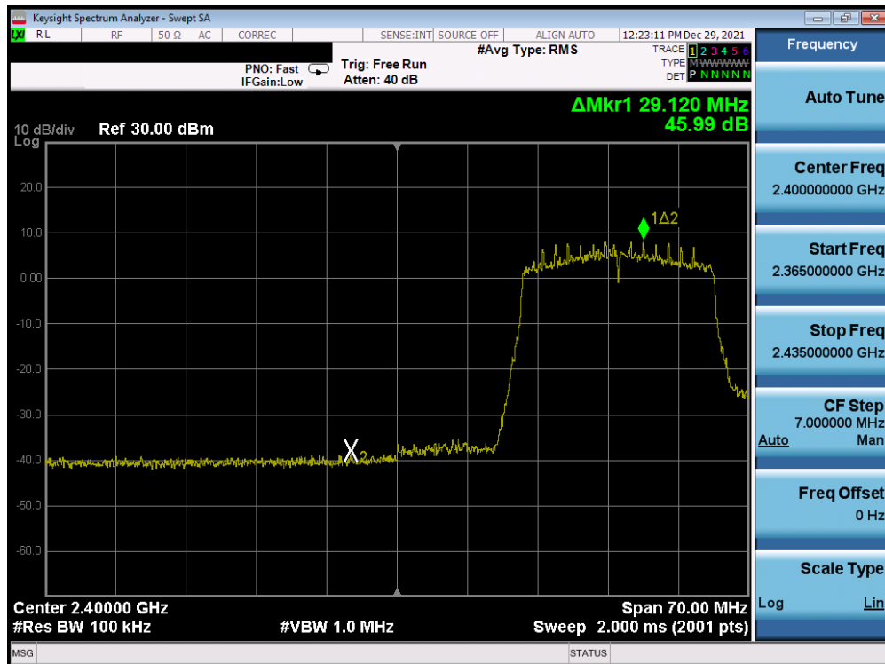
Plot 7-314. Band Edge Plot Antenna 1a (802.11ax (SU - 2.4GHz) – Ch. 3) – MCS0
