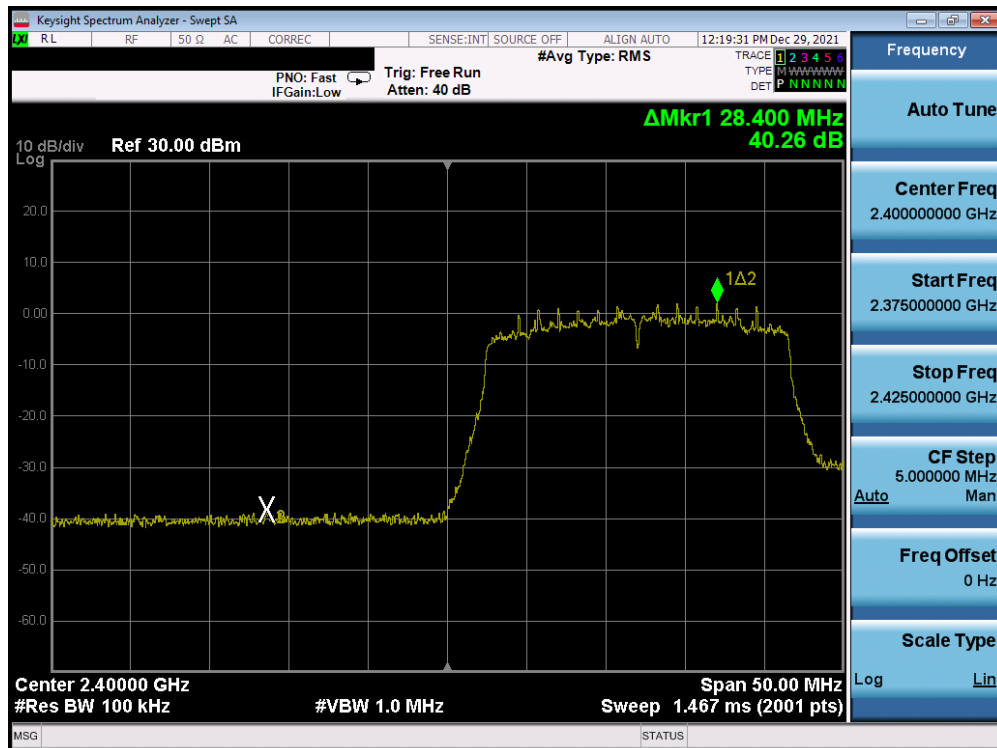
Plot 7-312. Band Edge Plot Antenna 1a (802.11ax (SU - 2.4GHz) – Ch. 1) – MCS0
