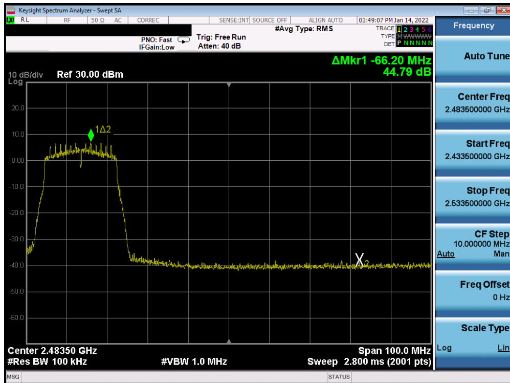
Plot 7-306. Band Edge Plot Antenna 1a (802.11n (2.4GHz) - Ch. 8) - MCS0
