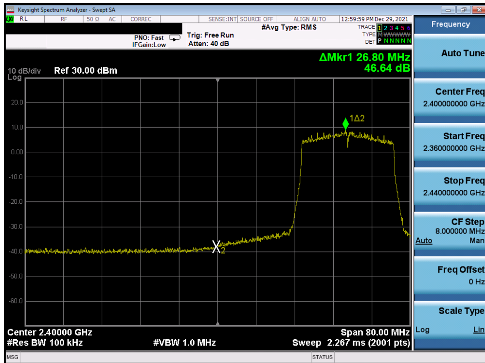
Plot 7-353. Band Edge Plot Antenna 1a (802.11ax (SU - 2.4GHz) – Ch. 4) – MCS3
