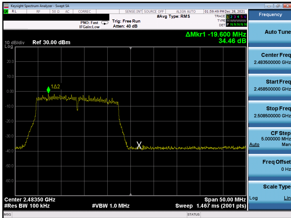
Plot 7-277. Band Edge Plot Antenna 3a (802.11n (2.4GHz) – Ch. 13) – MCS5
