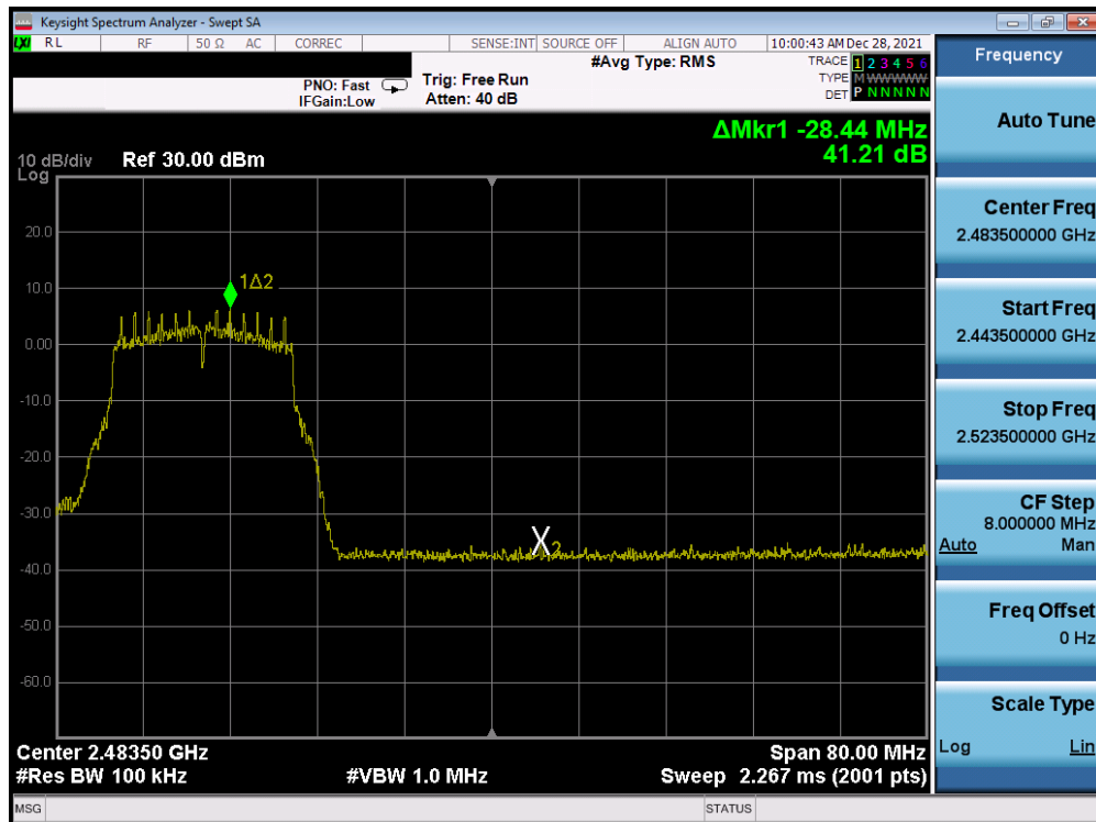
Plot 7-333. Band Edge Plot Antenna 1a (802.11g – Ch. 10) – 18Mbps
