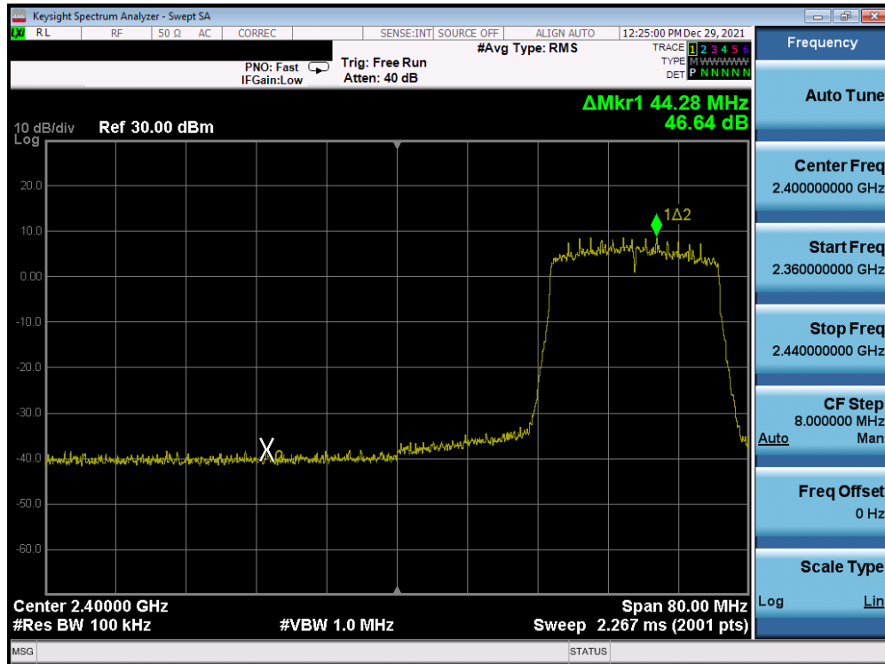
Plot 7-315. Band Edge Plot Antenna 1a (802.11ax (SU - 2.4GHz) – Ch. 4) – MCS0
