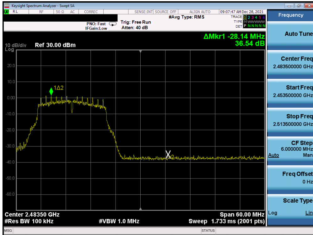
Plot 7-299. Band Edge Plot Antenna 1a (802.11g - Ch. 12) - 6Mbps
