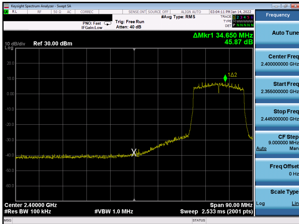
Plot 7-316. Band Edge Plot Antenna 1a (802.11ax (SU - 2.4GHz) – Ch. 5) – MCS0
