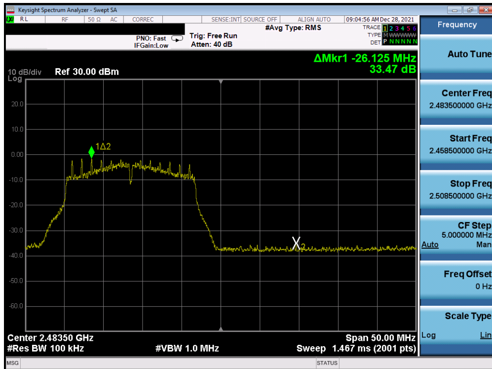
Plot 7-300. Band Edge Plot Antenna 1a (802.11g - Ch. 13) - 6Mbps
