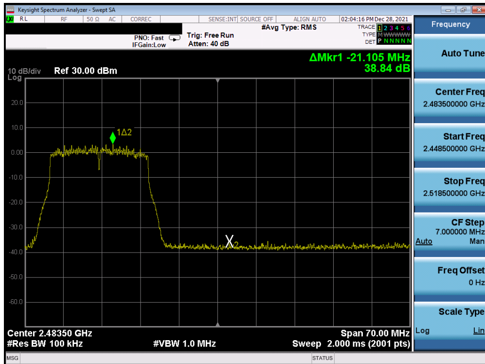
Plot 7-275. Band Edge Plot Antenna 3a (802.11n (2.4GHz) - Ch. 11) - MCS5
