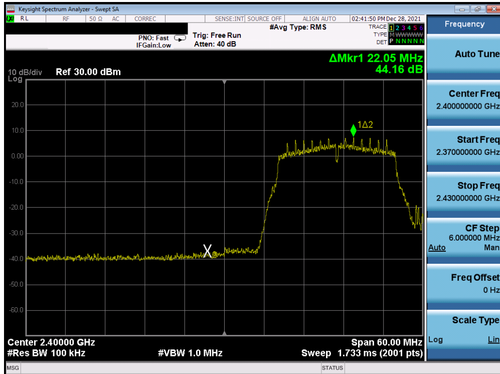
Plot 7-302. Band Edge Plot Antenna 1a (802.11n (2.4GHz) - Ch. 2) - MCS0
