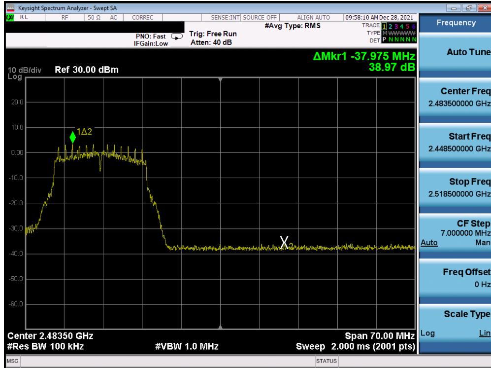
Plot 7-334. Band Edge Plot Antenna 1a (802.11g - Ch. 11) - 18Mbps
