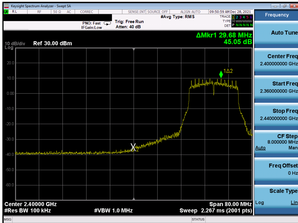
Plot 7-327. Band Edge Plot Antenna 1a (802.11g- Ch. 4) – 18Mbps
