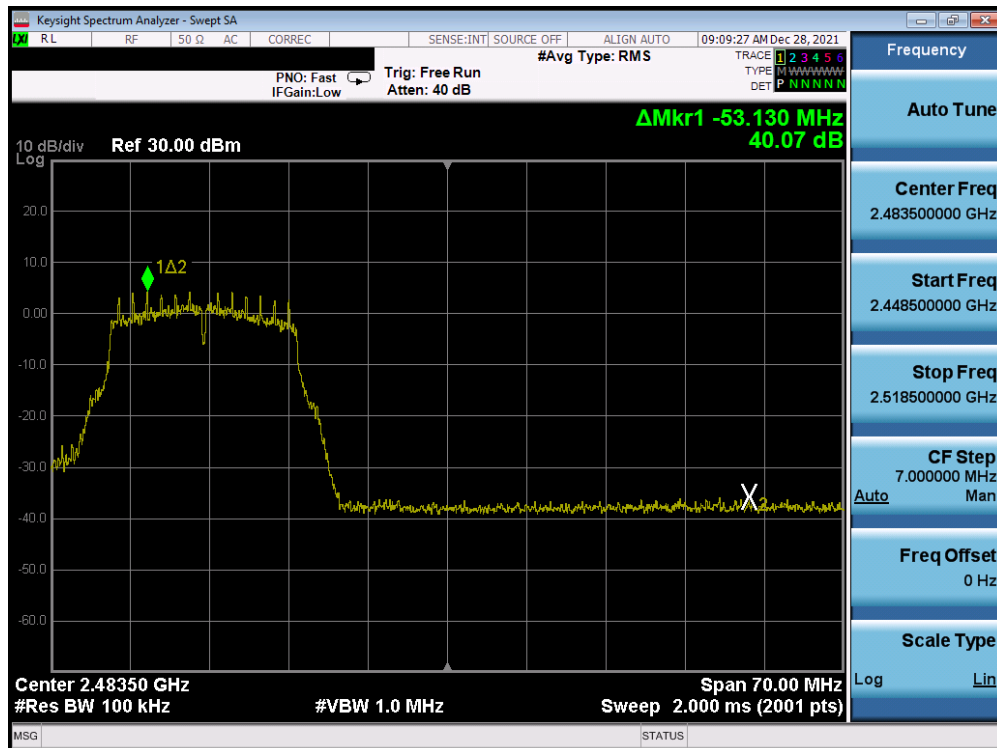
Plot 7-298. Band Edge Plot Antenna 1a (802.11g - Ch. 11) - 6Mbps
