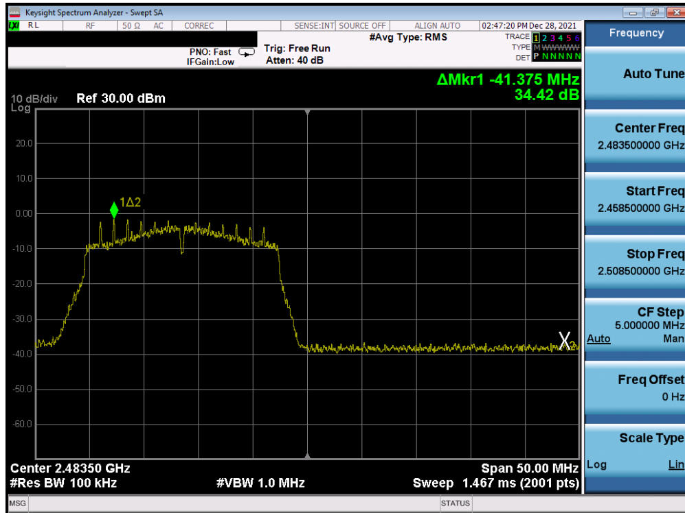
Plot 7-311. Band Edge Plot Antenna 1a (802.11n (2.4GHz) – Ch. 13) – MCS0
