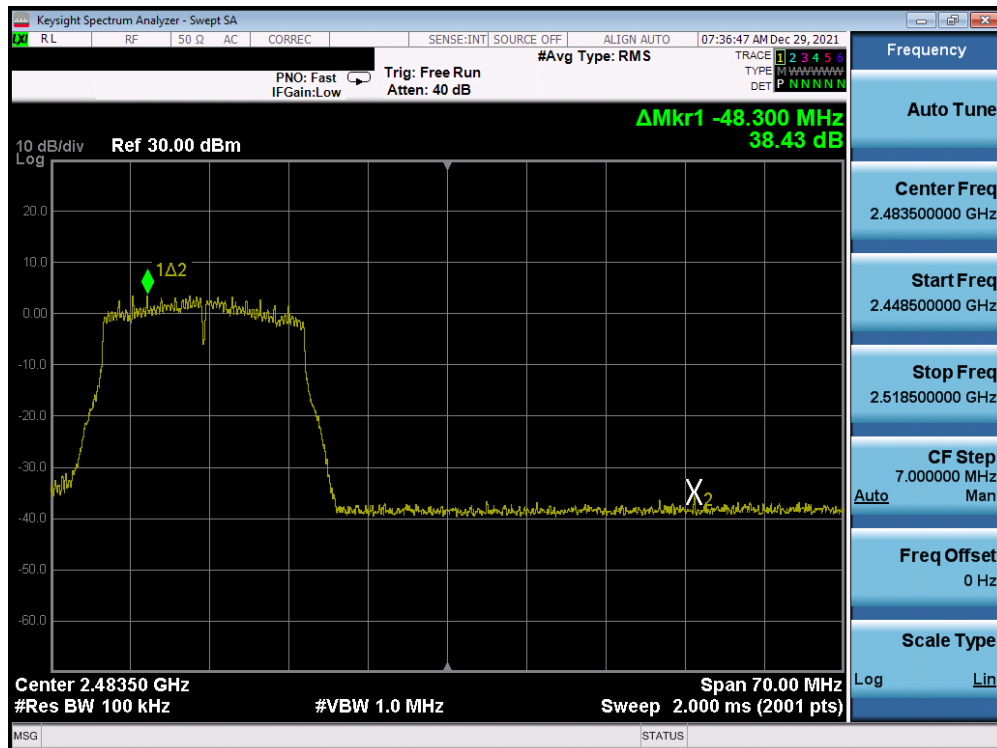
Plot 7-347. Band Edge Plot Antenna 1a (802.11n (2.4GHz) – Ch. 11) – MCS3
