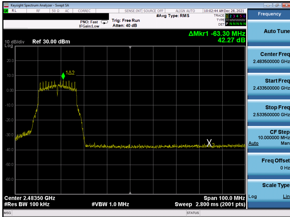
Plot 7-332. Band Edge Plot Antenna 1a (802.11g – Ch. 9) – 18Mbps
