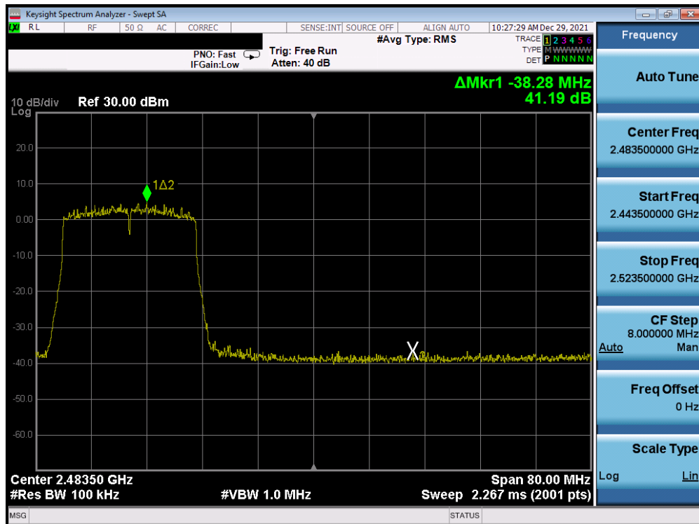
Plot 7-287. Band Edge Plot Antenna 3a (802.11ax (SU - 2.4GHz) – Ch. 10) – MCS5
