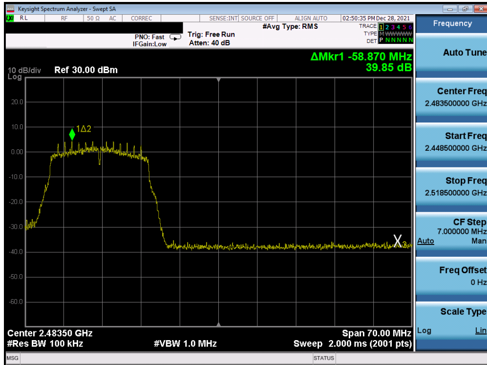
Plot 7-309. Band Edge Plot Antenna 1a (802.11n (2.4GHz) – Ch. 11) – MCS0
