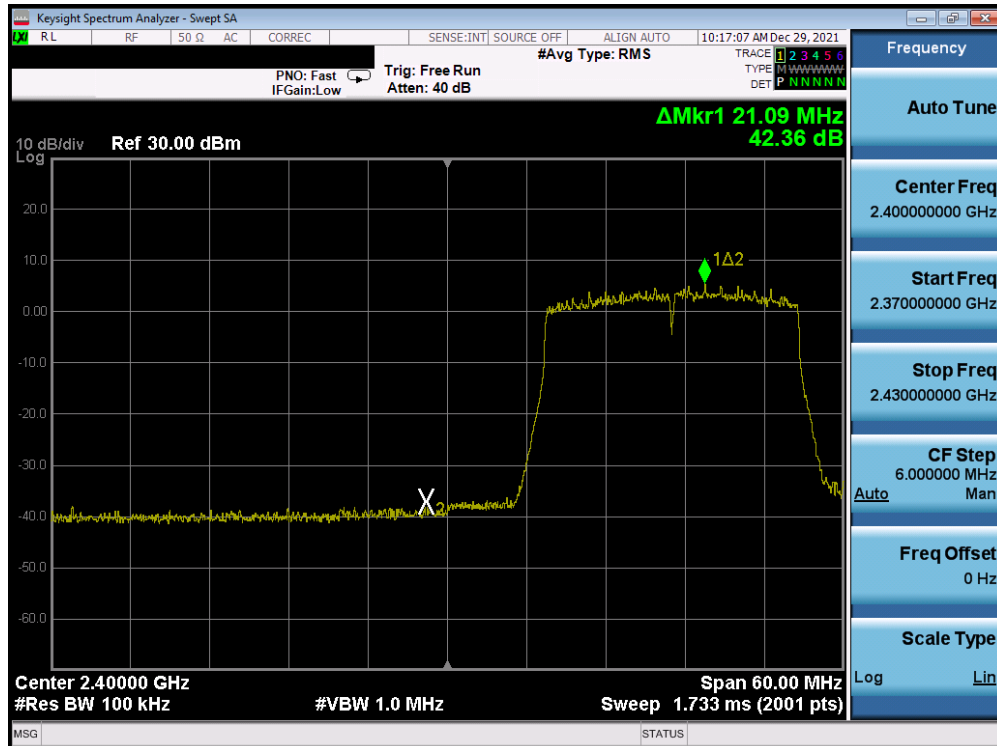
Plot 7-279. Band Edge Plot Antenna 3a (802.11ax (SU - 2.4GHz) – Ch. 2) – MCS5
