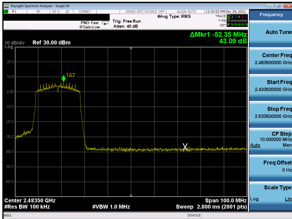
Plot 7-320. Band Edge Plot Antenna 1a (802.11ax (SU - 2.4GHz) – Ch. 9) – MCS0
