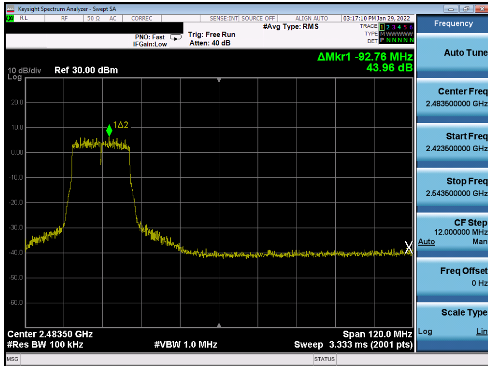
Plot 7-272. Band Edge Plot Antenna 3a (802.11n (2.4GHz) - Ch. 8) - MCS5
