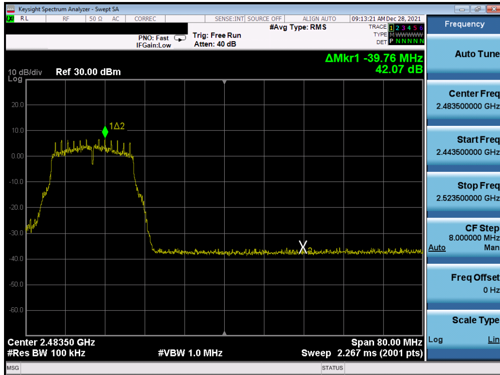
Plot 7-297. Band Edge Plot Antenna 1a (802.11g - Ch. 10) - 6Mbps
