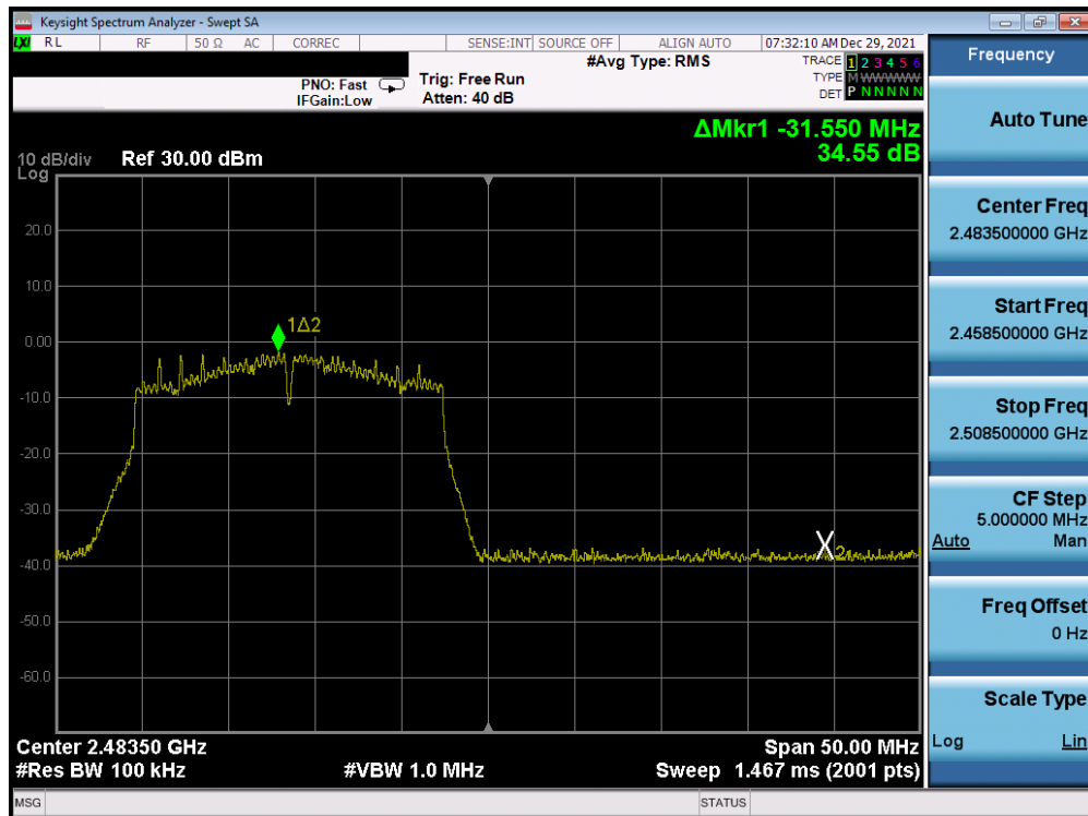
Plot 7-349. Band Edge Plot Antenna 1a (802.11n (2.4GHz) – Ch. 13) – MCS3
