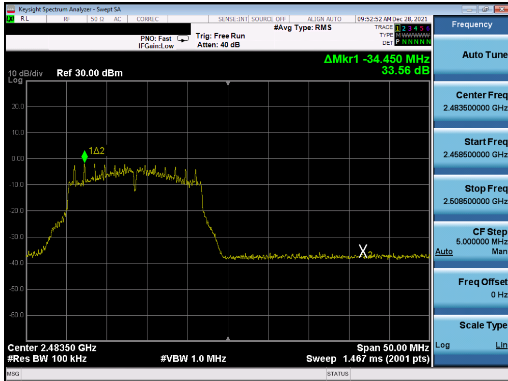
Plot 7-336. Band Edge Plot Antenna 1a (802.11g – Ch. 13) – 18Mbps
