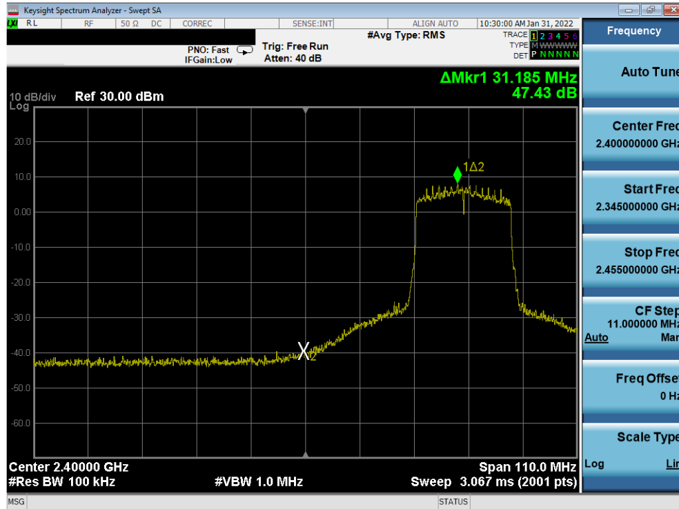
Plot 7-354. Band Edge Plot Antenna 1a (802.11ax (SU - 2.4GHz) – Ch. 5) – MCS3
