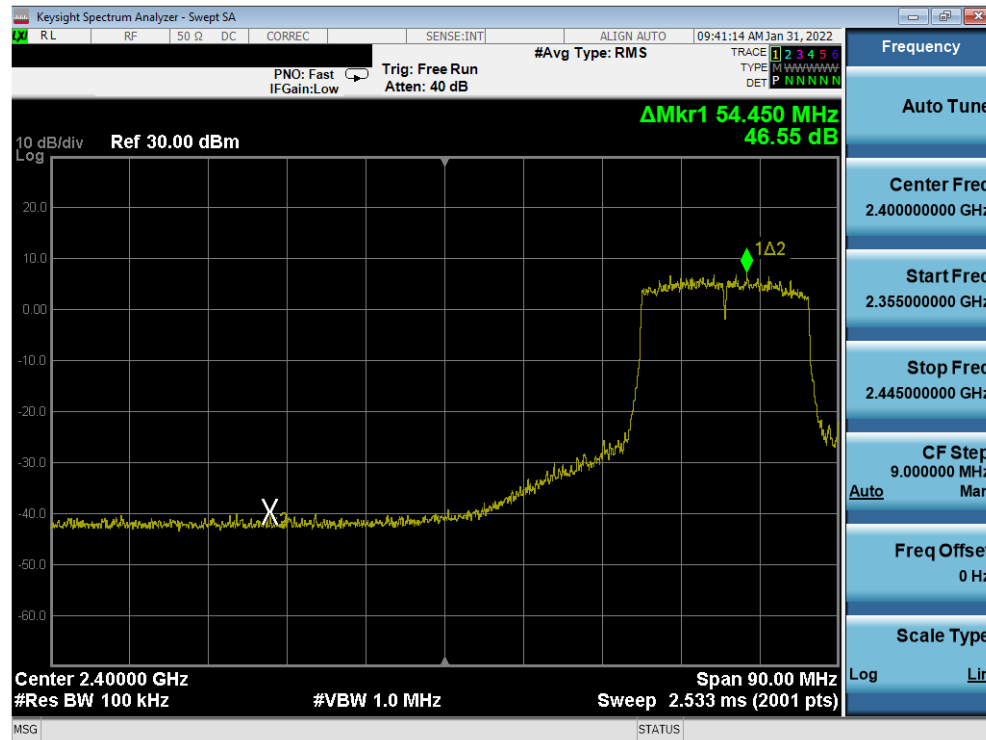
Plot 7-282. Band Edge Plot Antenna 3a (802.11ax (SU - 2.4GHz) – Ch. 5) – MCS5
