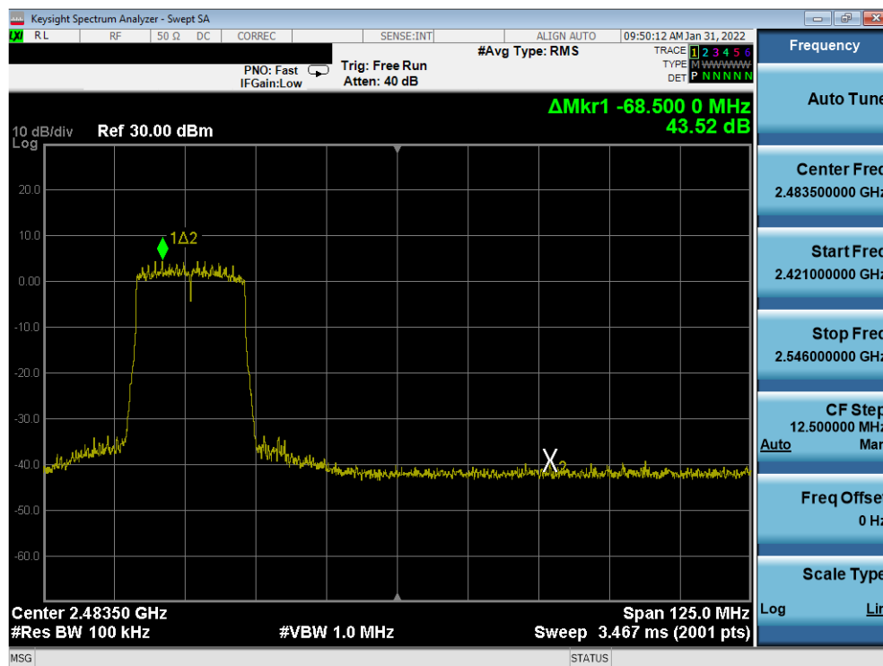
Plot 7-285. Band Edge Plot Antenna 3a (802.11ax (SU - 2.4GHz) – Ch. 8) – MCS5
