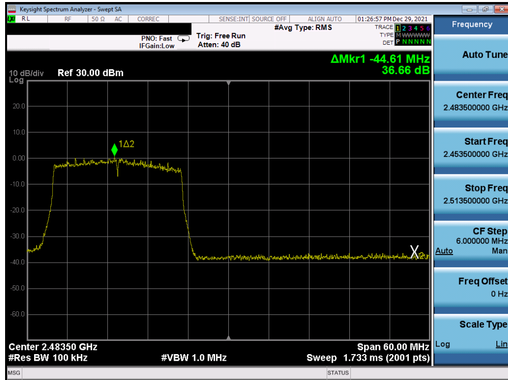
Plot 7-362. Band Edge Plot Antenna 1a (802.11ax (SU - 2.4GHz) – Ch. 12) – MCS3
