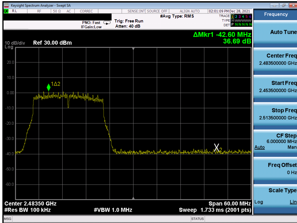
Plot 7-276. Band Edge Plot Antenna 3a (802.11n (2.4GHz) – Ch. 12) – MCS5
