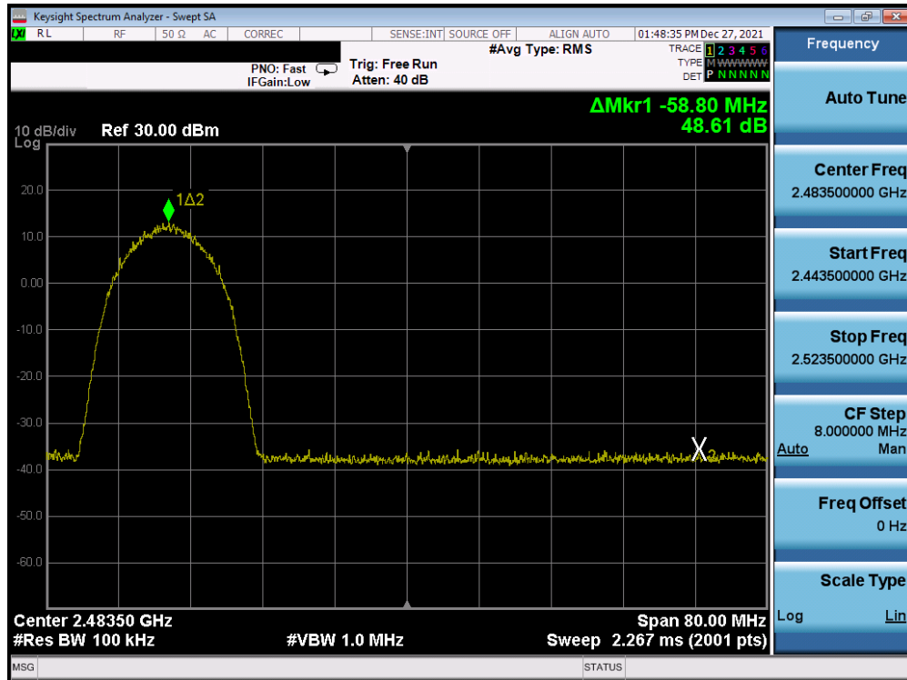
Plot 7-367. Band Edge Plot Antenna 1a (802.11b – Ch. 10) – 11Mbps
