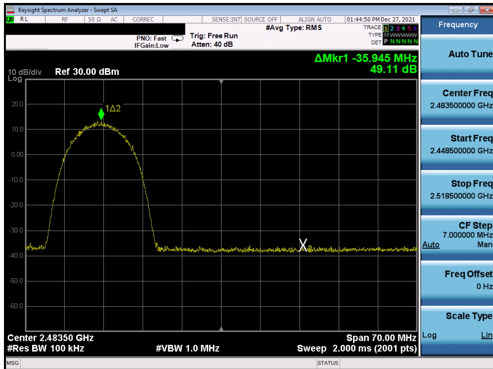
Plot 7-368. Band Edge Plot Antenna 1a (802.11b – Ch. 11) – 11Mbps
