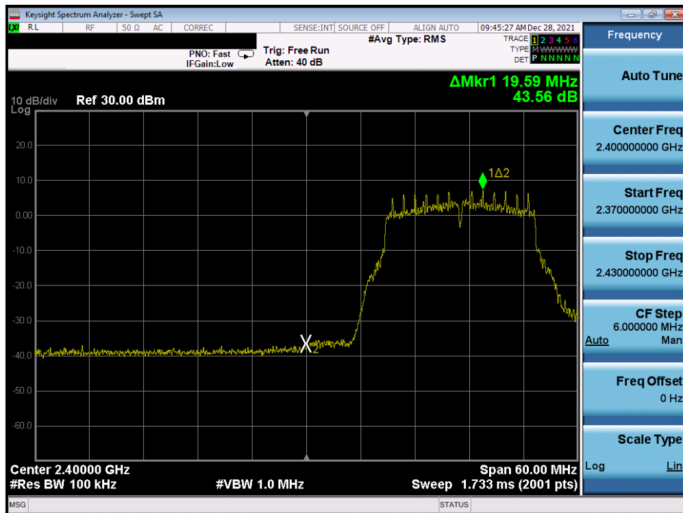
Plot 7-325. Band Edge Plot Antenna 1a (802.11g- Ch. 2) – 18Mbps
