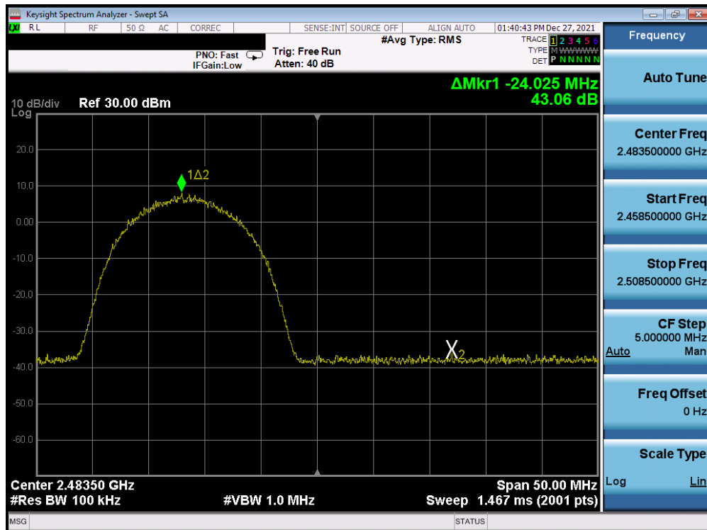
Plot 7-370. Band Edge Plot Antenna 1a (802.11b – Ch. 13) – 11Mbps
