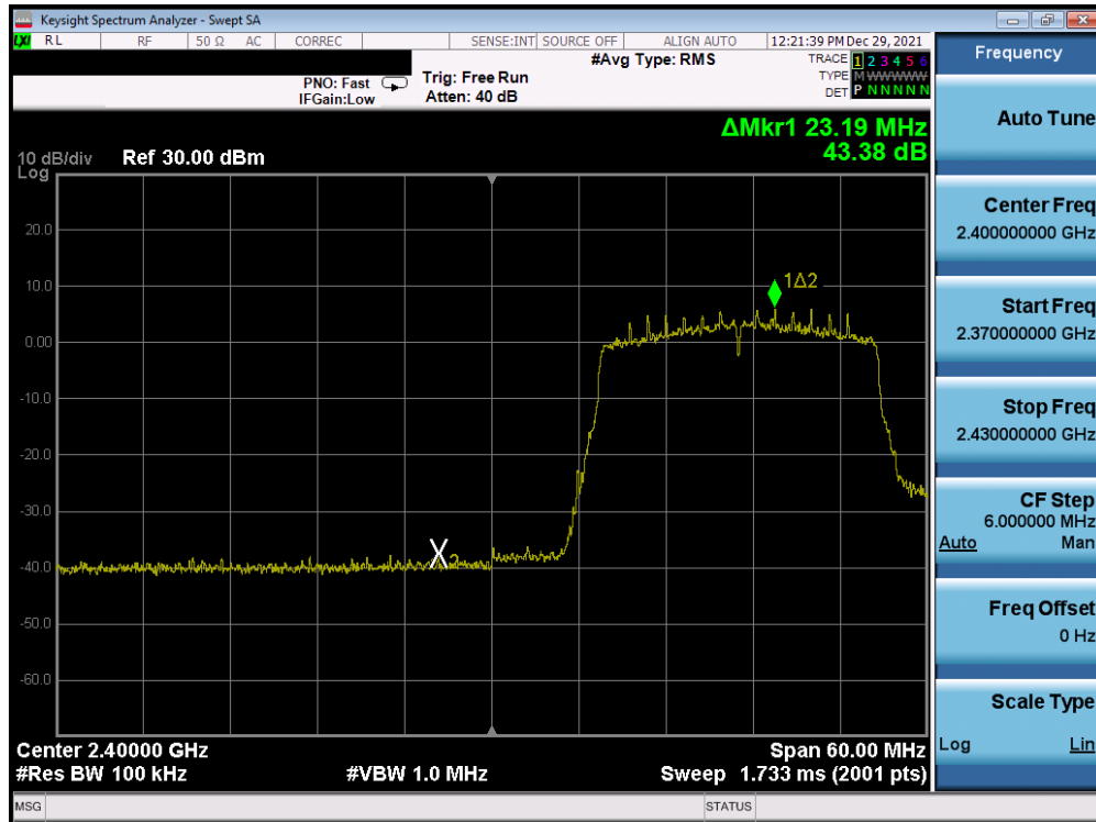
Plot 7-313. Band Edge Plot Antenna 1a (802.11ax (SU - 2.4GHz) – Ch. 2) – MCS0
