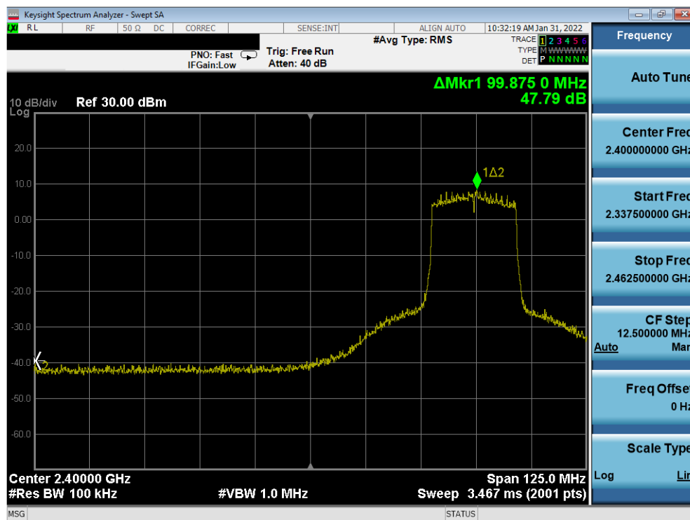
Plot 7-355. Band Edge Plot Antenna 1a (802.11ax (SU - 2.4GHz) – Ch. 6 (Low)) – MCS3
