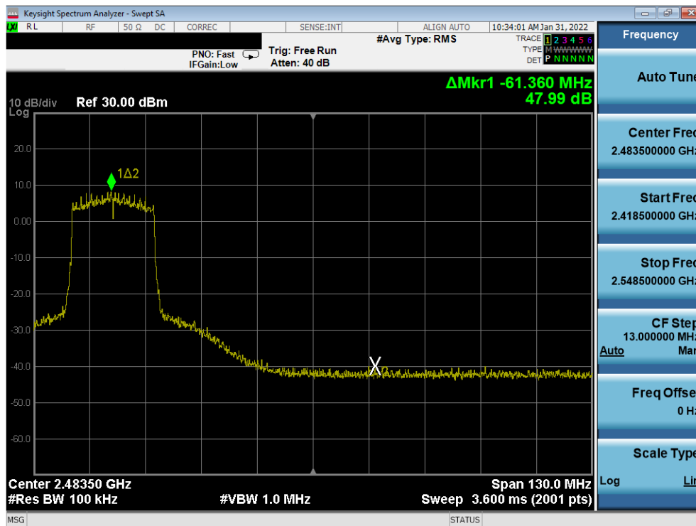
Plot 7-356. Band Edge Plot Antenna 1a (802.11ax (SU - 2.4GHz) – Ch. 6 (High)) – MCS3
