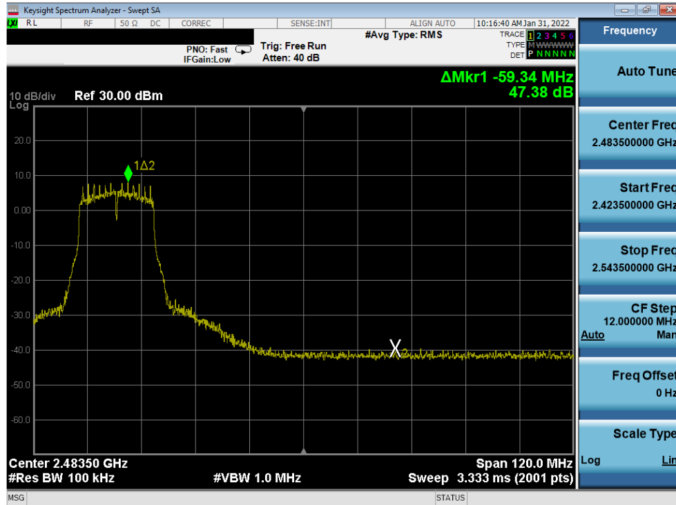
Plot 7-330. Band Edge Plot Antenna 1a (802.11g - Ch. 7) - 18Mbps
