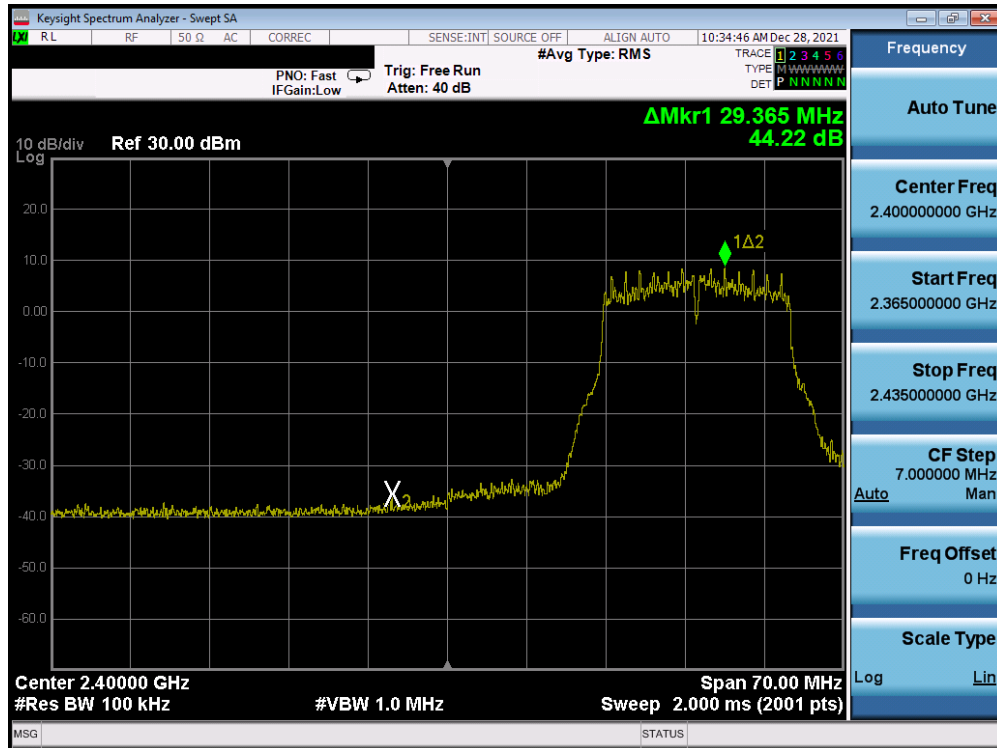
Plot 7-373. Band Edge Plot Antenna 1a (802.11g- Ch. 3) - 36Mbps
