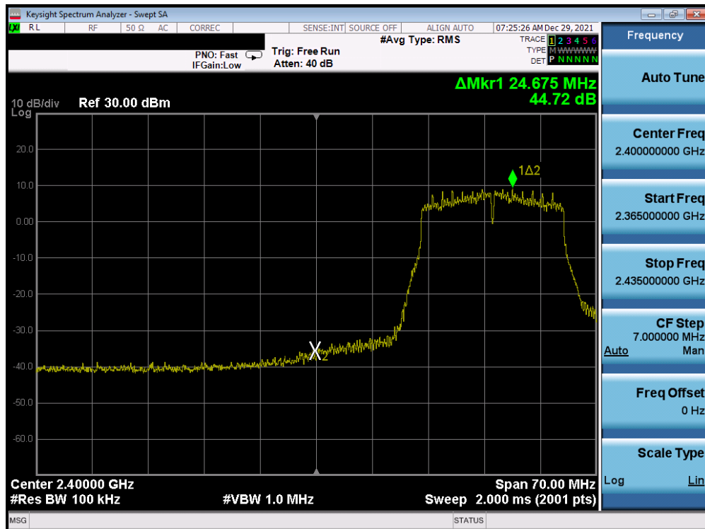
Plot 7-339. Band Edge Plot Antenna 1a (802.11n (2.4GHz) - Ch. 3) - MCS3
