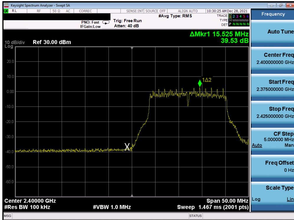
Plot 7-371. Band Edge Plot Antenna 1a (802.11g- Ch. 1) – 36Mbps
