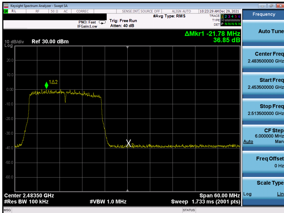
Plot 7-289. Band Edge Plot Antenna 3a (802.11ax (SU - 2.4GHz) – Ch. 12) – MCS5
