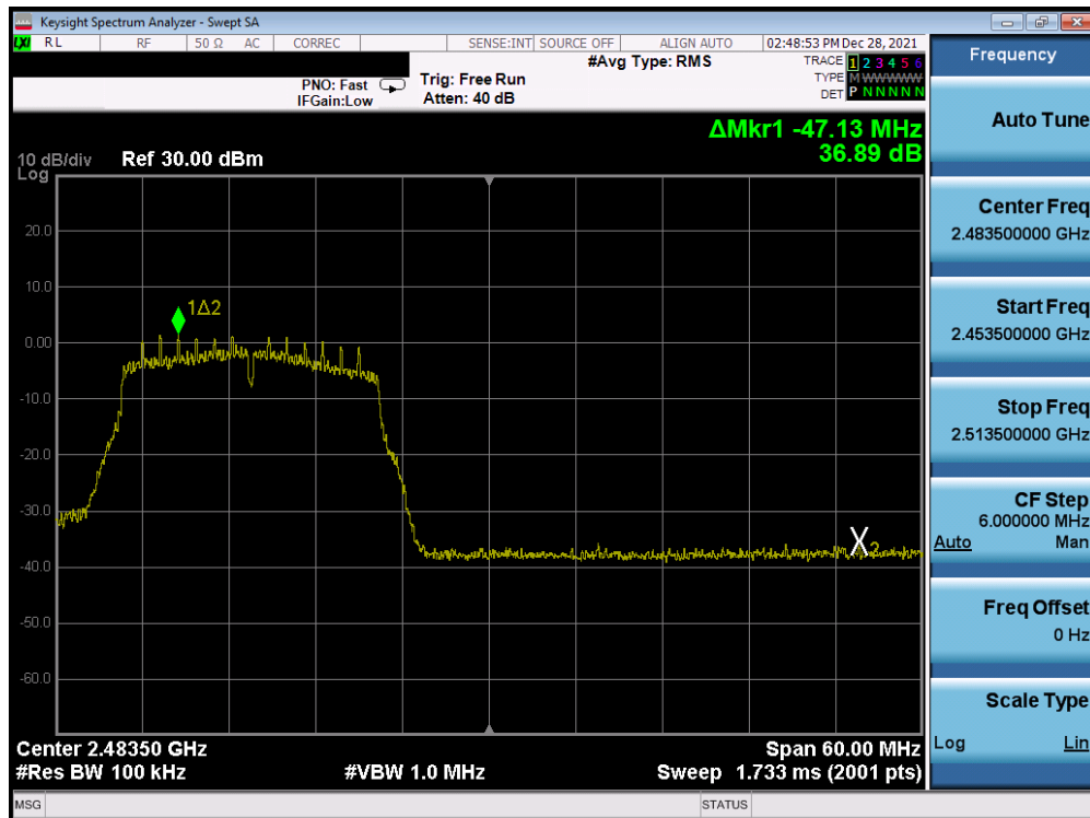
Plot 7-310. Band Edge Plot Antenna 1a (802.11n (2.4GHz) – Ch. 12) – MCS0
