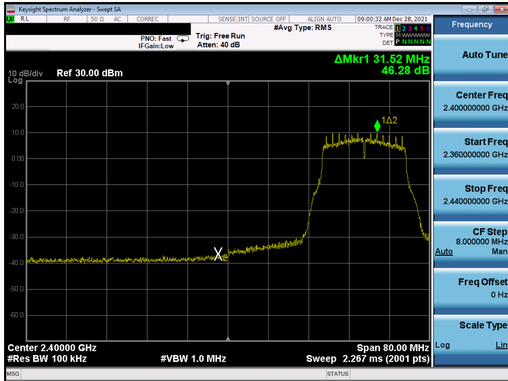
Plot 7-293. Band Edge Plot Antenna 1a (802.11g- Ch. 4) – 6Mbps
