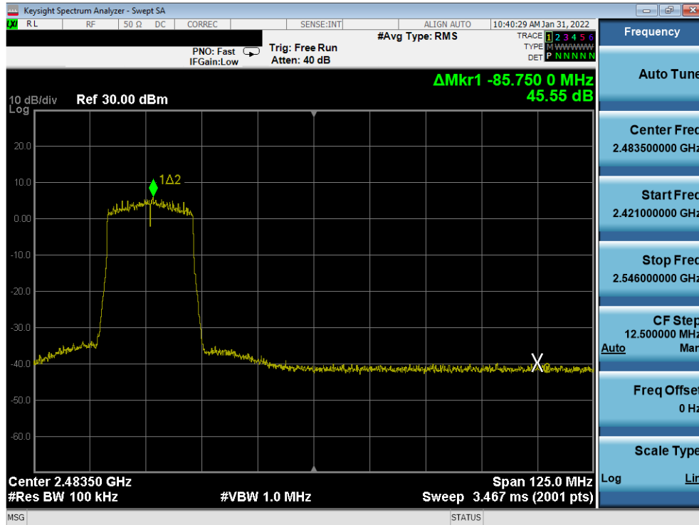
Plot 7-358. Band Edge Plot Antenna 1a (802.11ax (SU - 2.4GHz) – Ch. 8) – MCS3
