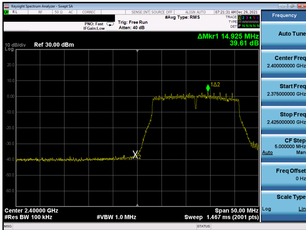
Plot 7-337. Band Edge Plot Antenna 1a (802.11n (2.4GHz) – Ch. 1) – MCS3
