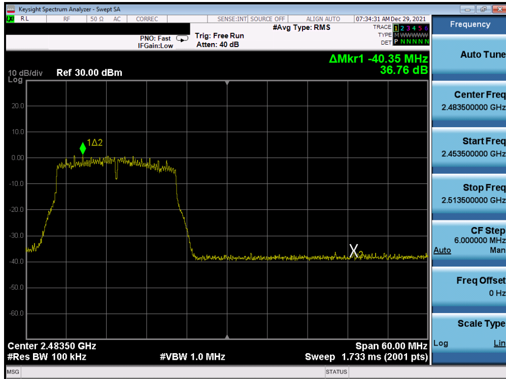
Plot 7-348. Band Edge Plot Antenna 1a (802.11n (2.4GHz) – Ch. 12) – MCS3
