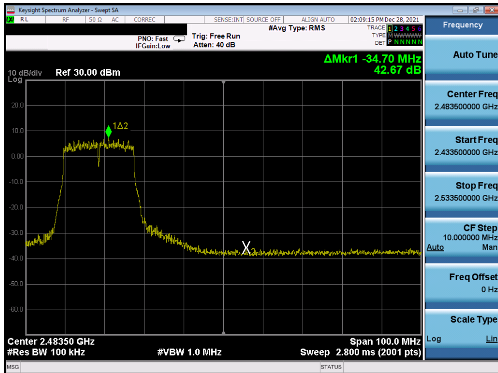
Plot 7-273. Band Edge Plot Antenna 3a (802.11n (2.4GHz) - Ch. 9) - MCS5
