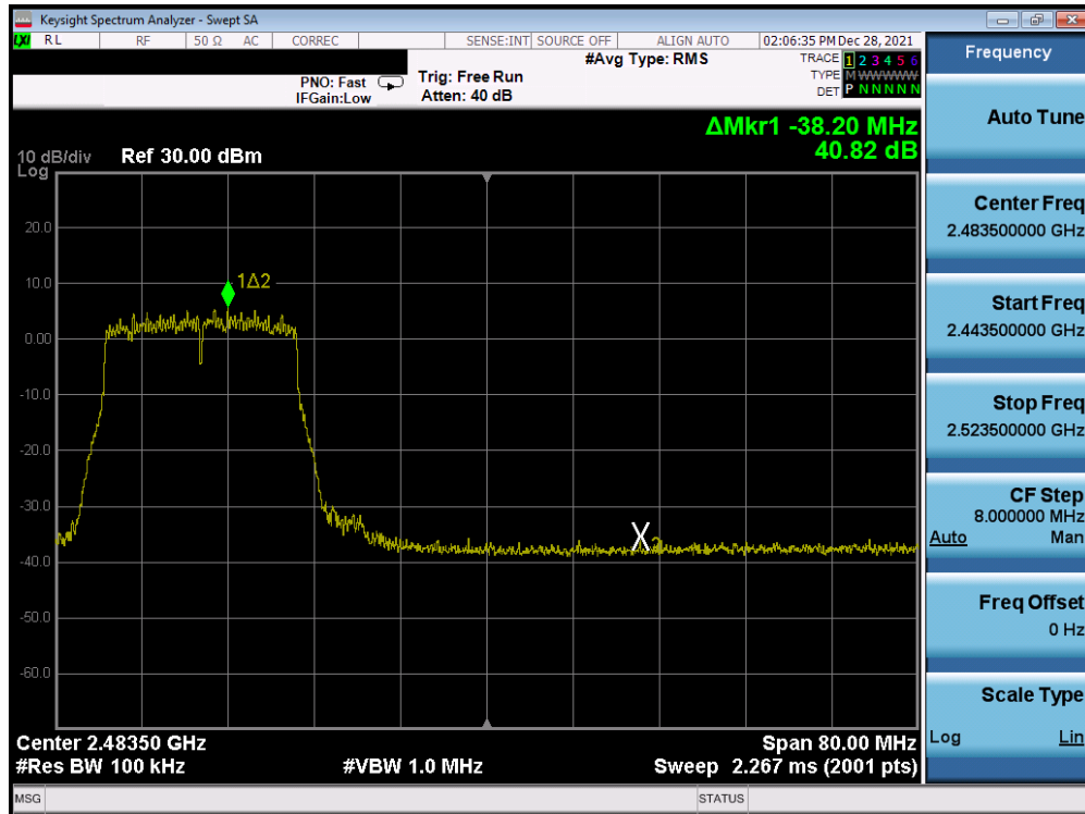
Plot 7-274. Band Edge Plot Antenna 3a (802.11n (2.4GHz) - Ch. 10) - MCS5
