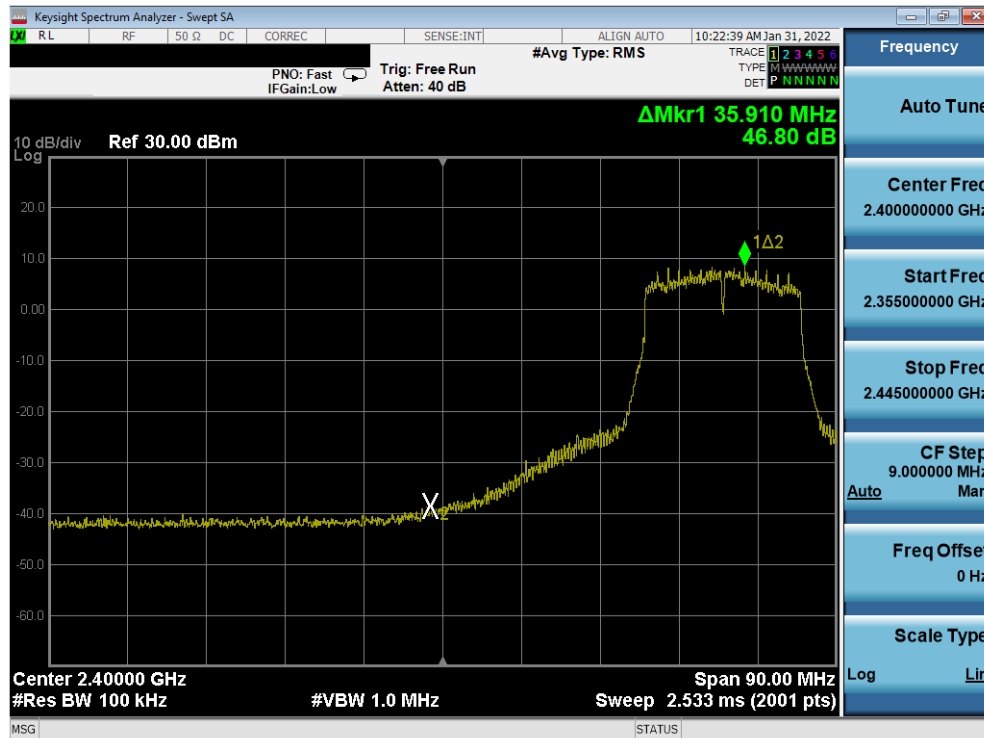
Plot 7-341. Band Edge Plot Antenna 1a (802.11n (2.4GHz) - Ch. 5) - MCS3
