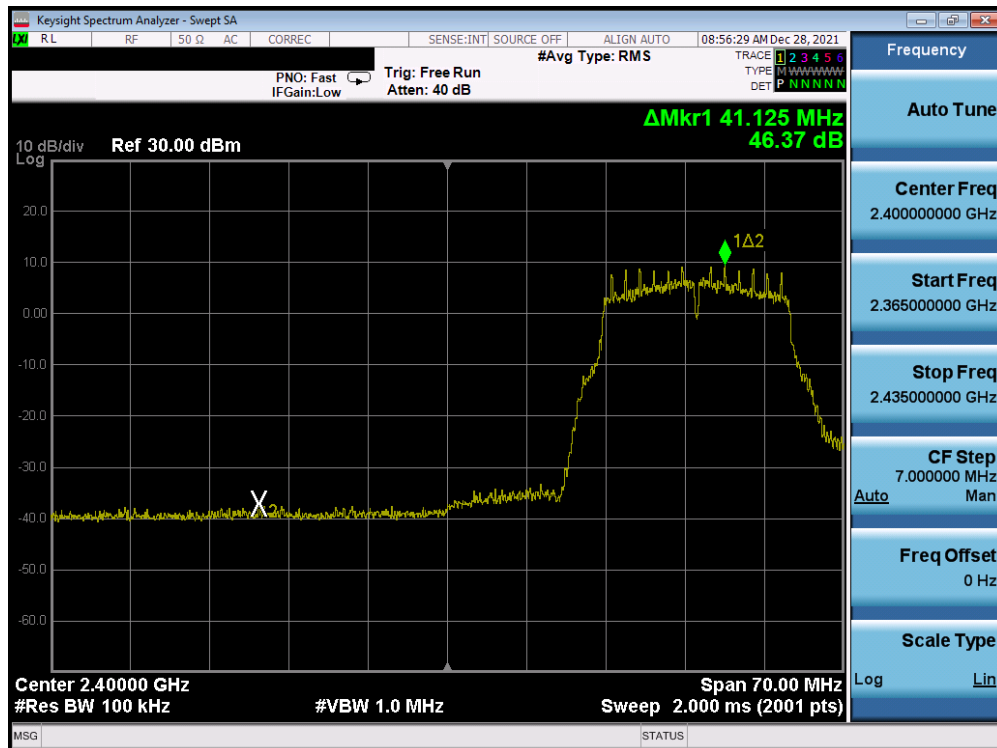
Plot 7-292. Band Edge Plot Antenna 1a (802.11g- Ch. 3) – 6Mbps
