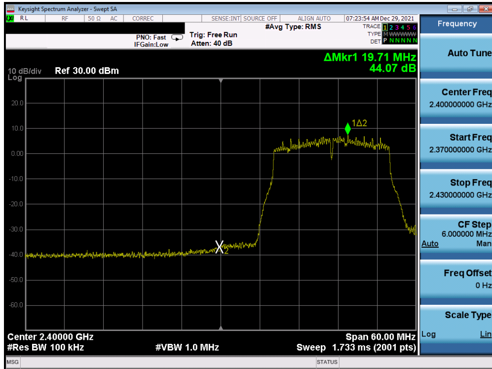
Plot 7-338. Band Edge Plot Antenna 1a (802.11n (2.4GHz) - Ch. 2) - MCS3
