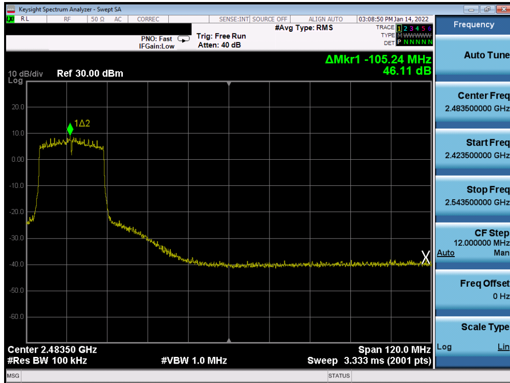
Plot 7-317. Band Edge Plot Antenna 1a (802.11ax (SU - 2.4GHz) – Ch. 6(High)) – MCS0
