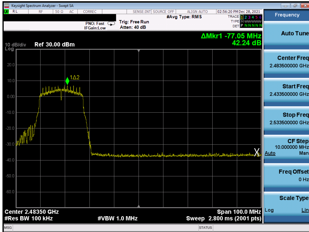
Plot 7-307. Band Edge Plot Antenna 1a (802.11n (2.4GHz) - Ch. 9) - MCS0
