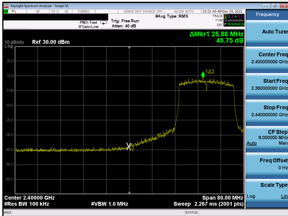
Plot 7-281. Band Edge Plot Antenna 3a (802.11ax (SU - 2.4GHz) – Ch. 4) – MCS5
