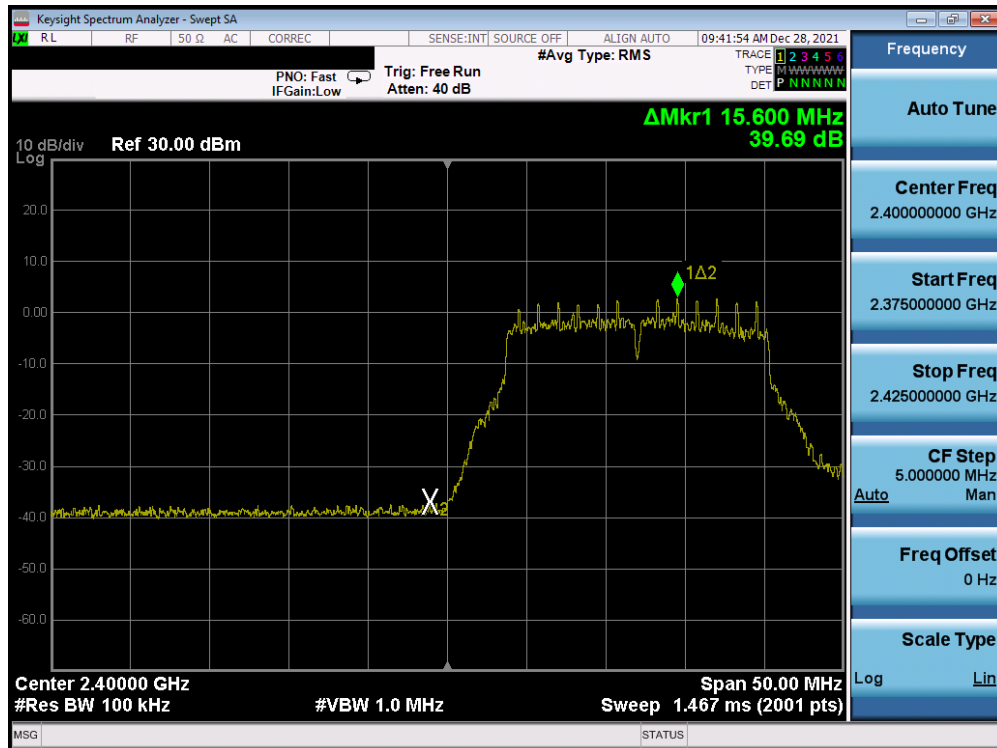
Plot 7-324. Band Edge Plot Antenna 1a (802.11g- Ch. 1) – 18Mbps
