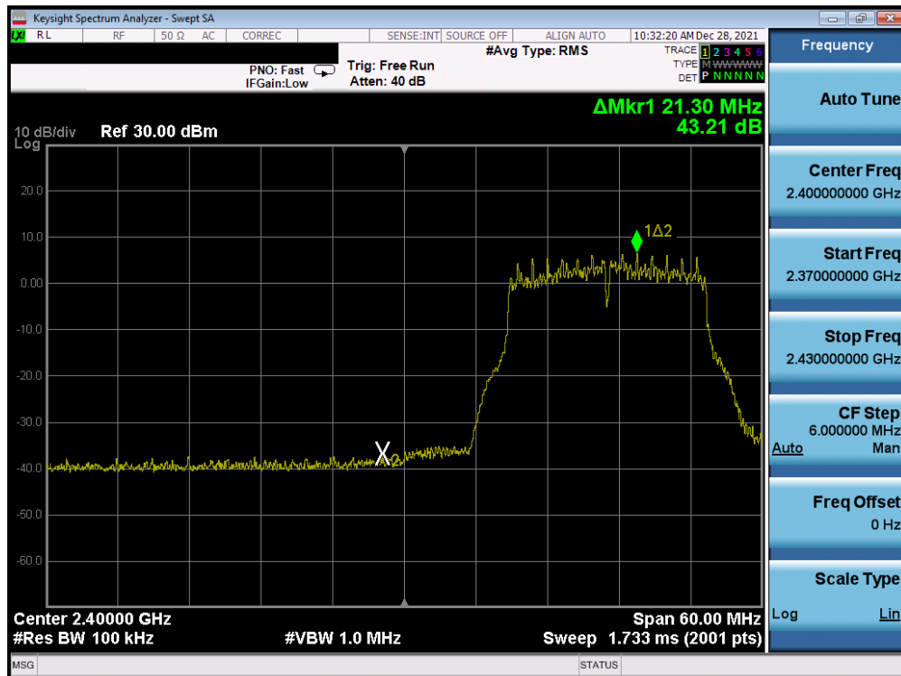
Plot 7-372. Band Edge Plot Antenna 1a (802.11g- Ch. 2) – 36Mbps
