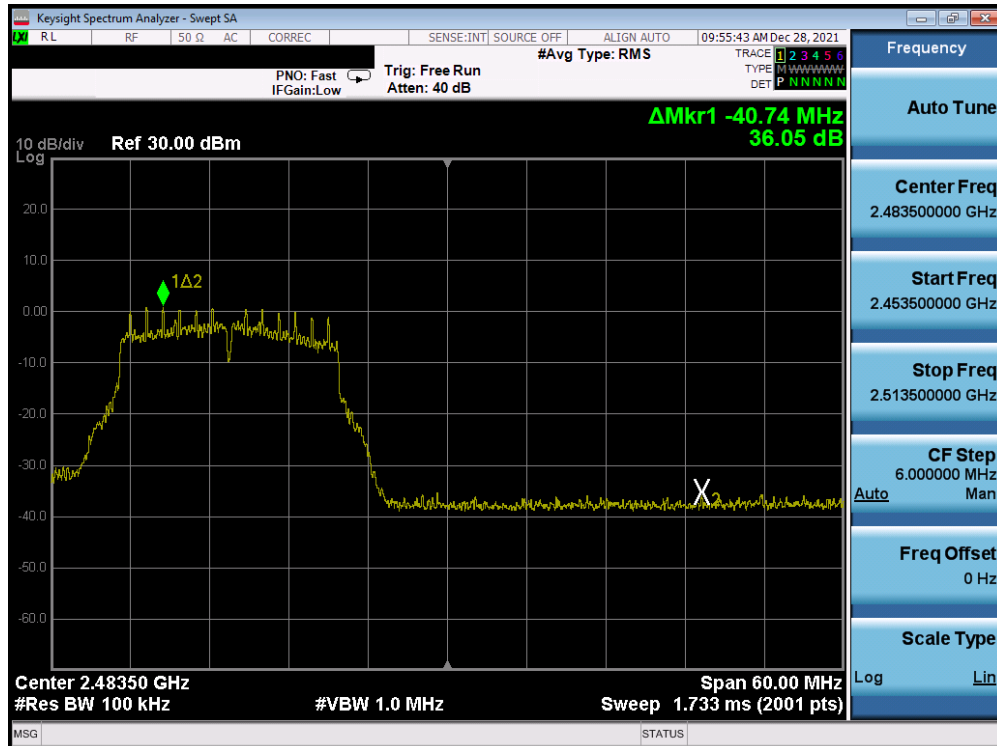
Plot 7-335. Band Edge Plot Antenna 1a (802.11g - Ch. 12) - 18Mbps
