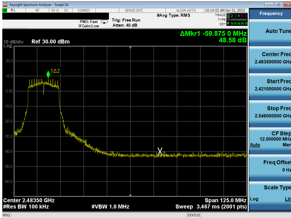
Plot 7-329. Band Edge Plot Antenna 1a (802.11g – Ch. 6 (High)) – 18Mbps
