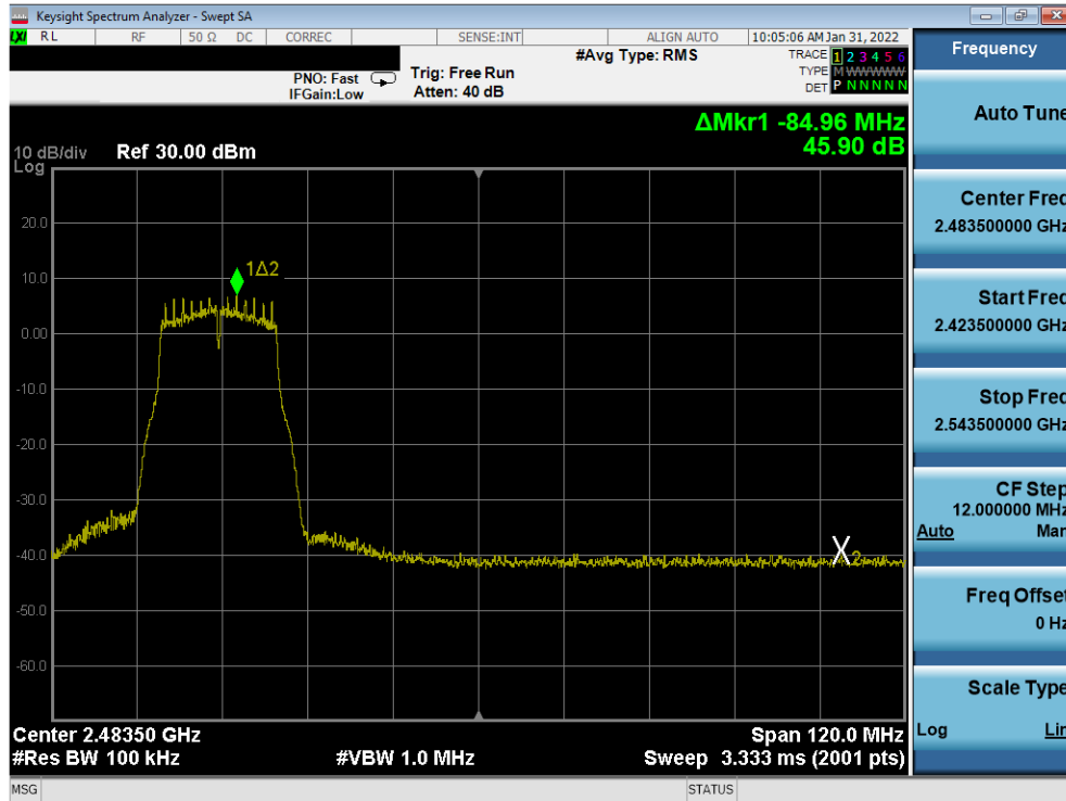
Plot 7-295. Band Edge Plot Antenna 1a (802.11g - Ch. 8) - 6Mbps
