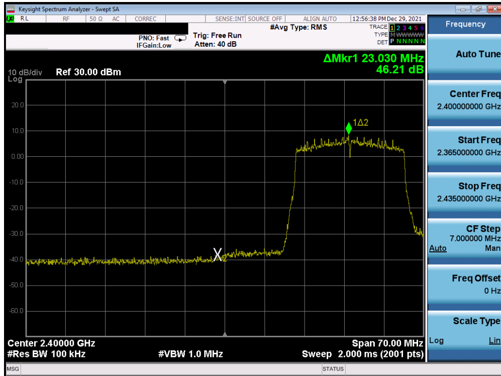
Plot 7-352. Band Edge Plot Antenna 1a (802.11ax (SU - 2.4GHz) – Ch. 3) – MCS3
