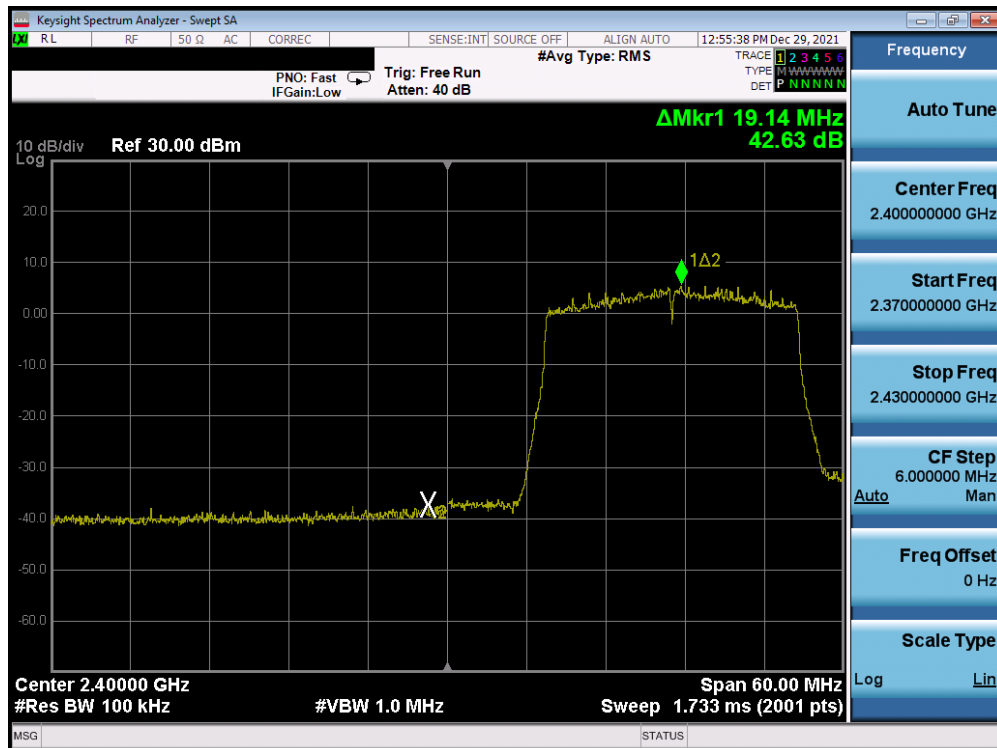
Plot 7-351. Band Edge Plot Antenna 1a (802.11ax (SU - 2.4GHz) – Ch. 2) – MCS3
