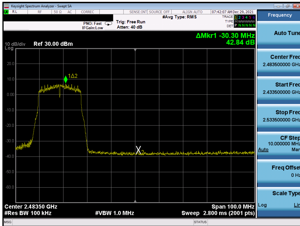
Plot 7-345. Band Edge Plot Antenna 1a (802.11n (2.4GHz) - Ch. 9) - MCS3
