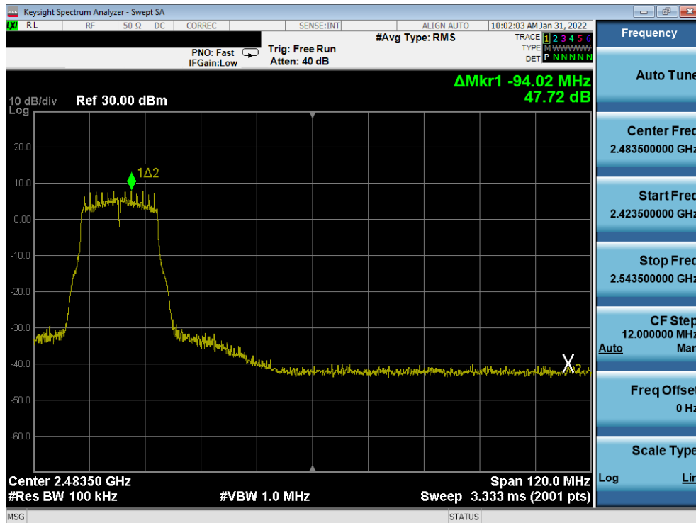
Plot 7-294. Band Edge Plot Antenna 1a (802.11g – Ch. 7) – 6Mbps
