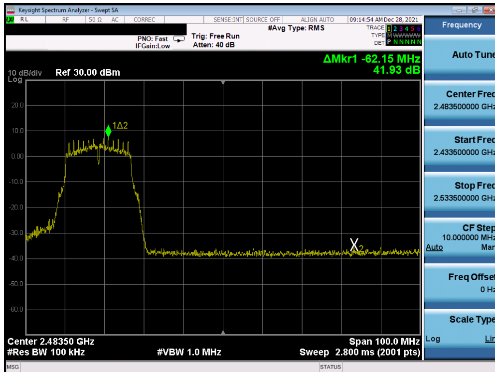
Plot 7-296. Band Edge Plot Antenna 1a (802.11g - Ch. 9) - 6Mbps
