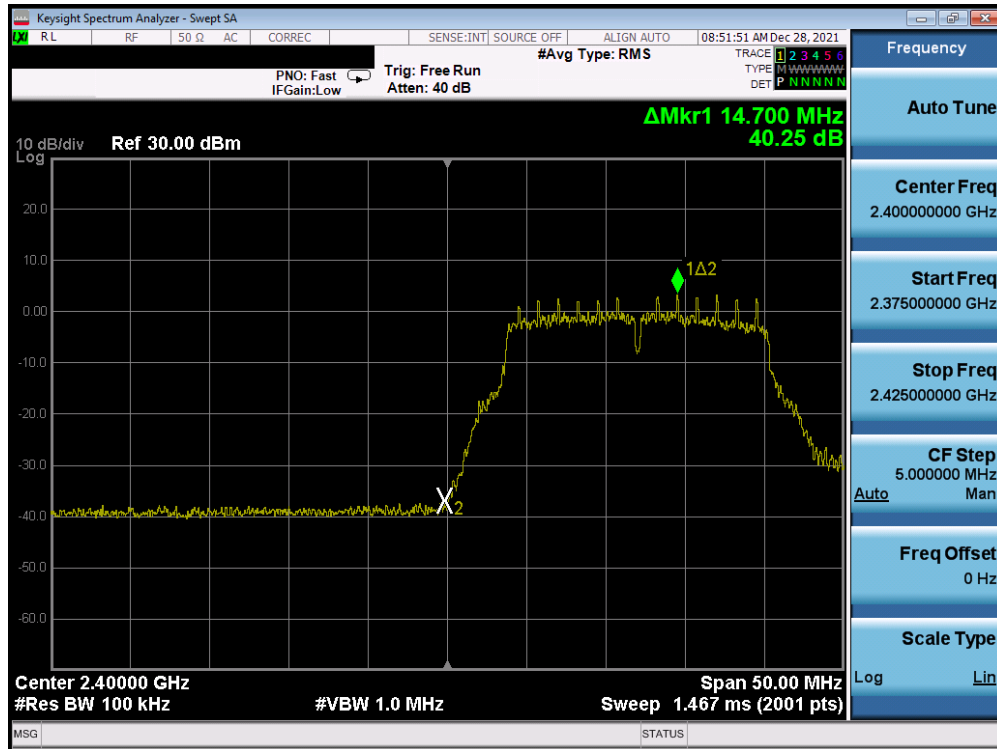
Plot 7-290. Band Edge Plot Antenna 1a (802.11g– Ch. 1) – 6Mbps
