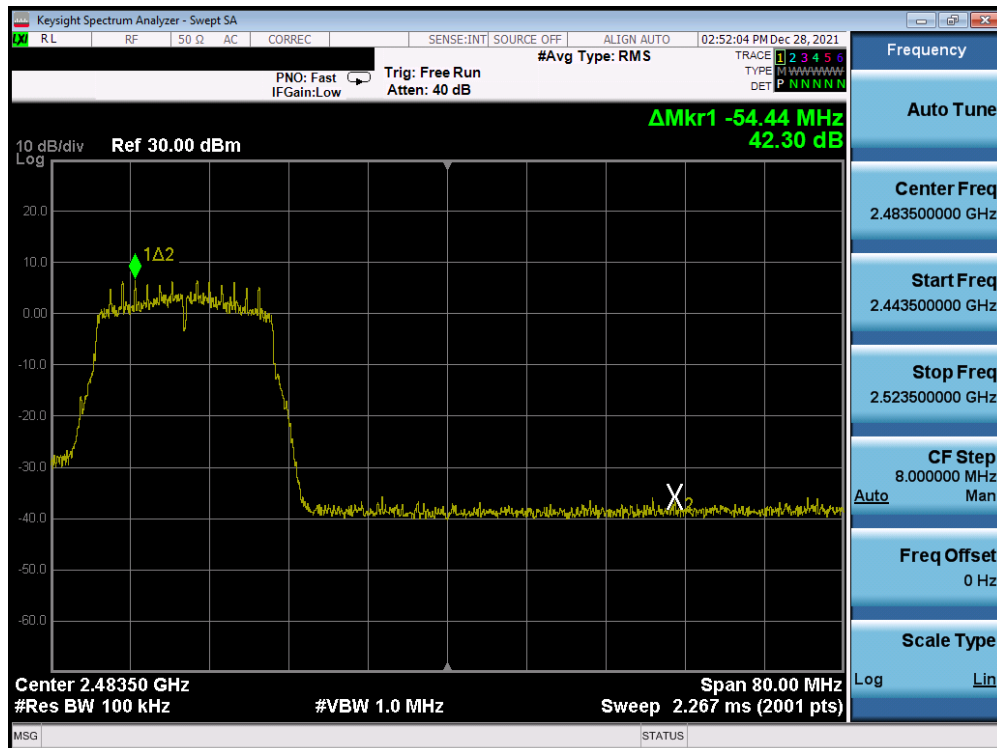
Plot 7-308. Band Edge Plot Antenna 1a (802.11n (2.4GHz) - Ch. 10) - MCS0
