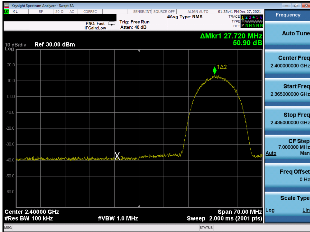
Plot 7-365. Band Edge Plot Antenna 1a (802.11b – Ch. 3) – 11Mbps
