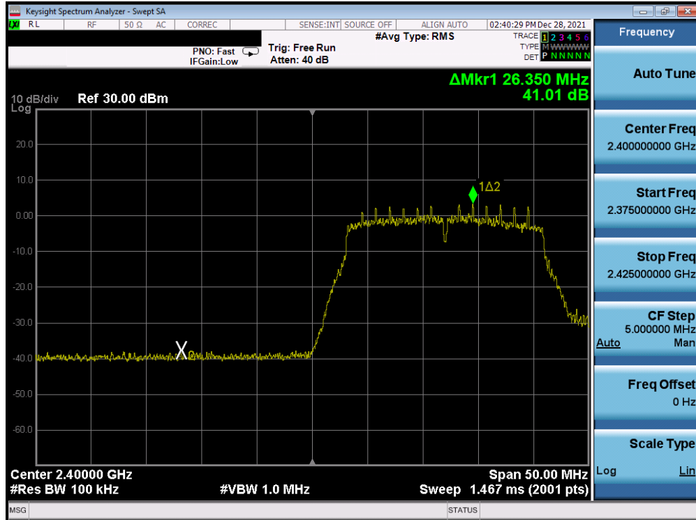
Plot 7-301. Band Edge Plot Antenna 1a (802.11n (2.4GHz) - Ch. 1) - MCS0
