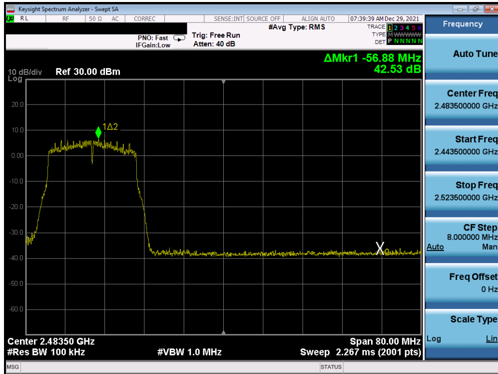
Plot 7-346. Band Edge Plot Antenna 1a (802.11n (2.4GHz) – Ch. 10) – MCS3
