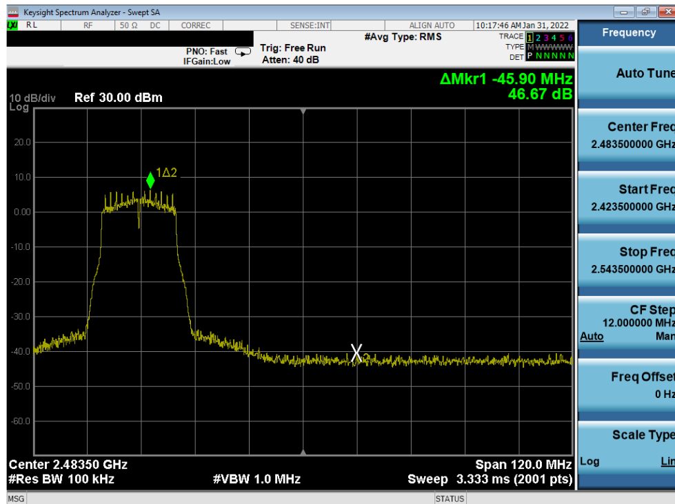
Plot 7-331. Band Edge Plot Antenna 1a (802.11g - Ch. 8) - 18Mbps
