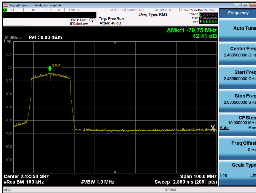
Plot 7-359. Band Edge Plot Antenna 1a (802.11ax (SU - 2.4GHz) – Ch. 9) – MCS3
