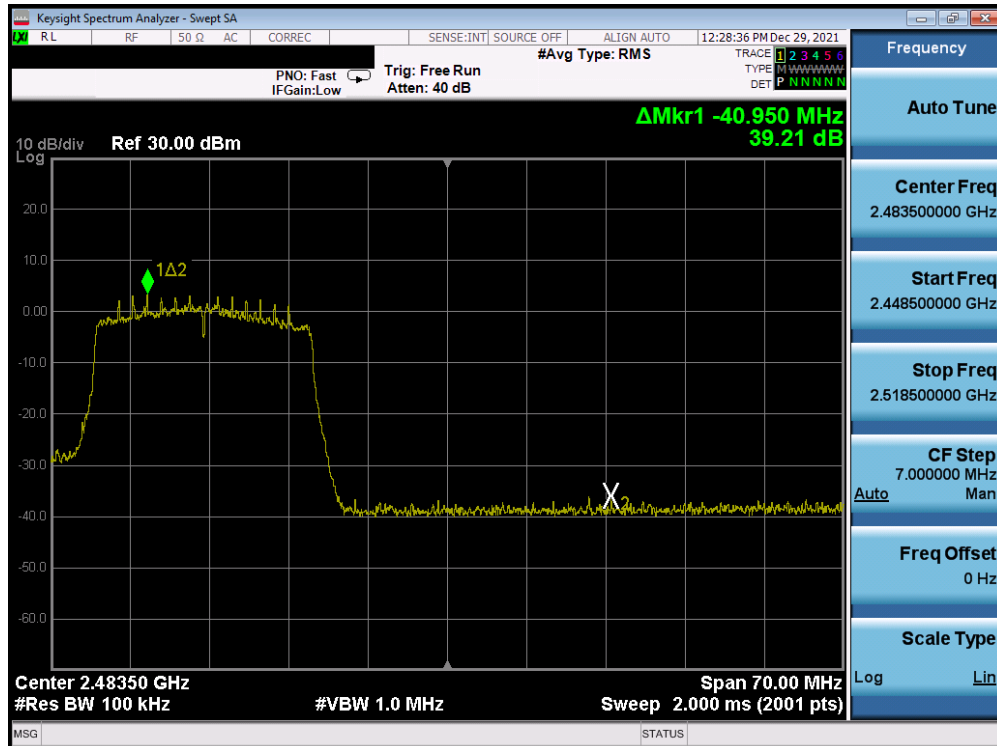
Plot 7-322. Band Edge Plot Antenna 1a (802.11ax (SU - 2.4GHz) – Ch. 11) – MCS0
