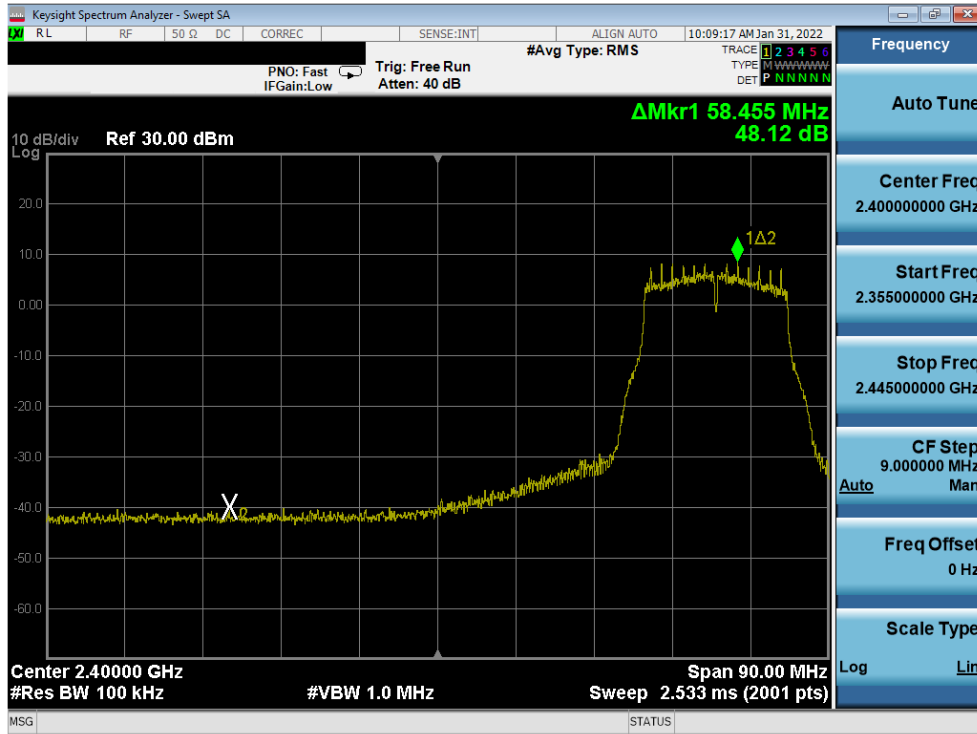
Plot 7-328. Band Edge Plot Antenna 1a (802.11g– Ch. 5) – 18Mbps
