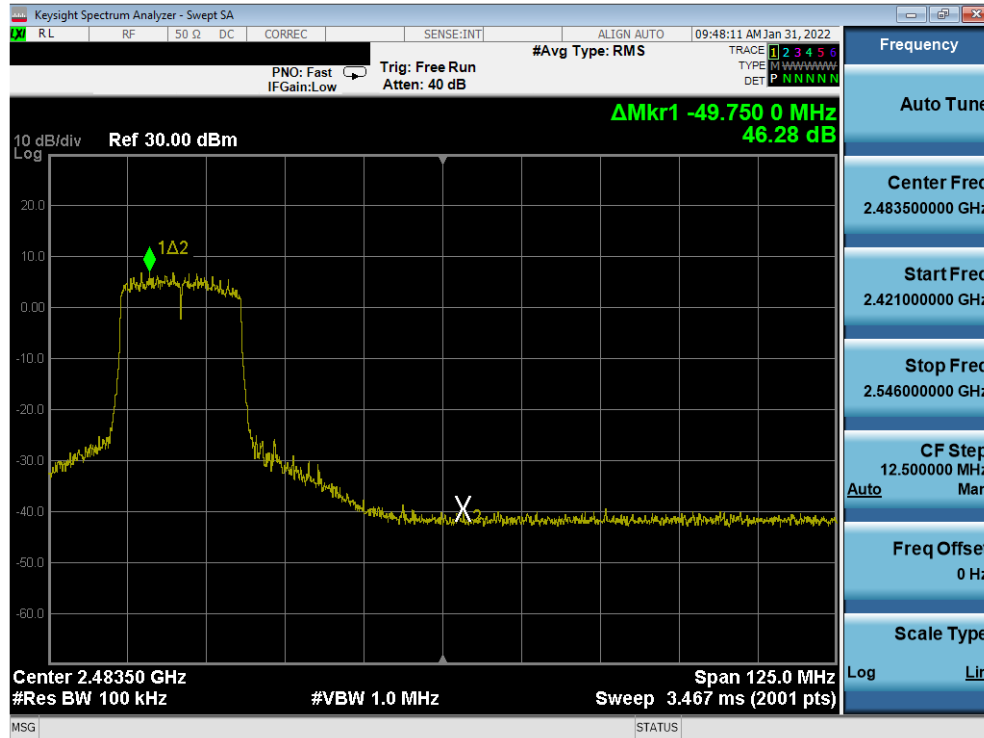
Plot 7-284. Band Edge Plot Antenna 3a (802.11ax (SU - 2.4GHz) – Ch. 7) – MCS5
