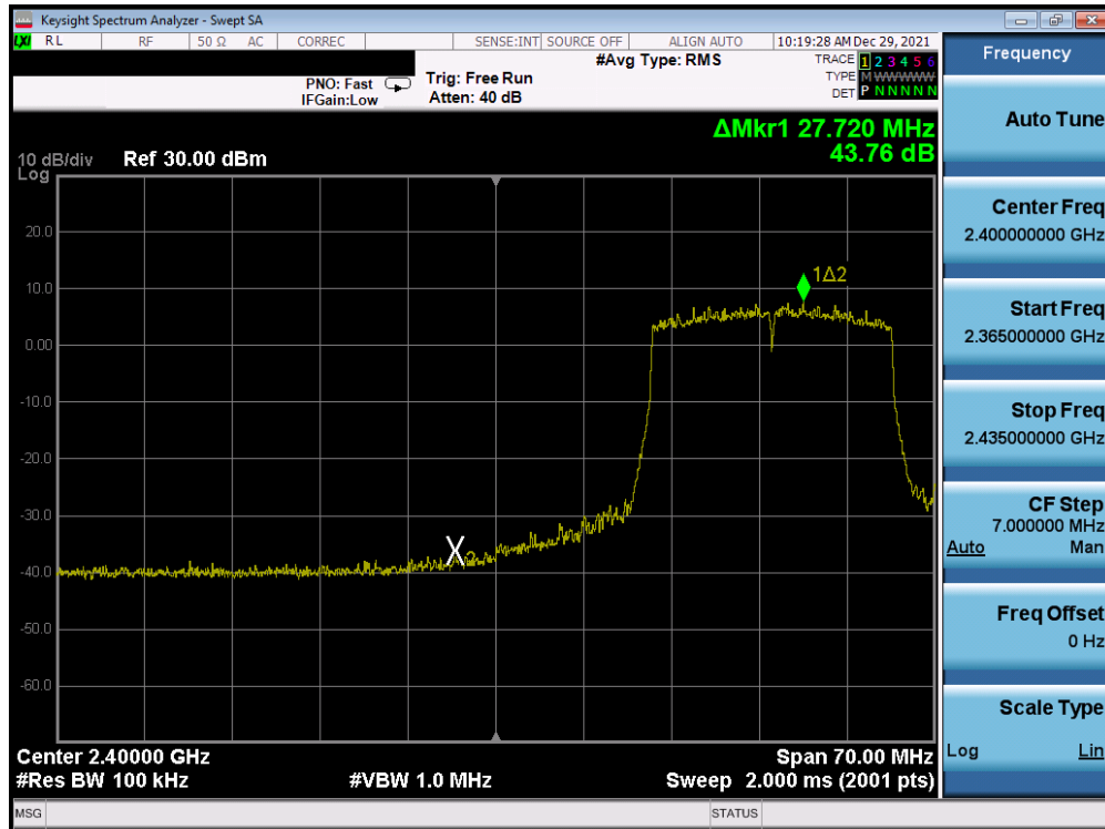
Plot 7-280. Band Edge Plot Antenna 3a (802.11ax (SU - 2.4GHz) – Ch. 3) – MCS5
