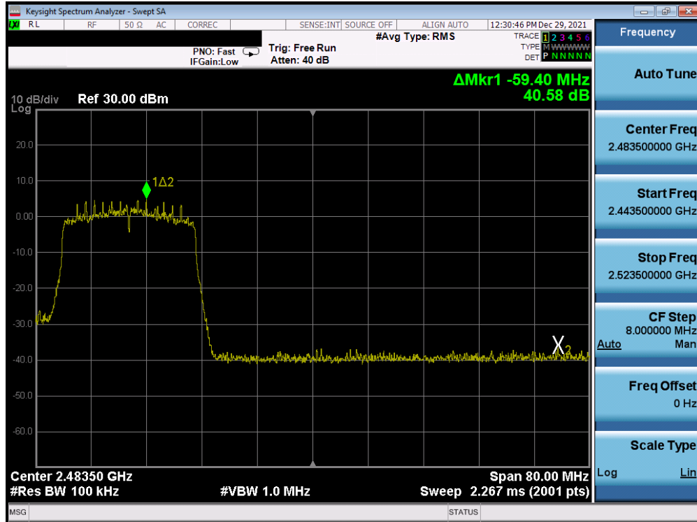
Plot 7-321. Band Edge Plot Antenna 1a (802.11ax (SU - 2.4GHz) – Ch. 10) – MCS0
