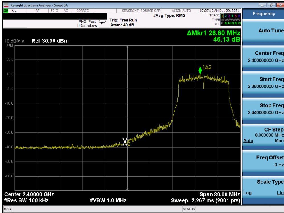
Plot 7-340. Band Edge Plot Antenna 1a (802.11n (2.4GHz) - Ch. 4) - MCS3
