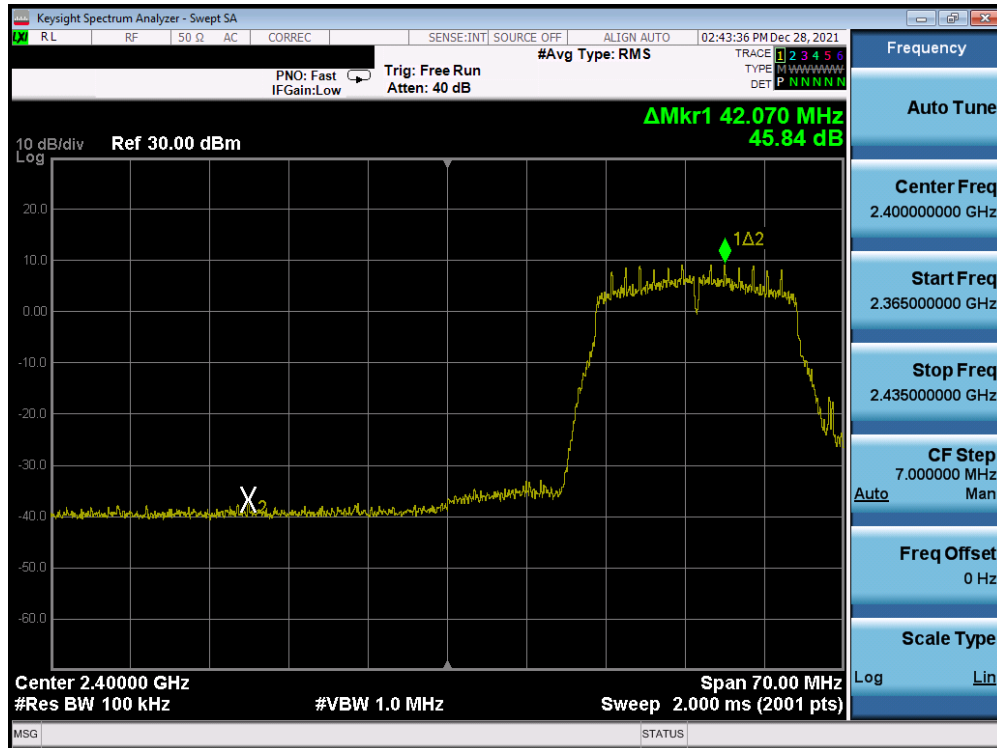
Plot 7-303. Band Edge Plot Antenna 1a (802.11n (2.4GHz) – Ch. 3) – MCS0
