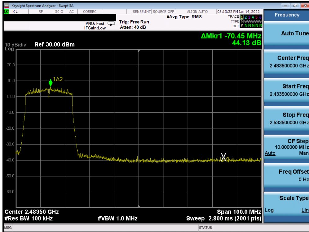
Plot 7-319. Band Edge Plot Antenna 1a (802.11ax (SU - 2.4GHz) – Ch. 8) – MCS0
