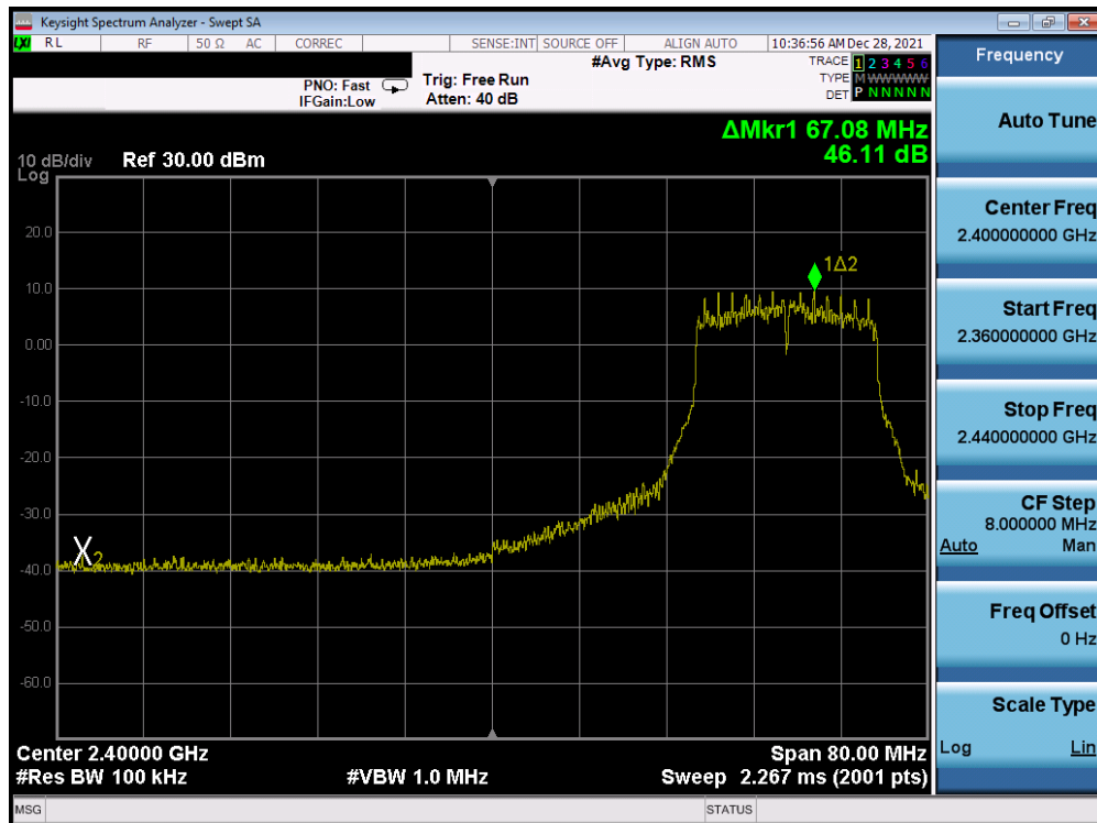
Plot 7-374. Band Edge Plot Antenna 1a (802.11g- Ch. 4) - 36Mbps
