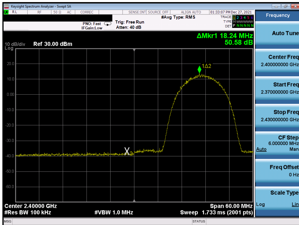
Plot 7-364. Band Edge Plot Antenna 1a (802.11b – Ch. 2) – 11Mbps
