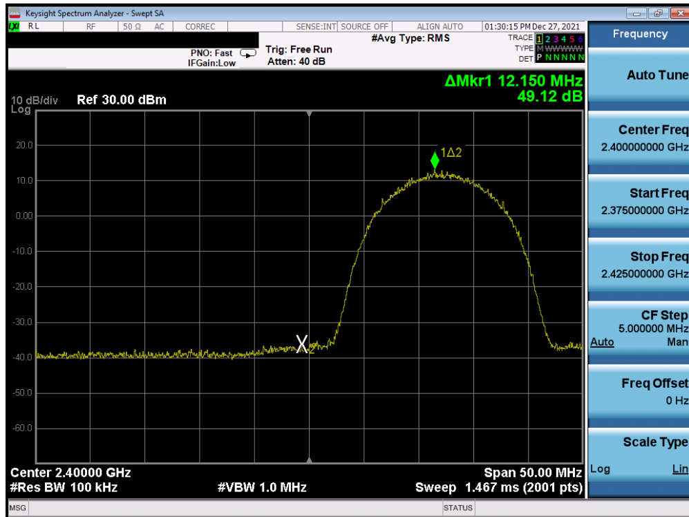
Plot 7-363. Band Edge Plot Antenna 1a (802.11b – Ch. 1) – 11Mbps
