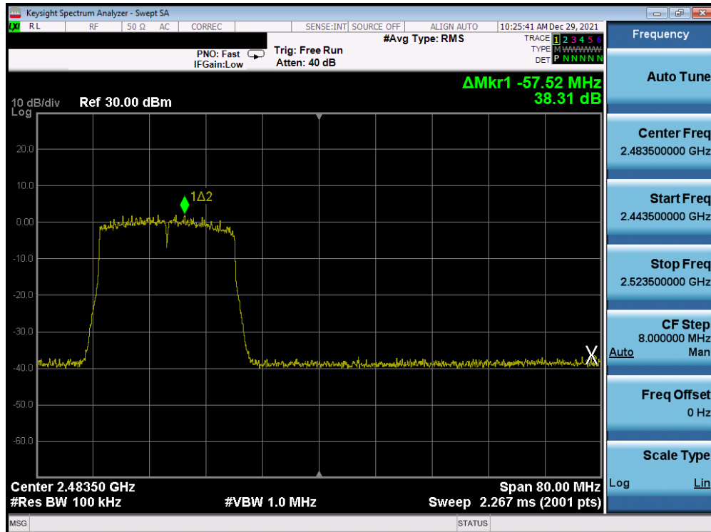
Plot 7-288. Band Edge Plot Antenna 3a (802.11ax (SU - 2.4GHz) – Ch. 11) – MCS5
