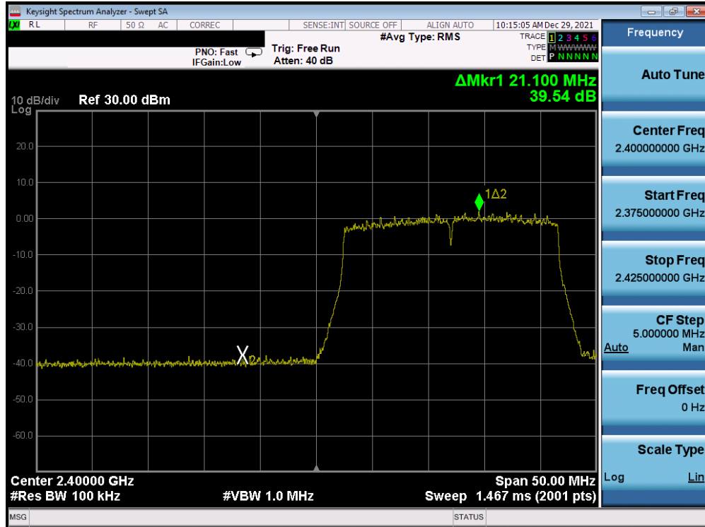
Plot 7-278. Band Edge Plot Antenna 3a (802.11ax (SU - 2.4GHz) – Ch. 1) – MCS5
