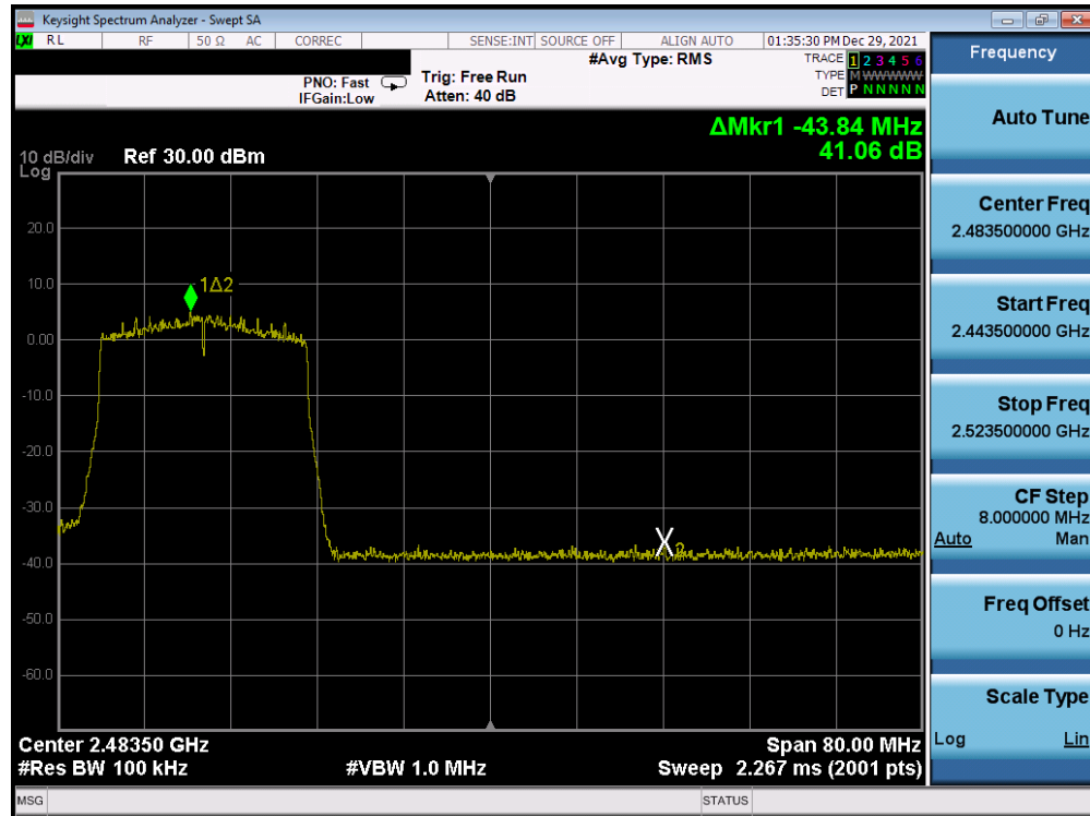
Plot 7-360. Band Edge Plot Antenna 1a (802.11ax (SU - 2.4GHz) – Ch. 10) – MCS3
