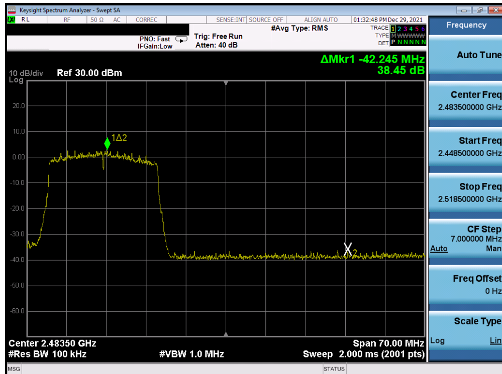
Plot 7-361. Band Edge Plot Antenna 1a (802.11ax (SU - 2.4GHz) – Ch. 11) – MCS3
