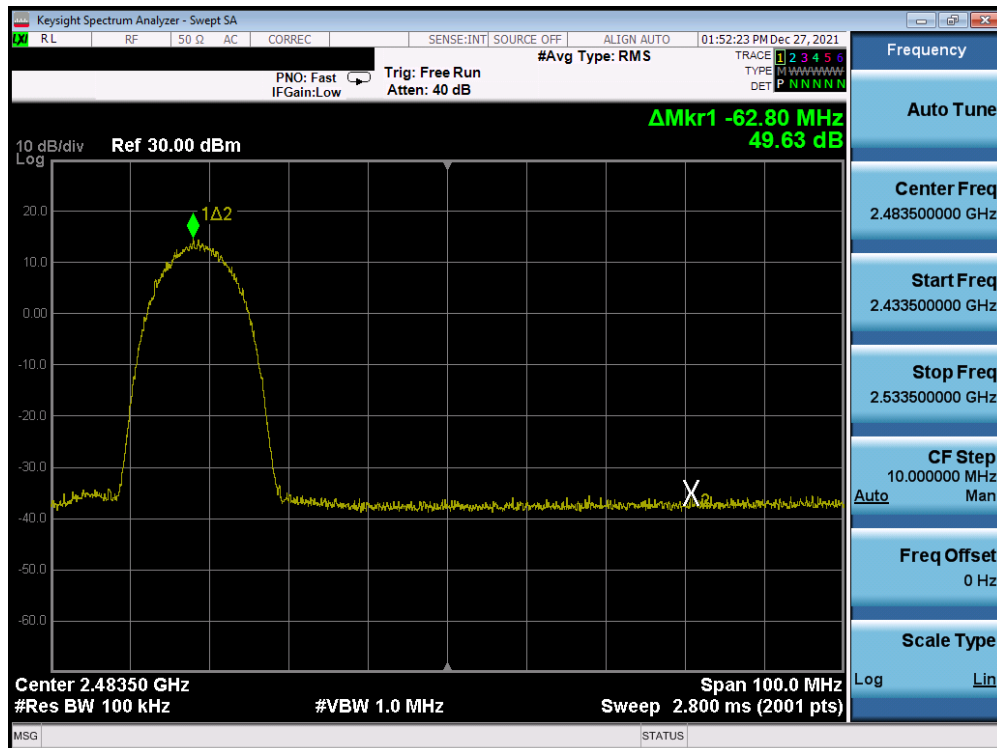
Plot 7-366. Band Edge Plot Antenna 1a (802.11b – Ch. 9) – 11Mbps
