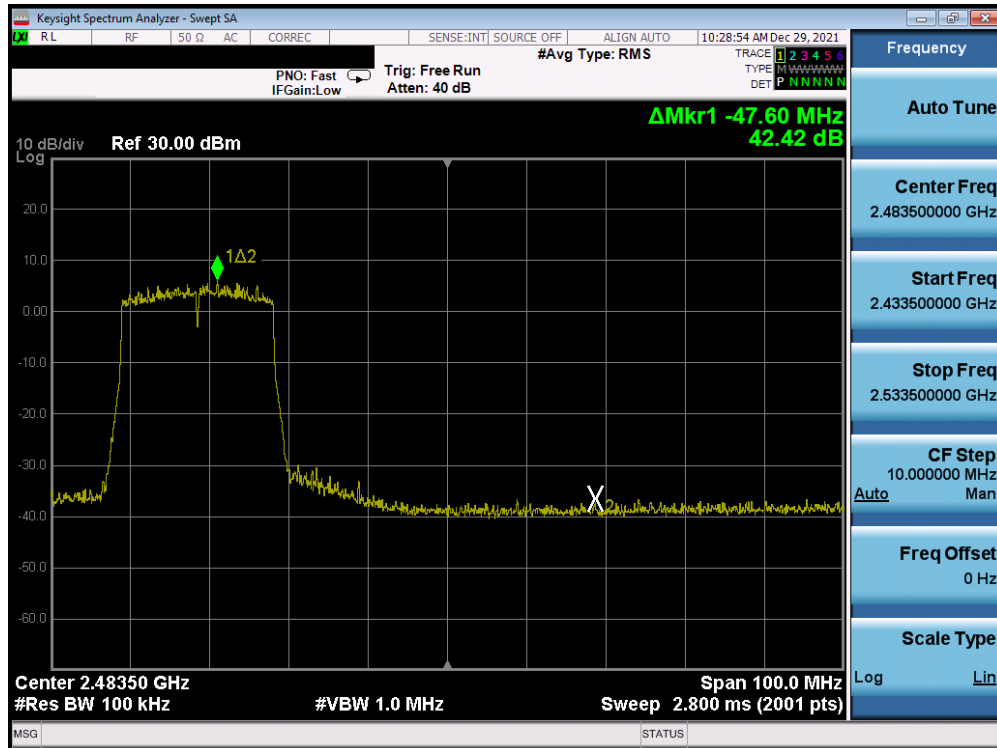
Plot 7-286. Band Edge Plot Antenna 3a (802.11ax (SU - 2.4GHz) – Ch. 9) – MCS5
