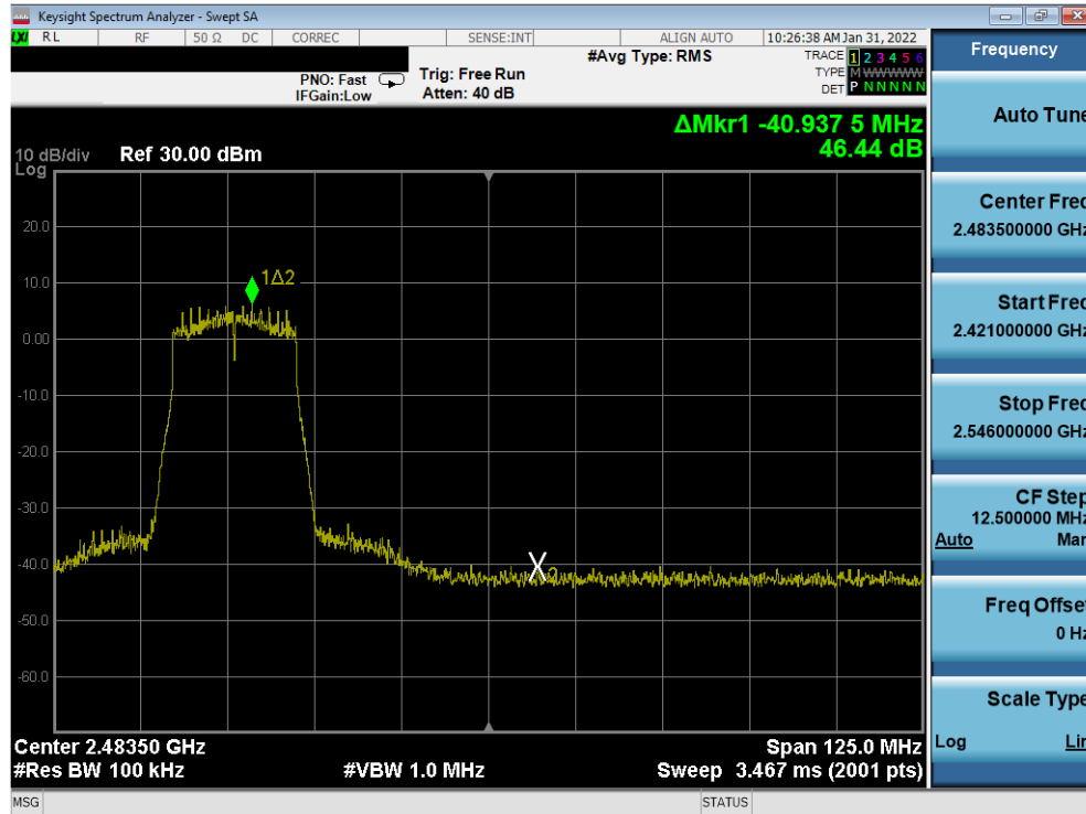
Plot 7-344. Band Edge Plot Antenna 1a (802.11n (2.4GHz) - Ch. 8) - MCS3
