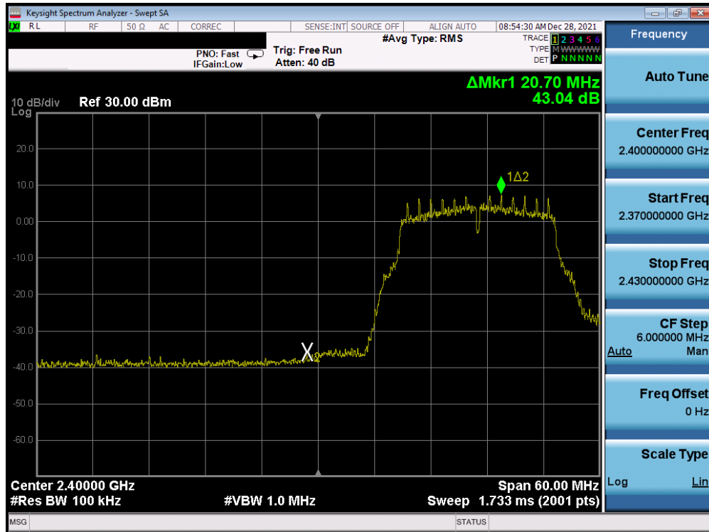
Plot 7-291. Band Edge Plot Antenna 1a (802.11g- Ch. 2) – 6Mbps
