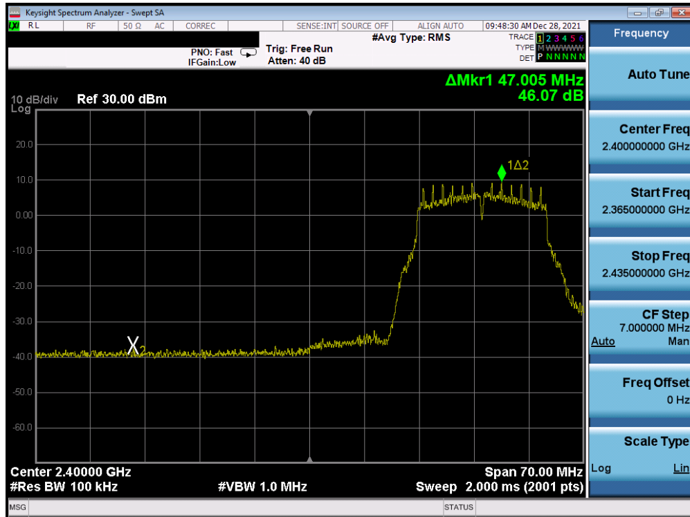
Plot 7-326. Band Edge Plot Antenna 1a (802.11g- Ch. 3) – 18Mbps
