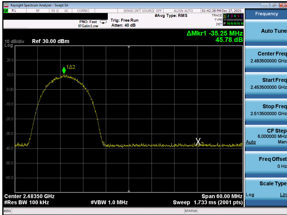
Plot 7-369. Band Edge Plot Antenna 1a (802.11b – Ch. 12) – 11Mbps
