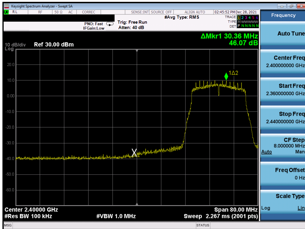
Plot 7-304. Band Edge Plot Antenna 1a (802.11n (2.4GHz) – Ch. 4) – MCS0
