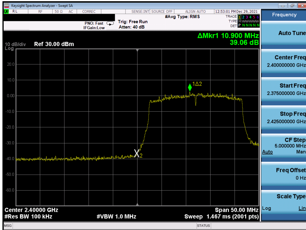
Plot 7-350. Band Edge Plot Antenna 1a (802.11ax (SU - 2.4GHz) – Ch. 1) – MCS3
