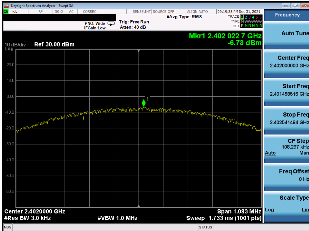
Plot 7-28. Power Spectral Density Plot Antenna 3A (Bluetooth (LE), 1Mbps, iPA – Ch. 0)
