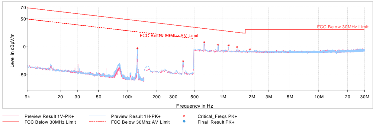
Plot 6-3. Radiated Spurious Emissions 9kHz-30MHz (Charging Rate 10C, with AC/DC Adapter)
