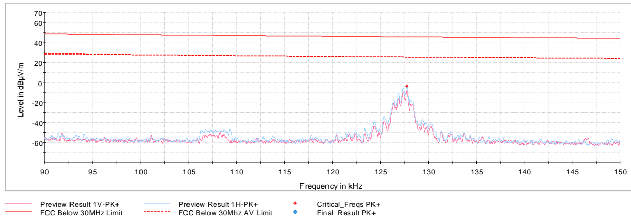
Plot 6-2. Radiated Restricted Lower Band Edge Peak Measurement (Charging Rate 10C)
