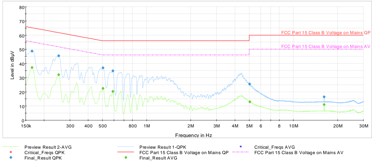
Plot 6-5. AC Line Conducted Plot (L1, Charging Rate 10C, with AC/DC Adapter)
