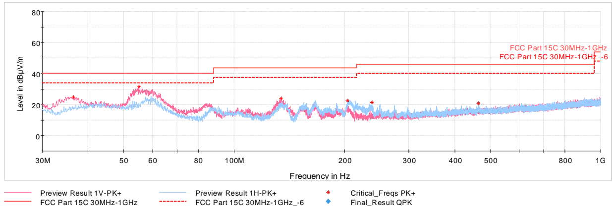
Plot 6-4. Radiated Spurious Emissions 30MHz-1GHz (Charging Rate 10C, with AC/DC Adapter)
