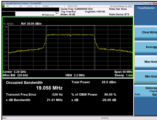
Plot 7-26. 26dB BW & 99% OBW Antenna WF8 (20MHz BW 802.11ax(SU) – Ch. 56, MCS3)
