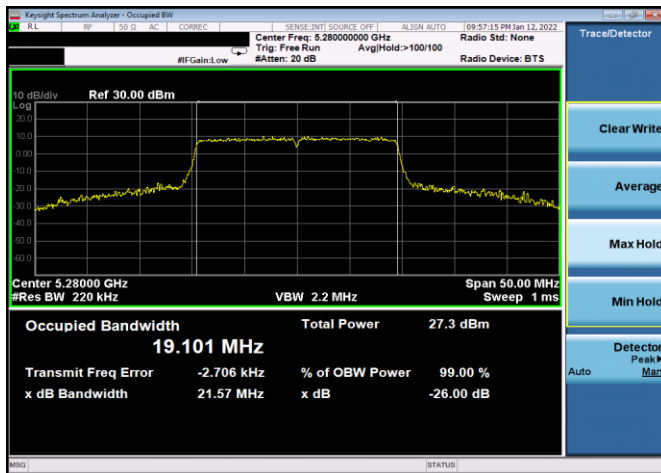
Plot 7-44. 26dB BW & 99% OBW Antenna WF8 (20MHz BW 802.11ax(SU) – Ch. 56, MCS5)
