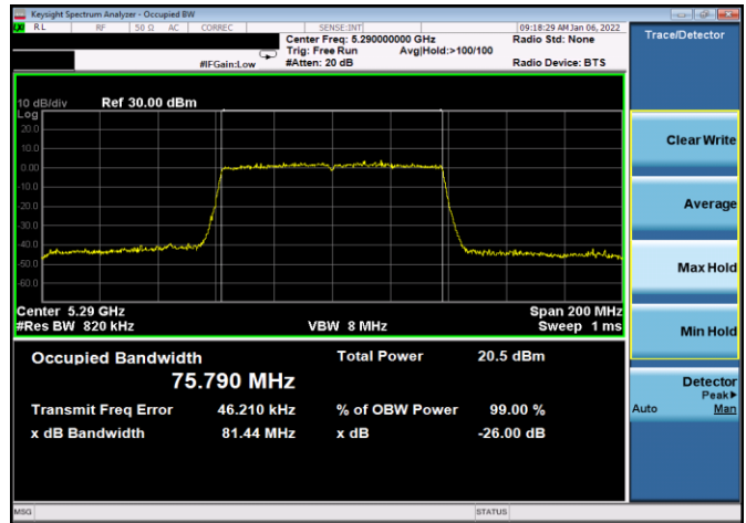
Plot 7-47. 26dB BW & 99% OBW Antenna WF8 (80MHz BW 802.11ac – Ch. 58, MCS5)
