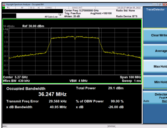
Plot 7-27. 26dB BW & 99% OBW Antenna WF8 (40MHz BW 802.11n – Ch. 54, MCS3)
