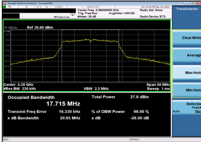
Plot 7-43. 26dB BW & 99% OBW Antenna WF8 (20MHz BW 802.11n – Ch. 56, MCS5)
