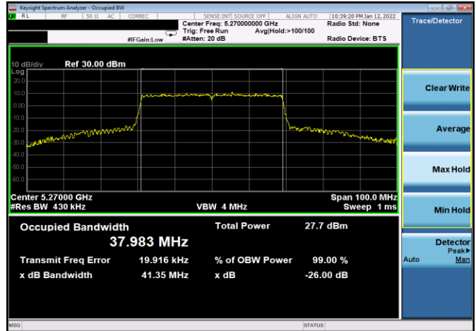
Plot 7-46. 26dB BW & 99% OBW Antenna WF8 (40MHz BW 802.11ax(SU) – Ch. 54, MCS5)
