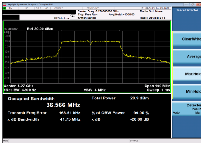
Plot 7-45. 26dB BW & 99% OBW Antenna WF8 (40MHz BW 802.11n – Ch. 54, MCS5)
