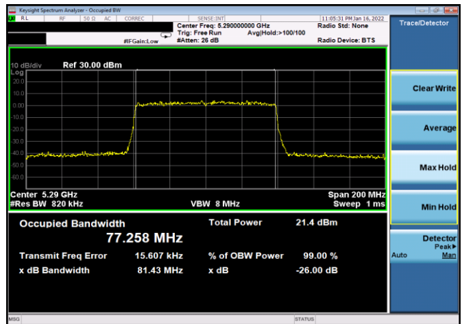
Plot 7-48. 26dB BW & 99% OBW Antenna WF8 (80MHz BW 802.11ax(SU) – Ch. 58, MCS5)
