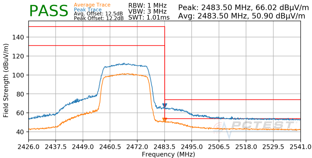
Plot 7-651. Radiated Restricted Upper Band Edge Measurement Antenna WF7b
