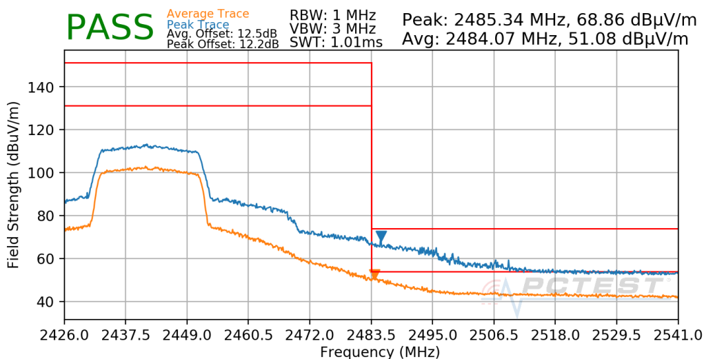
Plot 7-636. Radiated Restricted Upper Band Edge Measurement Antenna WF7b
