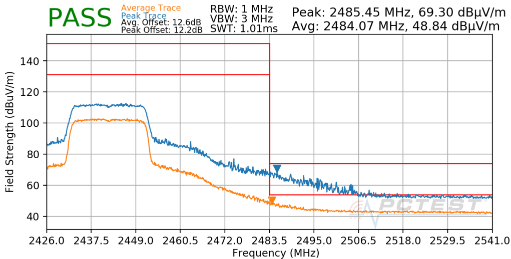
Plot 7-637. Radiated Restricted Upper Band Edge Measurement Antenna WF7b
