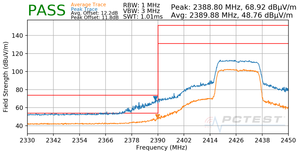
Plot 7-625. Radiated Restricted Lower Band Edge Measurement Antenna WF7b
