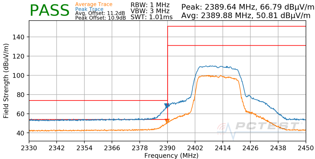
Plot 7-654. Radiated Restricted Lower Band Edge Measurement CDD
