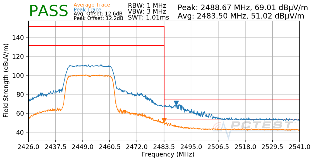
Plot 7-643. Radiated Restricted Upper Band Edge Measurement Antenna WF7b
