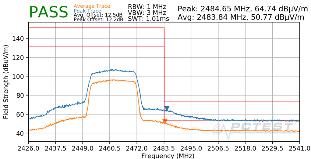
Plot 7-648. Radiated Restricted Upper Band Edge Measurement Antenna WF7b
