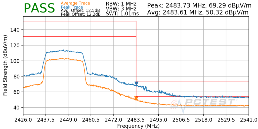
Plot 7-639. Radiated Restricted Upper Band Edge Measurement Antenna WF7b
