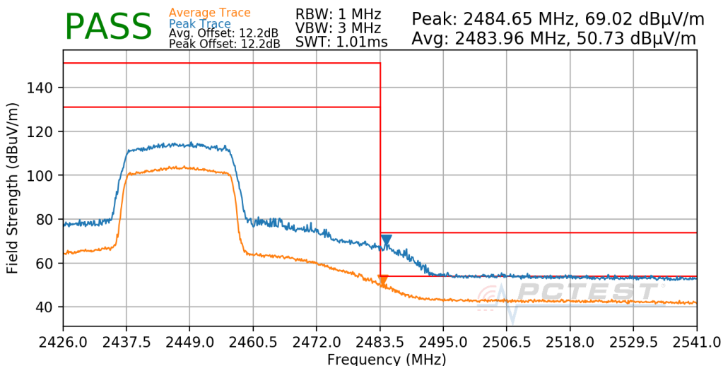
Plot 7-638. Radiated Restricted Upper Band Edge Measurement Antenna WF7b
