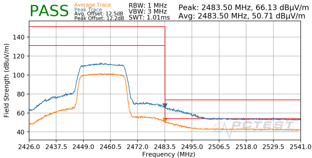
Plot 7-645. Radiated Restricted Upper Band Edge Measurement Antenna WF7b
