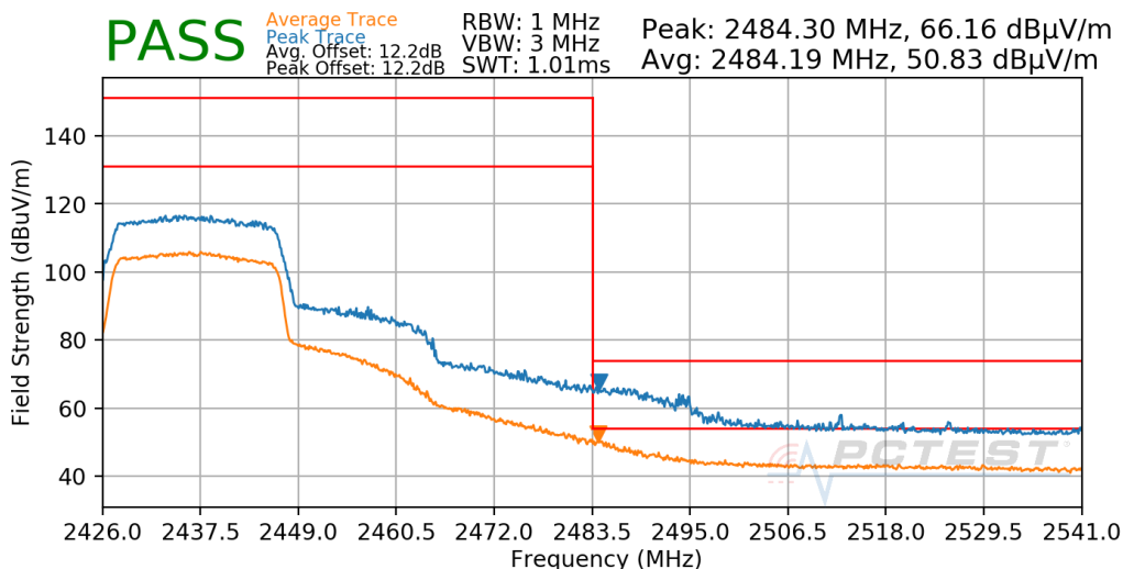
Plot 7-632. Radiated Restricted Upper Band Edge Measurement Antenna WF7b
