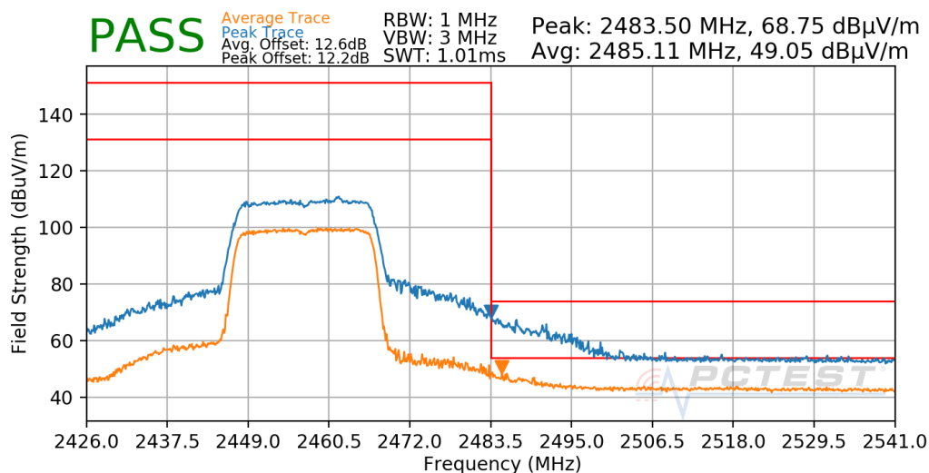
Plot 7-646. Radiated Restricted Upper Band Edge Measurement Antenna WF7b
