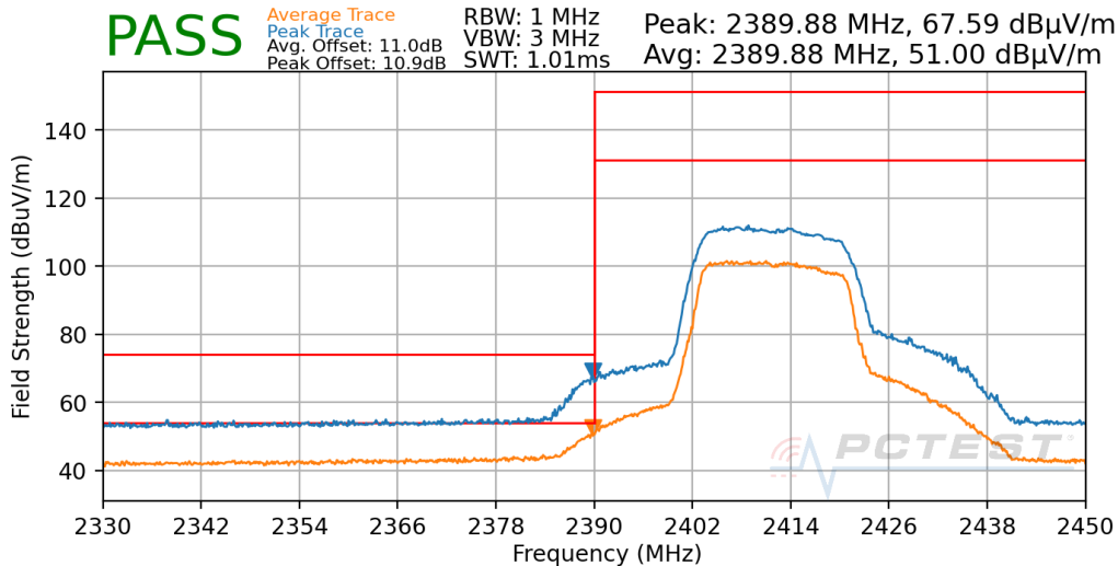
Plot 7-653. Radiated Restricted Lower Band Edge Measurement CDD
