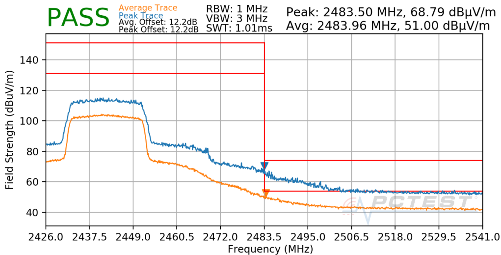
Plot 7-635. Radiated Restricted Upper Band Edge Measurement Antenna WF7b
