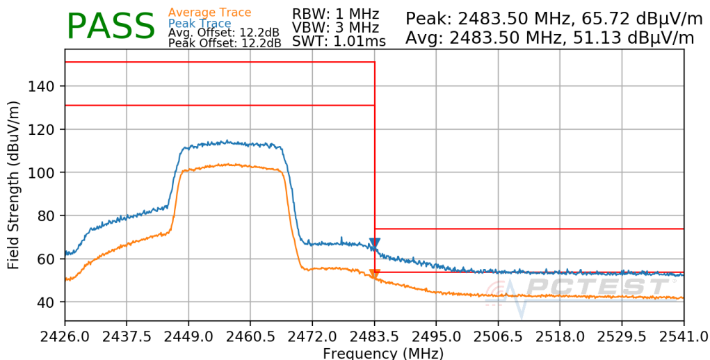
Plot 7-644. Radiated Restricted Upper Band Edge Measurement Antenna WF7b
