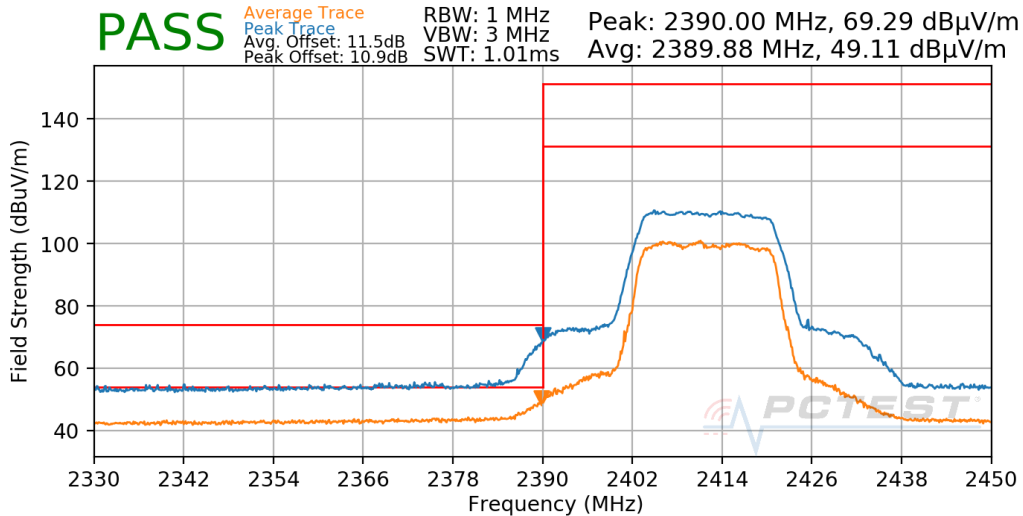
Plot 7-655. Radiated Restricted Lower Band Edge Measurement CDD
