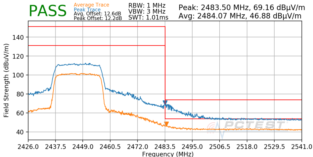
Plot 7-640. Radiated Restricted Upper Band Edge Measurement Antenna WF7b
