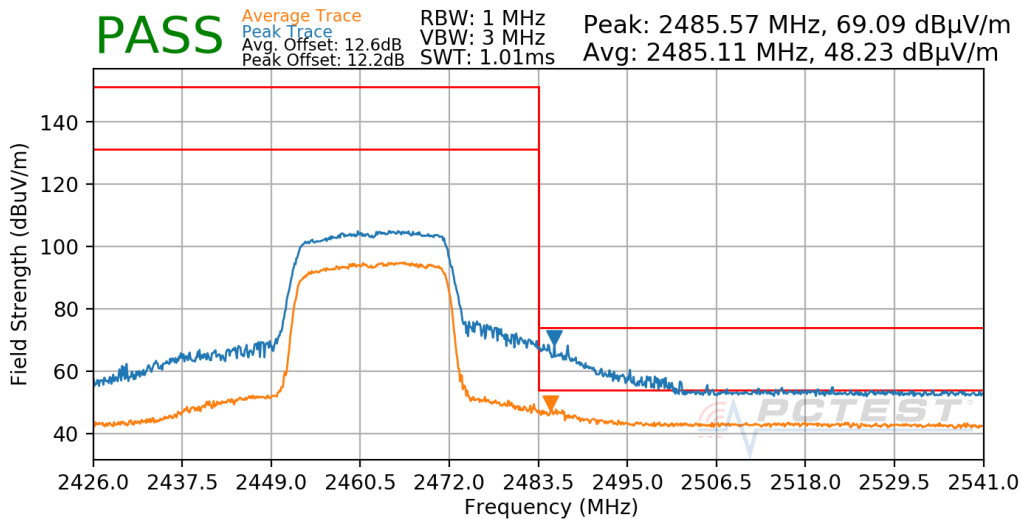
Plot 7-649. Radiated Restricted Upper Band Edge Measurement Antenna WF7b
