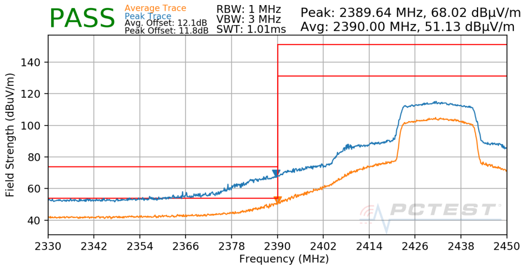
Plot 7-627. Radiated Restricted Lower Band Edge Measurement Antenna WF7b
