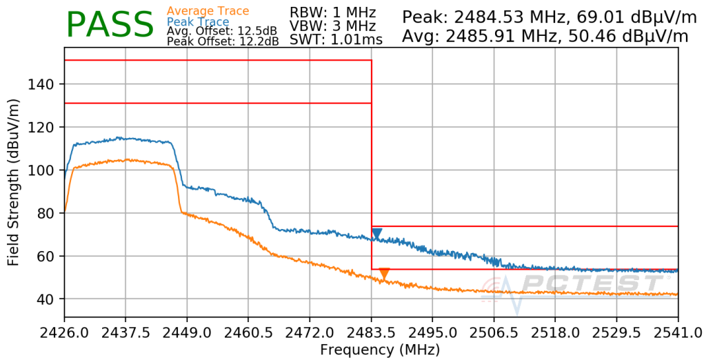
Plot 7-633. Radiated Restricted Upper Band Edge Measurement Antenna WF7b
