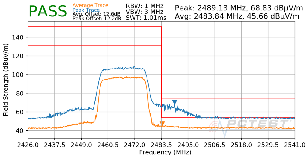
Plot 7-652. Radiated Restricted Upper Band Edge Measurement Antenna WF7b
