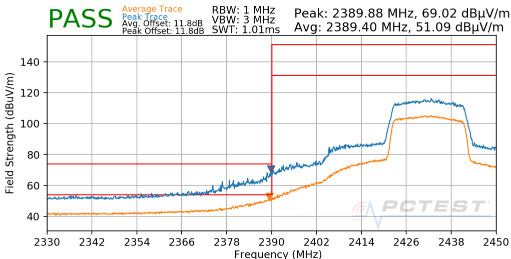
Plot 7-626. Radiated Restricted Lower Band Edge Measurement Antenna WF7b
