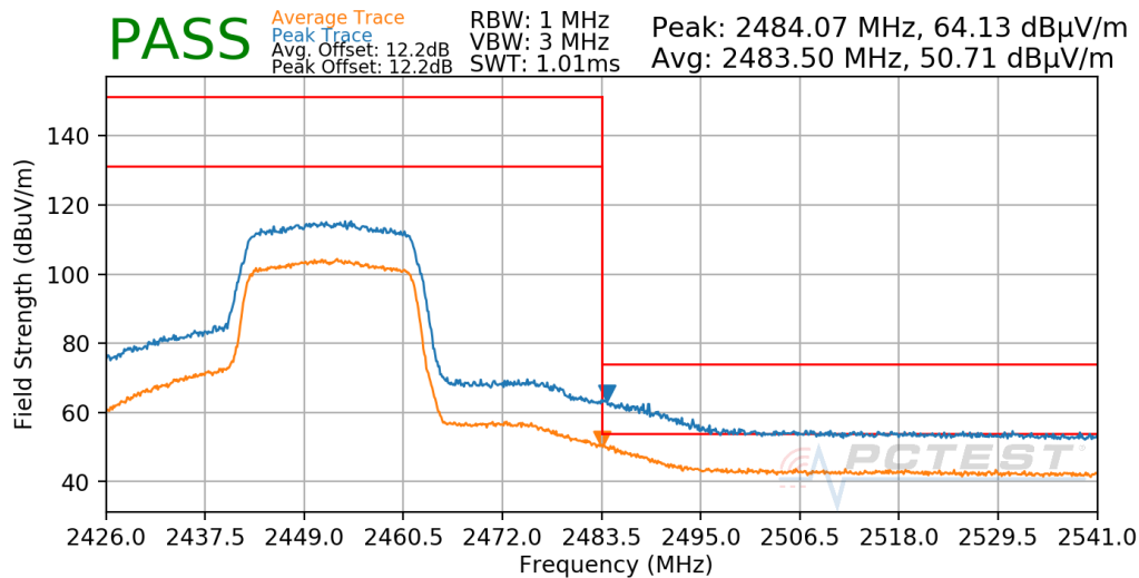
Plot 7-641. Radiated Restricted Upper Band Edge Measurement Antenna WF7b
