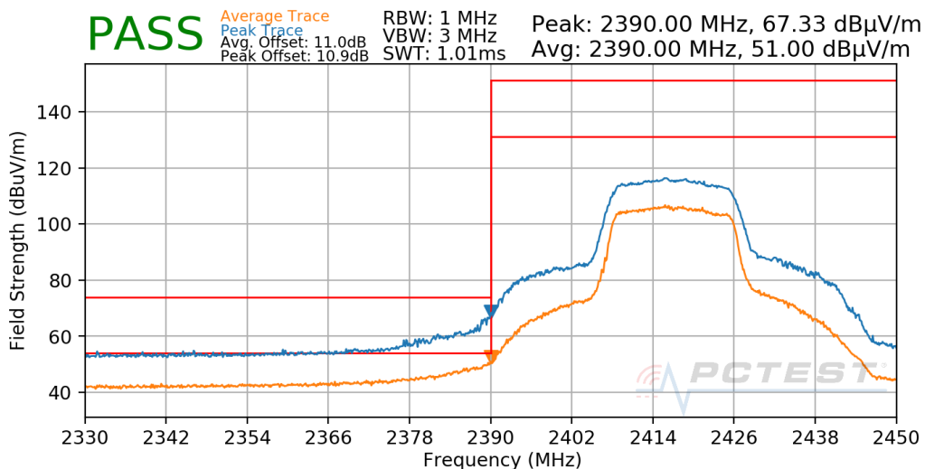
Plot 7-656. Radiated Restricted Lower Band Edge Measurement CDD
