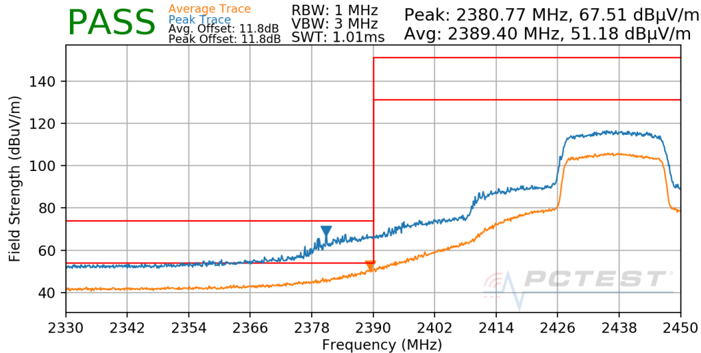
Plot 7-629. Radiated Restricted Lower Band Edge Measurement Antenna WF7b
