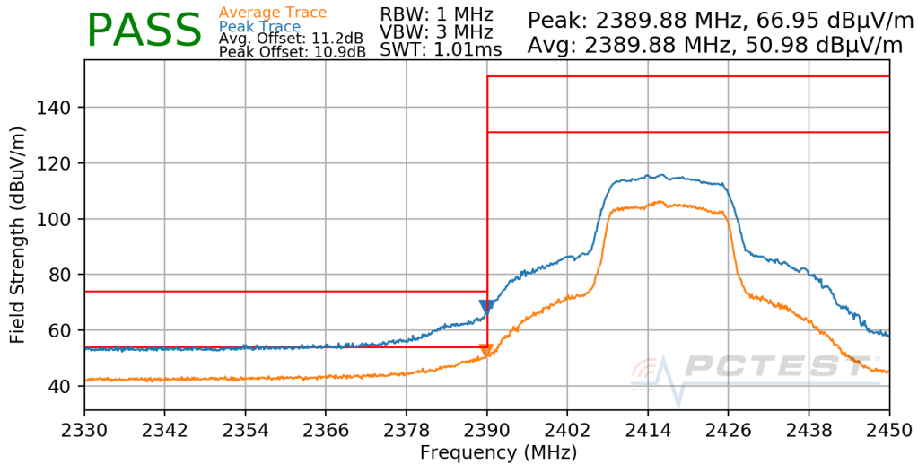
Plot 7-657. Radiated Restricted Lower Band Edge Measurement CDD
