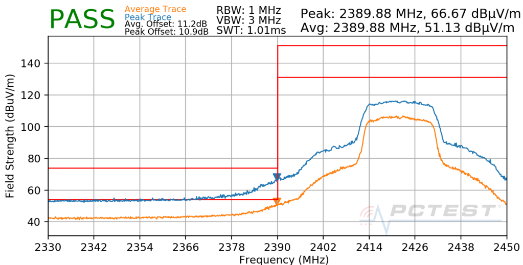
Plot 7-660. Radiated Restricted Lower Band Edge Measurement CDD
