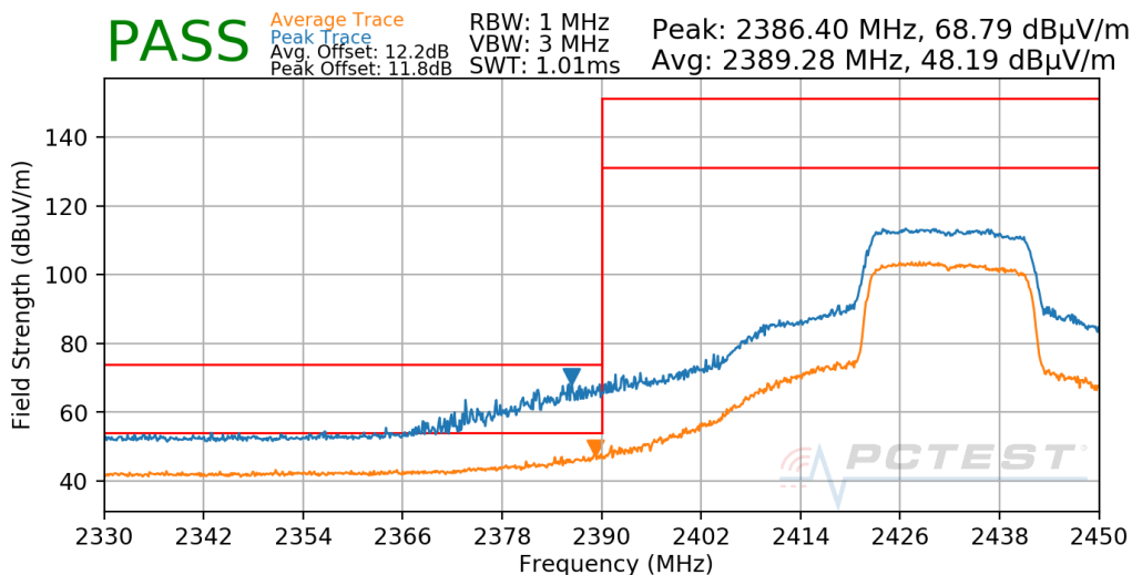
Plot 7-628. Radiated Restricted Lower Band Edge Measurement Antenna WF7b
