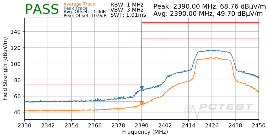
Plot 7-662. Radiated Restricted Lower Band Edge Measurement CDD
