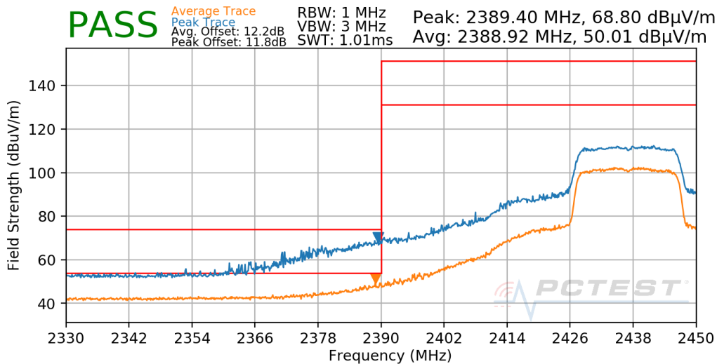
Plot 7-631. Radiated Restricted Lower Band Edge Measurement Antenna WF7b
