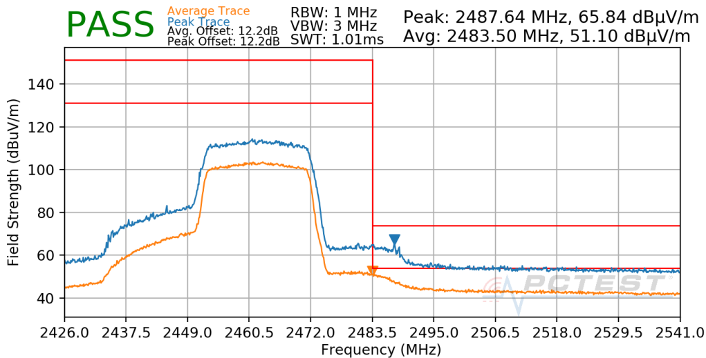
Plot 7-647. Radiated Restricted Upper Band Edge Measurement Antenna WF7b
