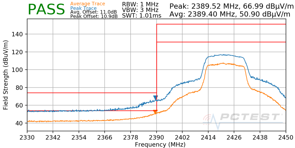
Plot 7-659. Radiated Restricted Lower Band Edge Measurement CDD
