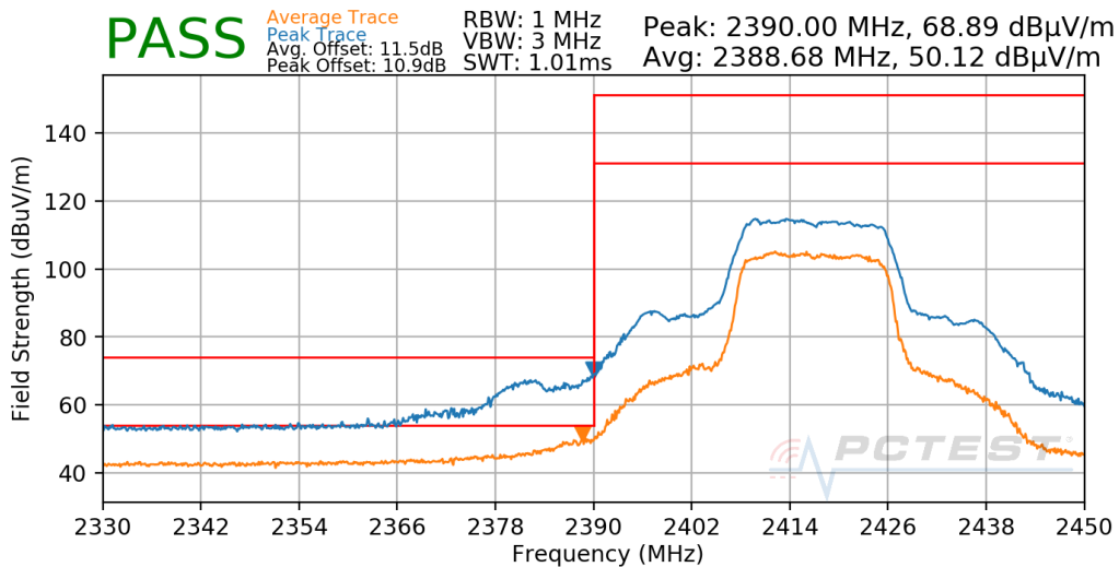
Plot 7-658. Radiated Restricted Lower Band Edge Measurement CDD
