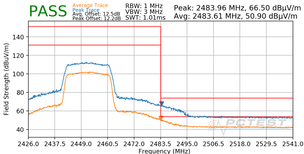
Plot 7-642. Radiated Restricted Upper Band Edge Measurement Antenna WF7b
