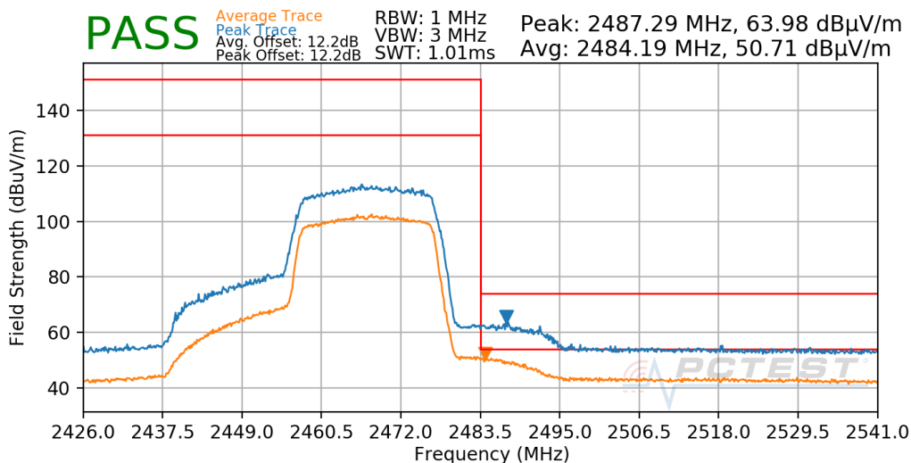
Plot 7-650. Radiated Restricted Upper Band Edge Measurement Antenna WF7b
