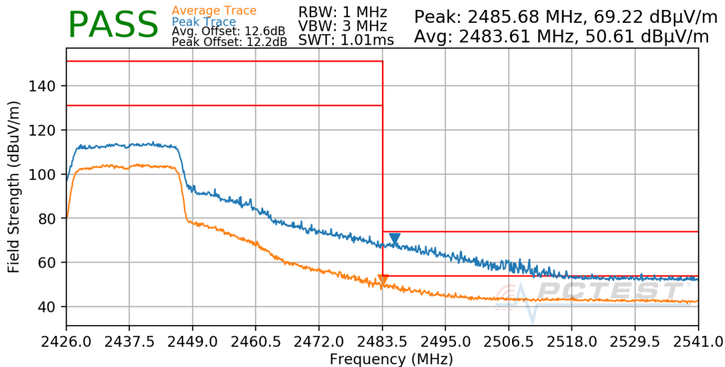
Plot 7-634. Radiated Restricted Upper Band Edge Measurement Antenna WF7b
