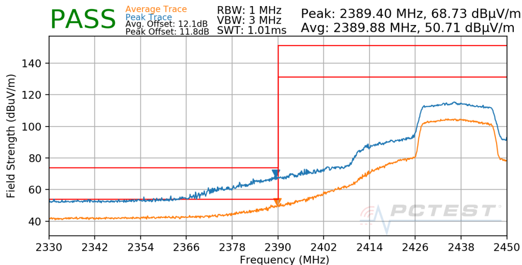
Plot 7-630. Radiated Restricted Lower Band Edge Measurement Antenna WF7b
