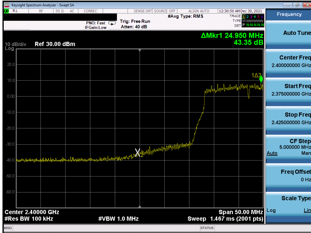
Plot 7-364. Band Edge Plot Antenna WF7b (802.11n (2.4GHz) – Ch. 3) – MCS3
