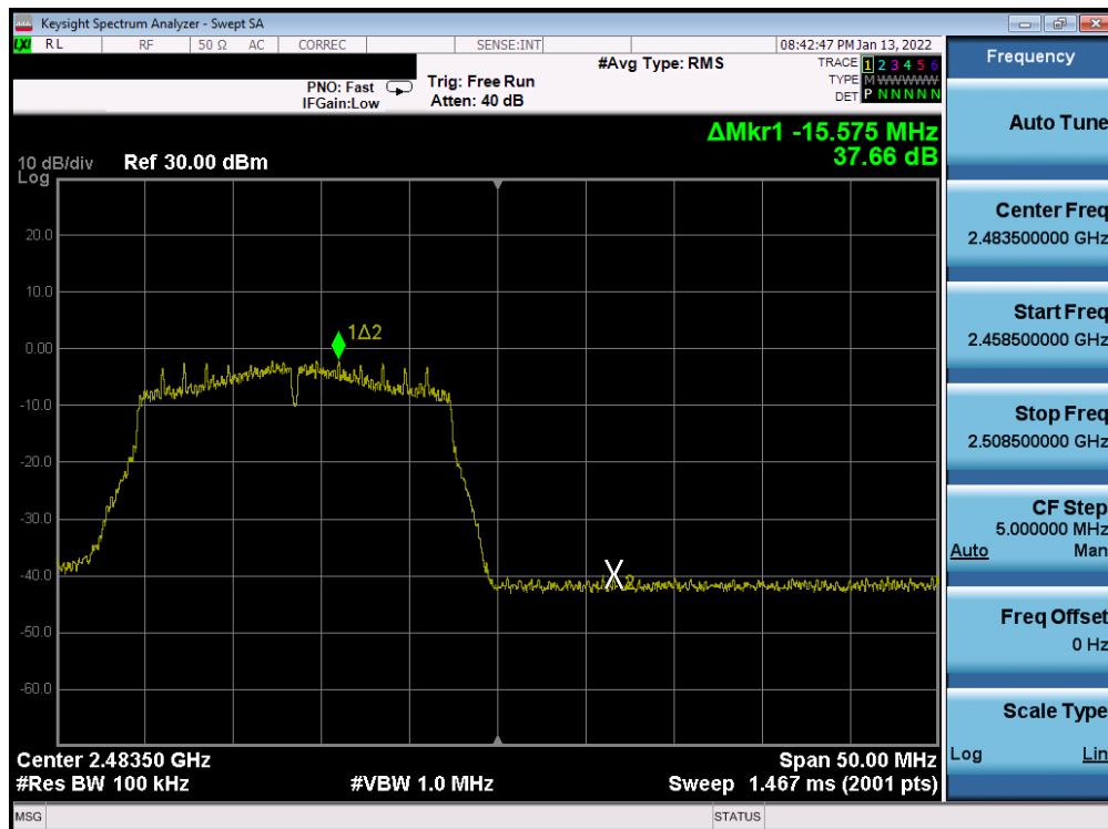
Plot 7-334. Band Edge Plot Antenna WF7b (802.11n (2.4GHz) – Ch. 13) – MCS0
