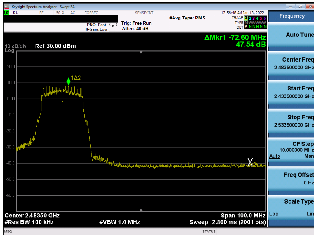
Plot 7-316. Band Edge Plot Antenna WF7b (802.11g - Ch. 9) - 6Mbps
