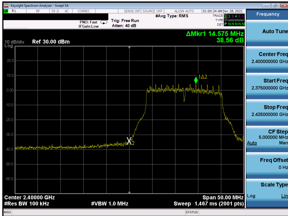
Plot 7-398. Band Edge Plot Antenna WF7b (802.11g – Ch. 1) – 36Mbps
