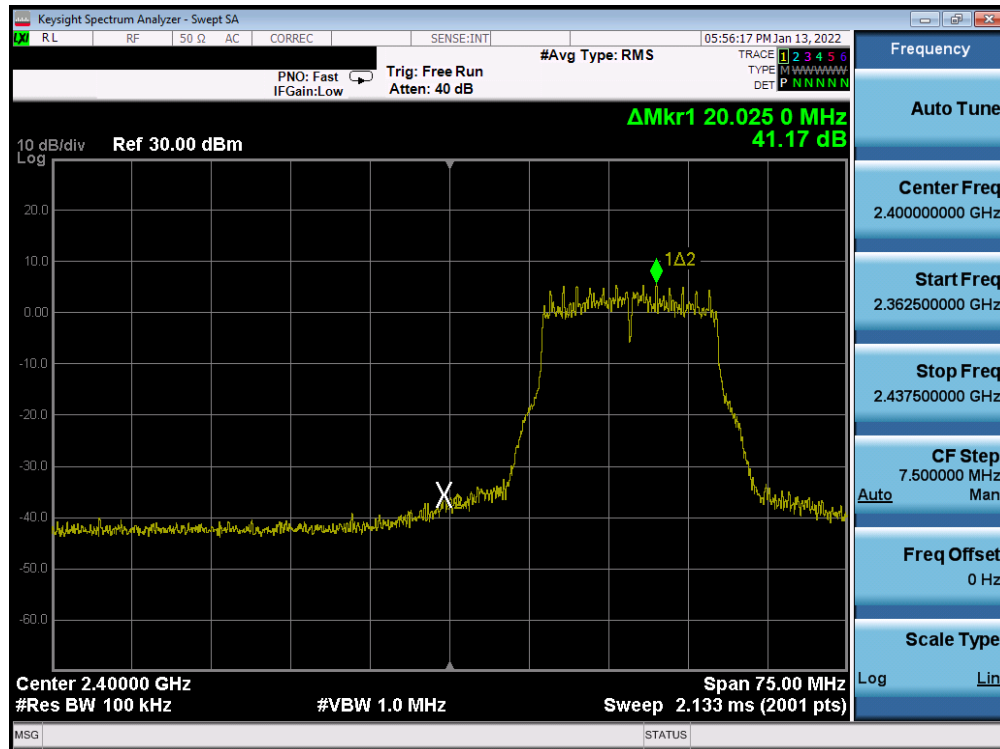
Plot 7-399. Band Edge Plot Antenna WF7b (802.11g – Ch. 2) – 36Mbps
