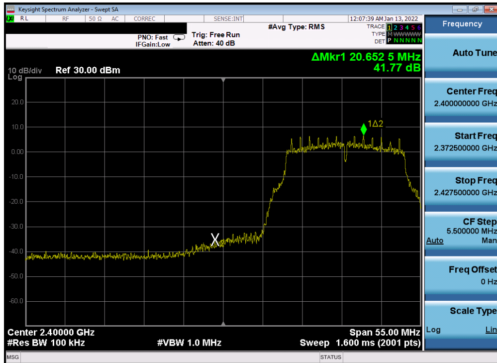
Plot 7-308. Band Edge Plot Antenna WF7b (802.11g - Ch. 2) - 6Mbps
