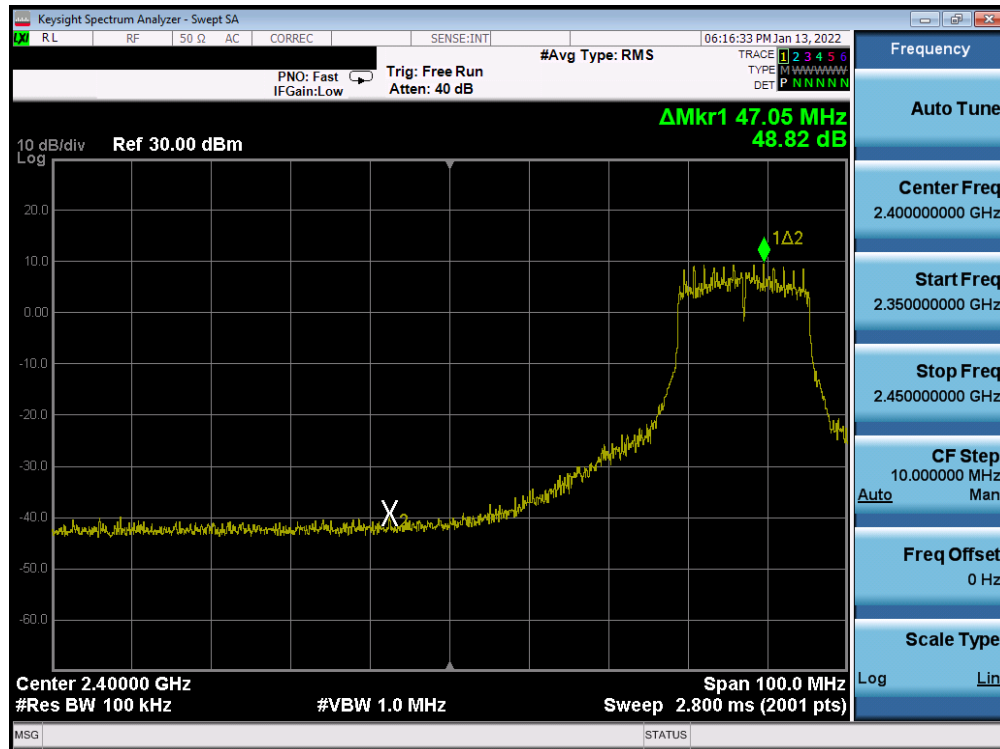
Plot 7-403. Band Edge Plot Antenna WF7b (802.11g - Ch. 6 (low)) - 36Mbps
