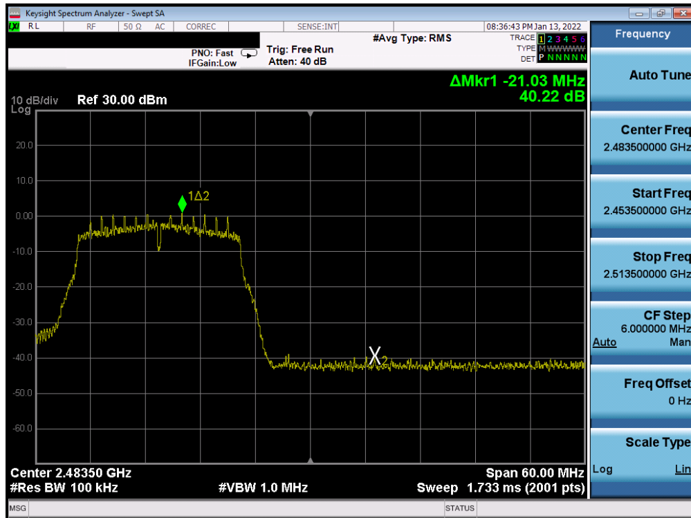
Plot 7-333. Band Edge Plot Antenna WF7b (802.11n (2.4GHz) – Ch. 12) – MCS0
