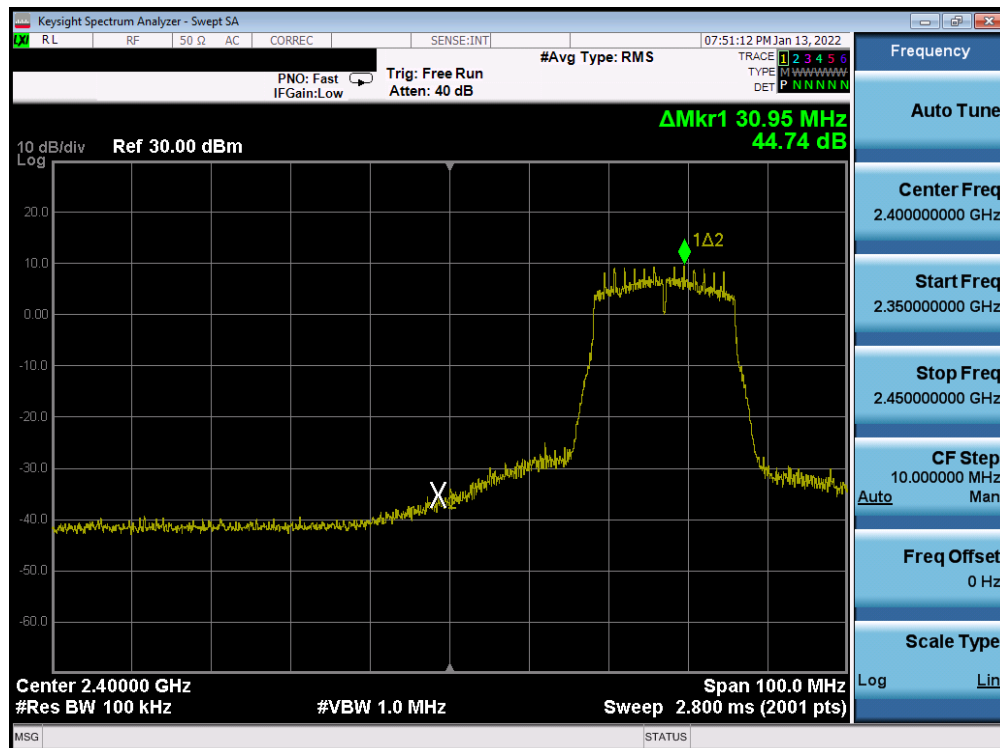
Plot 7-324. Band Edge Plot Antenna WF7b (802.11n (2.4GHz) – Ch. 4) – MCS0
