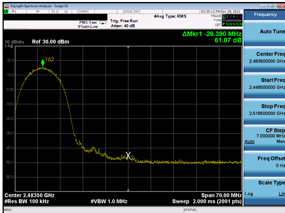
Plot 7-394. Band Edge Plot Antenna WF7b (802.11b – Ch. 10) – 11Mbps
