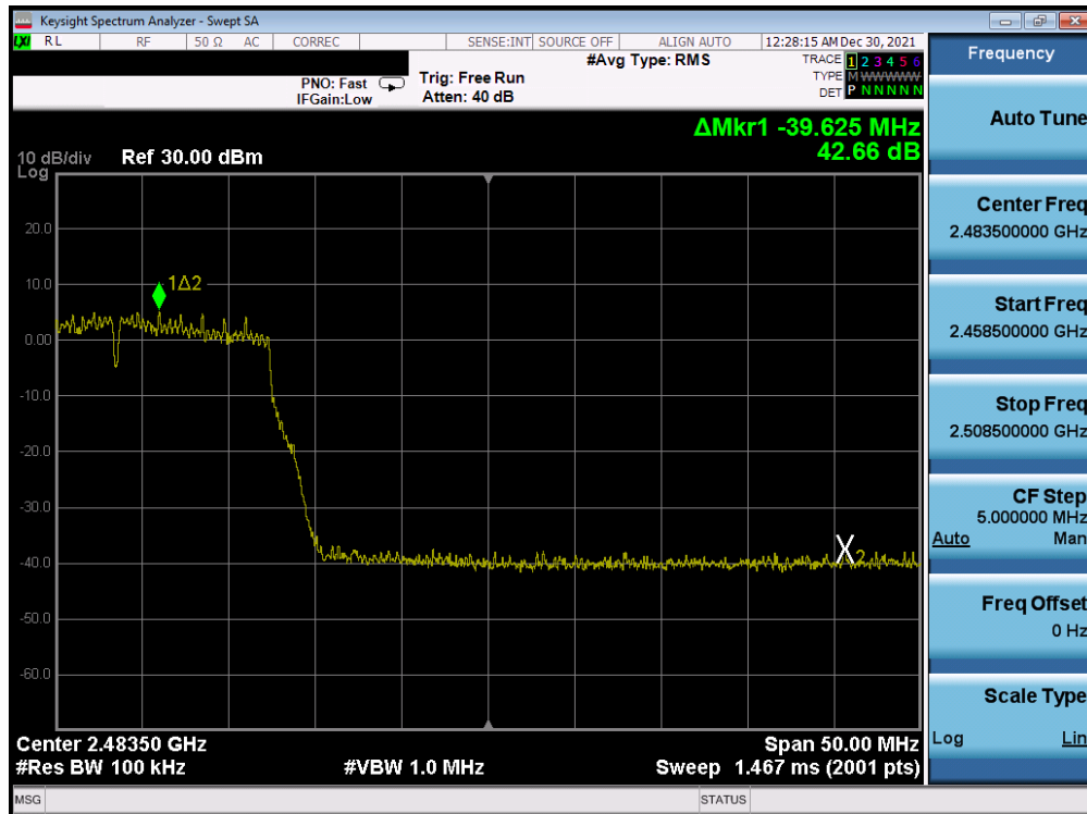
Plot 7-373. Band Edge Plot Antenna WF7b (802.11n (2.4GHz) – Ch. 11) – MCS3
