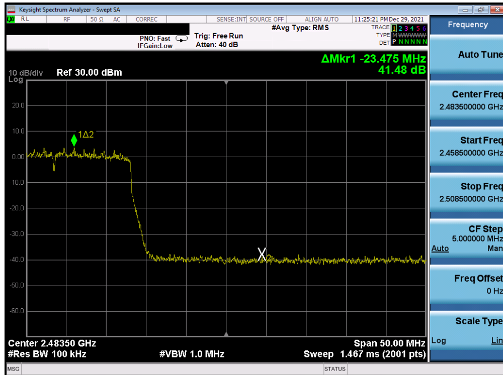
Plot 7-305. Band Edge Plot Antenna WF8 (802.11ax (SU - 2.4GHz) – Ch. 11) – MCS5
