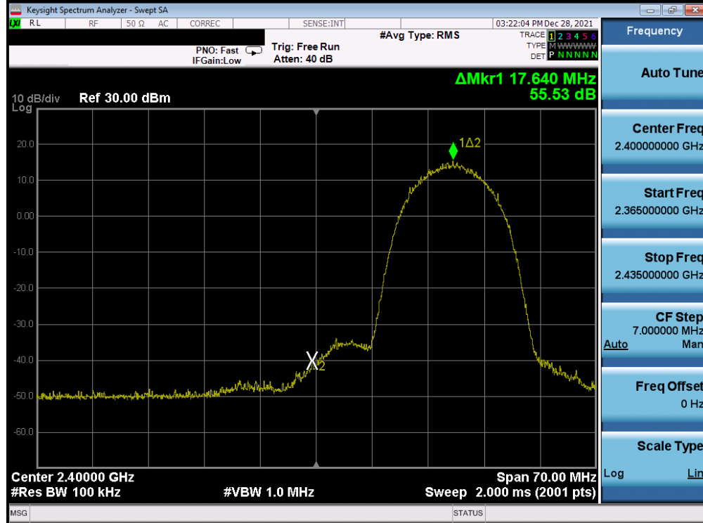
Plot 7-390. Band Edge Plot Antenna WF7b (802.11b – Ch. 2) – 11Mbps
