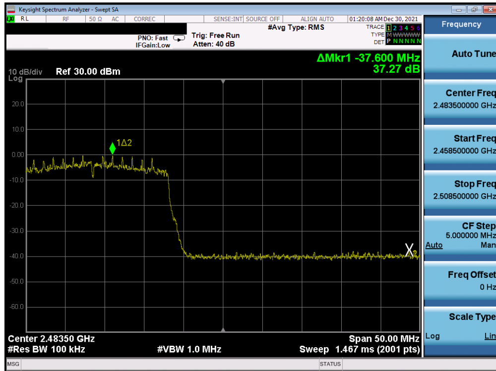
Plot 7-347. Band Edge Plot Antenna WF7b (802.11ax (SU - 2.4GHz) – Ch. 12) – MCS0
