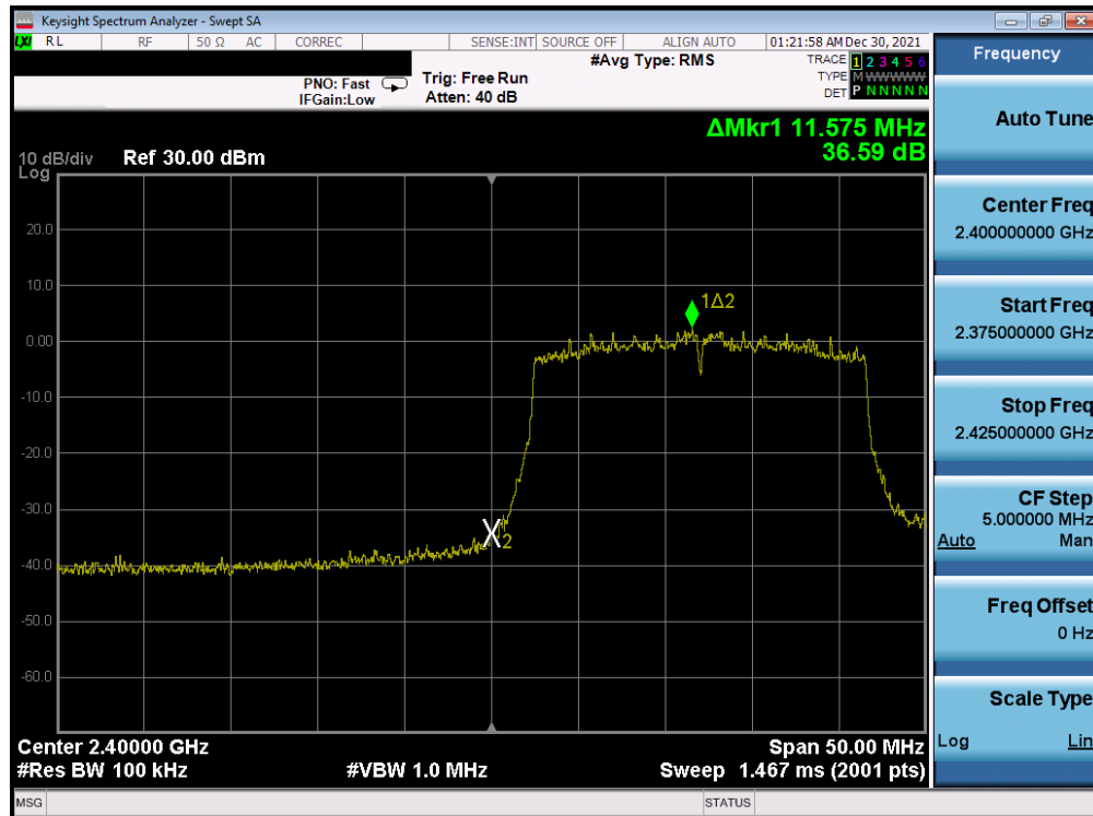
Plot 7-376. Band Edge Plot Antenna WF7b (802.11ax (SU - 2.4GHz) – Ch. 1) – MCS3
