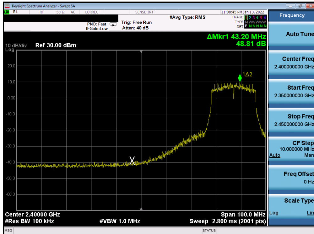
Plot 7-367. Band Edge Plot Antenna WF7b (802.11n (2.4GHz) – Ch. 6 (low)) – MCS3
