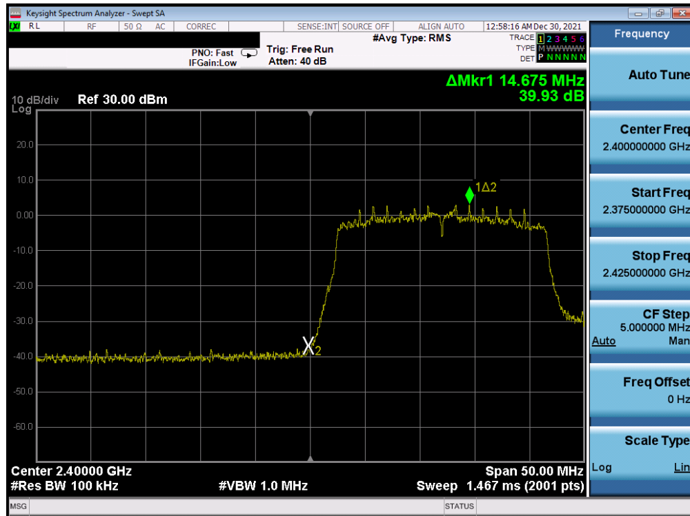
Plot 7-335. Band Edge Plot Antenna WF7b (802.11ax (SU - 2.4GHz) – Ch. 1) – MCS0
