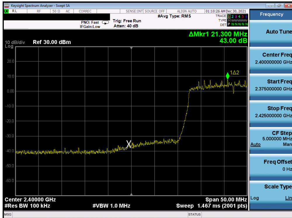
Plot 7-337. Band Edge Plot Antenna WF7b (802.11ax (SU - 2.4GHz) - Ch. 3) - MCS0
