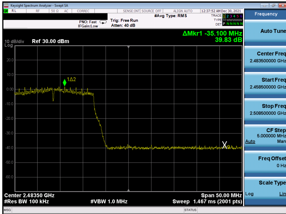
Plot 7-374. Band Edge Plot Antenna WF7b (802.11n (2.4GHz) – Ch. 12) – MCS3
