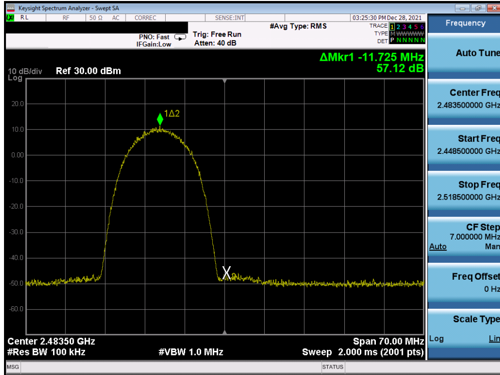
Plot 7-397. Band Edge Plot Antenna WF7b (802.11b – Ch. 13) – 11Mbps
