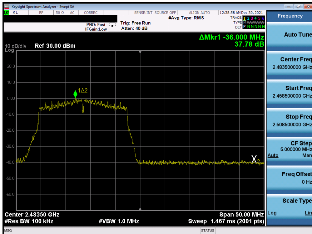
Plot 7-375. Band Edge Plot Antenna WF7b (802.11n (2.4GHz) – Ch. 13) – MCS3
