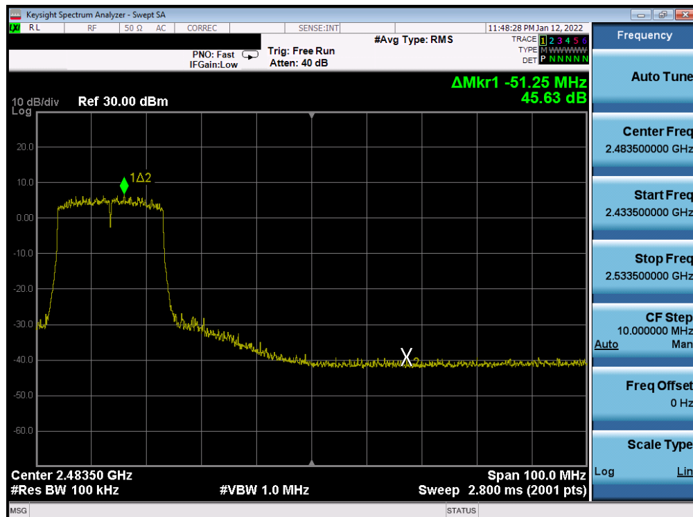
Plot 7-302. Band Edge Plot Antenna WF8 (802.11ax (SU - 2.4GHz) – Ch. 8) – MCS5
