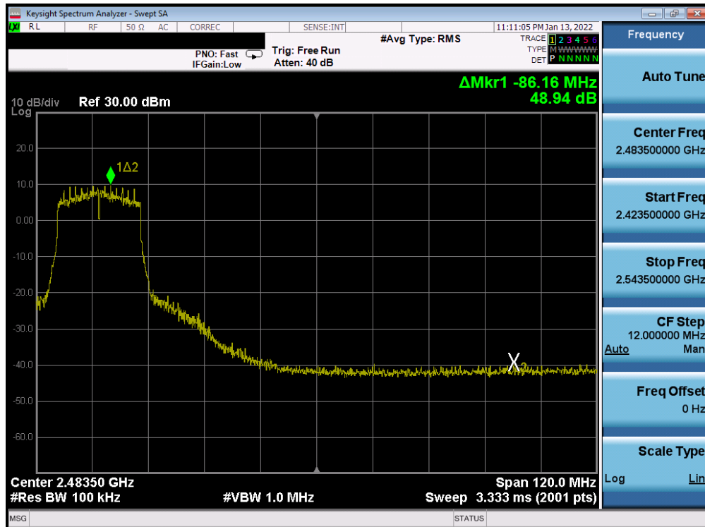
Plot 7-368. Band Edge Plot Antenna WF7b (802.11n (2.4GHz) - Ch. 6 (high)) - MCS3
