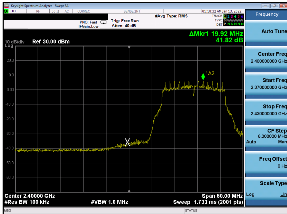
Plot 7-349. Band Edge Plot Antenna WF7b (802.11g – Ch. 2) – 18Mbps
