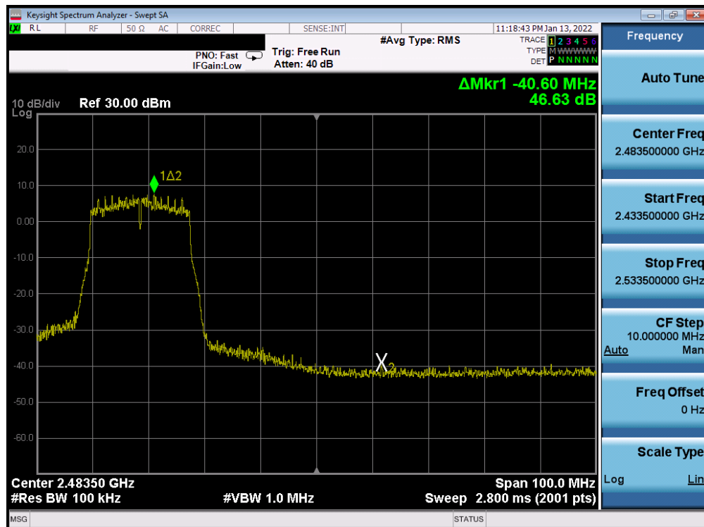
Plot 7-371. Band Edge Plot Antenna WF7b (802.11n (2.4GHz) – Ch. 9) – MCS3
