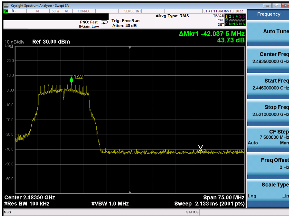
Plot 7-359. Band Edge Plot Antenna WF7b (802.11g - Ch. 11) - 18Mbps
