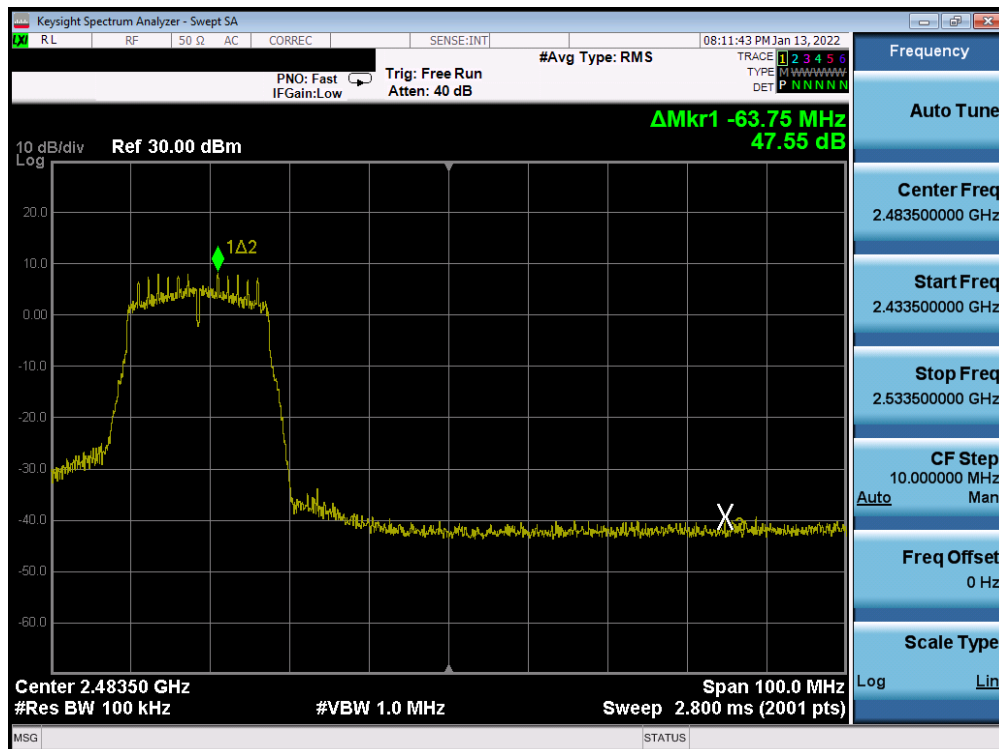
Plot 7-330. Band Edge Plot Antenna WF7b (802.11n (2.4GHz) – Ch. 9) – MCS0
