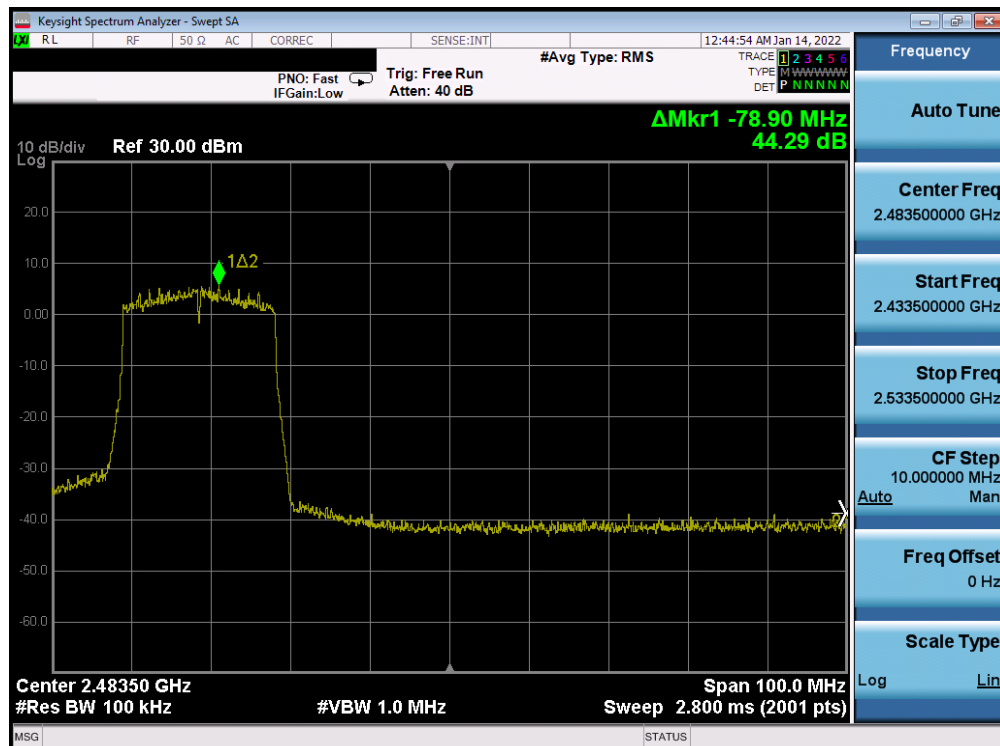
Plot 7-385. Band Edge Plot Antenna WF7b (802.11ax (SU - 2.4GHz) - Ch. 9) - MCS3
