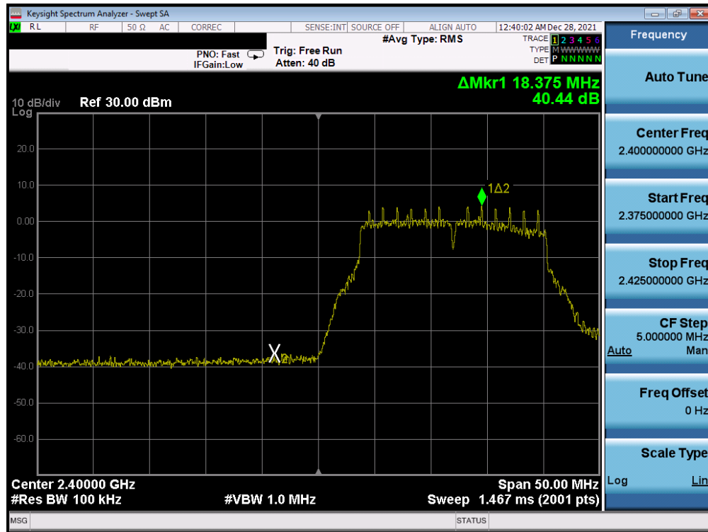
Plot 7-348. Band Edge Plot Antenna WF7b (802.11g – Ch. 1) – 18Mbps
