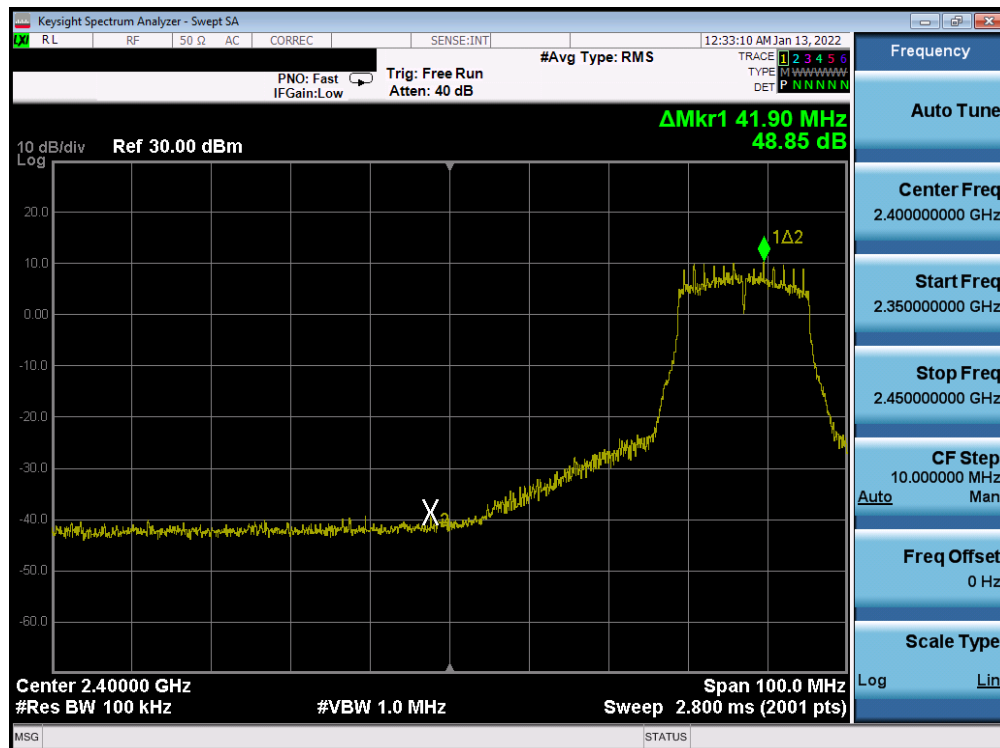
Plot 7-312. Band Edge Plot Antenna WF7b (802.11g – Ch. 6 (low)) – 6Mbps
