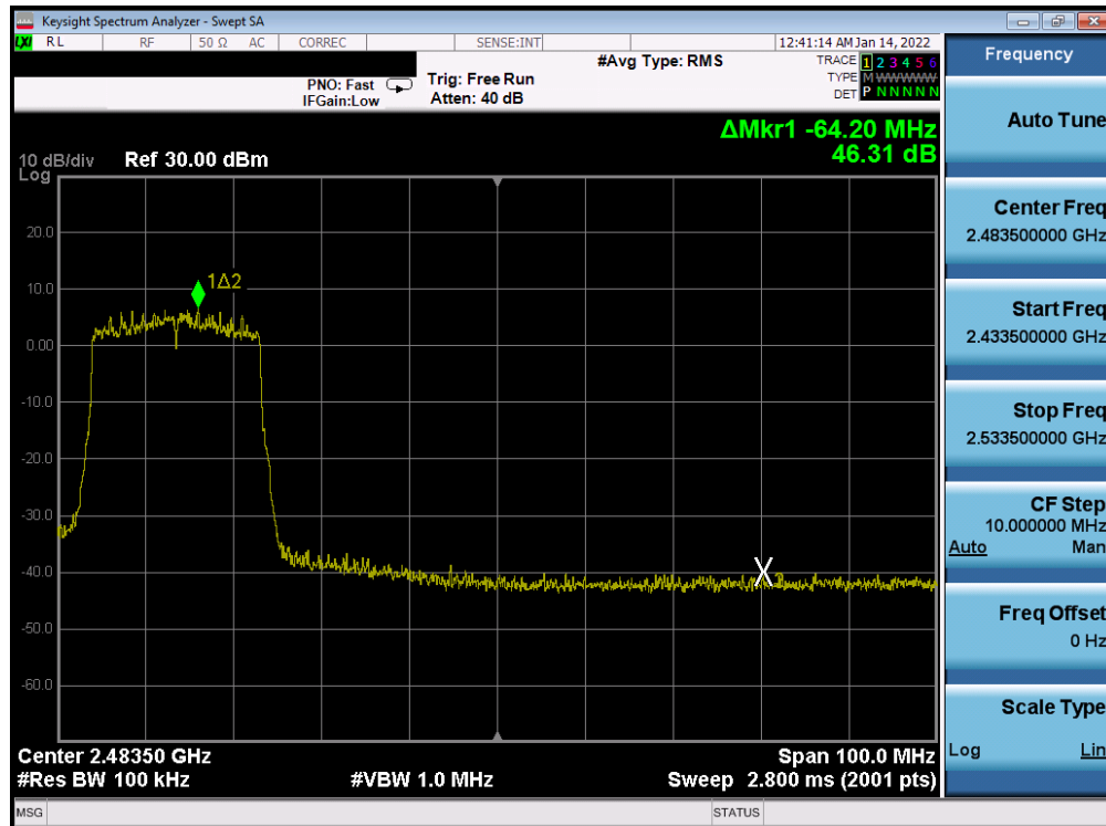
Plot 7-384. Band Edge Plot Antenna WF7b (802.11ax (SU - 2.4GHz) - Ch. 8) - MCS3
