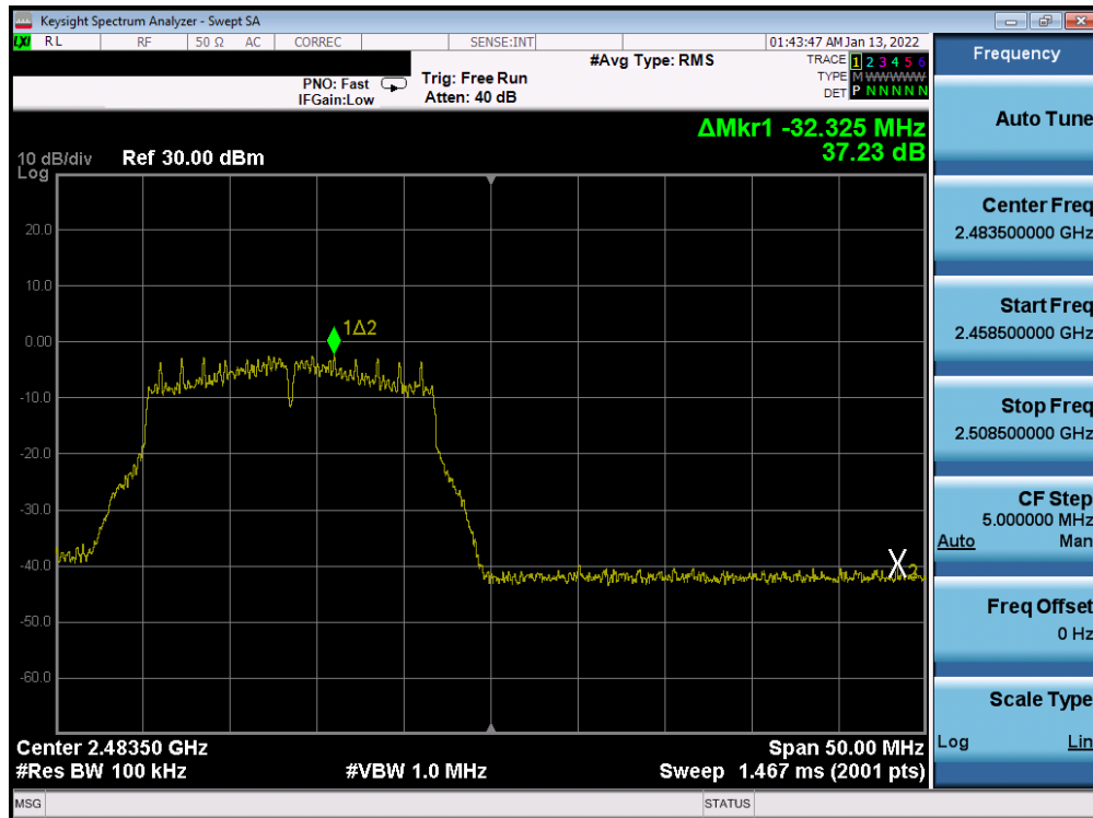
Plot 7-361. Band Edge Plot Antenna WF7b (802.11g - Ch. 13) - 18Mbps
