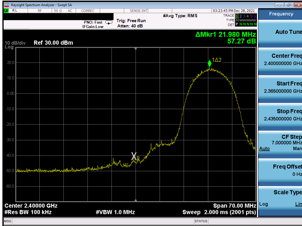
Plot 7-391. Band Edge Plot Antenna WF7b (802.11b – Ch. 3) – 11Mbps
