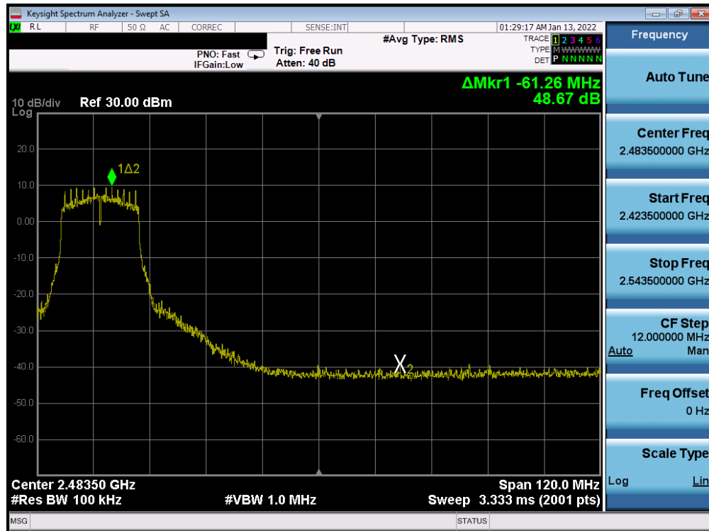
Plot 7-354. Band Edge Plot Antenna WF7b (802.11g – Ch. 6 (high)) – 18Mbps
