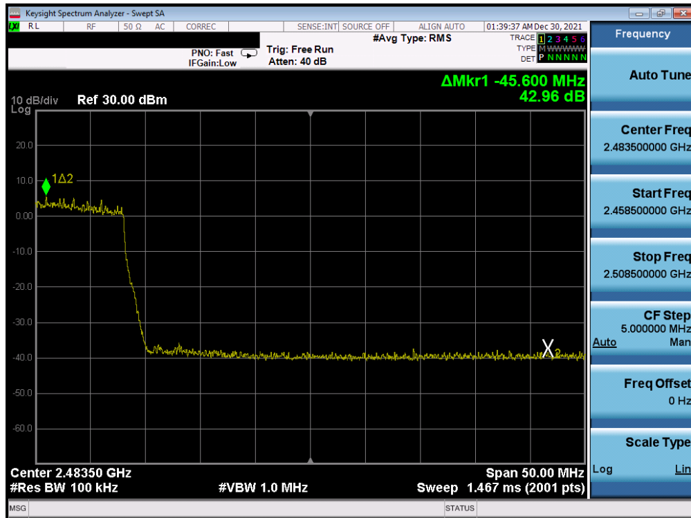
Plot 7-386. Band Edge Plot Antenna WF7b (802.11ax (SU - 2.4GHz) – Ch. 10) – MCS3
