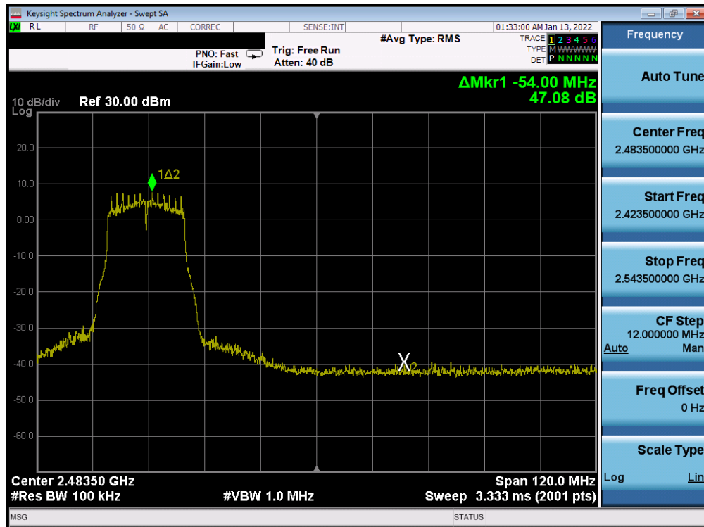
Plot 7-356. Band Edge Plot Antenna WF7b (802.11g - Ch. 8) - 18Mbps
