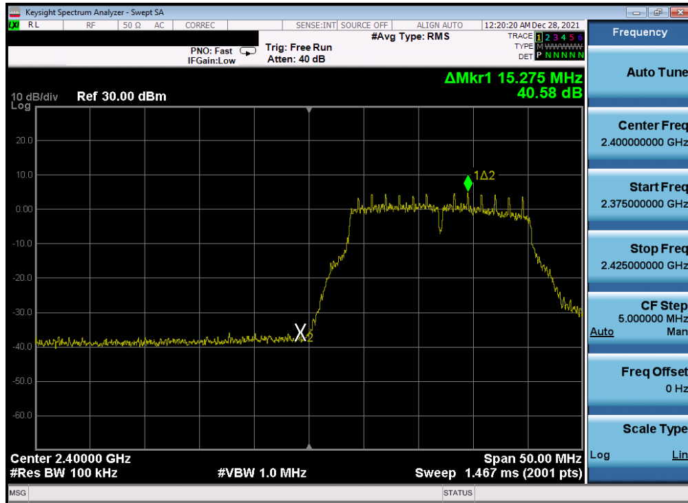
Plot 7-307. Band Edge Plot Antenna WF7b (802.11g - Ch. 1) - 6Mbps
