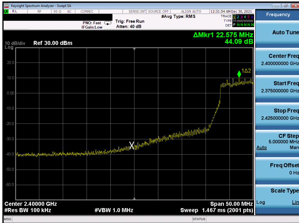
Plot 7-365. Band Edge Plot Antenna WF7b (802.11n (2.4GHz) – Ch. 4) – MCS3
