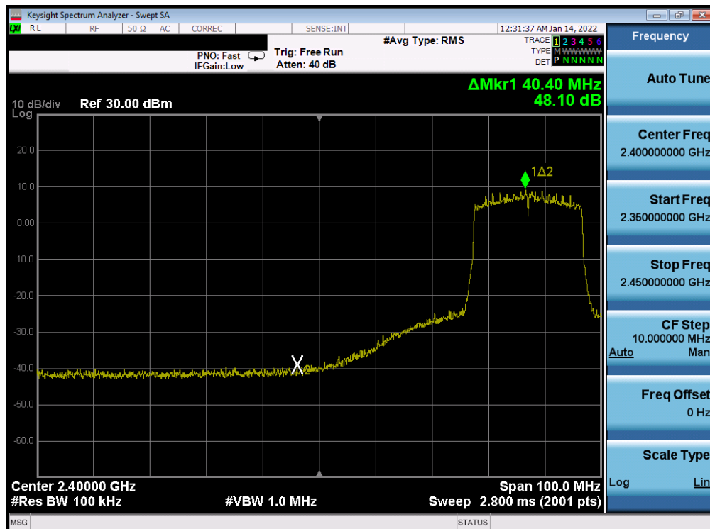
Plot 7-381. Band Edge Plot Antenna WF7b (802.11ax (SU - 2.4GHz) - Ch. 6 (low)) - MCS3
