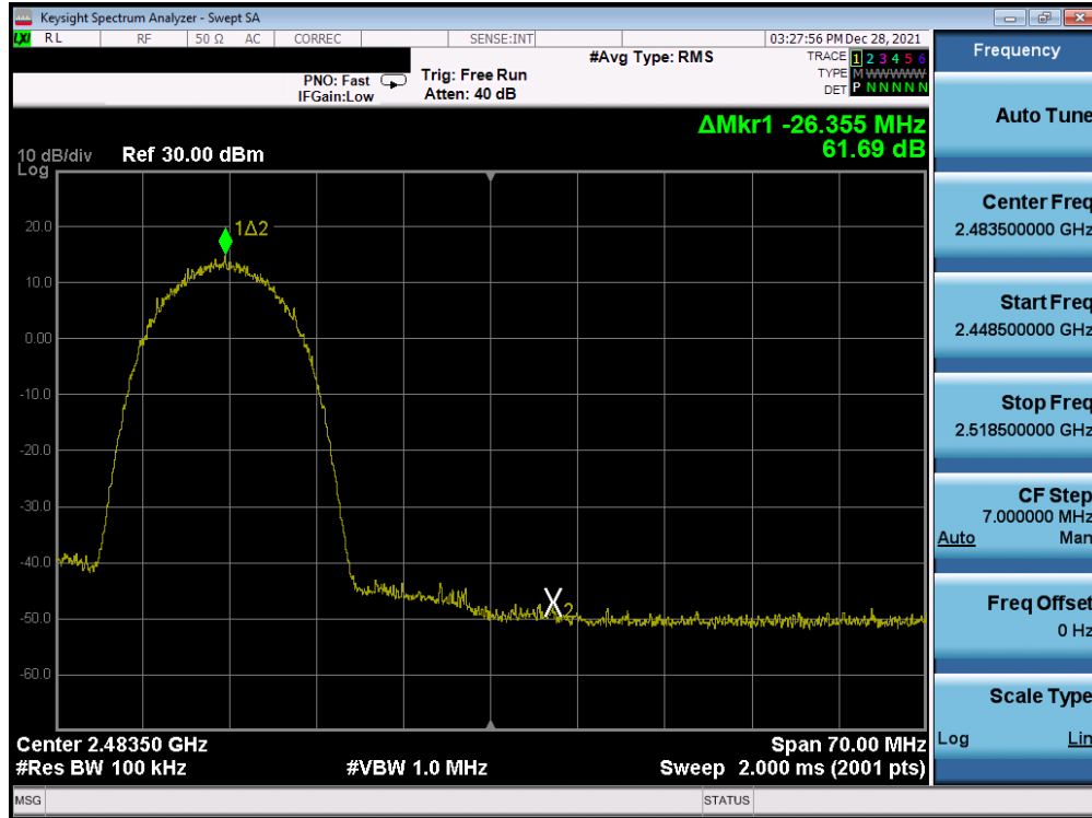
Plot 7-395. Band Edge Plot Antenna WF7b (802.11b – Ch. 11) – 11Mbps
