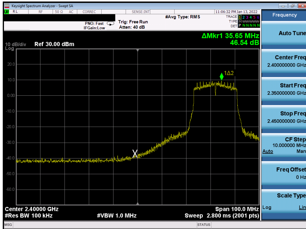
Plot 7-366. Band Edge Plot Antenna WF7b (802.11n (2.4GHz) – Ch. 5) – MCS3
