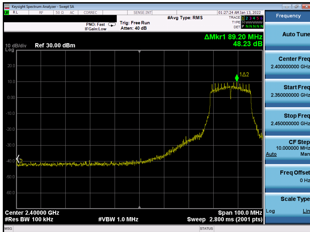
Plot 7-353. Band Edge Plot Antenna WF7b (802.11g – Ch. 6 (low)) – 18Mbps
