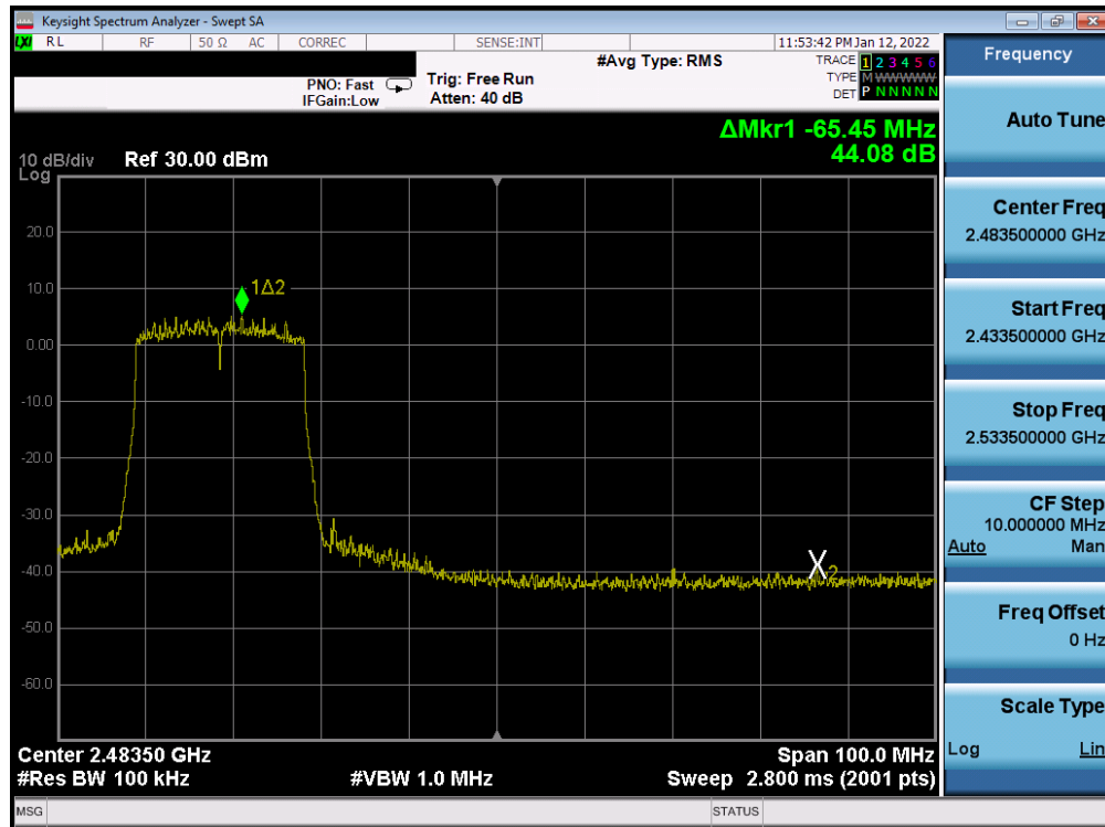
Plot 7-303. Band Edge Plot Antenna WF8 (802.11ax (SU - 2.4GHz) – Ch. 9) – MCS5
