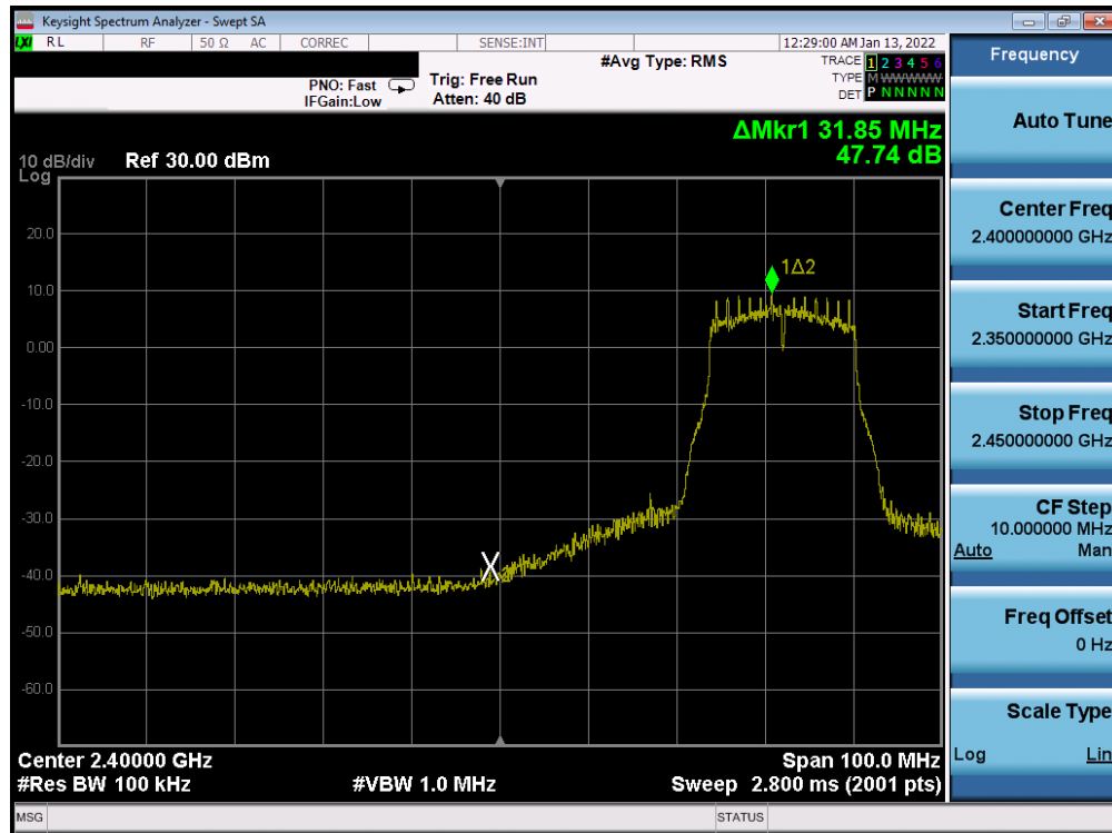
Plot 7-311. Band Edge Plot Antenna WF7b (802.11g – Ch. 5) – 6Mbps
