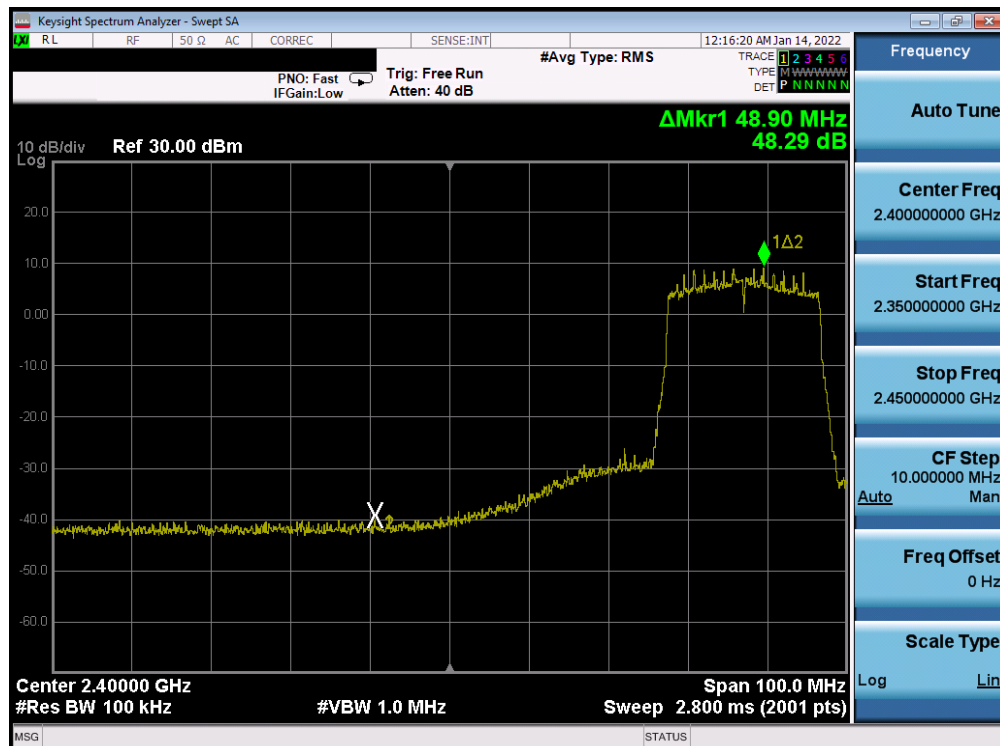
Plot 7-340. Band Edge Plot Antenna WF7b (802.11ax (SU - 2.4GHz) - Ch. 6 (low)) - MCS0
