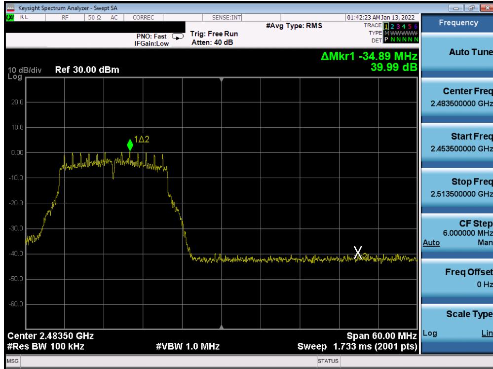
Plot 7-360. Band Edge Plot Antenna WF7b (802.11g - Ch. 12) - 18Mbps
