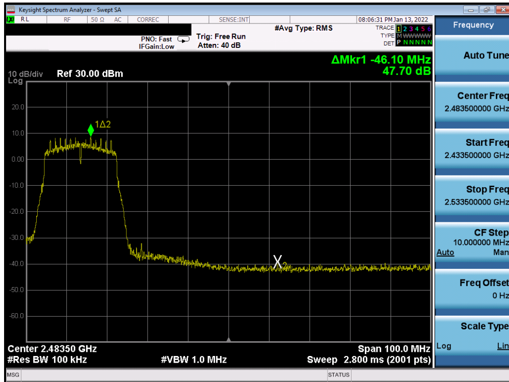
Plot 7-329. Band Edge Plot Antenna WF7b (802.11n (2.4GHz) – Ch. 8) – MCS0
