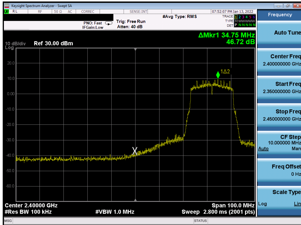
Plot 7-325. Band Edge Plot Antenna WF7b (802.11n (2.4GHz) – Ch. 5) – MCS0
