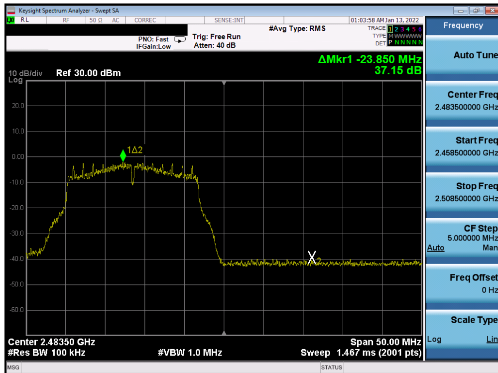
Plot 7-320. Band Edge Plot Antenna WF7b (802.11g - Ch. 13) - 6Mbps
