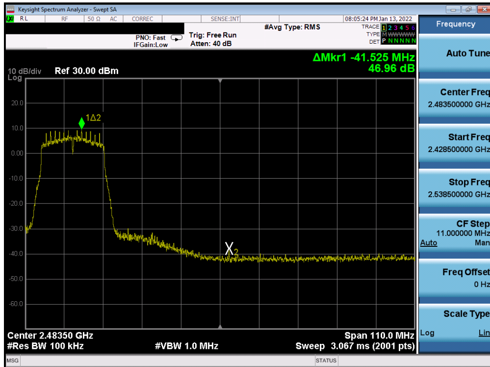
Plot 7-328. Band Edge Plot Antenna WF7b (802.11n (2.4GHz) – Ch. 7) – MCS0
