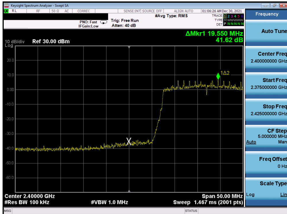
Plot 7-336. Band Edge Plot Antenna WF7b (802.11ax (SU - 2.4GHz) – Ch. 2) – MCS0
