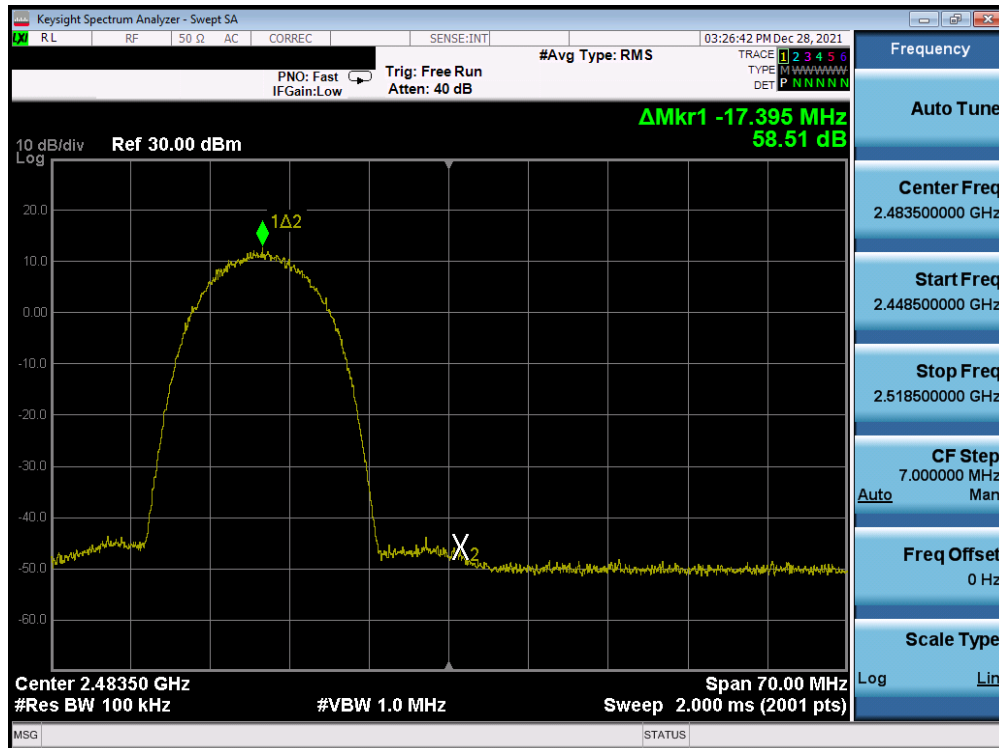
Plot 7-396. Band Edge Plot Antenna WF7b (802.11b – Ch. 12) – 11Mbps
