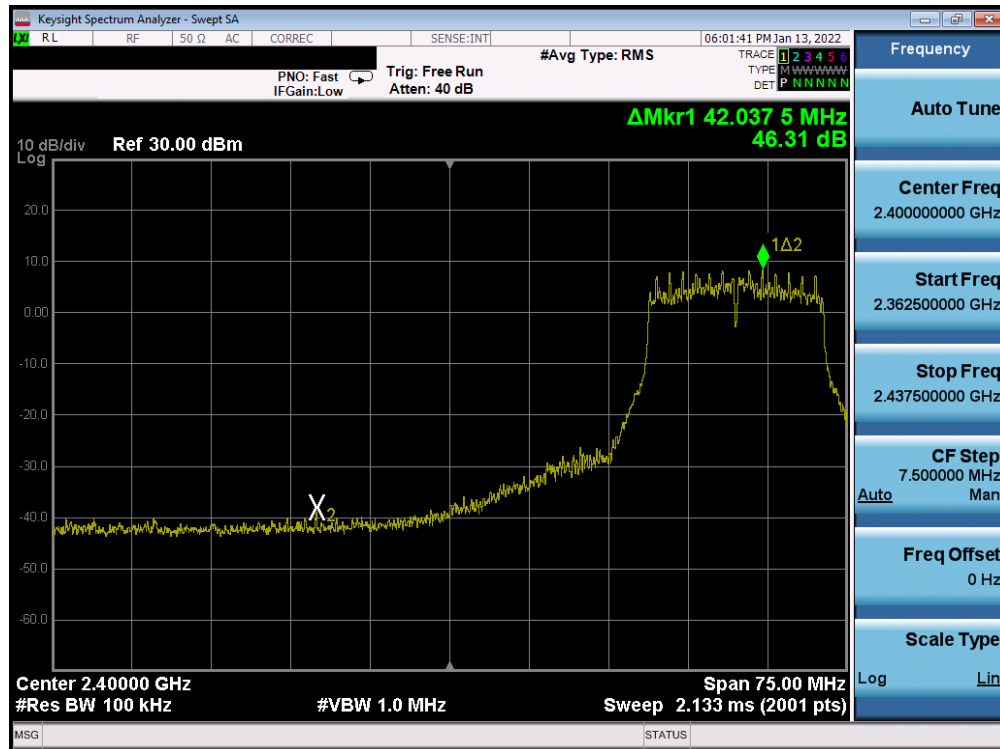
Plot 7-401. Band Edge Plot Antenna WF7b (802.11g – Ch. 4) – 36Mbps
