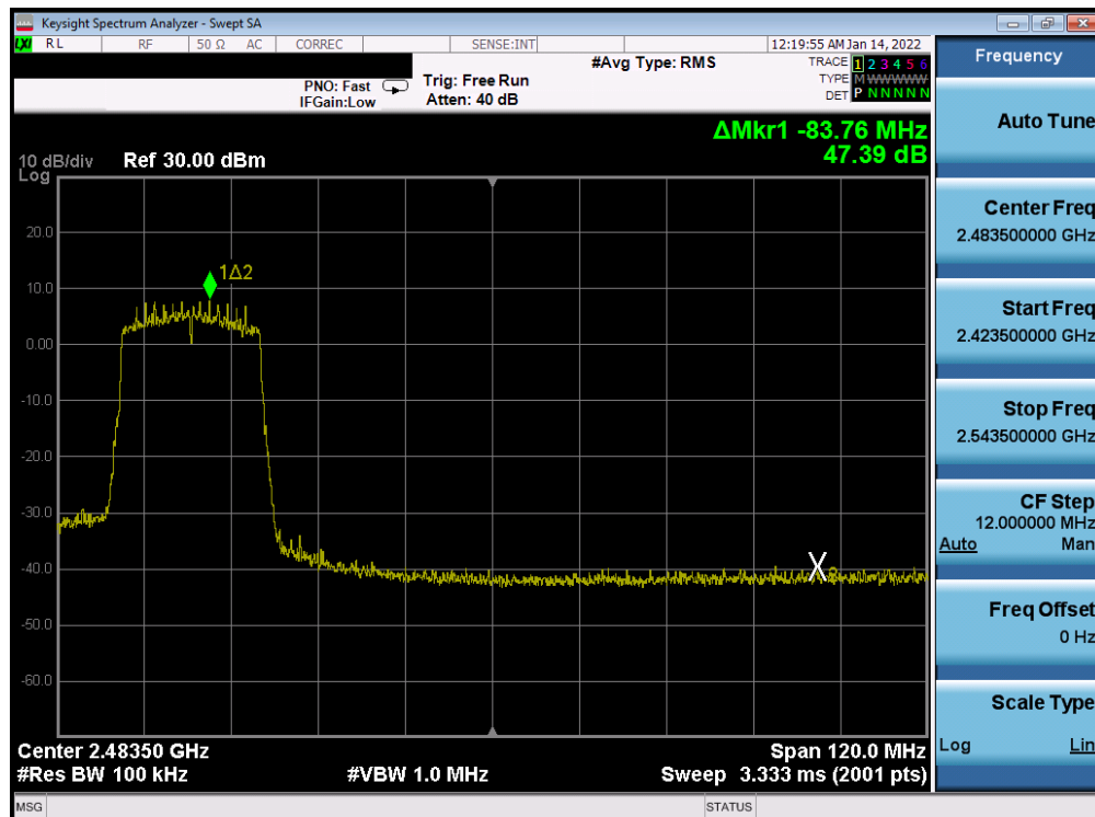
Plot 7-342. Band Edge Plot Antenna WF7b (802.11ax (SU - 2.4GHz) – Ch. 7) – MCS0
