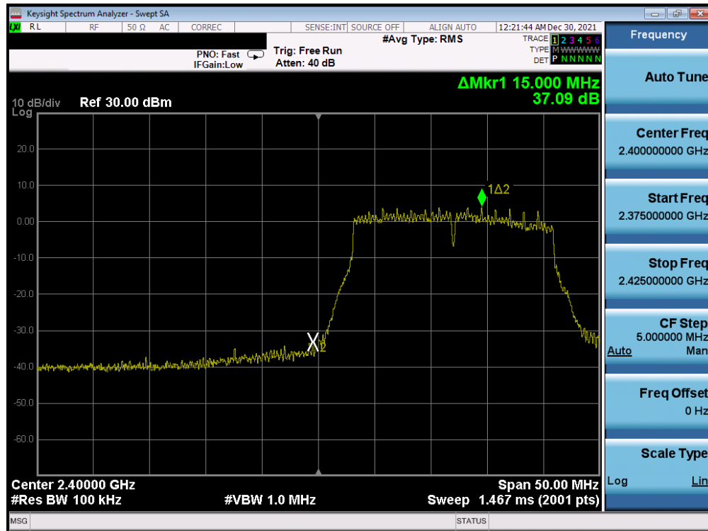
Plot 7-362. Band Edge Plot Antenna WF7b (802.11n (2.4GHz) – Ch. 1) – MCS3
