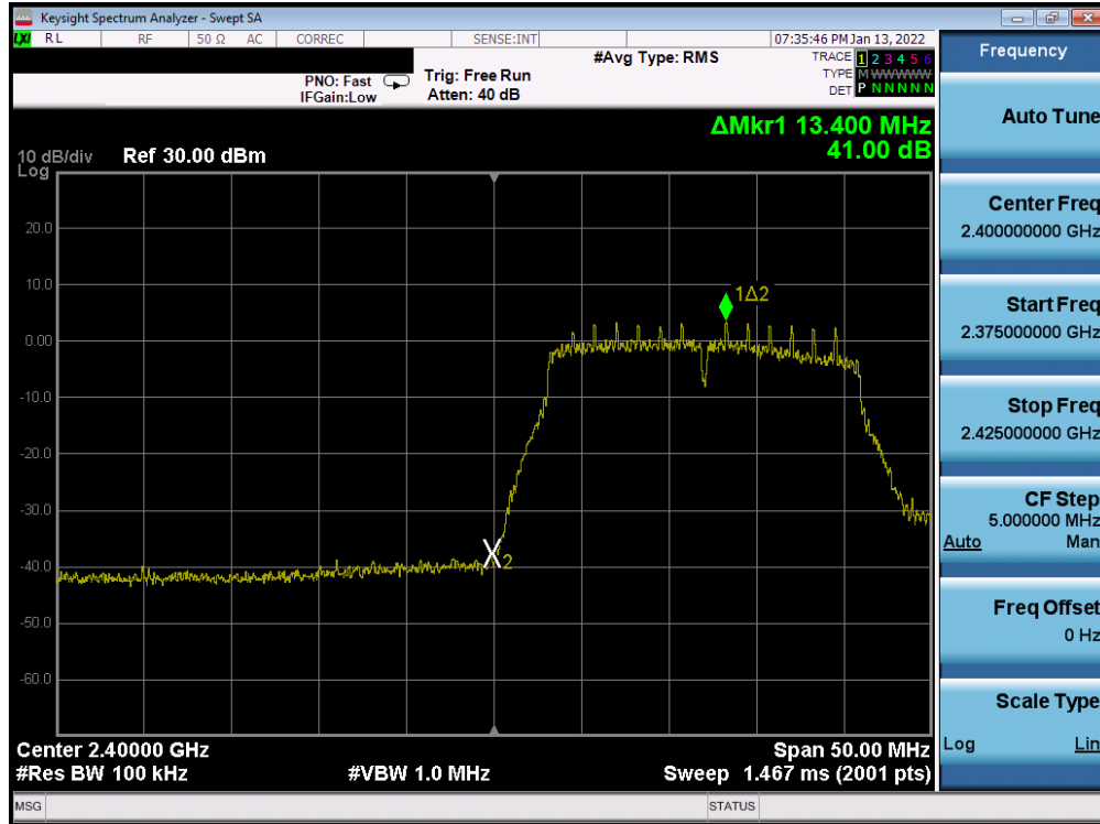
Plot 7-321. Band Edge Plot Antenna WF7b (802.11n (2.4GHz) – Ch. 1) – MCS0
