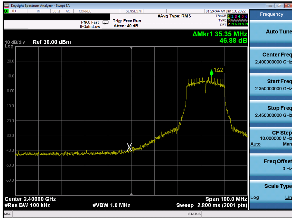
Plot 7-352. Band Edge Plot Antenna WF7b (802.11g – Ch. 5) – 18Mbps
