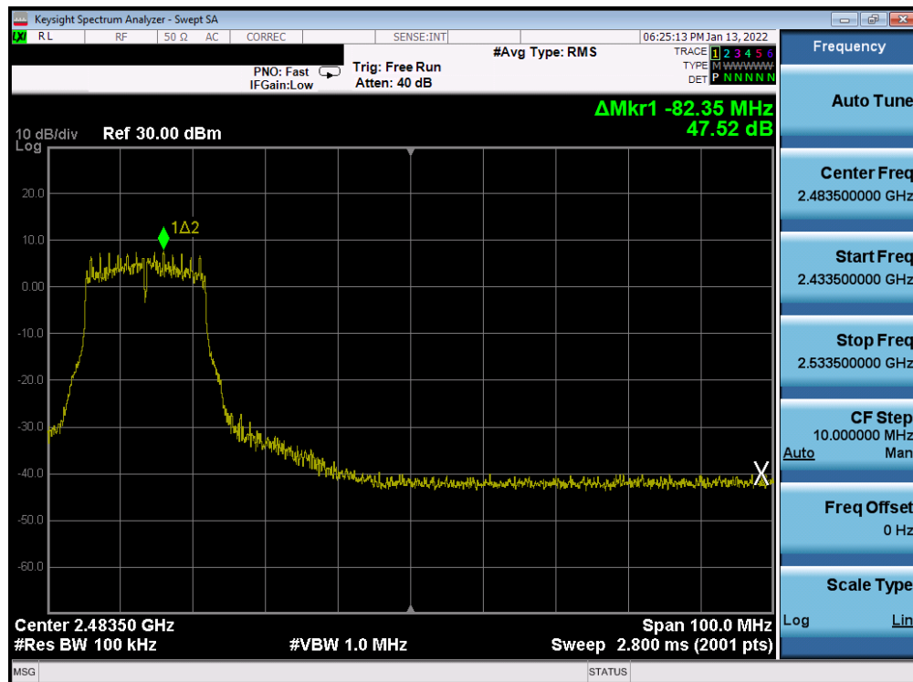
Plot 7-406. Band Edge Plot Antenna WF7b (802.11g - Ch. 8) - 36Mbps
