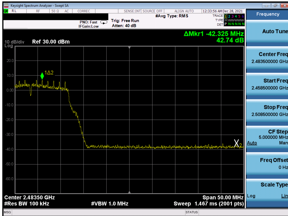
Plot 7-318. Band Edge Plot Antenna WF7b (802.11g – Ch. 11) – 6Mbps
