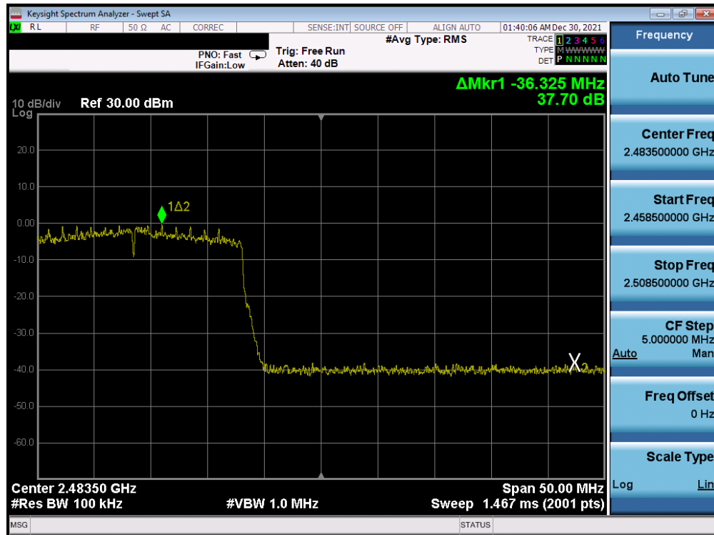
Plot 7-388. Band Edge Plot Antenna WF7b (802.11ax (SU - 2.4GHz) – Ch. 12) – MCS3
