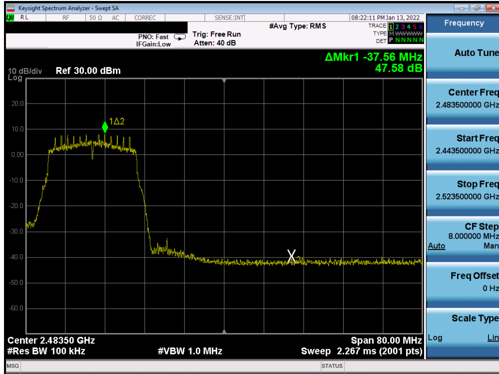
Plot 7-331. Band Edge Plot Antenna WF7b (802.11n (2.4GHz) – Ch. 10) – MCS0
