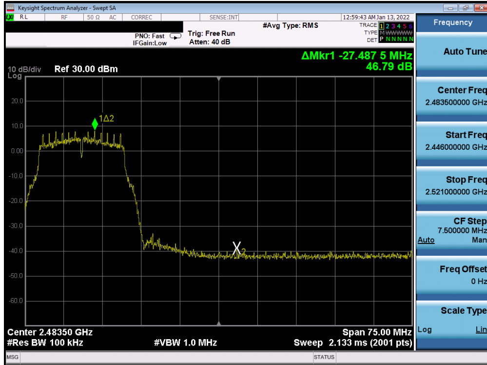
Plot 7-317. Band Edge Plot Antenna WF7b (802.11g – Ch. 10) – 6Mbps
