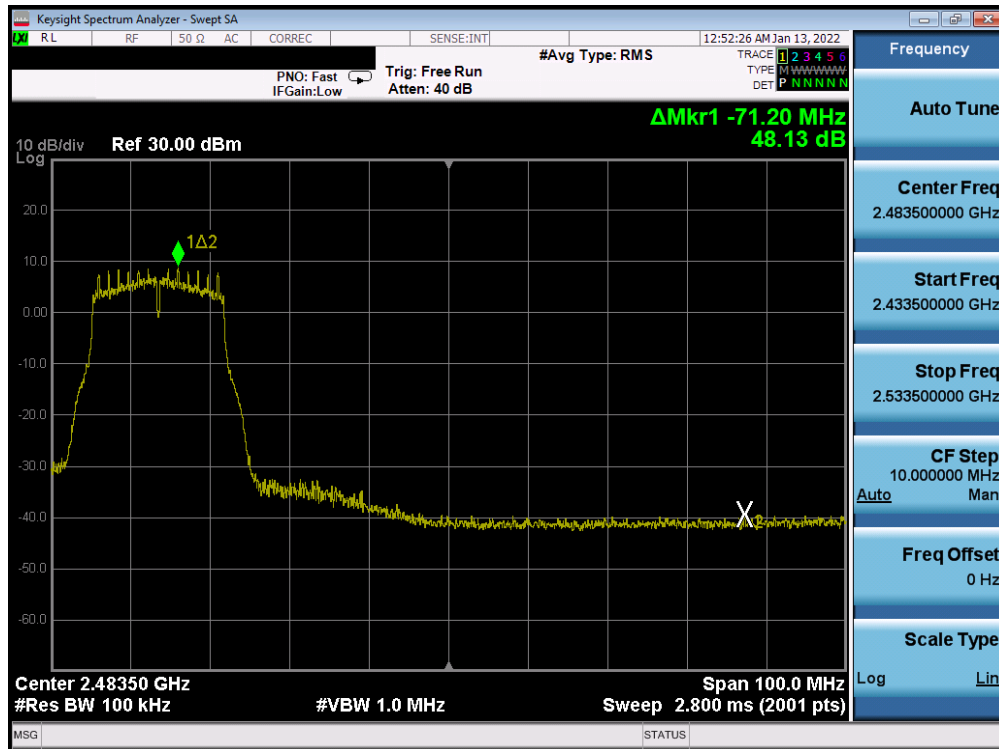
Plot 7-315. Band Edge Plot Antenna WF7b (802.11g - Ch. 8) - 6Mbps
