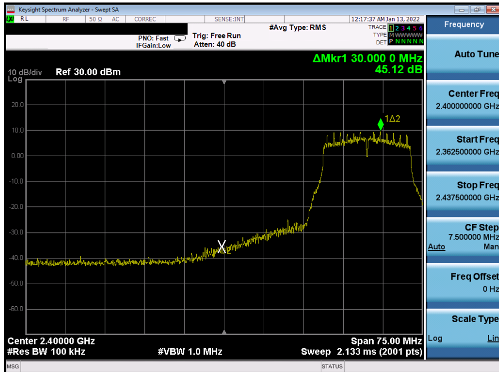
Plot 7-310. Band Edge Plot Antenna WF7b (802.11g - Ch. 4) - 6Mbps
