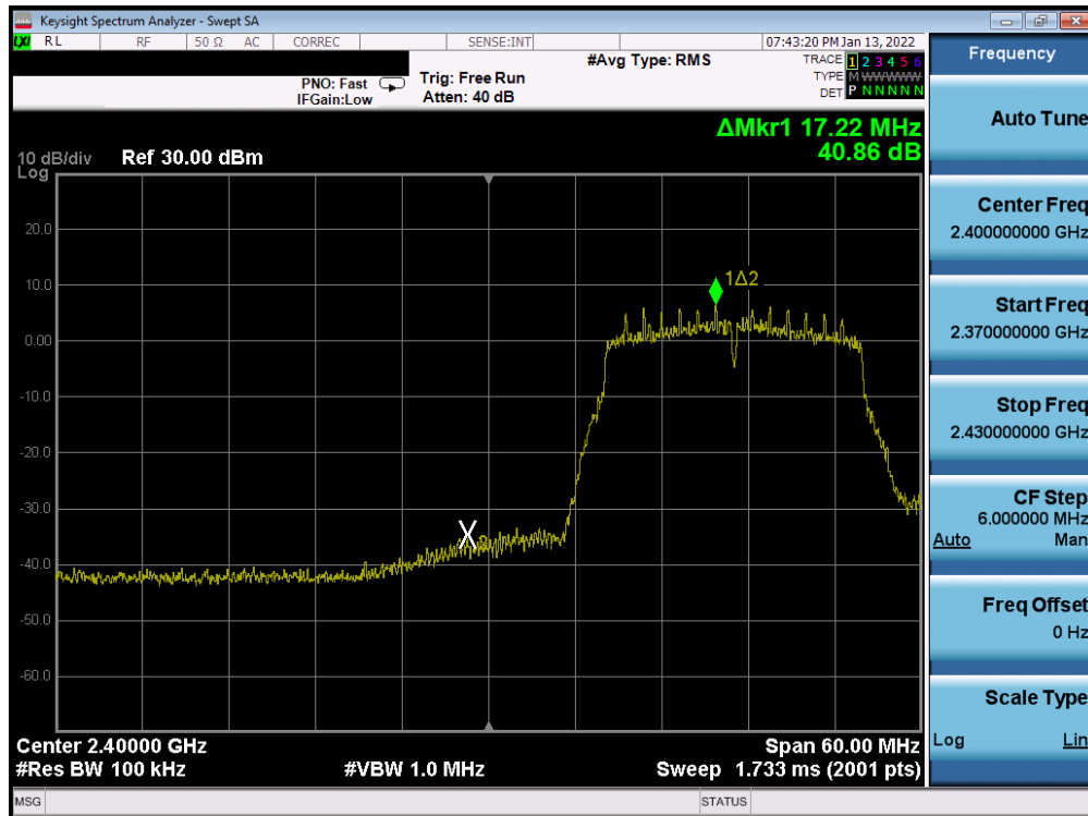
Plot 7-322. Band Edge Plot Antenna WF7b (802.11n (2.4GHz) – Ch. 2) – MCS0
