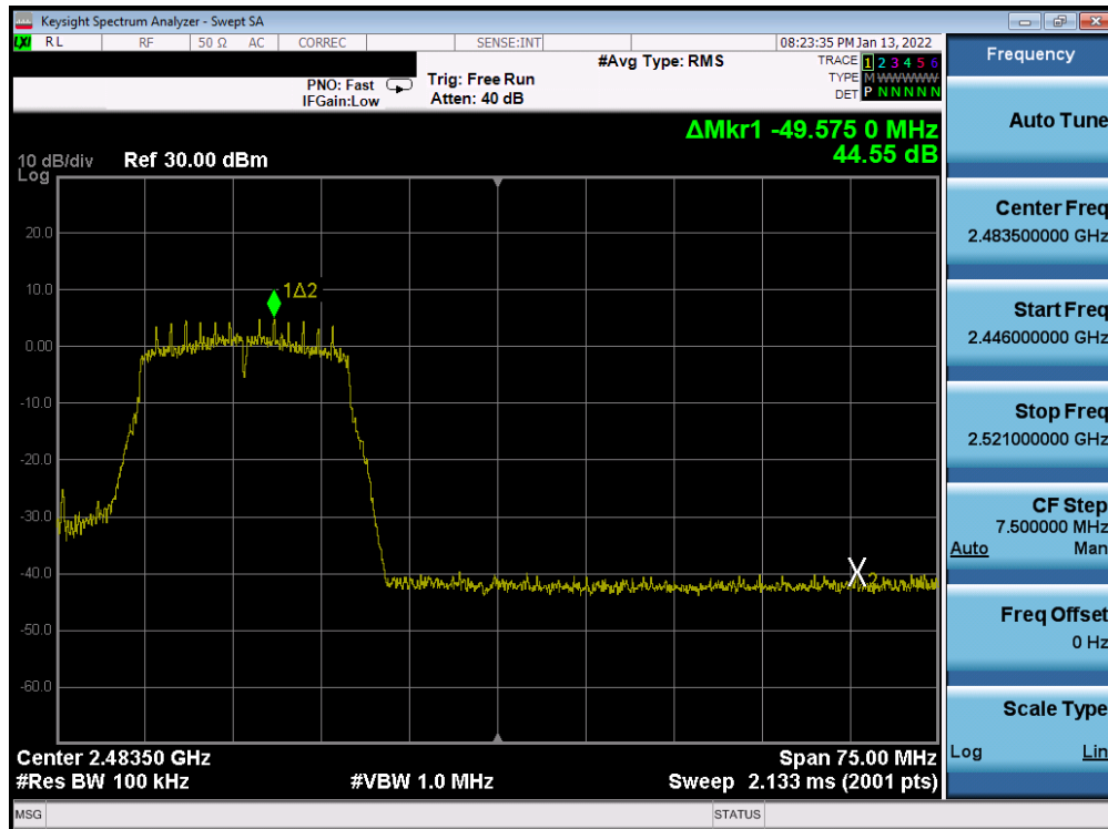
Plot 7-332. Band Edge Plot Antenna WF7b (802.11n (2.4GHz) – Ch. 11) – MCS0
