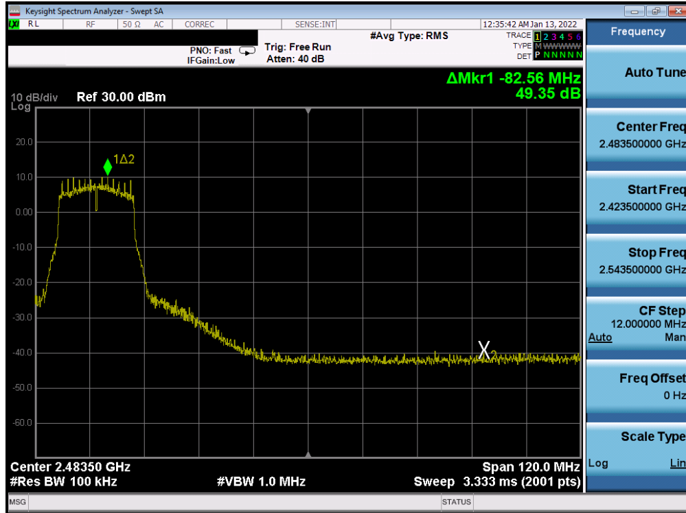
Plot 7-313. Band Edge Plot Antenna WF7b (802.11g - Ch. 6 (high)) - 6Mbps
