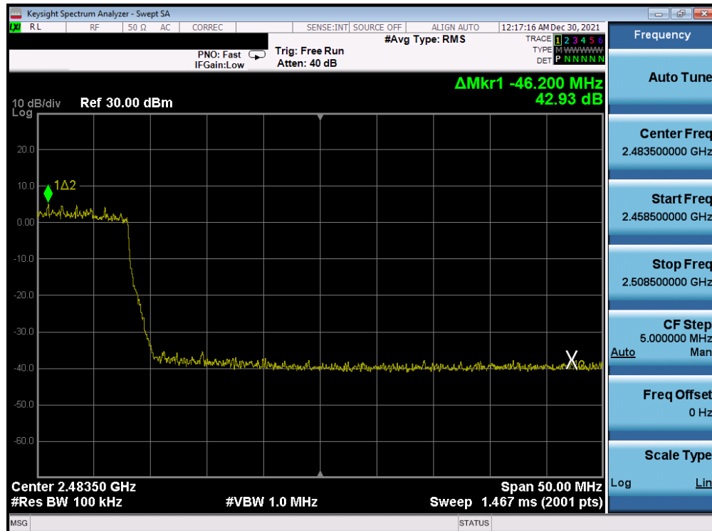
Plot 7-304. Band Edge Plot Antenna WF8 (802.11ax (SU - 2.4GHz) – Ch. 10) – MCS5
