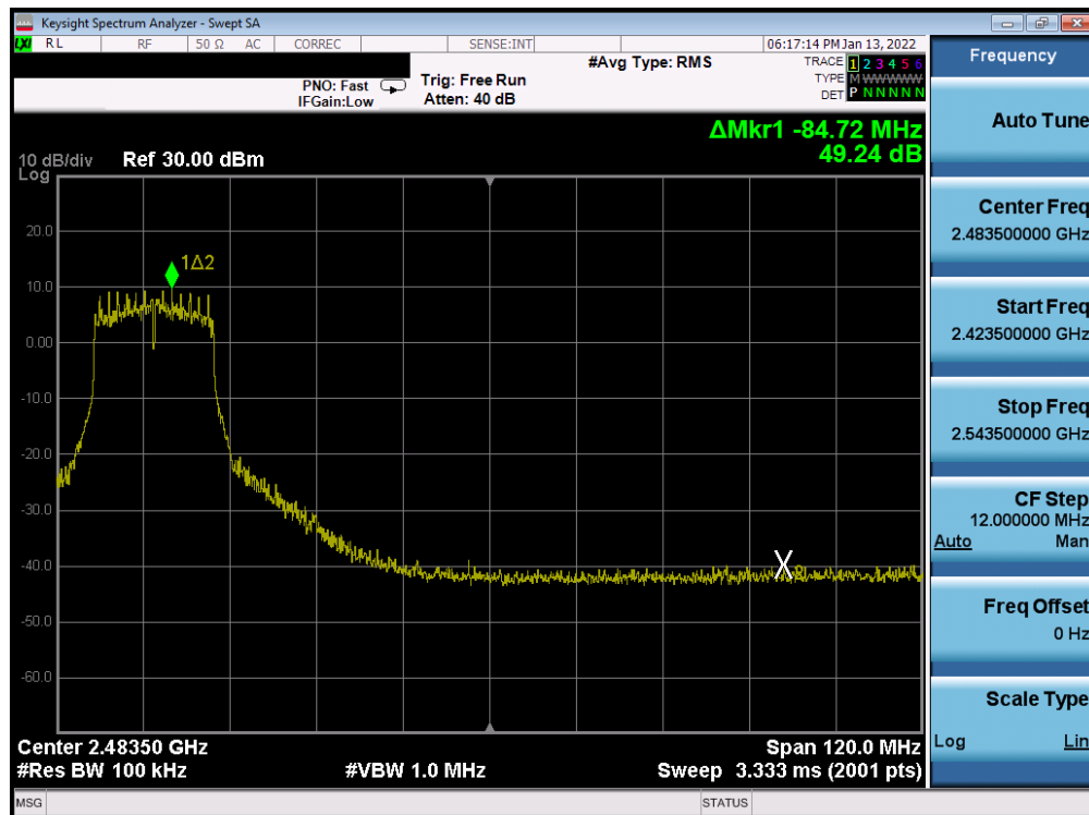
Plot 7-404. Band Edge Plot Antenna WF7b (802.11g - Ch. 6 (high)) - 36Mbps
