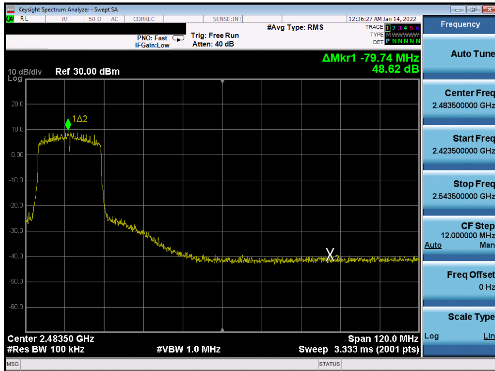
Plot 7-382. Band Edge Plot Antenna WF7b (802.11ax (SU - 2.4GHz) – Ch. 6 (high)) – MCS3
