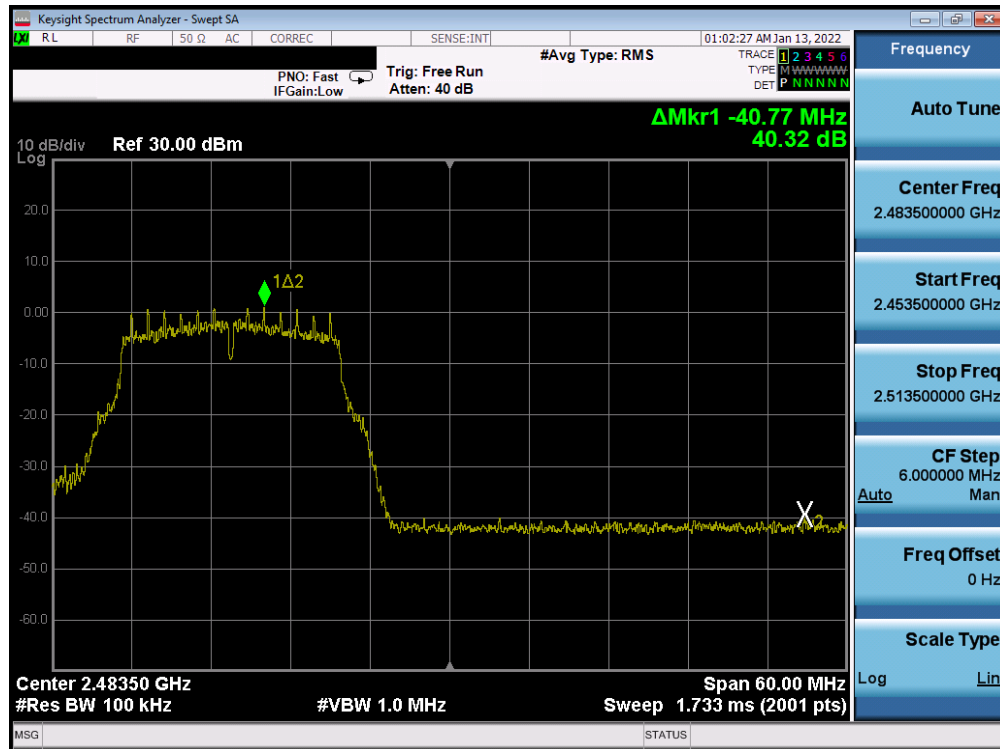
Plot 7-319. Band Edge Plot Antenna WF7b (802.11g - Ch. 12) - 6Mbps
