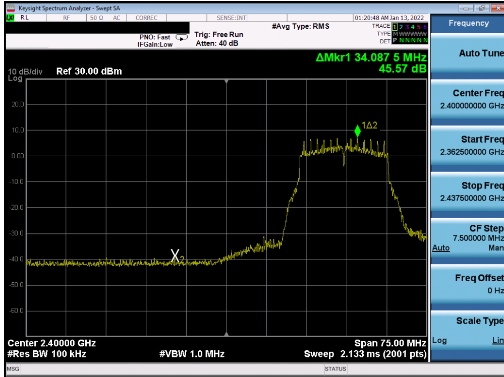
Plot 7-350. Band Edge Plot Antenna WF7b (802.11g – Ch. 3) – 18Mbps
