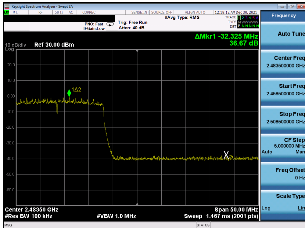
Plot 7-306. Band Edge Plot Antenna WF8 (802.11ax (SU - 2.4GHz) – Ch. 12) – MCS5
