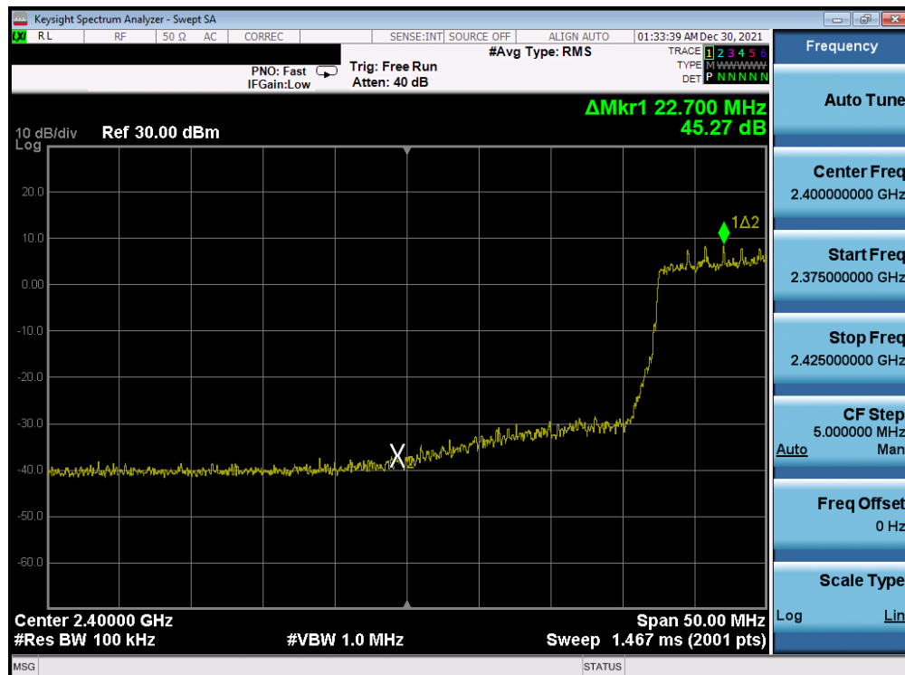
Plot 7-379. Band Edge Plot Antenna WF7b (802.11ax (SU - 2.4GHz) – Ch. 4) – MCS3
