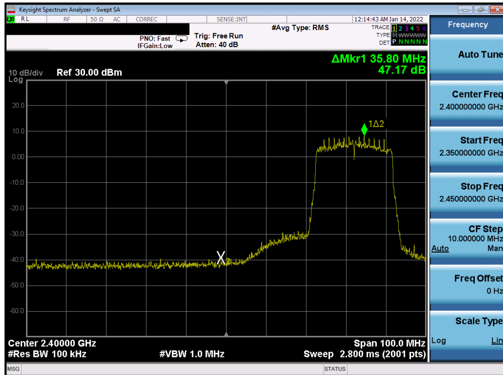
Plot 7-339. Band Edge Plot Antenna WF7b (802.11ax (SU - 2.4GHz) - Ch. 5) - MCS0
