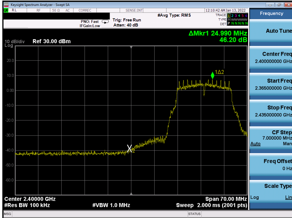
Plot 7-309. Band Edge Plot Antenna WF7b (802.11g - Ch. 3) - 6Mbps
