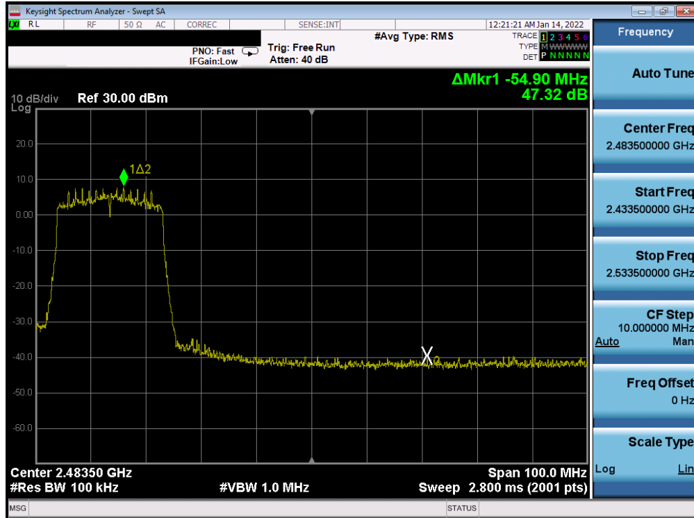
Plot 7-343. Band Edge Plot Antenna WF7b (802.11ax (SU - 2.4GHz) - Ch. 8) - MCS0
