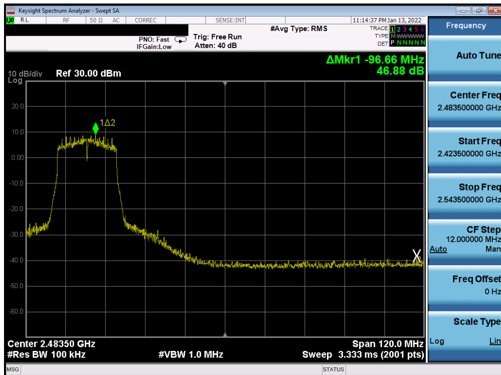
Plot 7-369. Band Edge Plot Antenna WF7b (802.11n (2.4GHz) - Ch. 7) - MCS3
