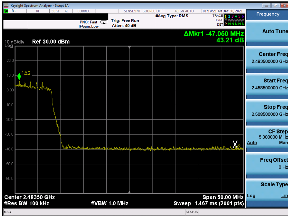
Plot 7-345. Band Edge Plot Antenna WF7b (802.11ax (SU - 2.4GHz) – Ch. 10) – MCS0
