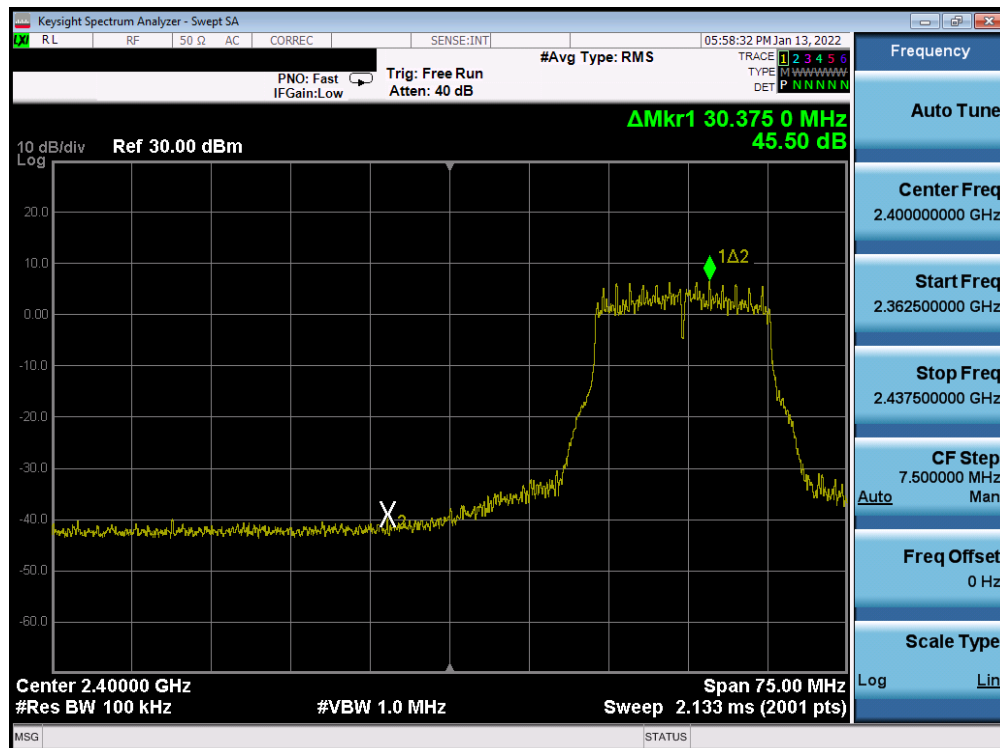
Plot 7-400. Band Edge Plot Antenna WF7b (802.11g – Ch. 3) – 36Mbps
