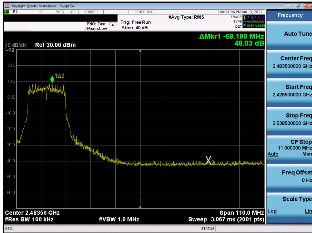
Plot 7-405. Band Edge Plot Antenna WF7b (802.11g - Ch. 7) - 36Mbps
