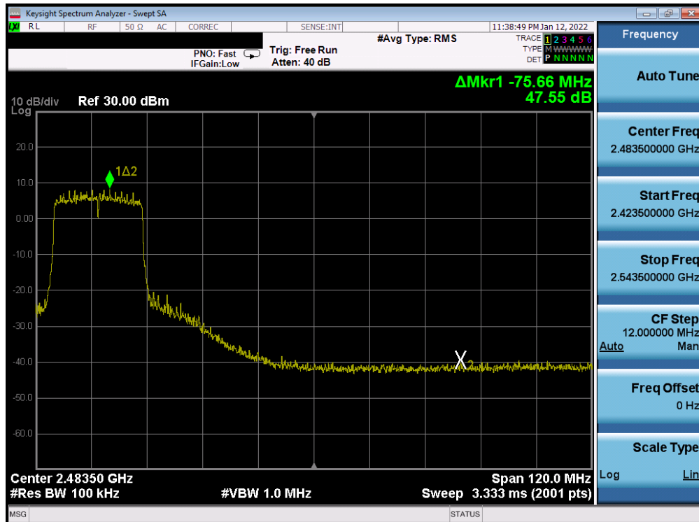
Plot 7-300. Band Edge Plot Antenna WF8 (802.11ax (SU - 2.4GHz) – Ch. 6 (high)) – MCS5
