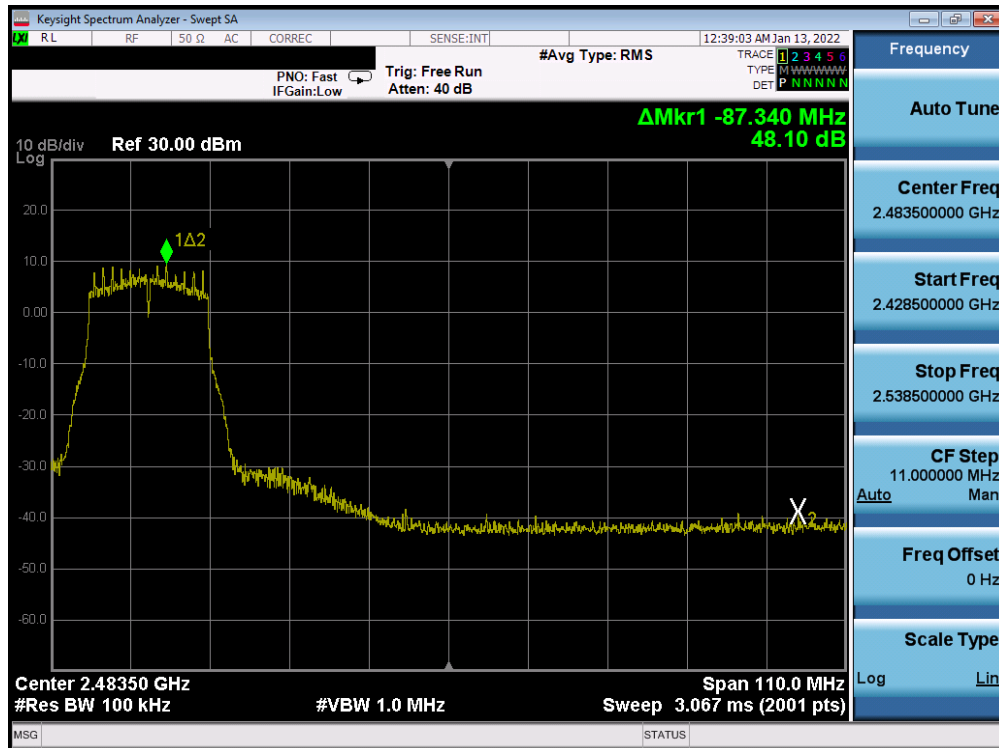
Plot 7-314. Band Edge Plot Antenna WF7b (802.11g - Ch. 7) - 6Mbps
