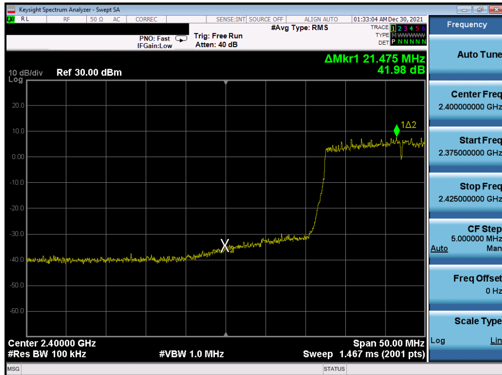
Plot 7-378. Band Edge Plot Antenna WF7b (802.11ax (SU - 2.4GHz) – Ch. 3) – MCS3
