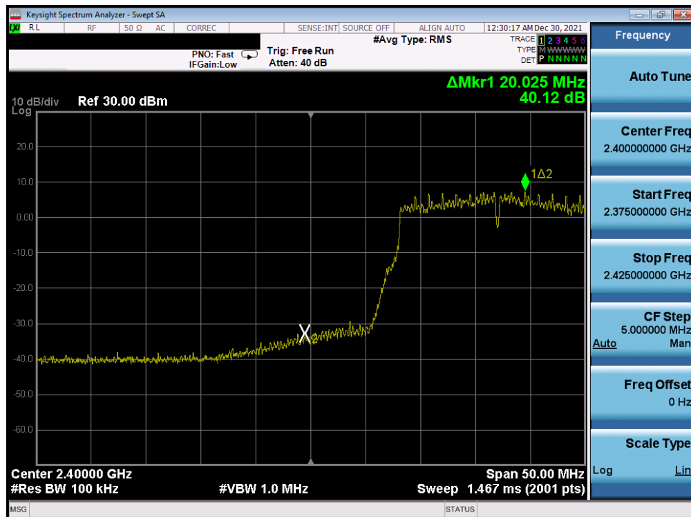
Plot 7-363. Band Edge Plot Antenna WF7b (802.11n (2.4GHz) – Ch. 2) – MCS3
