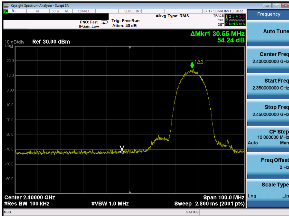
Plot 7-392. Band Edge Plot Antenna WF7b (802.11b – Ch. 4) – 11Mbps
