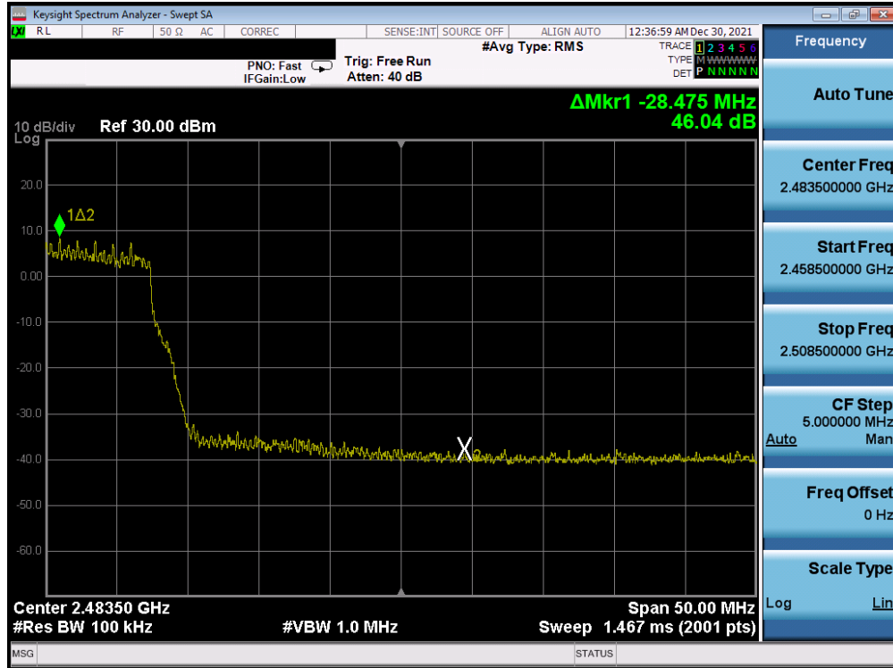
Plot 7-372. Band Edge Plot Antenna WF7b (802.11n (2.4GHz) – Ch. 10) – MCS3
