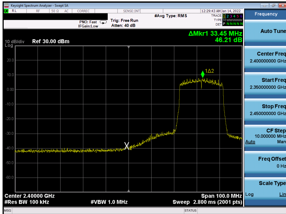
Plot 7-380. Band Edge Plot Antenna WF7b (802.11ax (SU - 2.4GHz) - Ch. 5) - MCS3
