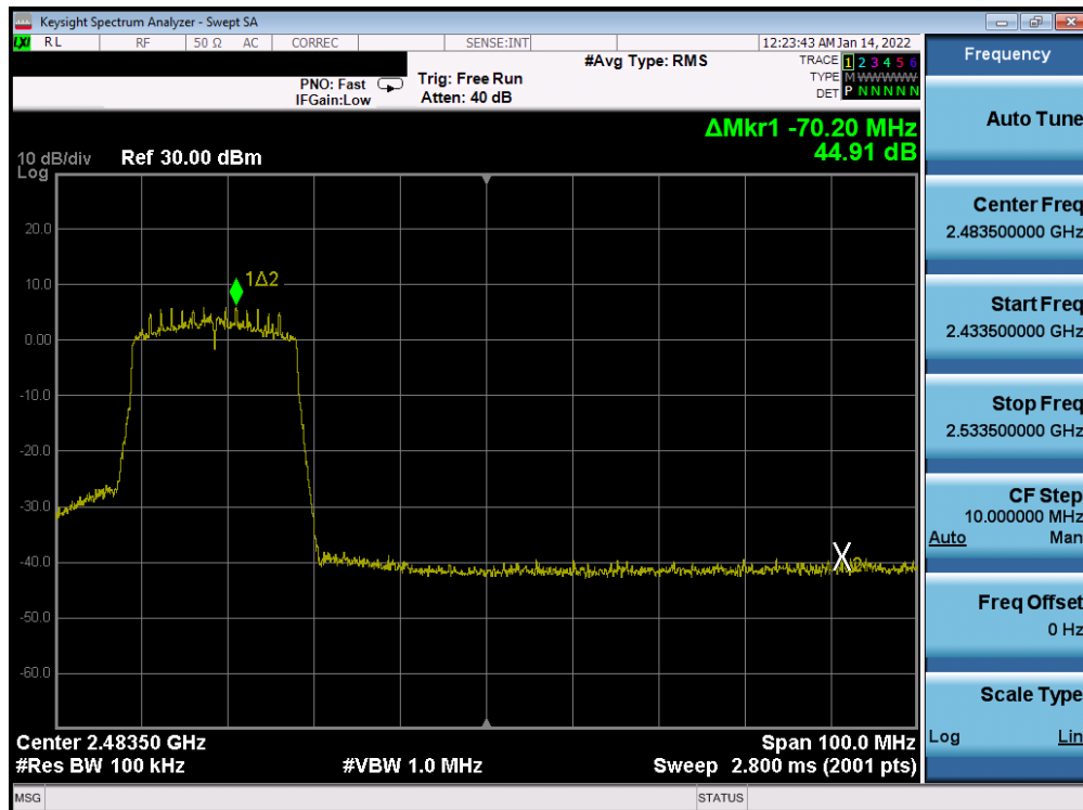
Plot 7-344. Band Edge Plot Antenna WF7b (802.11ax (SU - 2.4GHz) - Ch. 9) - MCS0
