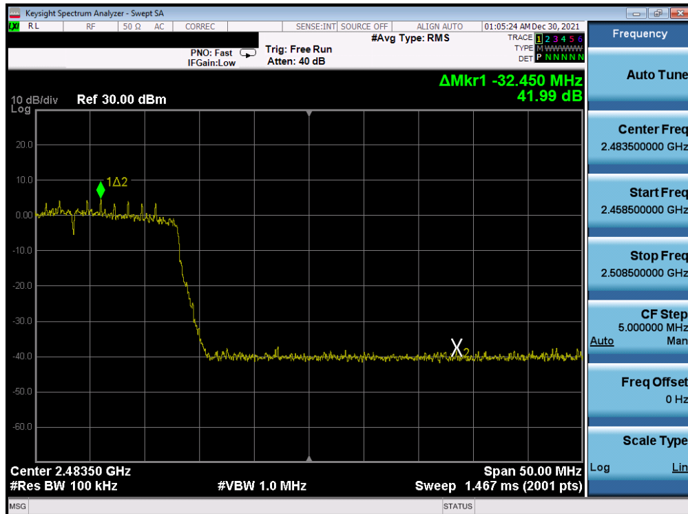
Plot 7-346. Band Edge Plot Antenna WF7b (802.11ax (SU - 2.4GHz) – Ch. 11) – MCS0
