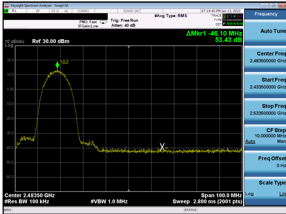
Plot 7-393. Band Edge Plot Antenna WF7b (802.11b – Ch. 9) – 11Mbps
