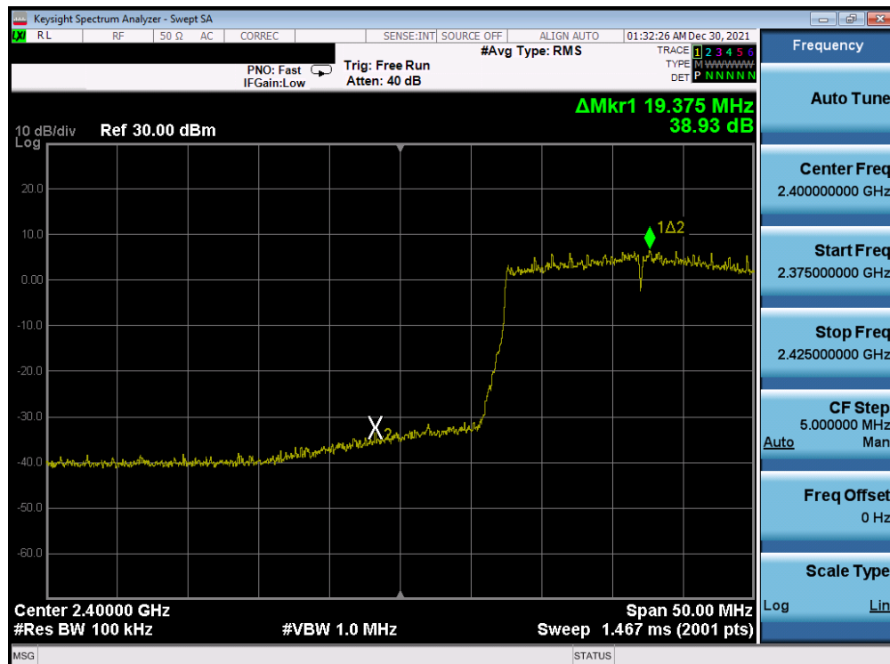
Plot 7-377. Band Edge Plot Antenna WF7b (802.11ax (SU - 2.4GHz) – Ch. 2) – MCS3
