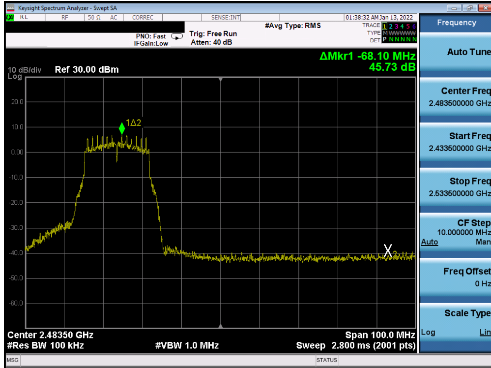
Plot 7-358. Band Edge Plot Antenna WF7b (802.11g - Ch. 10) - 18Mbps
