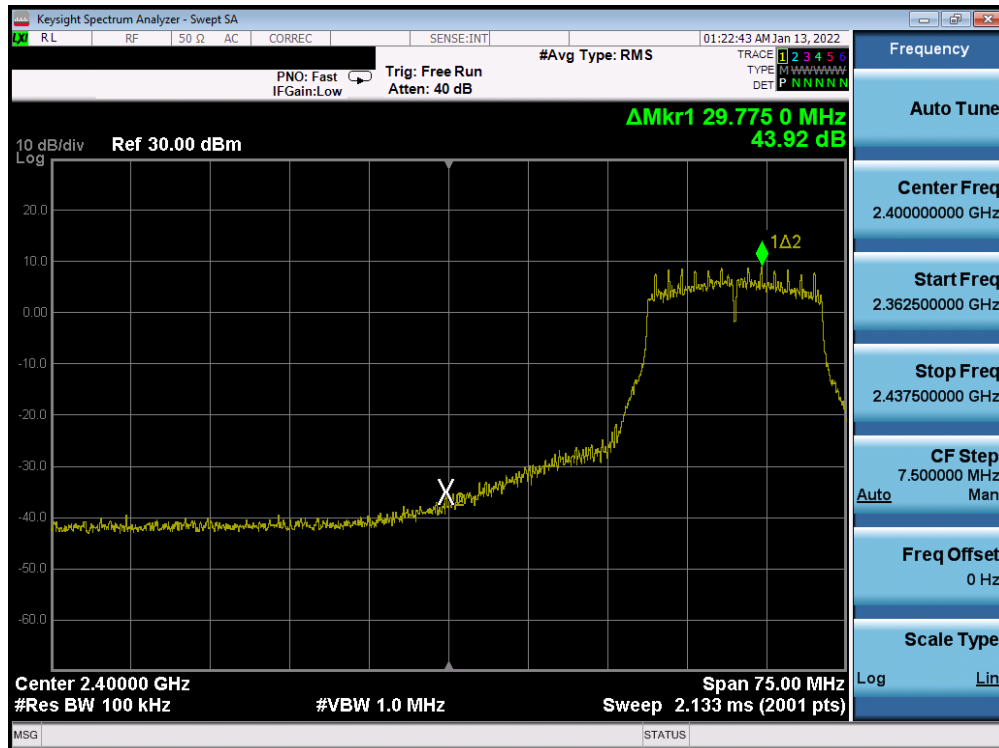
Plot 7-351. Band Edge Plot Antenna WF7b (802.11g – Ch. 4) – 18Mbps
