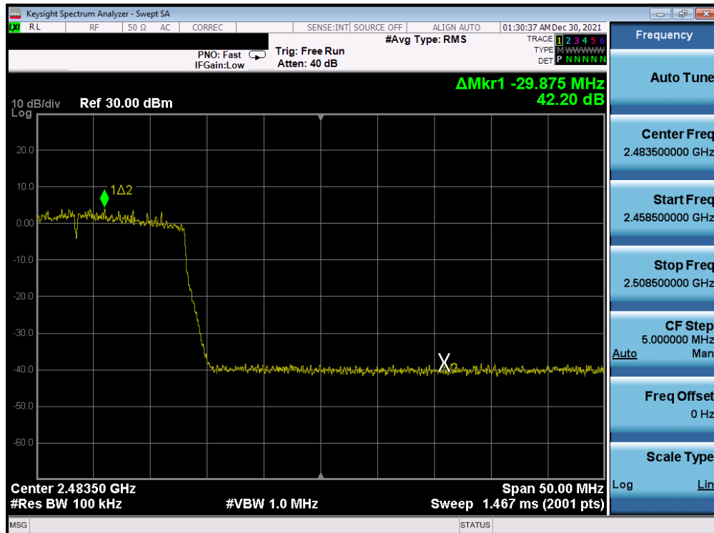
Plot 7-387. Band Edge Plot Antenna WF7b (802.11ax (SU - 2.4GHz) – Ch. 11) – MCS3
