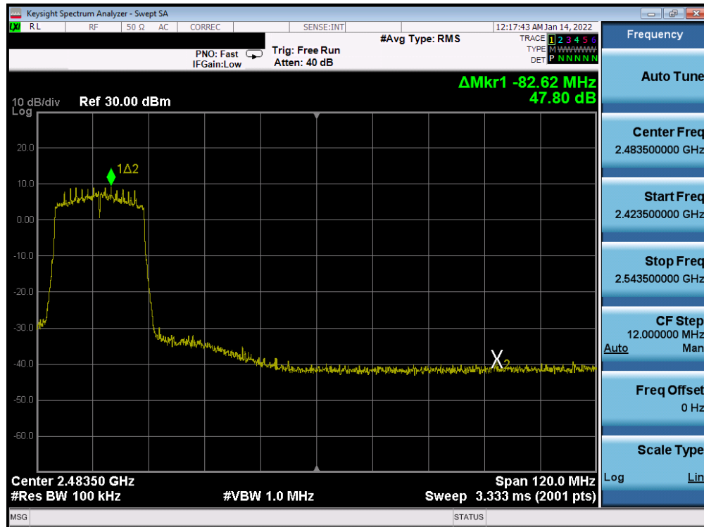
Plot 7-341. Band Edge Plot Antenna WF7b (802.11ax (SU - 2.4GHz) – Ch. 6 (high)) – MCS0
