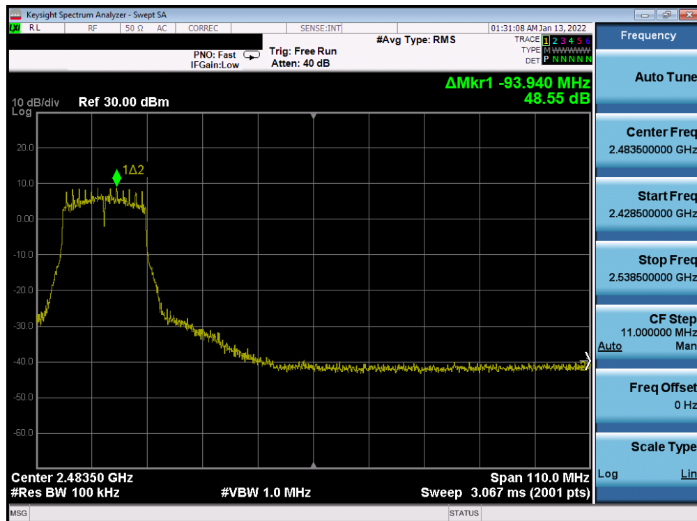
Plot 7-355. Band Edge Plot Antenna WF7b (802.11g – Ch. 7) – 18Mbps
