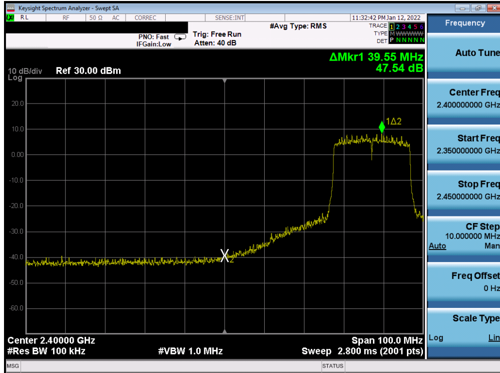
Plot 7-299. Band Edge Plot Antenna WF8 (802.11ax (SU - 2.4GHz) – Ch. 6 (low)) – MCS5
