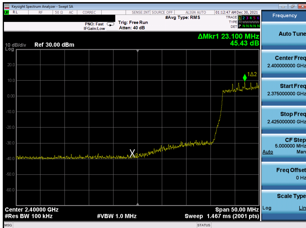
Plot 7-338. Band Edge Plot Antenna WF7b (802.11ax (SU - 2.4GHz) - Ch. 4) - MCS0
