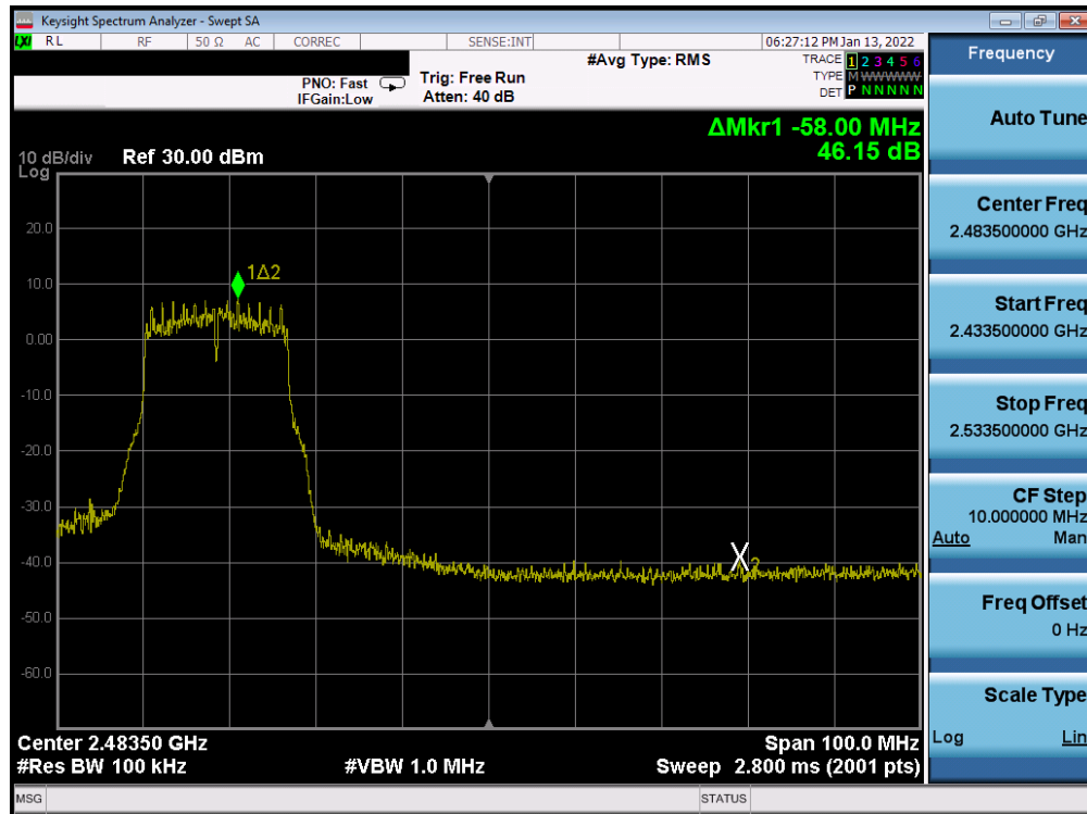
Plot 7-407. Band Edge Plot Antenna WF7b (802.11g - Ch. 9) - 36Mbps
