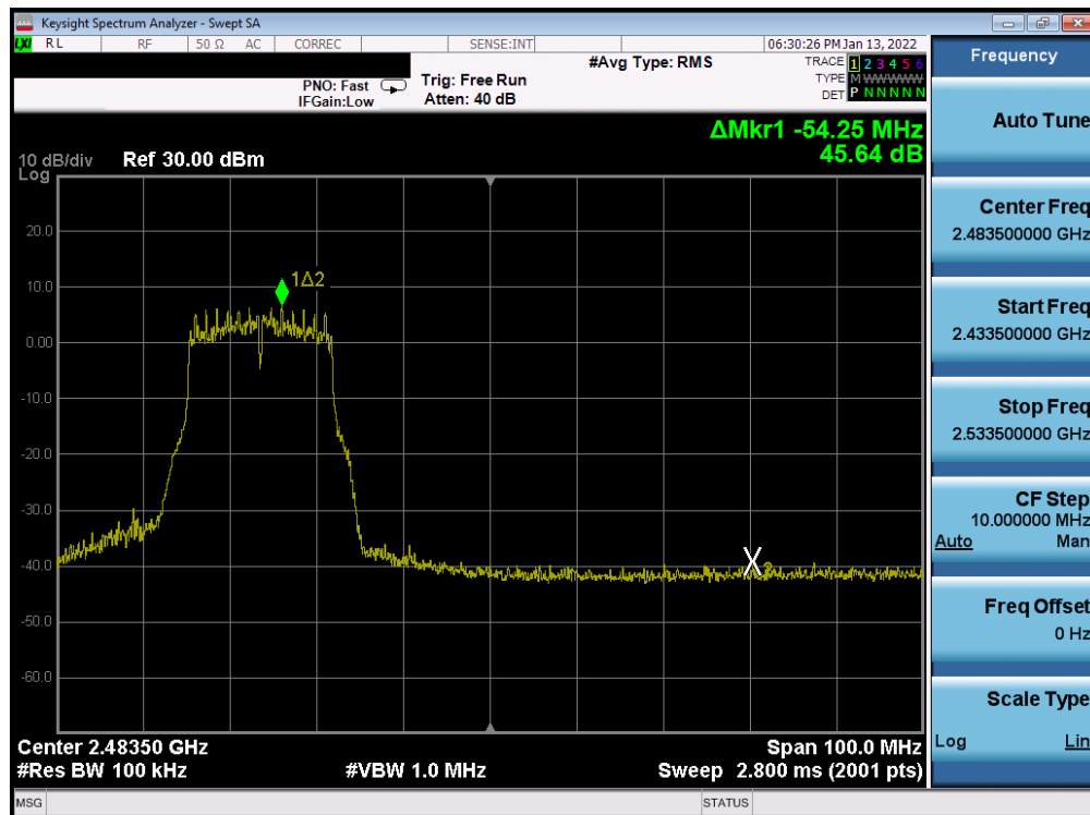
Plot 7-408. Band Edge Plot Antenna WF7b (802.11g - Ch. 10) - 36Mbps
