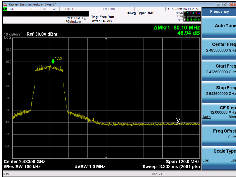
Plot 7-370. Band Edge Plot Antenna WF7b (802.11n (2.4GHz) – Ch. 8) – MCS3
