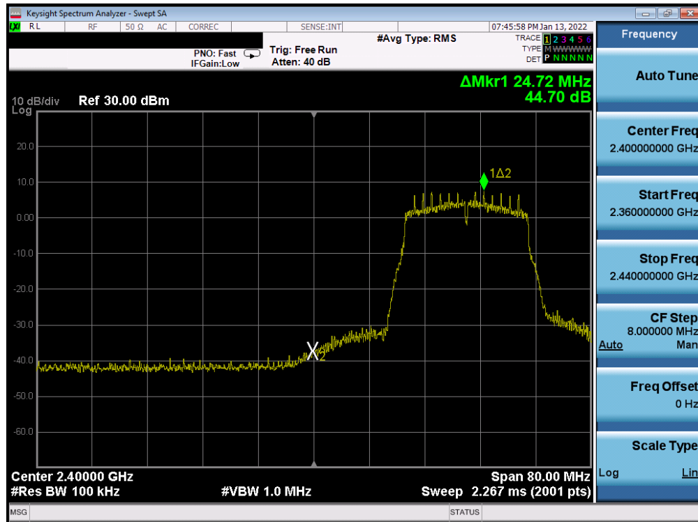
Plot 7-323. Band Edge Plot Antenna WF7b (802.11n (2.4GHz) – Ch. 3) – MCS0
