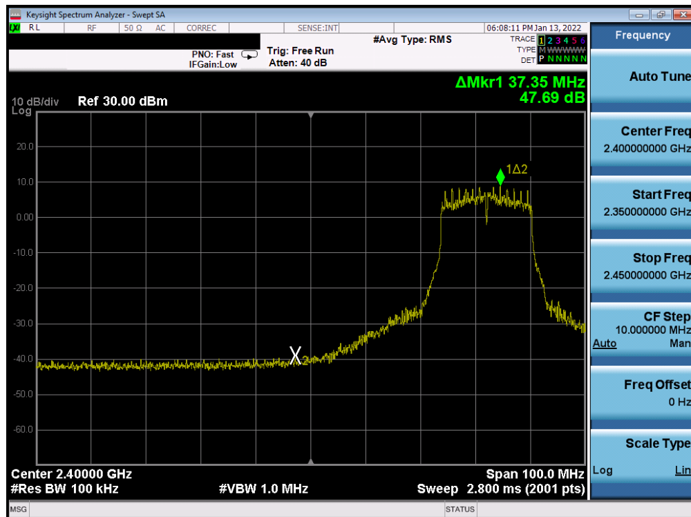
Plot 7-402. Band Edge Plot Antenna WF7b (802.11g – Ch. 5) – 36Mbps
