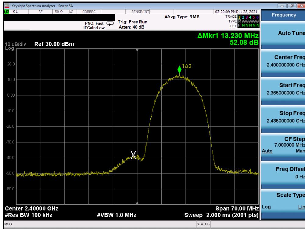
Plot 7-389. Band Edge Plot Antenna WF7b (802.11b – Ch. 1) – 11Mbps
