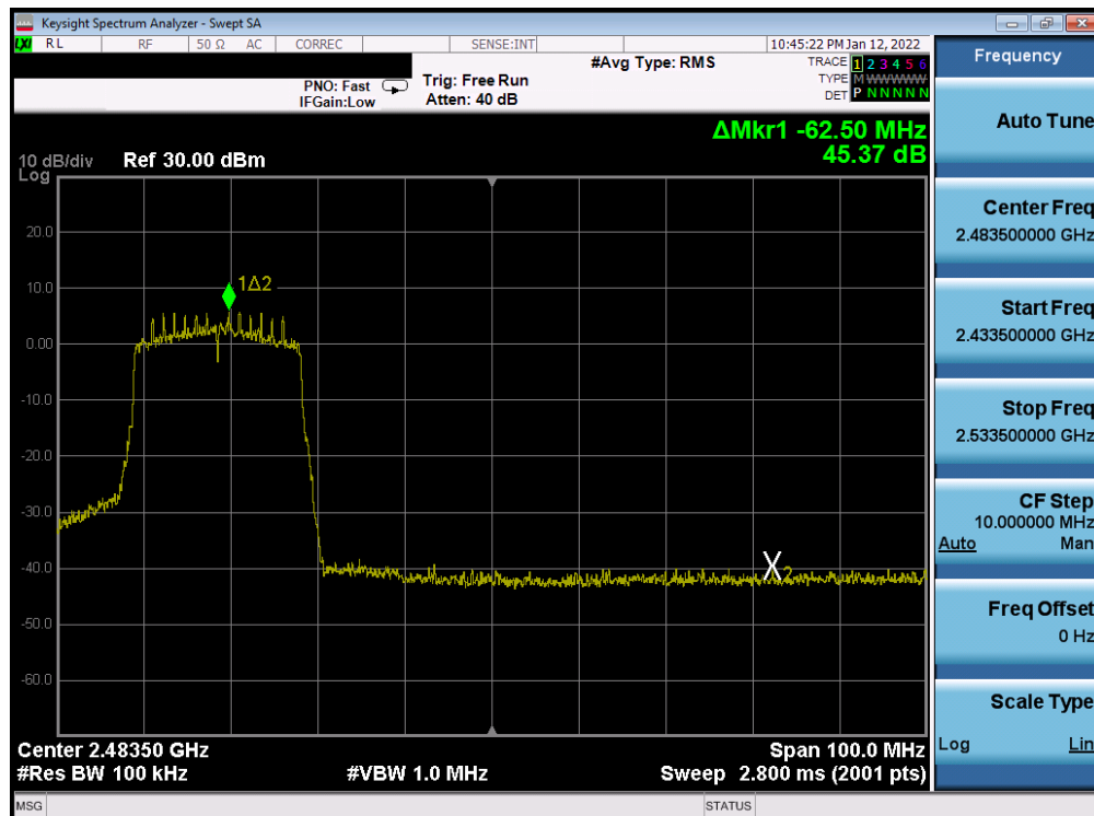
Plot 7-212. Band Edge Plot Antenna WF8 (802.11ax (SU - 2.4GHz) – Ch. 9) – MCS0
