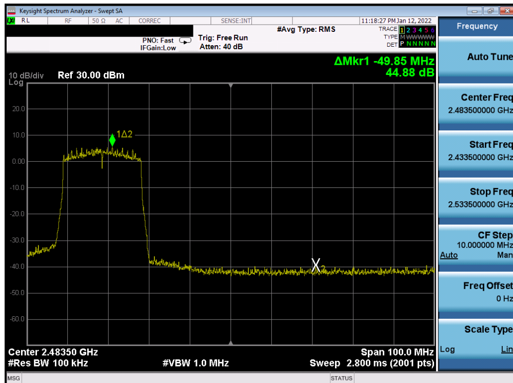
Plot 7-253. Band Edge Plot Antenna WF8 (802.11ax (SU - 2.4GHz) – Ch. 9) – MCS3
