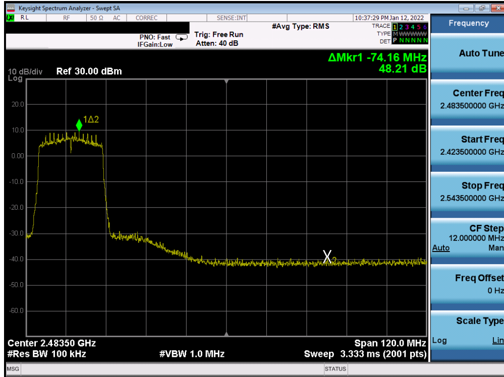
Plot 7-209. Band Edge Plot Antenna WF8 (802.11ax (SU - 2.4GHz) – Ch. 6 (high)) – MCS0
