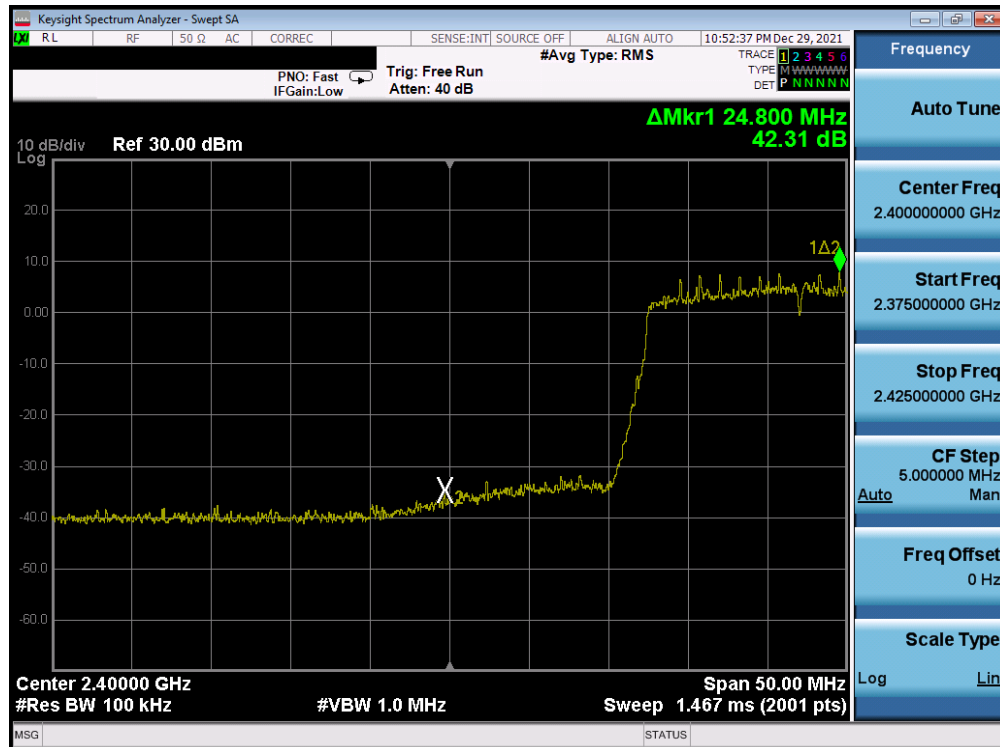
Plot 7-205. Band Edge Plot Antenna WF8 (802.11ax (SU - 2.4GHz) – Ch. 3) – MCS0
