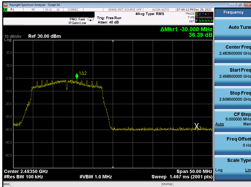
Plot 7-202. Band Edge Plot Antenna WF8 (802.11n (2.4GHz) – Ch. 13) – MCS0
