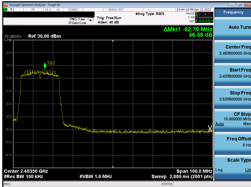
Plot 7-211. Band Edge Plot Antenna WF8 (802.11ax (SU - 2.4GHz) – Ch. 8) – MCS0
