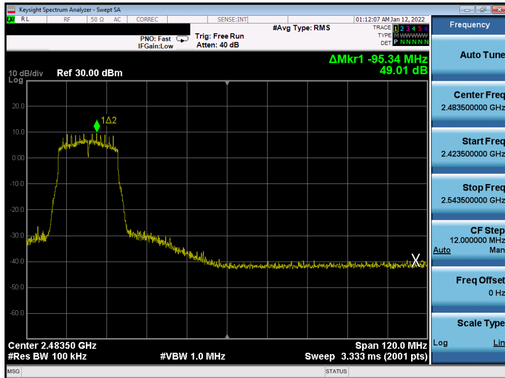
Plot 7-196. Band Edge Plot Antenna WF8 (802.11n (2.4GHz) – Ch. 7) – MCS0
