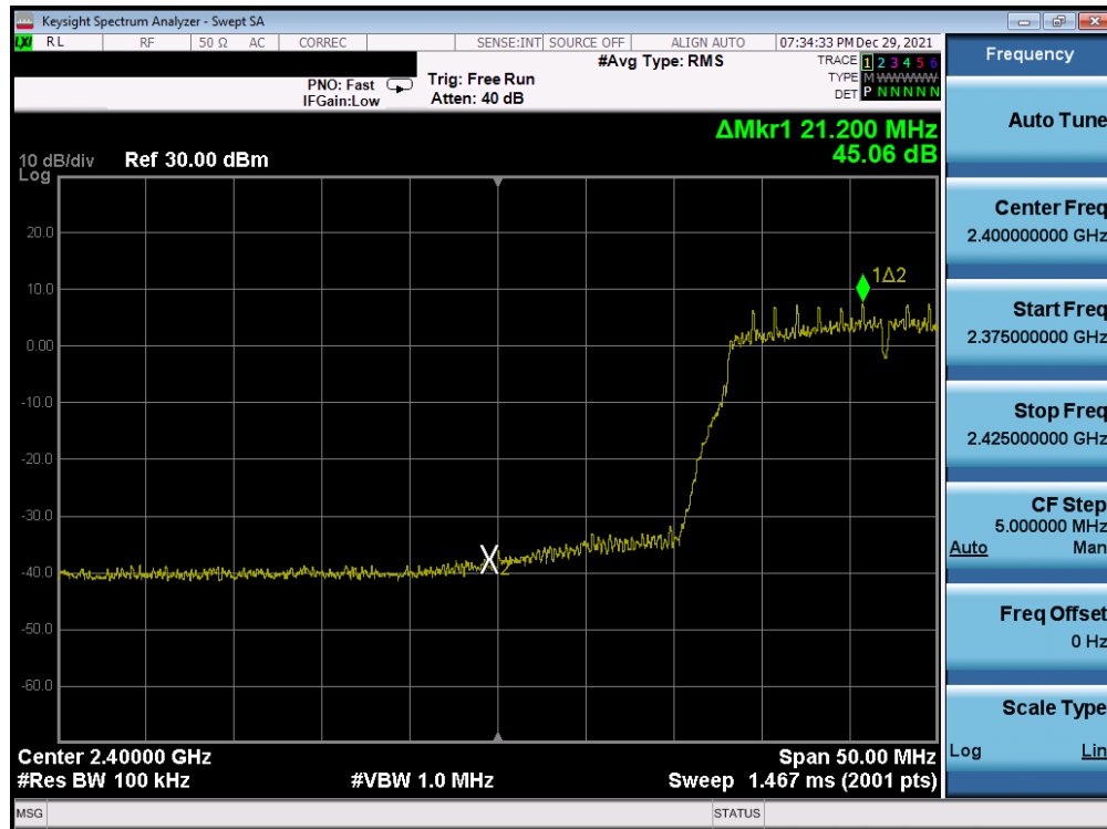
Plot 7-191. Band Edge Plot Antenna WF8 (802.11n (2.4GHz) – Ch. 3) – MCS0
