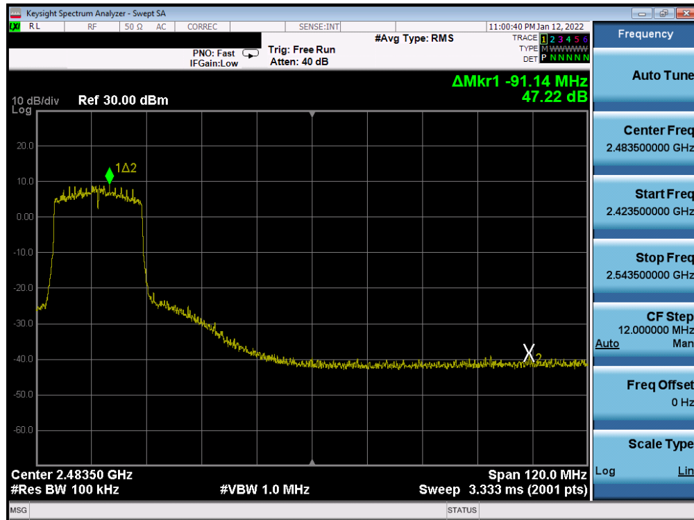
Plot 7-250. Band Edge Plot Antenna WF8 (802.11ax (SU - 2.4GHz) – Ch. 6 (high)) – MCS3
