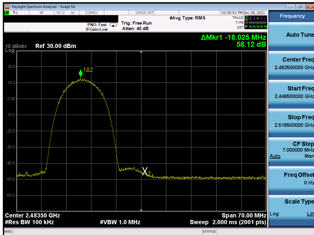
Plot 7-264. Band Edge Plot Antenna WF8 (802.11b - Ch. 12) - 11Mbps
