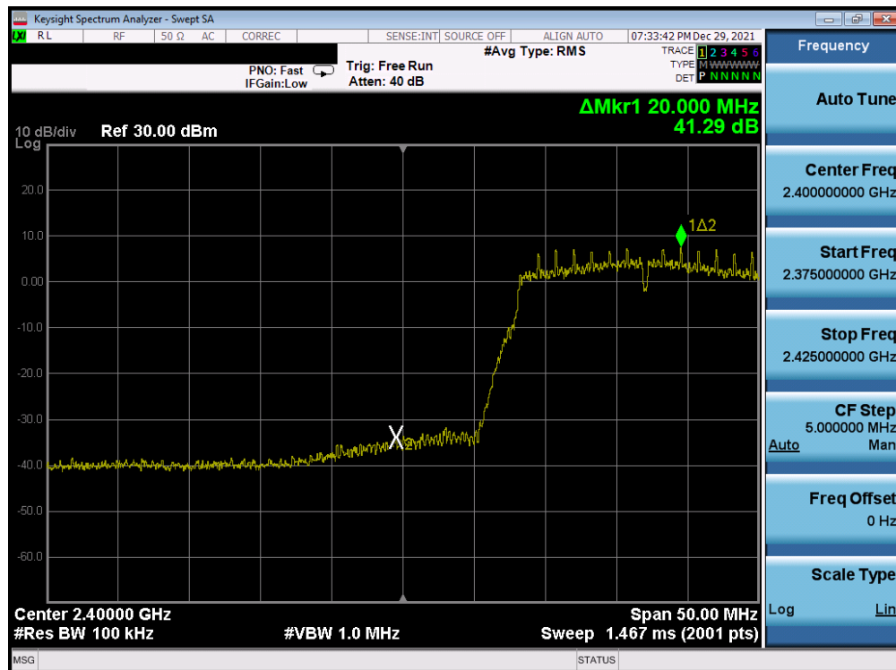
Plot 7-190. Band Edge Plot Antenna WF8 (802.11n (2.4GHz) – Ch. 2) – MCS0
