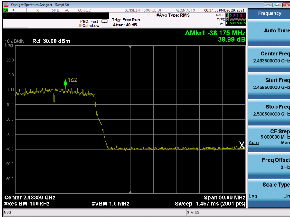
Plot 7-242. Band Edge Plot Antenna WF8 (802.11n (2.4GHz) – Ch. 12) – MCS3
