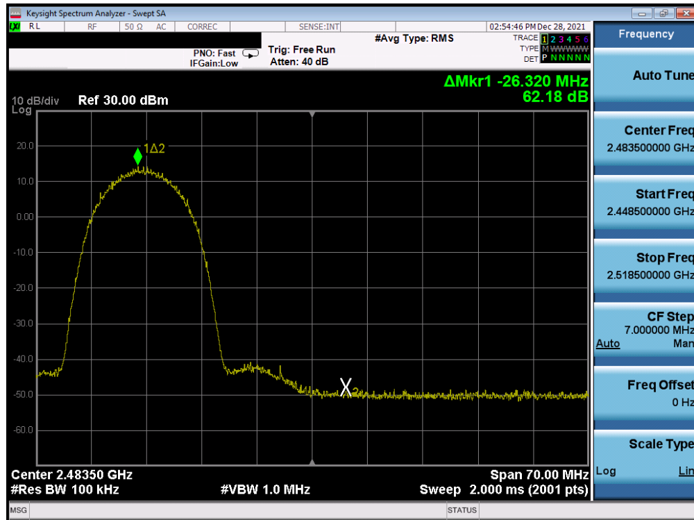
Plot 7-263. Band Edge Plot Antenna WF8 (802.11b - Ch. 11) - 11Mbps
