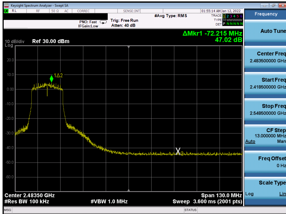
Plot 7-236. Band Edge Plot Antenna WF8 (802.11n (2.4GHz) – Ch. 6 (high)) – MCS3
