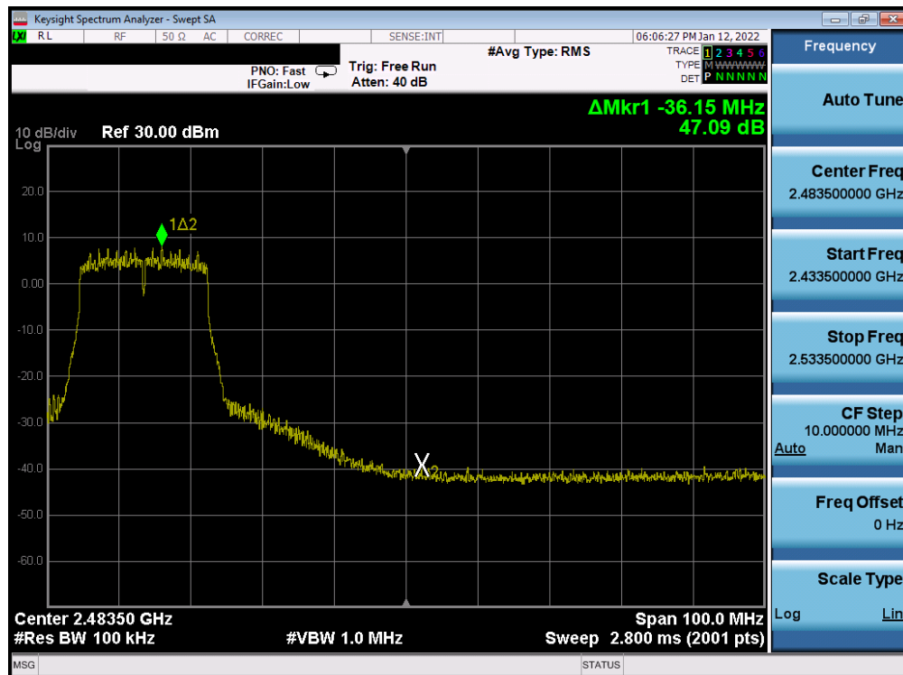
Plot 7-288. Band Edge Plot Antenna WF8 (802.11n (2.4GHz) - Ch. 8) - MCS5
