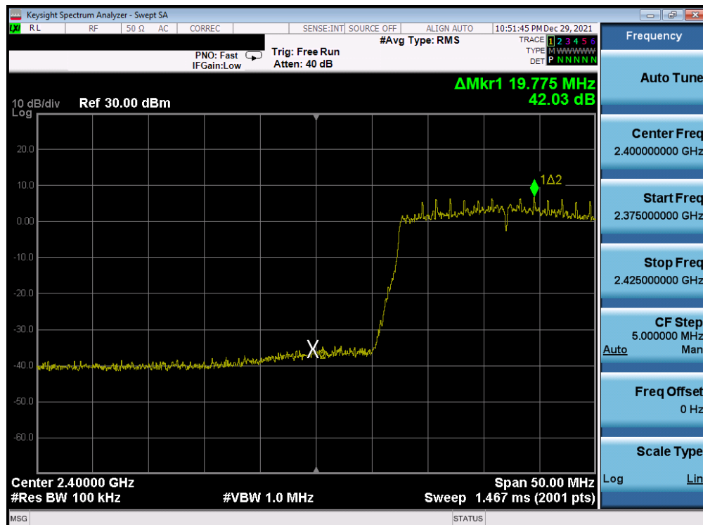
Plot 7-204. Band Edge Plot Antenna WF8 (802.11ax (SU - 2.4GHz) – Ch. 2) – MCS0
