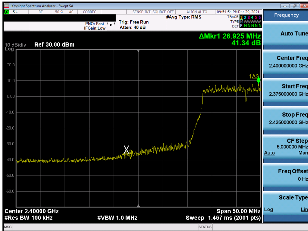
Plot 7-282. Band Edge Plot Antenna WF8 (802.11n (2.4GHz) – Ch. 3) – MCS5
