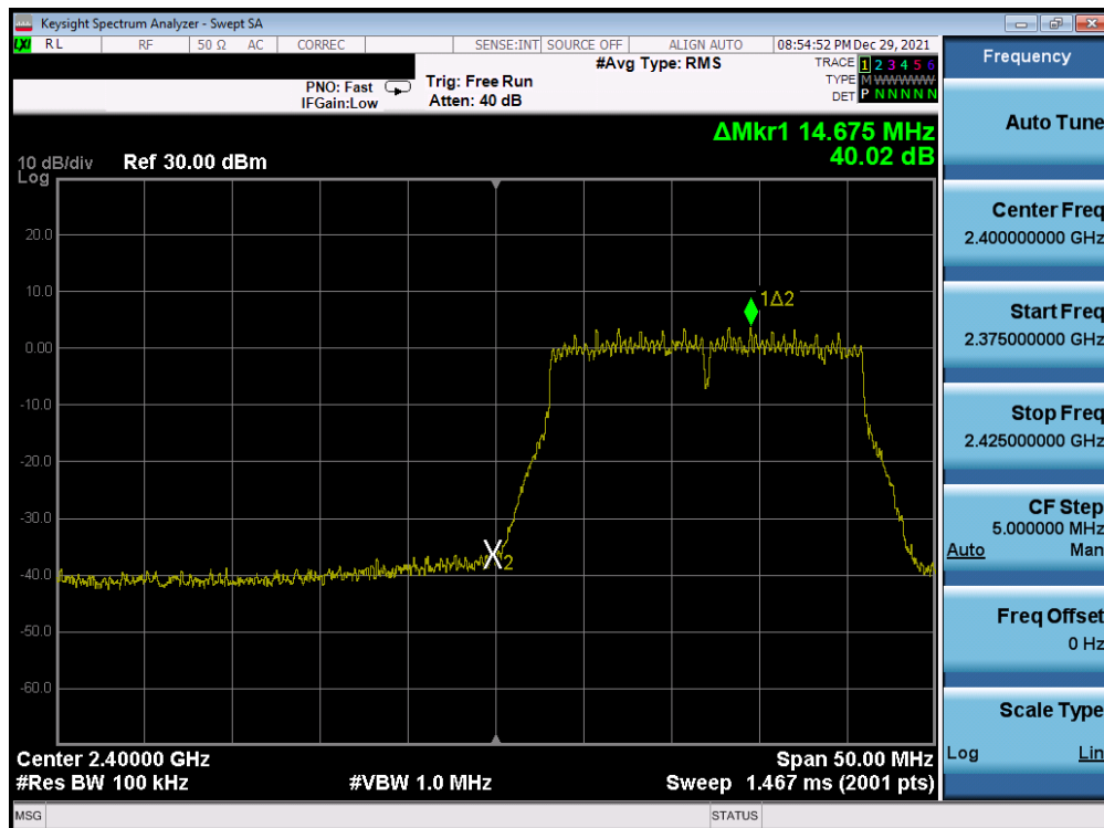
Plot 7-280. Band Edge Plot Antenna WF8 (802.11n (2.4GHz) – Ch. 1) – MCS5
