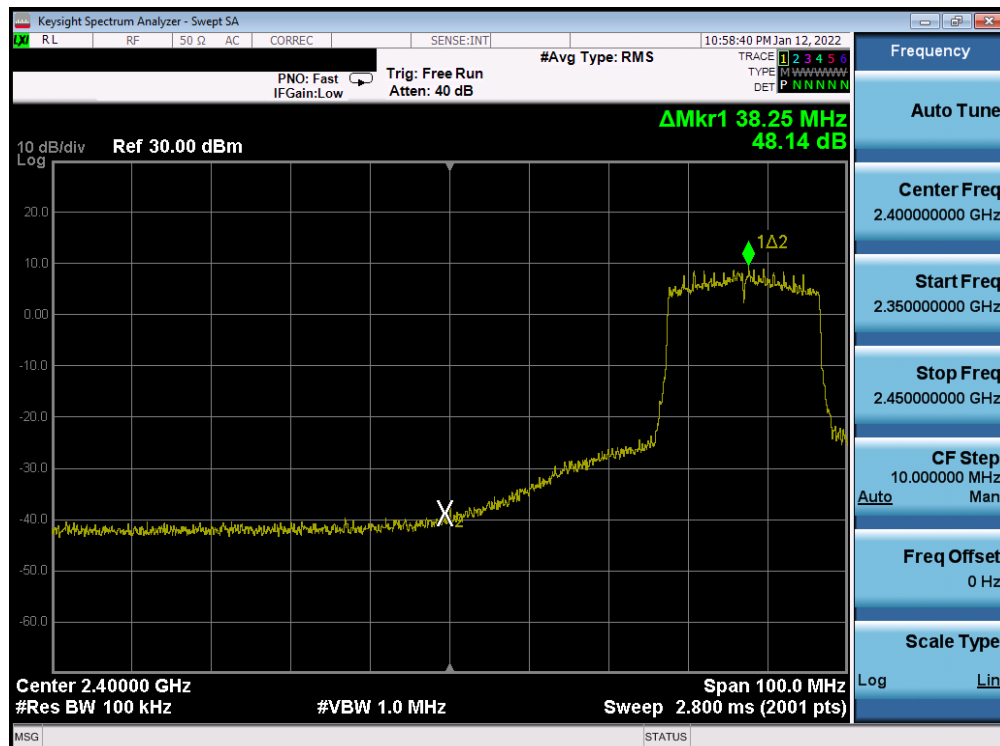
Plot 7-249. Band Edge Plot Antenna WF8 (802.11ax (SU - 2.4GHz) – Ch. 6 (low)) – MCS3
