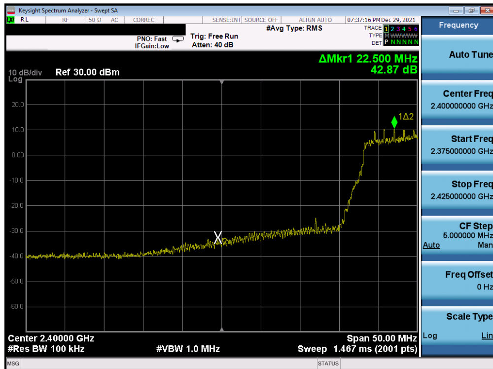
Plot 7-192. Band Edge Plot Antenna WF8 (802.11n (2.4GHz) – Ch. 4) – MCS0
