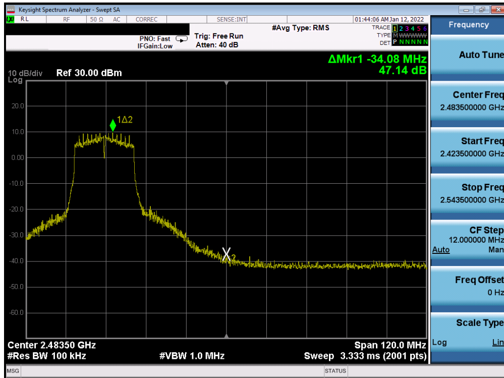
Plot 7-238. Band Edge Plot Antenna WF8 (802.11n (2.4GHz) - Ch. 8) - MCS3
