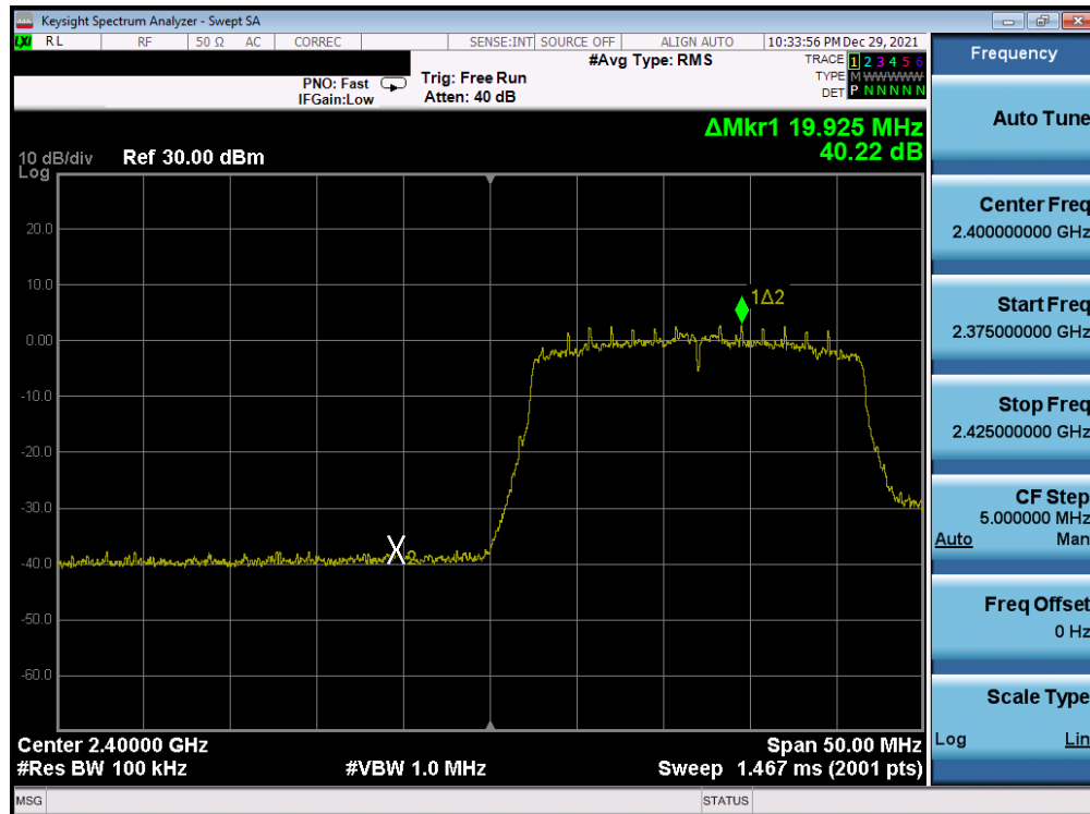
Plot 7-203. Band Edge Plot Antenna WF8 (802.11ax (SU - 2.4GHz) – Ch. 1) – MCS0
