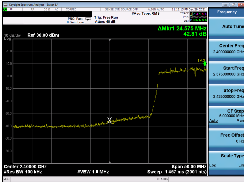
Plot 7-246. Band Edge Plot Antenna WF8 (802.11ax (SU - 2.4GHz) – Ch. 3) – MCS3
