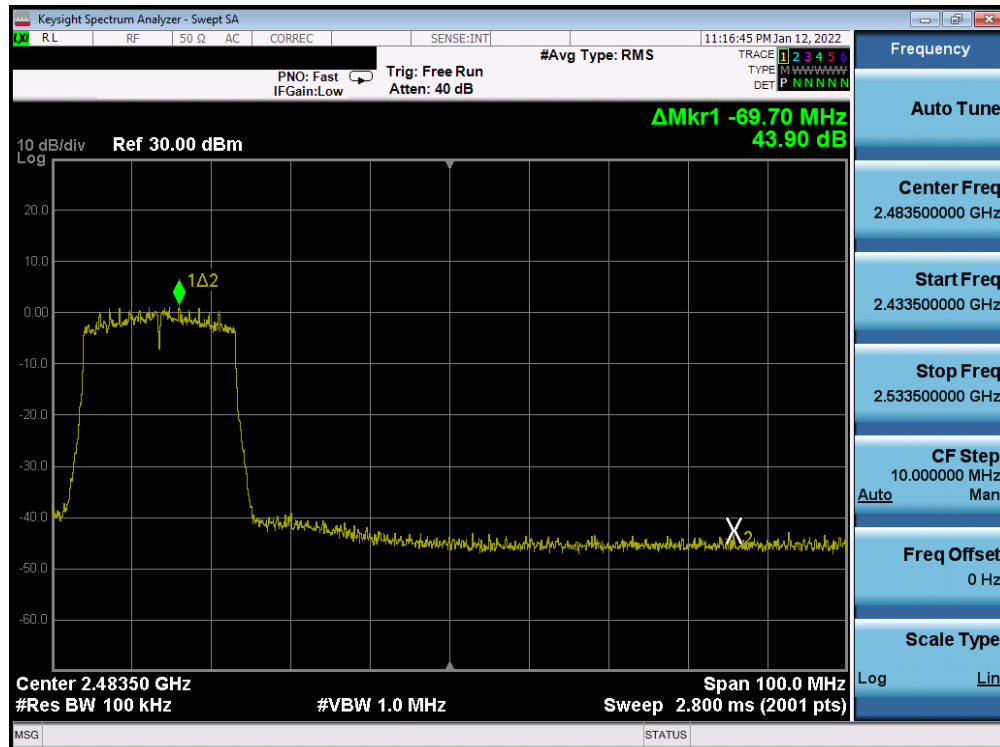
Plot 7-252. Band Edge Plot Antenna WF8 (802.11ax (SU - 2.4GHz) – Ch. 8) – MCS3
