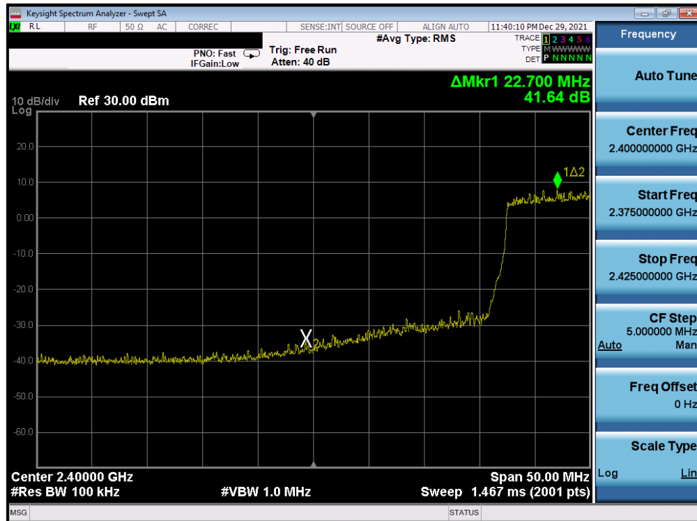
Plot 7-297. Band Edge Plot Antenna WF8 (802.11ax (SU - 2.4GHz) – Ch. 4) – MCS5
