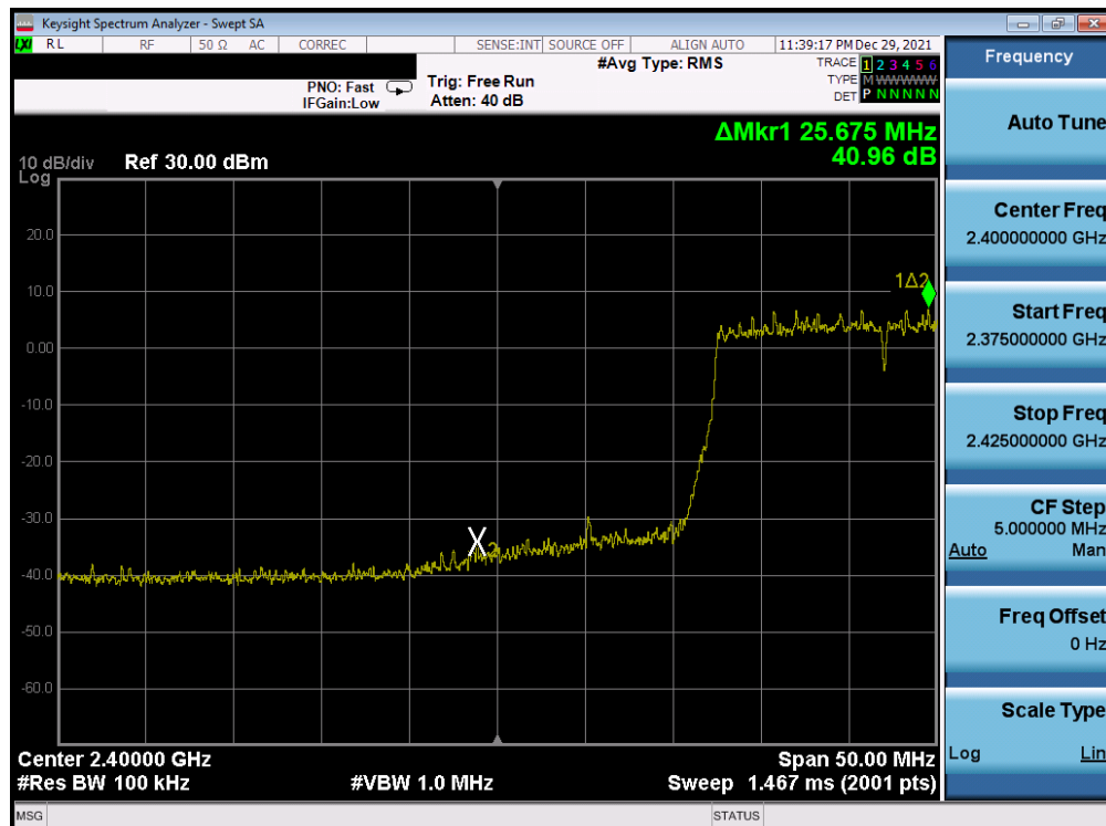
Plot 7-296. Band Edge Plot Antenna WF8 (802.11ax (SU - 2.4GHz) – Ch. 3) – MCS5
