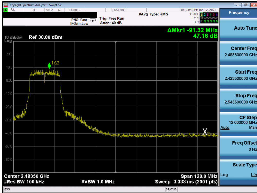
Plot 7-287. Band Edge Plot Antenna WF8 (802.11n (2.4GHz) - Ch. 7) - MCS5
