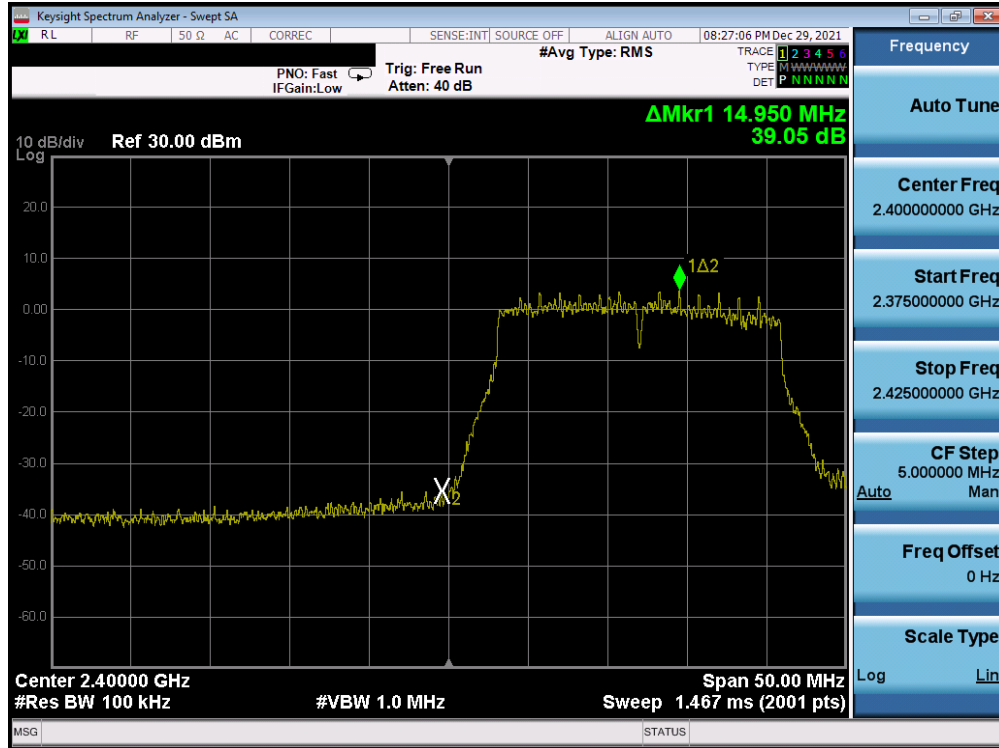
Plot 7-230. Band Edge Plot Antenna WF8 (802.11n (2.4GHz) - Ch. 1) - MCS3
