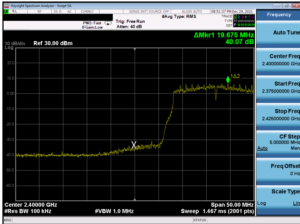
Plot 7-231. Band Edge Plot Antenna WF8 (802.11n (2.4GHz) - Ch. 2) - MCS3
