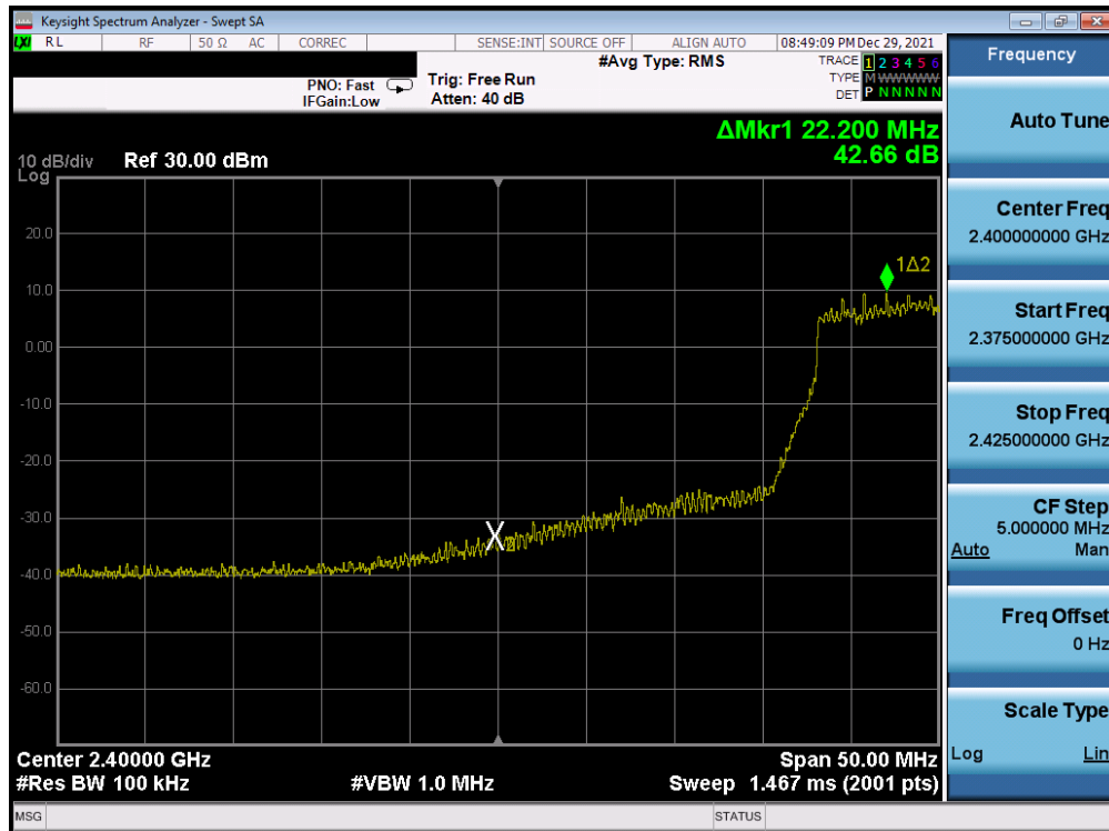
Plot 7-233. Band Edge Plot Antenna WF8 (802.11n (2.4GHz) – Ch. 4) – MCS3
