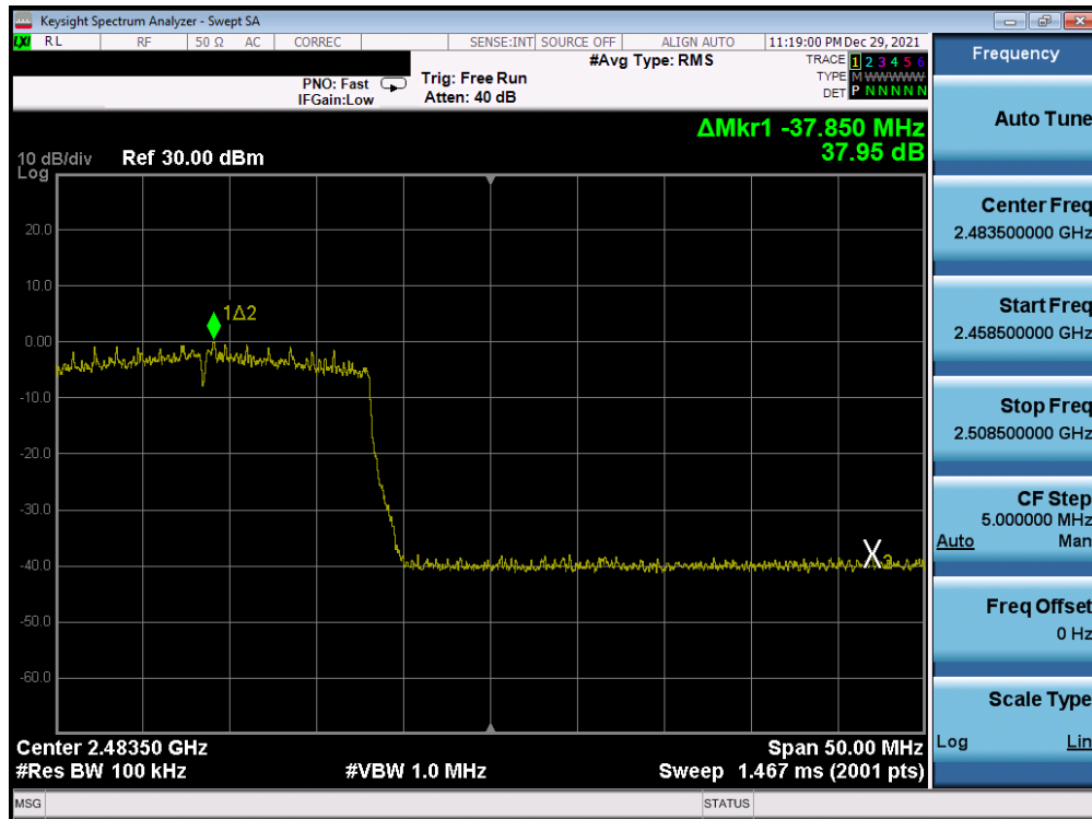
Plot 7-256. Band Edge Plot Antenna WF8 (802.11ax (SU - 2.4GHz) – Ch. 12) – MCS3
