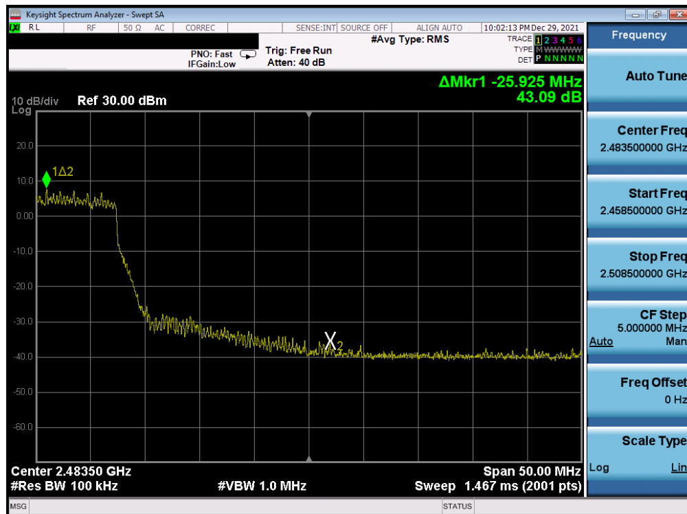
Plot 7-290. Band Edge Plot Antenna WF8 (802.11n (2.4GHz) - Ch. 10) - MCS5
