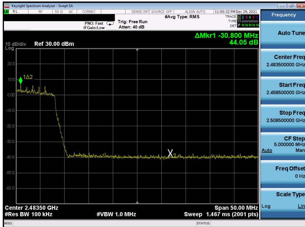
Plot 7-213. Band Edge Plot Antenna WF8 (802.11ax (SU - 2.4GHz) – Ch. 10) – MCS0
