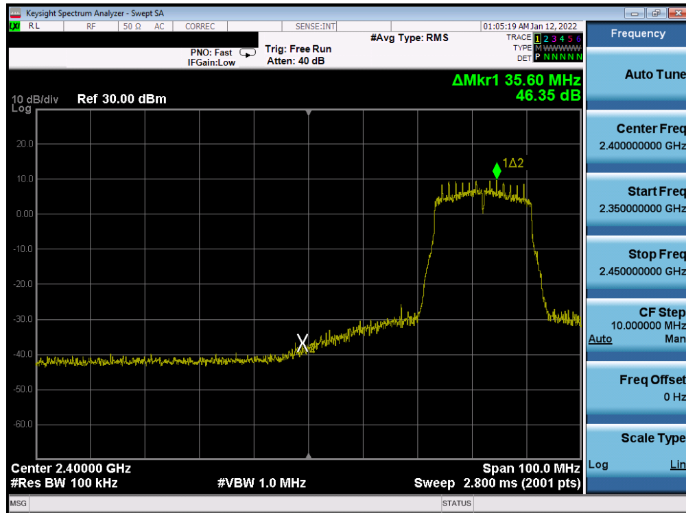
Plot 7-193. Band Edge Plot Antenna WF8 (802.11n (2.4GHz) – Ch. 5) – MCS0
