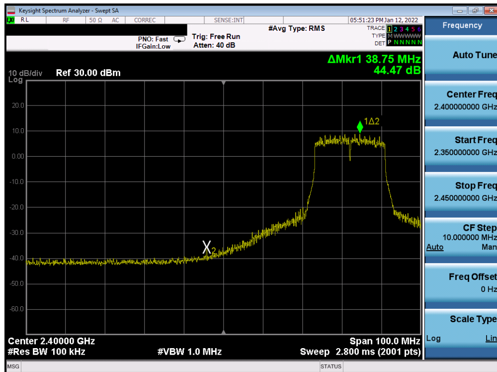
Plot 7-284. Band Edge Plot Antenna WF8 (802.11n (2.4GHz) – Ch. 5) – MCS5
