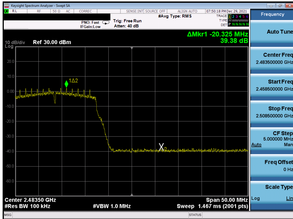
Plot 7-201. Band Edge Plot Antenna WF8 (802.11n (2.4GHz) – Ch. 12) – MCS0
