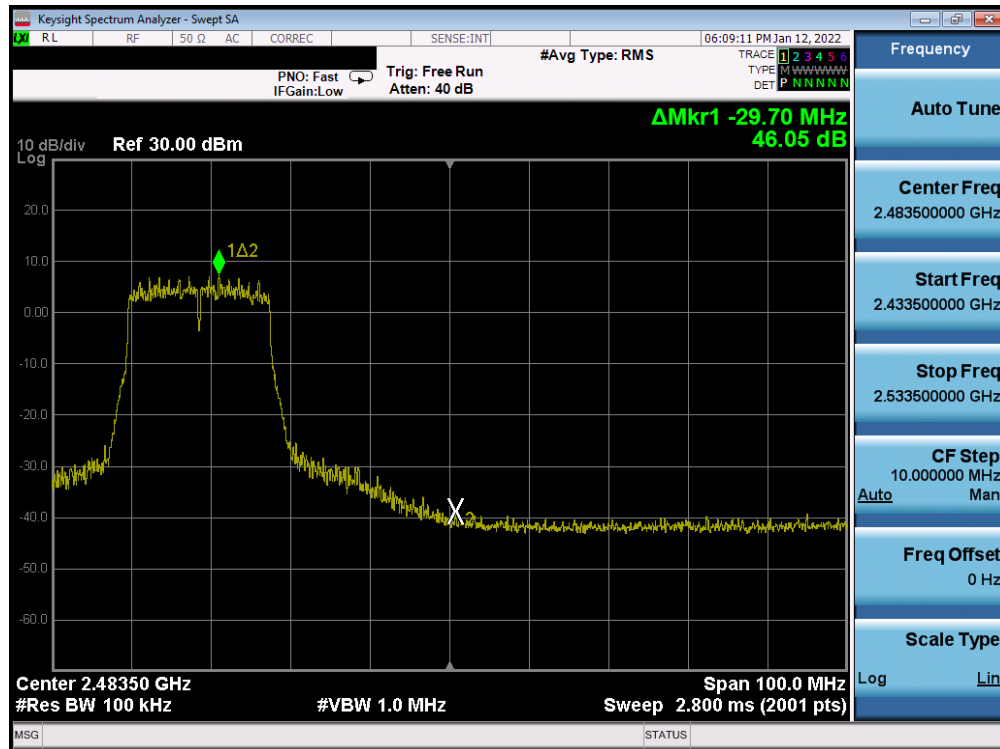
Plot 7-289. Band Edge Plot Antenna WF8 (802.11n (2.4GHz) - Ch. 9) - MCS5
