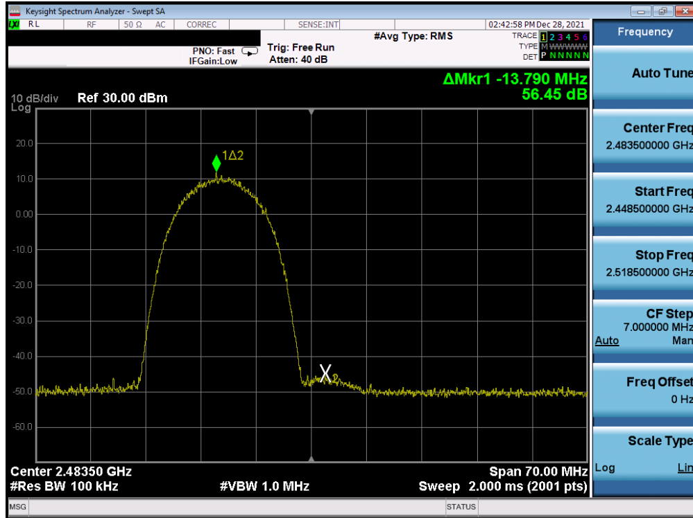
Plot 7-265. Band Edge Plot Antenna WF8 (802.11b – Ch. 13) – 11Mbps
