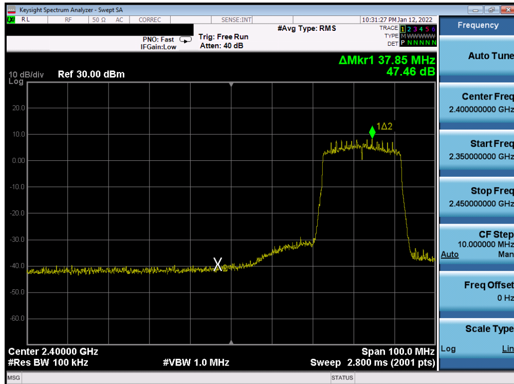
Plot 7-207. Band Edge Plot Antenna WF8 (802.11ax (SU - 2.4GHz) – Ch. 5) – MCS0
