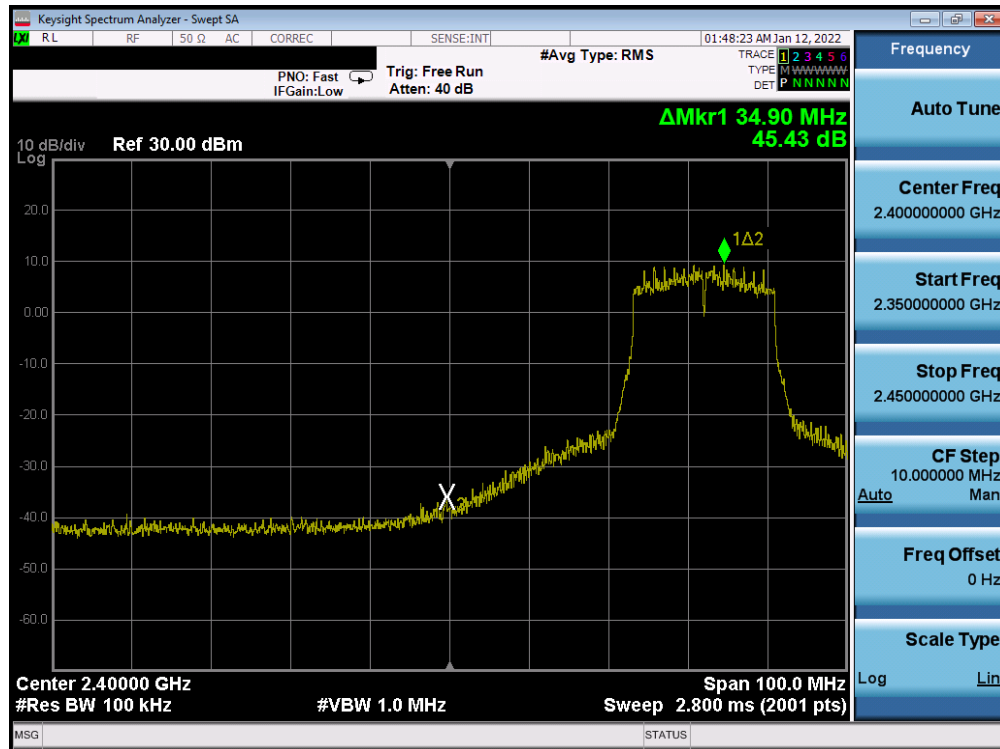
Plot 7-234. Band Edge Plot Antenna WF8 (802.11n (2.4GHz) – Ch. 5) – MCS3
