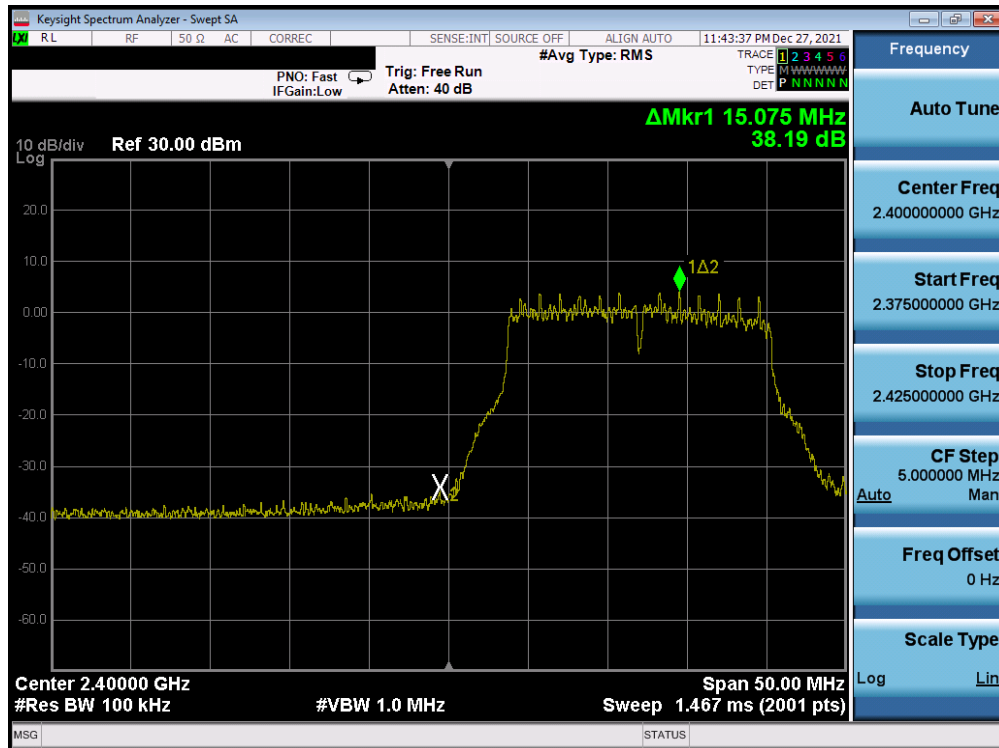
Plot 7-266. Band Edge Plot Antenna WF8 (802.11g – Ch. 1) – 36Mbps
