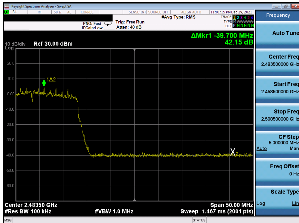
Plot 7-214. Band Edge Plot Antenna WF8 (802.11ax (SU - 2.4GHz) – Ch. 11) – MCS0
