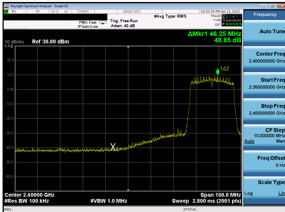
Plot 7-208. Band Edge Plot Antenna WF8 (802.11ax (SU - 2.4GHz) – Ch. 6 (low)) – MCS0
