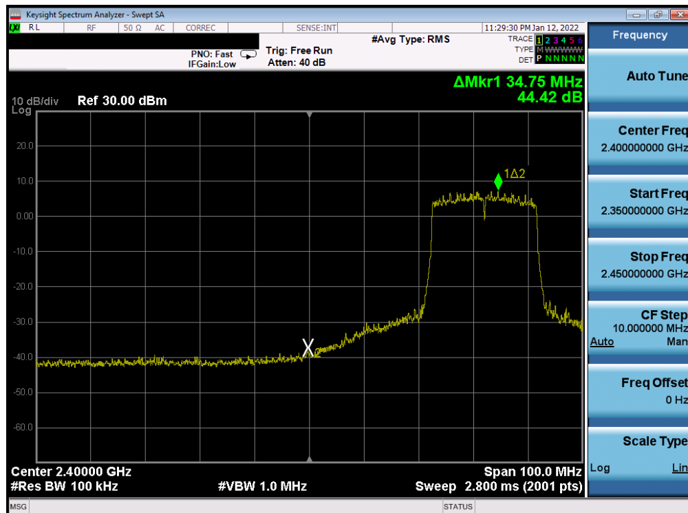
Plot 7-298. Band Edge Plot Antenna WF8 (802.11ax (SU - 2.4GHz) – Ch. 5) – MCS5
