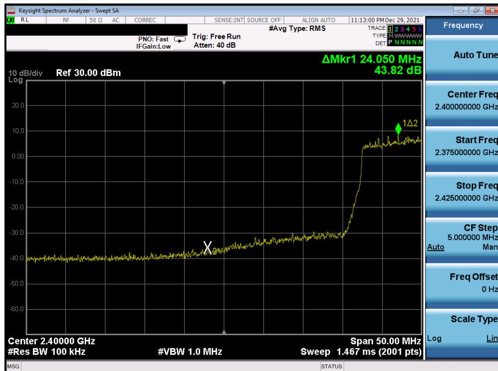
Plot 7-247. Band Edge Plot Antenna WF8 (802.11ax (SU - 2.4GHz) – Ch. 4) – MCS3
