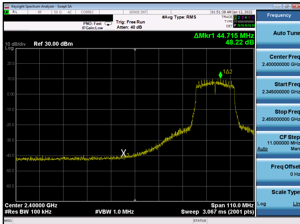
Plot 7-235. Band Edge Plot Antenna WF8 (802.11n (2.4GHz) – Ch. 6 (low)) – MCS3
