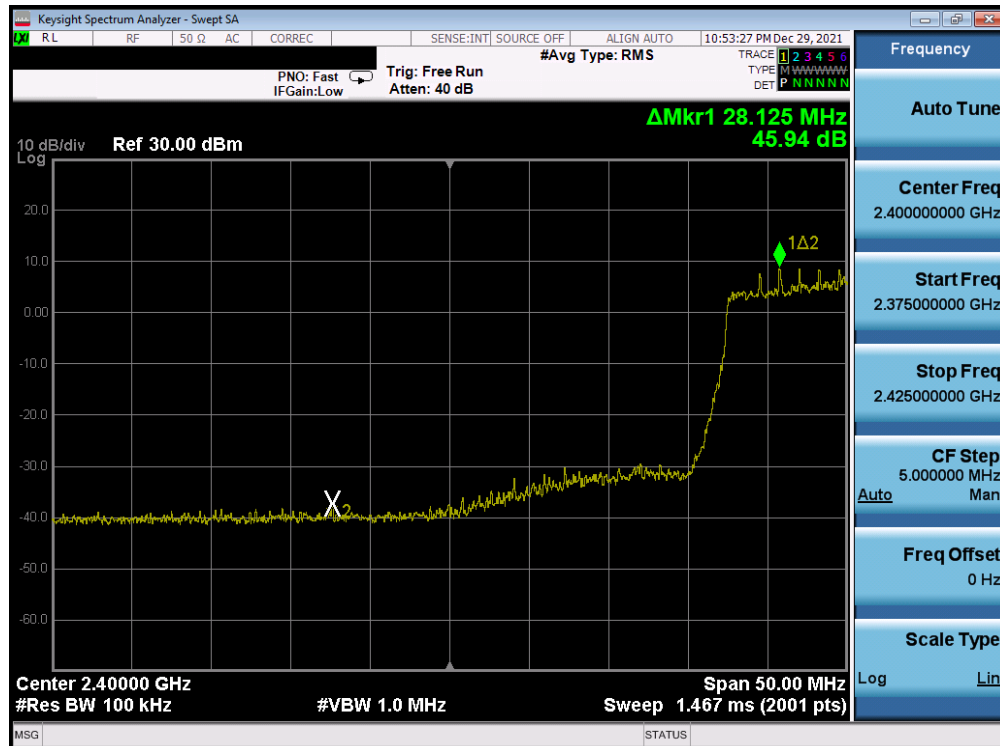
Plot 7-206. Band Edge Plot Antenna WF8 (802.11ax (SU - 2.4GHz) – Ch. 4) – MCS0
