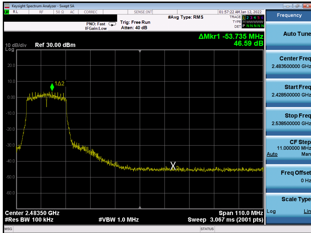
Plot 7-237. Band Edge Plot Antenna WF8 (802.11n (2.4GHz) – Ch. 7) – MCS3
