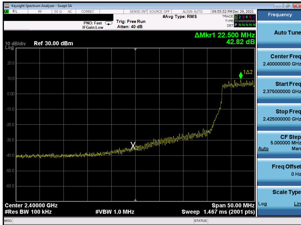
Plot 7-283. Band Edge Plot Antenna WF8 (802.11n (2.4GHz) – Ch. 4) – MCS5
