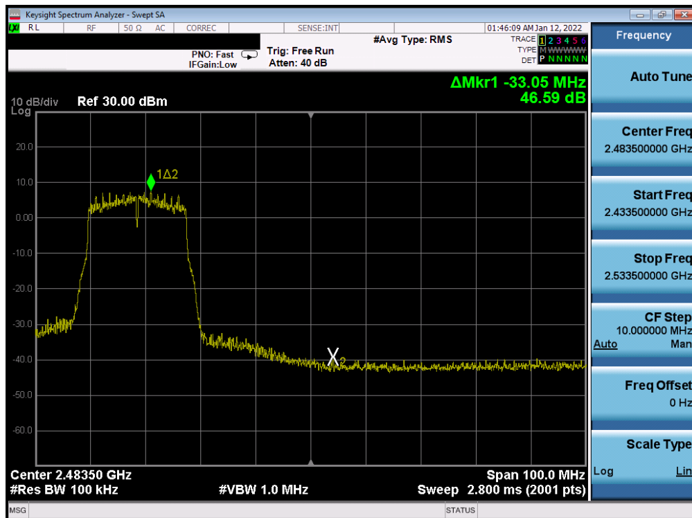
Plot 7-239. Band Edge Plot Antenna WF8 (802.11n (2.4GHz) - Ch. 9) - MCS3
