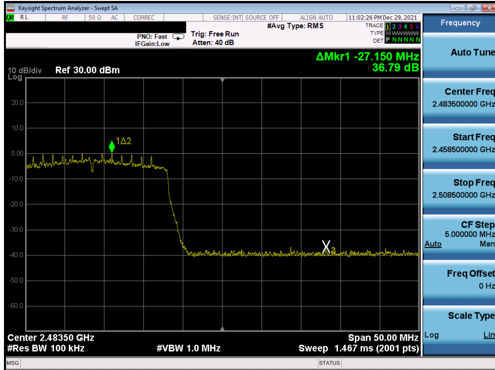
Plot 7-215. Band Edge Plot Antenna WF8 (802.11ax (SU - 2.4GHz) – Ch. 12) – MCS0
