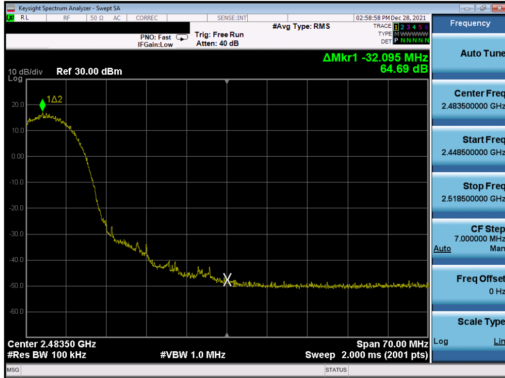
Plot 7-261. Band Edge Plot Antenna WF8 (802.11b - Ch. 9) - 11Mbps
