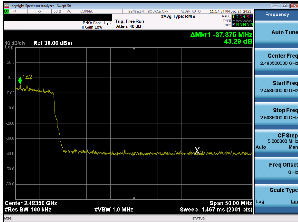
Plot 7-254. Band Edge Plot Antenna WF8 (802.11ax (SU - 2.4GHz) – Ch. 10) – MCS3
