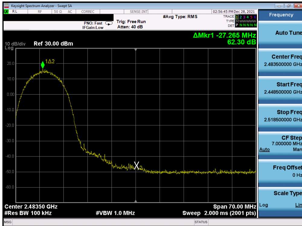
Plot 7-262. Band Edge Plot Antenna WF8 (802.11b - Ch. 10) - 11Mbps
