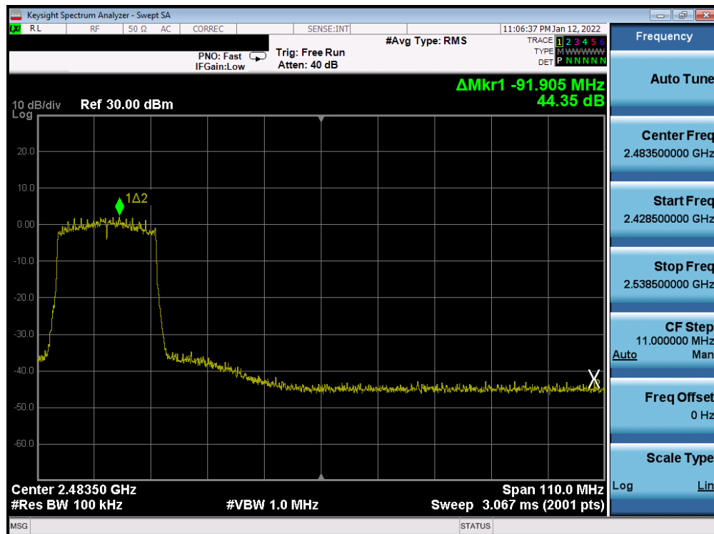
Plot 7-251. Band Edge Plot Antenna WF8 (802.11ax (SU - 2.4GHz) – Ch. 7) – MCS3
