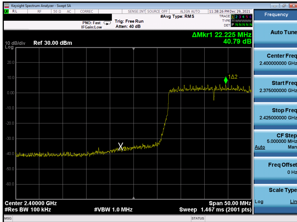
Plot 7-295. Band Edge Plot Antenna WF8 (802.11ax (SU - 2.4GHz) – Ch. 2) – MCS5
