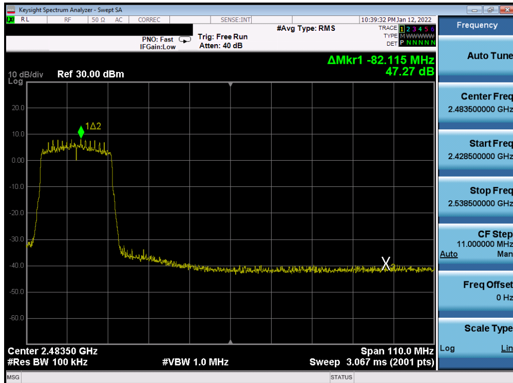
Plot 7-210. Band Edge Plot Antenna WF8 (802.11ax (SU - 2.4GHz) – Ch. 7) – MCS0
