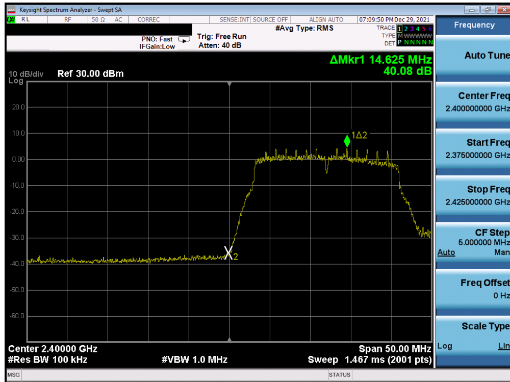
Plot 7-189. Band Edge Plot Antenna WF8 (802.11n (2.4GHz) – Ch. 1) – MCS0
