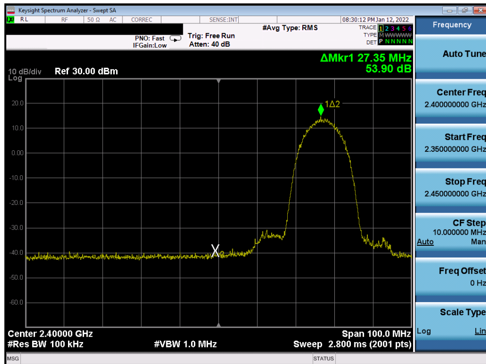
Plot 7-260. Band Edge Plot Antenna WF8 (802.11b – Ch. 4) – 11Mbps
