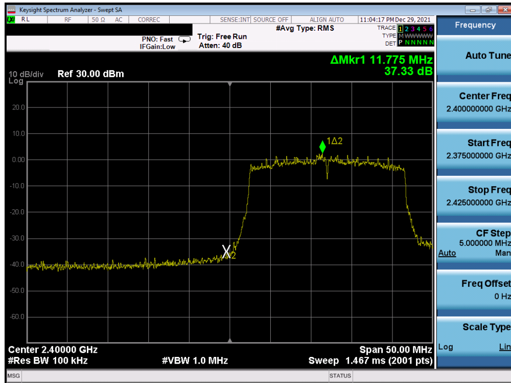
Plot 7-244. Band Edge Plot Antenna WF8 (802.11ax (SU - 2.4GHz) – Ch. 1) – MCS3
