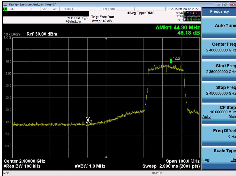
Plot 7-248. Band Edge Plot Antenna WF8 (802.11ax (SU - 2.4GHz) – Ch. 5) – MCS3
