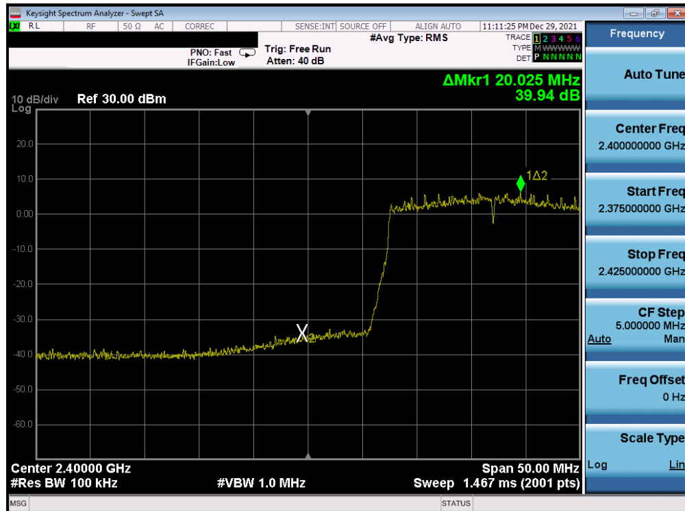
Plot 7-245. Band Edge Plot Antenna WF8 (802.11ax (SU - 2.4GHz) – Ch. 2) – MCS3
