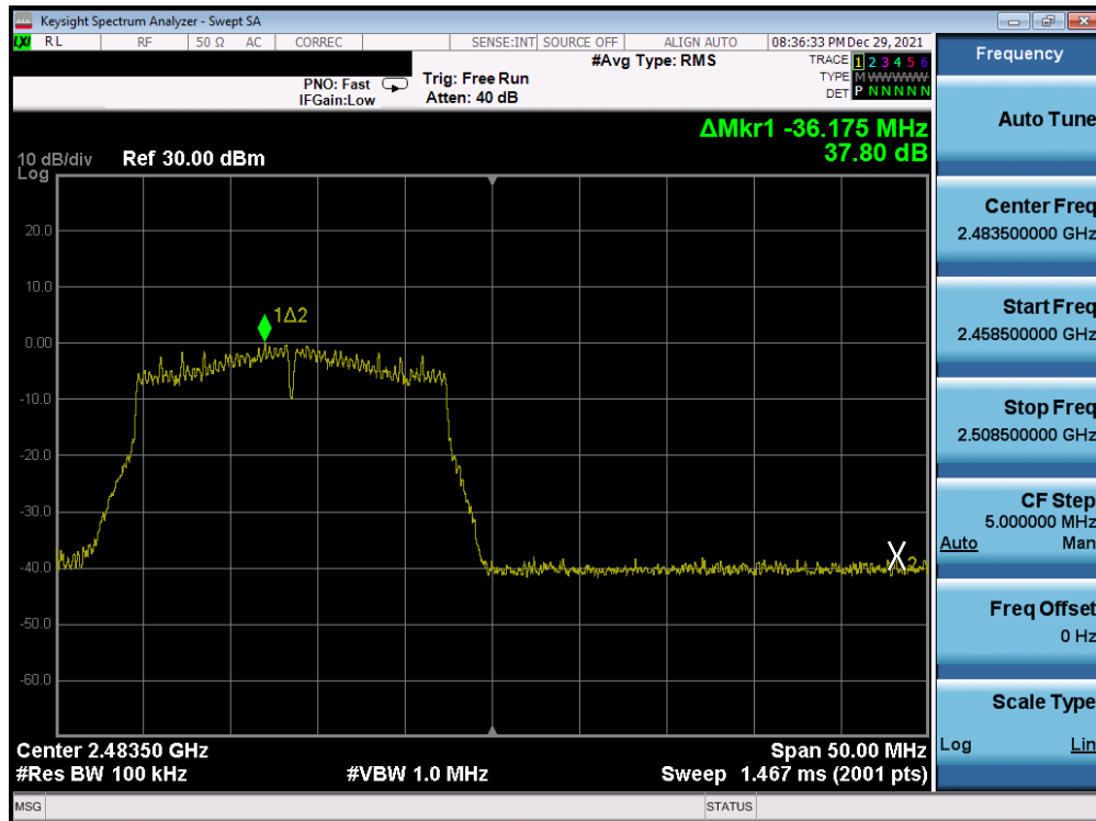
Plot 7-243. Band Edge Plot Antenna WF8 (802.11n (2.4GHz) – Ch. 13) – MCS3
