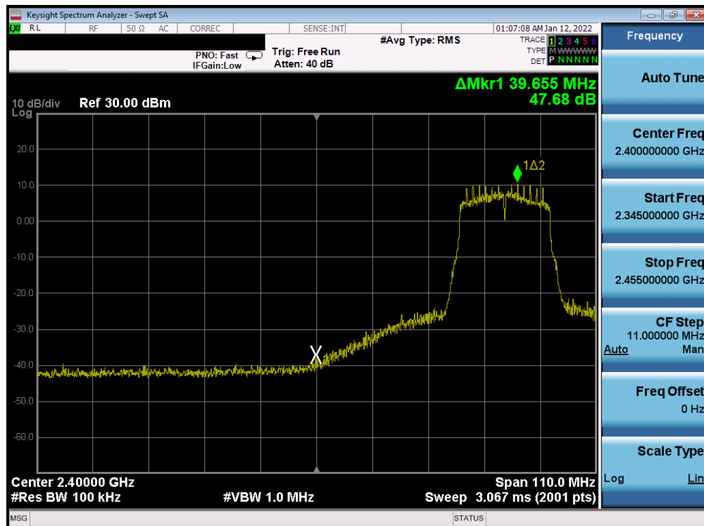
Plot 7-194. Band Edge Plot Antenna WF8 (802.11n (2.4GHz) – Ch. 6 (low)) – MCS0
