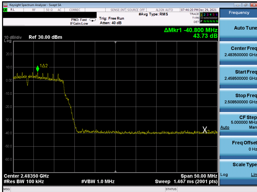
Plot 7-200. Band Edge Plot Antenna WF8 (802.11n (2.4GHz) – Ch. 11) – MCS0
