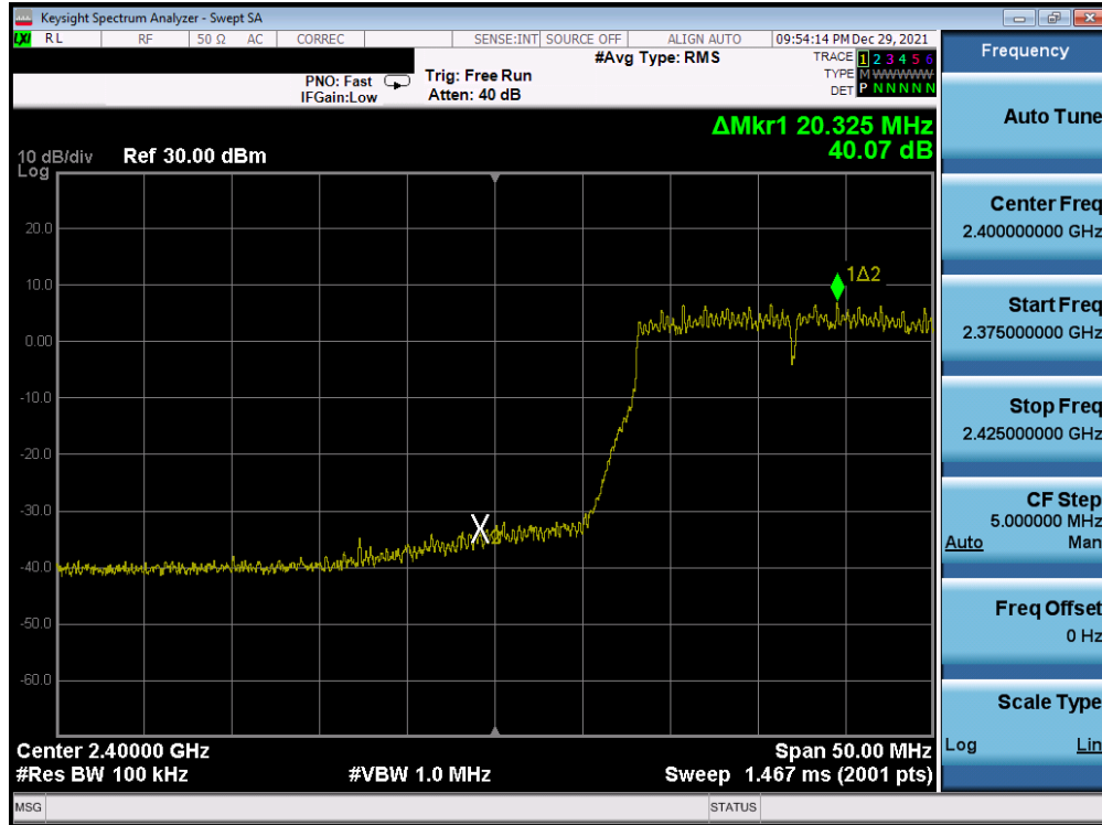
Plot 7-281. Band Edge Plot Antenna WF8 (802.11n (2.4GHz) – Ch. 2) – MCS5
