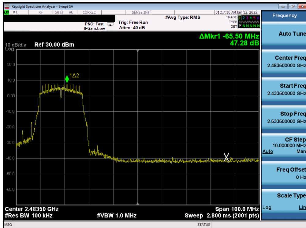
Plot 7-198. Band Edge Plot Antenna WF8 (802.11n (2.4GHz) – Ch. 9) – MCS0
