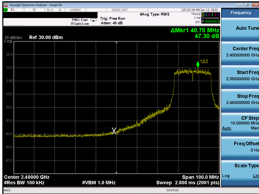
Plot 7-285. Band Edge Plot Antenna WF8 (802.11n (2.4GHz) – Ch. 6 (low)) – MCS5
