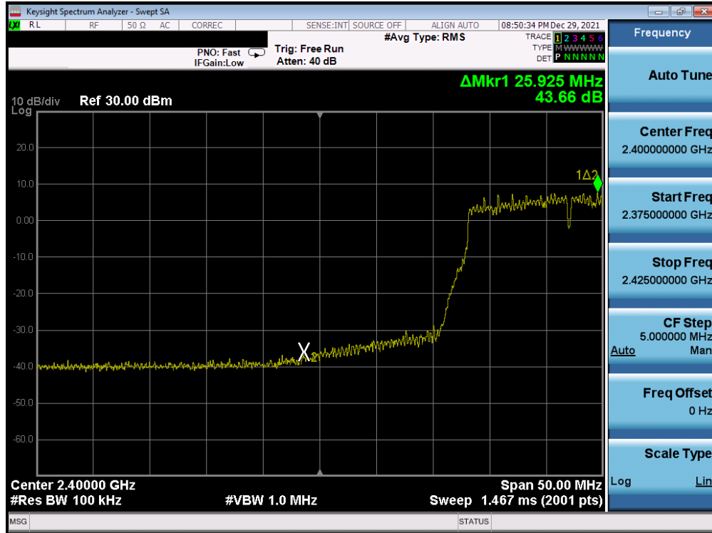
Plot 7-232. Band Edge Plot Antenna WF8 (802.11n (2.4GHz) – Ch. 3) – MCS3
