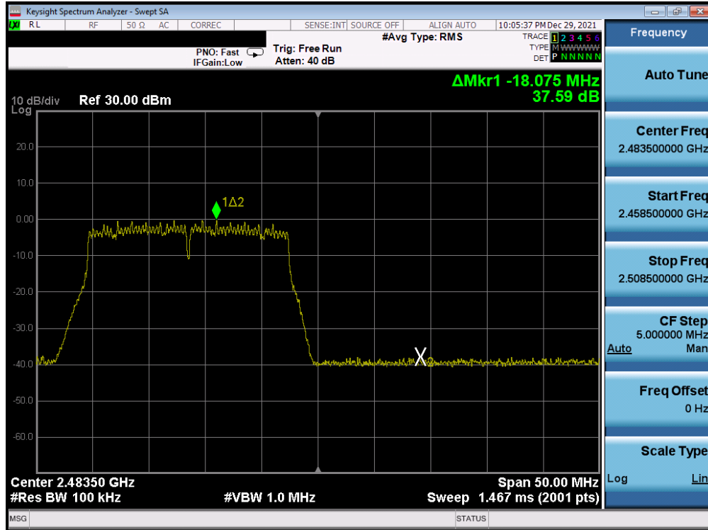
Plot 7-293. Band Edge Plot Antenna WF8 (802.11n (2.4GHz) – Ch. 13) – MCS5
