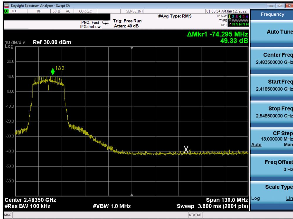
Plot 7-195. Band Edge Plot Antenna WF8 (802.11n (2.4GHz) – Ch. 6 (high)) – MCS0
