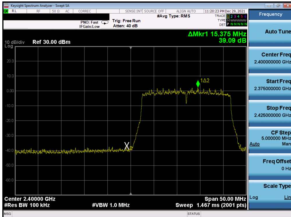
Plot 7-294. Band Edge Plot Antenna WF8 (802.11ax (SU - 2.4GHz) – Ch. 1) – MCS5
