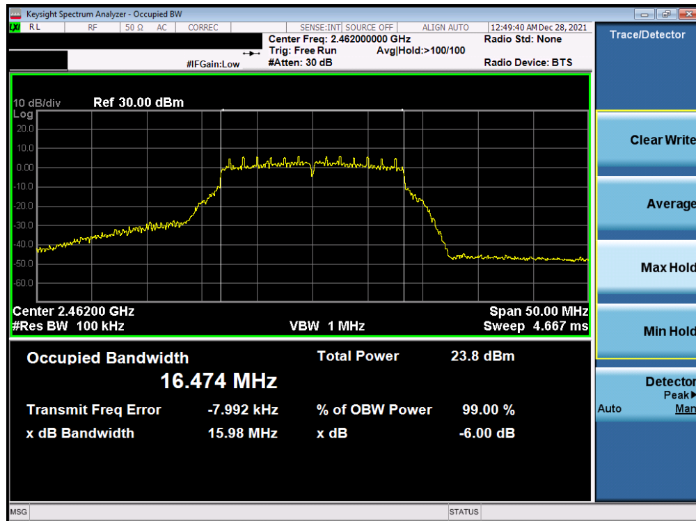
Plot 7-42. 6dB Bandwidth Plot Antenna WF7b (802.11g – Ch. 11) – 18Mbps
