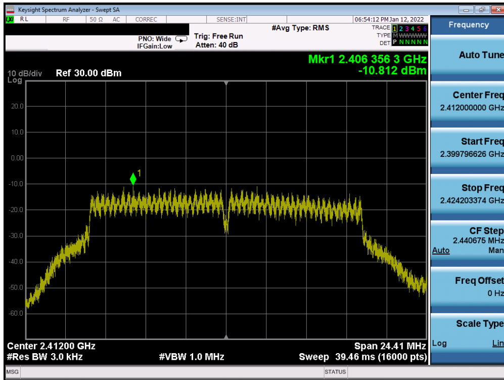
Plot 7-61. Power Spectral Density Plot Antenna WF8 (802.11g – Ch. 1) – 6Mbps
