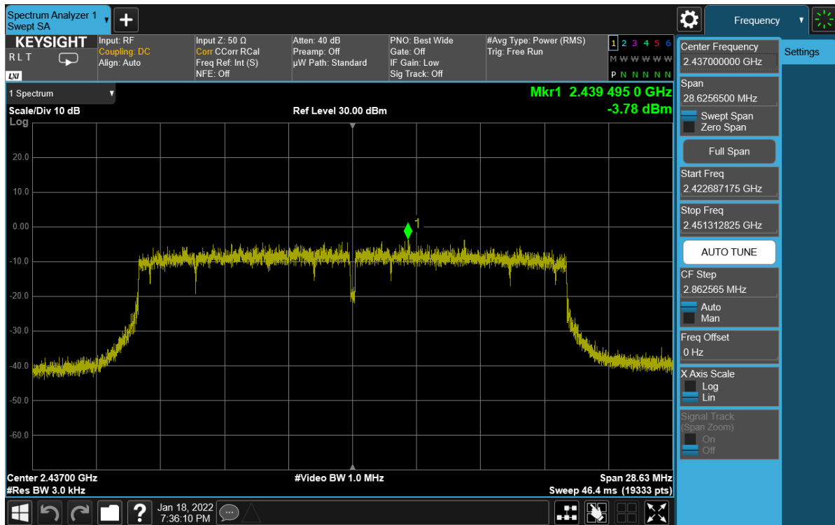
Plot 7-89. Power Spectral Density Plot Antenna WF8 (802.11ax (SU - 2.4GHz) – Ch. 6) – MCS5
