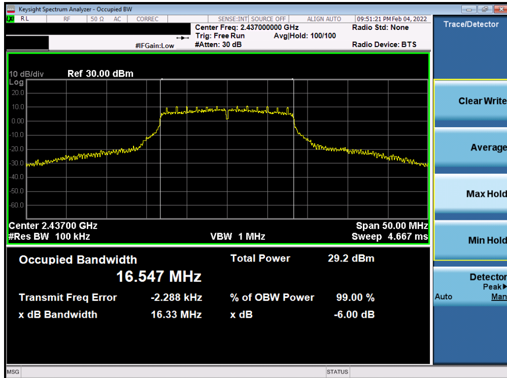
Plot 7-2. 6dB Bandwidth Plot Antenna WF8 (802.11g - Ch. 6) - 6Mbps
