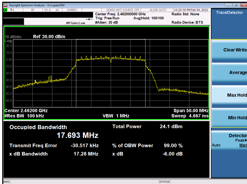
Plot 7-36. 6dB Bandwidth Plot Antenna WF7b (802.11n (2.4GHz) – Ch. 11) – MCS0
