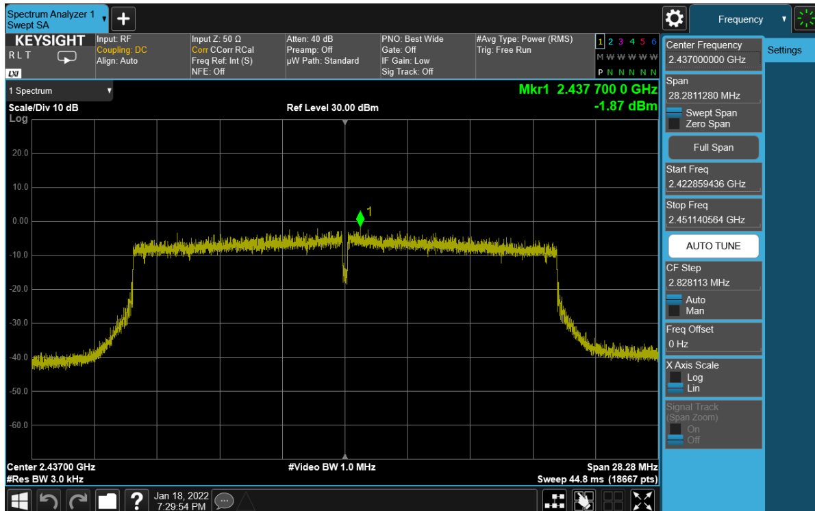
Plot 7-68. Power Spectral Density Plot Antenna WF8 (802.11ax (SU - 2.4GHz) – Ch. 6) – MCS0
