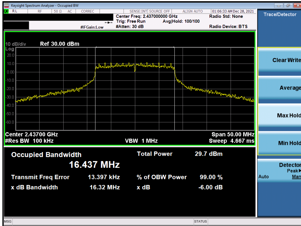
Plot 7-53. 6dB Bandwidth Plot Antenna WF7b (802.11g - Ch. 6) - 36Mbps
