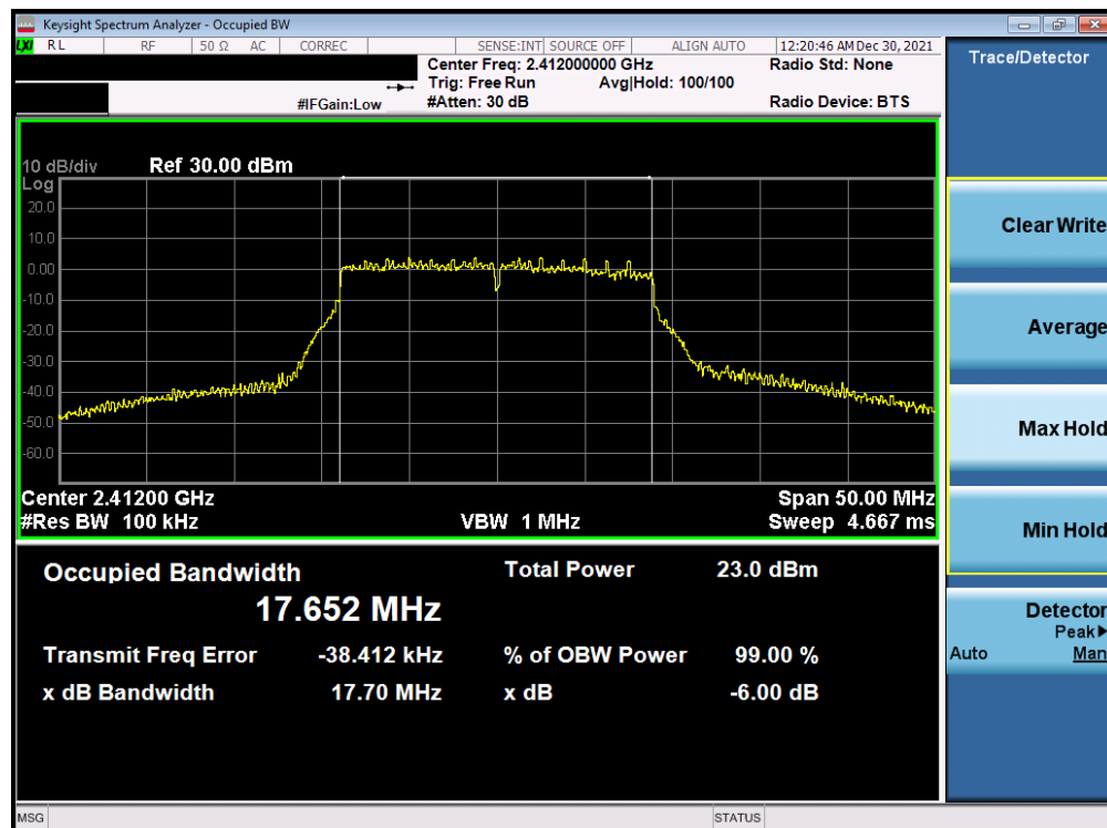
Plot 7-43. 6dB Bandwidth Plot Antenna WF7b (802.11n (2.4GHz) – Ch. 1) – MCS3
