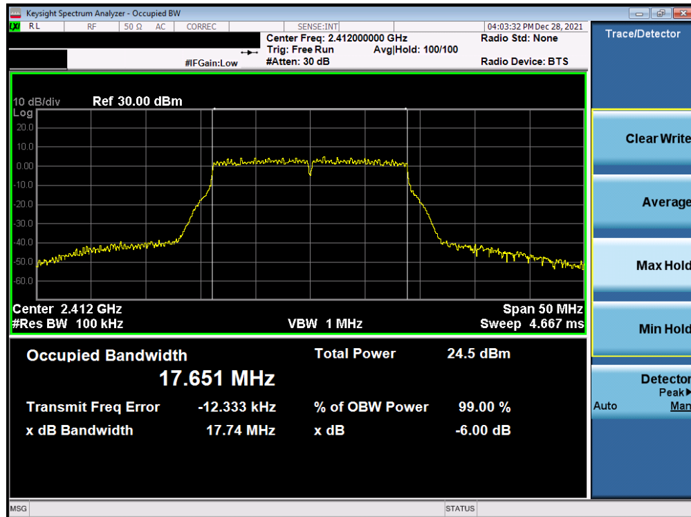
Plot 7-55. 6dB Bandwidth Plot Antenna WF7b (802.11n (2.4GHz) – Ch. 1) – MCS5
