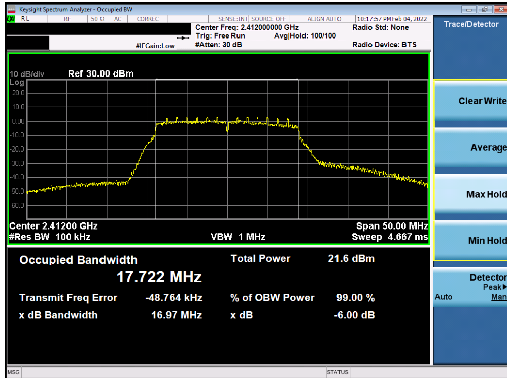
Plot 7-34. 6dB Bandwidth Plot Antenna WF7b (802.11n (2.4GHz) - Ch. 1) - MCS0
