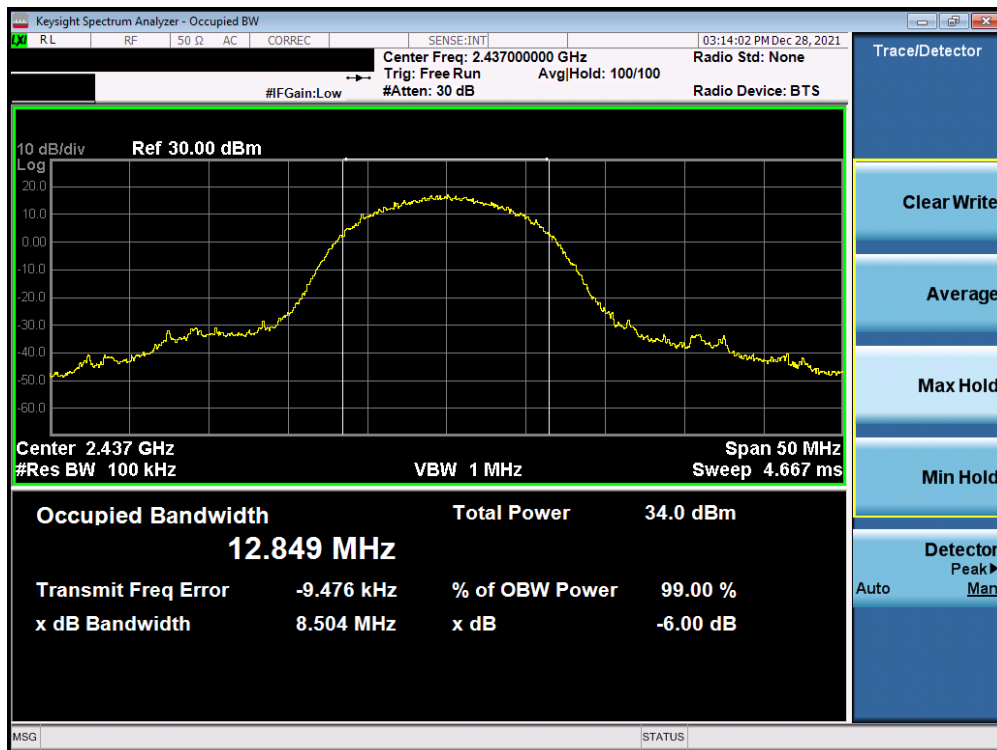
Plot 7-50. 6dB Bandwidth Plot Antenna WF7b (802.11b – Ch. 6) – 11Mbps
