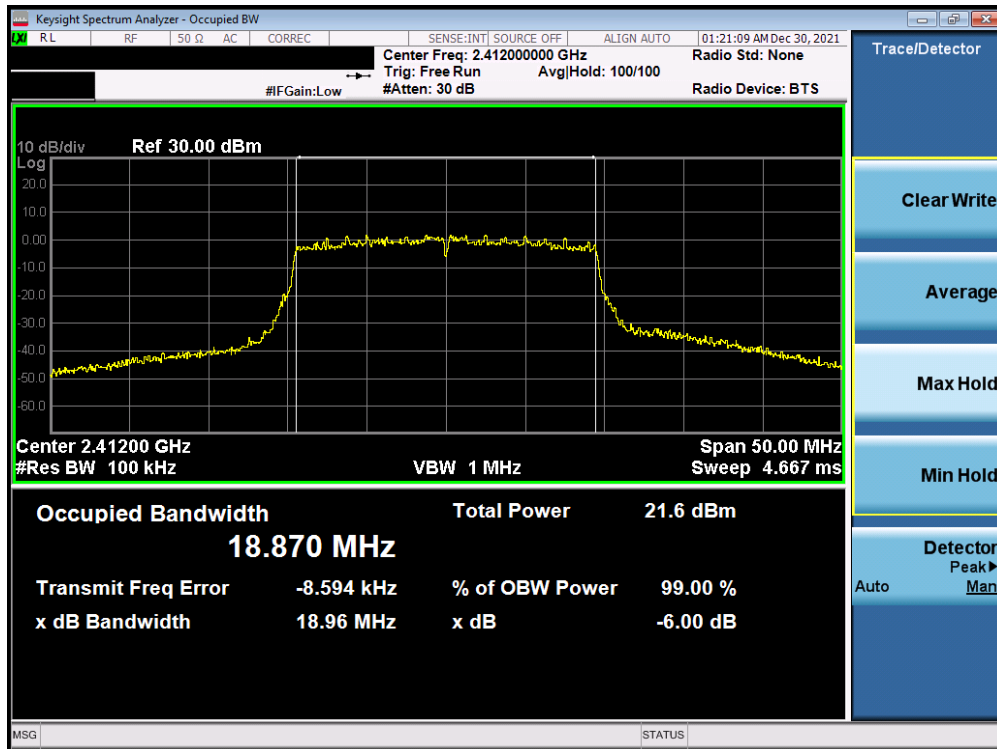
Plot 7-46. 6dB Bandwidth Plot Antenna WF7b (802. 11ax (SU - 2.4GHz) – Ch. 1) – MCS3
