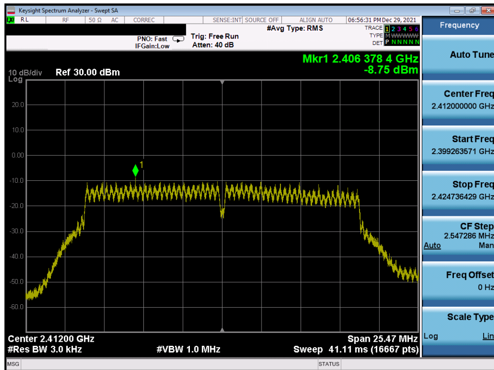
Plot 7-64. Power Spectral Density Plot Antenna WF8 (802.11n (2.4GHz) – Ch. 1) – MCS0
