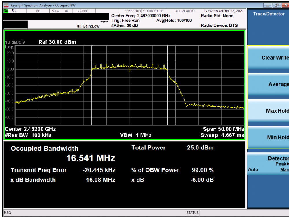
Plot 7-33. 6dB Bandwidth Plot Antenna WF7b (802.11g - Ch. 11) - 6Mbps
