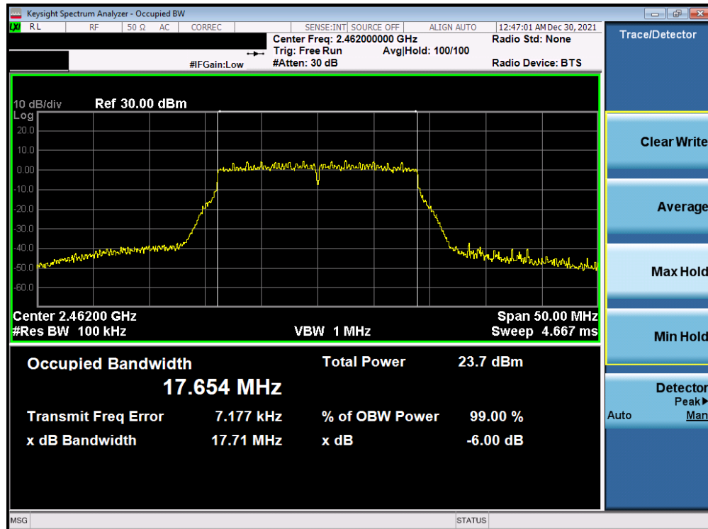
Plot 7-57. 6dB Bandwidth Plot Antenna WF7b (802.11n (2.4GHz) – Ch. 11) – MCS5
