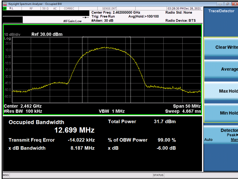
Plot 7-51. 6dB Bandwidth Plot Antenna WF7b (802.11b – Ch. 11) – 11Mbps
