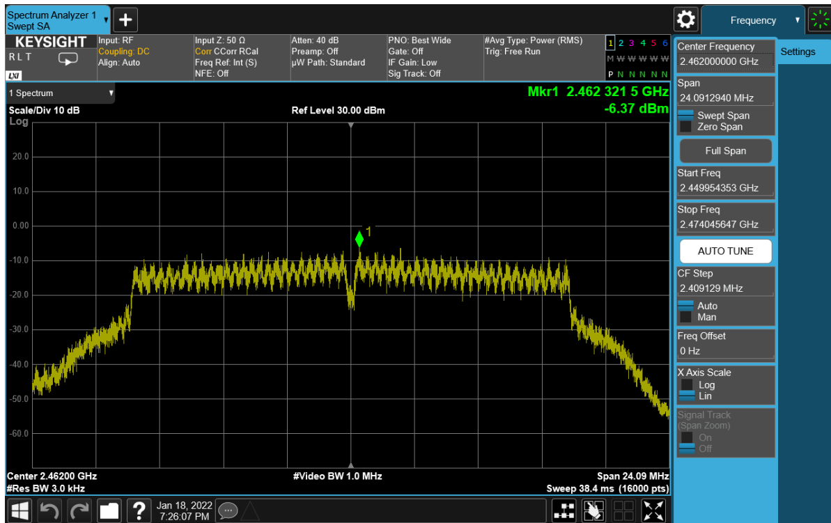
Plot 7-63. Power Spectral Density Plot Antenna WF8 (802.11g – Ch. 11) – 6Mbps
