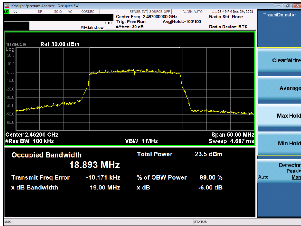
Plot 7-18. 6dB Bandwidth Plot Antenna WF8 (802. 11ax (SU - 2.4GHz) – Ch. 11) – MCS3
