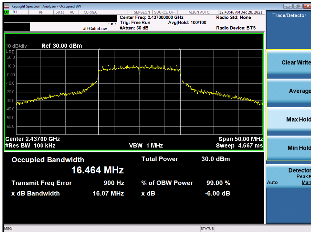
Plot 7-41. 6dB Bandwidth Plot Antenna WF7b (802.11g – Ch. 6) – 18Mbps
