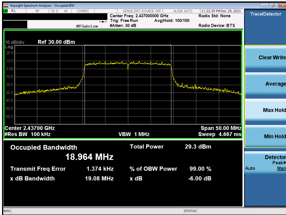
Plot 7-29. 6dB Bandwidth Plot Antenna WF8 (802.11ax (SU - 2.4GHz) – Ch. 6) – MCS5
