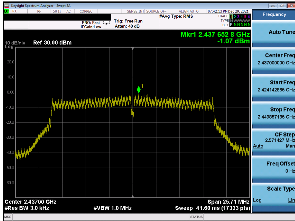
Plot 7-65. Power Spectral Density Plot Antenna WF8 (802.11n (2.4GHz) – Ch. 6) – MCS0
