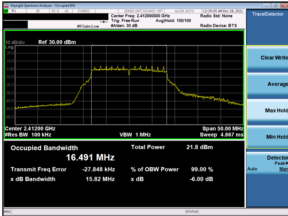
Plot 7-40. 6dB Bandwidth Plot Antenna WF7b (802.11g – Ch. 1) – 18Mbps
