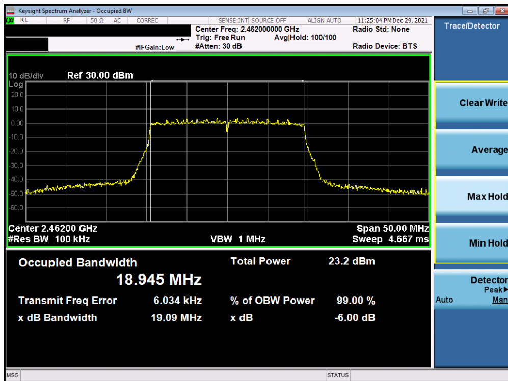
Plot 7-30. 6dB Bandwidth Plot Antenna WF8 (802.11ax (SU - 2.4GHz) – Ch. 11) – MCS5
