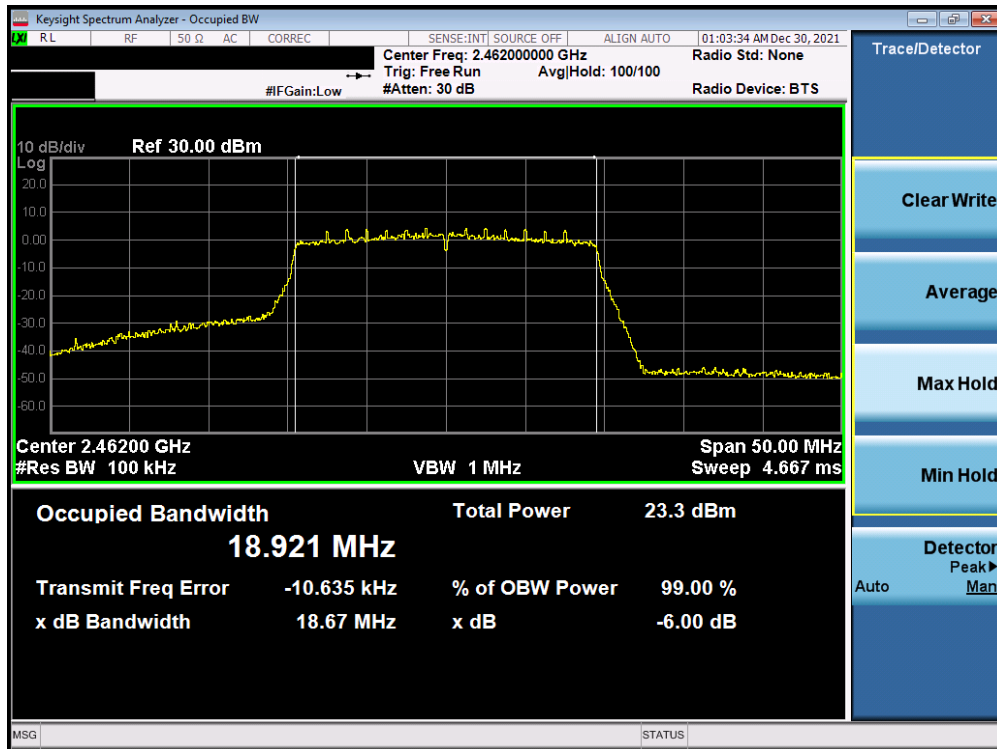
Plot 7-39. 6dB Bandwidth Plot Antenna WF7b (802. 11ax (SU - 2.4GHz) – Ch. 11) – MCS0
