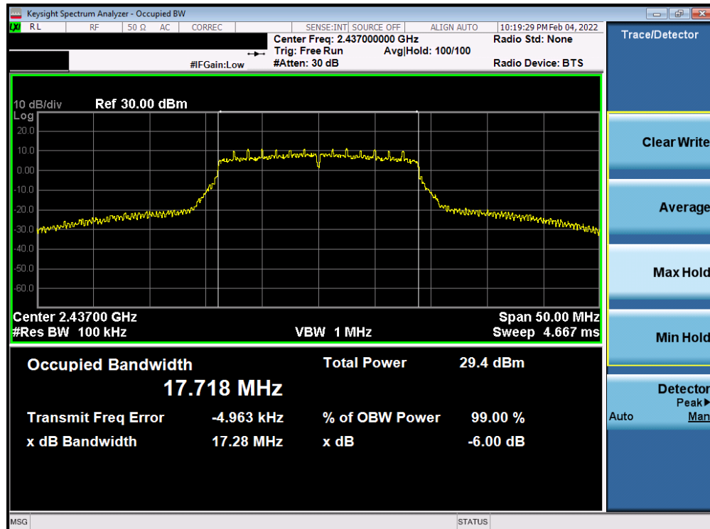
Plot 7-35. 6dB Bandwidth Plot Antenna WF7b (802.11n (2.4GHz) – Ch. 6) – MCS0
