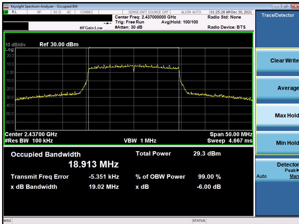
Plot 7-47. 6dB Bandwidth Plot Antenna WF7b (802. 11ax (SU - 2.4GHz) – Ch. 6) – MCS3
