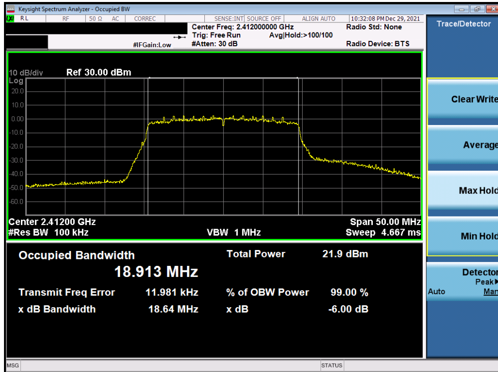
Plot 7-7. 6dB Bandwidth Plot Antenna WF8 (802.11ax (SU - 2.4GHz) - Ch. 1) - MCS0
