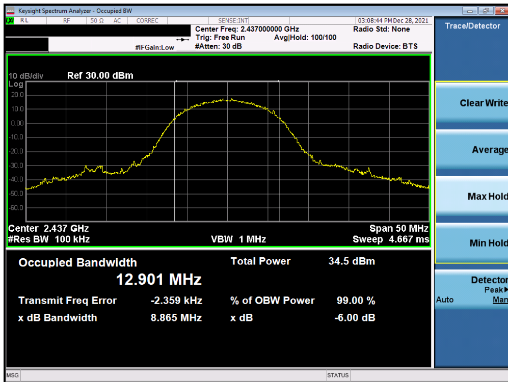
Plot 7-20. 6dB Bandwidth Plot Antenna WF8 (802.11b – Ch. 6) – 11Mbps
