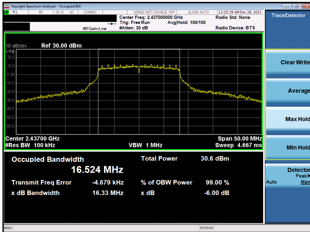
Plot 7-32. 6dB Bandwidth Plot Antenna WF7b (802.11g – Ch. 6) – 6Mbps
