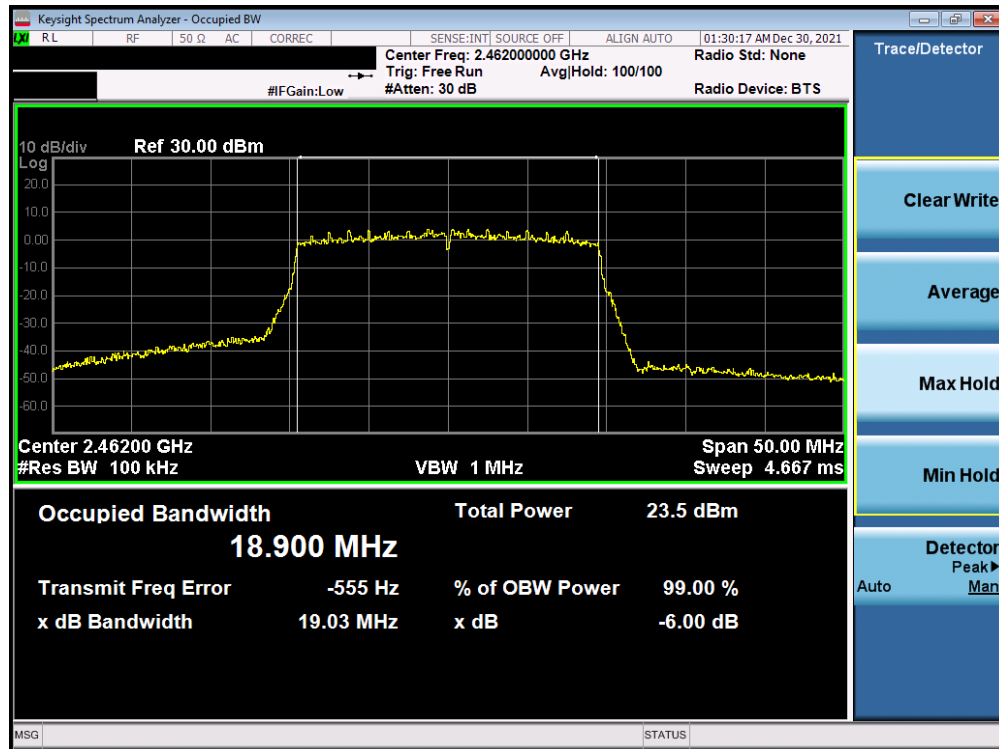
Plot 7-48. 6dB Bandwidth Plot Antenna WF7b (802. 11ax (SU - 2.4GHz) – Ch. 11) – MCS3
