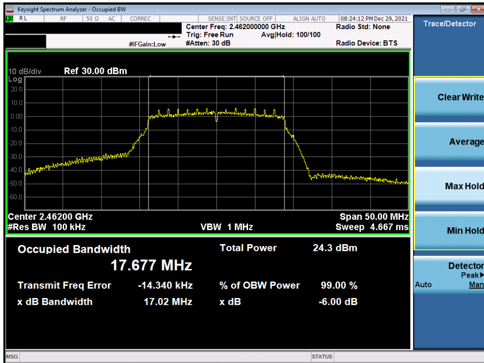
Plot 7-6. 6dB Bandwidth Plot Antenna WF8 (802.11n (2.4GHz) - Ch. 11) - MCS0
