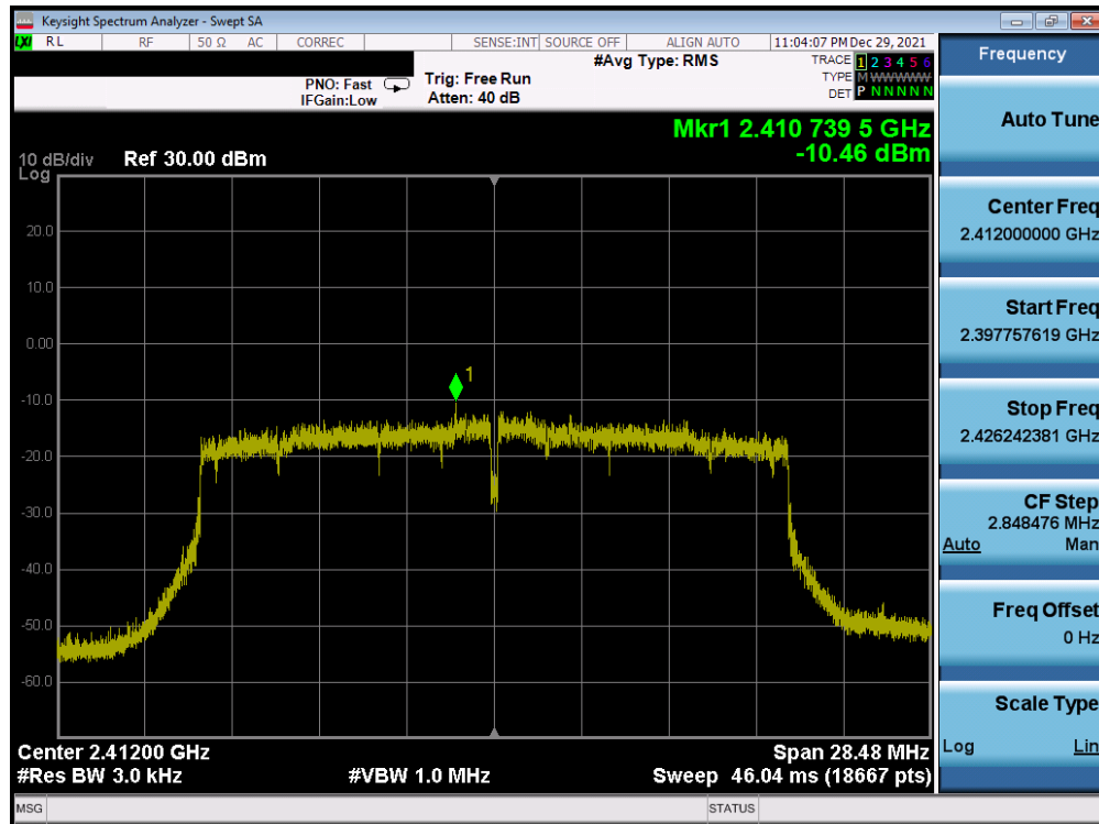
Plot 7-76. Power Spectral Density Plot Antenna WF8 (802.11ax (SU - 2.4GHz) – Ch. 1) – MCS3
