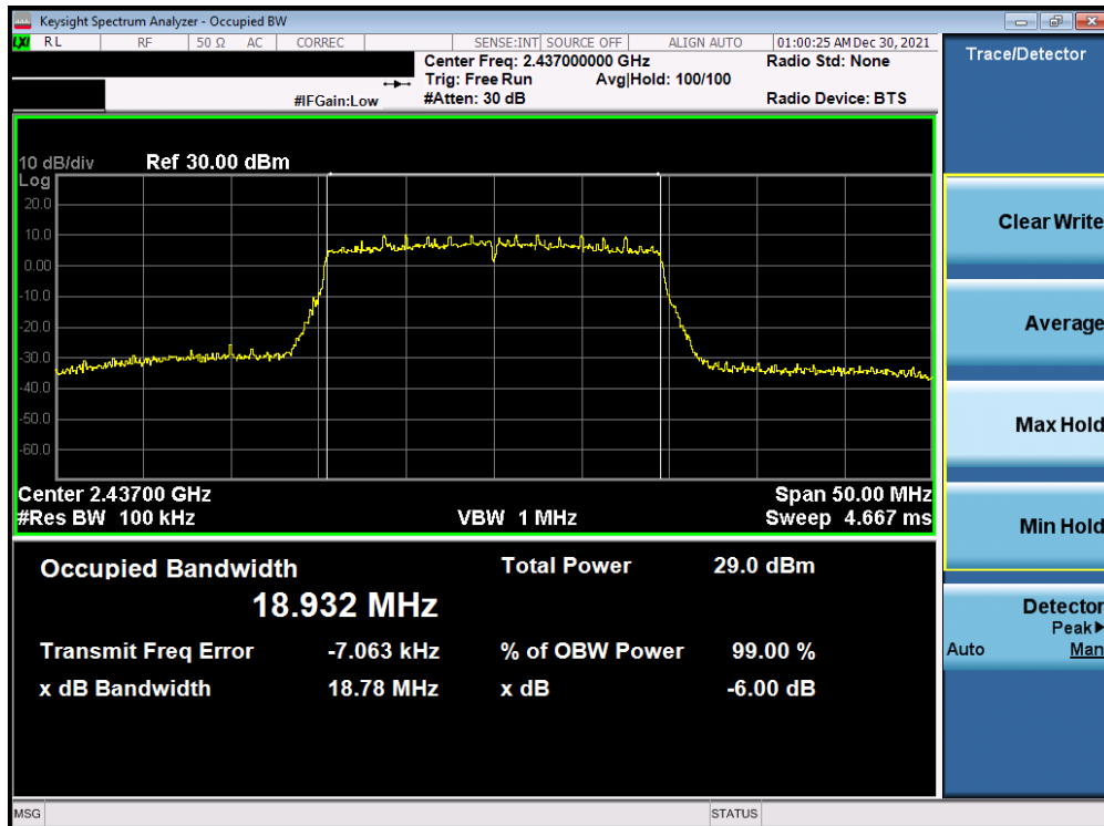
Plot 7-38. 6dB Bandwidth Plot Antenna WF7b (802.11ax (SU - 2.4GHz) – Ch. 6) – MCS0
