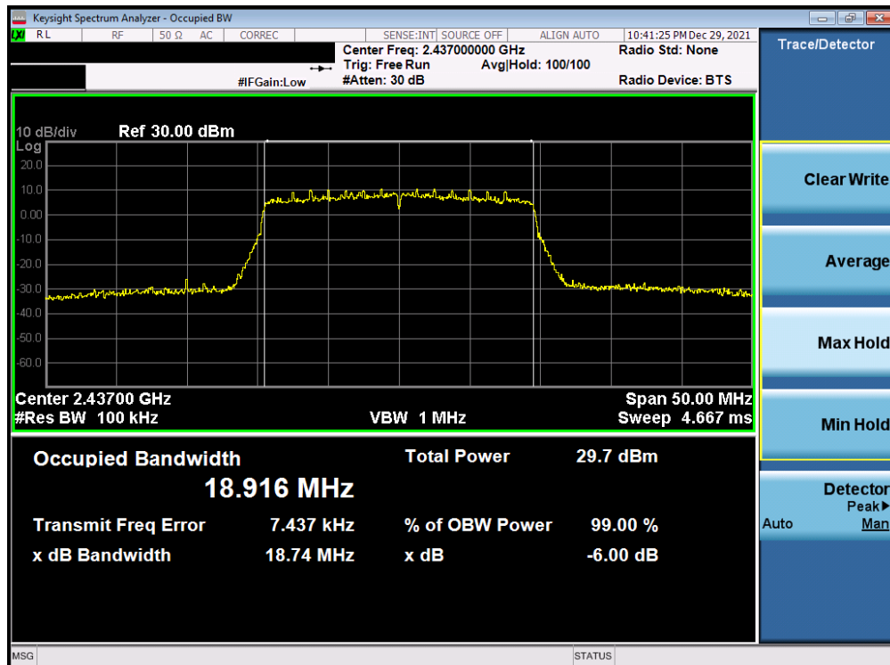
Plot 7-8. 6dB Bandwidth Plot Antenna WF8 (802.11ax (SU - 2.4GHz) - Ch. 6) - MCS0
