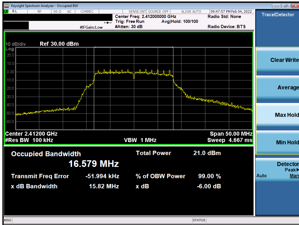
Plot 7-1. 6dB Bandwidth Plot Antenna WF8 (802.11g - Ch. 1) - 6Mbps
