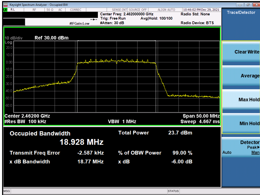
Plot 7-9. 6dB Bandwidth Plot Antenna WF8 (802. 11ax (SU - 2.4GHz) – Ch. 11) – MCS0
