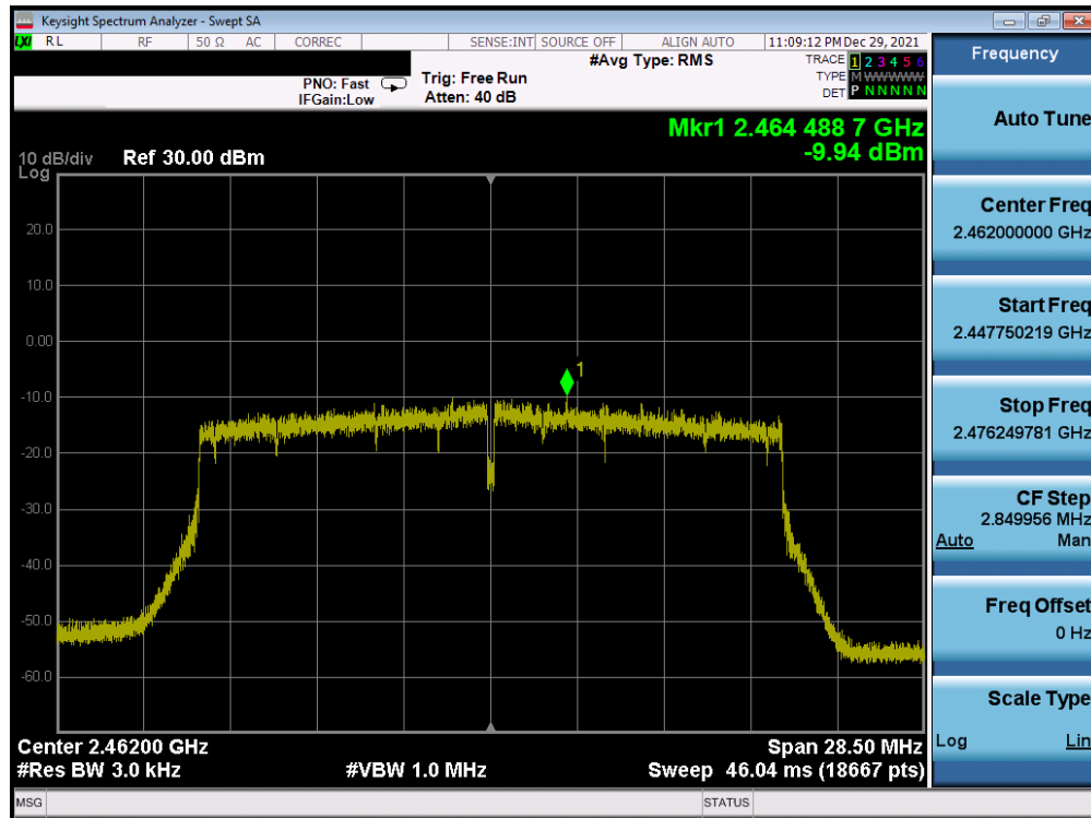
Plot 7-78. Power Spectral Density Plot Antenna WF8 (802.11ax (SU - 2.4GHz) – Ch. 11) – MCS3
