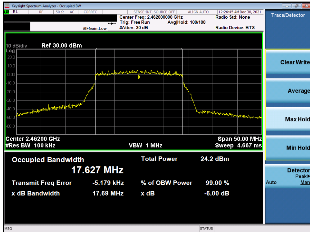
Plot 7-45. 6dB Bandwidth Plot Antenna WF7b (802.11n (2.4GHz) – Ch. 11) – MCS3
