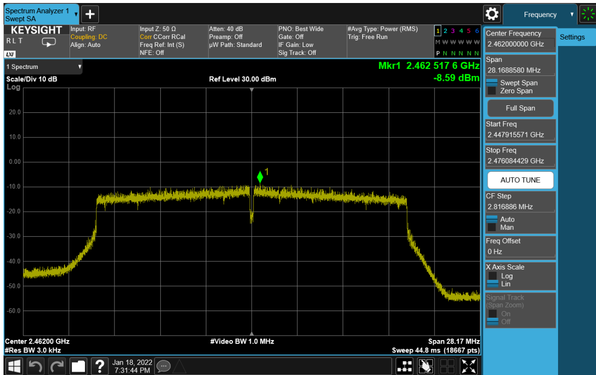
Plot 7-69. Power Spectral Density Plot Antenna WF8 (802.11ax (SU - 2.4GHz) – Ch. 11) – MCS0
