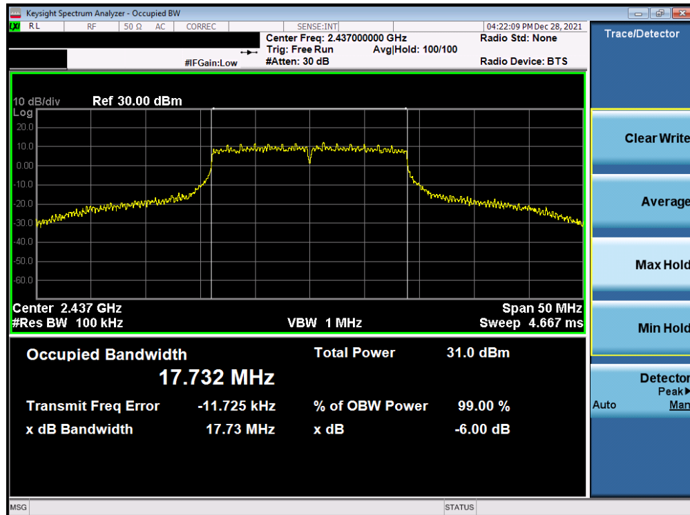
Plot 7-56. 6dB Bandwidth Plot Antenna WF7b (802.11n (2.4GHz) – Ch. 6) – MCS5
