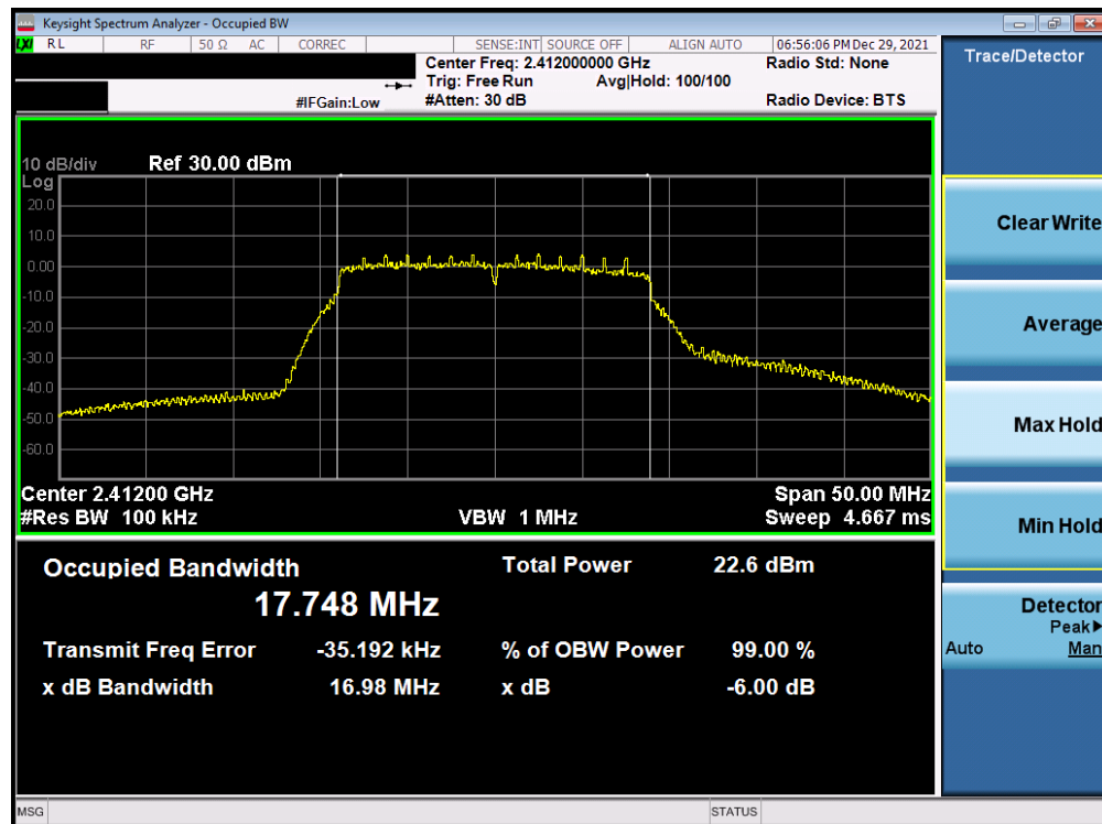
Plot 7-4. 6dB Bandwidth Plot Antenna WF8 (802.11n (2.4GHz) – Ch. 1) – MCS0
