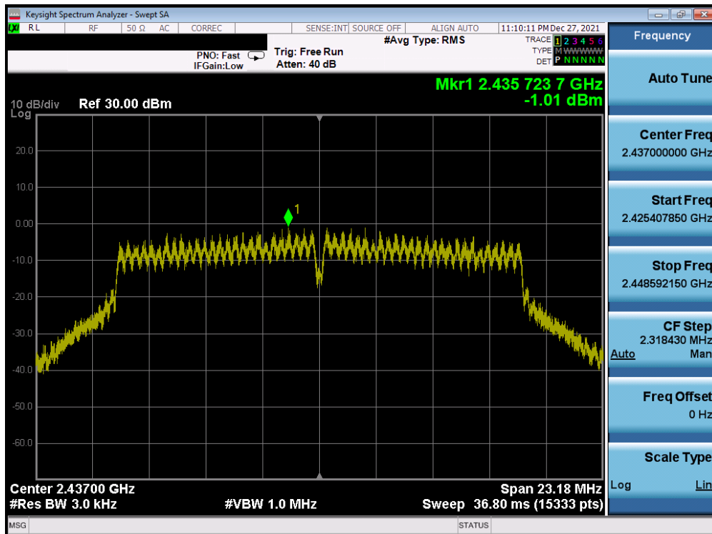
Plot 7-62. Power Spectral Density Plot Antenna WF8 (802.11g – Ch. 6) – 6Mbps
