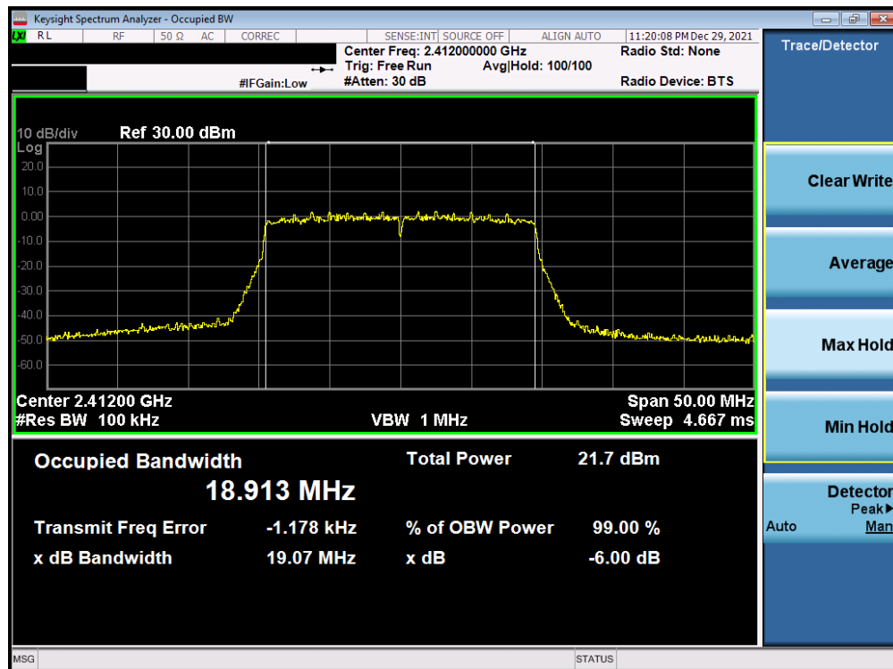
Plot 7-28. 6dB Bandwidth Plot Antenna WF8 (802.11ax (SU - 2.4GHz) – Ch. 1) – MCS5
