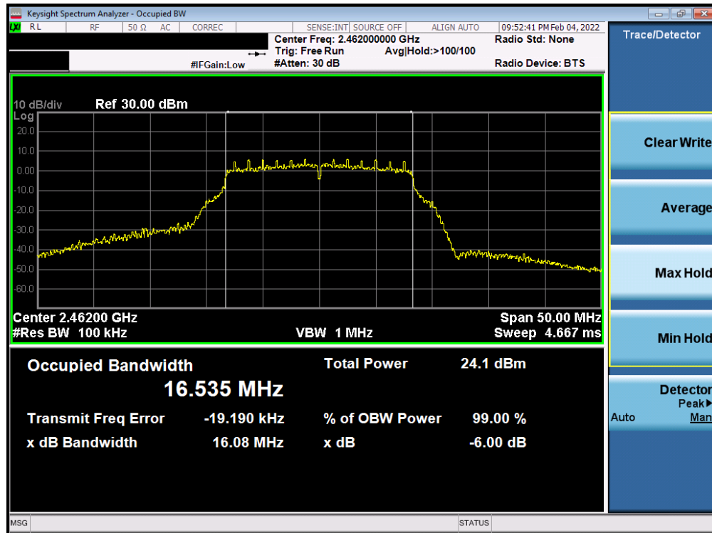
Plot 7-3. 6dB Bandwidth Plot Antenna WF8 (802.11g – Ch. 11) – 6Mbps
