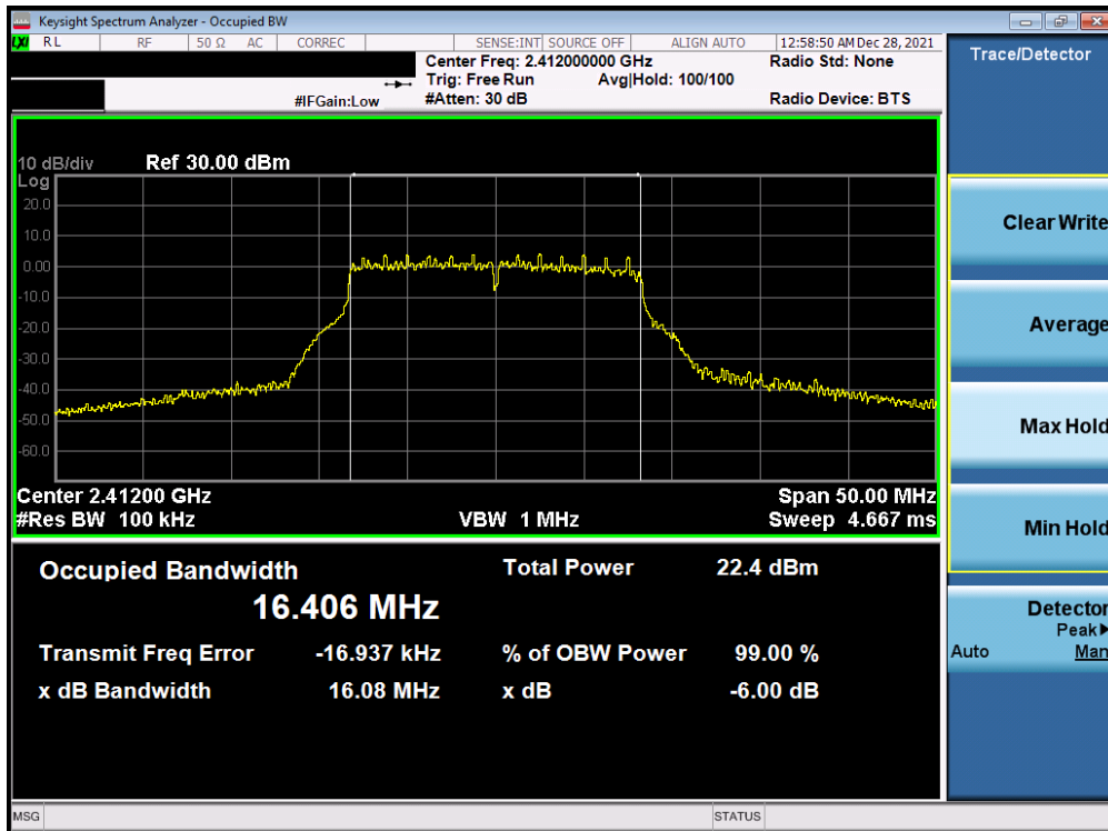
Plot 7-52. 6dB Bandwidth Plot Antenna WF7b (802.11g – Ch. 1) – 36Mbps
