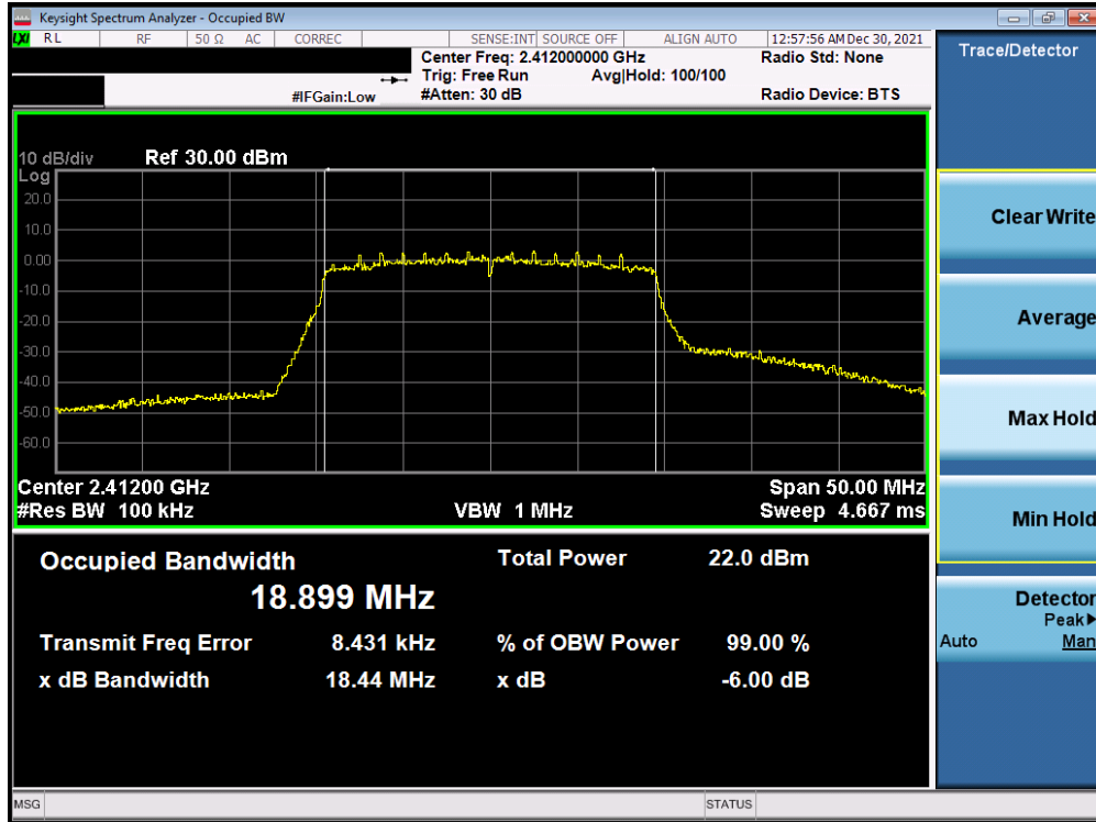
Plot 7-37. 6dB Bandwidth Plot Antenna WF7b (802.11ax (SU - 2.4GHz) – Ch. 1) – MCS0
