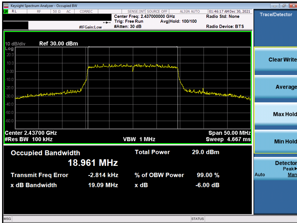
Plot 7-59. 6dB Bandwidth Plot Antenna WF7b (802.11ax (SU - 2.4GHz) – Ch. 6) – MCS5
