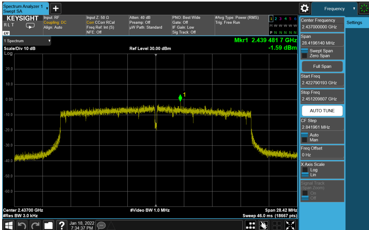
Plot 7-77. Power Spectral Density Plot Antenna WF8 (802.11ax (SU - 2.4GHz) – Ch. 6) – MCS3
