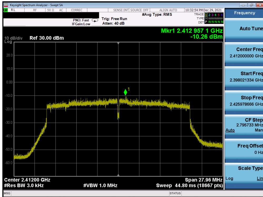
Plot 7-67. Power Spectral Density Plot Antenna WF8 (802.11ax (SU - 2.4GHz) – Ch. 1) – MCS0
