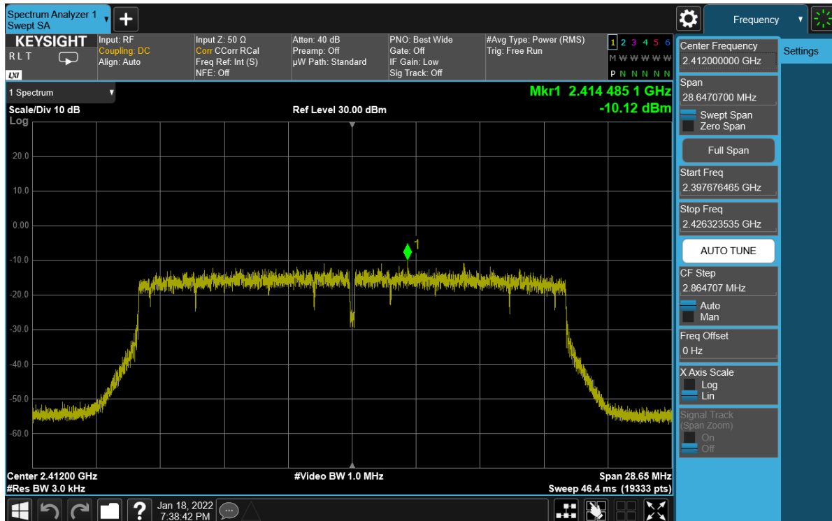
Plot 7-88. Power Spectral Density Plot Antenna WF8 (802.11ax (SU - 2.4GHz) – Ch. 1) – MCS5
