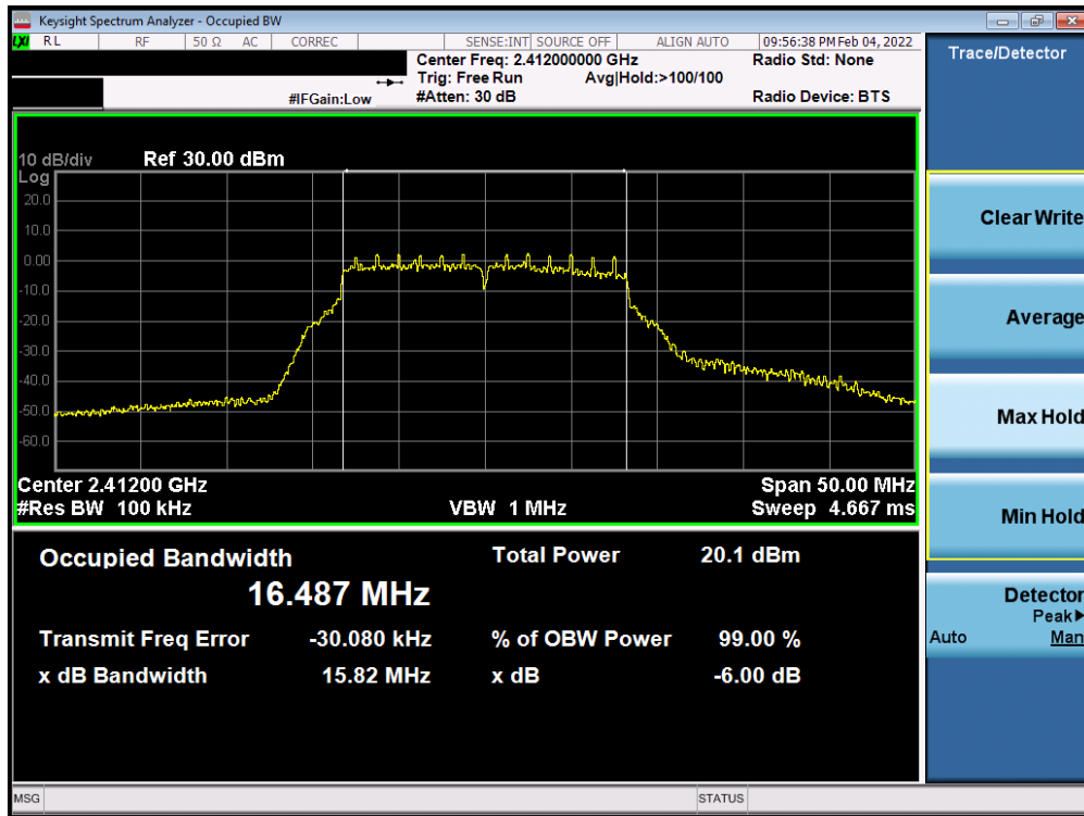
Plot 7-10. 6dB Bandwidth Plot Antenna WF8 (802.11g – Ch. 1) – 18Mbps
