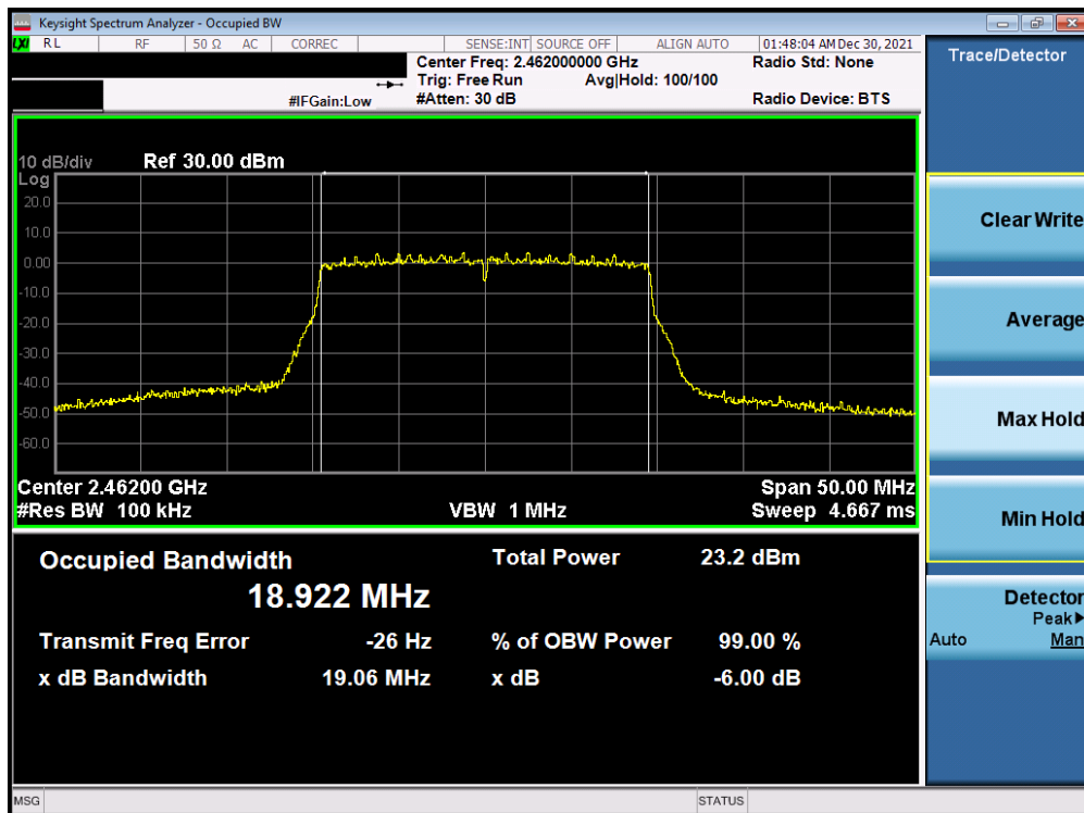
Plot 7-60. 6dB Bandwidth Plot Antenna WF7b (802.11ax (SU - 2.4GHz) – Ch. 11) – MCS5
