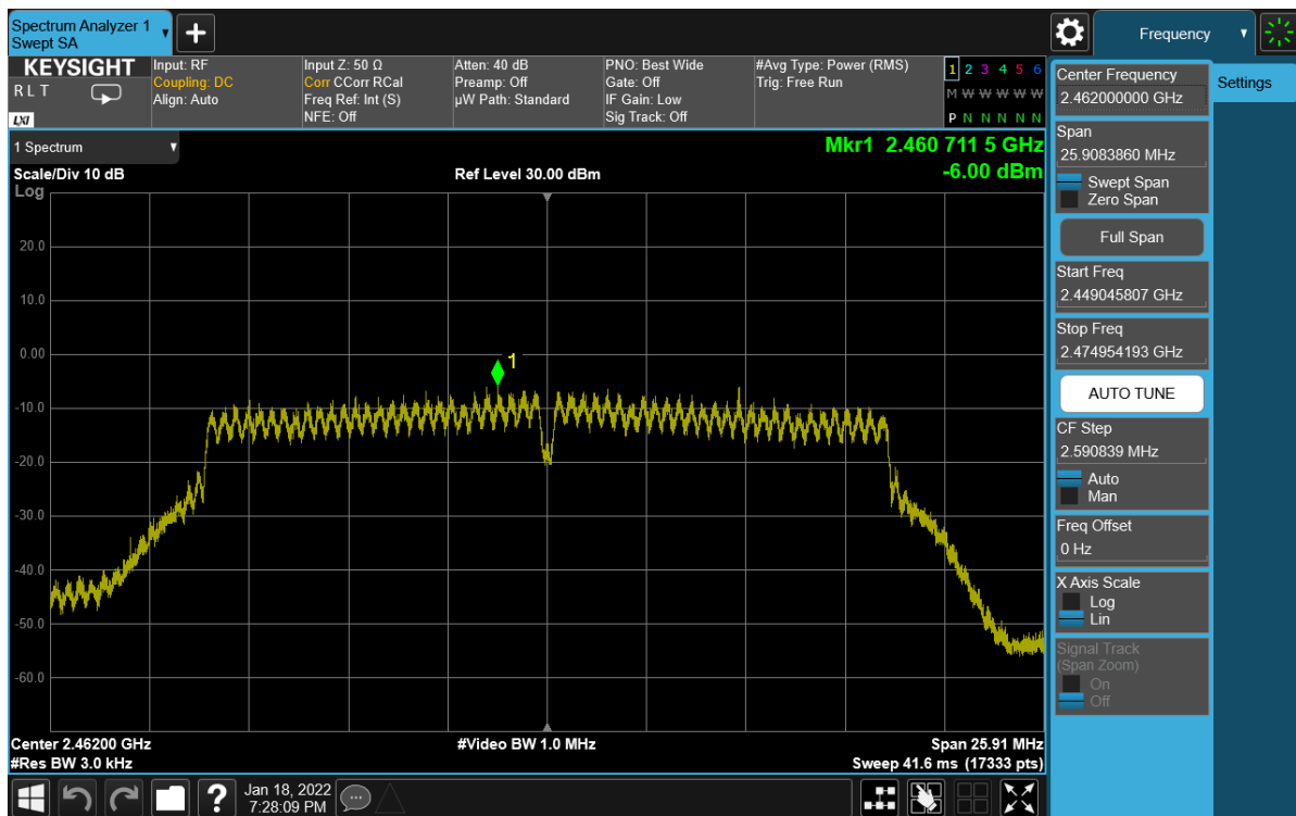
Plot 7-66. Power Spectral Density Plot Antenna WF8 (802.11n (2.4GHz) – Ch. 11) – MCS0
