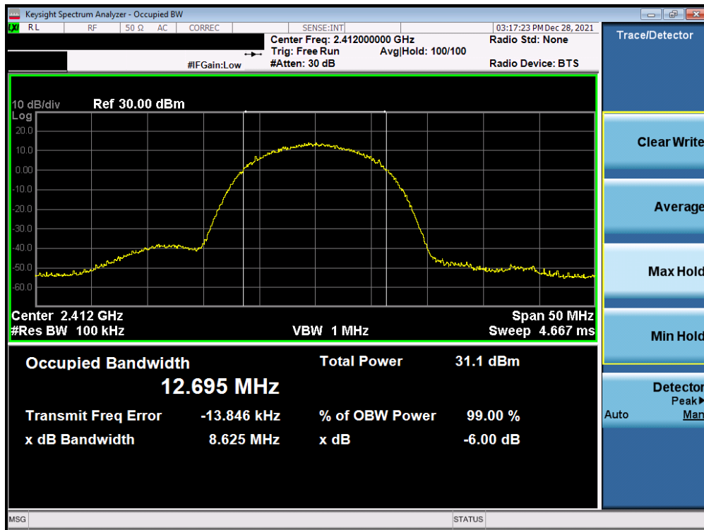
Plot 7-49. 6dB Bandwidth Plot Antenna WF7b (802.11b – Ch. 1) – 11Mbps
