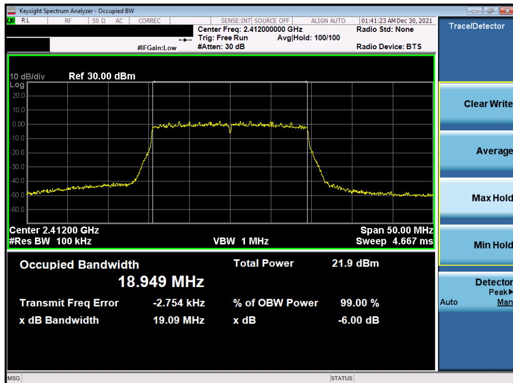
Plot 7-58. 6dB Bandwidth Plot Antenna WF7b (802.11ax (SU - 2.4GHz) – Ch. 1) – MCS5
