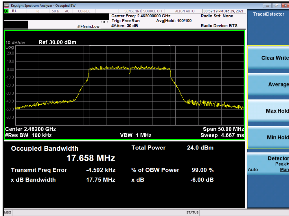
Plot 7-27. 6dB Bandwidth Plot Antenna WF8 (802.11n (2.4GHz) – Ch. 11) – MCS5
