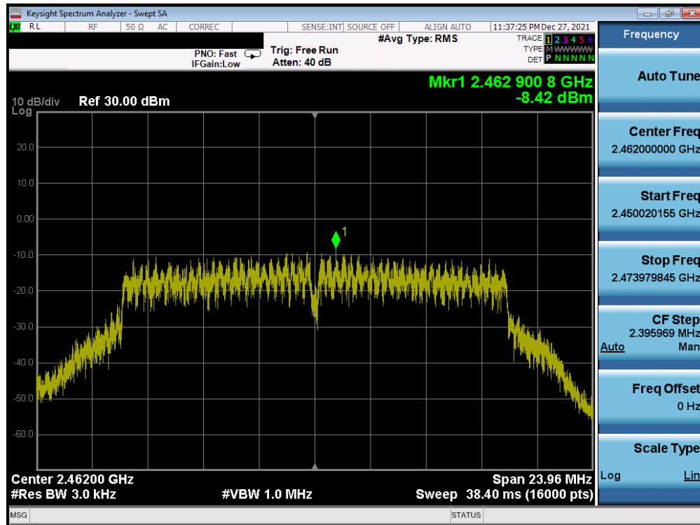
Plot 7-72. Power Spectral Density Plot Antenna WF8 (802.11g – Ch. 11) – 18Mbps
