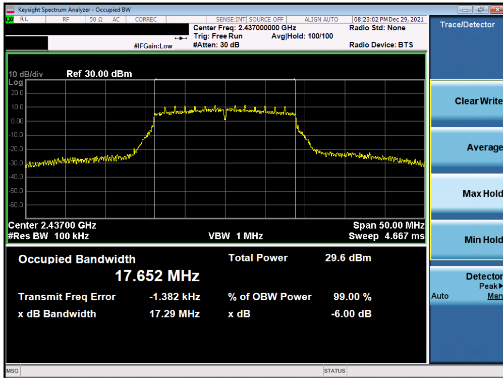
Plot 7-5. 6dB Bandwidth Plot Antenna WF8 (802.11n (2.4GHz) - Ch. 6) - MCS0
