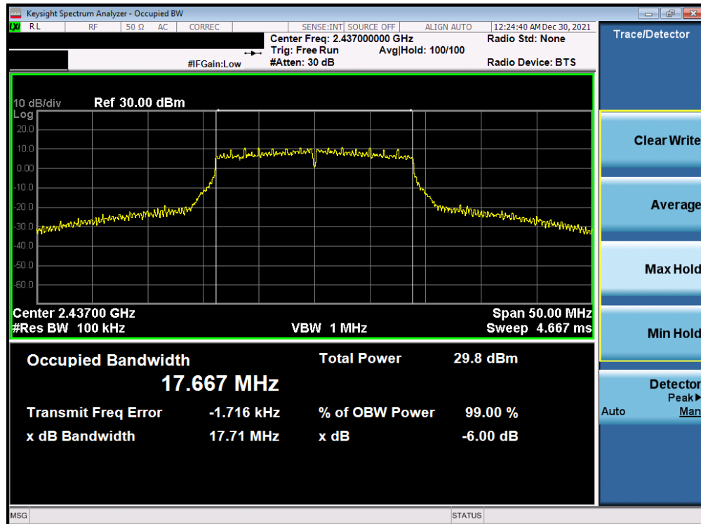
Plot 7-44. 6dB Bandwidth Plot Antenna WF7b (802.11n (2.4GHz) – Ch. 6) – MCS3
