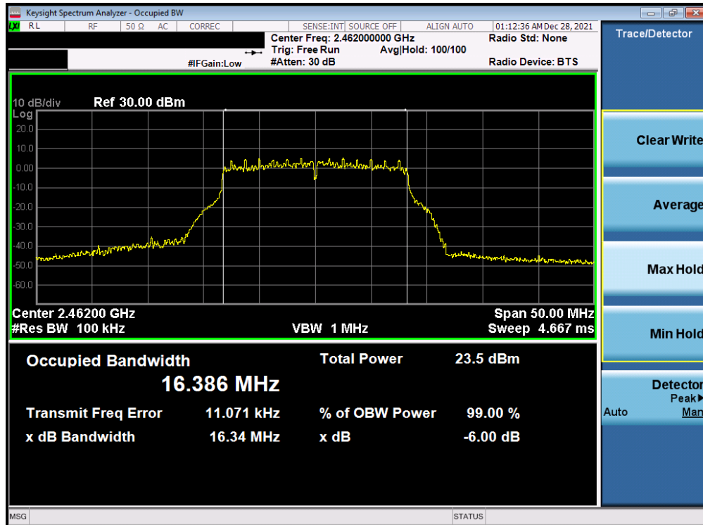
Plot 7-54. 6dB Bandwidth Plot Antenna WF7b (802.11g - Ch. 11) - 36Mbps
