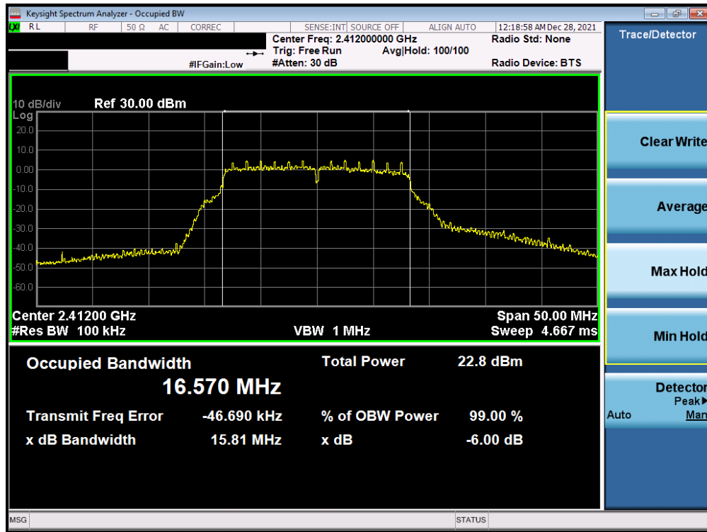
Plot 7-31. 6dB Bandwidth Plot Antenna WF7b (802.11g – Ch. 1) – 6Mbps
