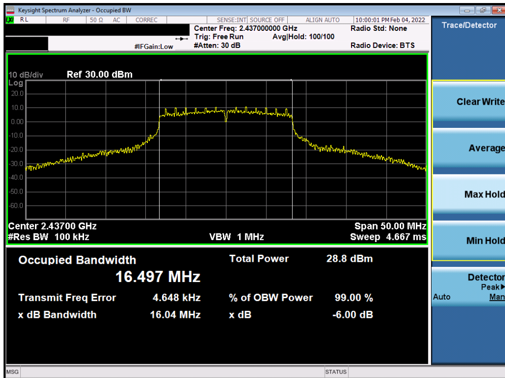
Plot 7-11. 6dB Bandwidth Plot Antenna WF8 (802.11g – Ch. 6) – 18Mbps
