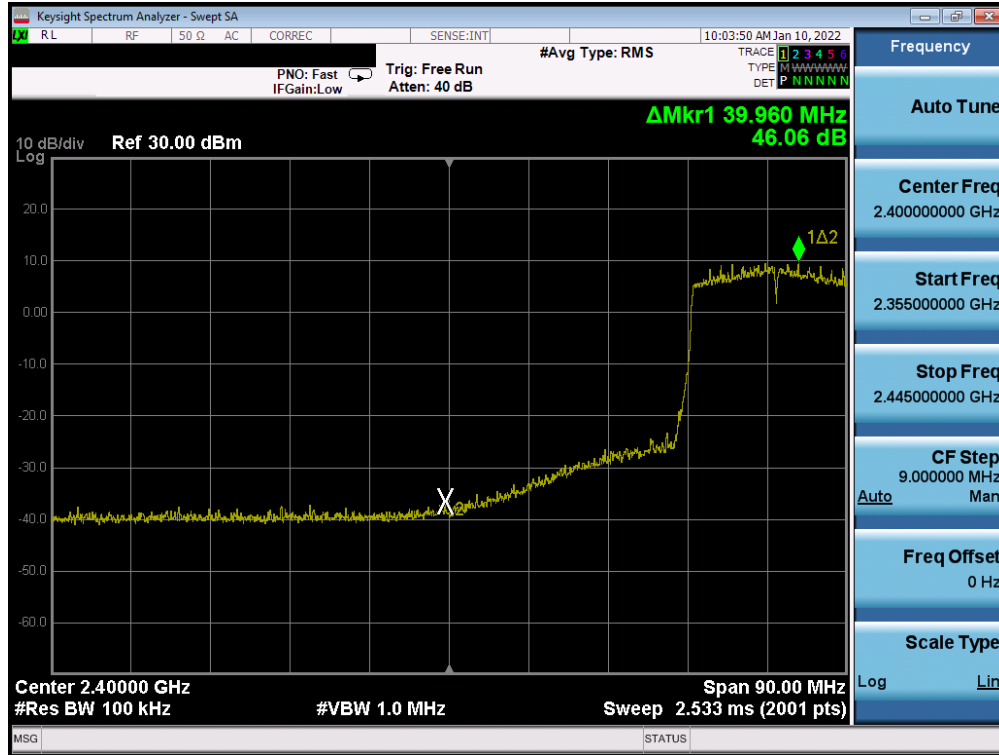
Plot 7-81. Band Edge Antenna WF8 (802.11ax OFDMA – RU242 – Ch. 6)
