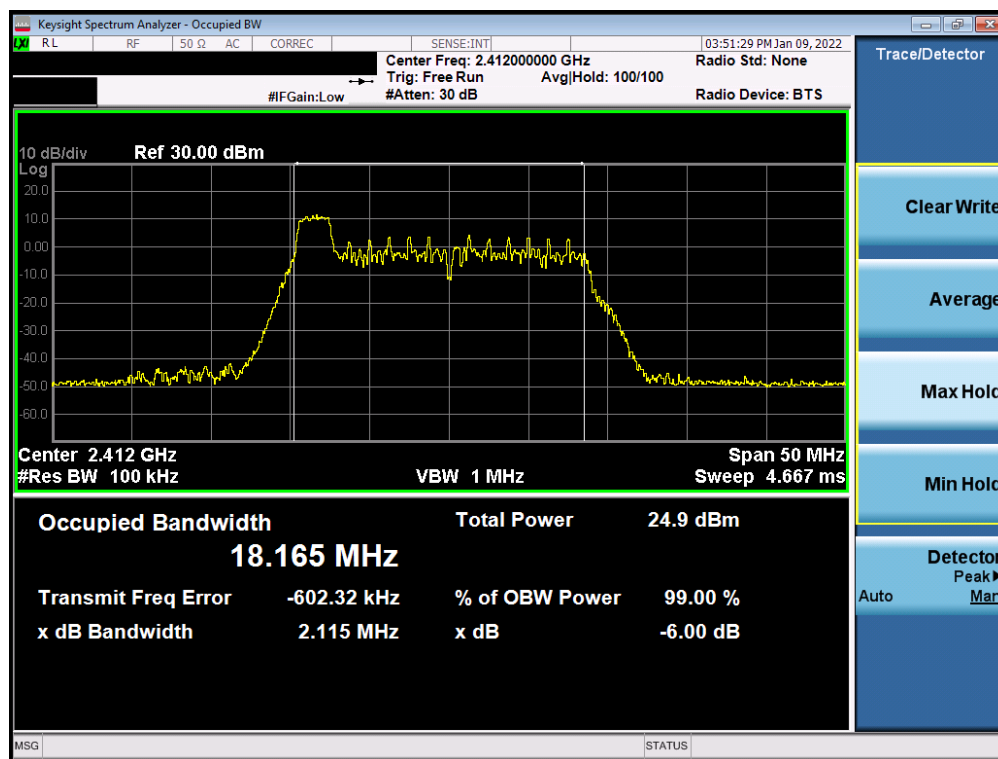
Plot 7-13. 6dB BW & 99% OBW Plot Antenna WF7b (802.11ax OFDMA – RU26 Index 0 – Ch. 1)
