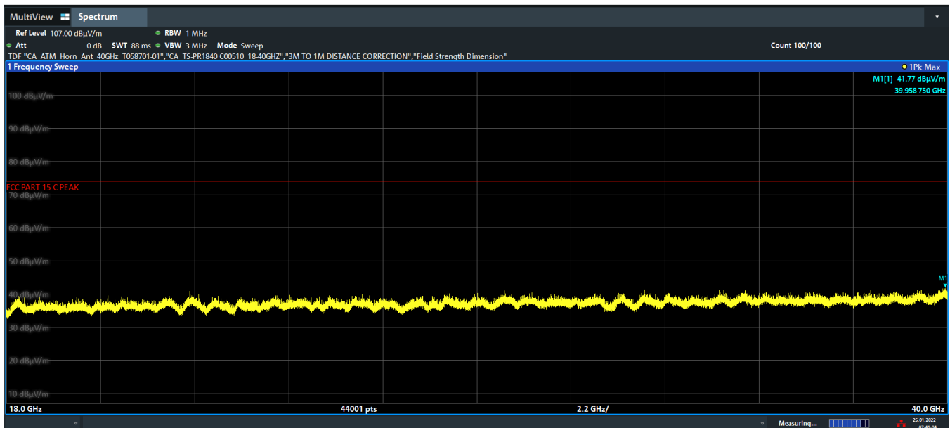
Plot 7-94. Radiated Spurious Emissions Above 18GHz – Simultaneous Tx (1Mbps, ePA – Ch. 39, UNII 11n – Ch. 36, Pol. V)
