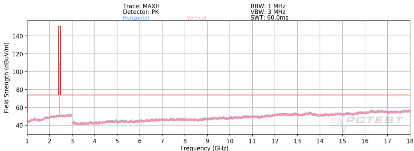
Plot 7-85. Radiated Spurious Emissions 1-18GHz Antenna WF7b (1Mbps, ePA – Ch. 19)
