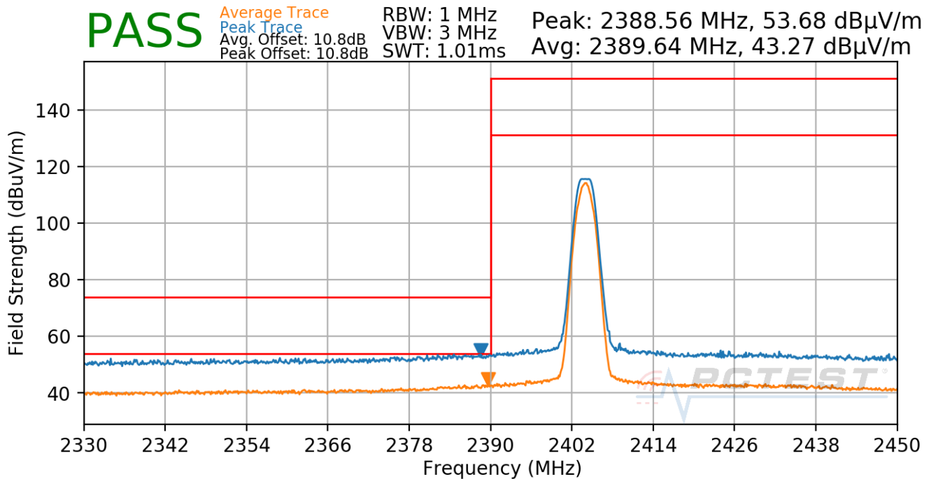
Plot 7-101. Radiated Restricted Lower Band Edge Measurement Antenna WF7b (Average & Peak)
