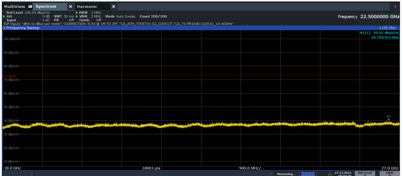
Plot 7-92. Radiated Spurious Emissions Above 18GHz TxBF (1Mbps, ePA – Ch. 39, Pol. V)
