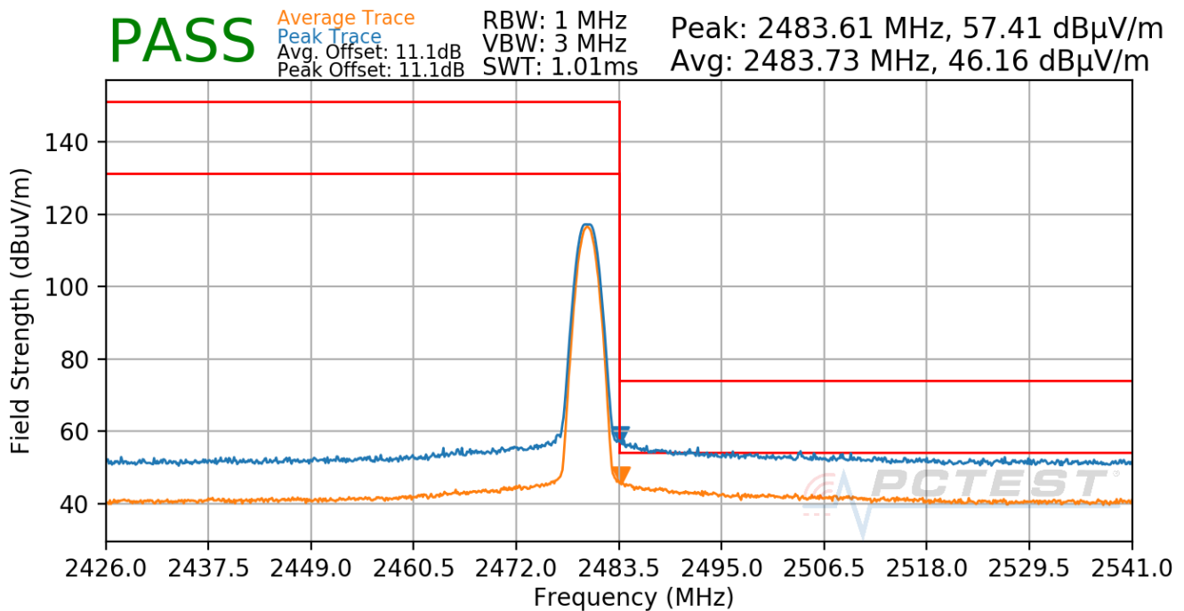
Plot 7-100. Radiated Restricted Upper Band Edge Measurement Antenna WF7b (Average & Peak)
