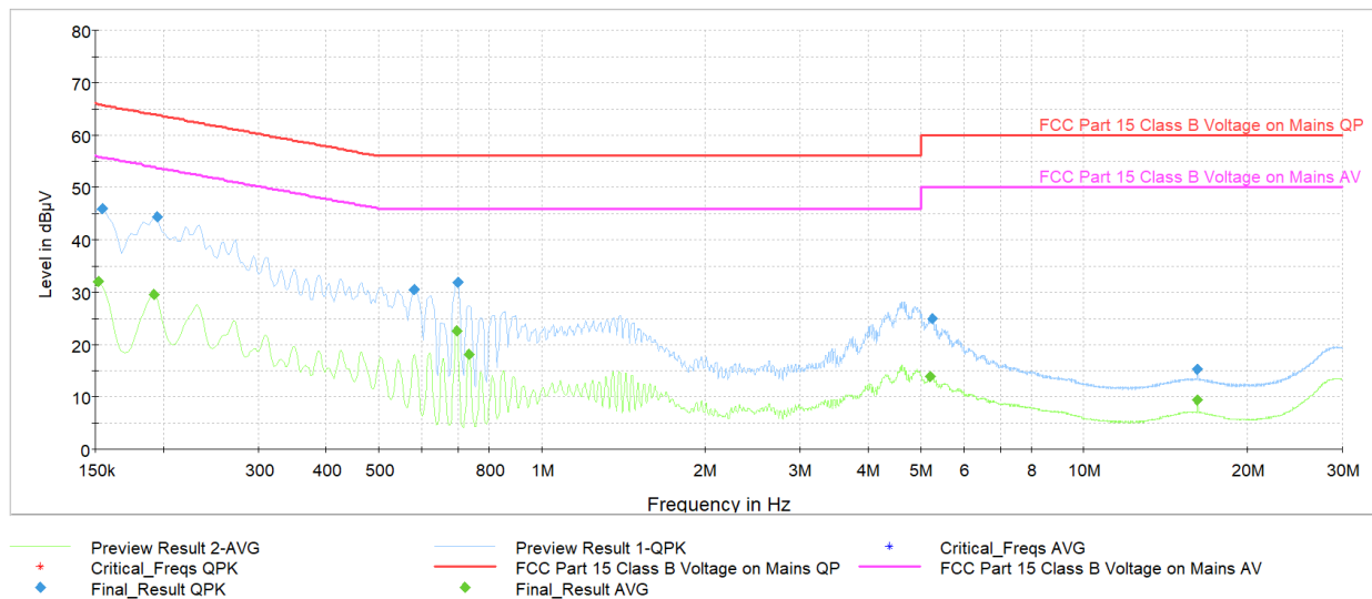
Plot 7-110. AC Line Conducted Plot with Bluetooth LE Tx BF (N, 1Mbps ePA – Ch.19, with AC/DC Adapter)
