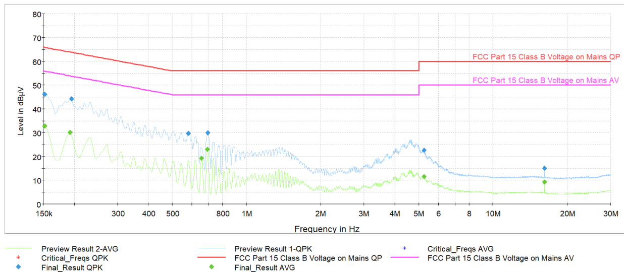
Plot 7-109. AC Line Conducted Plot with Bluetooth LE Tx BF (L1, 1Mbps ePA – Ch.19 with AC/DC Adapter)
