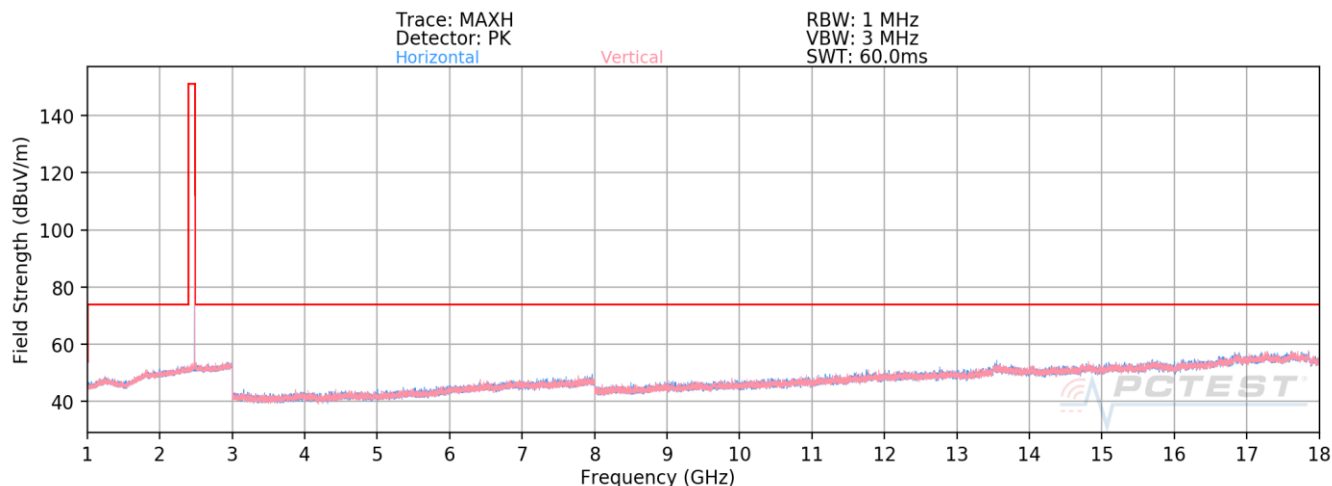
Plot 7-83. Radiated Spurious Emissions 1-18GHz Antenna WF8 (1Mbps ePA – Ch. 39)
