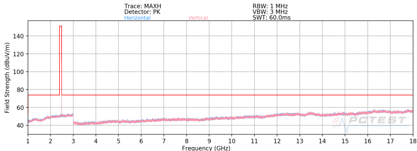
Plot 7-86. Radiated Spurious Emissions 1-18GHz Antenna WF7b (1Mbps ePA – Ch. 39)
