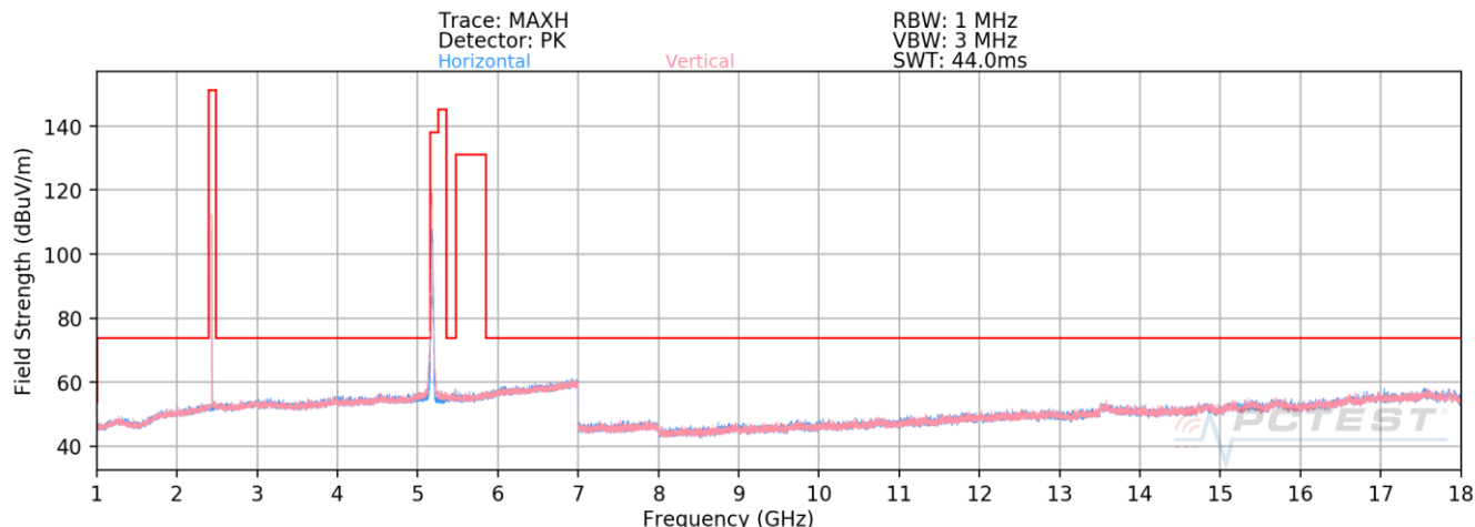
Plot 7-90. Radiated Spurious Emissions above 1GHz Simultaneous Tx
