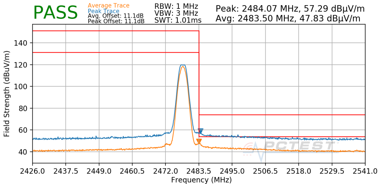
Plot 7-106. Radiated Restricted Upper Band Edge Measurement TxBF (Average & Peak)
