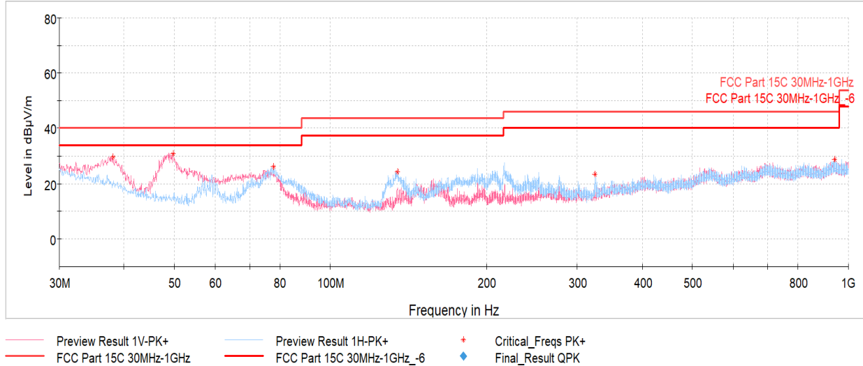
Plot 7-107. Radiated Spurious Emissions Below 1GHz TxBF (1Mbps, ePA – Ch.19, Pol. H & V, with AC/DC Adapter)
