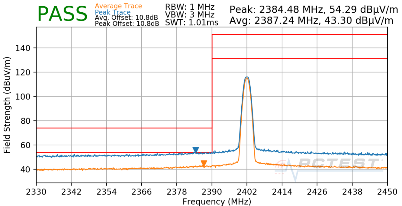
Plot 7-99. Radiated Restricted Lower Band Edge Measurement Antenna WF7b (Average & Peak)
