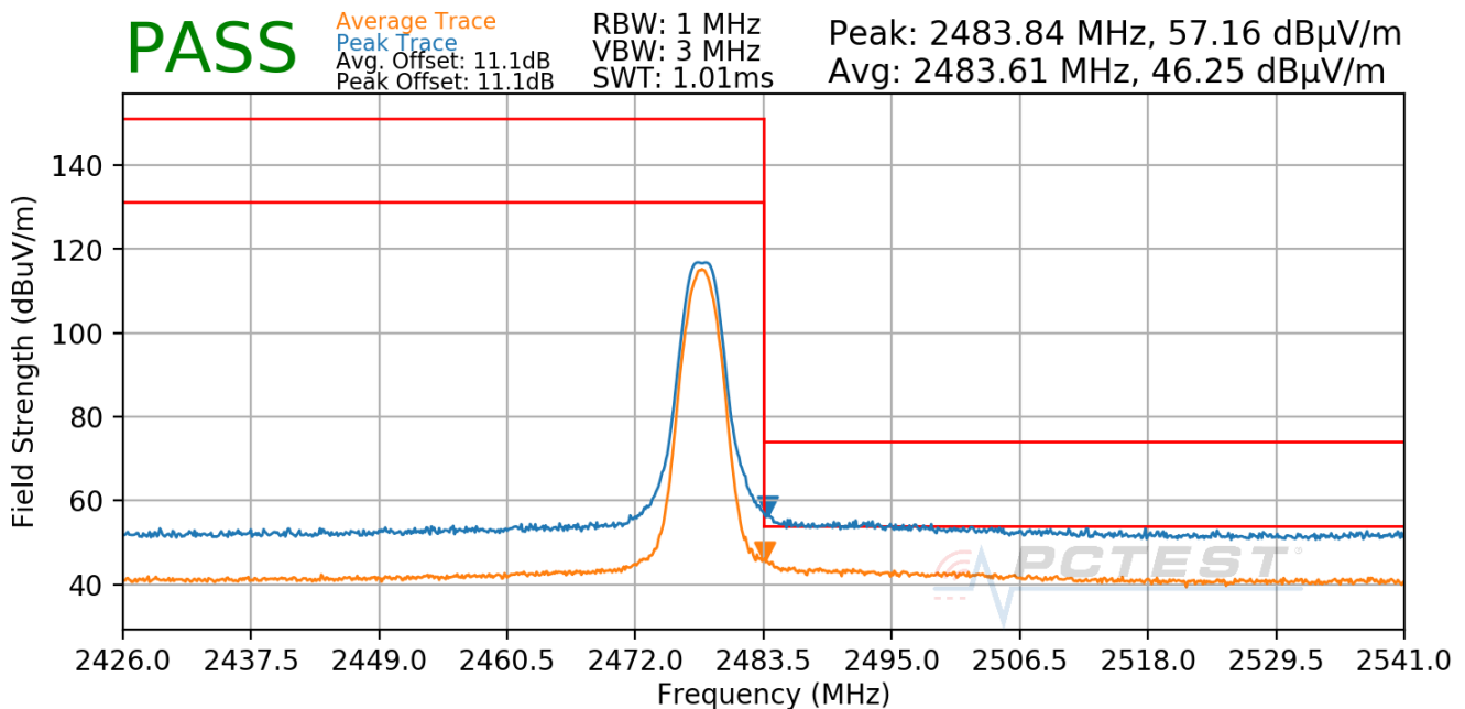
Plot 7-98. Radiated Restricted Upper Band Edge Measurement Antenna WF8 (Average & Peak)
