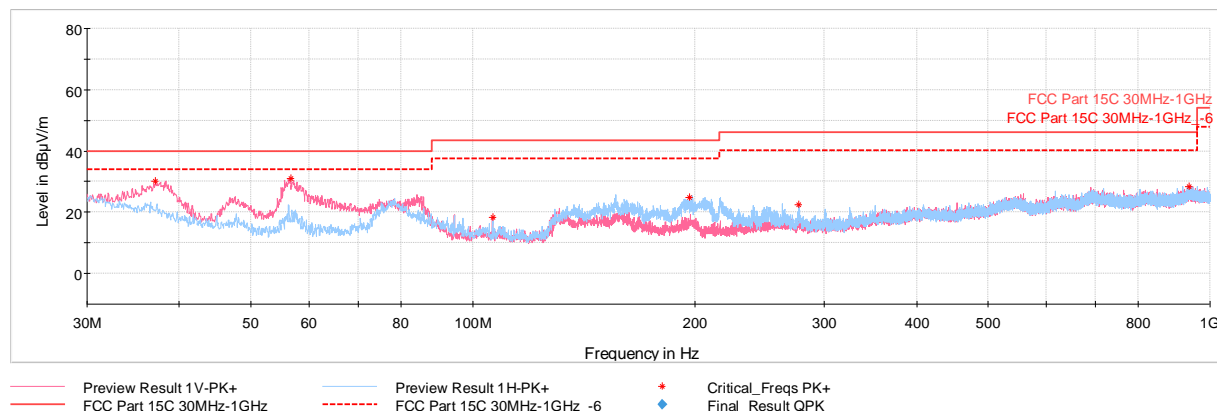
Plot 7-108. Radiated Spurious Emissions below 1GHz Simultaneous Transmission (with AC/DC adapter)
