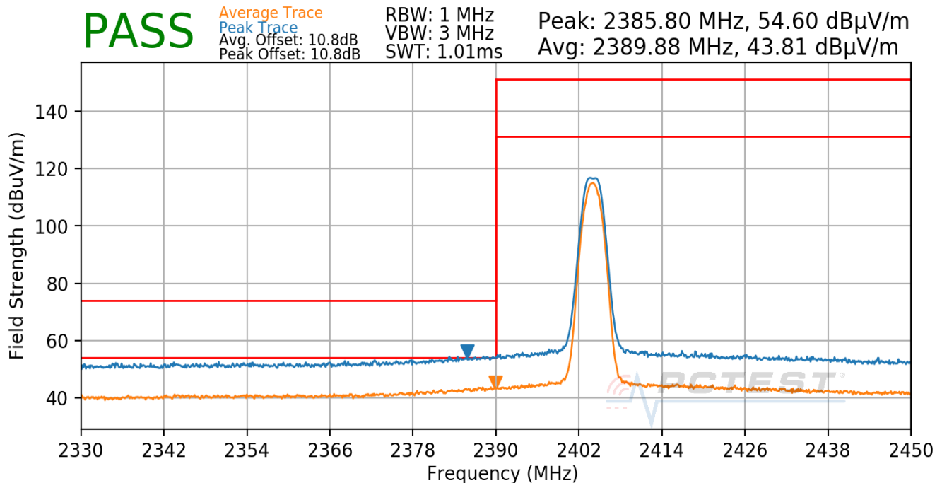
Plot 7-97. Radiated Restricted Lower Band Edge Measurement Antenna WF8 (Average & Peak)
