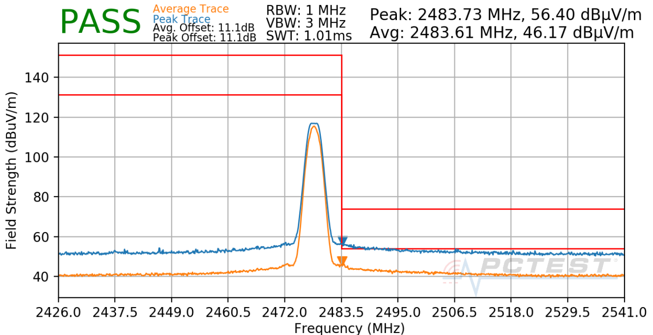
Plot 7-102. Radiated Restricted Upper Band Edge Measurement Antenna WF7b (Average & Peak)
