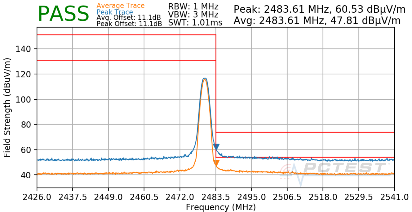
Plot 7-96. Radiated Restricted Upper Band Edge Measurement Antenna WF8 (Average & Peak)
