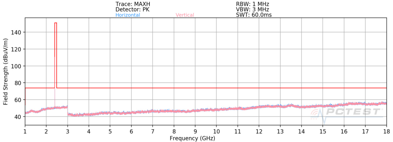
Plot 7-84. Radiated Spurious Emissions 1-18GHz Antenna WF7b (1Mbps, ePA – Ch. 0)
