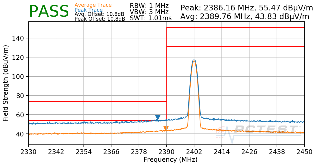
Plot 7-95. Radiated Restricted Lower Band Edge Measurement Antenna WF8 (Average & Peak)
