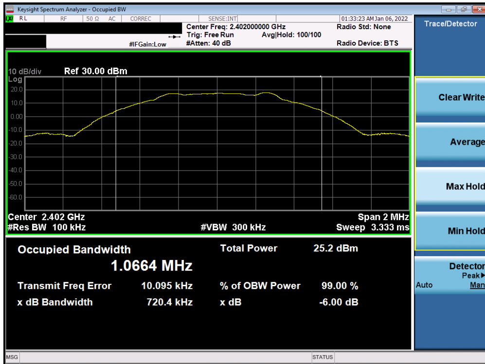
Plot 7-7. 6dB BW & 99% OBW Plot Antenna WF7b (Bluetooth (LE), 1Mbps, ePA – Ch. 0)
