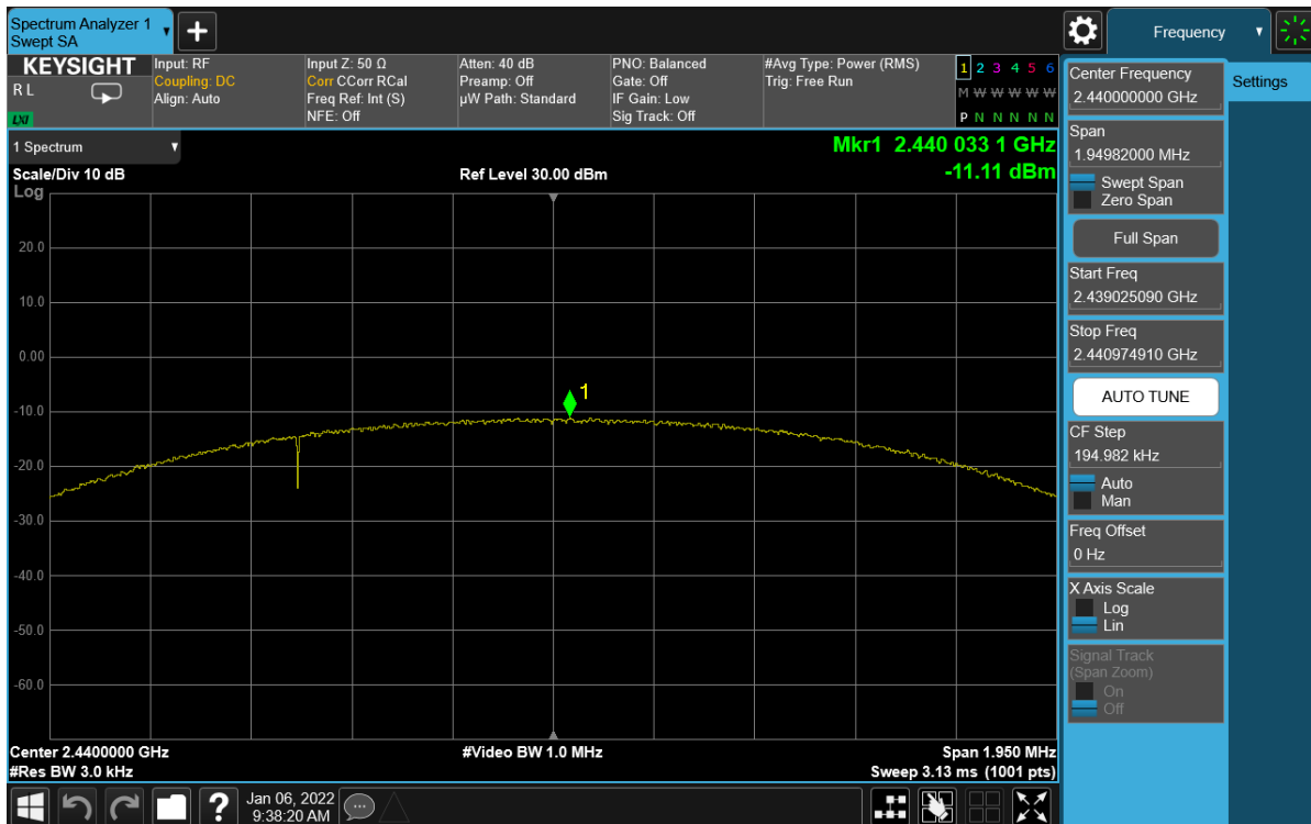
Plot 7-58. Power Spectral Density Plot Antenna WF7b (Bluetooth (LE), 2Mbps, iPA – Ch. 19)
