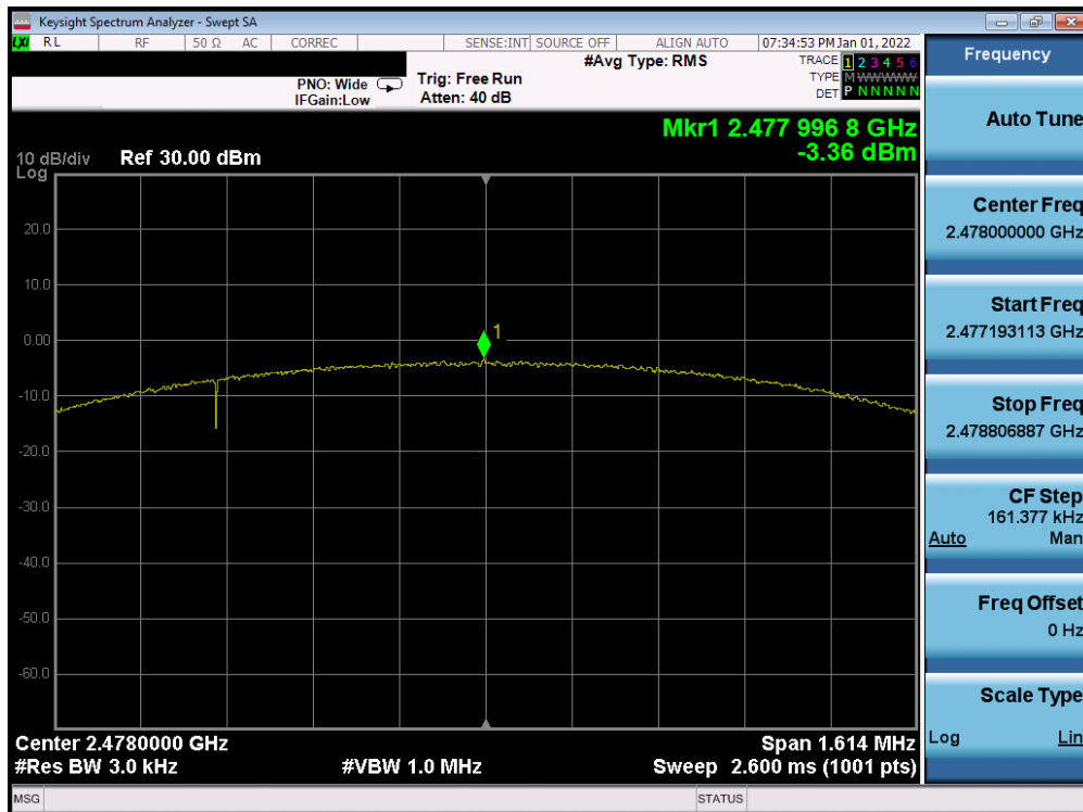
Plot 7-54. Power Spectral Density Plot Antenna WF7b (Bluetooth (LE), 2Mbps, ePA – Ch. 38)
