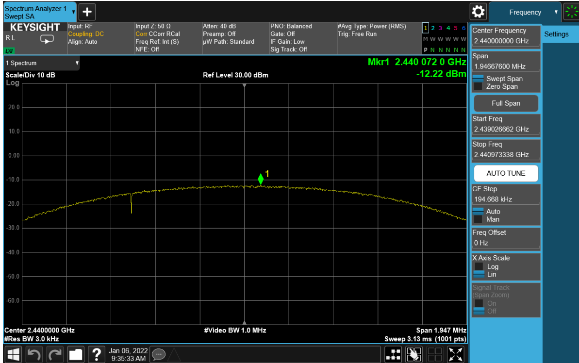
Plot 7-57. Power Spectral Density Plot Antenna WF8 (Bluetooth (LE), 2Mbps, iPA – Ch. 19)
