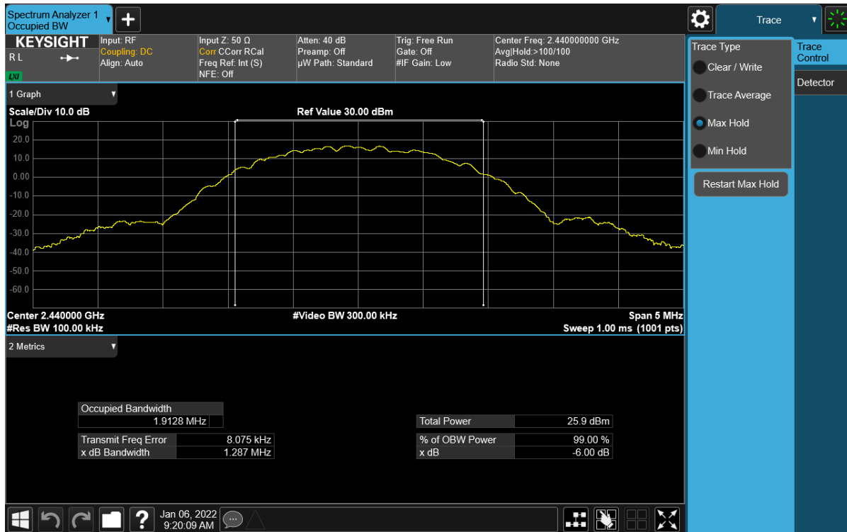
Plot 7-5. 6dB BW & 99% OBW Plot Antenna WF8 (Bluetooth (LE), 2Mbps, ePA – Ch. 19)
