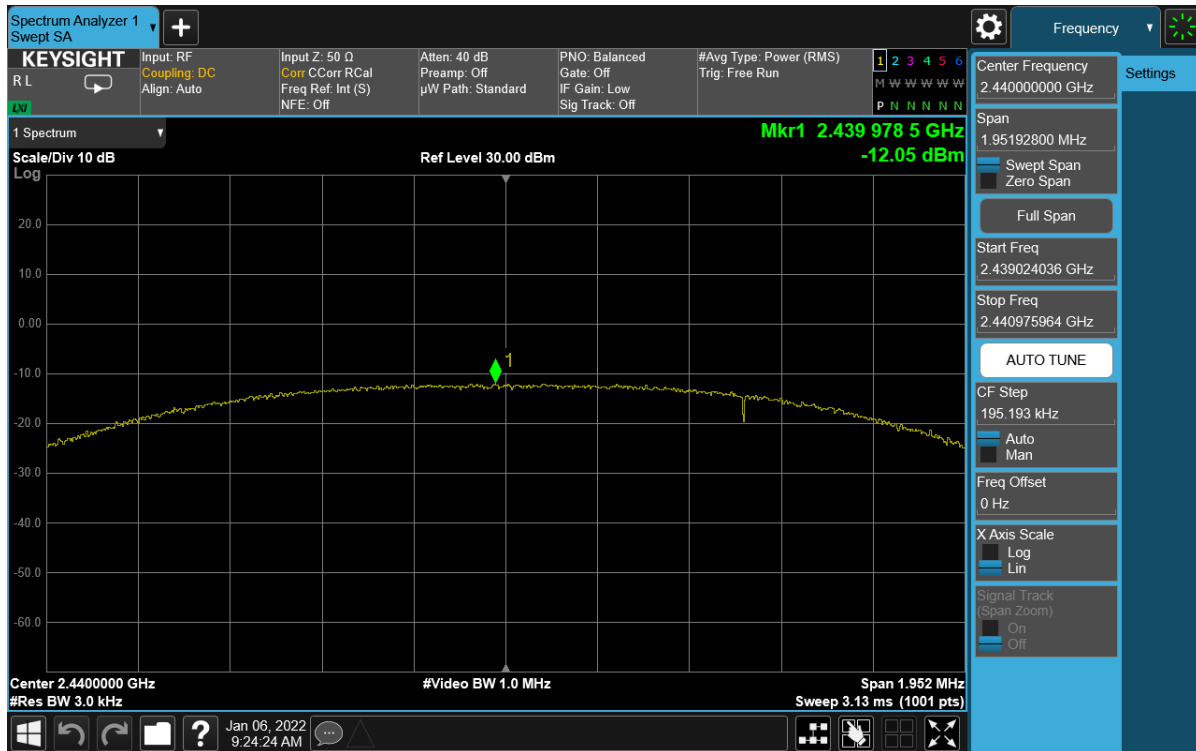
Plot 7-23. Power Spectral Density Plot Antenna WF8 (Bluetooth (LE), 2Mbps, iPA – Ch. 19)
