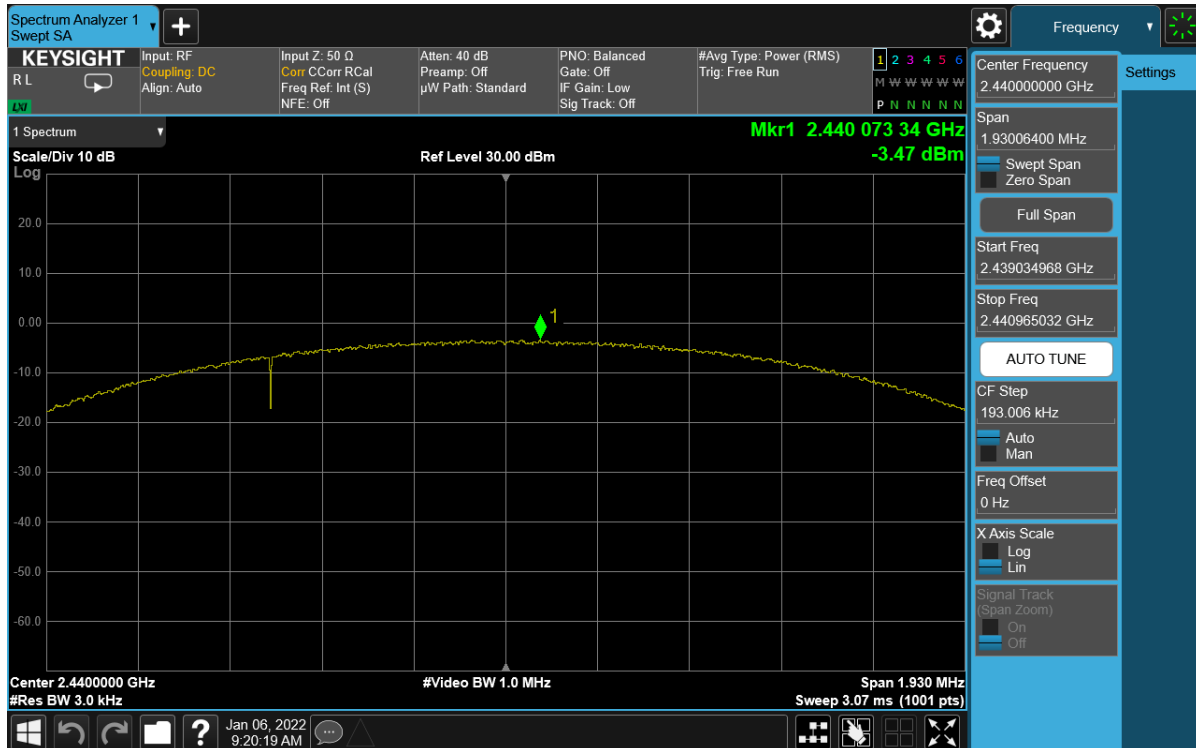
Plot 7-20. Power Spectral Density Plot Antenna WF8 (Bluetooth (LE), 2Mbps, ePA – Ch. 19)
