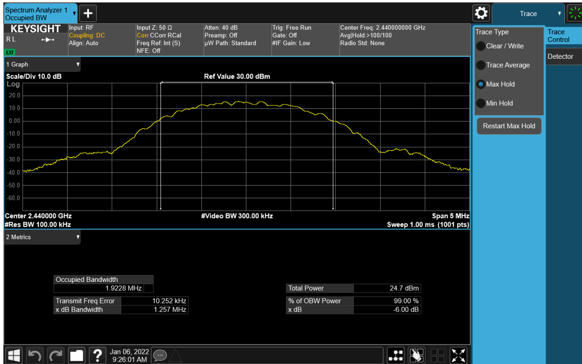
Plot 7-11. 6dB BW & 99% OBW Plot Antenna WF7b (Bluetooth (LE), 2Mbps, ePA – Ch. 19)
