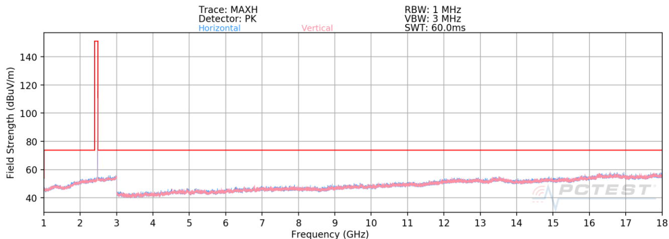
Plot 7-86. Radiated Spurious Emissions Above 1GHz Antenna WF7b (4Mbps, HDR4, ePA – Ch. 73)
