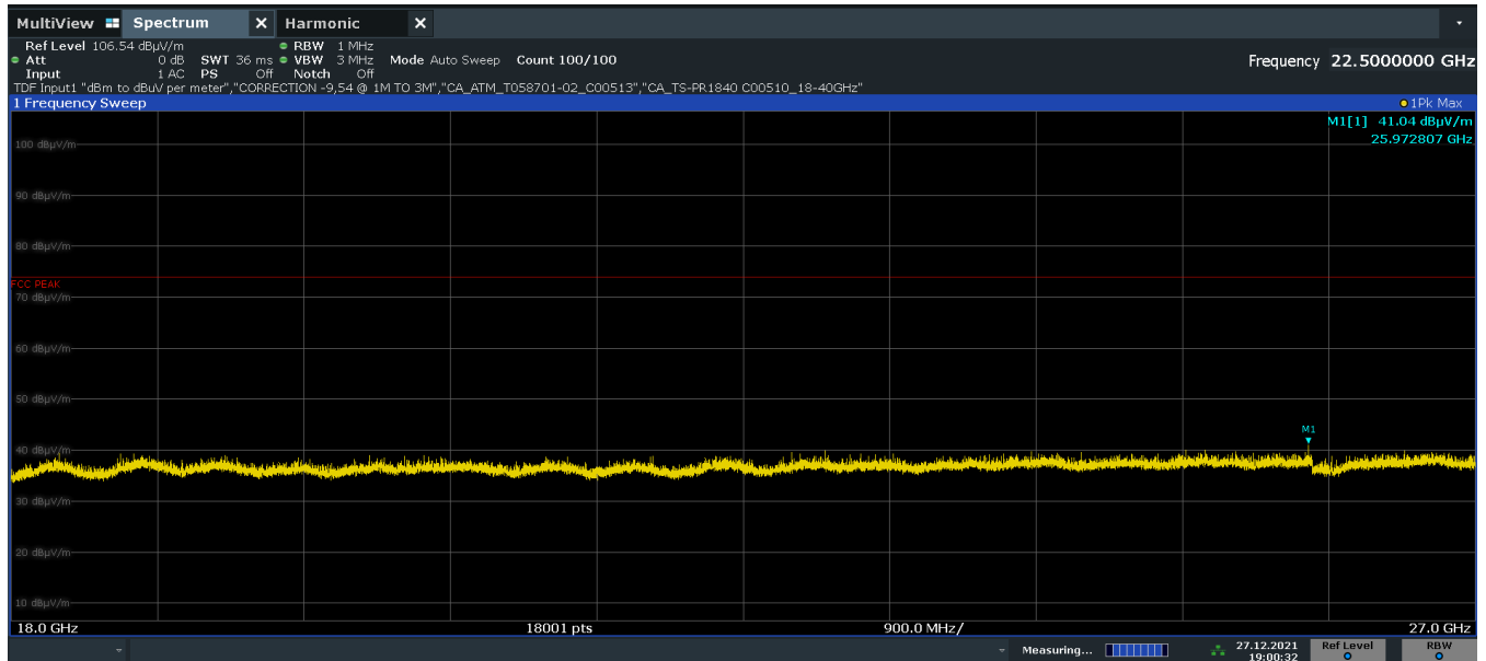
Plot 7-90. Radiated Spurious Emissions Above 18GHz TxBF (4Mbps – Ch.38, ePA, Ant. Pol. V)
