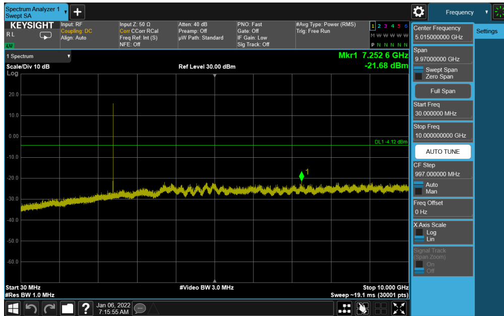
Plot 7-75. Conducted Spurious Plot Antenna WF7b (Bluetooth (HDR4), 4 Mbps, ePA – Ch. 1)
