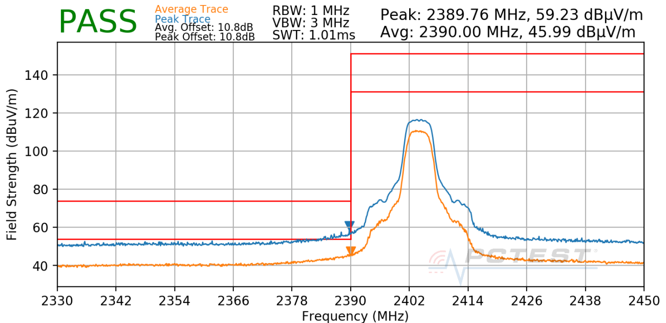
Plot 7-93. Radiated Restricted Lower Band Edge Measurement Antenna WF8 (Average & Peak)
