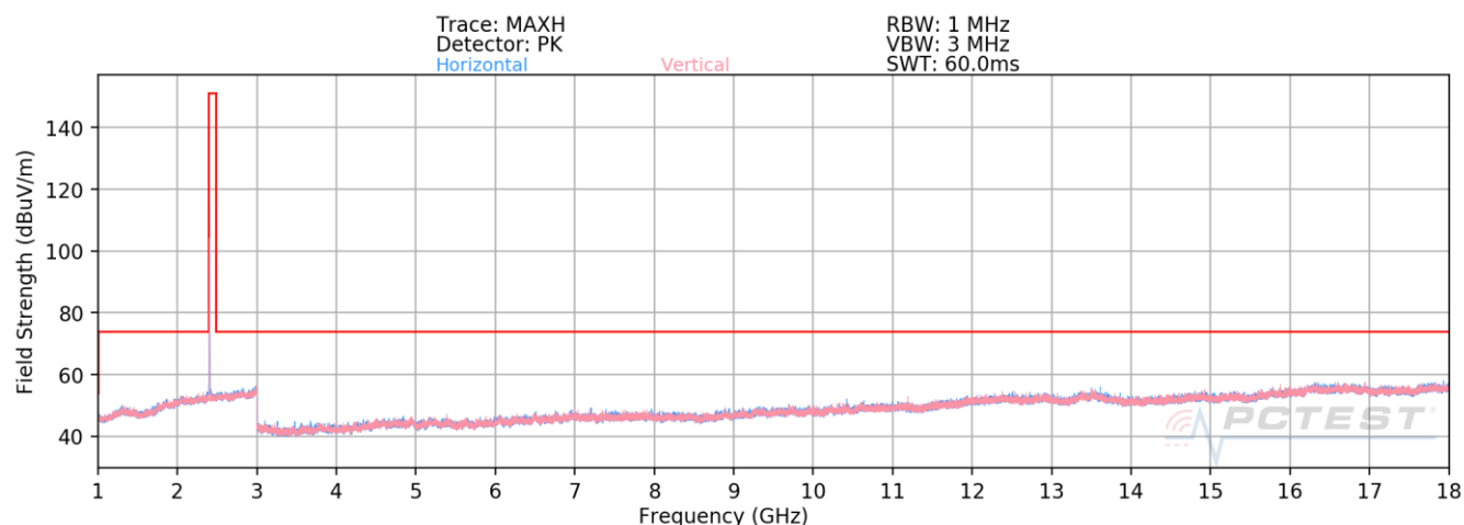
Plot 7-81. Radiated Spurious Emissions Above 1GHz Antenna WF8 (4Mbps, HDR4, ePA – Ch. 1)
