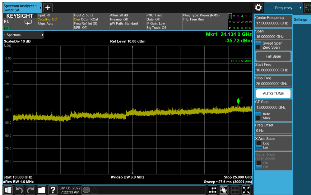
Plot 7-78. Conducted Spurious Plot Antenna WF7b (Bluetooth (HDR4), 4 Mbps, ePA – Ch. 38)
