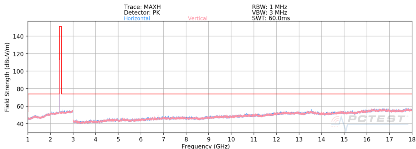
Plot 7-84. Radiated Spurious Emissions Above 1GHz Antenna WF7b (4Mbps, HDR4, ePA – Ch. 1)
