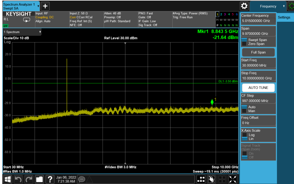
Plot 7-77. Conducted Spurious Plot Antenna WF7b (Bluetooth (HDR4), 4 Mbps, ePA – Ch. 38)
