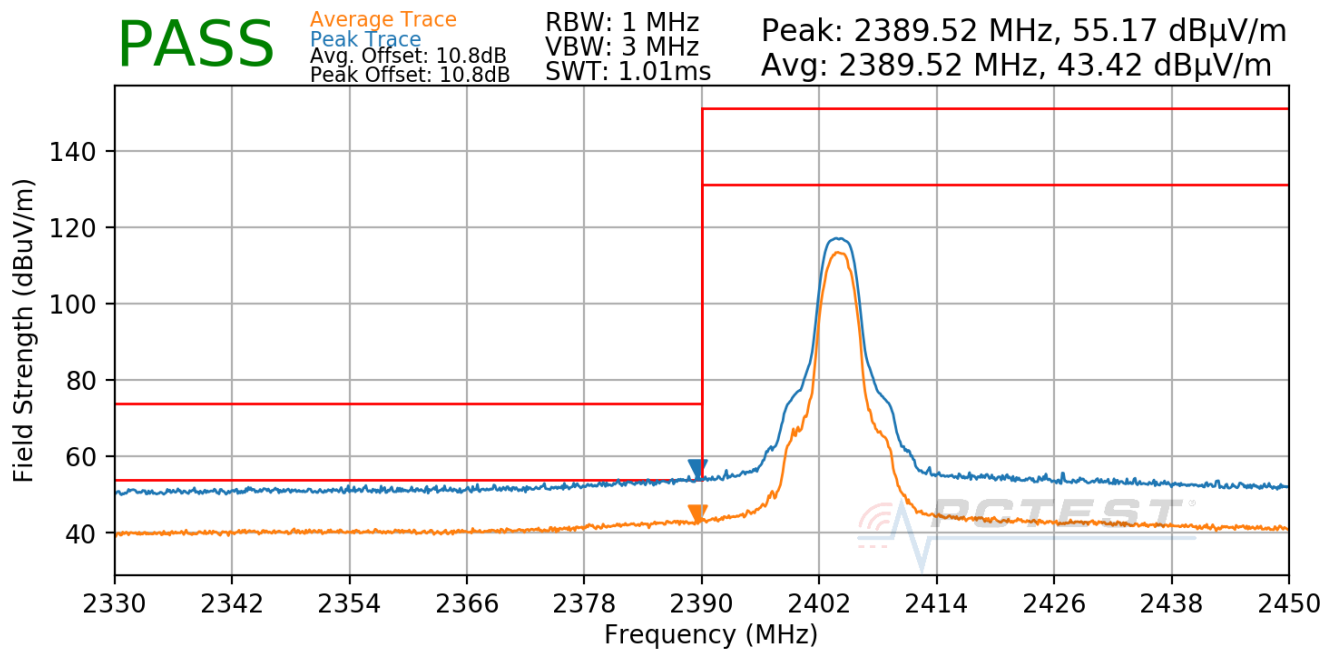
Plot 7-92. Radiated Restricted Lower Band Edge Measurement Antenna WF8 (Average & Peak)
