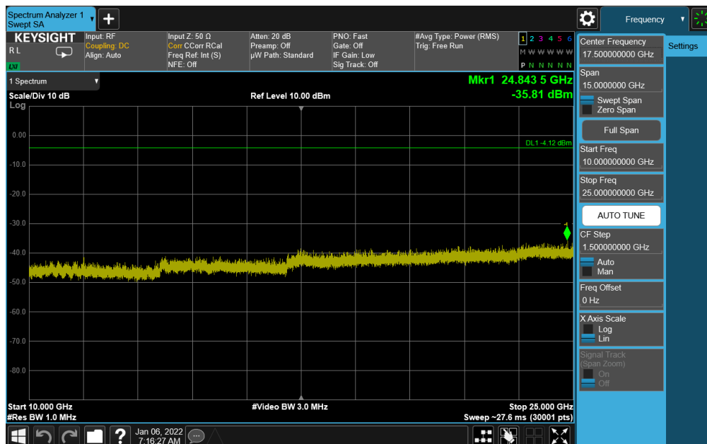
Plot 7-76. Conducted Spurious Plot Antenna WF7b (Bluetooth (HDR4), 4 Mbps, ePA – Ch. 1)
