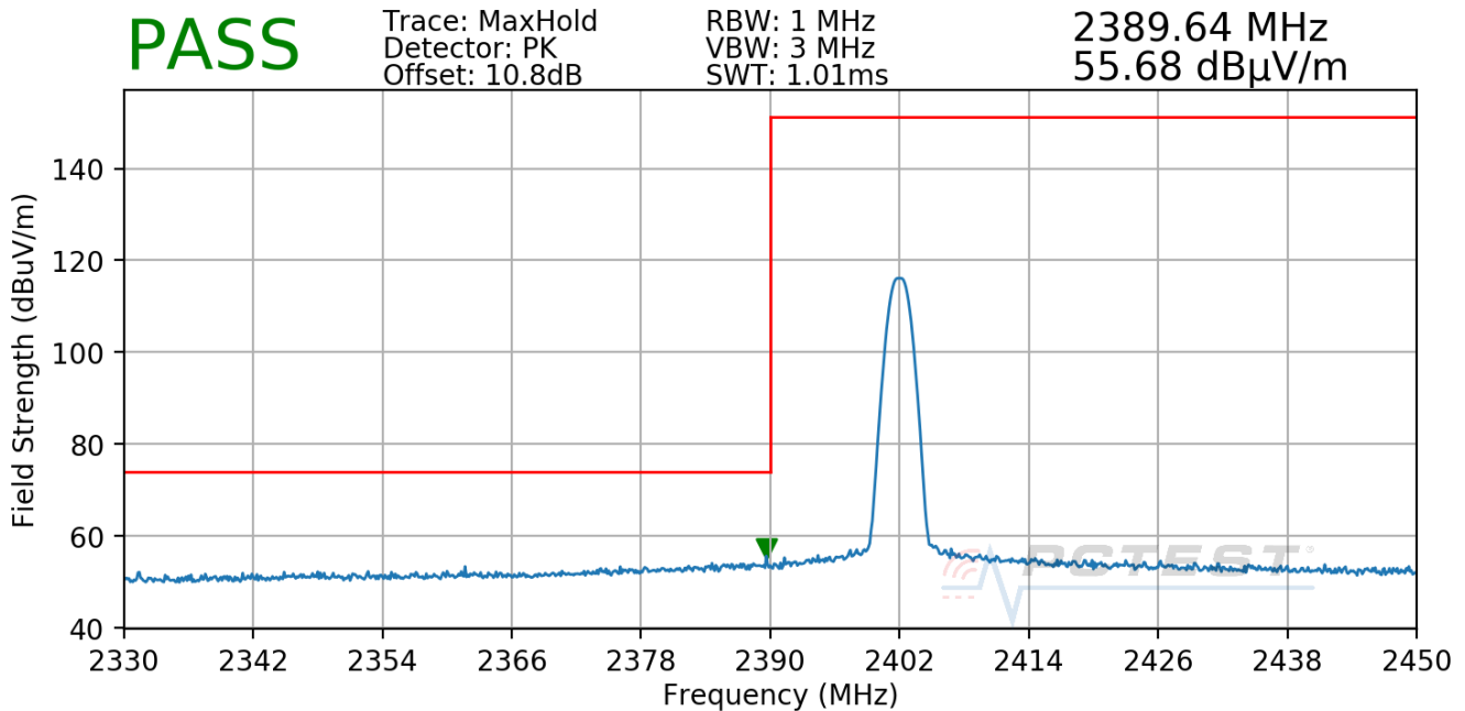
Plot 7-72. Radiated Restricted Lower Band Edge Measurement Antenna WF7b
