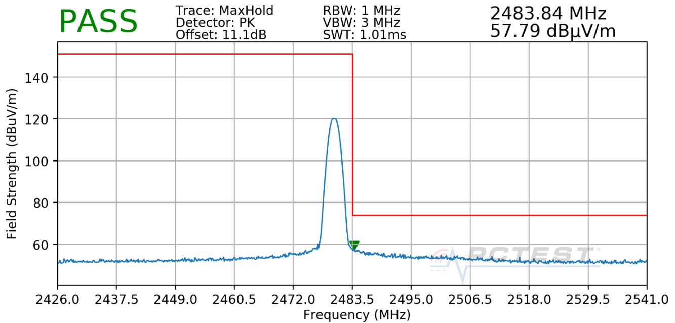
Plot 7-78. Radiated Restricted Upper Band Edge Measurement TxBF
