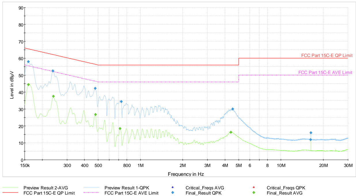
Plot 7-81. AC Line-Conducted Test Plot TxBF (L1, GFSK ePA – Ch.39, with AC/DC Adapter)
