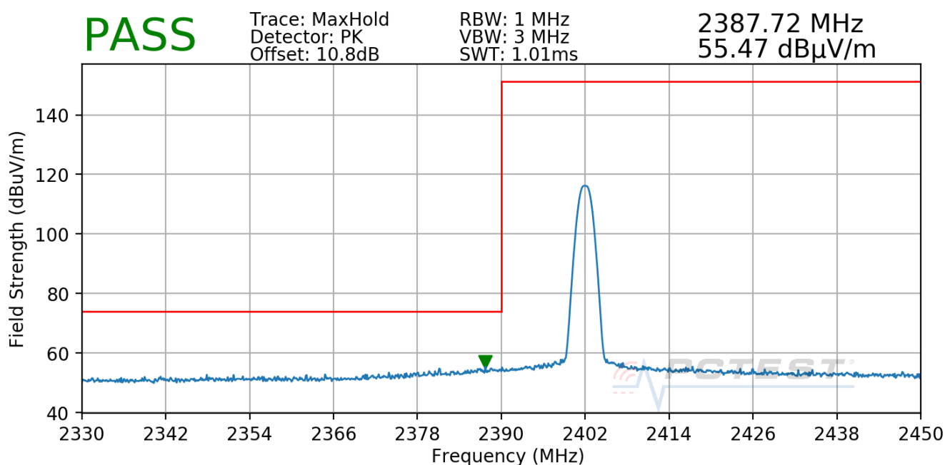
Plot 7-68. Radiated Restricted Lower Band Edge Measurement Antenna WF8
