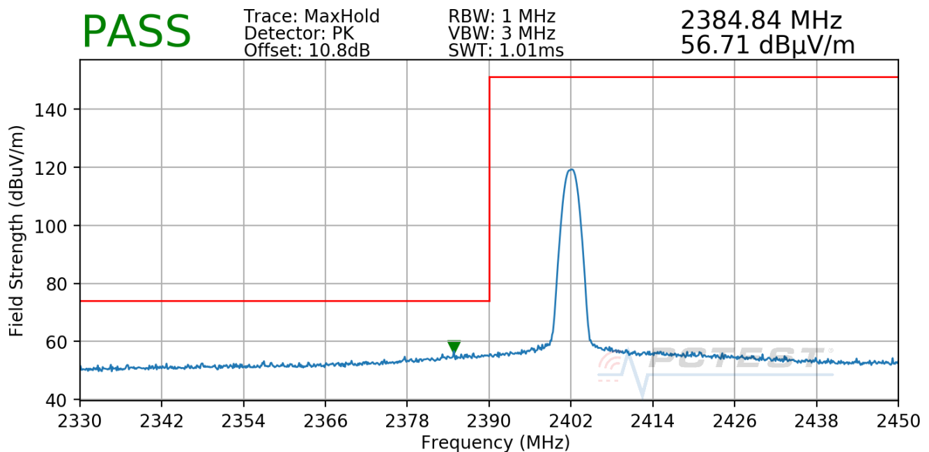
Plot 7-76. Radiated Restricted Lower Band Edge Measurement TxBF
