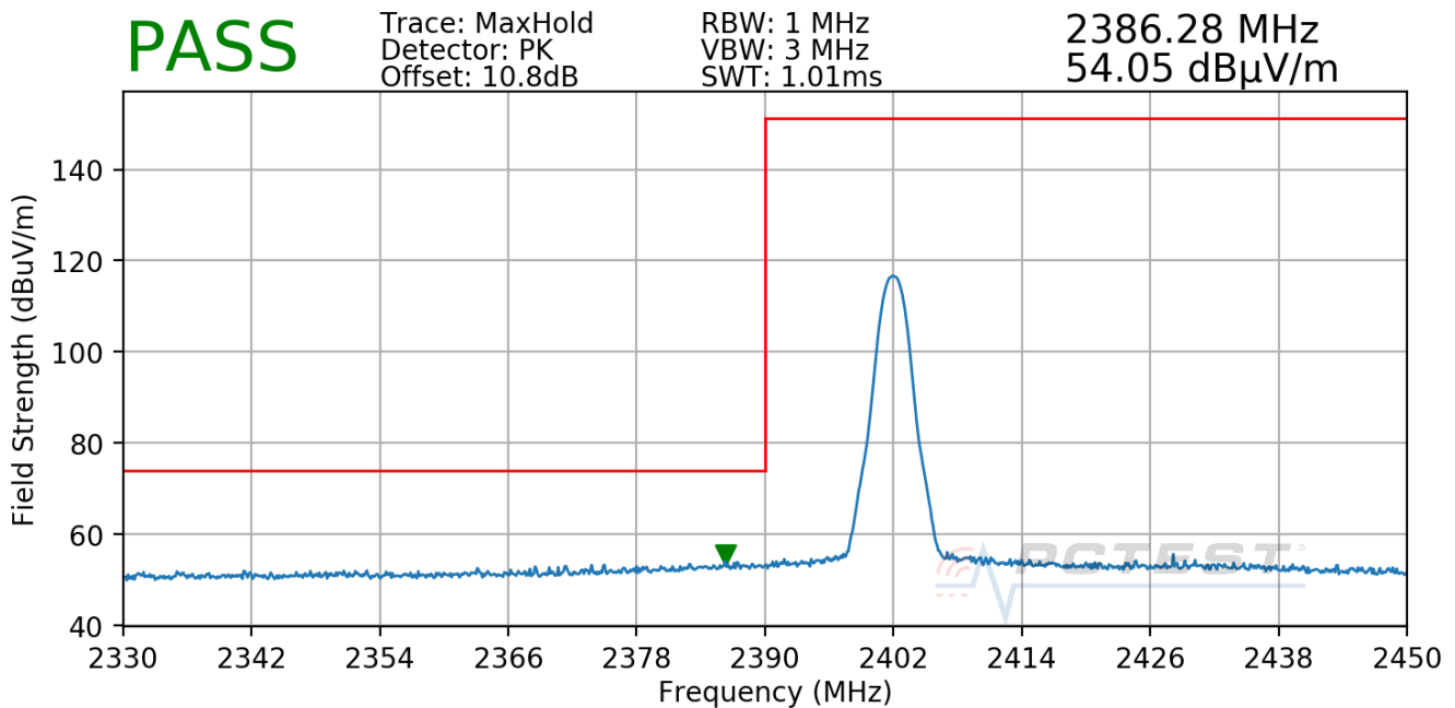
Plot 7-73. Radiated Restricted Lower Band Edge Measurement Antenna WF7b
