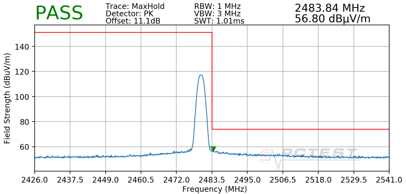
Plot 7-74. Radiated Restricted Upper Band Edge Measurement Antenna WF7b
