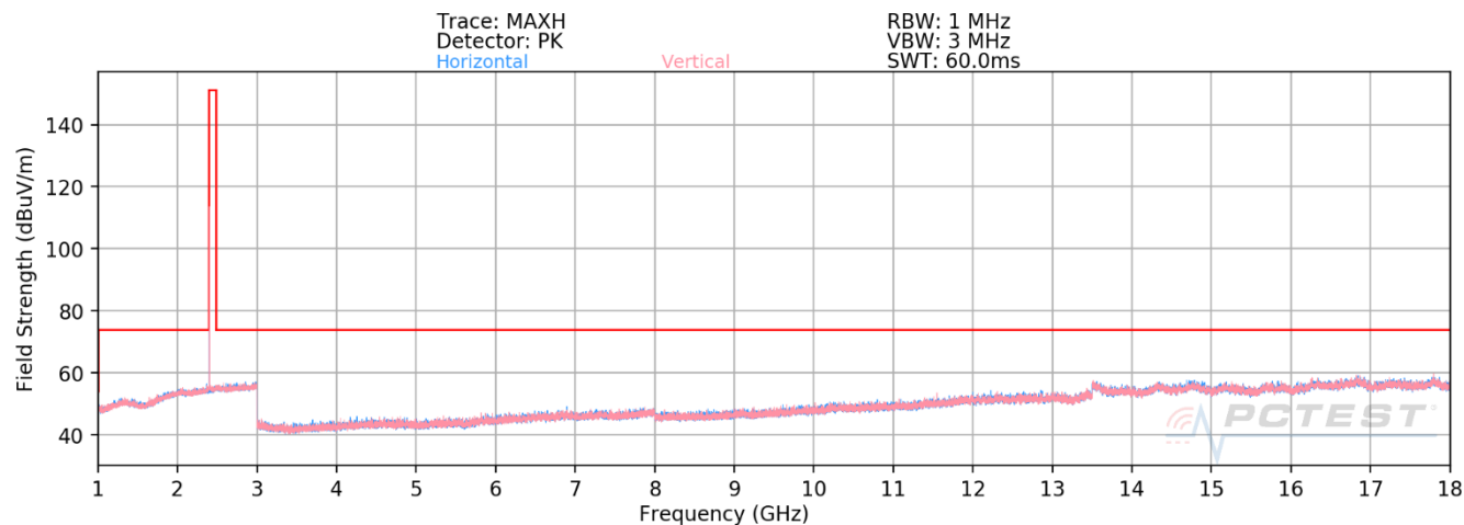
Plot 7-60. Radiated Spurious Emissions above 1GHz Antenna WF7b (BT GFSK ePA – Ch. 0)
