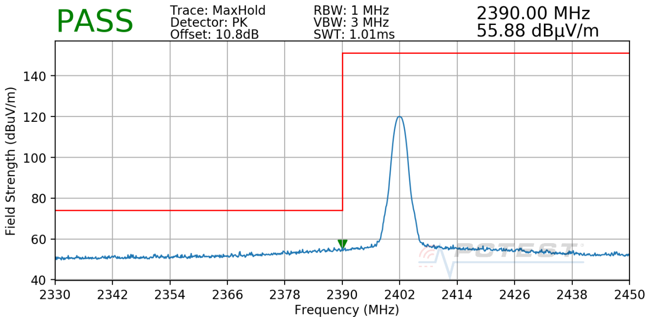
Plot 7-77. Radiated Restricted Lower Band Edge Measurement TxBF
