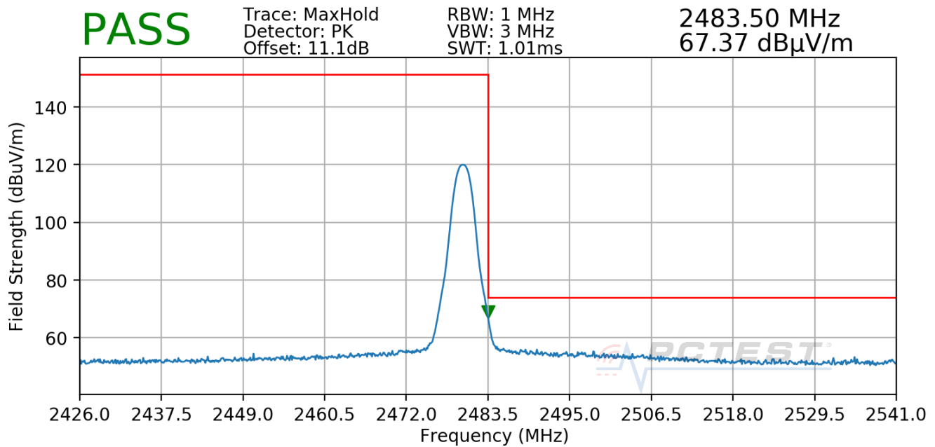
Plot 7-79. Radiated Restricted Upper Band Edge Measurement TxBF
