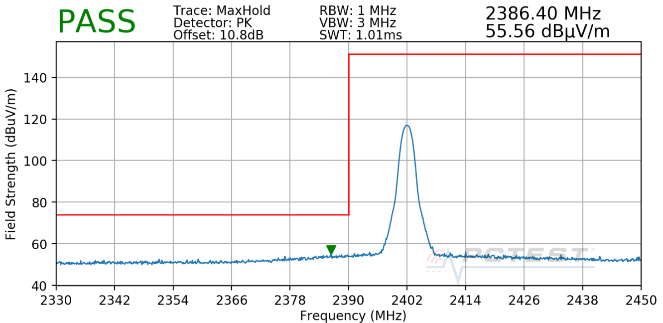
Plot 7-69. Radiated Restricted Lower Band Edge Measurement Antenna WF8
