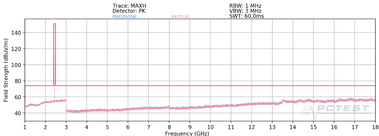
Plot 7-61. Radiated Spurious Emissions above 1GHz Antenna WF7b (BT GFSK ePA – Ch. 39)
