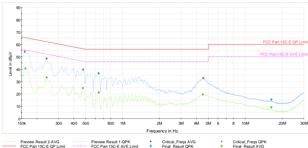
Plot 7-82. AC Line-Conducted Test Plot TxBF (N, GFSK ePA – Ch.39, with AC/DC Adapter)
