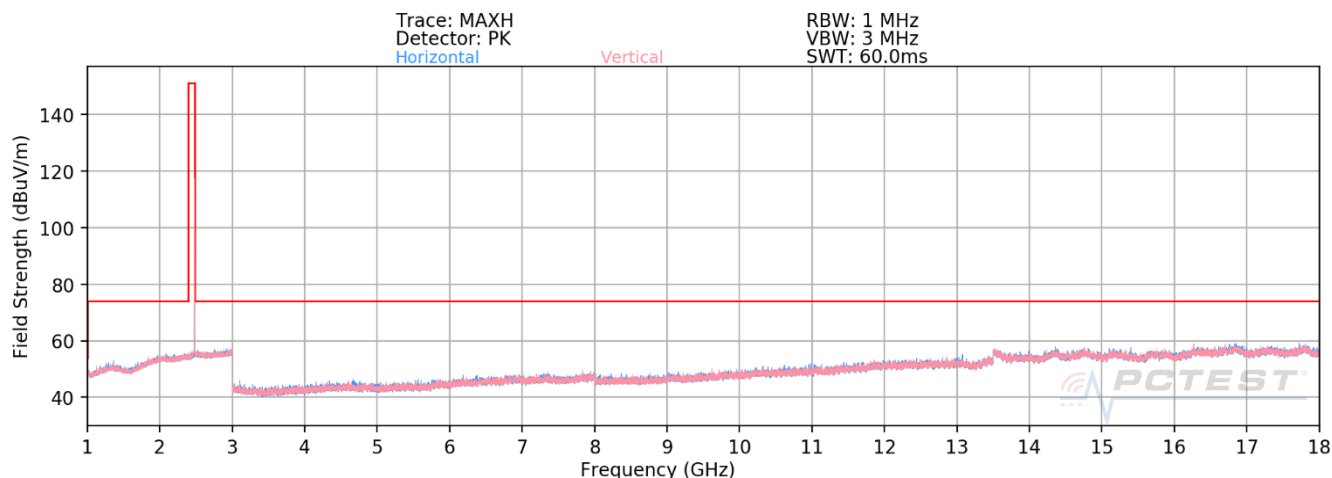
Plot 7-67. Radiated Spurious Emissions above 1GHz TxBF (BT GFSK ePA – Ch. 78)
