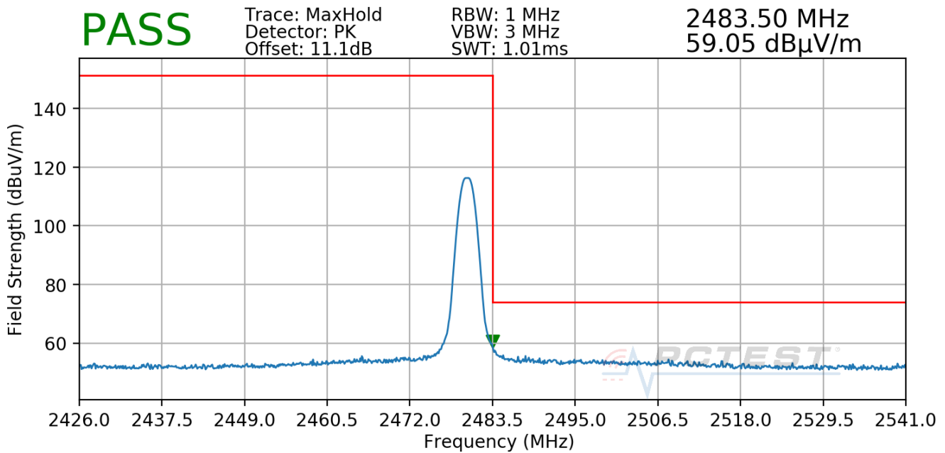
Plot 7-70. Radiated Restricted Upper Band Edge Measurement Antenna WF8
