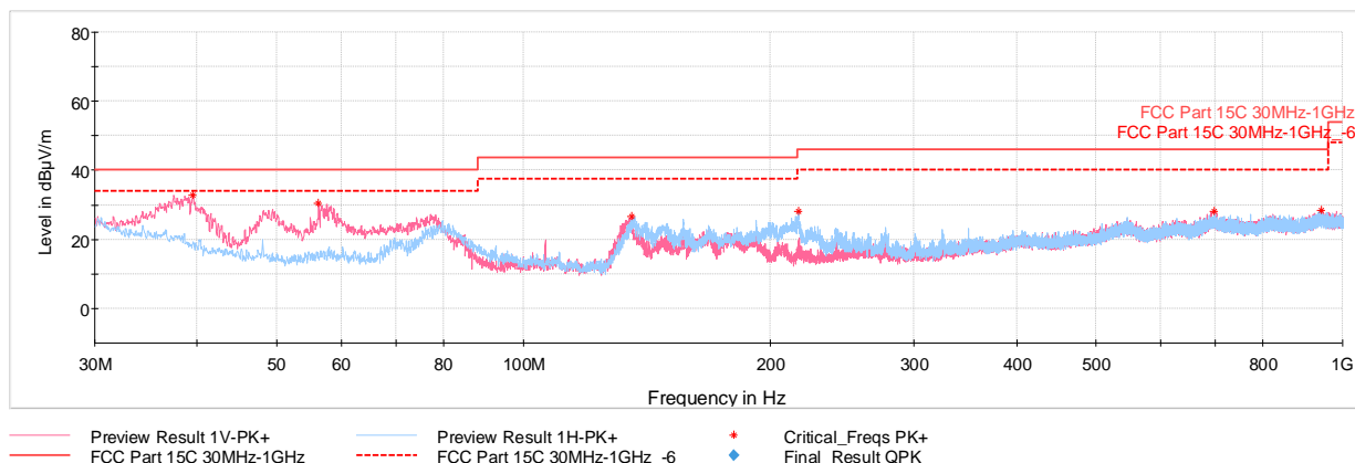
Plot 7-80. Radiated Spurious Emissions Below 1GHz TxBF (GFSK ePA – Ch.39, with AC/DC Adapter)
