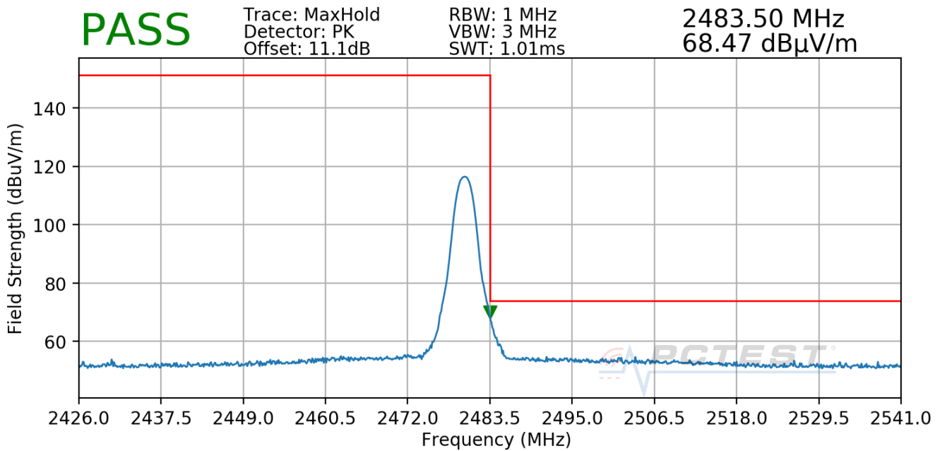
Plot 7-71. Radiated Restricted Upper Band Edge Measurement Antenna WF8
