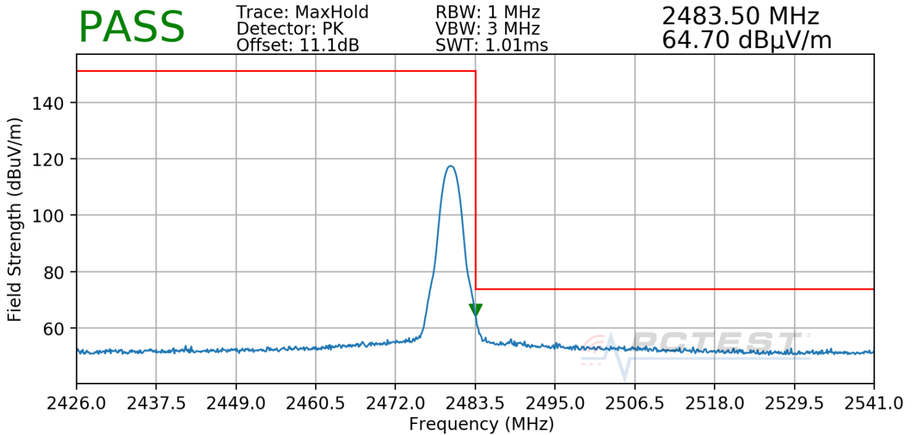
Plot 7-75. Radiated Restricted Upper Band Edge Measurement Antenna WF7b
