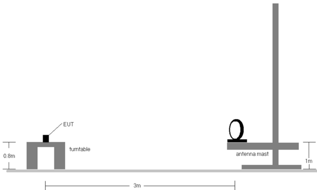
Figure 6-1. Test Setup
