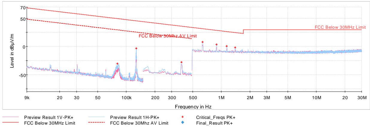
Plot 6-3. Radiated Spurious Emissions 9kHz-30MHz (Charging Rate 10C, with AC/DC Adapter)
