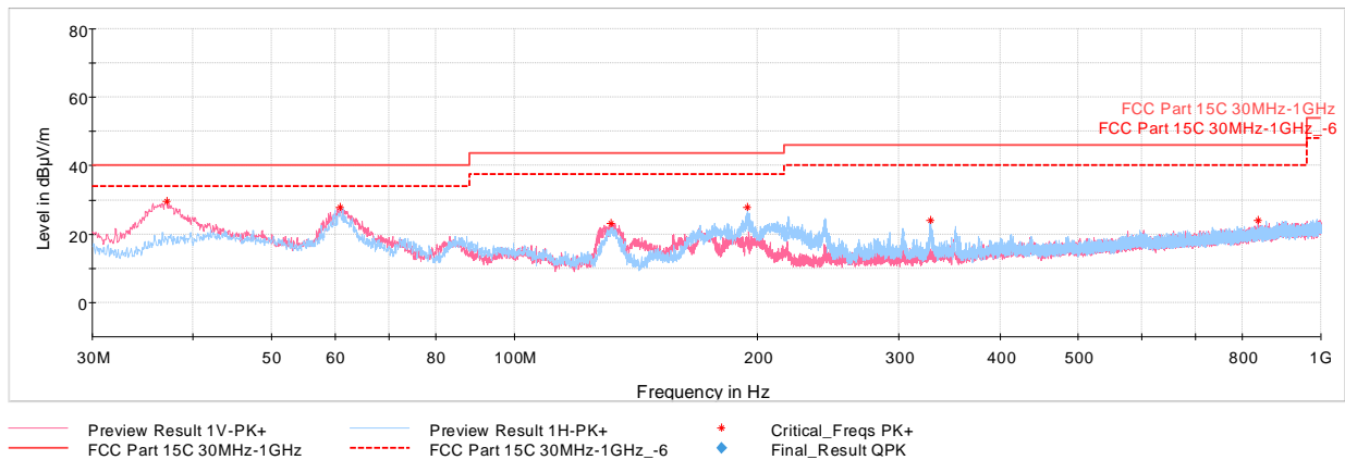
Plot 6-4. Radiated Spurious Emissions 30MHz-1GHz (Charging Rate 10C, with AC/DC Adapter)
