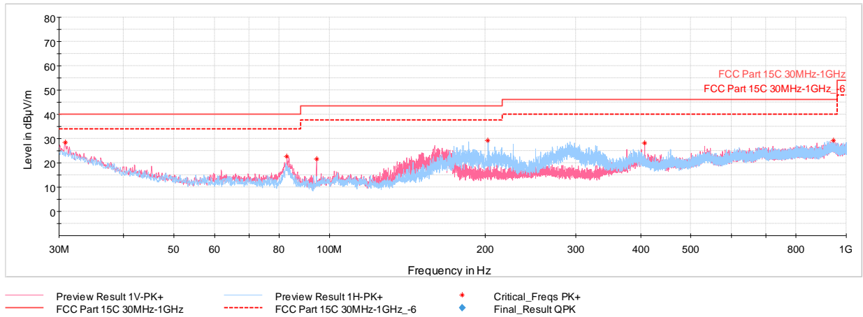
Plot 7-38. Radiated Spurious Plot below 1GHz (GFSK – Ch.39, Pol. H & V, with charging case powered by Host PC via USB-C cable)
