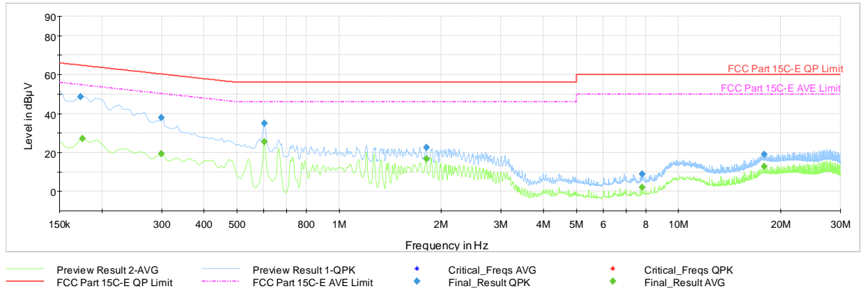
Plot 7-40. AC Line-Conducted Emissions (N, GFSK – Ch.39 with charging case powered by Host PC via USB-C cable)
