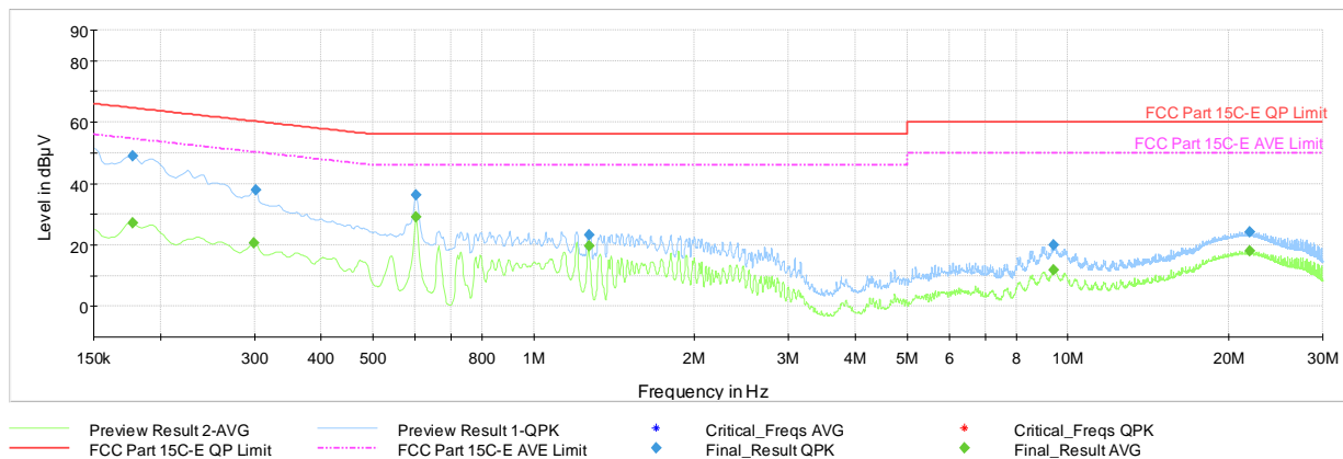
Plot 7-39. AC Line-Conducted Emissions (L1, GFSK – Ch.39 with charging case powered by Host PC via USB-C cable)
