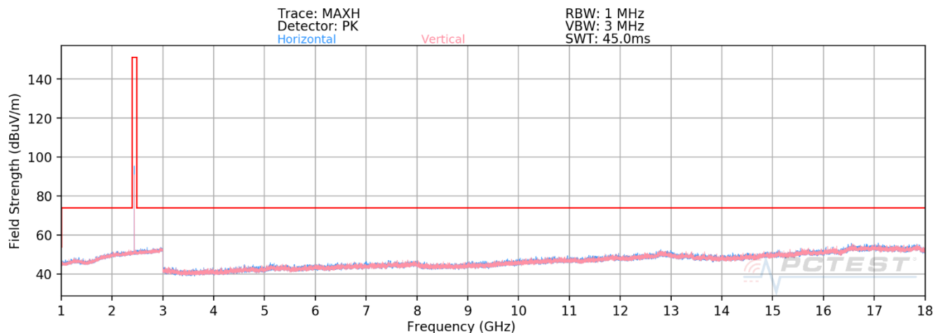
Plot 7-24. Radiated Spurious Emissions Above 1GHz (1Mbps – Ch. 19, Ant. Pol. H & V)
