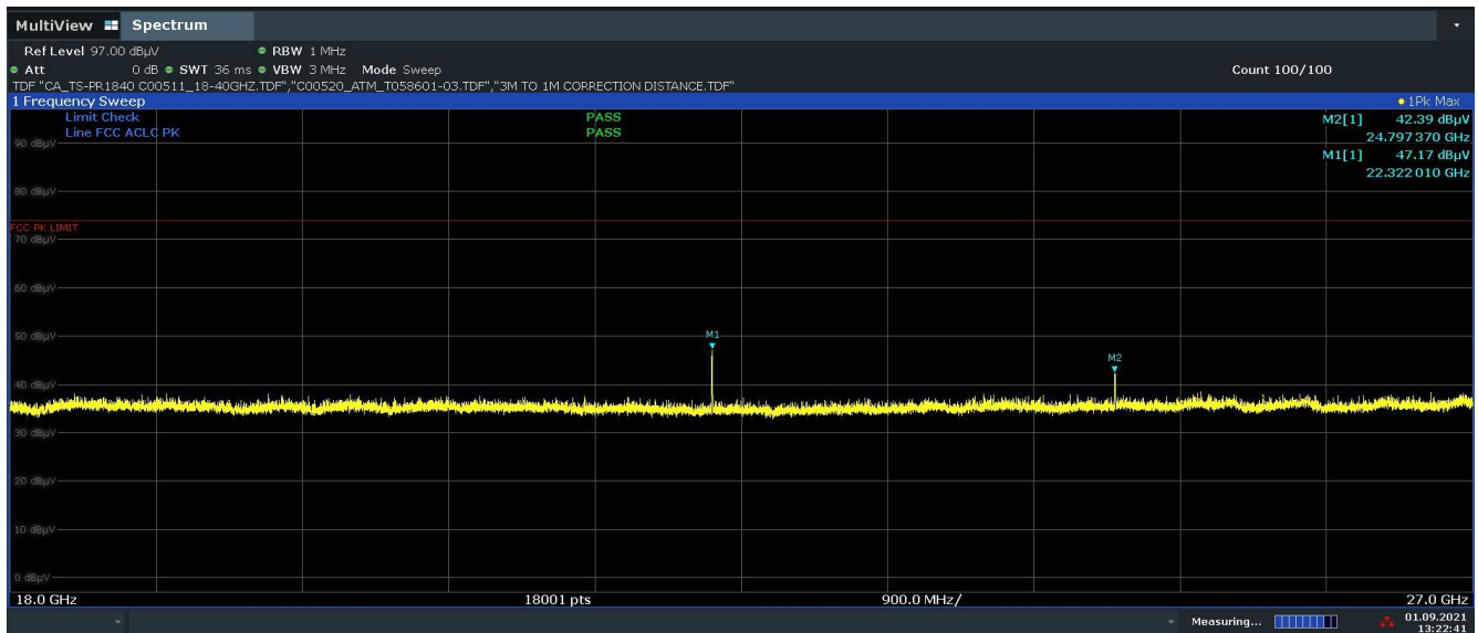
Plot 7-27. Radiated Spurious Emissions Above 18GHz (1Mbps – Ch.39, Pol. V)
