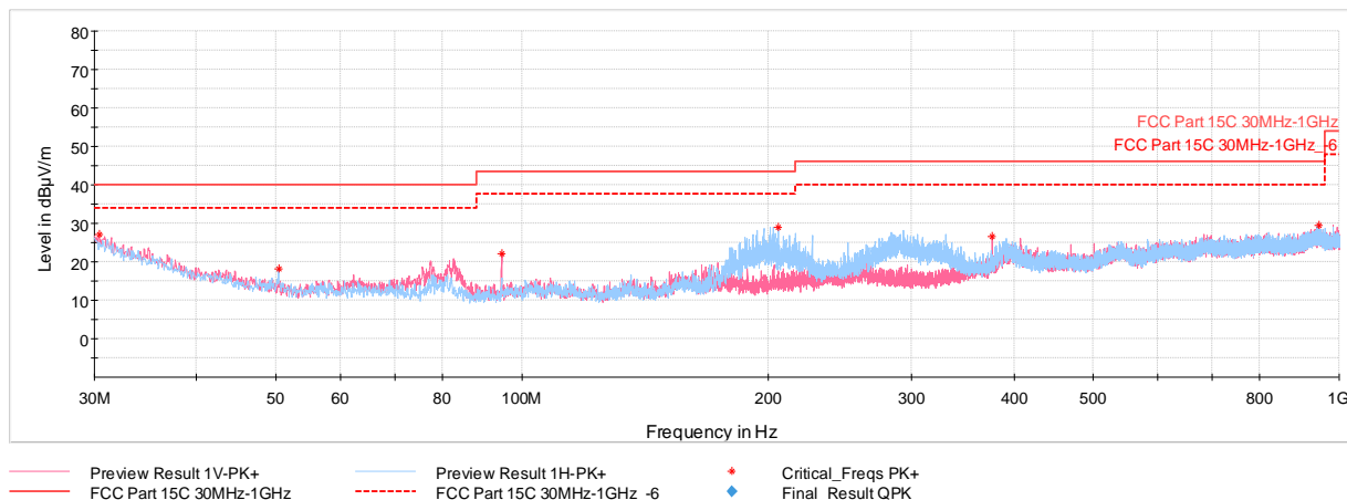
Plot 7-32. Radiated Spurious Emissions Below 1GHz (1Mbps – Ch.19, Pol. H & V, with charging case powered by Host PC via USB-C cable)
