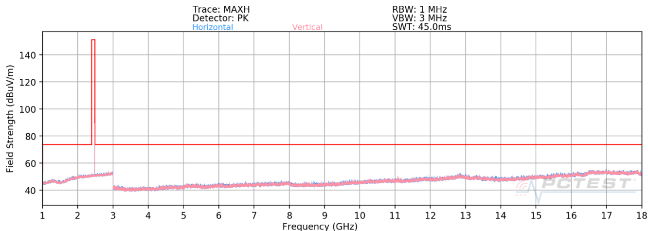
Plot 7-25. Radiated Spurious Emissions Above 1GHz (1Mbps – Ch. 39, Ant. Pol. H & V)
