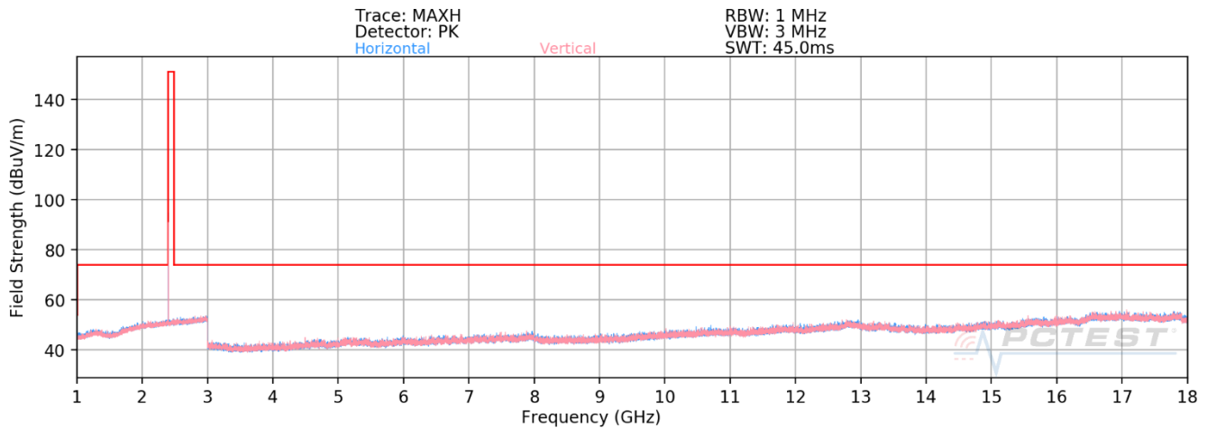
Plot 7-23. Radiated Spurious Emissions Above 1GHz (1Mbps – Ch. 0, Ant. Pol. H & V)
