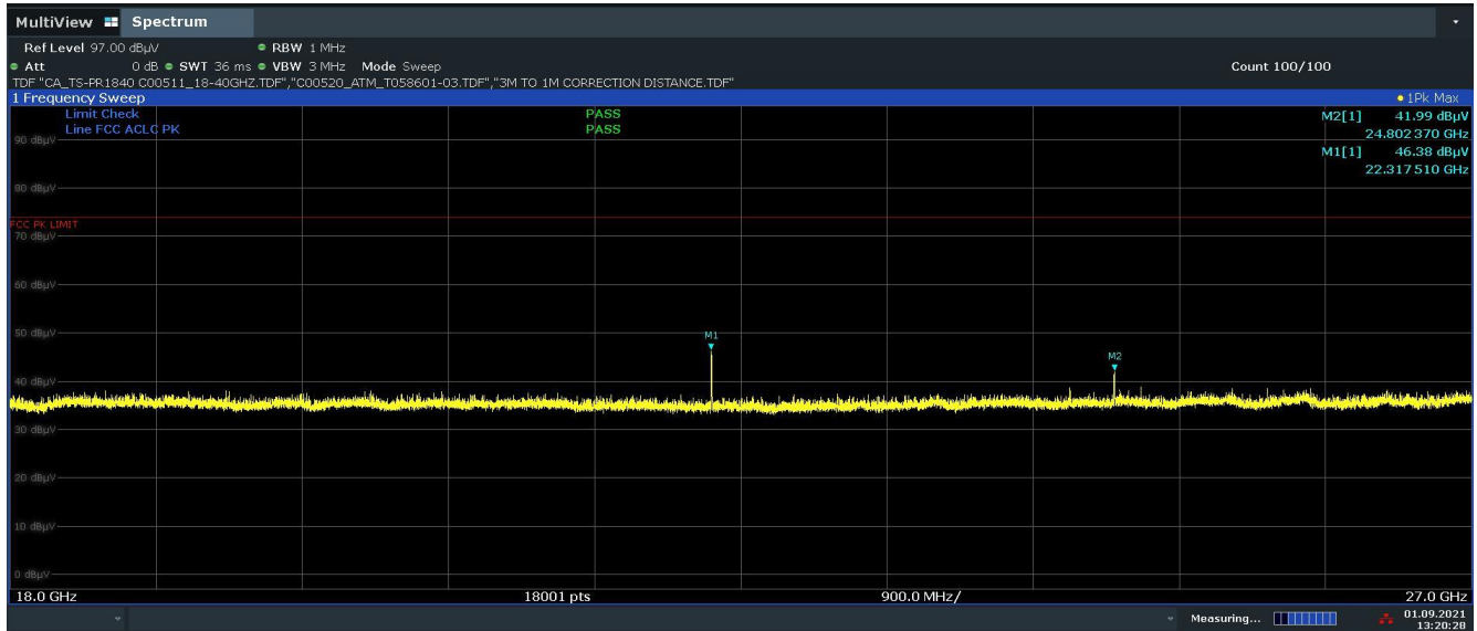
Plot 7-26. Radiated Spurious Emissions Above 18GHz (1Mbps – Ch.39, Pol. H)
