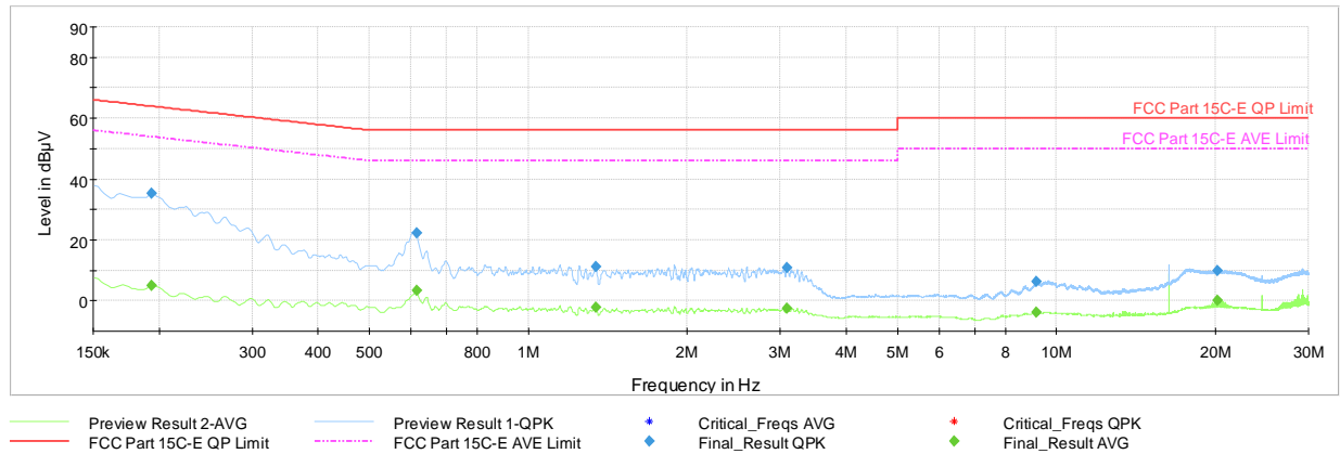
Plot 7-34. AC Line Conducted Emissions with Bluetooth LE (1Mbps – Ch.19, N, with charging case powered by Host PC via USB-C cable)
