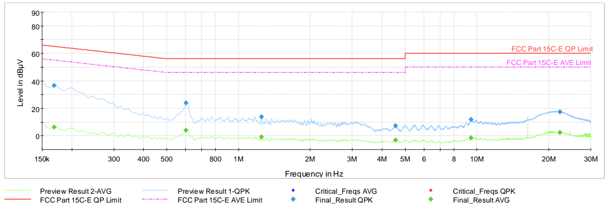
Plot 7-33. AC Line Conducted Emissions with Bluetooth LE (1Mbps – Ch.19, L1, with charging case powered by Host PC via USB-C cable)
