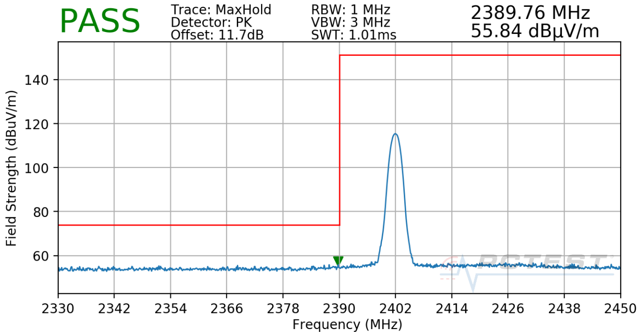
Plot 7-80. Radiated Restricted Lower Band Edge Measurement TxBF (Peak)
