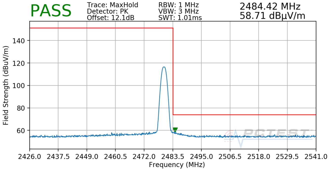
Plot 7-81. Radiated Restricted Upper Band Edge Measurement TxBF (Peak)
