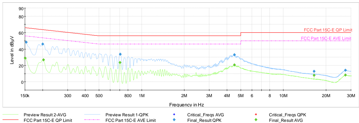
Plot 7-86. AC Line-Conducted Test Plot TxBF (N, GFSK ePA – Ch.0, with AC/DC Adapter)
