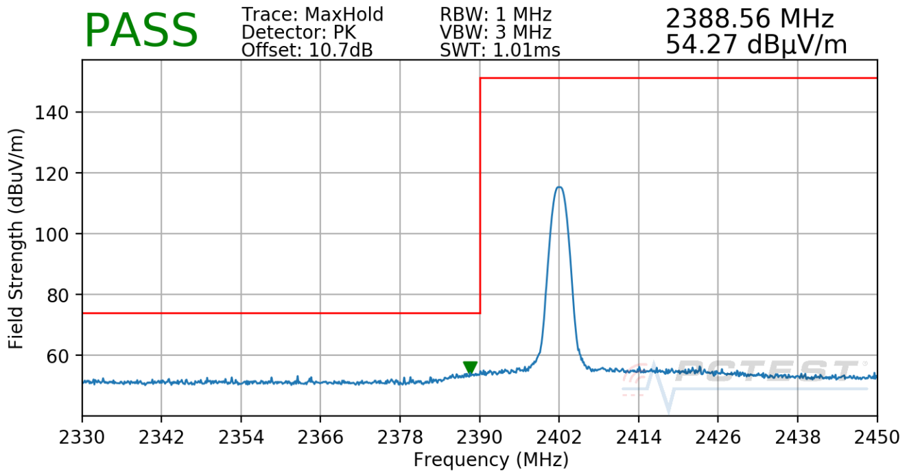
Plot 7-71. Radiated Restricted Lower Band Edge Measurement Antenna 3a (Peak)
