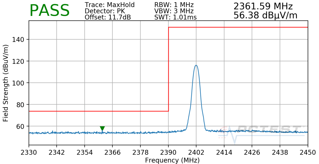
Plot 7-76. Radiated Restricted Lower Band Edge Measurement Antenna 1a (Peak)
