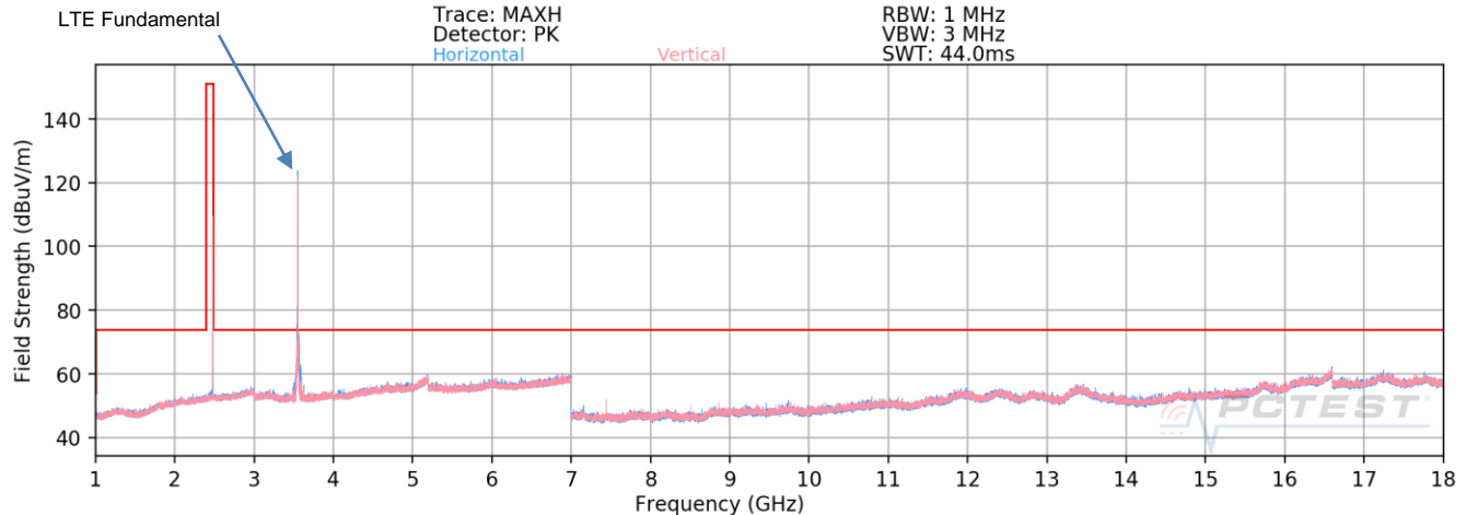
Plot 7-66. Radiated Spurious Emissions above 1GHz Simultaneous Tx
