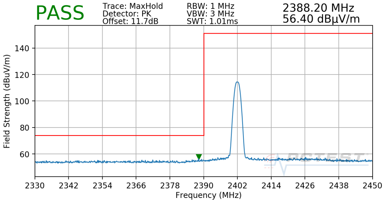
Plot 7-79. Radiated Restricted Lower Band Edge Measurement TxBF (Peak)
