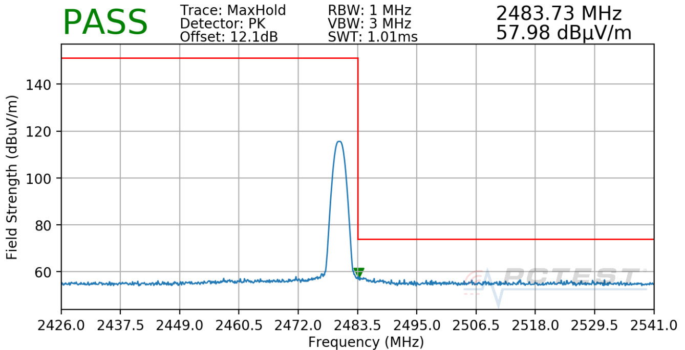
Plot 7-77. Radiated Restricted Upper Band Edge Measurement Antenna 1a (Peak)
