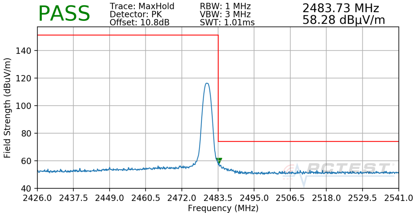
Plot 7-73. Radiated Restricted Upper Band Edge Measurement Antenna 3a (Peak)
