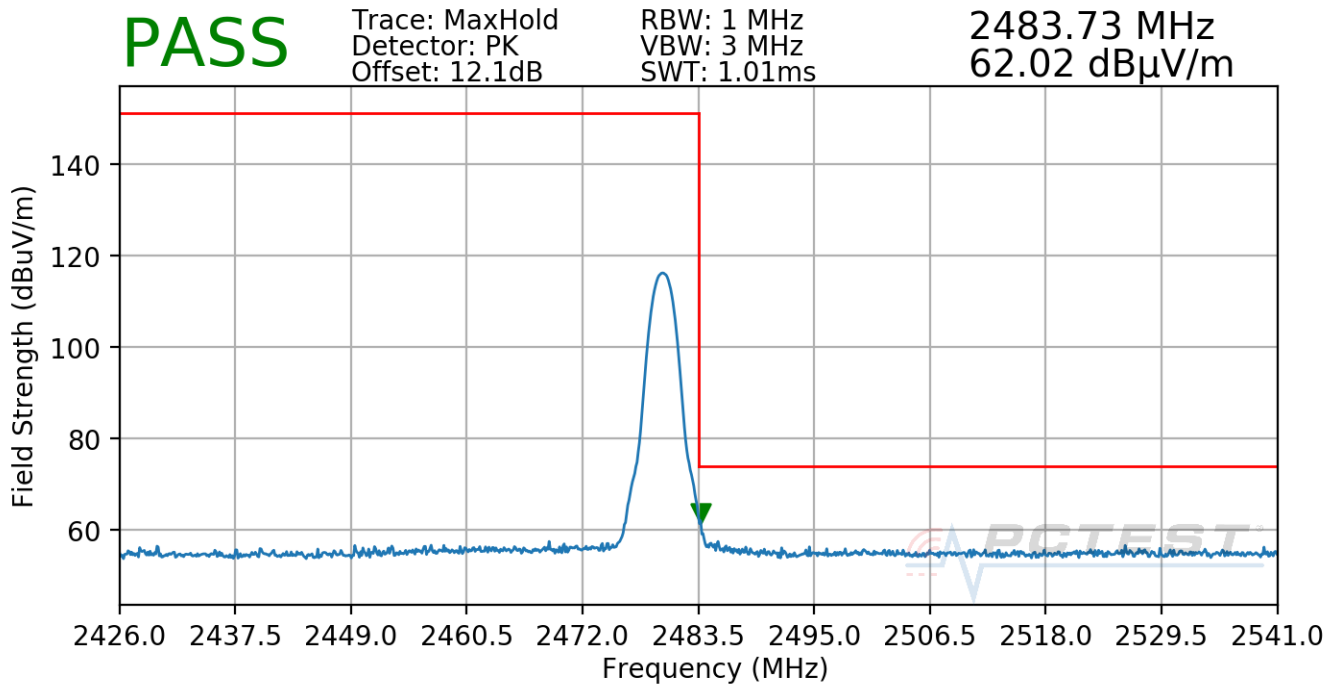
Plot 7-78. Radiated Restricted Upper Band Edge Measurement Antenna 1a (Peak)
