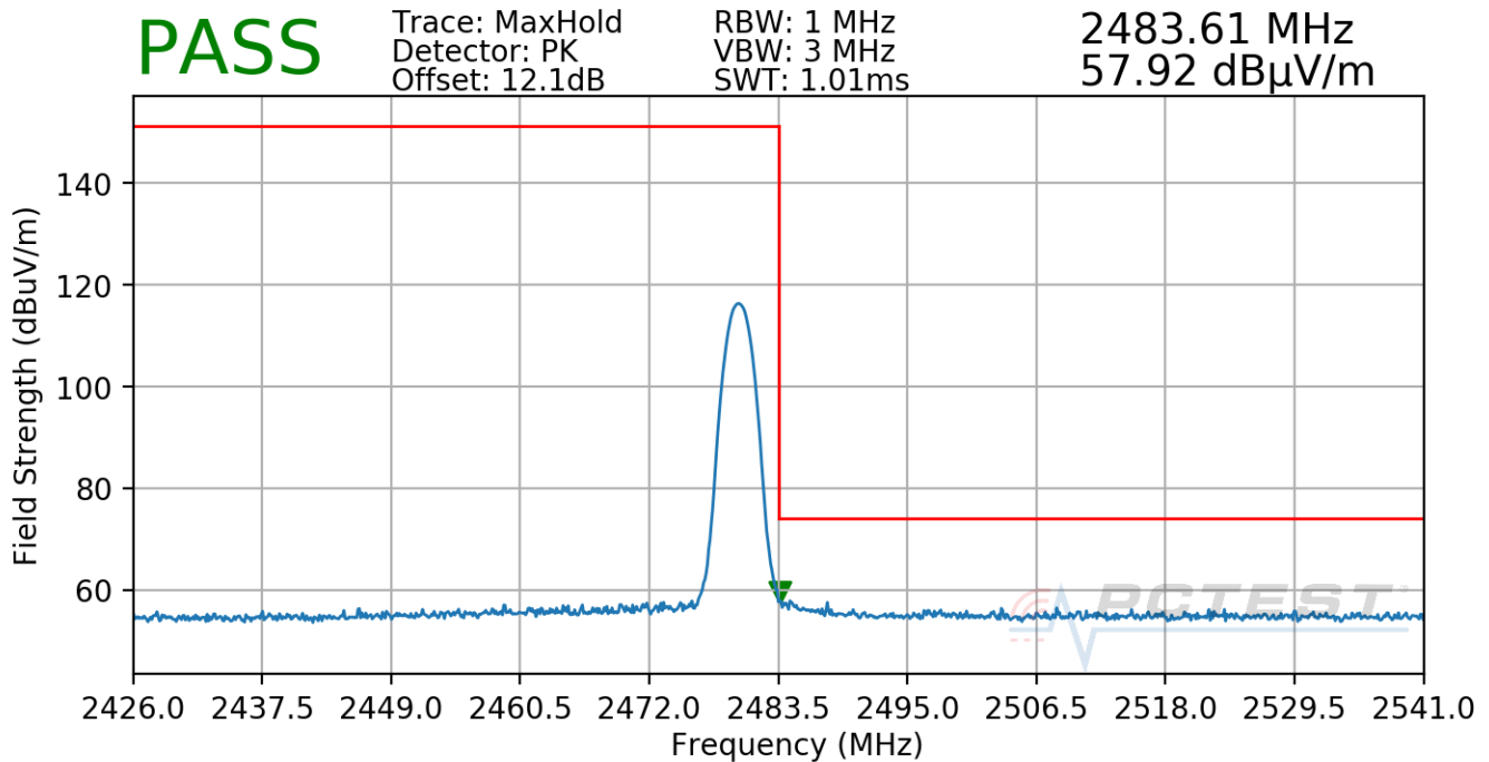
Plot 7-82. Radiated Restricted Upper Band Edge Measurement TxBF (Peak)
