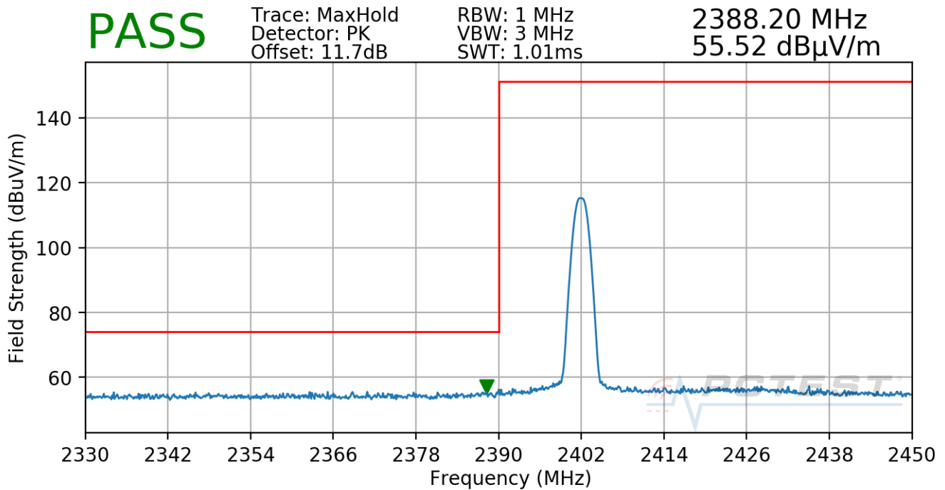
Plot 7-75. Radiated Restricted Lower Band Edge Measurement Antenna 1a (Peak)
