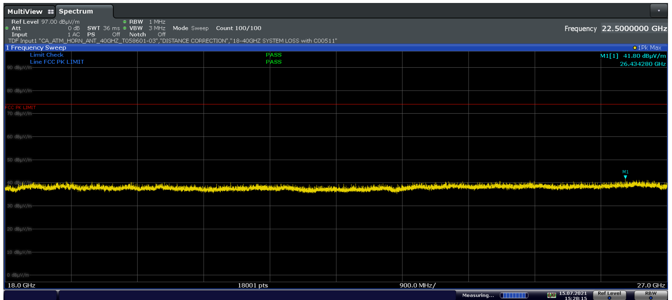
Plot 7-68. Radiated Spurious Emissions above 18GHz TxBF (GFSK ePA – Ch.39, Pol. V)
