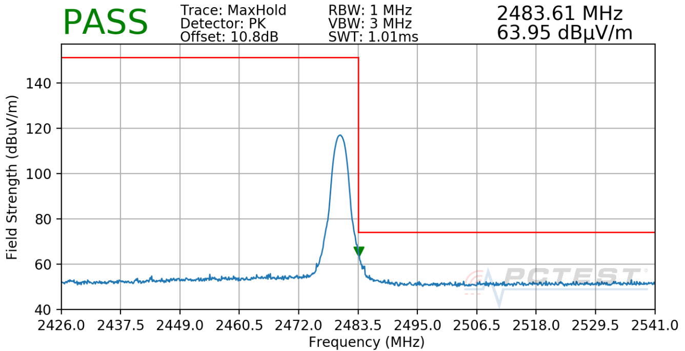
Plot 7-74. Radiated Restricted Upper Band Edge Measurement Antenna 3a (Peak)
