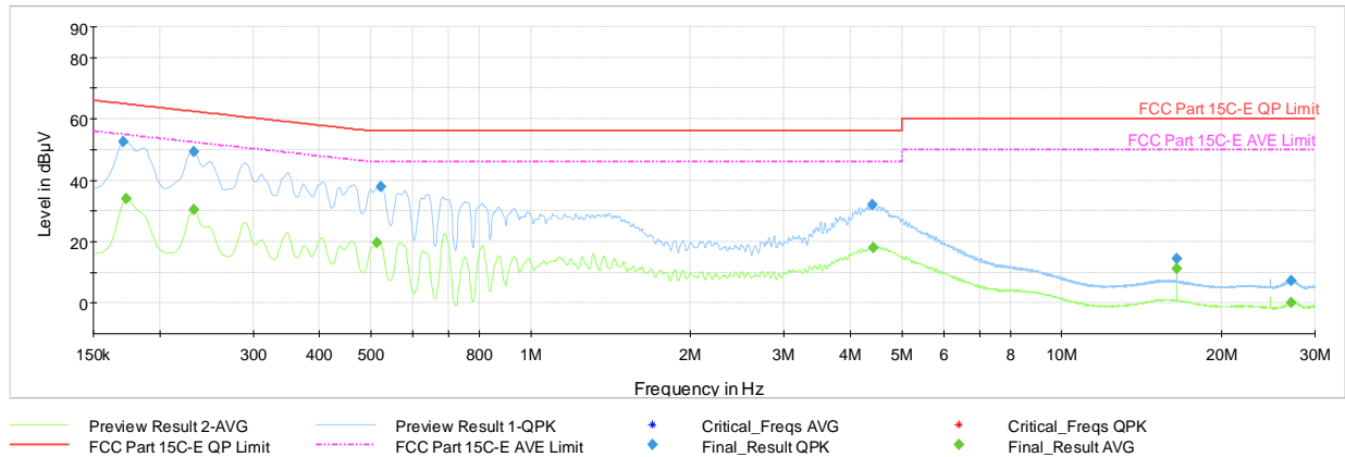
Plot 7-85. AC Line-Conducted Test Plot TxBF (L1, GFSK ePA – Ch.39, with AC/DC Adapter)
