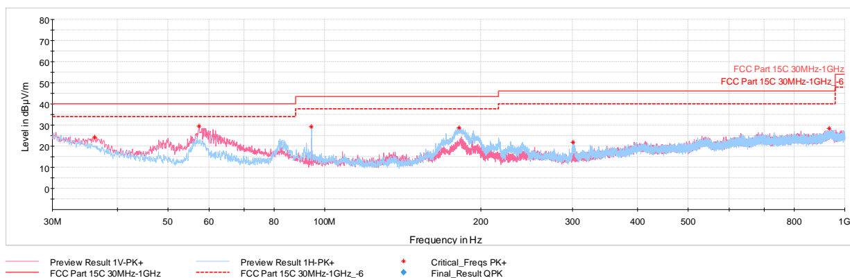
Plot 7-84. Radiated Spurious Emissions below 1GHz Simultaneous Transmission (with AC/DC Adapter)
