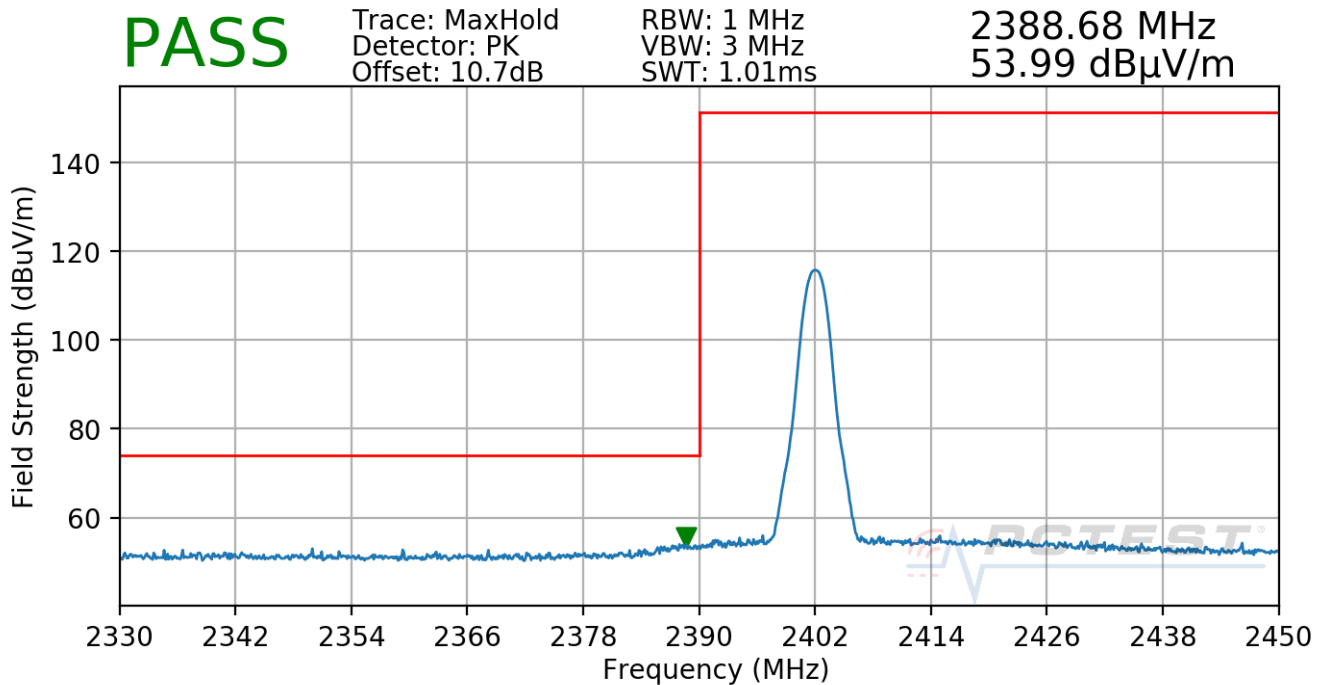
Plot 7-72. Radiated Restricted Lower Band Edge Measurement Antenna 3a (Peak)
