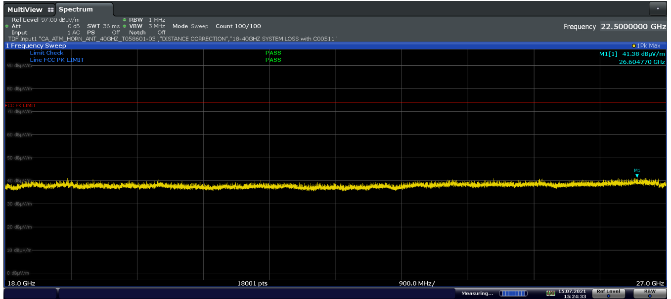
Plot 7-67. Radiated Spurious Emissions above 18GHz TxBF (GFSK ePA – Ch.39, Pol. H)
