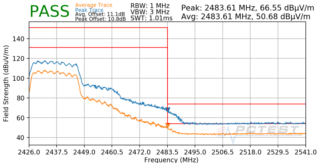
Plot 7-714. Radiated Restricted Upper Band Edge Measurement Antenna CDD
