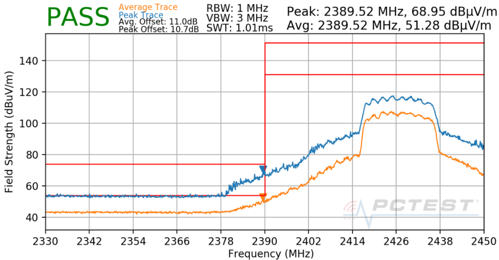
Plot 7-706. Radiated Restricted Lower Band Edge Measurement Antenna CDD
