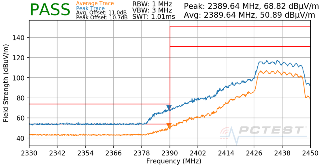
Plot 7-711. Radiated Restricted Lower Band Edge Measurement Antenna CDD
