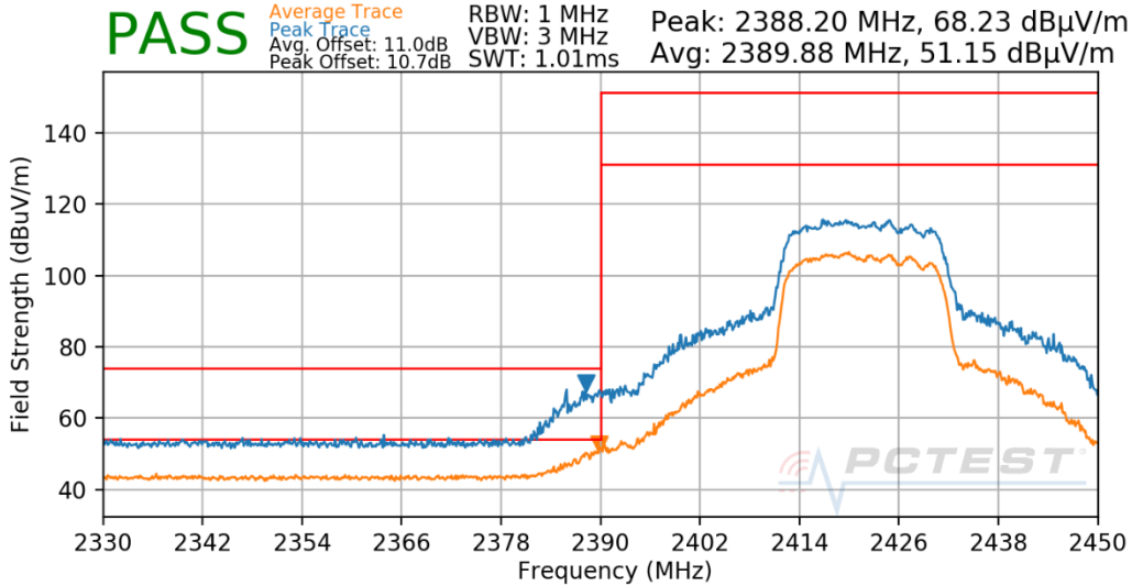
Plot 7-703. Radiated Restricted Lower Band Edge Measurement Antenna CDD
