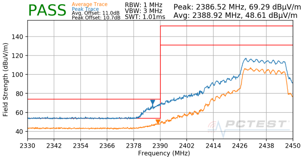
Plot 7-712. Radiated Restricted Lower Band Edge Measurement Antenna CDD
