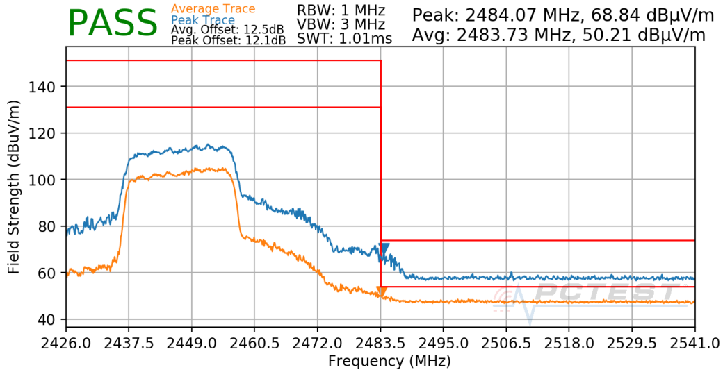
Plot 7-721. Radiated Restricted Upper Band Edge Measurement Antenna CDD
