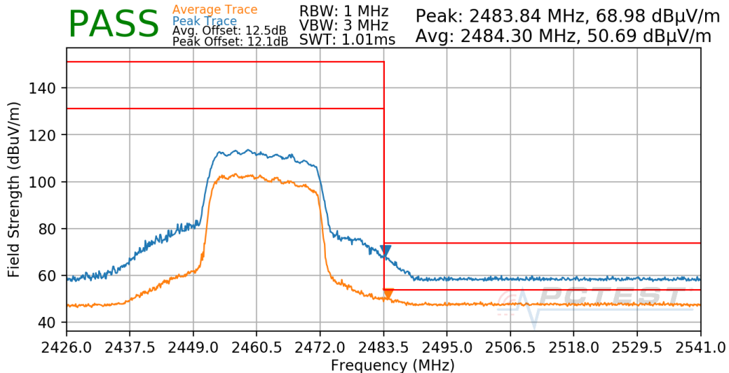
Plot 7-730. Radiated Restricted Upper Band Edge Measurement Antenna CDD
