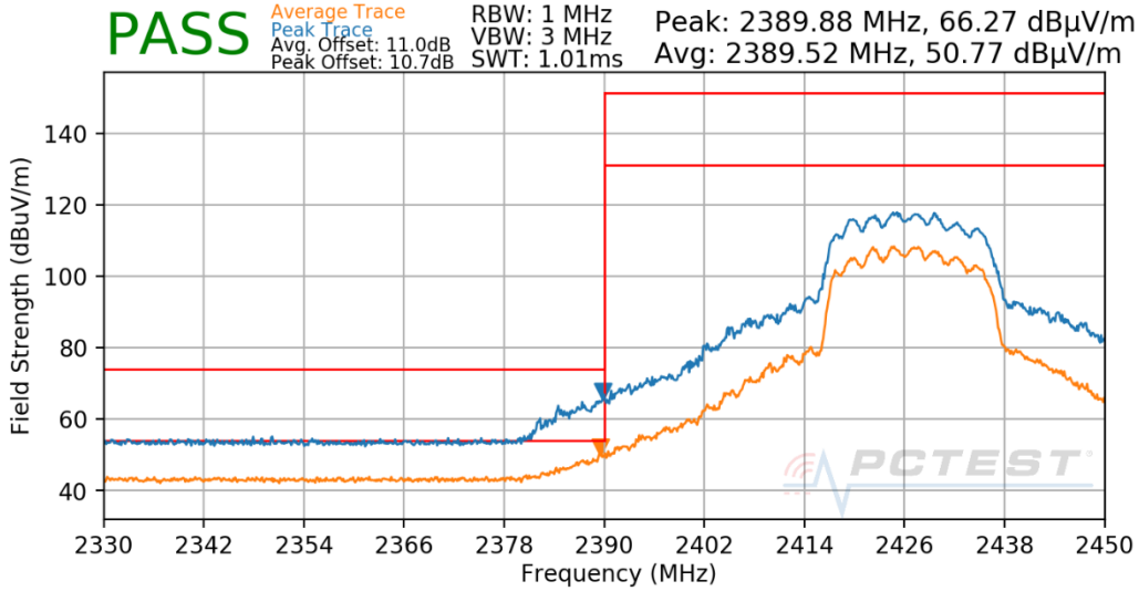
Plot 7-705. Radiated Restricted Lower Band Edge Measurement Antenna CDD
