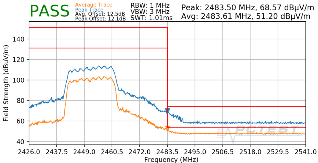
Plot 7-724. Radiated Restricted Upper Band Edge Measurement Antenna CDD
