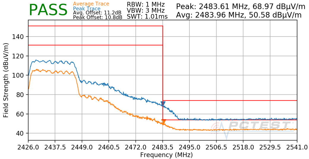
Plot 7-715. Radiated Restricted Upper Band Edge Measurement Antenna CDD
