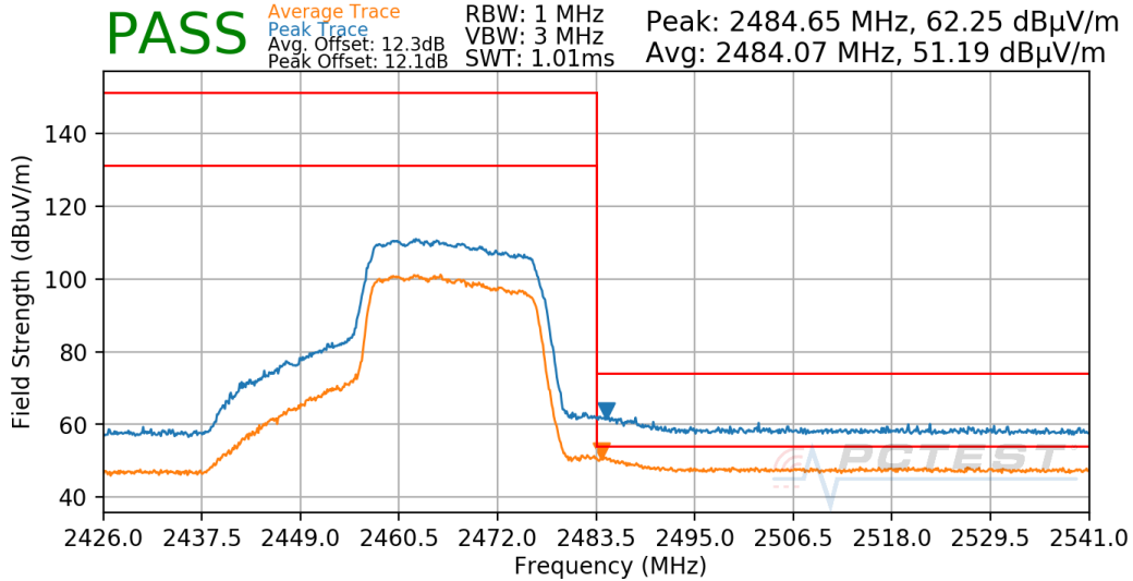
Plot 7-731. Radiated Restricted Upper Band Edge Measurement Antenna CDD
