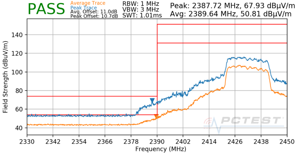
Plot 7-709. Radiated Restricted Lower Band Edge Measurement Antenna CDD
