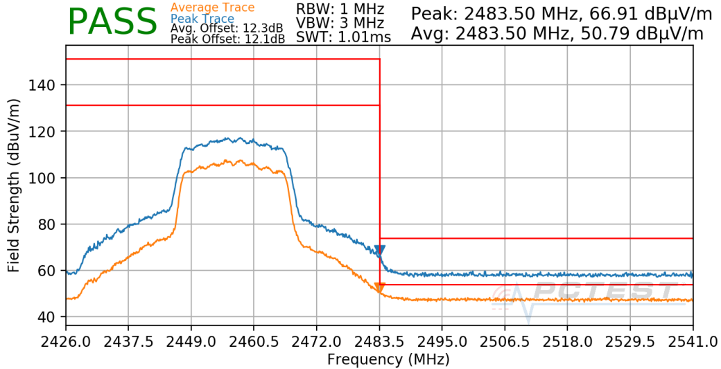
Plot 7-725. Radiated Restricted Upper Band Edge Measurement Antenna CDD
