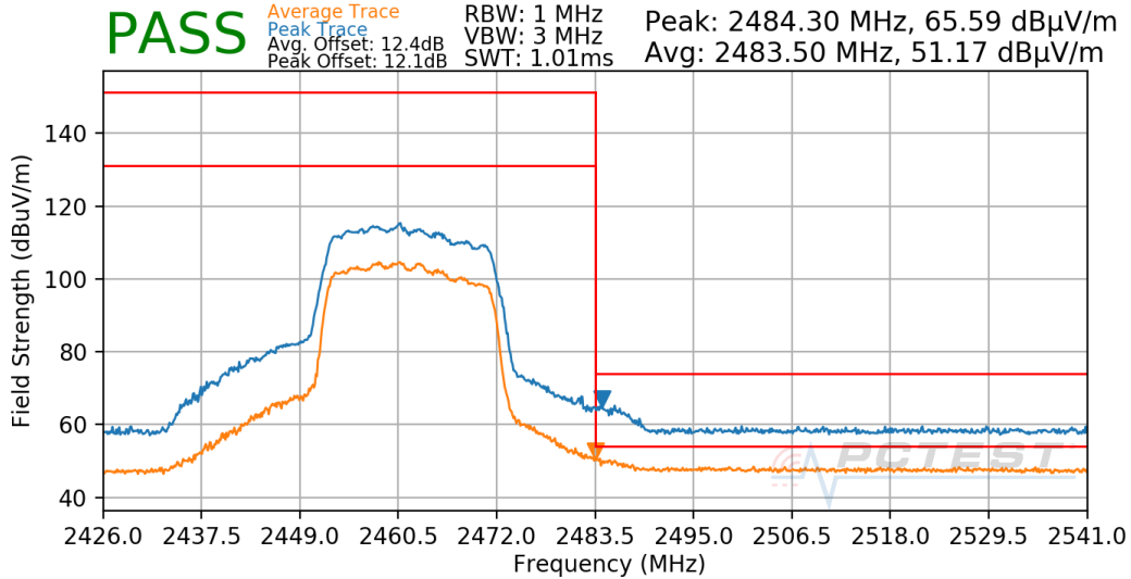
Plot 7-729. Radiated Restricted Upper Band Edge Measurement Antenna CDD
