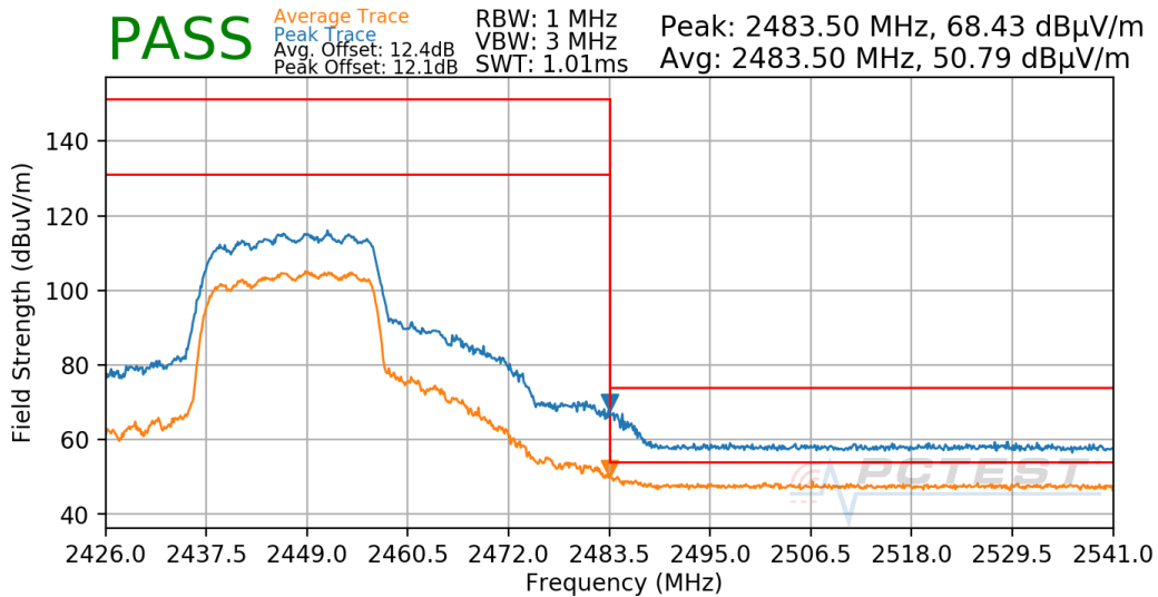
Plot 7-720. Radiated Restricted Upper Band Edge Measurement Antenna CDD
