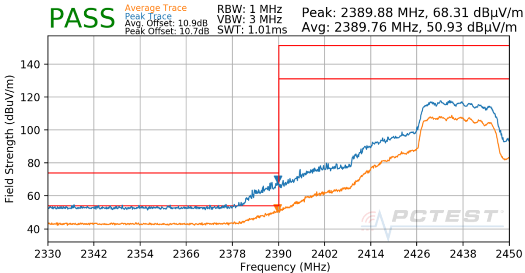
Plot 7-710. Radiated Restricted Lower Band Edge Measurement Antenna CDD
