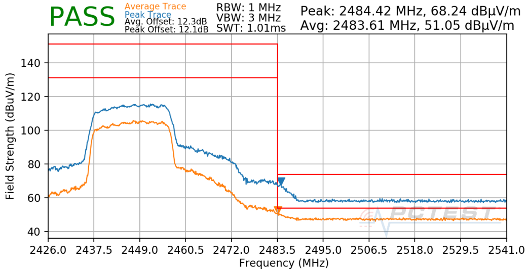
Plot 7-719. Radiated Restricted Upper Band Edge Measurement Antenna CDD
