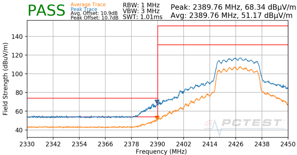
Plot 7-704. Radiated Restricted Lower Band Edge Measurement Antenna CDD
