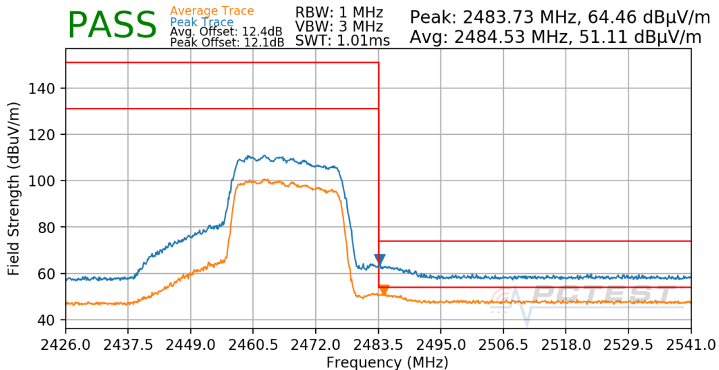
Plot 7-732. Radiated Restricted Upper Band Edge Measurement Antenna CDD
