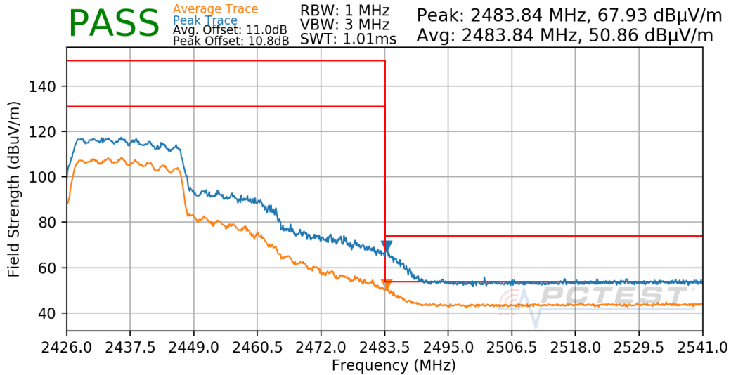
Plot 7-713. Radiated Restricted Upper Band Edge Measurement Antenna CDD
