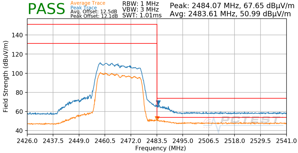
Plot 7-733. Radiated Restricted Upper Band Edge Measurement Antenna CDD
