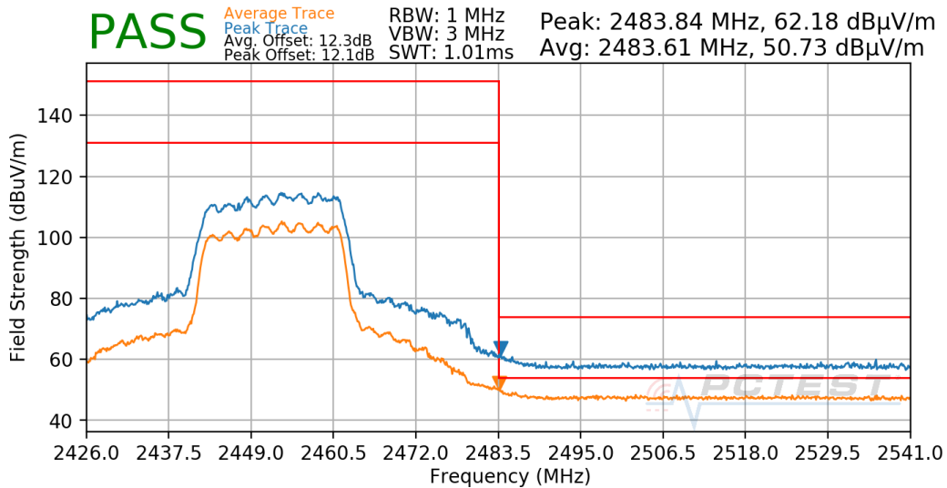
Plot 7-722. Radiated Restricted Upper Band Edge Measurement Antenna CDD
