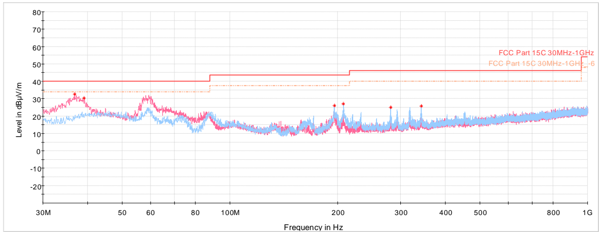
Plot 7-734. Radiated Spurious Emissions below 1GHz CDD 11n Ch.6, with AC/DC Adapter
