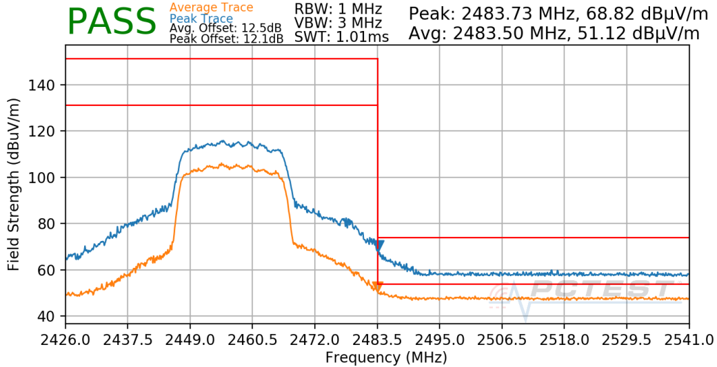
Plot 7-727. Radiated Restricted Upper Band Edge Measurement Antenna CDD
