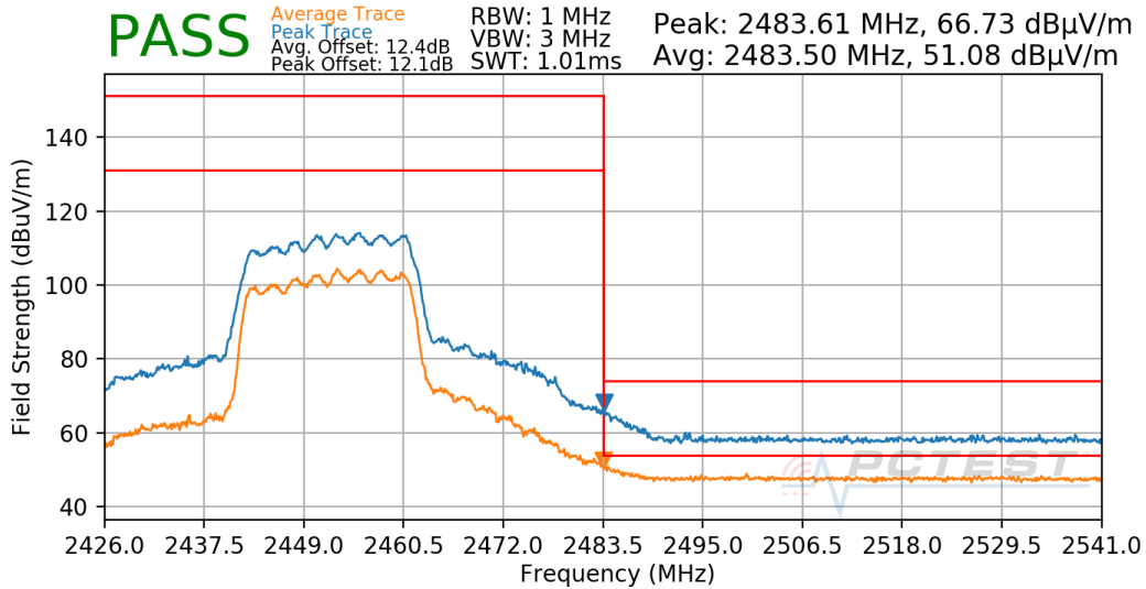
Plot 7-723. Radiated Restricted Upper Band Edge Measurement Antenna CDD
