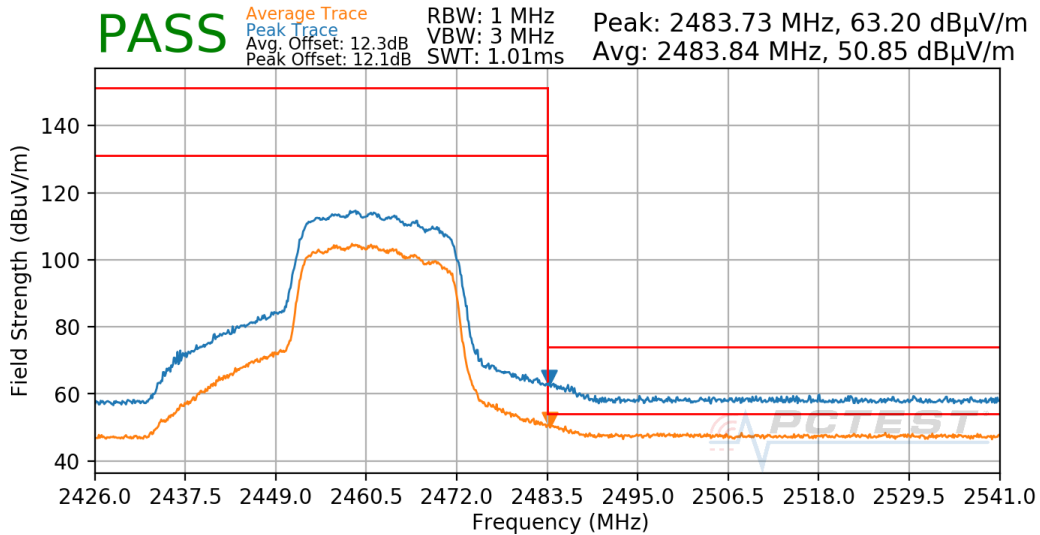
Plot 7-728. Radiated Restricted Upper Band Edge Measurement Antenna CDD
