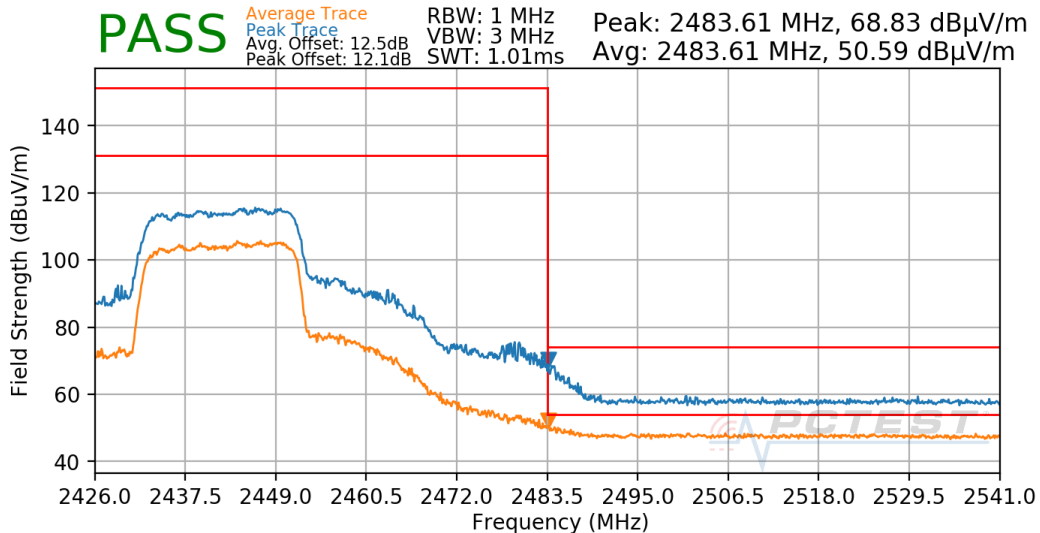
Plot 7-718. Radiated Restricted Upper Band Edge Measurement Antenna CDD
