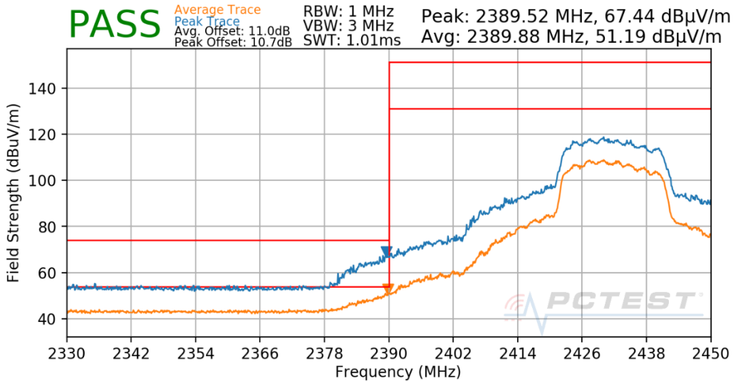
Plot 7-708. Radiated Restricted Lower Band Edge Measurement Antenna CDD
