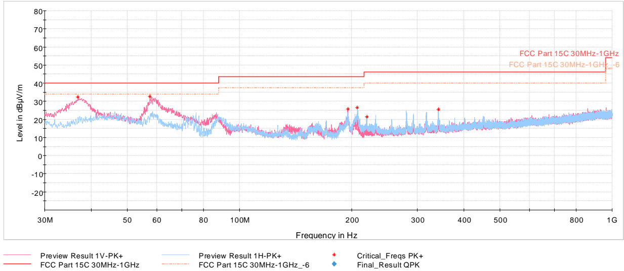
Plot 7-735. Radiated Spurious Emissions below 1GHz CDD 11ax - SU Ch.6, with AC/DC Adapter
