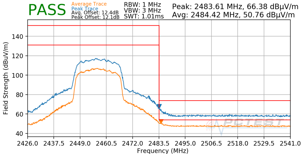
Plot 7-726. Radiated Restricted Upper Band Edge Measurement Antenna CDD
