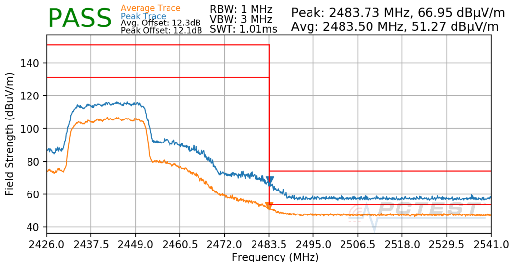
Plot 7-716. Radiated Restricted Upper Band Edge Measurement Antenna CDD
