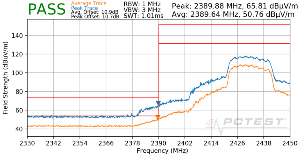
Plot 7-707. Radiated Restricted Lower Band Edge Measurement Antenna CDD
