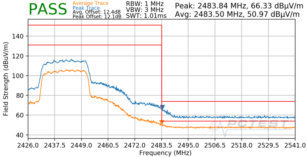
Plot 7-717. Radiated Restricted Upper Band Edge Measurement Antenna CDD
