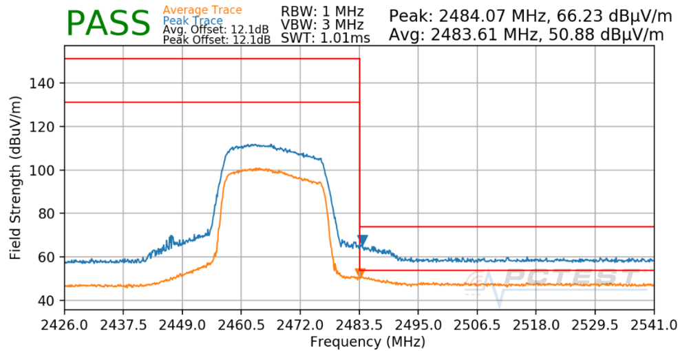
Plot 7-178. Radiated Restricted Upper Band Edge Measurement Antenna 1a (Peak & Average – RU242)
