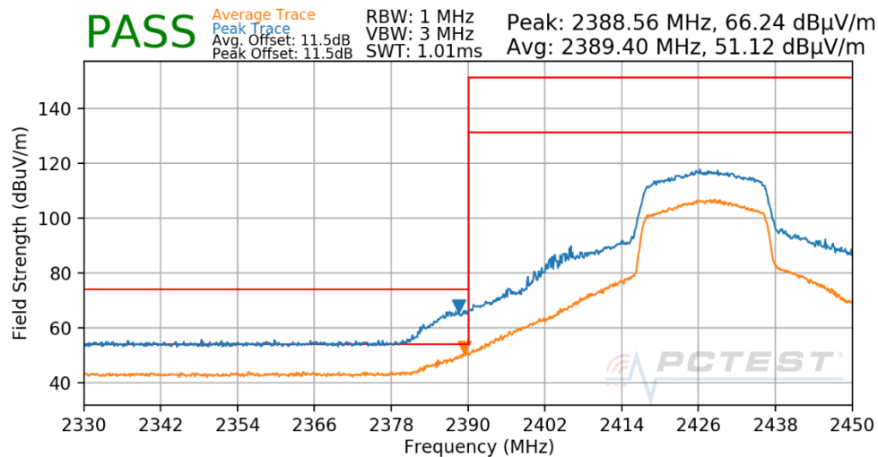
Plot 7-169. Radiated Restricted Lower Band Edge Measurement Antenna 1a (Peak & Average – RU242)
