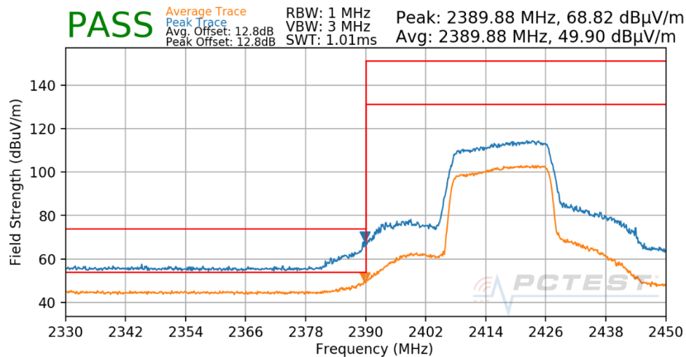
Plot 7-167. Radiated Restricted Lower Band Edge Measurement Antenna 1a (Peak & Average – RU242)
