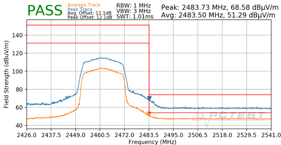
Plot 7-177. Radiated Restricted Upper Band Edge Measurement Antenna 1a (Peak & Average – RU242)
