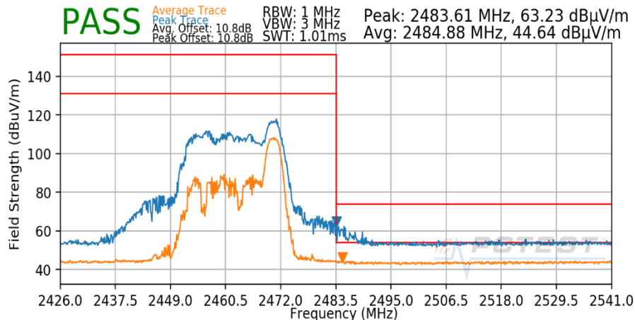
Plot 7-180. Radiated Restricted Upper Band Edge Measurement CDD (Peak & Average – RU26)
