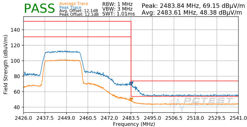
Plot 7-174. Radiated Restricted Upper Band Edge Measurement Antenna 1a (Peak & Average – RU242)
