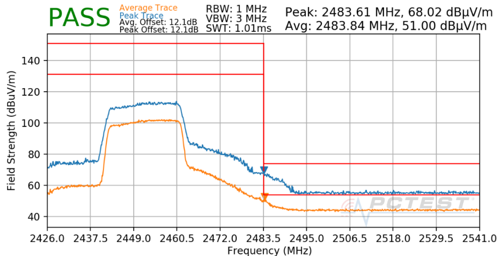
Plot 7-175. Radiated Restricted Upper Band Edge Measurement Antenna 1a (Peak & Average – RU242)
