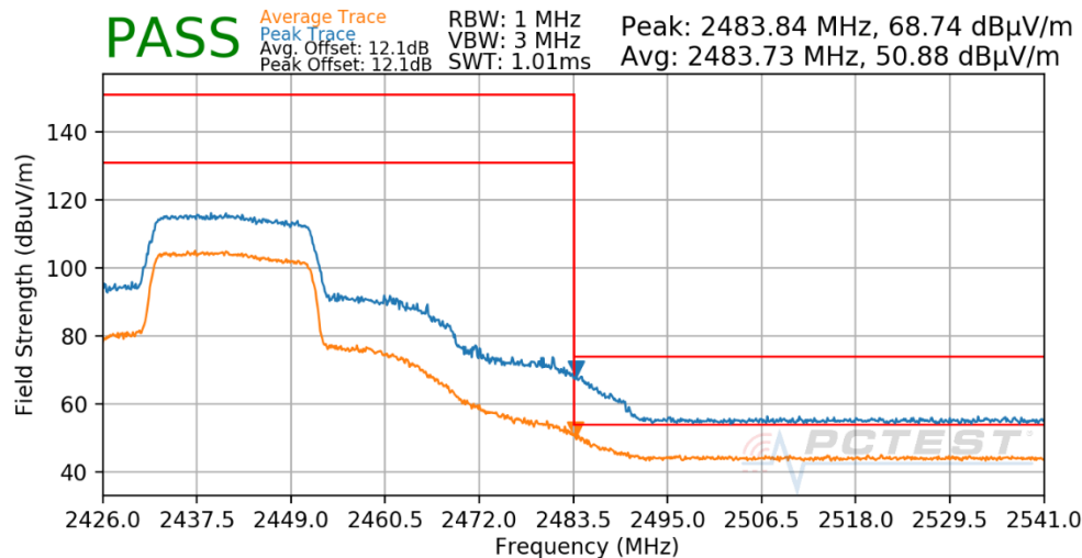
Plot 7-173. Radiated Restricted Upper Band Edge Measurement Antenna 1a (Peak & Average – RU242)
