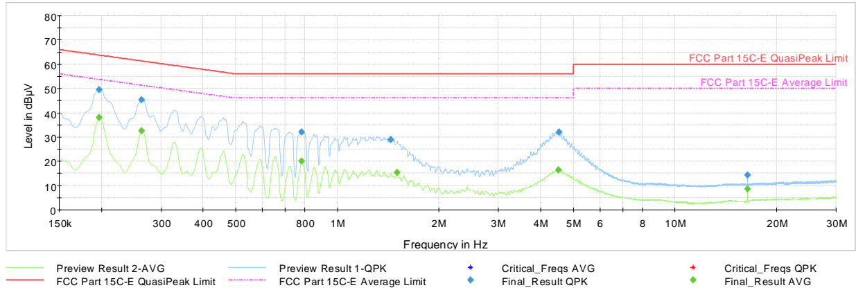
Plot 7-197. AC Line Conducted Emissions with 802.11ax CDD (RU26) Ch.6 (L1, with Adapter)
