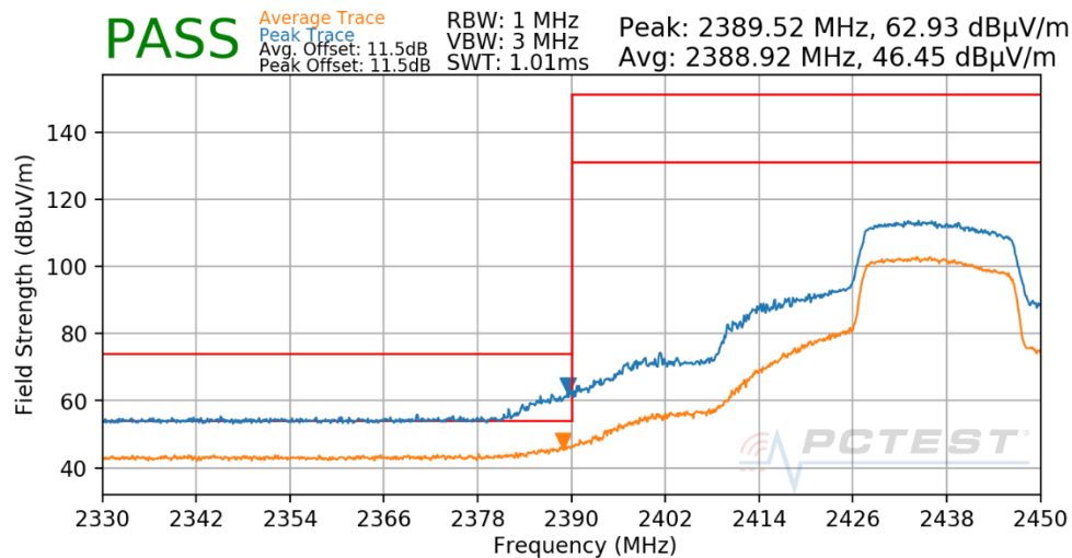
Plot 7-171. Radiated Restricted Lower Band Edge Measurement Antenna 1a (Peak & Average – RU242)
