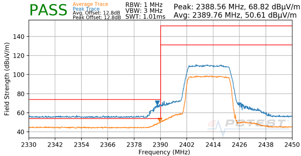
Plot 7-166. Radiated Restricted Lower Band Edge Measurement Antenna 1a (Peak & Average – RU242)
