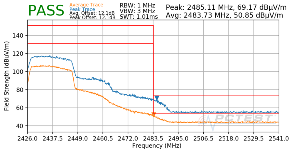
Plot 7-172. Radiated Restricted Upper Band Edge Measurement Antenna 1a (Peak & Average – RU242)
