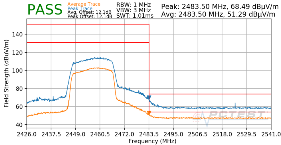
Plot 7-176. Radiated Restricted Upper Band Edge Measurement Antenna 1a (Peak & Average – RU242)
