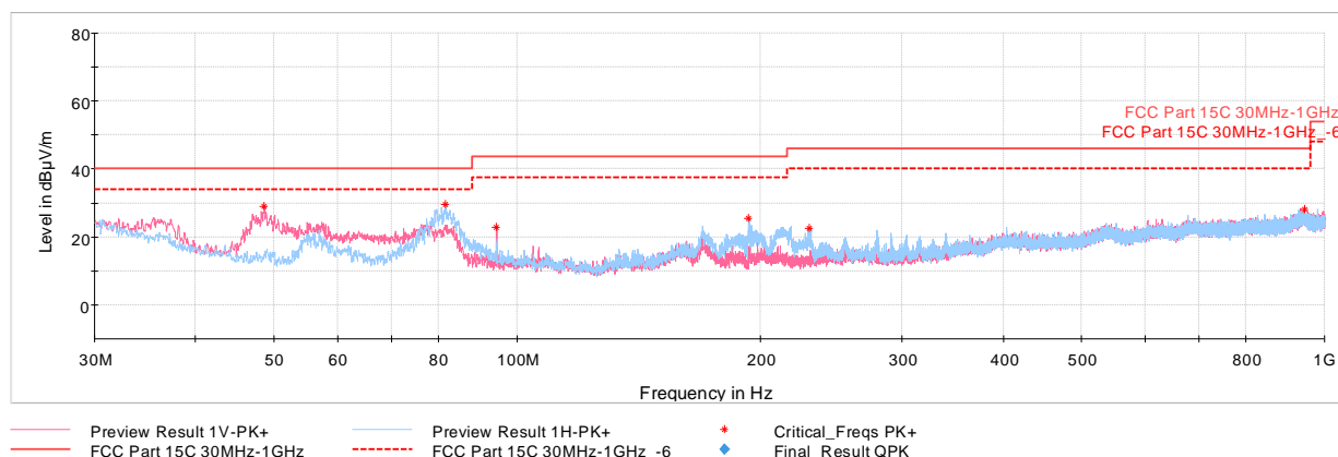
Plot 7-196. Radiated Spurious Emissions below 1GHz CDD Ch.6 (RU242), with AC/DC Adapter
