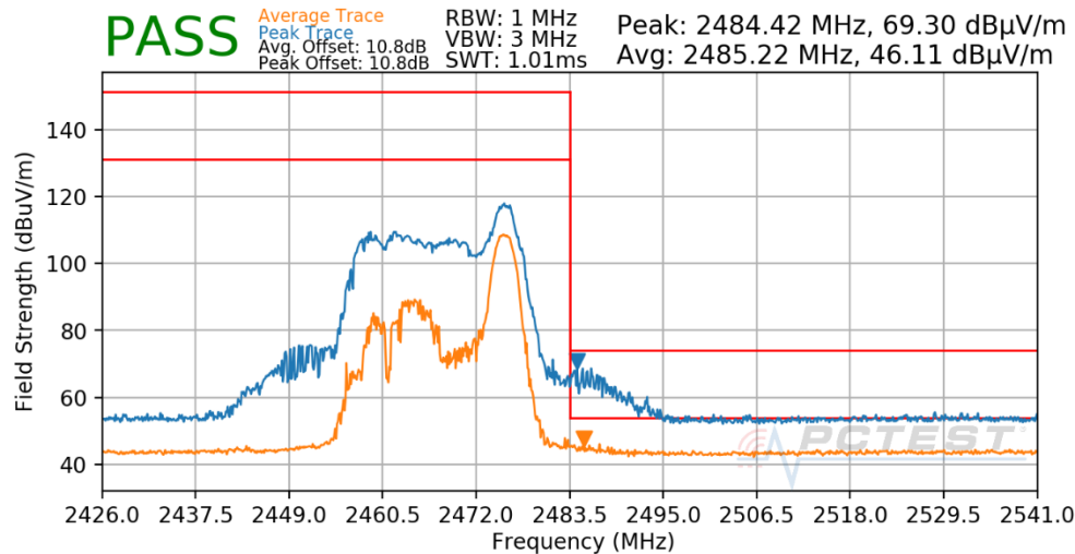
Plot 7-181. Radiated Restricted Upper Band Edge Measurement CDD (Peak & Average – RU26)
