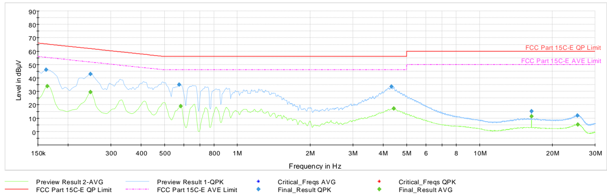
Plot 7-199. AC Line Conducted Emissions with 802.11ax CDD (RU242) Ch.6 (L1, with Adapter)
