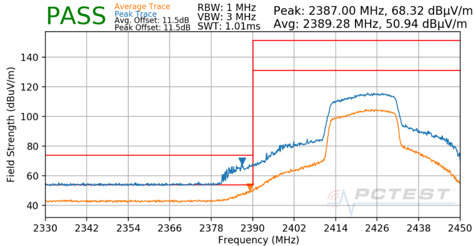
Plot 7-168. Radiated Restricted Lower Band Edge Measurement Antenna 1a (Peak & Average – RU242)
