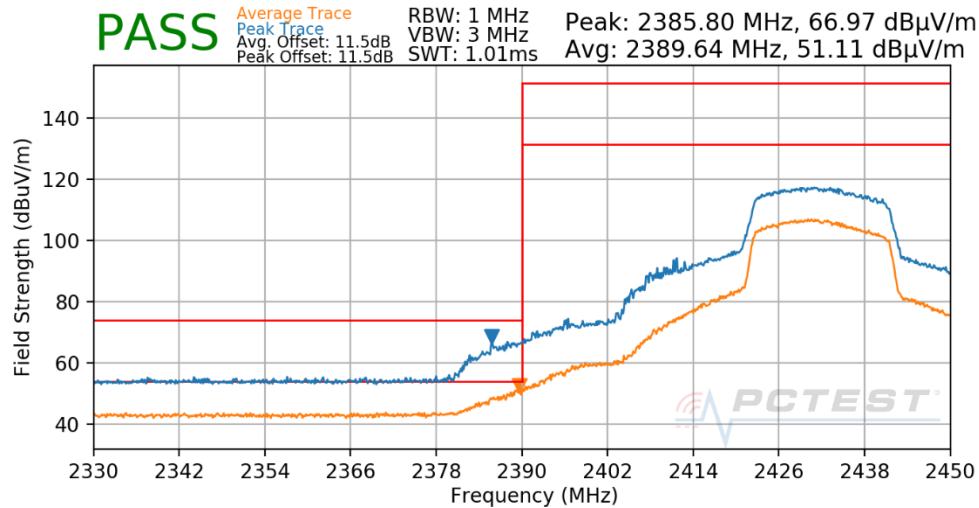
Plot 7-170. Radiated Restricted Lower Band Edge Measurement Antenna 1a (Peak & Average – RU242)
