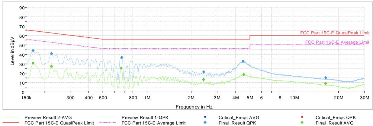
Plot 7-198. AC Line Conducted Emissions with 802.11ax CDD (RU26) Ch.6 (N, with Adapter)
