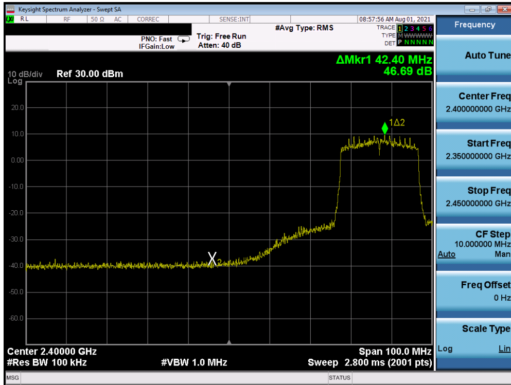
Plot 7-81. Band Edge Antenna 3a (802.11ax OFDMA – RU242 – Ch. 6)
