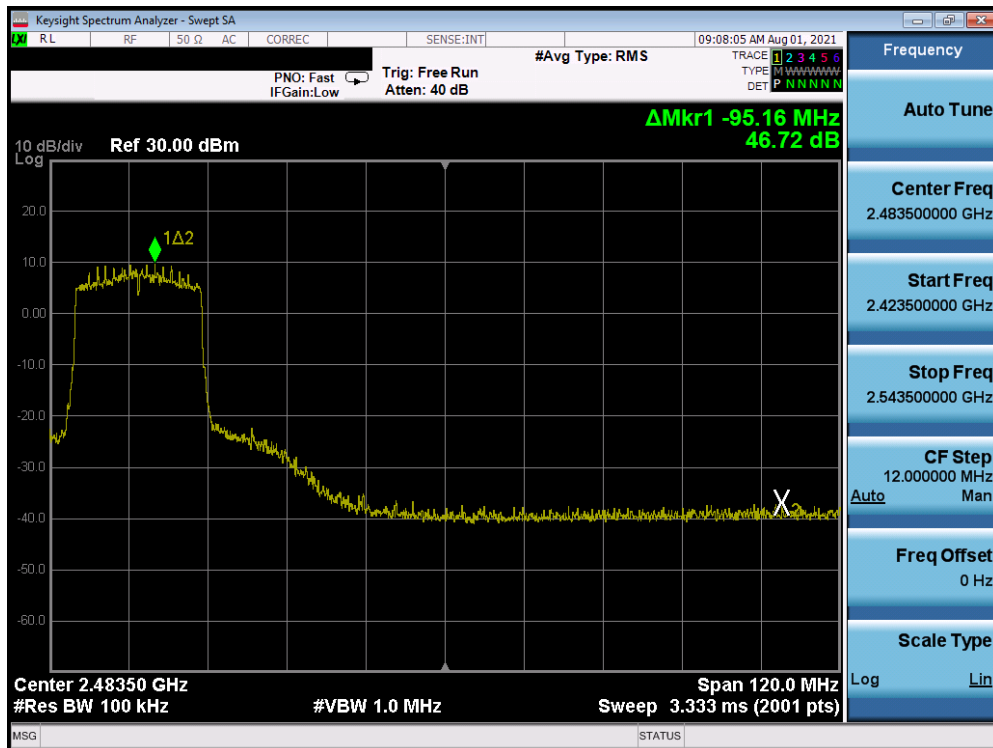
Plot 7-82. Band Edge Antenna 3a (802.11ax OFDMA – RU242 – Ch. 6)
