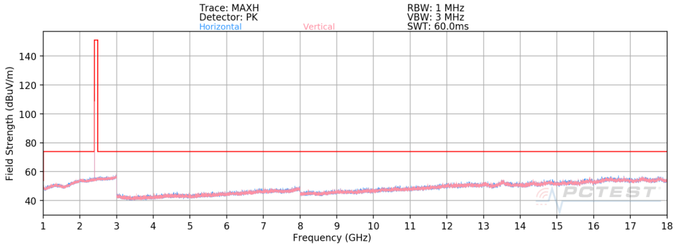
Plot 7-84. Radiated Spurious Emissions Above 1GHz Antenna 1a (1Mbps, ePA – Ch. 0)
