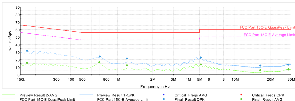
Plot 7-106. AC Line Conducted Plot with Bluetooth LE Tx BF (1Mbps, ePA – Ch.19, N, with AC/DC Adapter)
