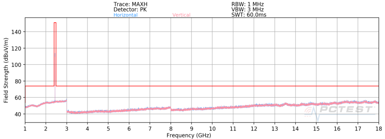
Plot 7-82. Radiated Spurious Emissions Above 1GHz Antenna 3a (1Mbps, ePA – Ch. 19)
