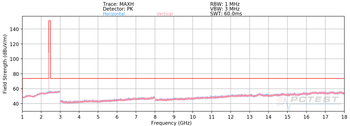
Plot 7-81. Radiated Spurious Emissions Above 1GHz Antenna 3a (1Mbps, ePA – Ch. 0)
