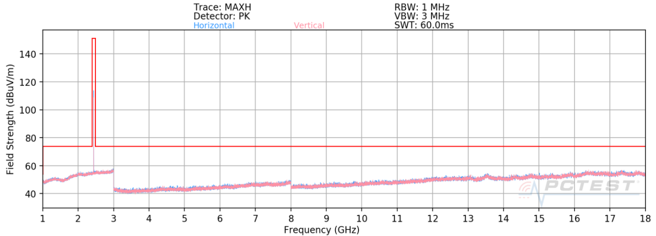
Plot 7-85. Radiated Spurious Emissions Above 1GHz Antenna 1a (1Mbps, ePA – Ch. 19)
