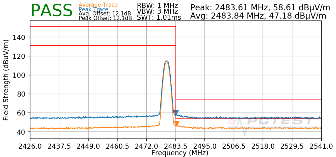
Plot 7-101. Radiated Restricted Upper Band Edge Measurement TxBF (Average & Peak)
