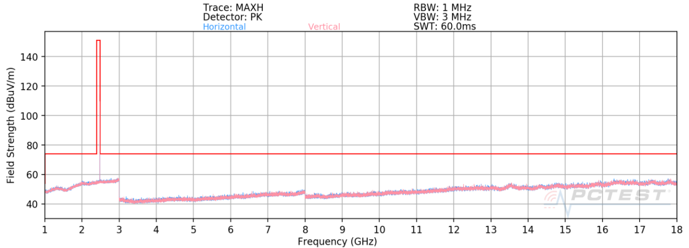
Plot 7-86. Radiated Spurious Emissions Above 1GHz Antenna 1a (1Mbps, ePA – Ch. 39)
