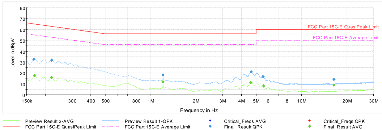
Plot 7-105. AC Line Conducted Plot with Bluetooth LE Tx BF (1Mbps, ePA – Ch.0, L1, with AC/DC Adapter)
