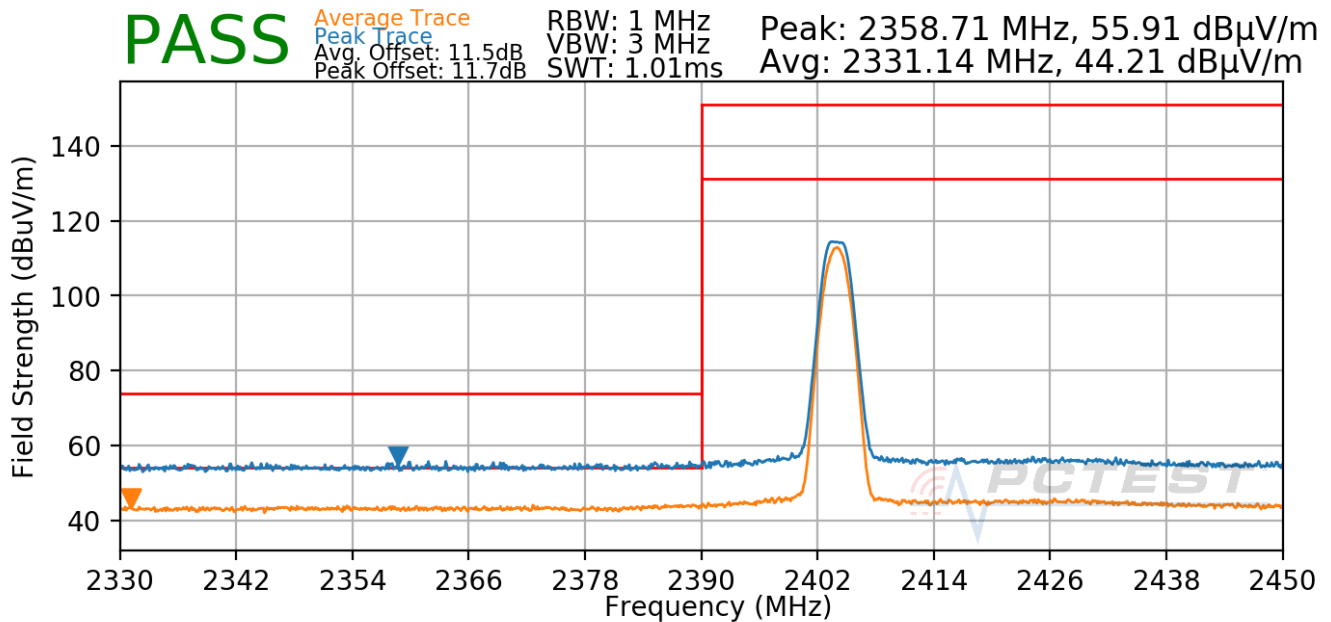
Plot 7-98. Radiated Restricted Lower Band Edge Measurement Antenna 1a (Average & Peak)
