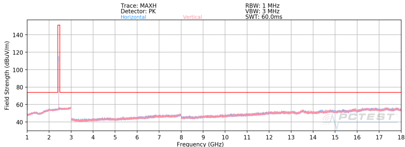
Plot 7-90. Radiated Spurious Emissions Above 1GHz TxBF (1Mbps, ePA – Ch. 19)
