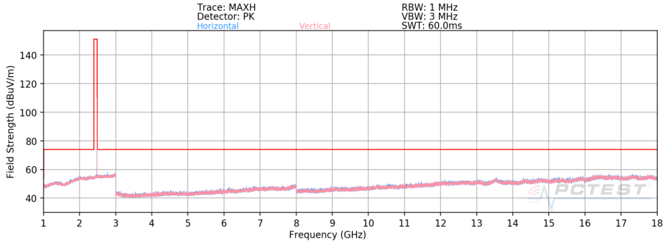
Plot 7-83. Radiated Spurious Emissions Above 1GHz Antenna 3a (1Mbps, ePA – Ch. 39)
