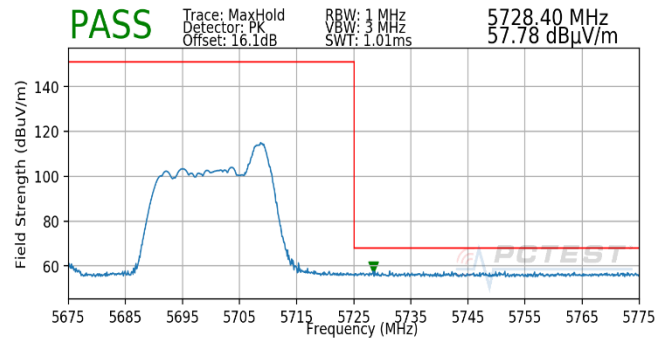
Plot 7-819. Antenna 1b (Pk, RU26, Index 8, Ch.140, MCS11)
